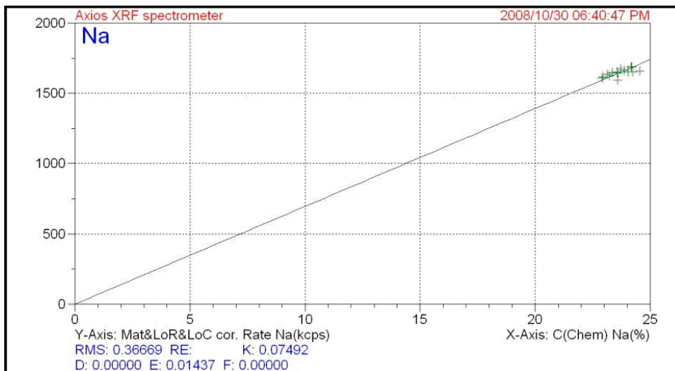
Figure 7-7: WDXRF Sodium calibration graph with FP corrections
