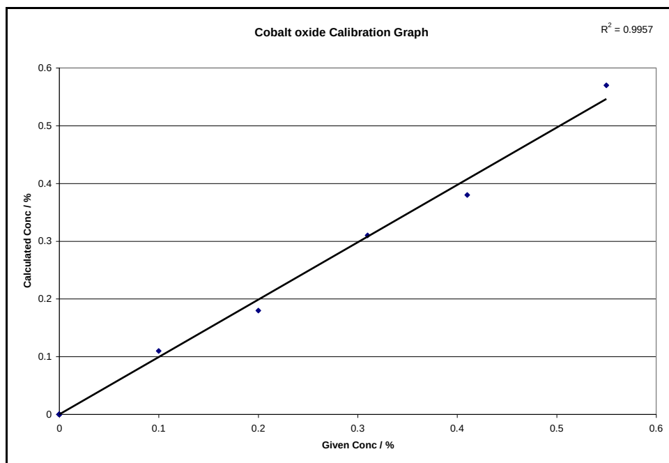
Figure C-0-2: Cobalt oxide calibration graph with sodium iodide as non-wetting agent ad FP corrections
