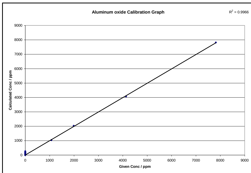
Figure D-0-2: Aluminum oxide calibration graph with potassium iodide as non-wetting agent and empirical corrections
