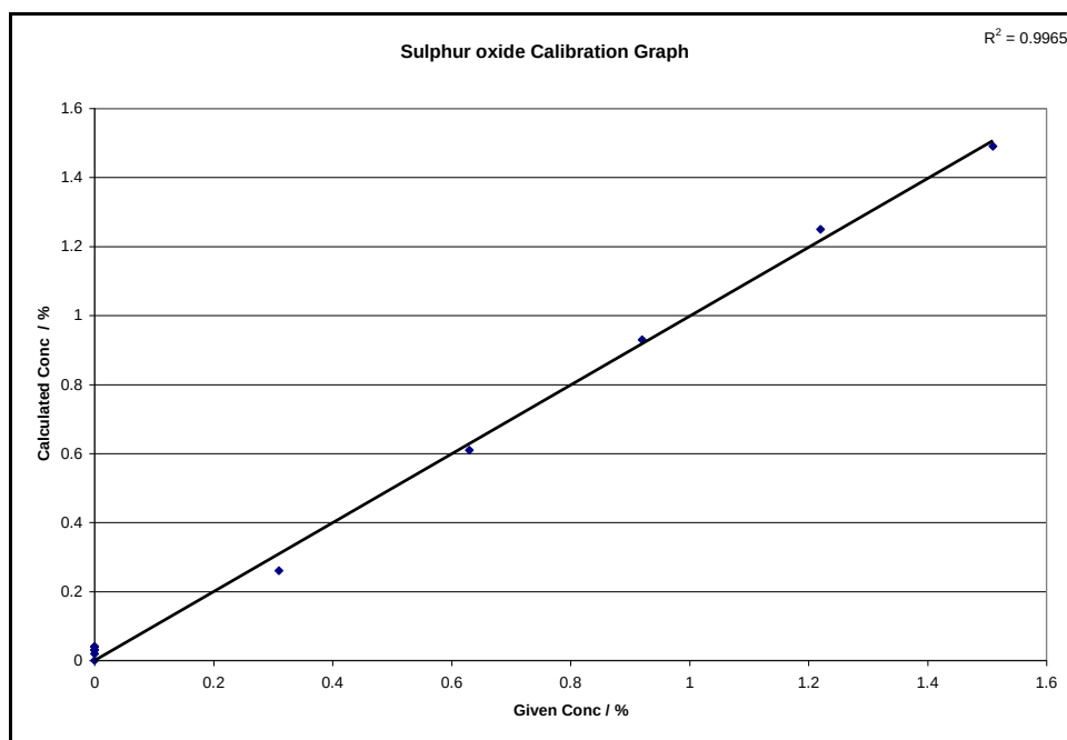
Figure C-0-6: Sulphur oxide calibration graph with sodium iodide as non-wetting agent and FP correction
