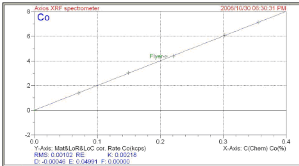
Figure F-0-14: Cobalt calibration graph on WDXRF with FP corrections
