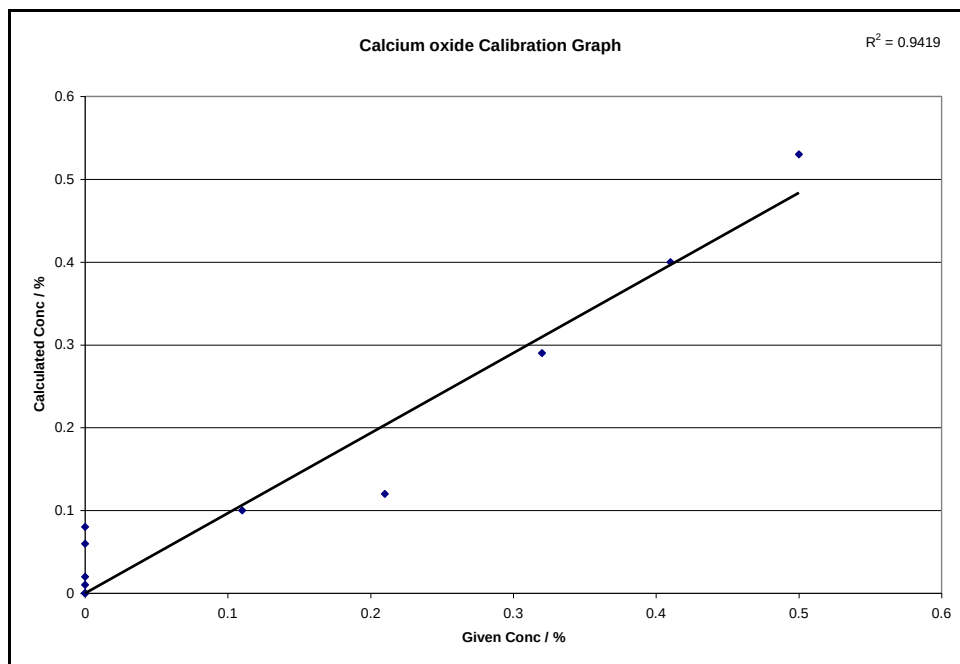
Figure C-0-5: Calcium oxide calibration graph with sodium iodide as non-wetting agent and FP corrections
