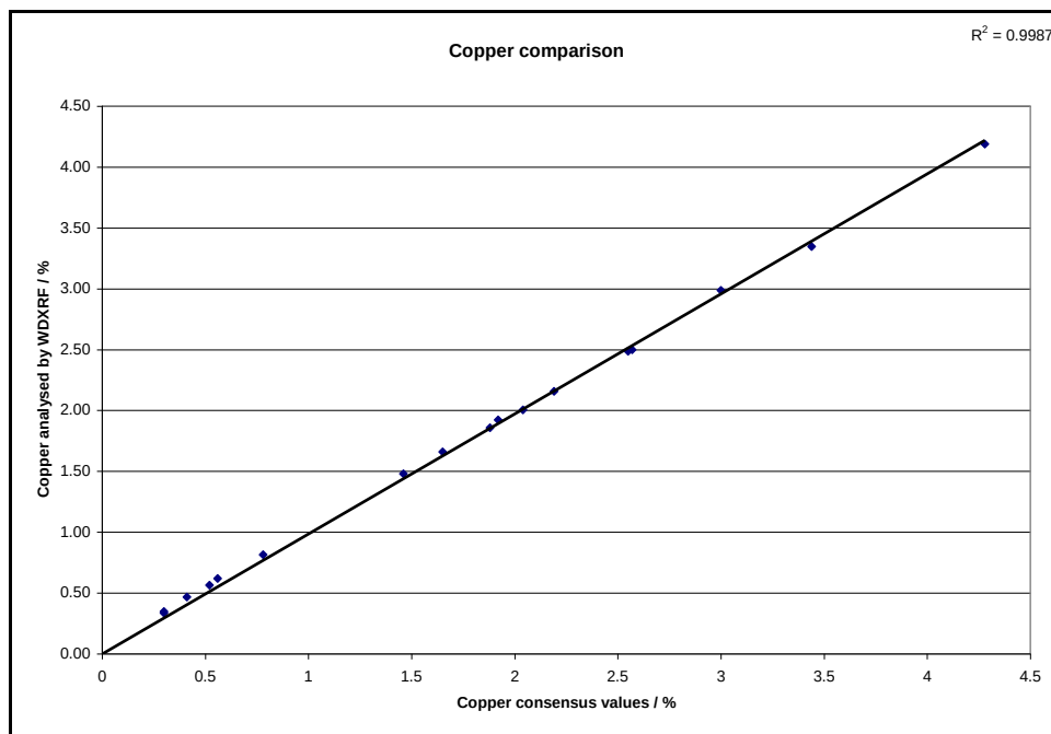
Figure 8-1: Comparison of consensus values and measured values for copper
