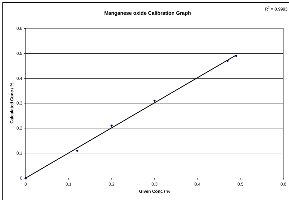
Figure C-0-19: Manganese oxide calibration graph with bromine gas as non-wetting agent
