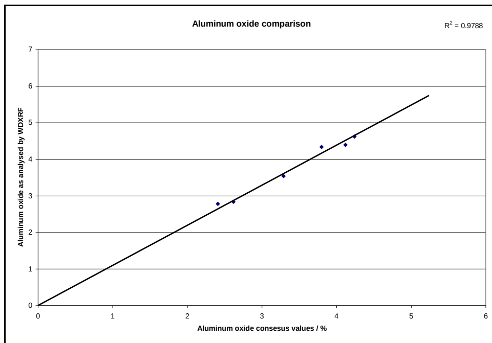
Figure 8-6: Comparison of consensus values and measured values for aluminum oxide
