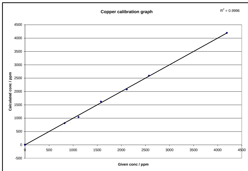
Figure 5-7: Copper calibration graph with empirical corrections applied
