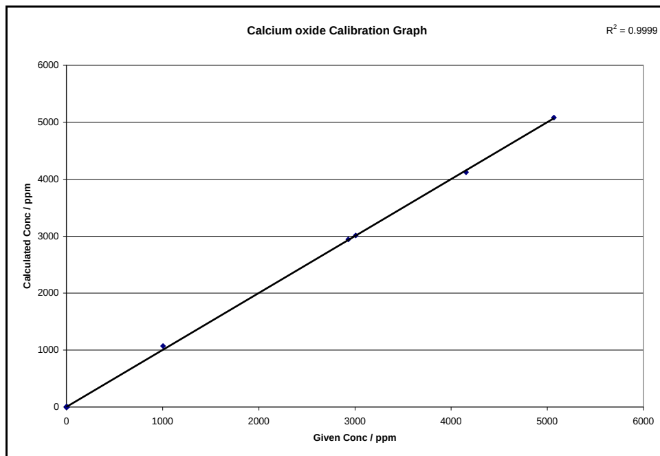
Figure D-0-4: Calcium oxide calibration graph with potassium iodide as non-wetting agent and empirical corrections
