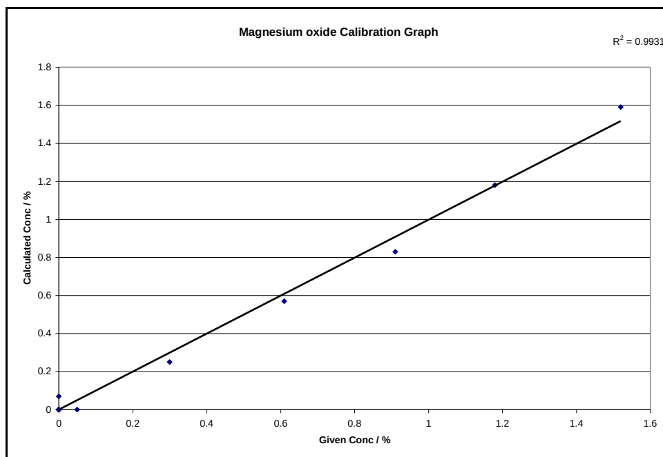
Figure C-0-12: Magnesium oxide calibration graph with bromine gas as non-wetting agent
