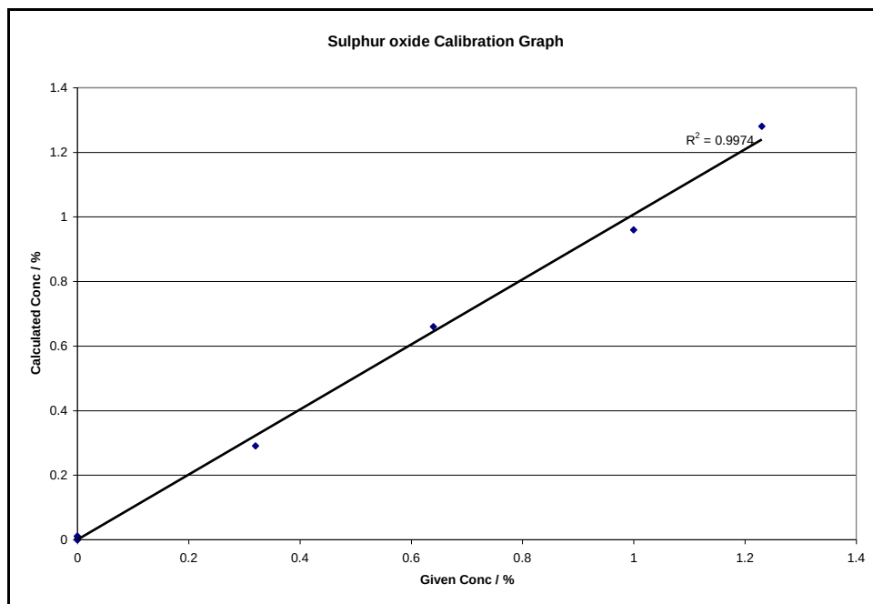
Figure C-0-15: Sulphur oxide calibration graph with bromine gas as non-wetting agent
