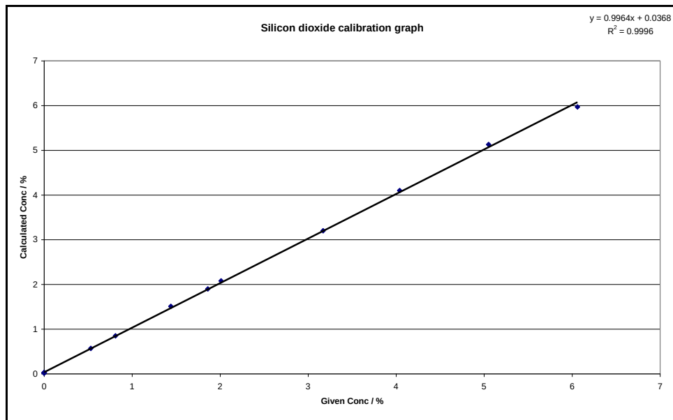
Figure F-0-3: Silicon dioxide calibration graph on EDXRF with FP corrections
