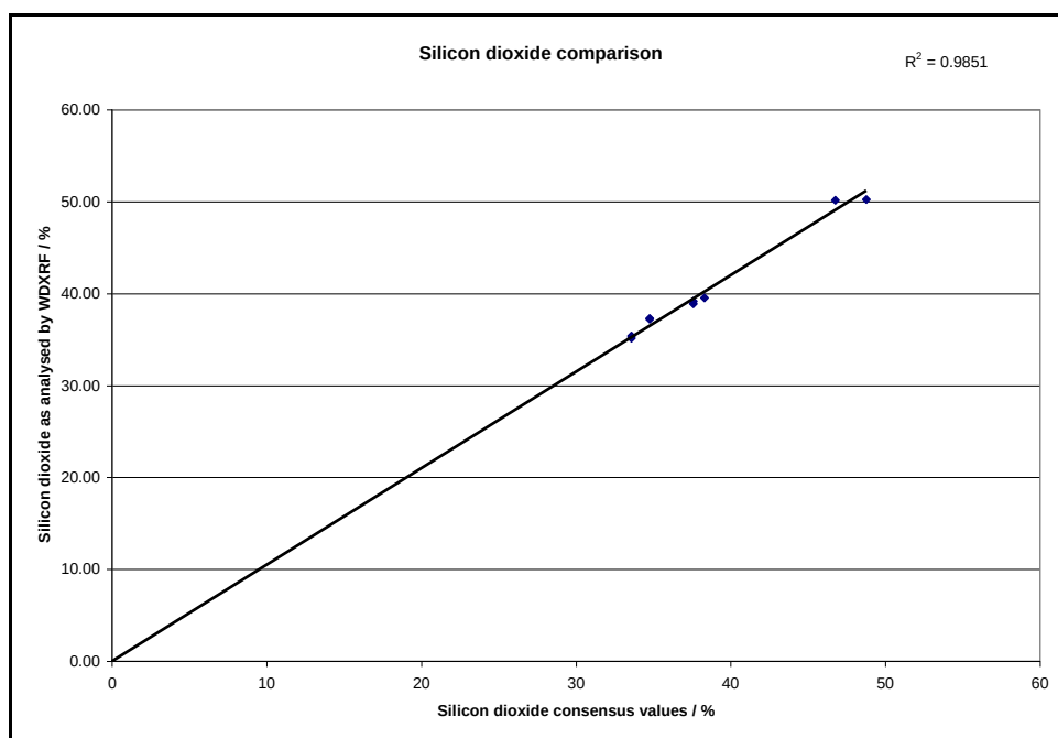
Figure 8-10: Comparison of consensus values and XRF values for silicon dioxide
