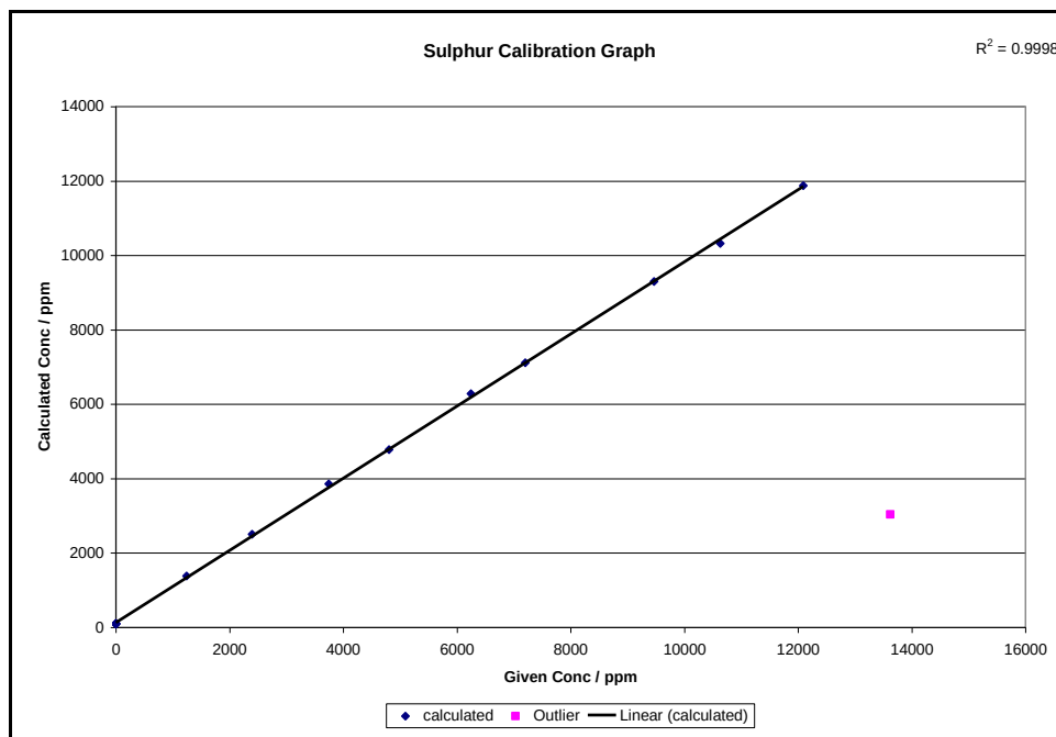
Figure 5-9: Sulphur calibration graph with outlier and empirical correction applied
