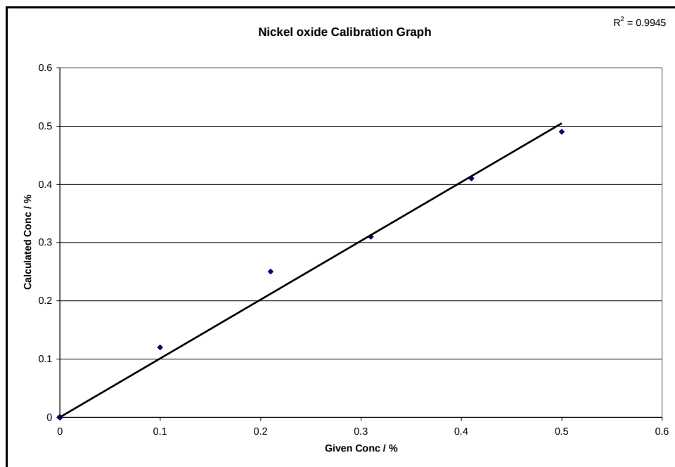
Figure C-0-1: Nickel oxide calibration graph with sodium iodide as non-wetting agent and FP corrections
