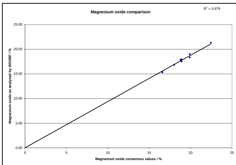
Figure 8-8: Comparison of consensus values and XRF values for magnesium oxide
