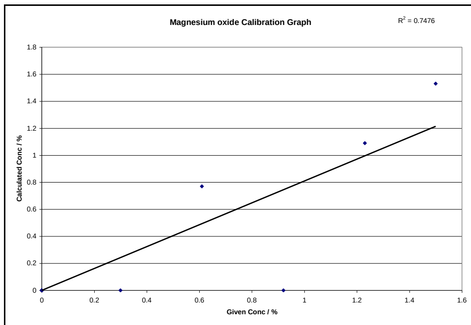
Figure C-0-9: Magnesium oxide with sodium iodide as non-wetting agent and FP corrections
