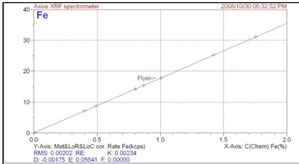
Figure F-0-13: Iron calibration graph on WDXRF with FP corrections
