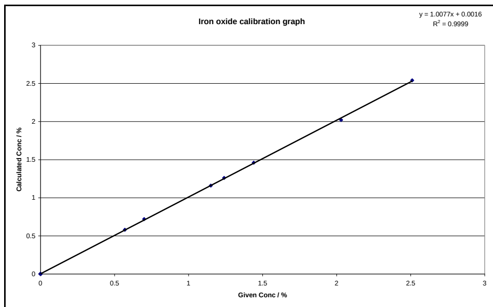
Figure F-0-6: Iron oxide calibration graph on EDXRF with FP corrections
