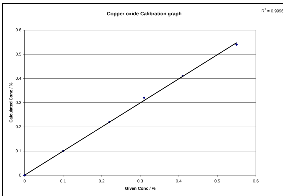
Figure 4-2: Copper oxide calibration graph with bromine gas as non-wetting agent
