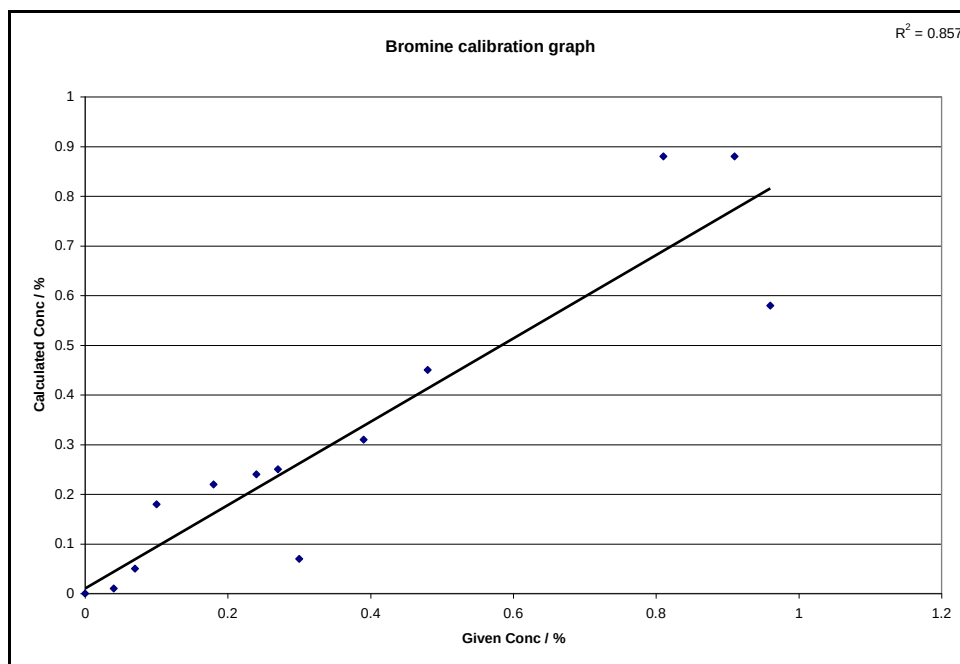
Figure 4-3: Bromine calibration graph with bromine as non-wetting agent
