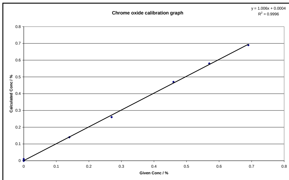
Figure F-0-5: Chromic oxide calibration graph on EDXRF with FP corrections
