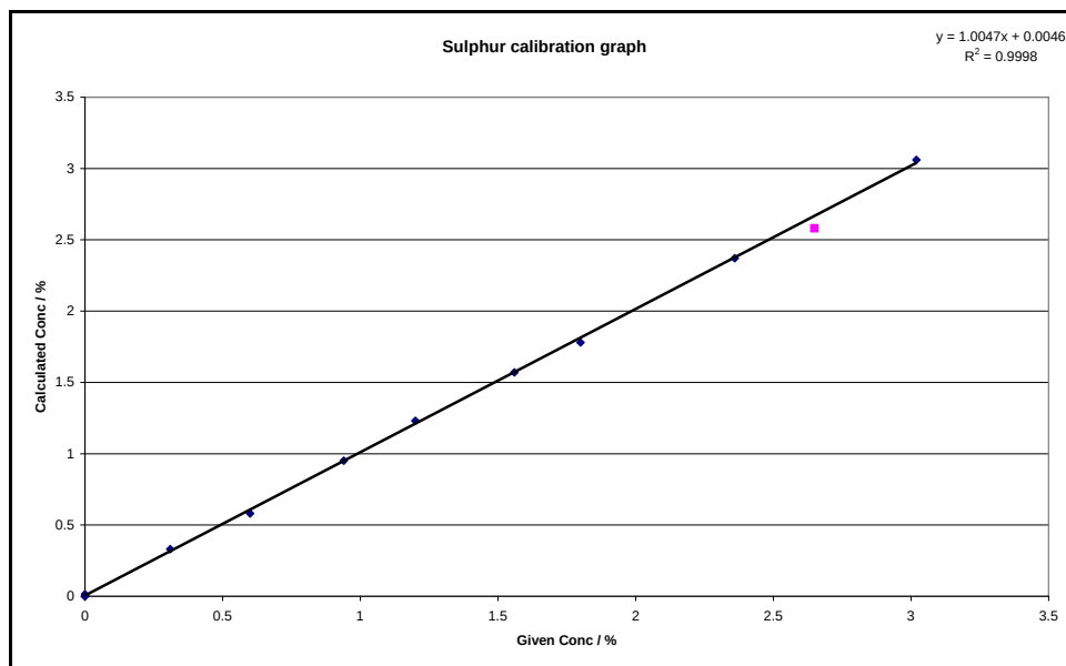
Figure 7-2: EDXRF Sulphur calibration graph with FP corrections
