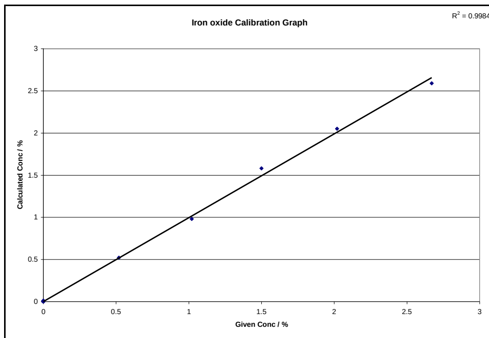
Figure C-0-20: Iron oxide calibration graph with bromine gas as non-wetting agent
