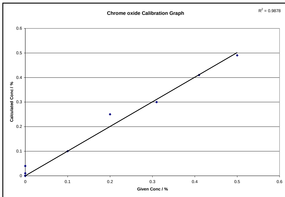
Figure C-0-4: Chromic oxide calibration graph with sodium iodide as non-wetting agent and FP corrections
