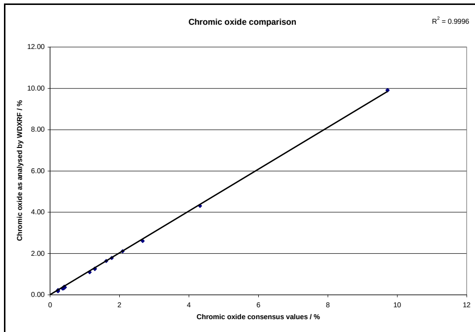
Figure 8-9: Comparison of consensus values and XRF values for chromic oxide
