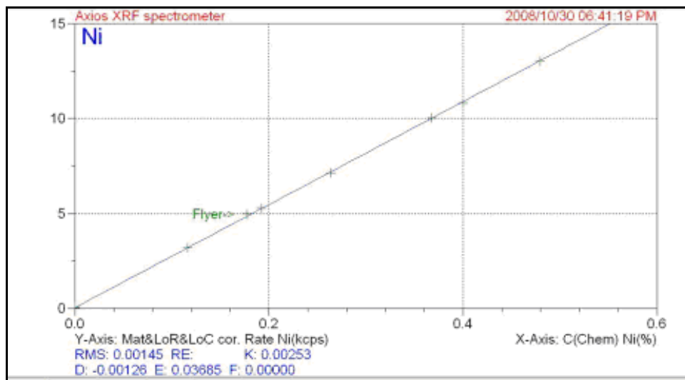
Figure F-0-15: Nickel calibration graph on WDXRF with FP corrections
