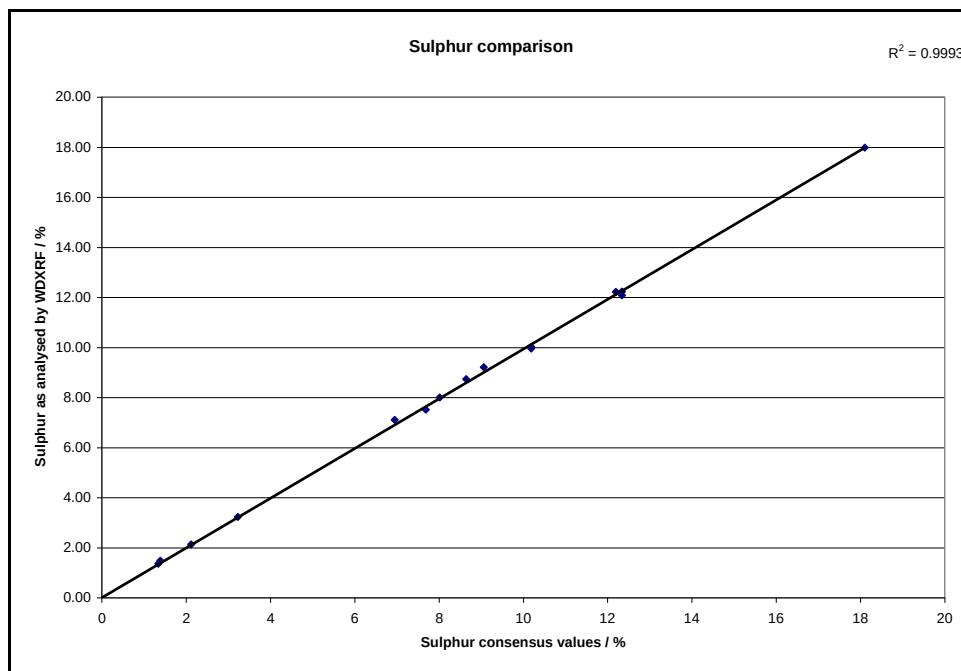
Figure 8-3: Comparison of consensus values and measured values for sulphur
