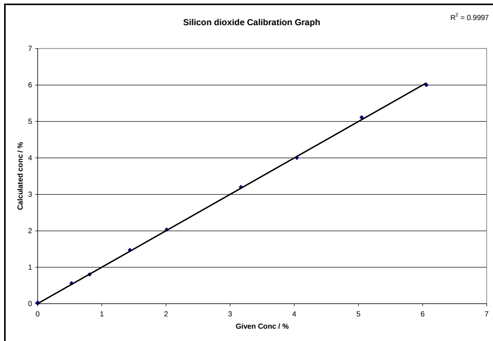
Figure D-0-3: Silicon dioxide calibration graph with potassium iodide as non-wetting agent and empirical corrections
