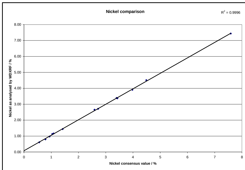
Figure 8-2: Comparison of consensus values and measured values for nickel
