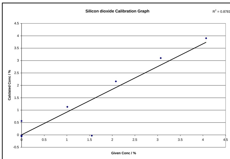
Figure C-0-14: Silicon dioxide calibration graph with bromine gas as non-wetting agent
