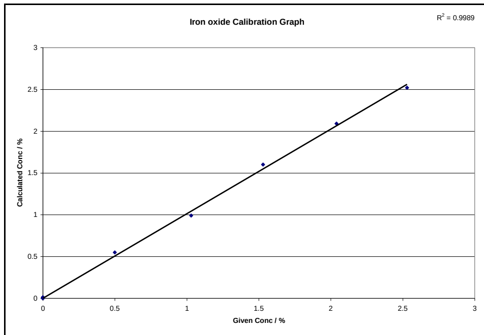
Figure C-0-3: Iron oxide calibration graph with sodium iodide as non-wetting agent and FP correction
