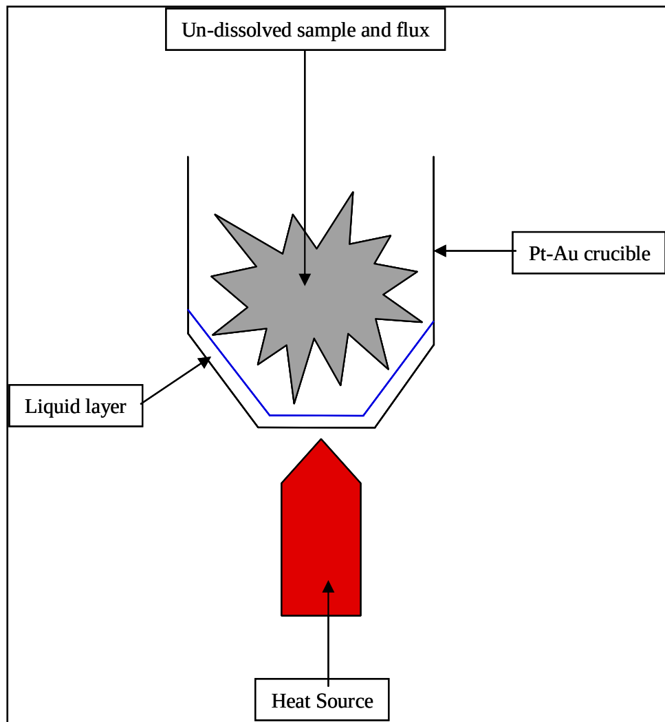
Figure 5-4: Picture illustrating heating mechanism from below only
