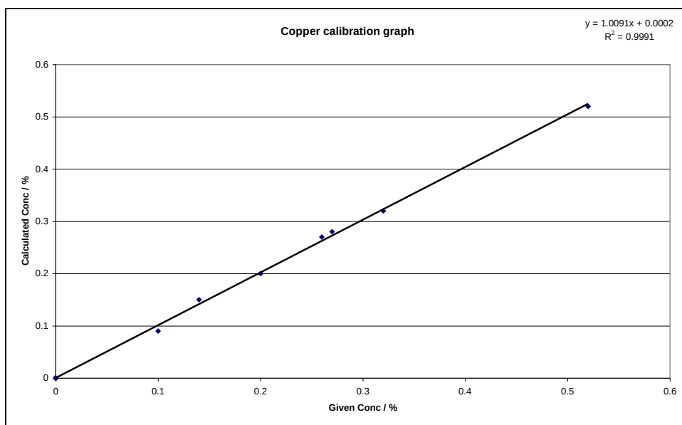
Figure 7-1: EDXRF Copper calibration graph with FP corrections 16
