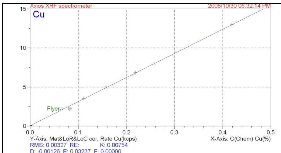
Figure 7-5: WDXRF Copper calibration graph with FP corrections
