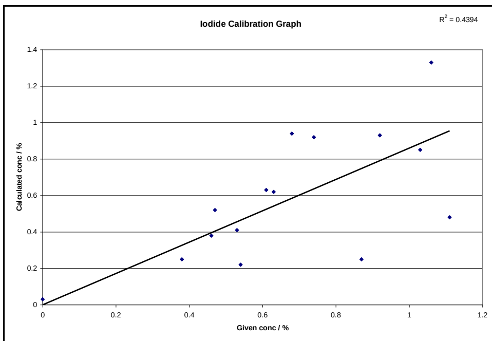
Figure 5-11: Iodide calibration graph with empirical corrections
