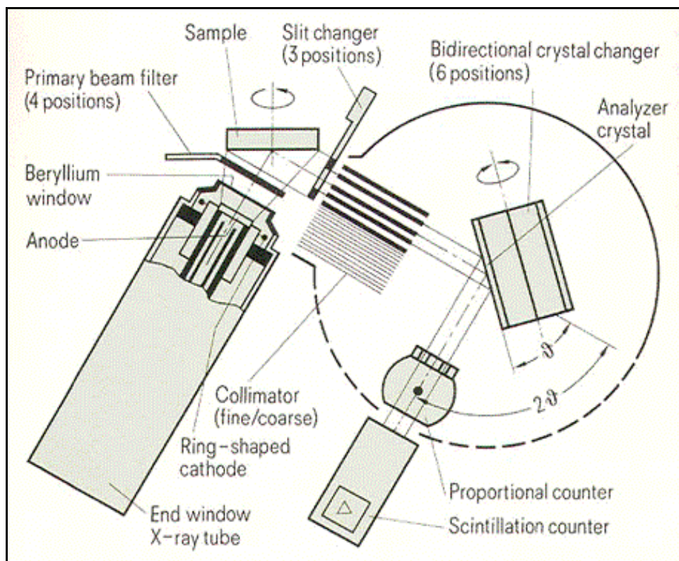
Figure 2-1: Schematic diagram of WDXRF 1
