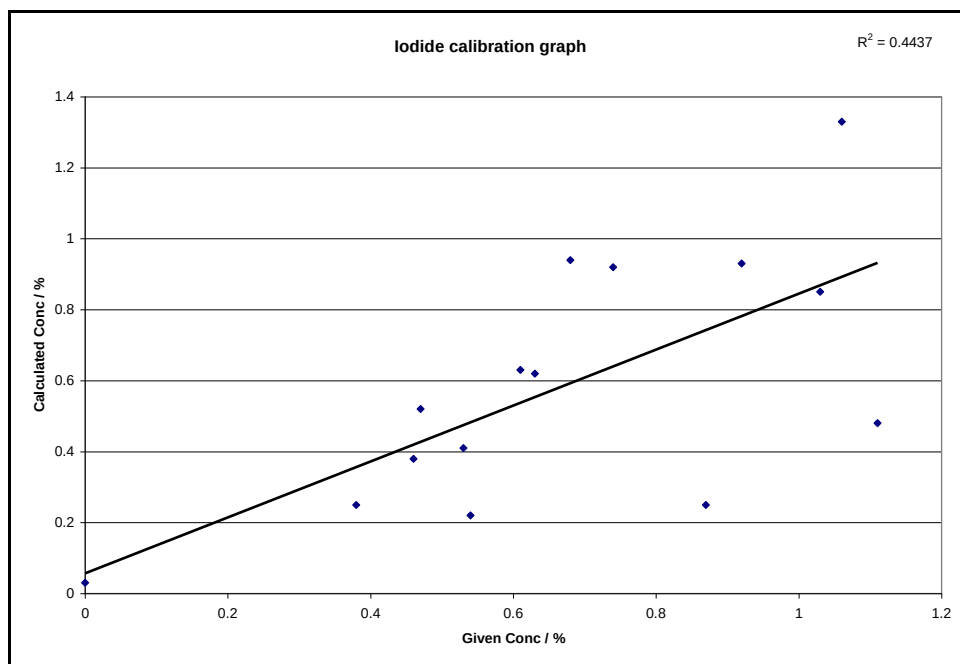
Figure 5-6: Iodide calibration graph with final calibration program and fundamental parameter correction model
