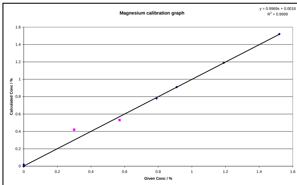
Figure F-0-1: Magnesium calibration graph on EDXRF with FP corrections
