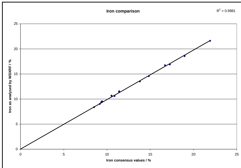
Figure 8-4: Comparison of consensus values and measured values for iron
