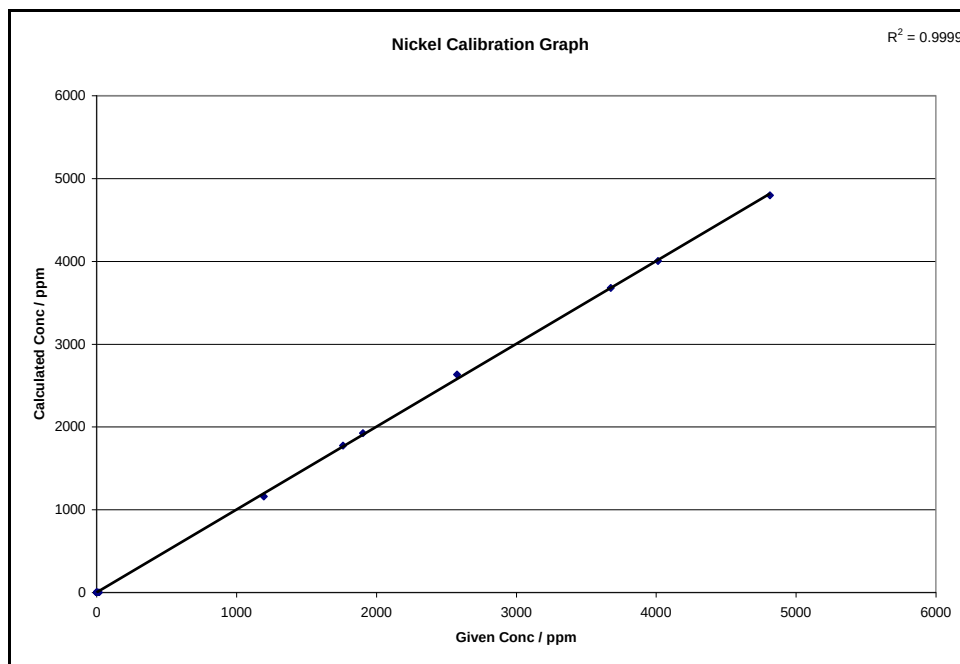
Figure D-0-8: Nickel calibration graph with potassium iodide as non-wetting agent and empirical corrections
