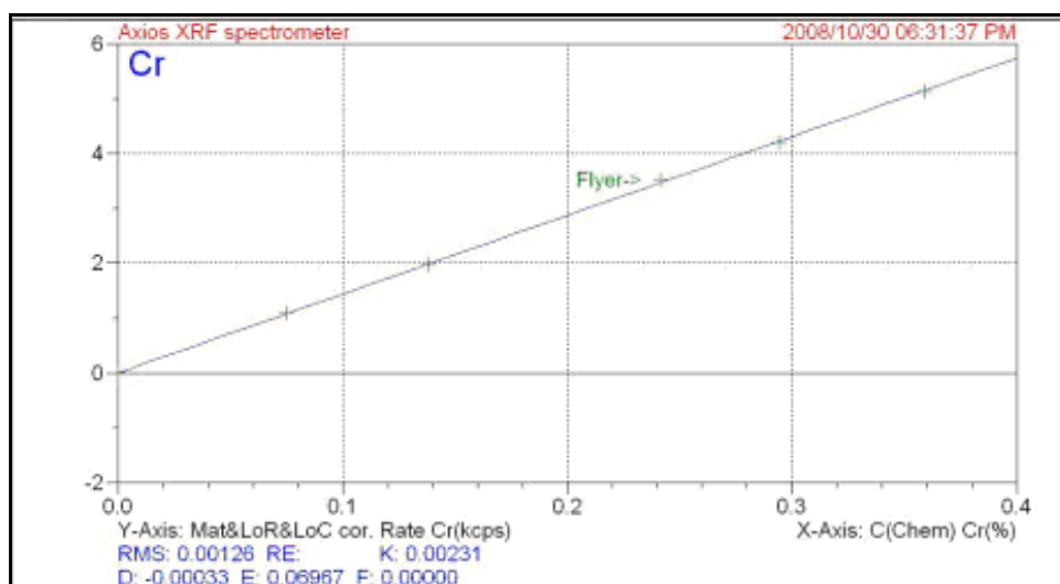
Figure F-0-12: Chrome calibration graph on WDXRF with FP corrections
