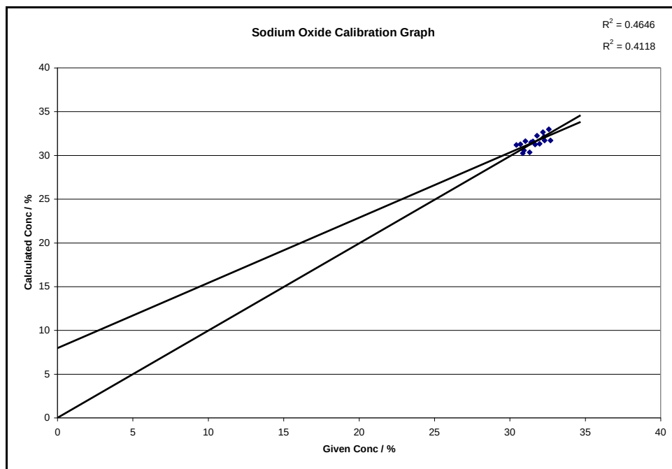
Figure 5-10: Sodium oxide calibration graph with empirical corrections
