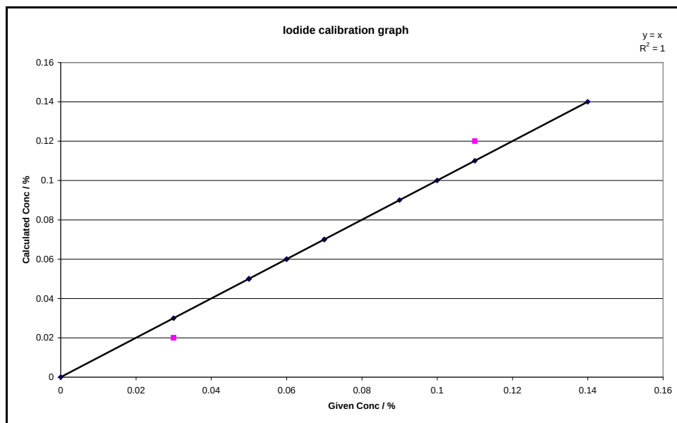
Figure 7-4: EDXRF Iodide calibration graph with FP corrections
