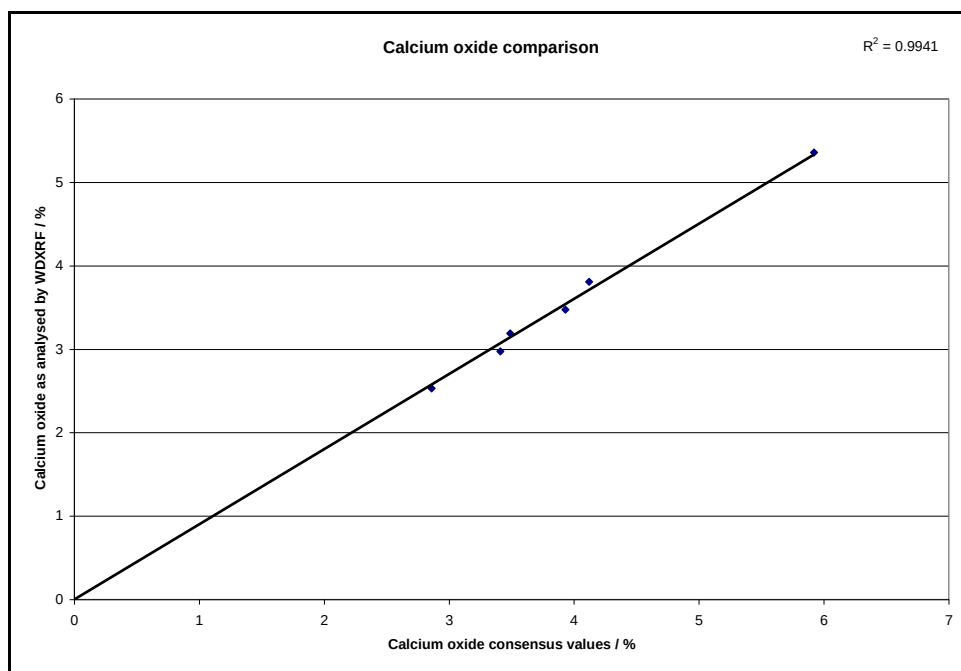
Figure 8-7: Comparison of consensus values and XRF values for calcium oxide
