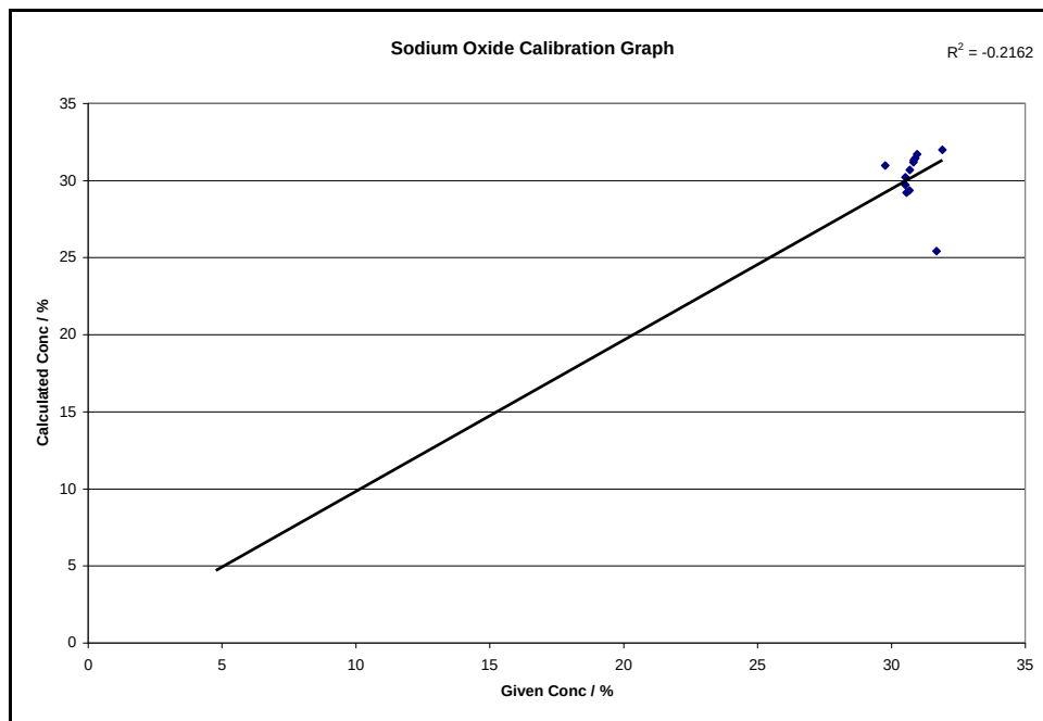
Figure C-0-11: Sodium oxide calibration graph with bromine gas as non-wetting agent
