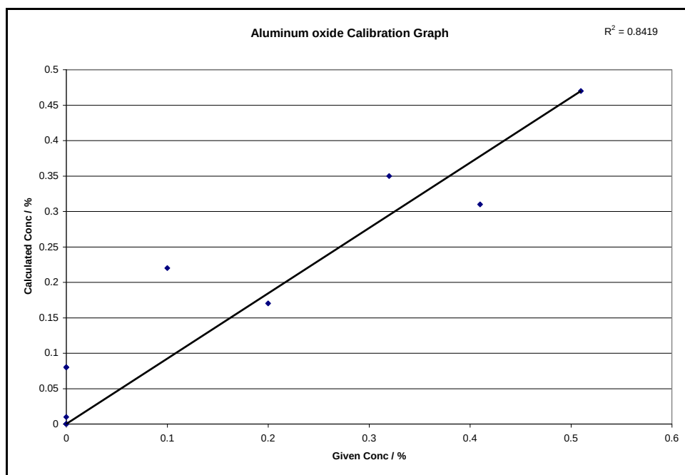
Figure C-0-8: Aluminum oxide calibration graph with sodium iodide as non-wetting agent and FP corrections
