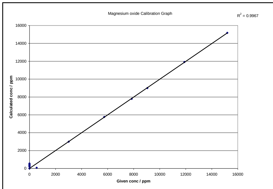
Figure D-0-1: Magnesium oxide calibration graph with potassium iodide as non-wetting agent and empirical corrections
