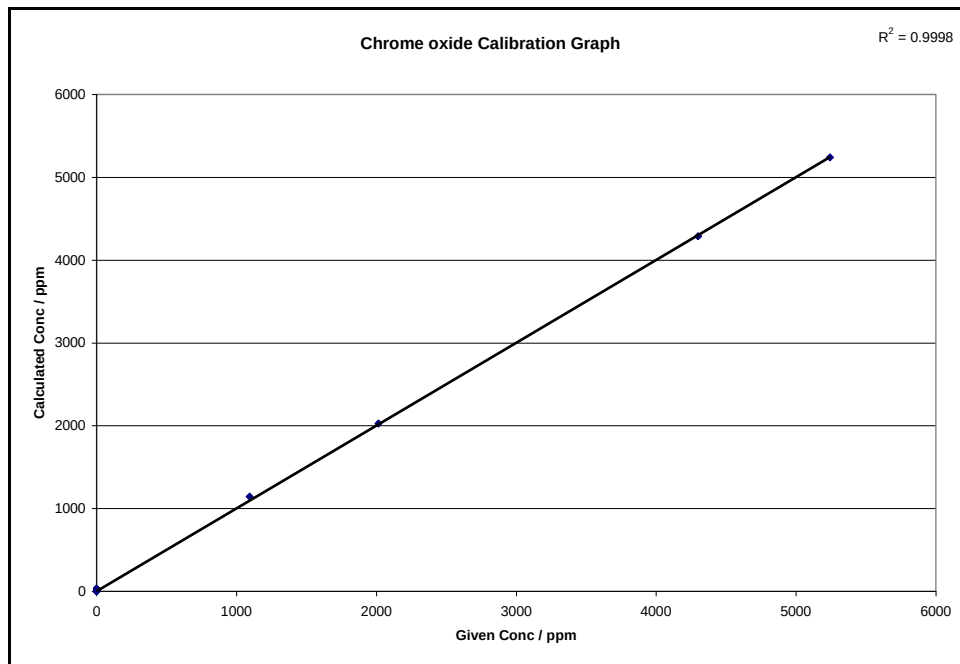
Figure D-0-5: Chromic oxide calibration graph with potassium iodide as non-wetting agent and empirical corrections
