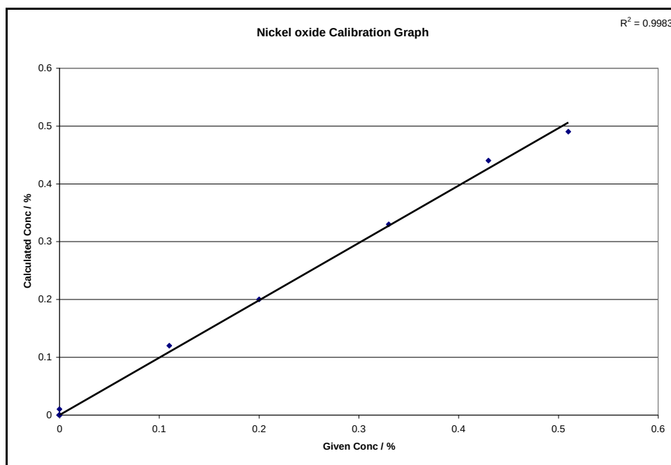
Figure C-0-22: Nickel oxide calibration graph with bromine gas as non-wetting agent
