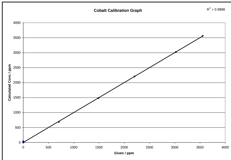
Figure D-0-7: Cobalt calibration graph with potassium iodide as non-wetting agent and empirical corrections
