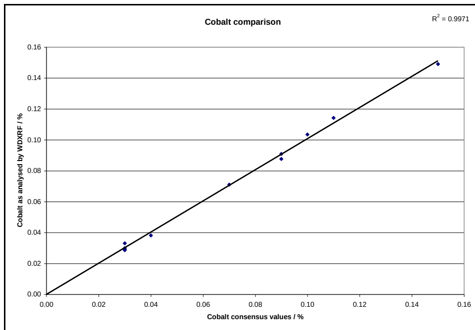
Figure 8-5: Comparison of consensus values and measured values for cobalt
