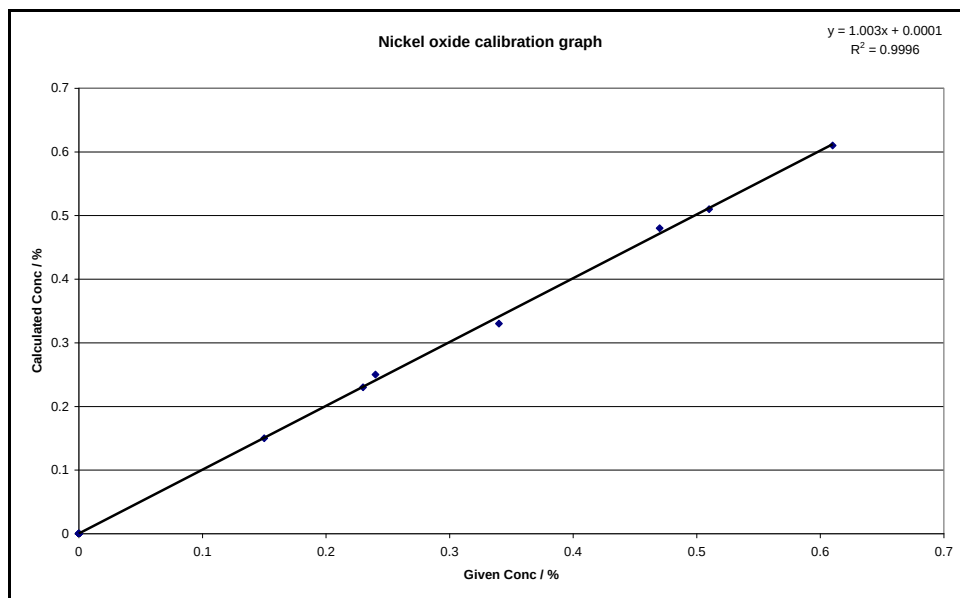
Figure F-0-8: Nickel oxide calibration graph on EDXRF with FP corrections
