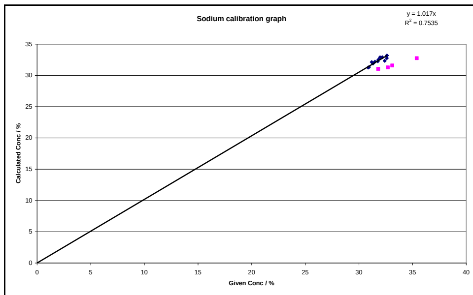
Figure 7-3: EDXRF Sodium calibration graph with FP corrections
