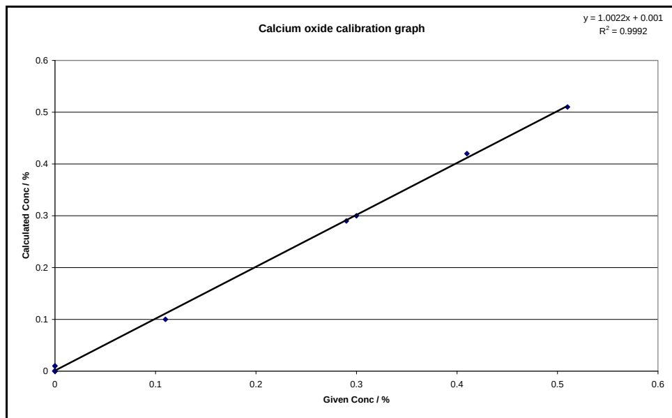
Figure F-0-4: Calcium oxide calibration graph on EDXRF with FP corrections
