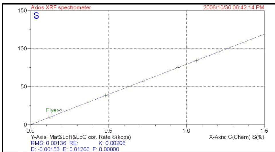
Figure 7-6: WDXRF Sulphur calibration graph with FP corrections
