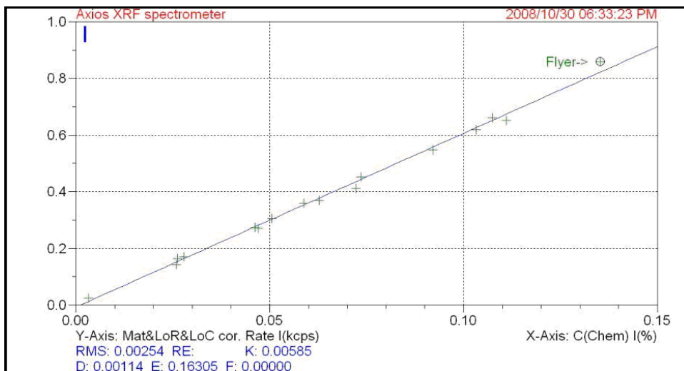
Figure 7-8: WDXRF Iodide calibration graph with FP corrections
