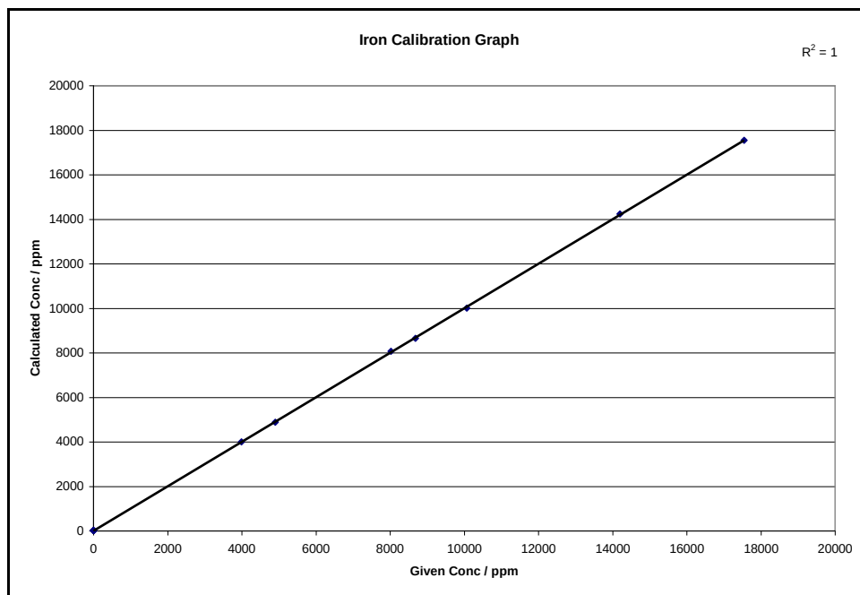
Figure D-0-6: Iron calibration graph with potassium iodide as non-wetting agent and empirical corrections
