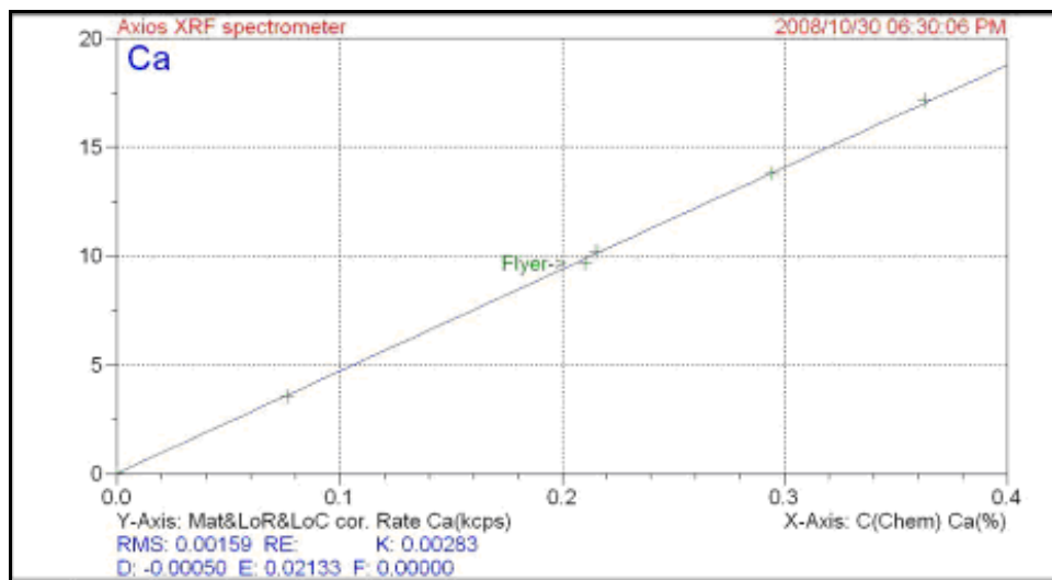
Figure F-0-11: Calcium calibration graph on WDXRF with FP corrections
