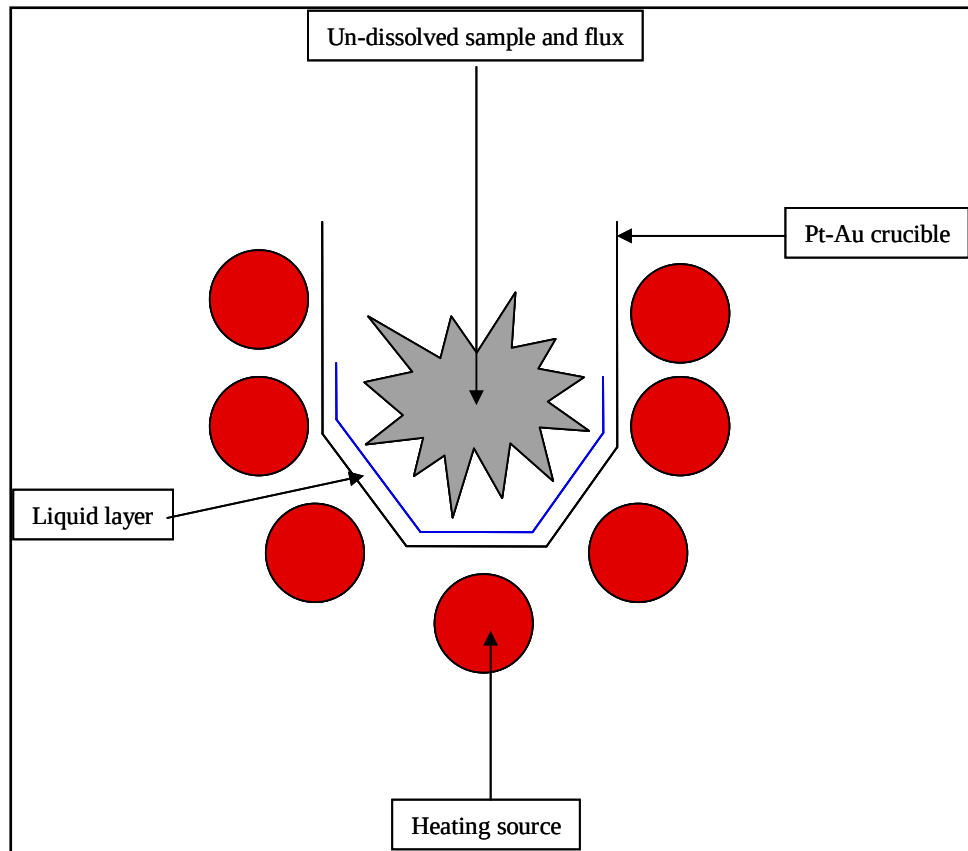
Figure 5-3: Picture illustrating heating mechanism of the Electrofluxer
