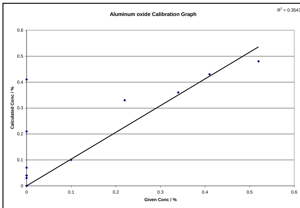
Figure C-0-13: Aluminum oxide calibration graph with bromine gas as non-wetting agent
