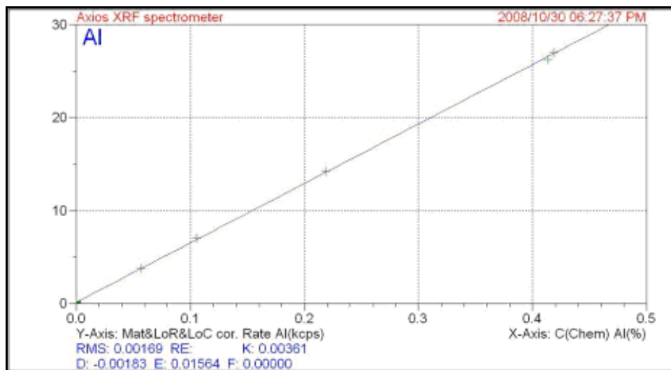
Figure F-0-9: Aluminum calibration graph on WDXRF with FP corrections
