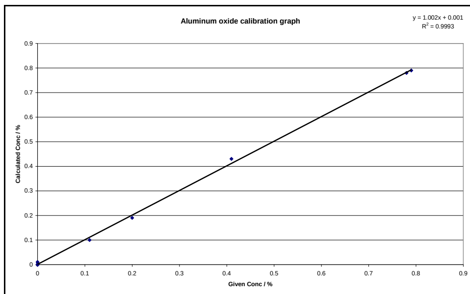
Figure F-0-2: Aluminum oxide calibration graph on EDXRF with FP corrections
