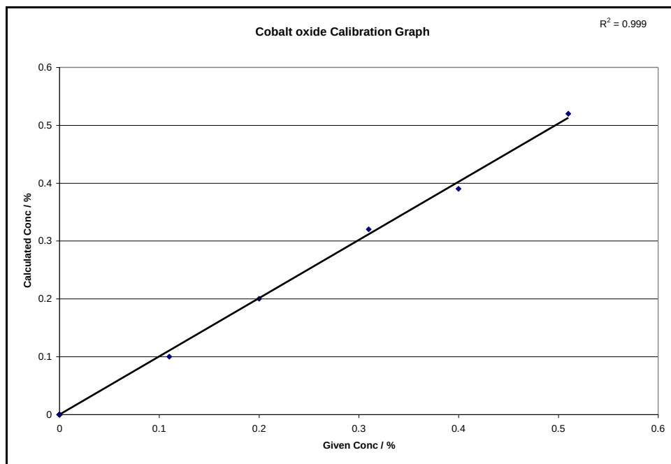
Figure C-0-21: Cobalt oxide calibration graph with bromine gas as non-wetting agent
