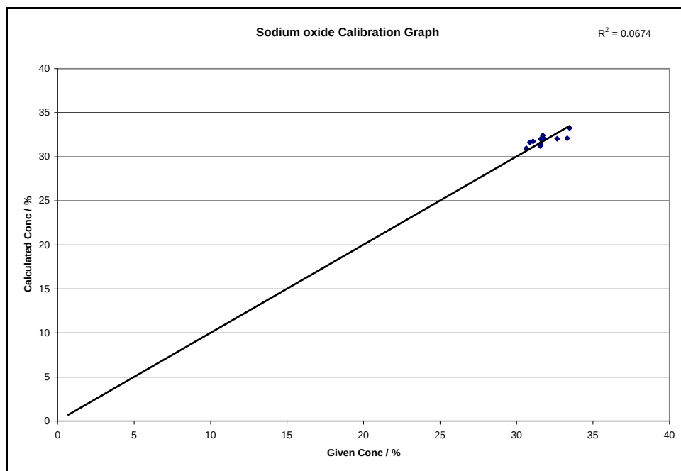
Figure C-0-10: Sodium oxide calibration graph with sodium iodide as non-wetting agent and FP corrections
