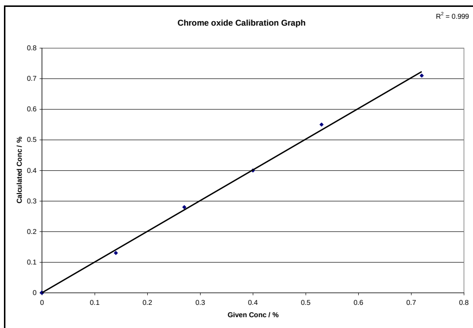
Figure C-0-18: Chromic oxide calibration graph with bromine gas as non-wetting agent
