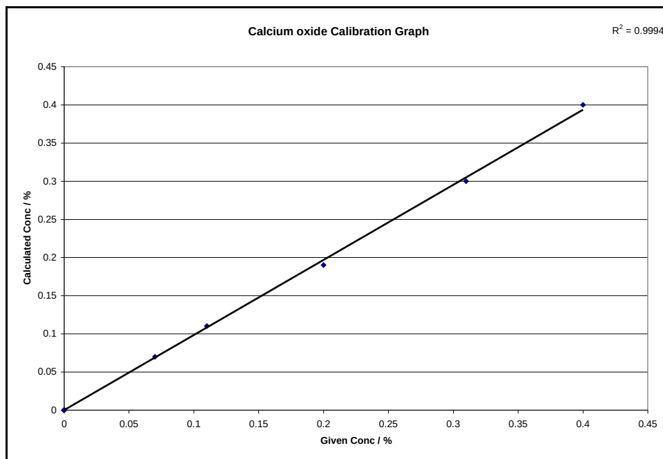
Figure C-0-17: Calcium oxide calibration graph with bromine gas as non-wetting agent
