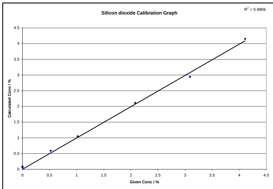
Figure C-0-7: Silicon dioxide calibration graph with sodium iodide as non-wetting agent and FP corrections
