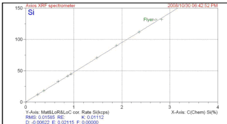
Figure F-0-10: Silica calibration graph on WDXRF with FP corrections
