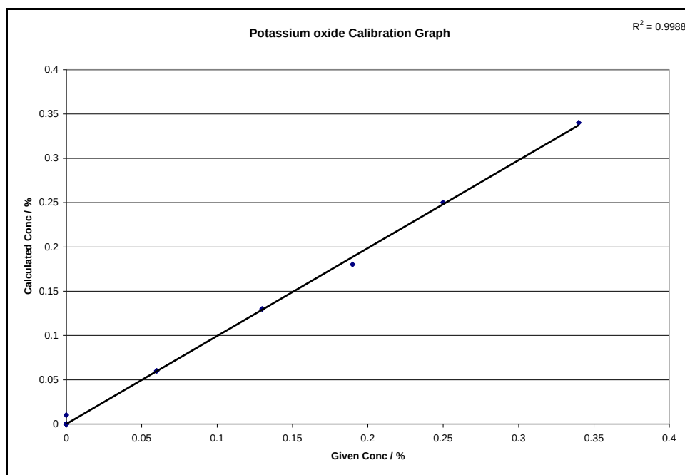
Figure C-0-16: Potassium oxide calibration graph with bromine gas as non-wetting agent
