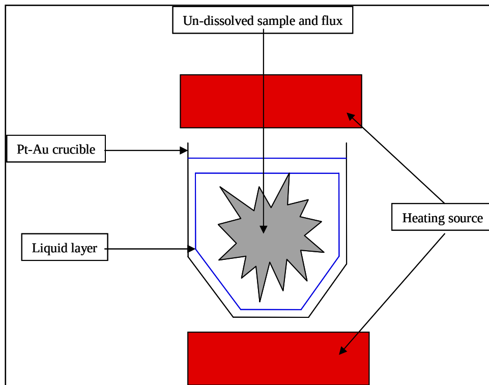
Figure 5-2: Picture illustrating heating mechanism of the Katanax
