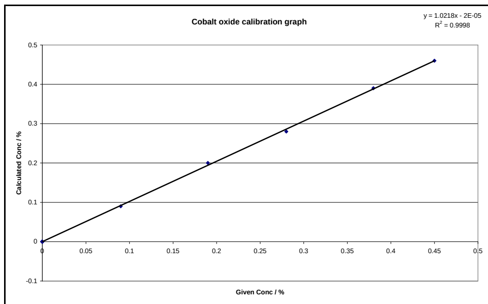
Figure F-0-7: Cobalt oxide calibration graph on EDXRF with FP corrections
