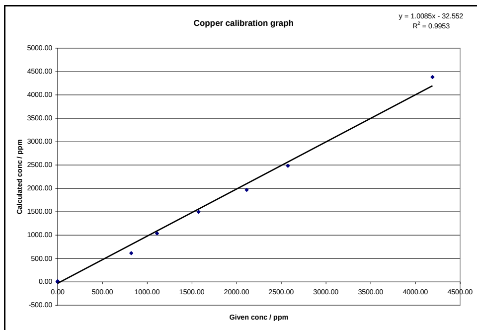
Figure 5-8: Copper calibration graph without empirical correction
