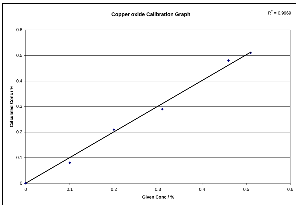
Figure 4-1: Copper oxide calibration graph with sodium iodide as non-wetting agent and fundamental parameter corrections
