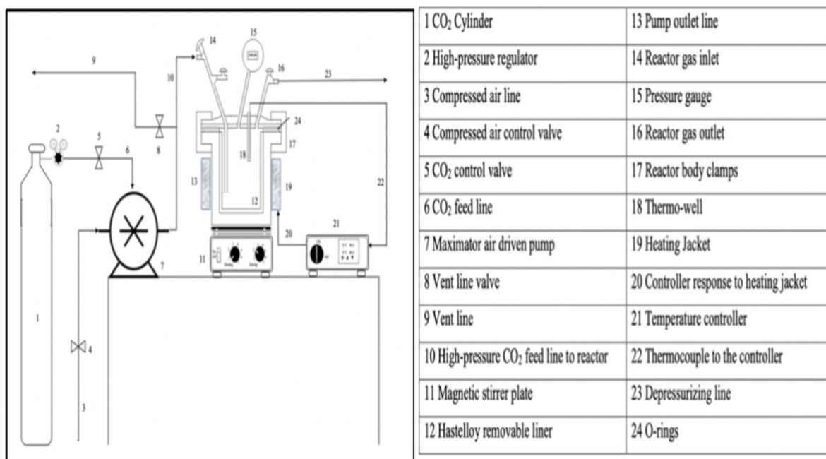
Figure 2.17: Experimental setup that Mawire (2019) used.
