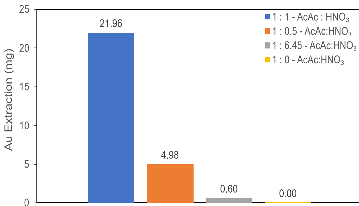
Figure 4.11: Au extracted when varying the volumetric ratio of AcAc to HNO 3 (6.34 M) at 100 Bar and 100°C for 8 hours.
