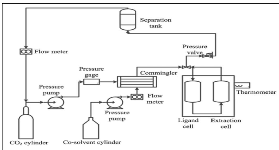
Figure 2.19: Experimental setup used by Liu et al. (2016).
