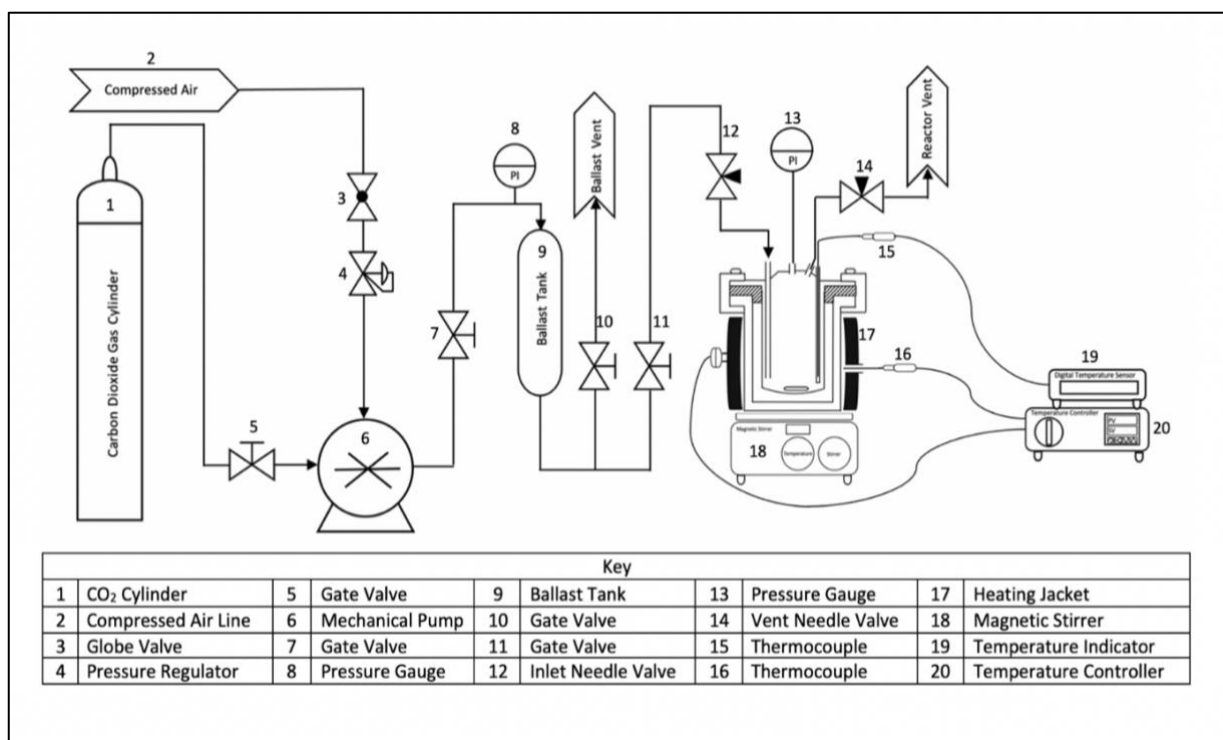
Figure 3.1: Supercritical fluid extraction experimental setup, adapted from Mawire (2019).
