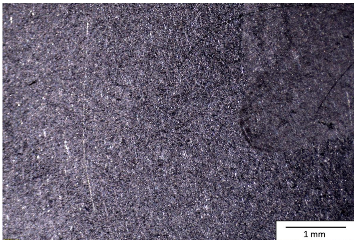
Figure 4.13: Corrosion of the Hastelloy bucket.
