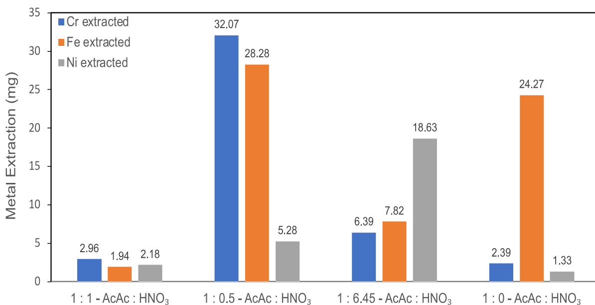
Figure 4.12: Cr, Fe and Ni extracted when varying the ratio of AcAc to HNO 3 at 100 Bar and 100°C for 8 hours.
