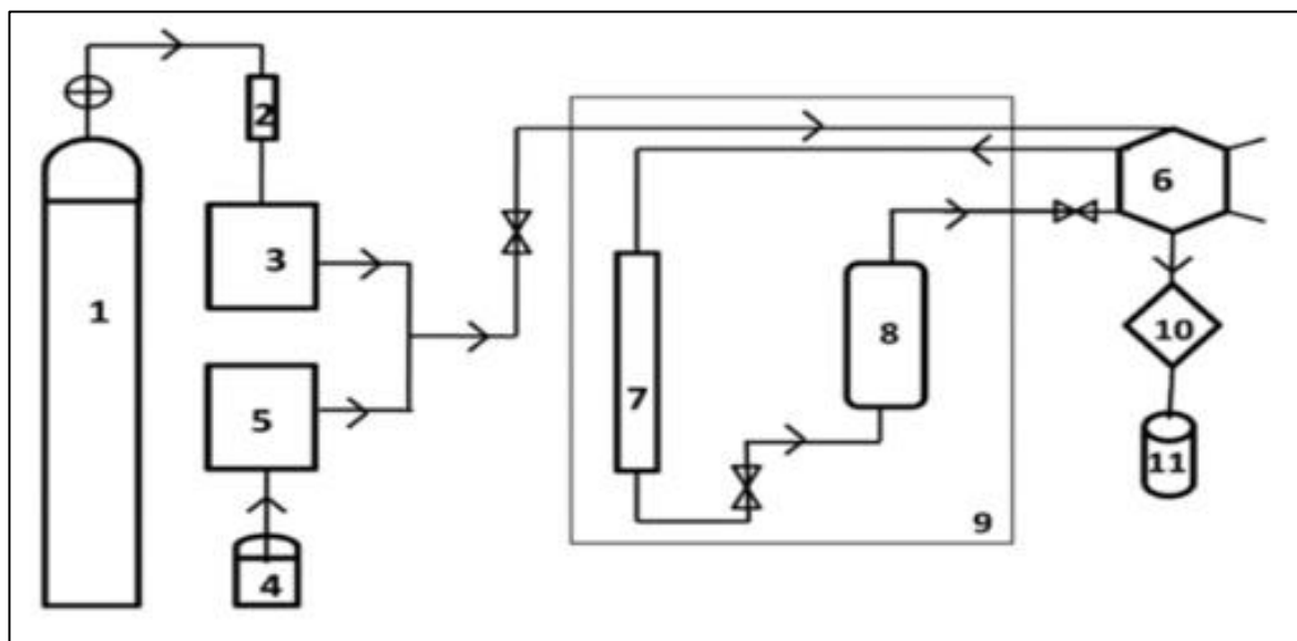
Figure 2.18: Experimental set up used by Pitchaiah et al. (2019). Carbon dioxide cylinder (1), molecular sieve filter (2), carbon dioxide pump (3), co-solvent reservoir (4), co-solvent pump (5), six way valve (6), heat exchanger (7), high pressure extraction vessel (8), oven (9), back pressure regulator (10) and collection vessel (11) (Pitchaiah et al., 2019).
