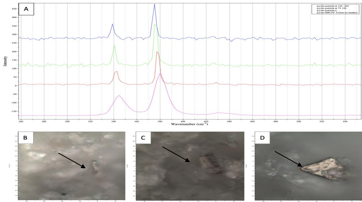
Figure 4.2: Micro-Raman spectra of three particles of pyrite (A–D). Figure A contains the identified pyrite spectrum. The blue, green and red spectra were produced from the pyrite particles identified in Figures B, C and D respectively (see the arrows). The pink spectrum is a reference pyrite sample from the RRUFF data base.
