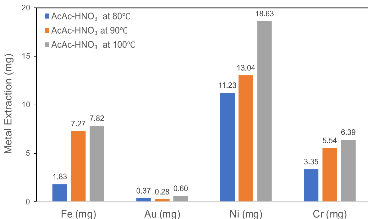
Figure 4.7: AcAc-HNO 3 (20 mL of 6.34 HNO 3 and 3 mL AcAc) metal extraction over a temperature range (80-100 °C) for 8 hr at 100 Bar.
