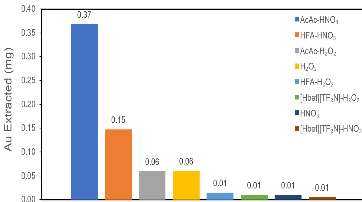
Figure 4.5: SFE of Au in different oxidants (20 mL \text{HNO}_3 or \text{H}_2\text{O}_2 ) and 3 mL of the ligands (Acetylacetone(AcAc), hexafluoroacetylacetone (HFA) and betaine bis(trifluoromethylsulfonyl)imide ([Hbet][TF 2 N]) ) at 100 Bar, 80°C for 8 h.
