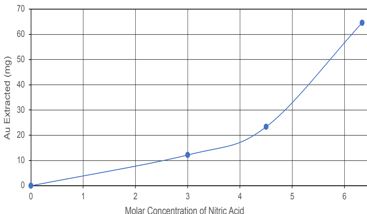
Figure 4.17: The effect of \text{HNO}_3 concentration on the extraction of Au at 100 Bar and 100^\circ\text{C} for 8 hours.
