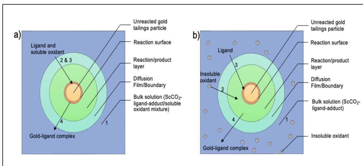
Figure 4.4: Possible transport steps in the SFE process.
