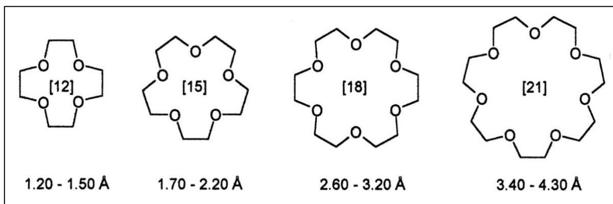
Figure 2.12: Crown ethers along with their associated cavity sizes (Steed, 2001).
