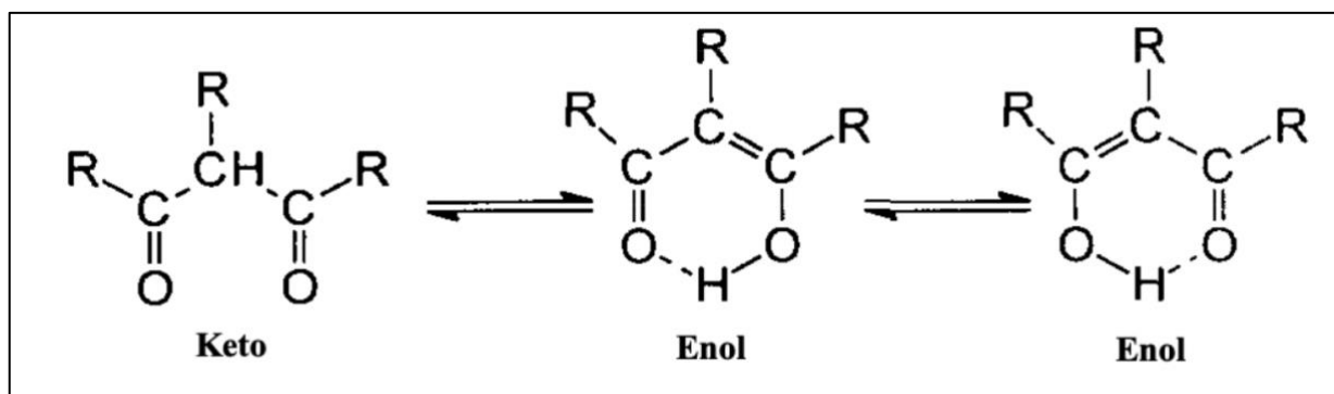
Figure 2.9: Keto-enol tautomerism in \beta -diketones (Özel et al., 1997).
