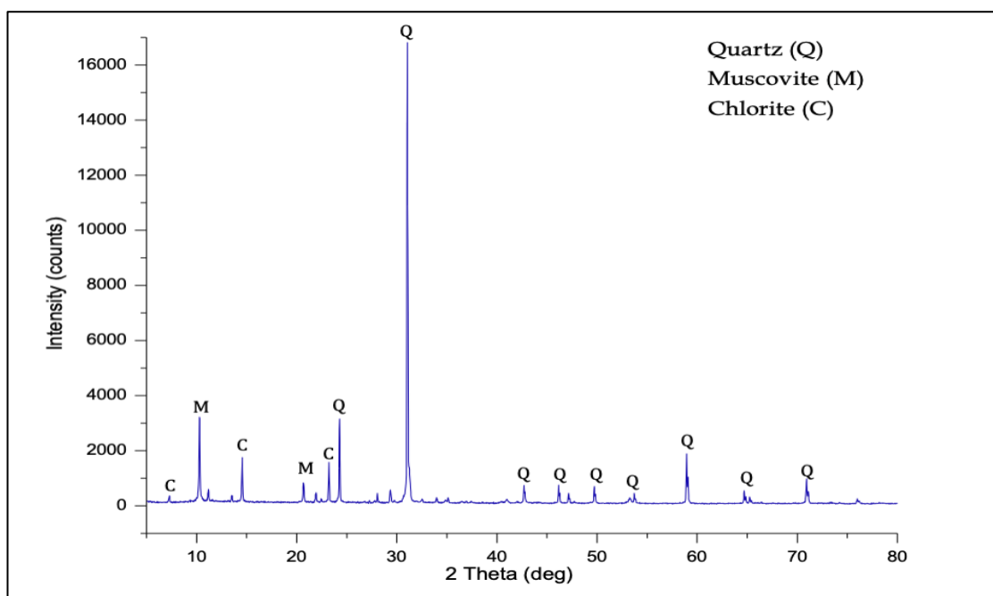
Figure 4.1: XRD diffractogram of the DRD Gold plant tailings [Cobalt anode - wavelength of 1.79 Å, 2 Theta range: 5-80 degrees and steps 0.0274 degrees].
