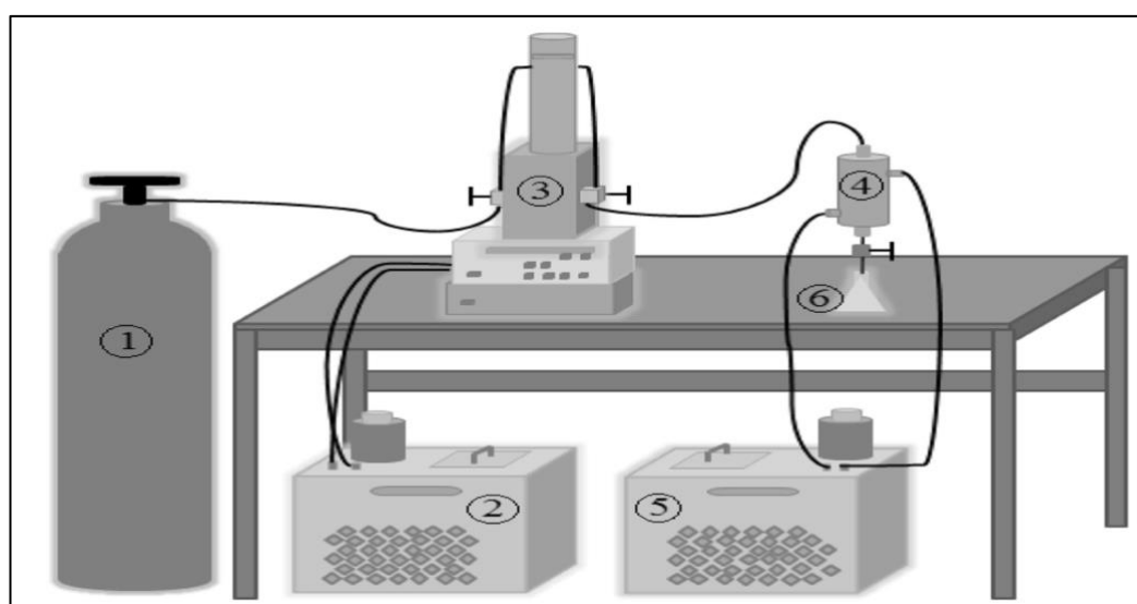
Figure 2.20: Experimental setup used by Argenta et al. (2017). Carbon dioxide cylinder (1), cooling bath (2), high pressure pump (3), extractor (4), heating bath (5), extracted sample (6) (Argenta et al., 2017).
