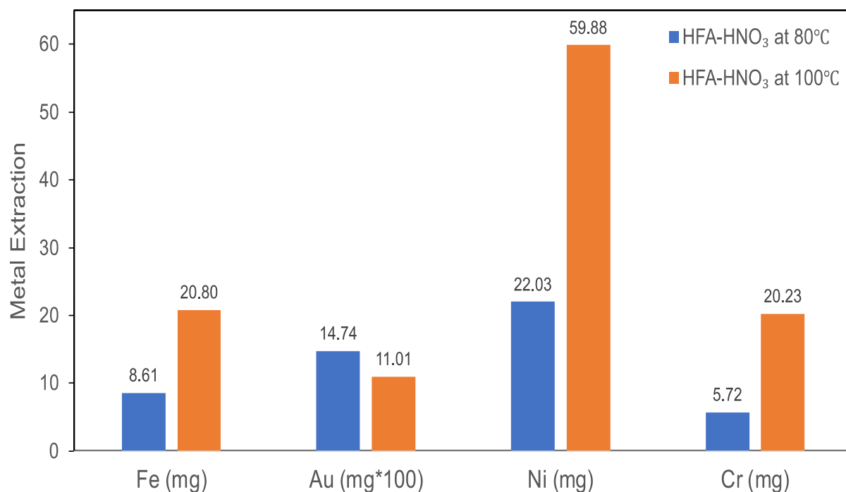
Figure 4.9: HFA-HNO 3 (20 mL of 6.34 HNO 3 and 3 mL HFA) metal extraction over a temperature range (80-100°C) for 8 hr at 100 Bar (Au is in mg*100 so that the difference can be seen).
