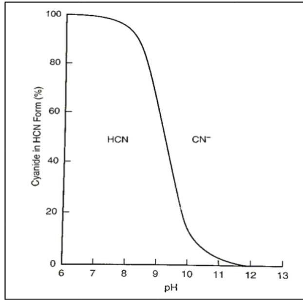
Figure 2.5: CN^- ions lost to the formation of HCN at varying pH's (Marsden & House, 2006).
