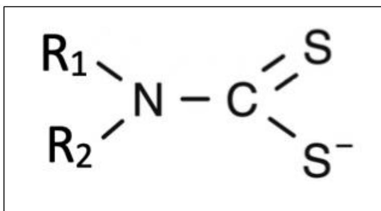
Figure 2.8: General structure of a dithiocarbamates (Ding et al., 2017).
