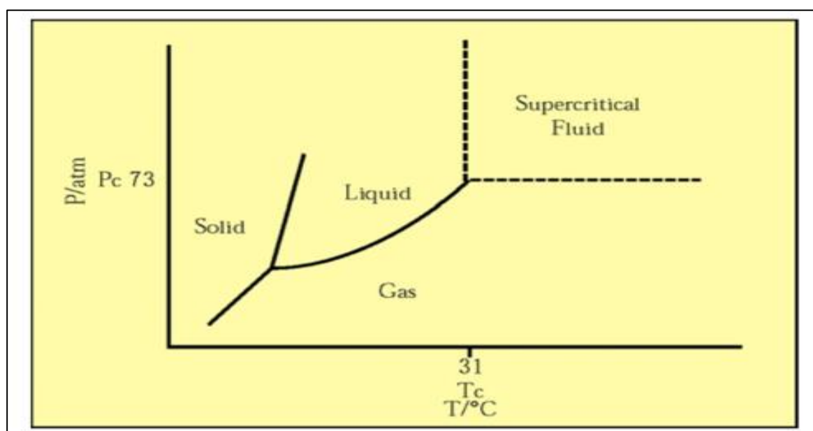
Figure 2.7: CO 2 phase diagram (Glennon et al., 1999).
