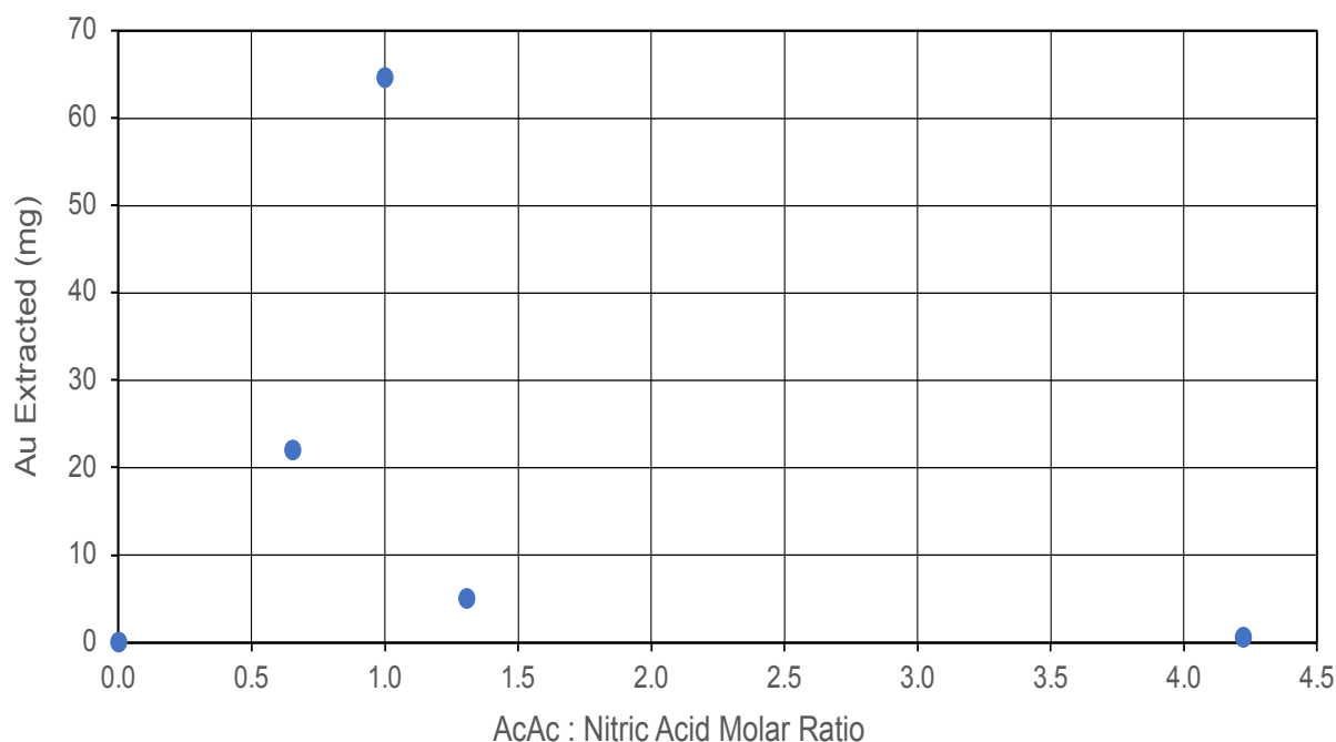
Figure 4.16: Au extracted when changing the molar ratio of AcAc to \text{HNO}_3 at 100 Bar and 100 °C for 8 hours.
