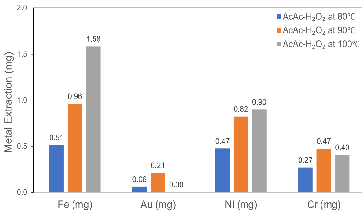
Figure 4.8: AcAc-H 2 O 2 (20 mL of 6.34 H 2 O 2 and 3 mL AcAc) metal extraction over a temperature range (80-100°C) for 8 hr at 100 Bar.
