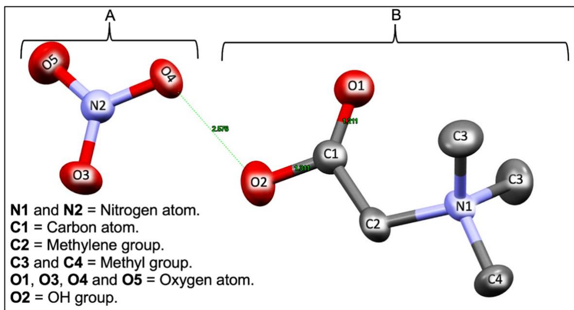
Figure 4.3: Molecular structure of crystalline precipitate (Trimethylammonioacetic acid nitrate).
