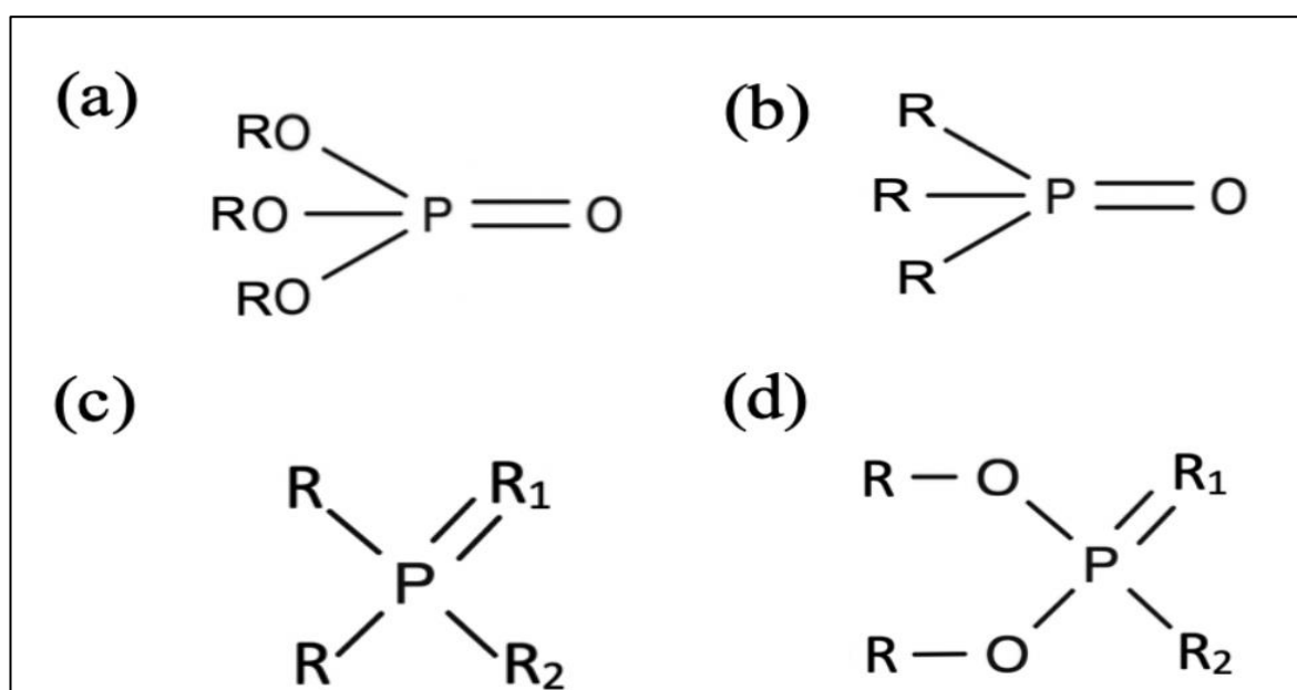
Figure 2.11: General chemical structures of different organophosphorus reagents (Ding et al., 2017; Erkey, 2000; Wai & Wang, 1997).
