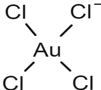
Figure 2.3: Square planar geometry of an auric gold complex (Lorösch, 2001).
