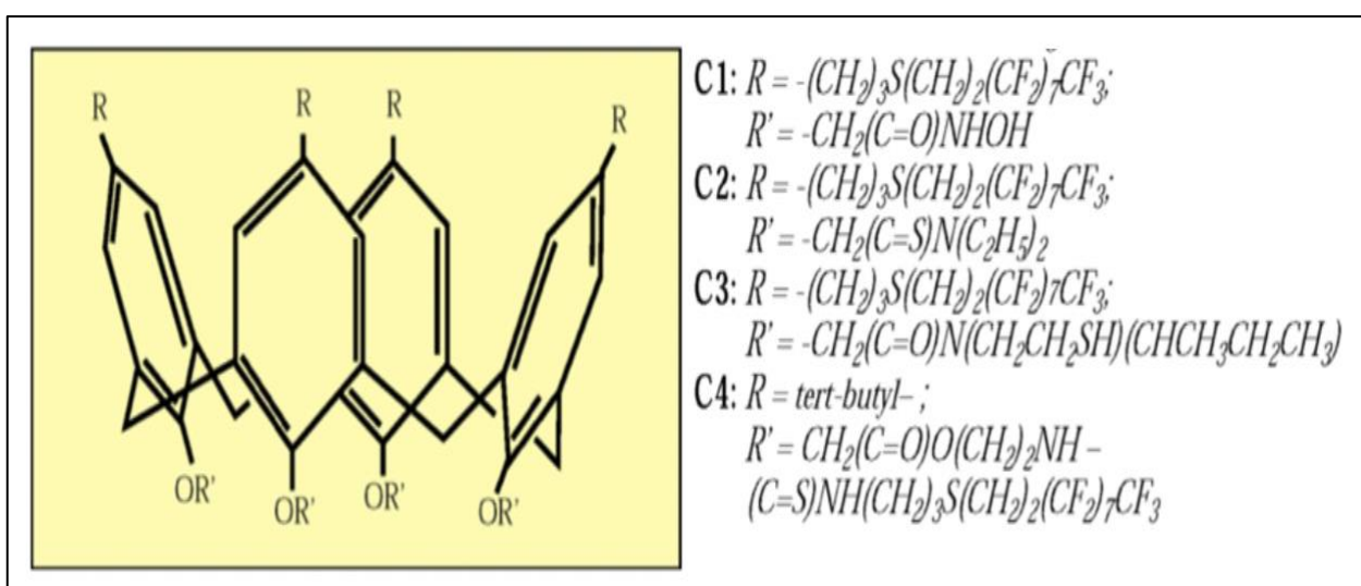
Figure 2.16: Fluorinated calixarene derivatives with lower rim sulphur donor atoms (Glennon et al., 1999).
