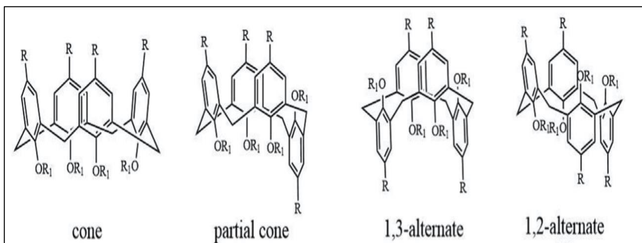
Figure 2.14: Different conformations of unsubstituted calix[4]arenes (Wang & Zhuang, 2020).
