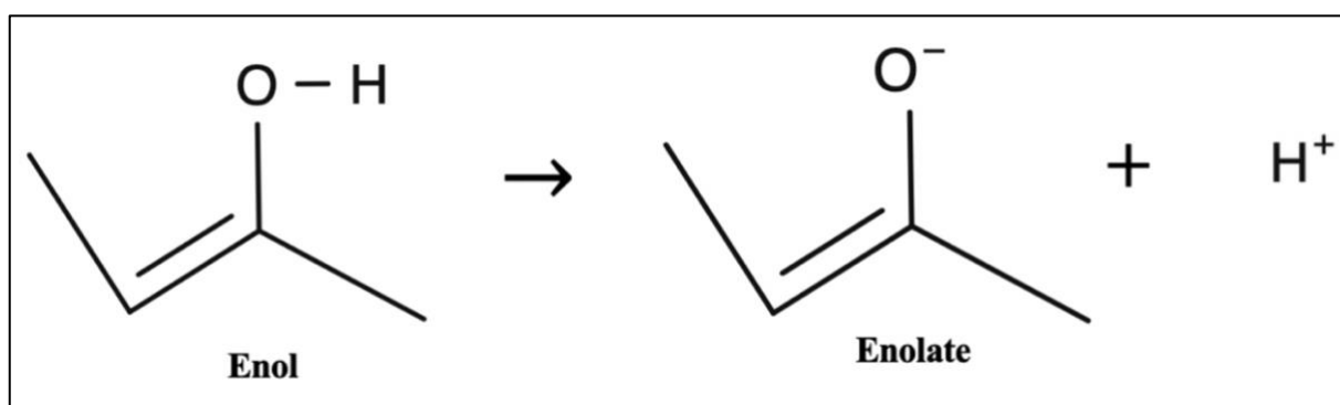
Figure 2.10: Enol vs Enolate form in \beta -diketones (Ding et al., 2017 ).
