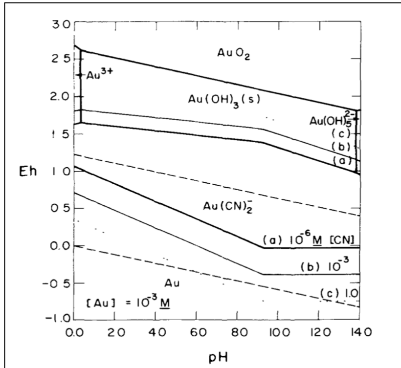
Figure 2.4: Eh-pH diagram for Au-CN-H 2 O system (Xue & Osseo-Asare, 1985).
