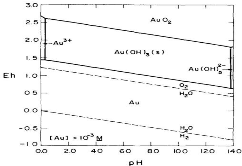
Figure 2.1: Eh vs pH diagram for gold (Xue & Osseo-Asare, 1985).
