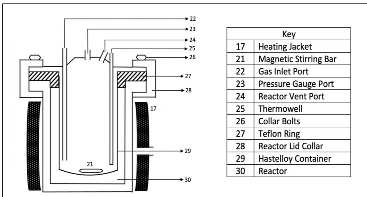
Figure 3.2: Supercritical fluid reactor, adapted from Mawire (2019).
