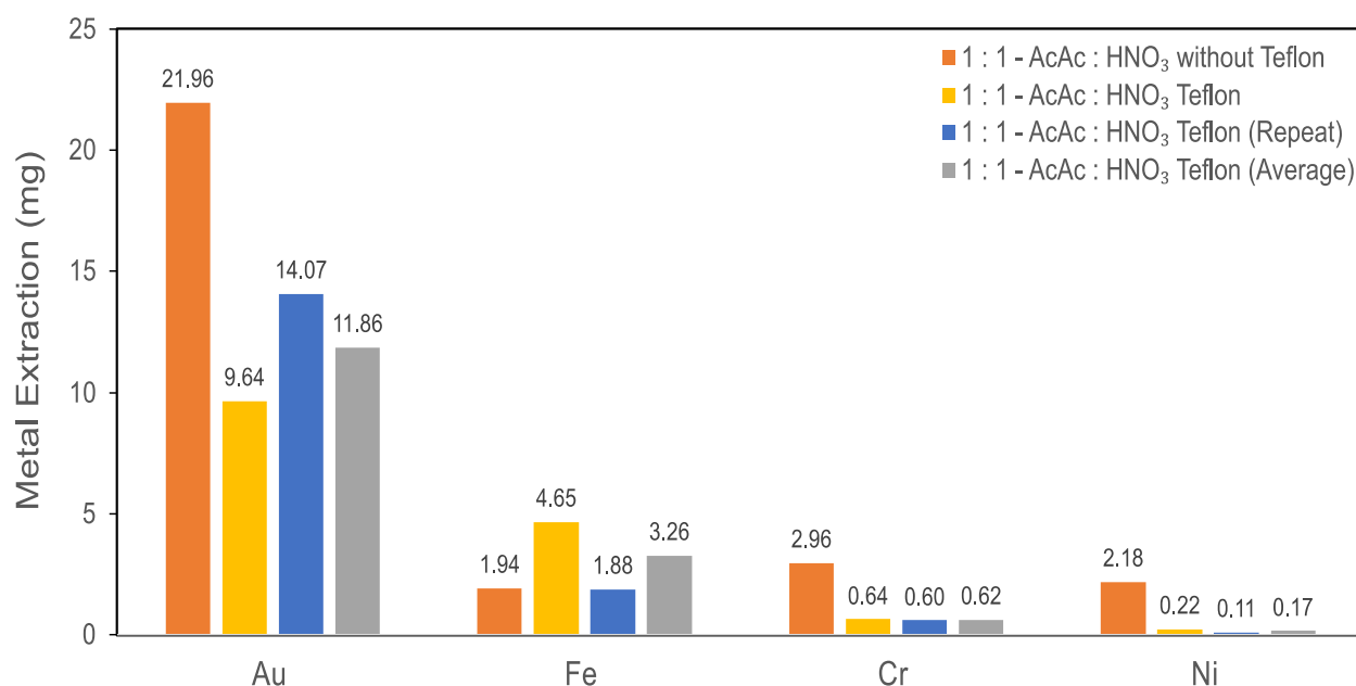
Figure 4.15: Metals extracted when using a Hastelloy bucket vs a Teflon liner at 100 Bar and 100 °C for 8 hours.
