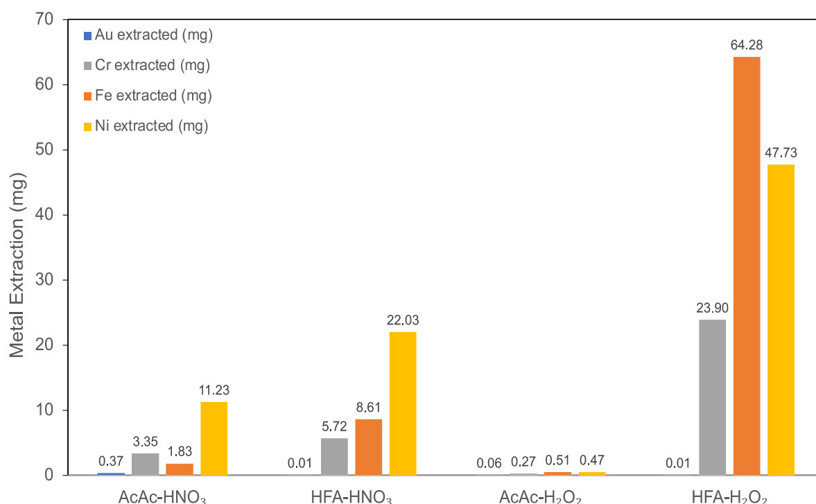
Figure 4 6: Metals extracted using AcAc/HFA with different oxidants after 8 hours at 100 Bar and 80 °C.
