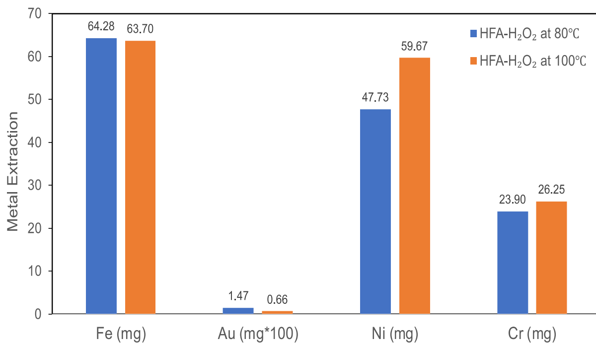
Figure 4.10: HFA-H 2 O 2 (20 mL of 6.34 H 2 O 2 and 3 mL HFA) metal extraction over a temperature range (80-100°C) for 8 hr at 100 Bar (Au is in mg*100 so that the difference can be seen).
