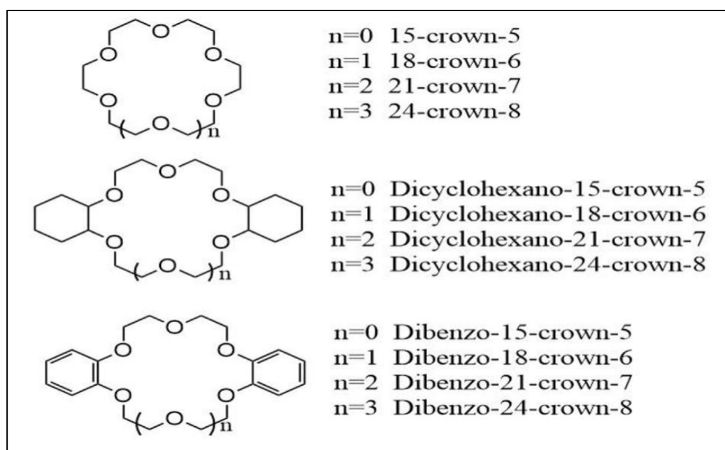
Figure 2.13: Common crown ethers (Wang & Zhuang, 2020).
