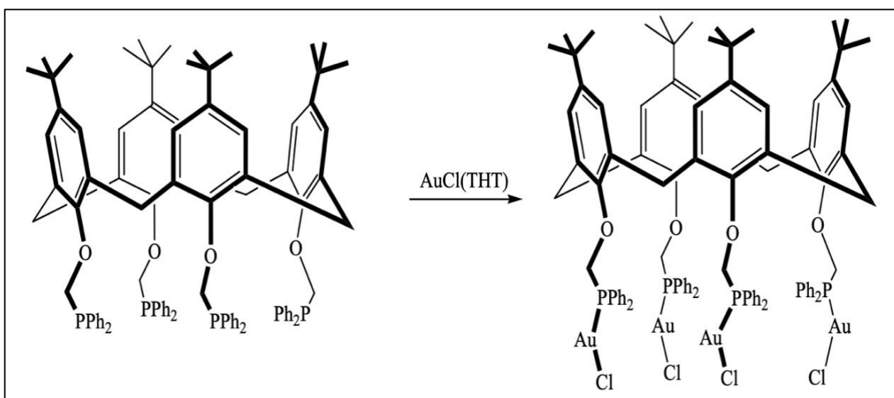
Figure 2.15: Tetragold complex (Silwa & Deska, 2008).
