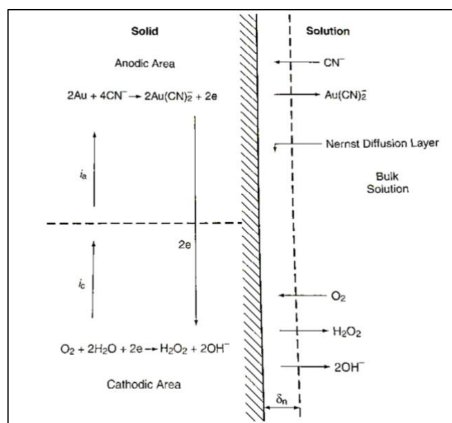
Figure 2.6: Steps involved in the dissolution of gold (Marsden & House, 2006).
