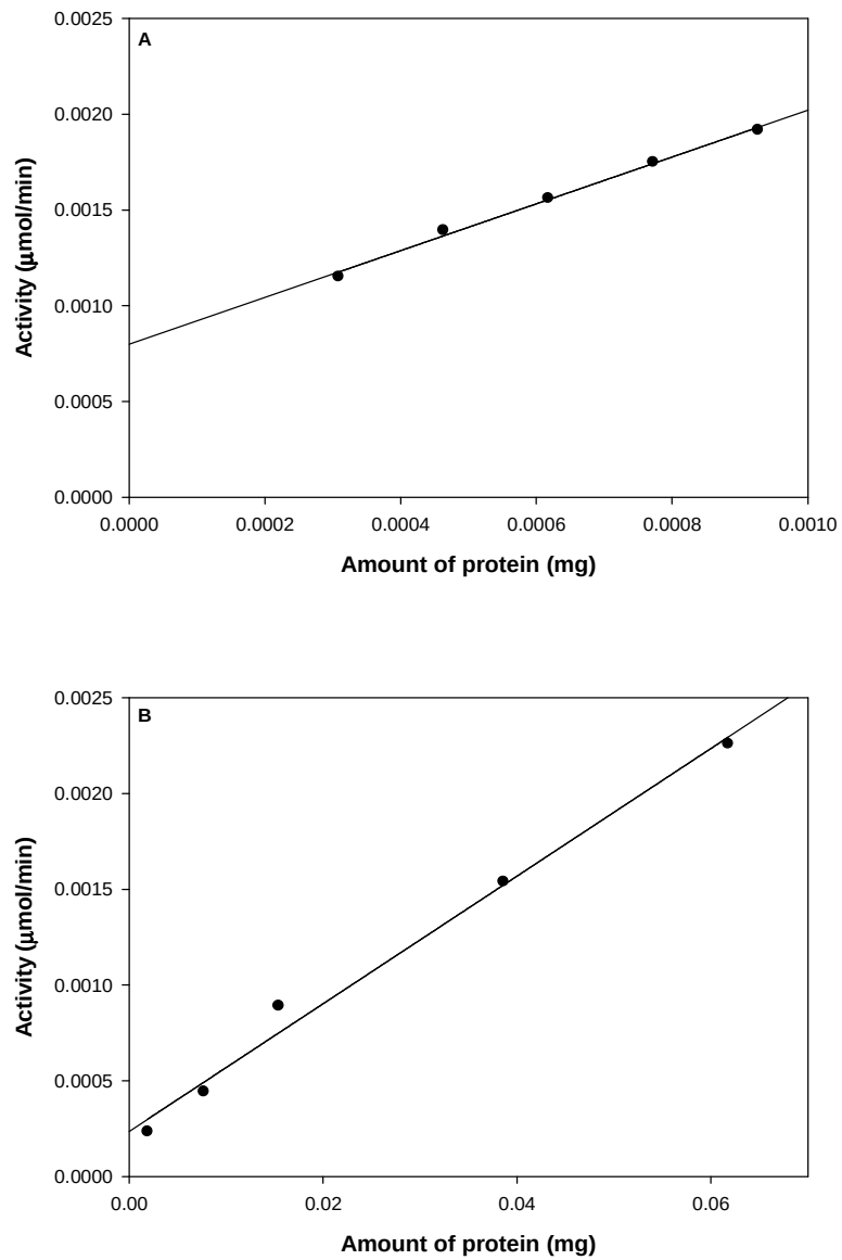
Figure 3-6: Specific activity of wild-type rGST M1-1 and F56S/R81A mutant.
