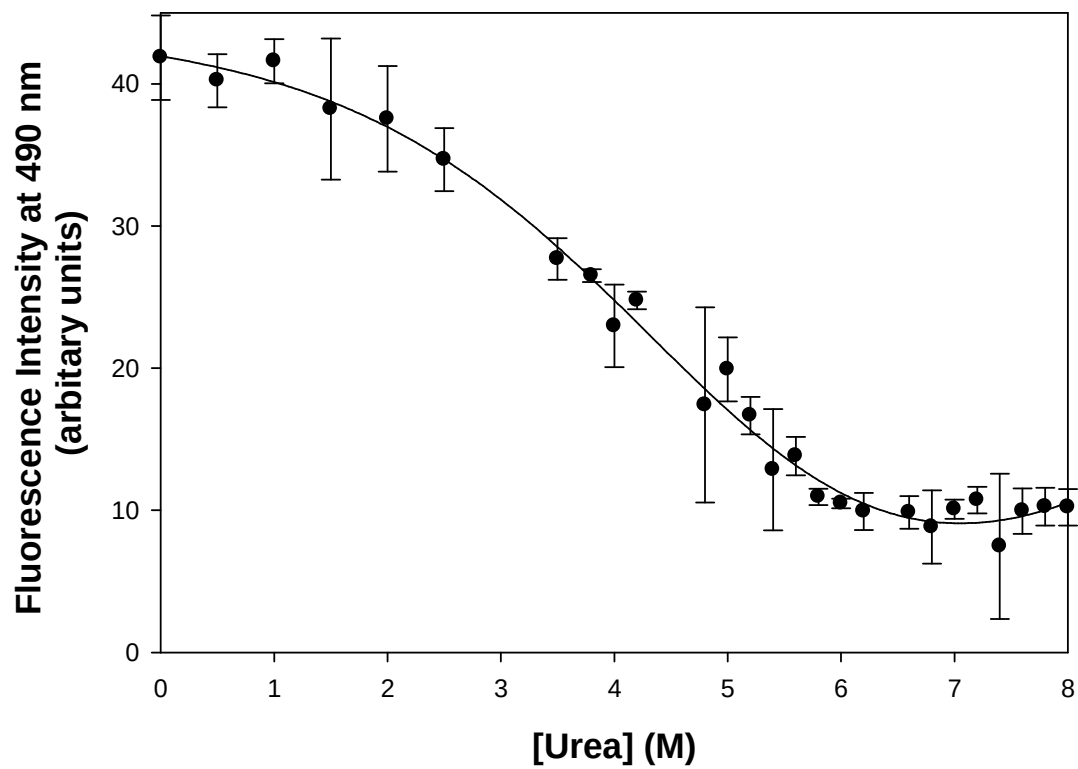
Figure 3-12: rGST M1 urea induced unfolding monitored by following ANS fluorescence.
