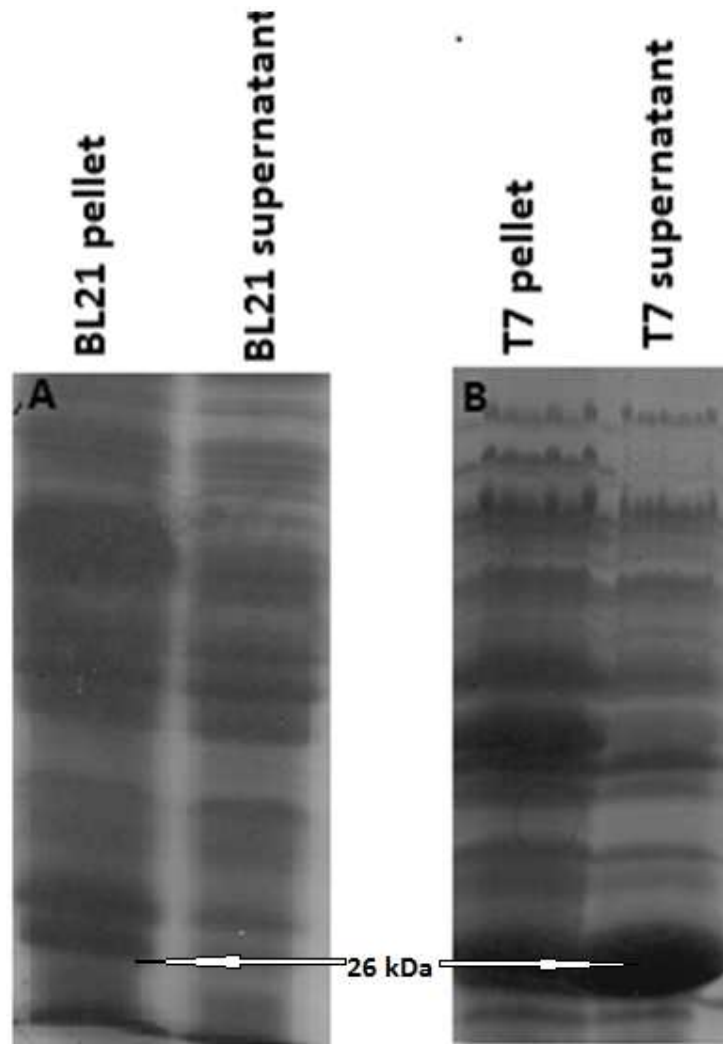
Figure 3-2: SDS-PAGE analysis of the F56S/R81A mutant protein overexpression.
