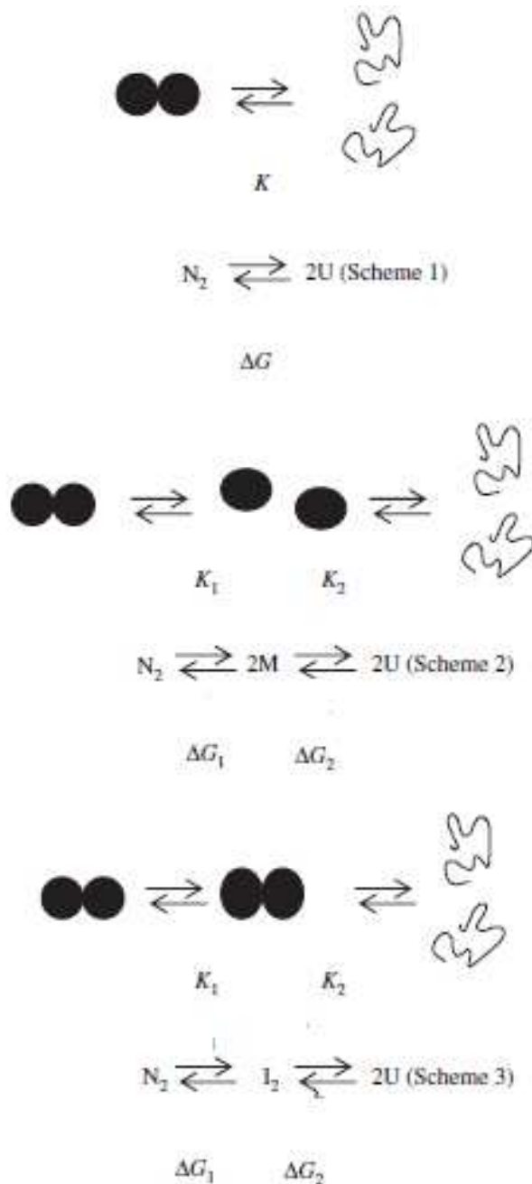
Figure 1-1: Commonly observed folding pathways for dimeric proteins.
