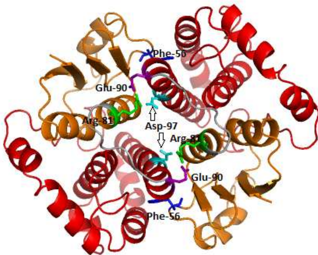
Figure 1-2: Three dimensional structure ribbon representation of homodimeric rGST M1-1 viewed down its two fold axis.
