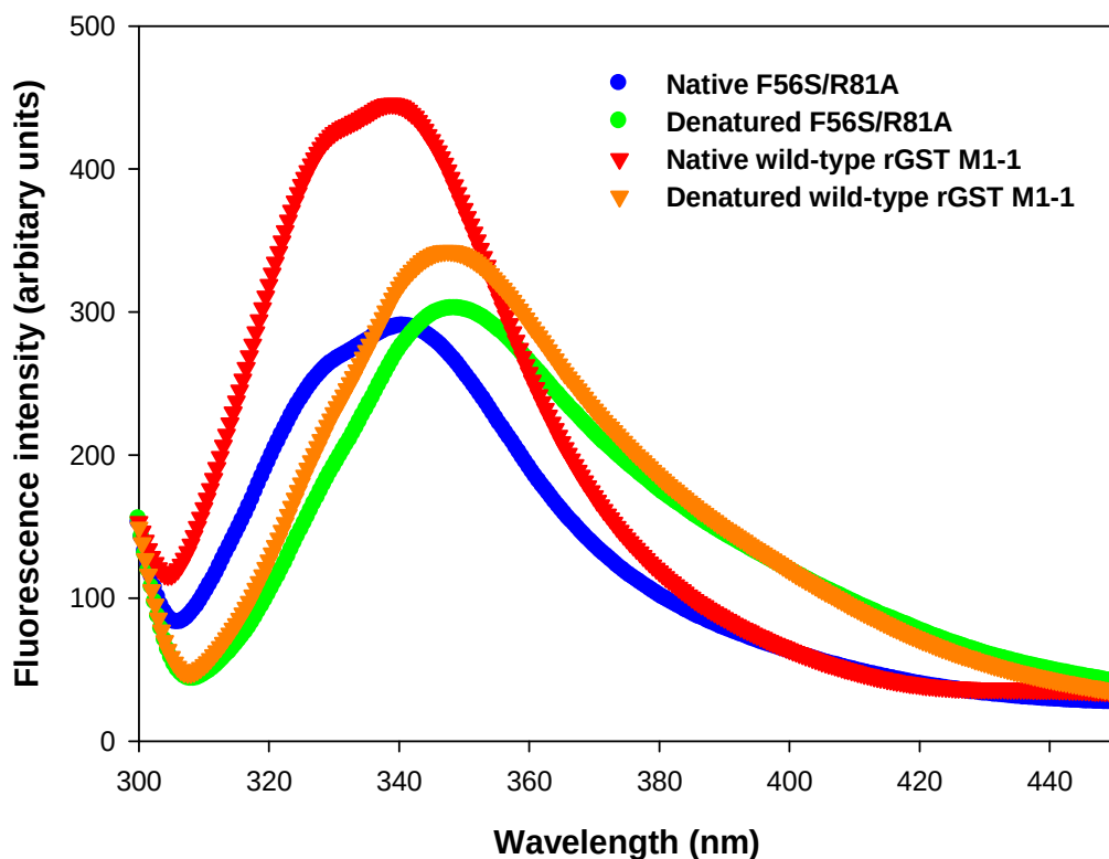
Figure 3-8: Fluorescence emission spectra of wild-type GST M1-1 and F56S/R81A monomeric mutant.
