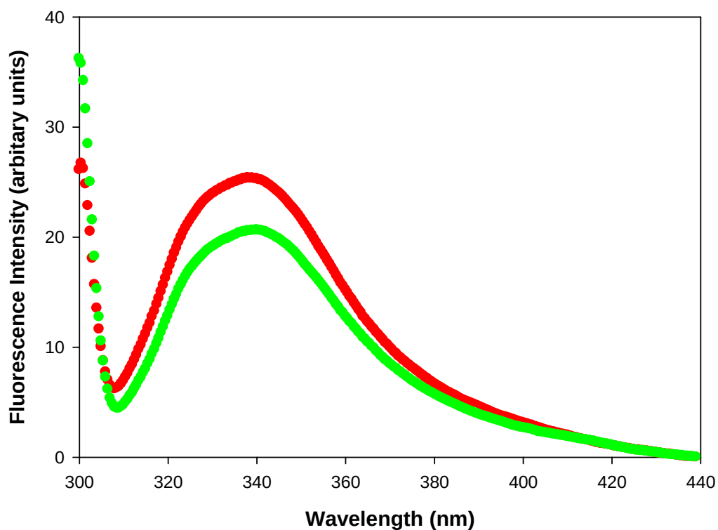
Figure 3-10: Recovery of the F56S/R81A rGST M1.
