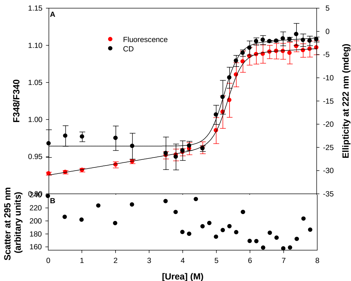
Figure 3-11: Urea-induced equilibrium unfolding of F56S/R81A.
