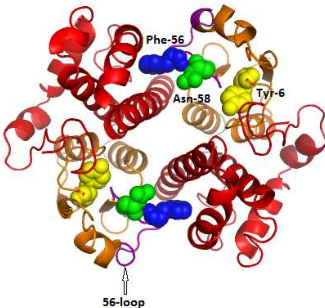
Figure 4-1: Important residues at the G-site of rGST M1-1.
