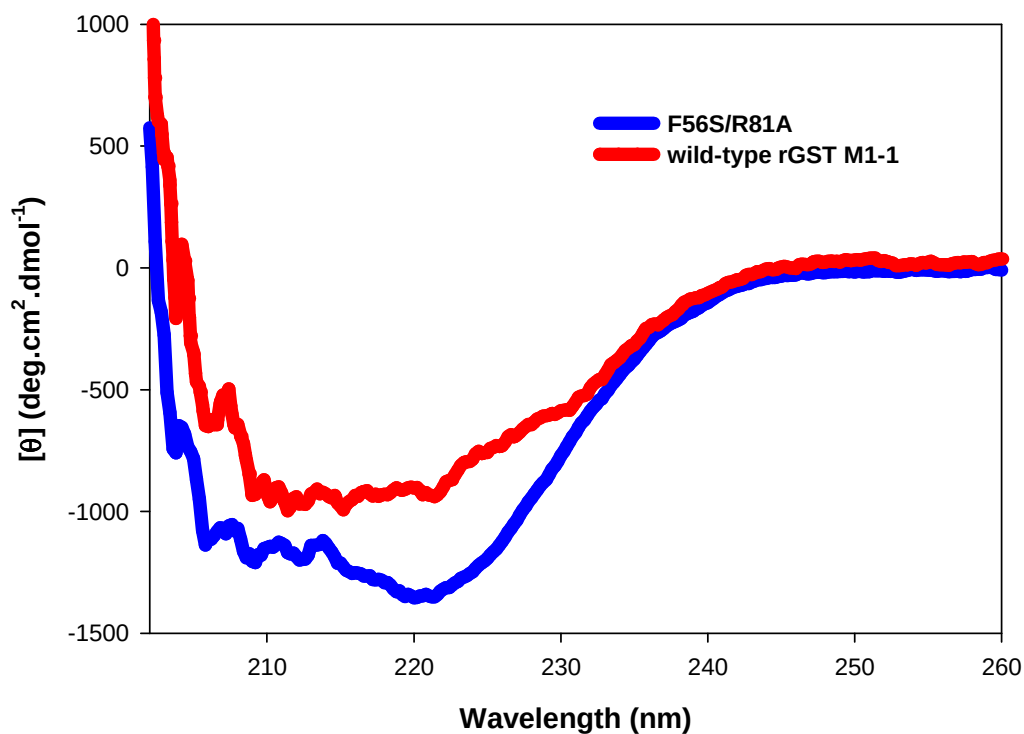
Figure 3-7: Far-UV circular dichroism spectra of native wild-type rGST M1-1 and F56S/R81A rGST M1.
