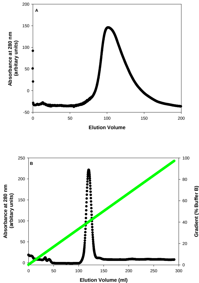
Figure 3-3: Elution profiles of wild-type rGST M1-1 and F56S/R81A rGST M1.
