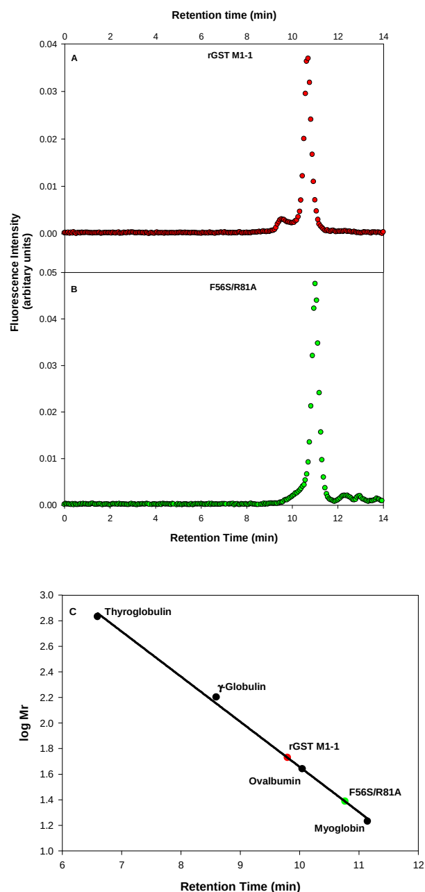
Figure 3-5: SE-HPLC elution profile of rGST M1-1 and F56S/R81A monomeric mutant.
