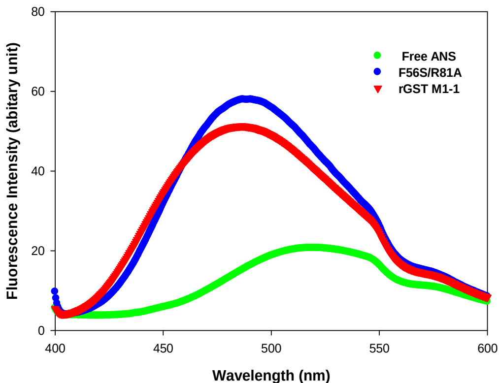
Figure 3-9: Fluorescence emission spectra of ANS bound to wild-type rGST M1-1 and the F56S/R81A rGST M1 mutant.
