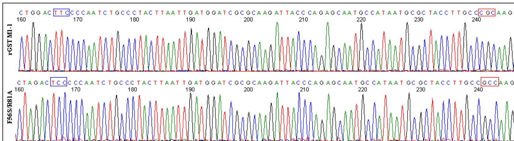
Figure 3-1: A portion of the nucleotide sequencing chromatograms for the rGST M1-1 cDNA ORF indicating the codon mutations responsible for the corresponding F56S/R81A rGST M1-1 double mutant protein sequence.
