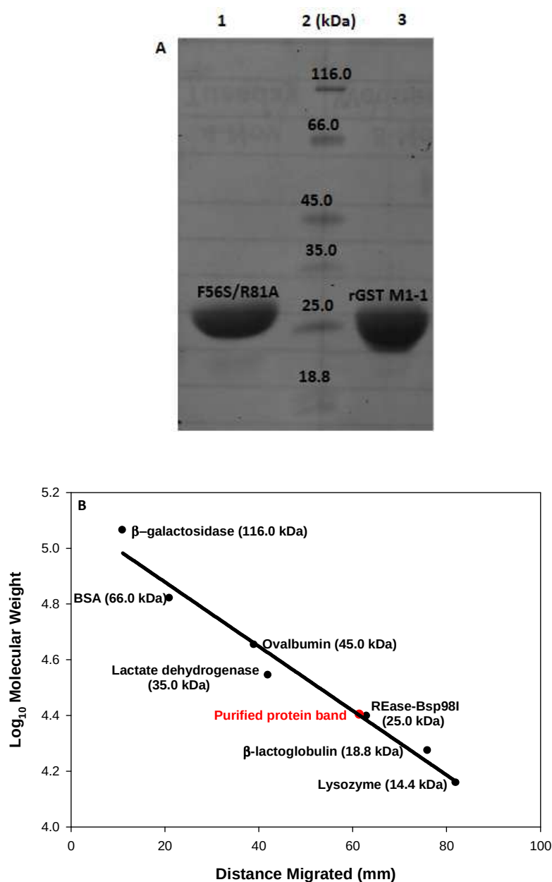
Figure 3-4: SDS-PAGE analysis of purified proteins.
