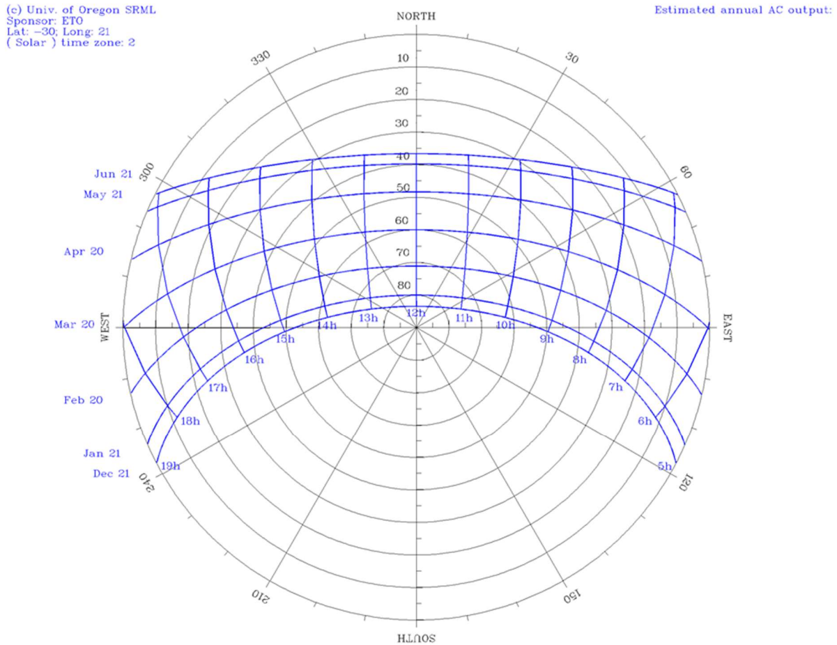
Figure 28: A solar position chart, calibrated to 30° South, 21° East. Source: University of Oregon Solar Radiation Monitoring Laboratory ( http://solardat.uoregon.edu ).
