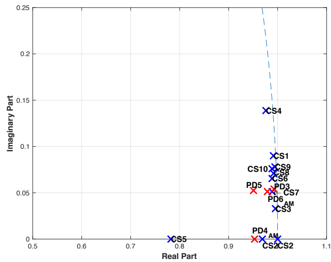
Figure 4.2.8: Pole-zero plot between control subjects (blue) and PD patients after medication (red) using X-axis data - conjugate counterparts are mirror image.
