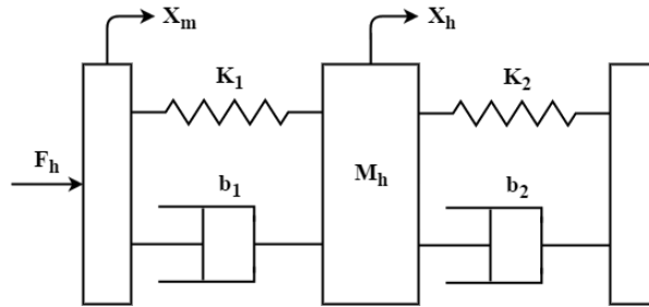
Figure 3.1.3: Spring-damper human arm/hand model [46].
