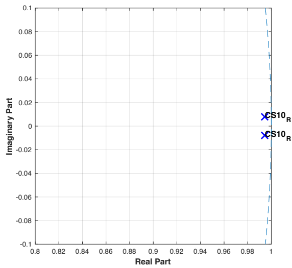
Figure E19: Pole-zero plot for control subject 10 using R^2 data.
