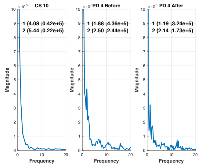
Figure F26: A comparison FFT plots between PD patient 4 (before and after medication) and control subject 10 using R^2 data.
