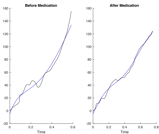
Figure D32: Measured (black) and simulated model (blue) output of PD patient 3 before and after medication with 82.1% and 90.6% best fit respectively.
