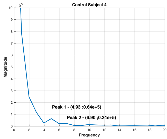
Figure F4: A FFT plot of control subject 4 using R^2 data.
