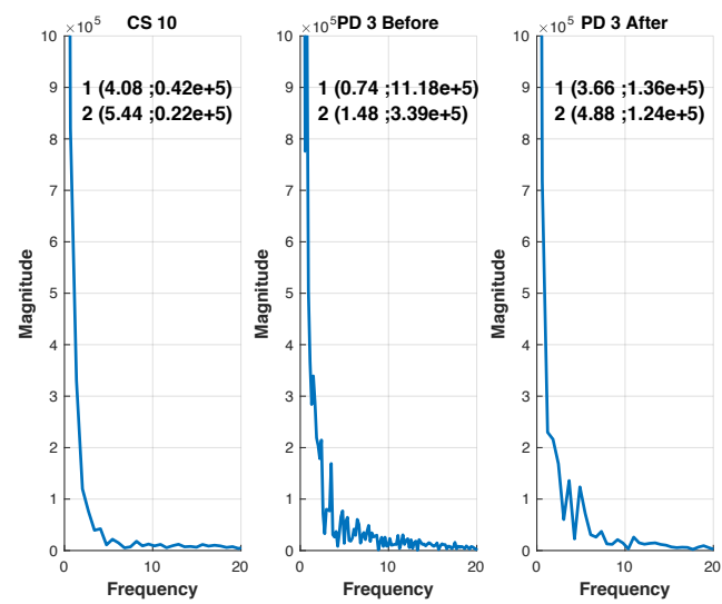
Figure F24: A comparison FFT plots between PD patient 3 (before and after medication) and control subject 10 using R^2 data.
