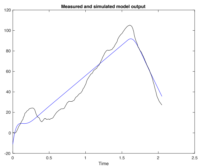
Figure D64: Measured (black) and simulated model (blue) output of ET patient 3 with 70.7% best fit.
