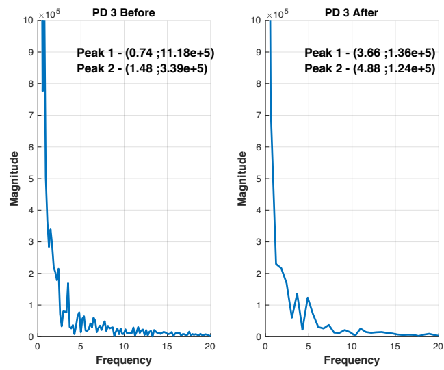
Figure F23: A FFT plot of PD patient 3 (before and after medication) using R^2 data.
