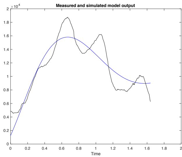
Figure E26: Measured (black) and simulated model (blue) output of control subject 8 with 58.3% best fit.
