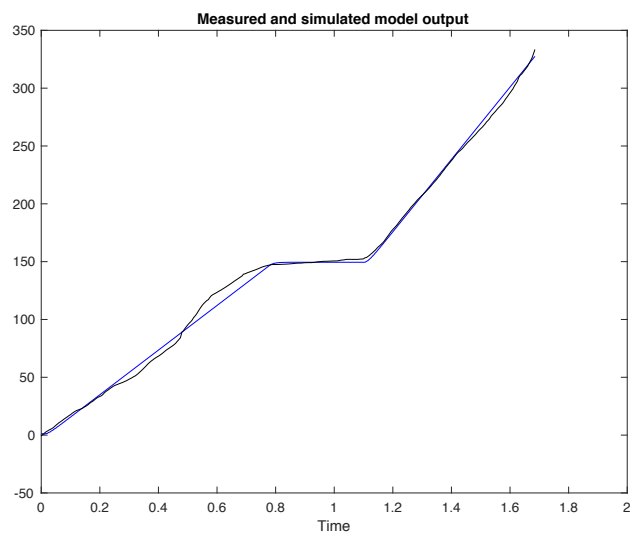
Figure C18: Measured (black) and simulated model (blue) output of control subject 9 with 94.7% best fit.
