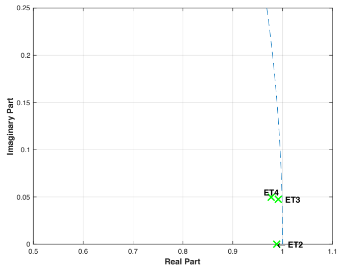
Figure 4.1.2: Combined X-axis data pole-zero plot for ET patients (green) - conjugate counterparts are mirror image.
