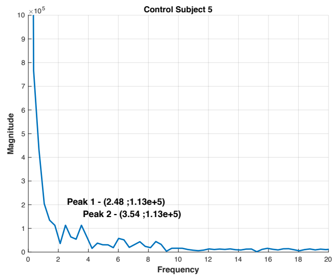
Figure F5: A FFT plot of control subject 5 using R^2 data.
