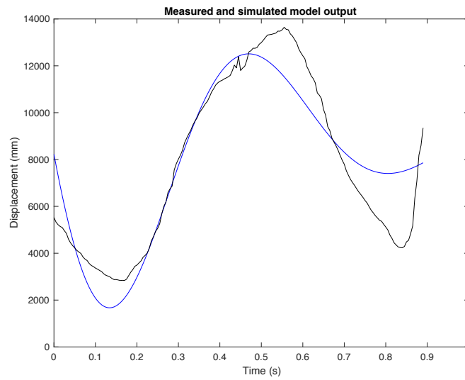
Figure 4.3.1: An example of a R^2 measured data plotted against simulated output data from the circle pattern with 63% best fit.
