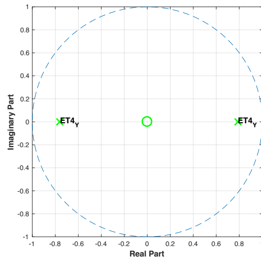
Figure C73: Pole-zero plot of ET patient 4 using Y-axis data.
