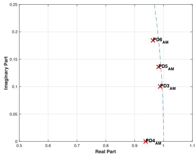
Figure 4.2.14: Combined Y-axis data pole-zero plot for PD patients after medication (red) - conjugate counterparts are mirror image.
