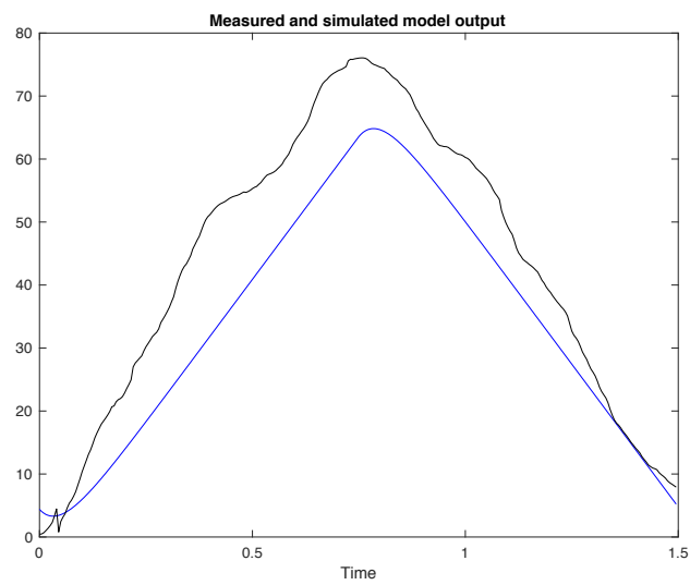
Figure D68: Measured (black) and simulated model (blue) output of ET patient 5 with 53.0% best fit.
