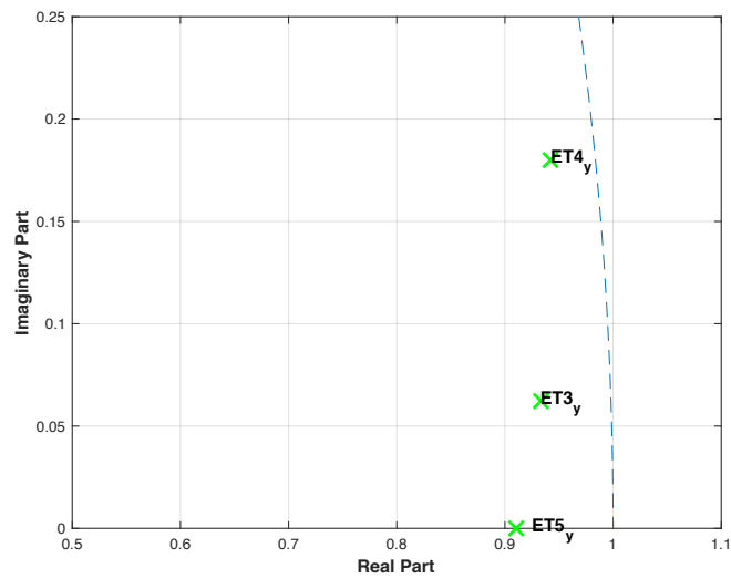
Figure 4.2.12: Combined Y-axis data pole-zero plot for ET patients (green) - conjugate counterparts are mirror image.
