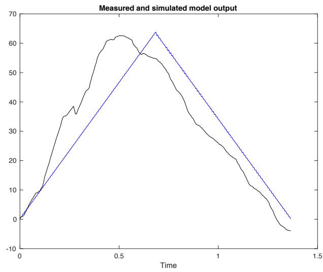
Figure D44: Measured (black) and simulated model (blue) output of control subject 3 with 51.9% best fit.
