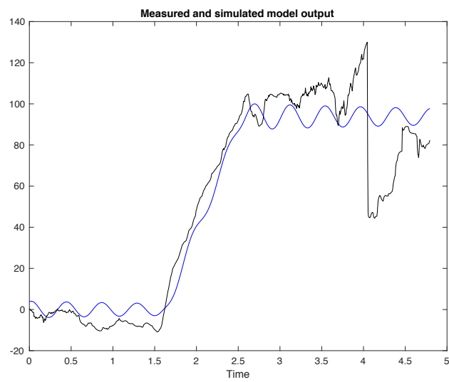
Figure C58: Measured (black) and simulated model (blue) output of control subject 6 with 69.2% best fit.
