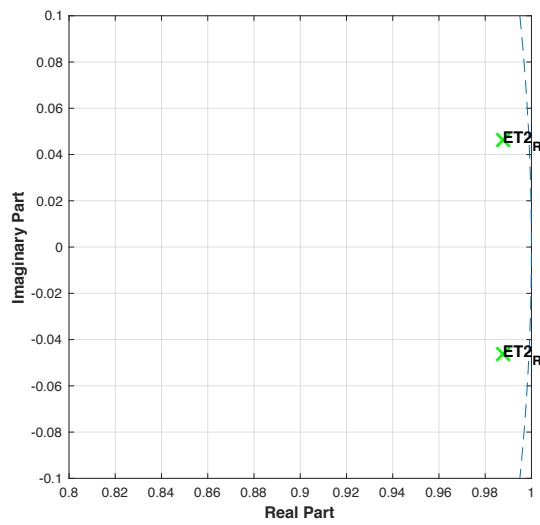
Figure E23: Pole-zero plot of ET patient 2 using R^2 data.
