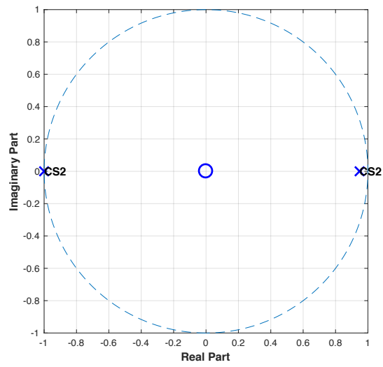
Figure C3: Pole-zero plot of control subject 2 using X-axis data.
