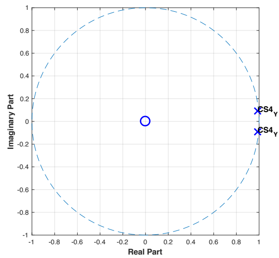
Figure C53: Pole-zero plot of control subject 4 using Y-axis data.
