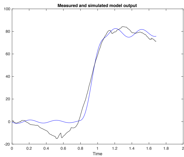
Figure C64: Measured (black) and simulated model (blue) output of control subject 9 with 84.2% best fit.
