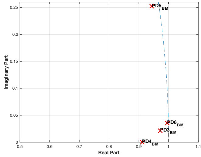
Figure 4.2.4: Combined X-axis data pole-zero plot for PD patients before medication (red) - conjugate counterparts are mirror image.
