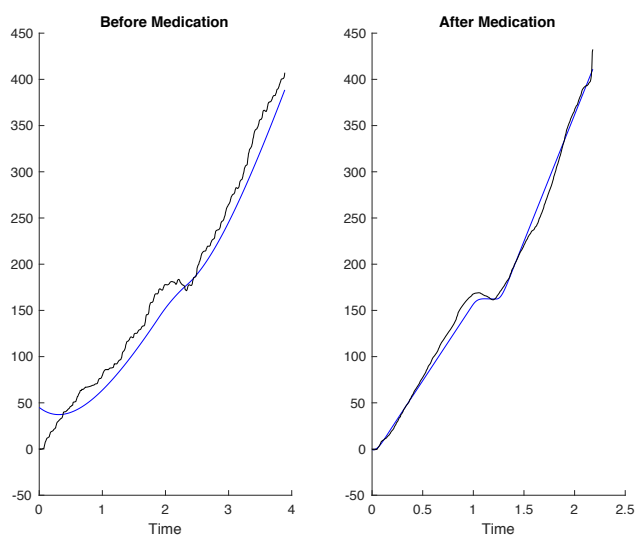
Figure C40: Measured (black) and simulated model (blue) output of PD patient 6 before and after medication with 82.0% and 92.8% best fit respectively.
