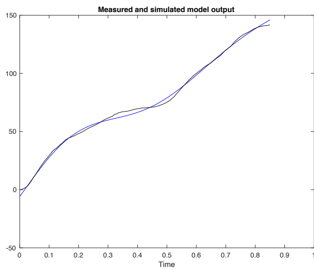
Figure D14: Measured (black) and simulated model (blue) output of control subject 7 with 94.7% best fit.
