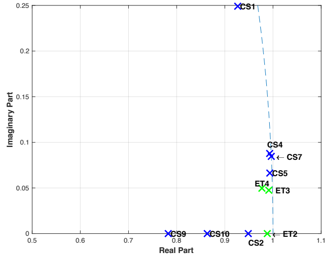
Figure 4.1.5: Pole-zero plot between the control subjects (blue) and ET patients (green) using X-axis data - conjugate counterparts are mirror image.
