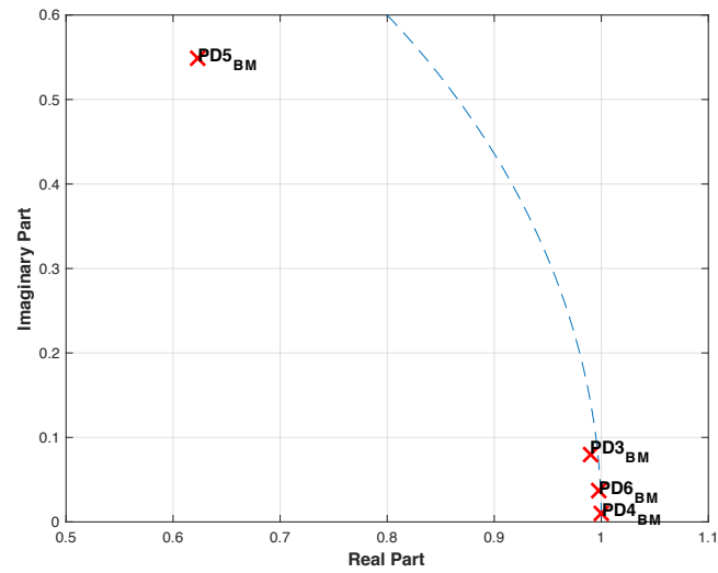
Figure 4.2.13: Combined Y-axis data pole-zero plot for PD patients before medication (red) - conjugate counterparts are mirror image.
