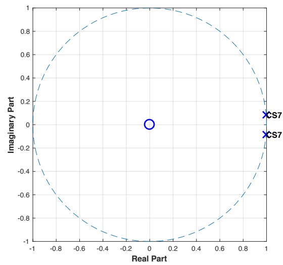
Figure C13: Pole-zero plot of control subject 7 using X-axis data.
