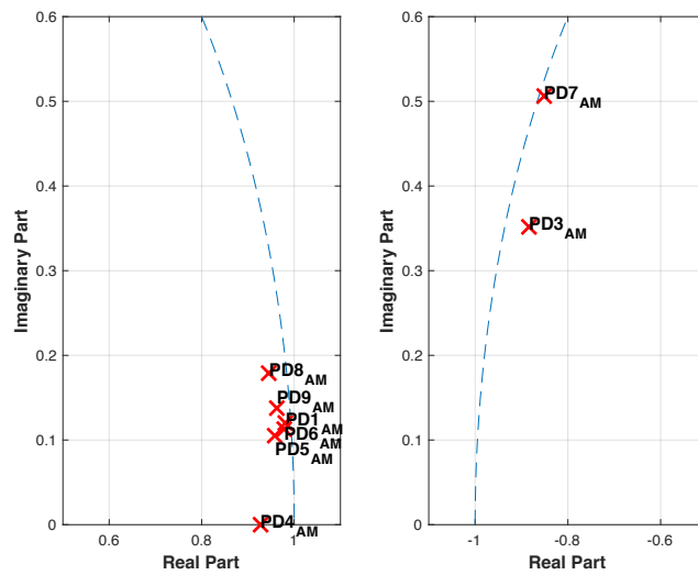
Figure 4.1.13: Combined Y-axis data pole-zero plot for PD patients after medication (red) - conjugate counterparts are mirror image.
