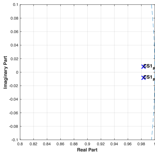
Figure E1: Pole-zero plot for control subject 1 using R^2 data.
