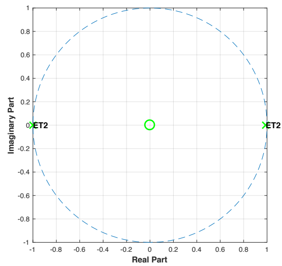
Figure C23: Pole-zero plot of ET patient 2 using X-axis data.
