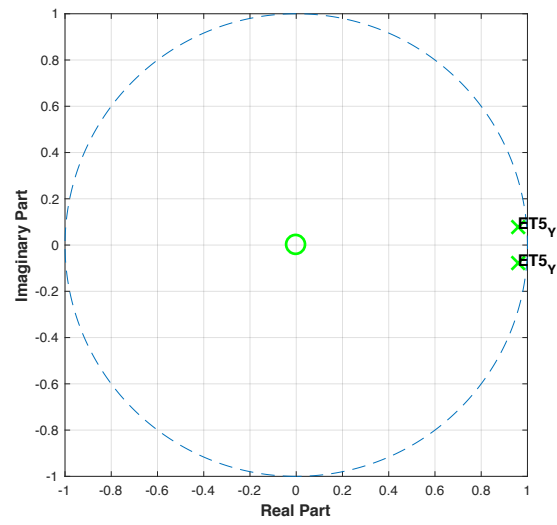
Figure C75: Pole-zero plot of ET patient 5 using Y-axis data.
