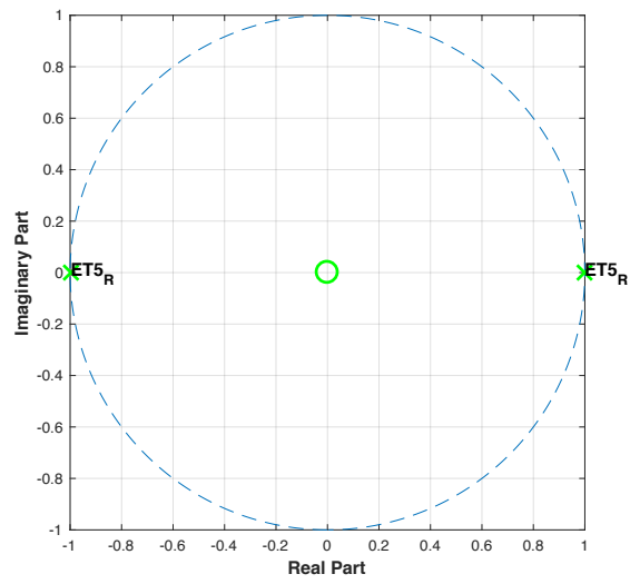
Figure E29: Pole-zero plot of ET patient 5 using R^2 data.
