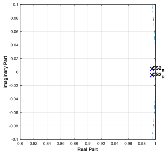
Figure E3: Pole-zero plot for control subject 2 using R^2 data.
