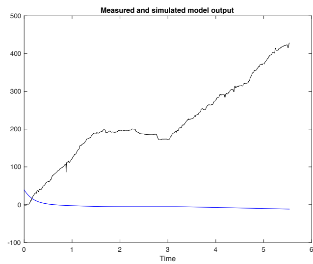
Figure C22: Measured (black) and simulated model (blue) output of ET patient 1 with - 134.8% best fit - omitted from the analysis.
