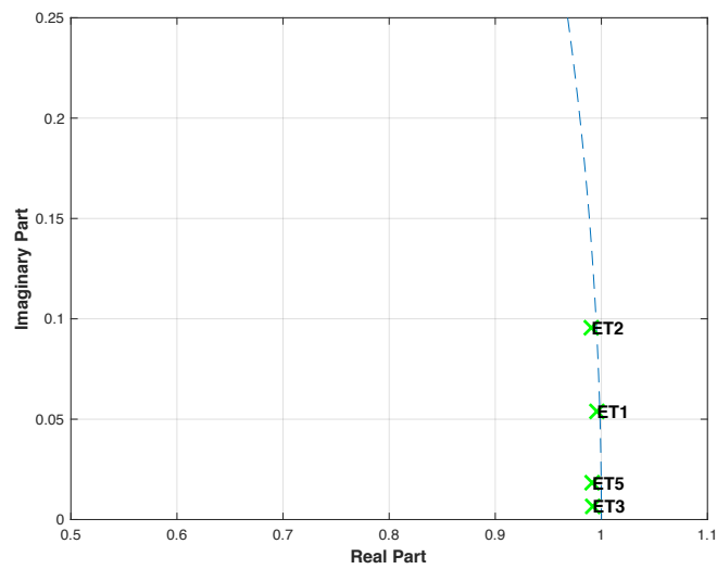
Figure 4.2.3: Combined X-axis data pole-zero plot for ET patients (green) - conjugate counterparts are mirror image.
