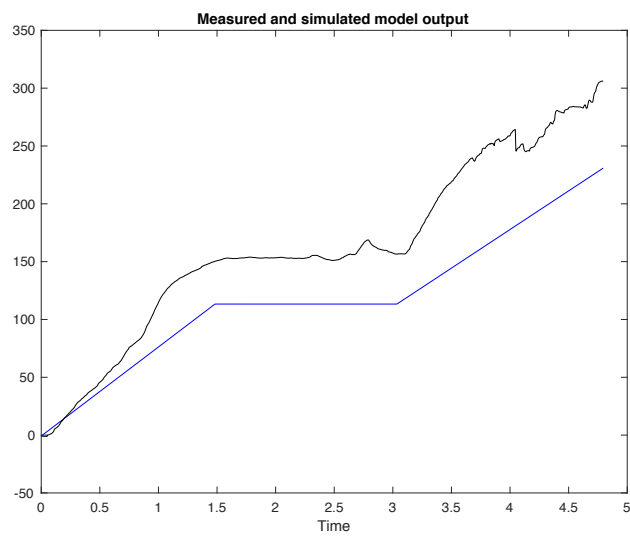
Figure C12: Measured (black) and simulated model (blue) output of control subject 6 with 33.9% best fit - omitted from the analysis.
