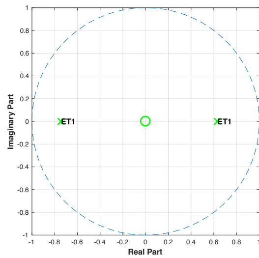
Figure C21: Pole-zero plot of ET patient 1 using X-axis data.
