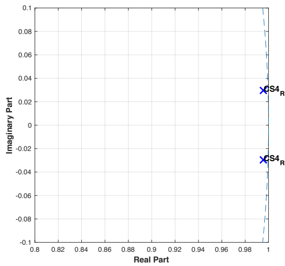
Figure E7: Pole-zero plot for control subject 4 using R^2 data.
