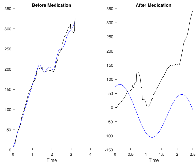
Figure C34: Measured (black) and simulated model (blue) output of PD patient 3 before and after medication with 89.7% and -89.6% (omitted from the analysis) best fit respectively.
