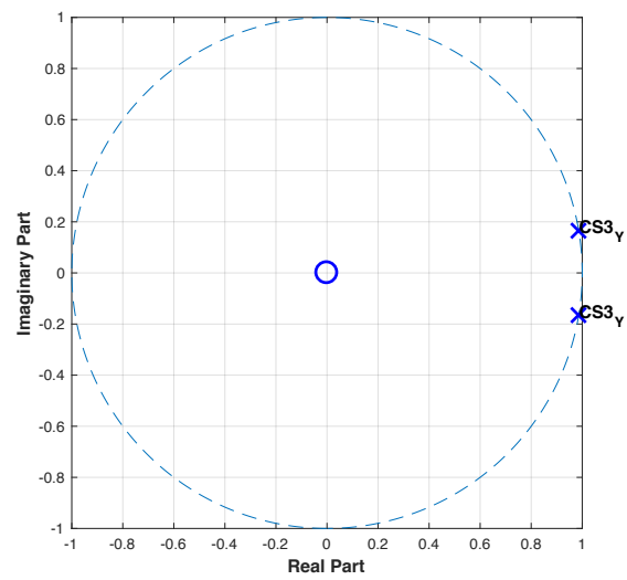
Figure C51: Pole-zero plot of control subject 3 using Y-axis data.
