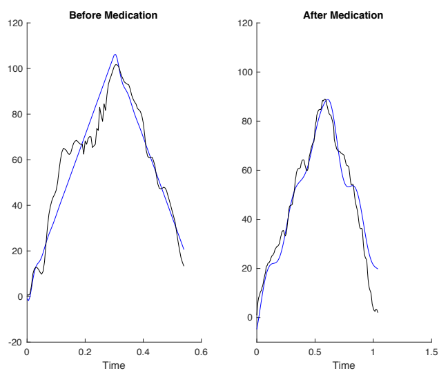
Figure D76: Measured (black) and simulated model (blue) output of PD patient 5 before and after medication with 71.3% and 73.1% best fit respectively.
