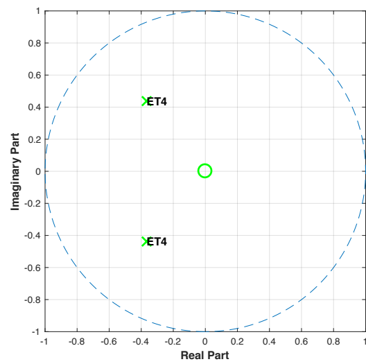
Figure D27: Pole-zero plot of ET patient 4 using X-axis data.
