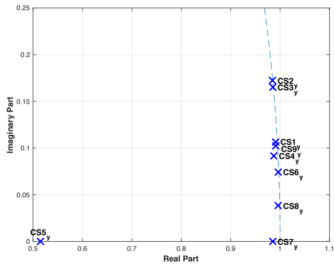
Figure 4.1.10: Combined Y-axis data pole-zero plot for control subjects (blue) - conjugate counterparts are mirror image.
