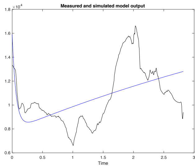
Figure E10: Measured (black) and simulated model (blue) output of control subject 5 with 15.5% best fit - omitted from the analysis.
