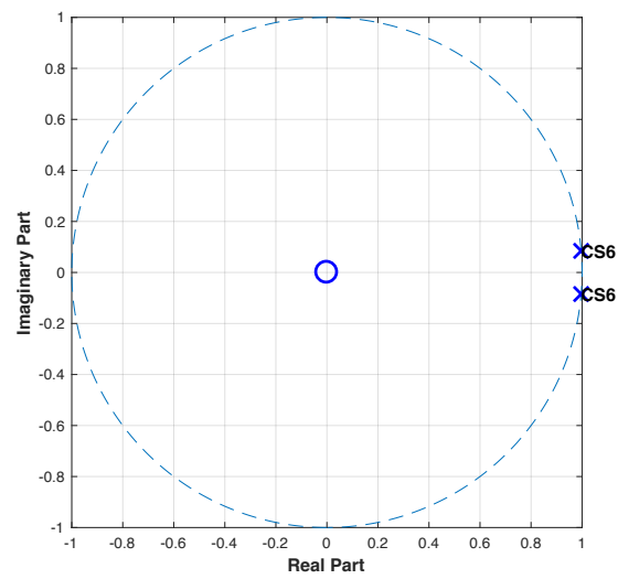
Figure C11: Pole-zero plot of control subject 6 using X-axis data.
