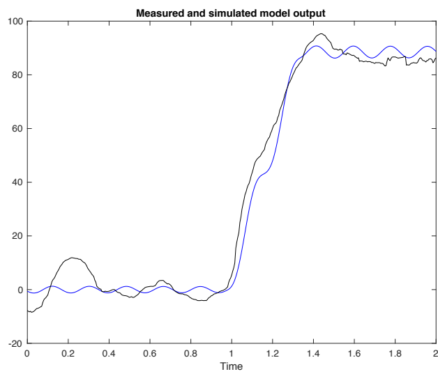
Figure C50: Measured (black) and simulated model (blue) output of control subject 2 with 86.9% best fit.
