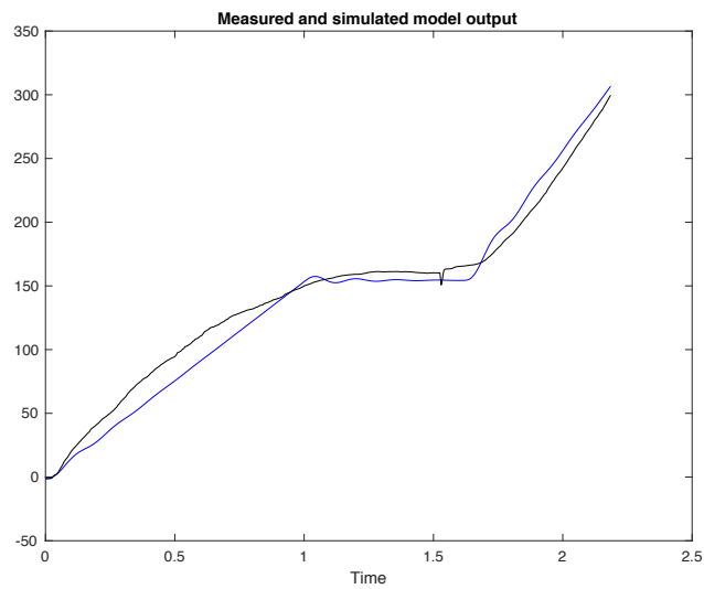
Figure C2: Measured (black) and simulated model (blue) output of control subject 1 with 82.0% best fit.
