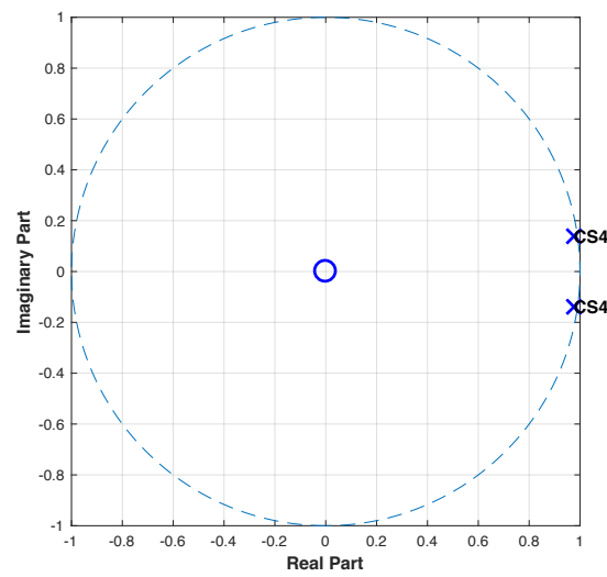
Figure D7: Pole-zero plot of control subject 4 using X-axis data.
