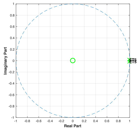
Figure D29: Pole-zero plot of ET patient 5 using X-axis data.
