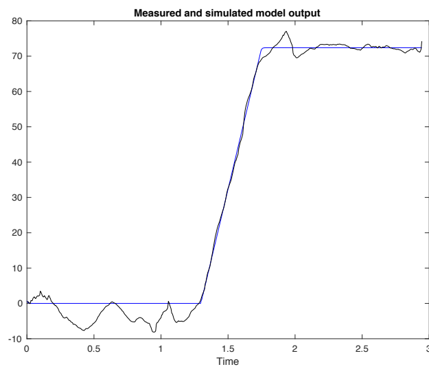
Figure C56: Measured (black) and simulated model (blue) output of control subject 5 with 91.9% best fit.
