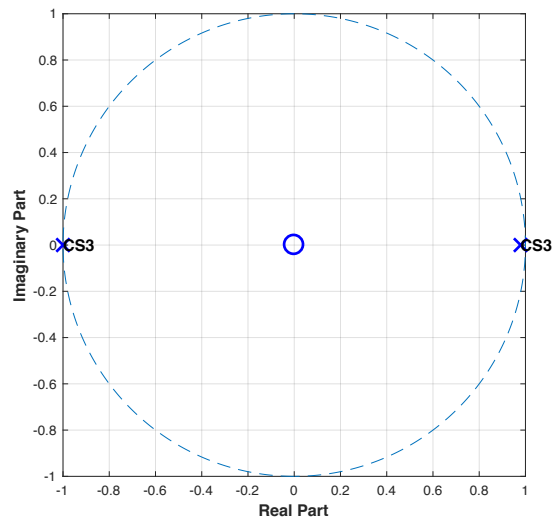
Figure C5: Pole-zero plot of control subject 3 using X-axis data.
