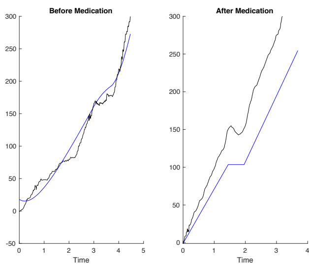
Figure C36: Measured (black) and simulated model (blue) output of PD patient 4 before and after medication with 82.6% and -39.2% (omitted from the analysis) best fit respectively.
