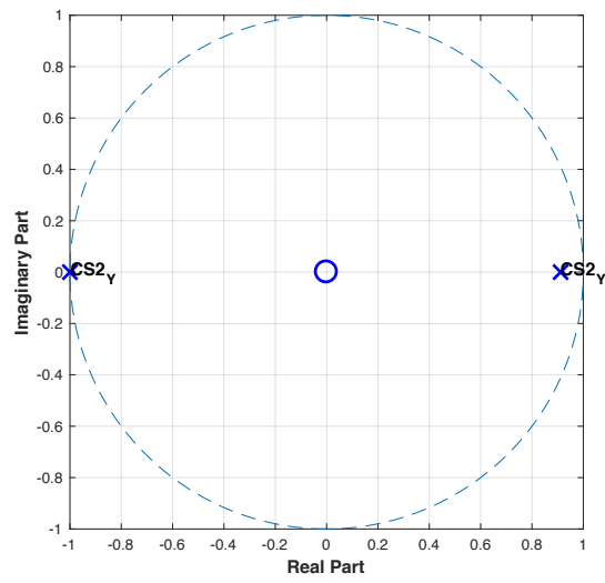
Figure D41: Pole-zero plot of control subject 2 using Y-axis data.
