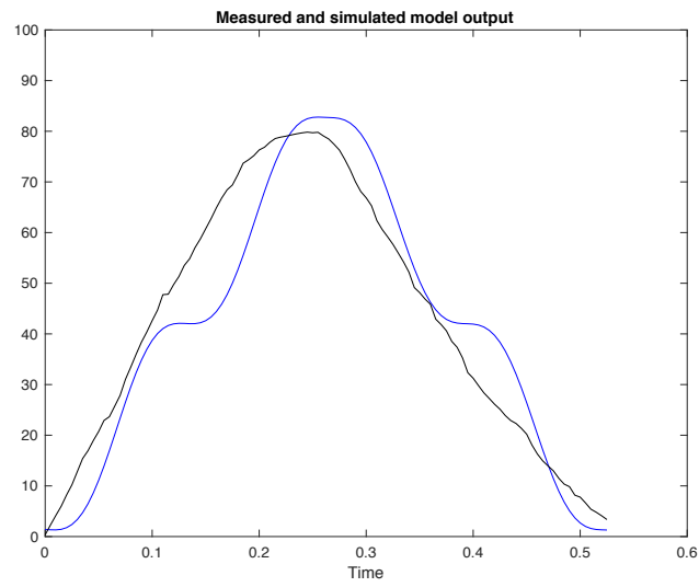
Figure D54: Measured (black) and simulated model (blue) output of control subject 8 with 63.9% best fit.
