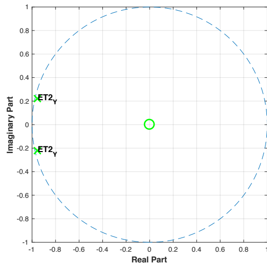
Figure C69: Pole-zero plot of ET patient 2 using Y-axis data.
