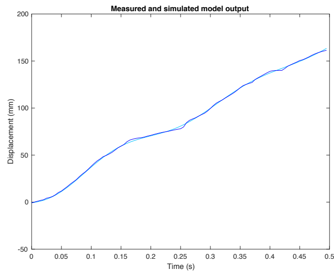
Figure 4.2.1: An example of an X-axis measured data plotted against simulated output data from the triangle pattern with 98% best fit.
