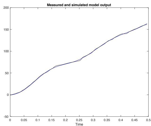
Figure D8: Measured (black) and simulated model (blue) output of control subject 4 with 98.0% best fit.
