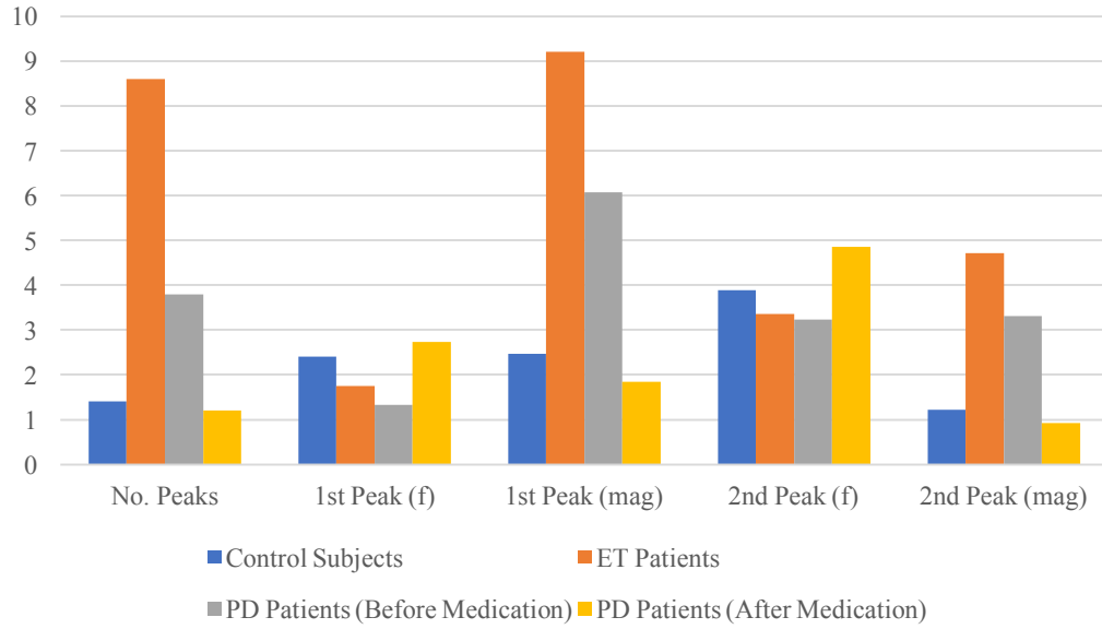
Figure 4.4.4: Average feature values shown graphically from tables 4.4.1, 4.4.2, 4.4.3 and 4.4.4.
