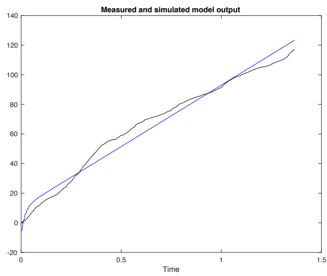
Figure D10: Measured (black) and simulated model (blue) output of control subject 5 with 86.3% best fit.
