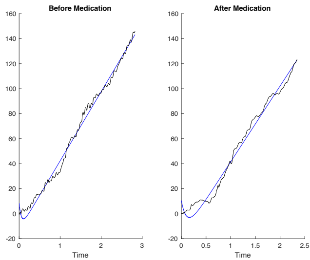
Figure D34: Measured (black) and simulated model (blue) output of PD patient 4 before and after medication with 91.0% and 87.16% best fit respectively.
