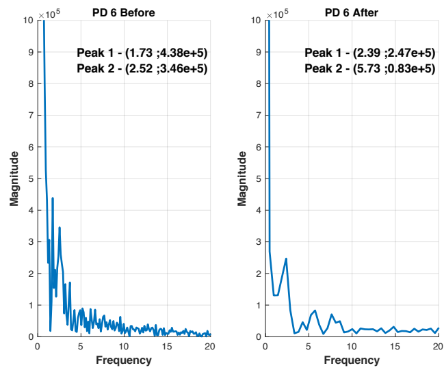
Figure F29: A FFT plot of PD patient 6 (before and after medication) using R^2 data.
