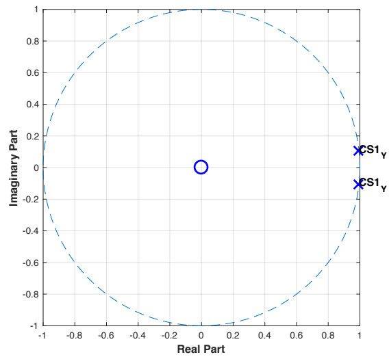
Figure C47: Pole-zero plot of control subject 1 using Y-axis data.
