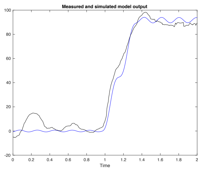
Figure C52: Measured (black) and simulated model (blue) output of control subject 3 with 85.4% best fit.
