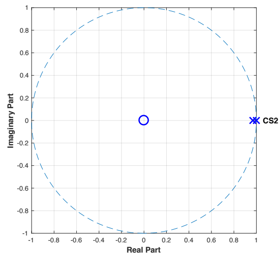
Figure D3: Pole-zero plot of control subject 2 using X-axis data.
