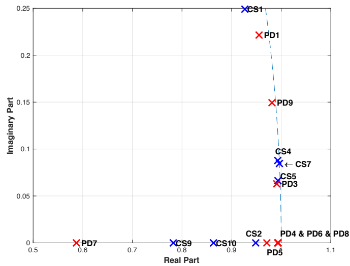
Figure 4.1.6: Pole-zero plot between control subjects (blue) and PD patients before medication (red) using X-axis data - conjugate counterparts are mirror image.
