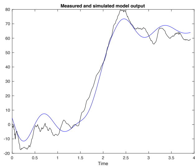
Figure C72: Measured (black) and simulated model (blue) output of ET patient 3 with 83.6% best fit.
