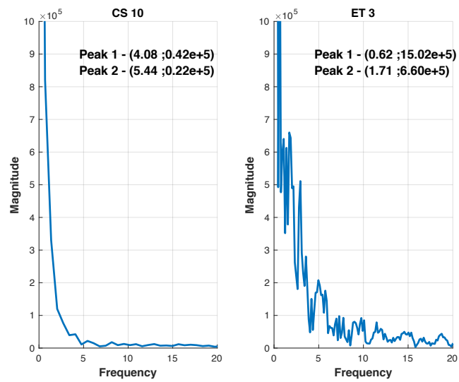
Figure F16: A comparison FFT plots between ET patient 3 and control subject 10 using R^2 data.
