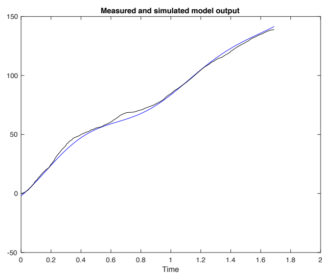
Figure D6: Measured (black) and simulated model (blue) output of control subject 3 with 94.2% best fit.
