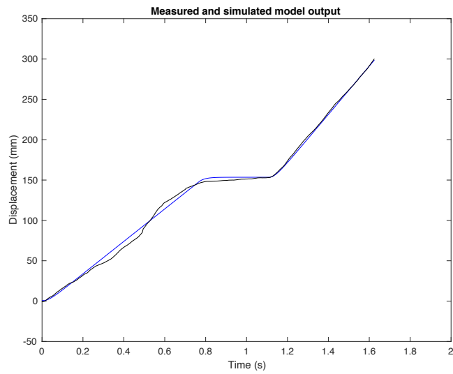
Figure 4.1: Measured (black) and simulated model (blue) output of control subject 10 with 95.0% best fit.
