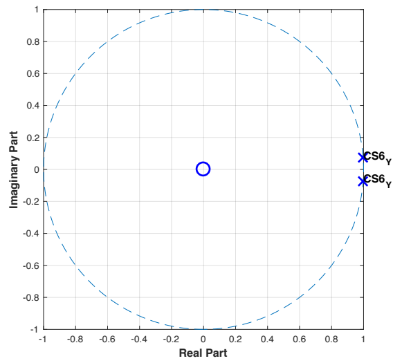
Figure C57: Pole-zero plot of control subject 6 using Y-axis data.
