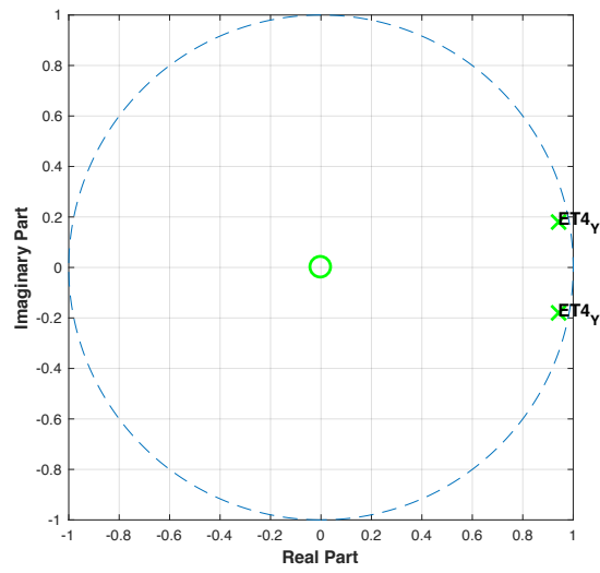
Figure D65: Pole-zero plot of ET patient 4 using Y-axis data.
