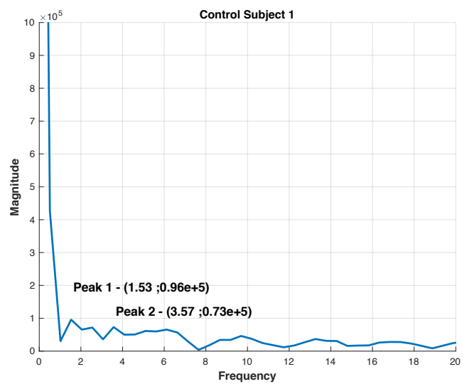
Figure F1: A FFT plot of control subject 1 using R^2 data.
