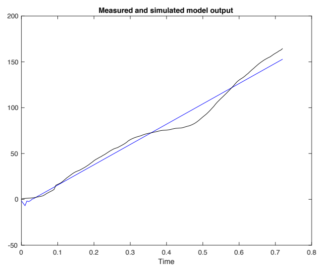
Figure D28: Measured (black) and simulated model (blue) output of ET patient 4 with 84.2% best fit.
