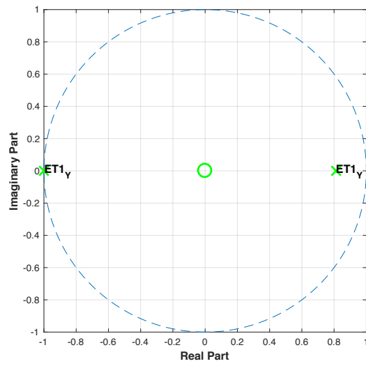
Figure D59: Pole-zero plot of ET patient 1 using Y-axis data.
