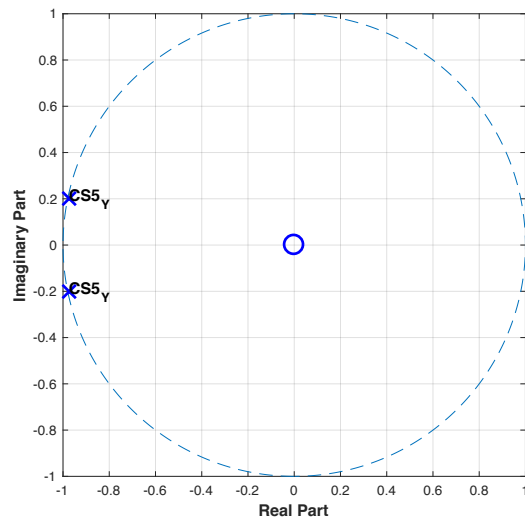
Figure D47: Pole-zero plot of control subject 5 using Y-axis data.
