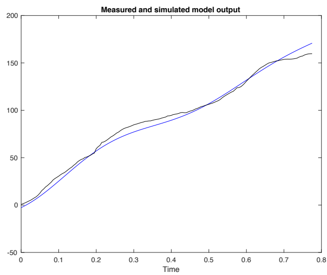
Figure D12: Measured (black) and simulated model (blue) output of control subject 6 with 89.7% best fit.
