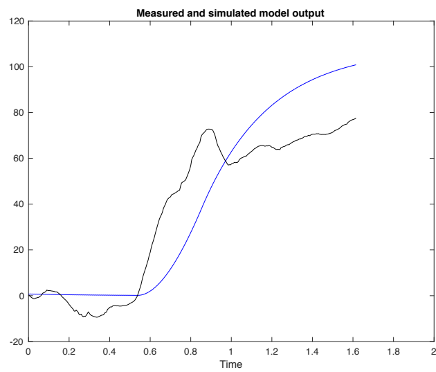
Figure C60: Measured (black) and simulated model (blue) output of control subject 7 with 84.1% best fit.
