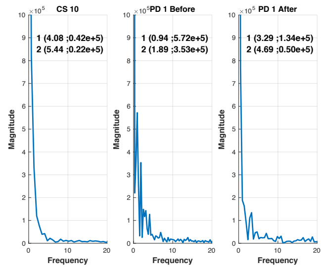
Figure F22: A comparison FFT plots between PD patient 1 (before and after medication) and control subject 10 using R^2 data.
