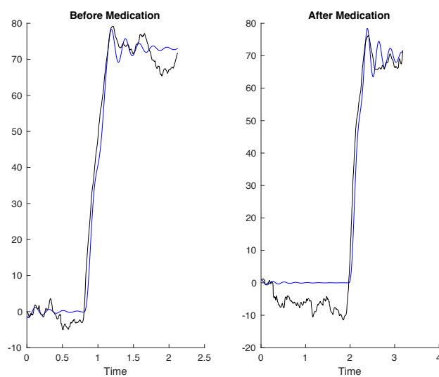
Figure C78: Measured (black) and simulated model (blue) output of PD patient 1 before and after medication with 87.6% and 81.0% best fit respectively.
