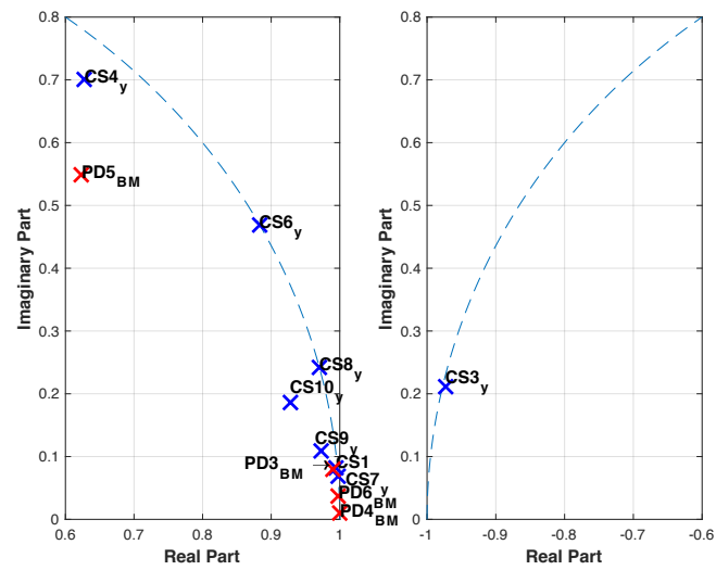
Figure 4.2.16: Pole-zero plot between control subjects (blue) and PD patients before medication (red) using Y-axis data - conjugate counterparts are mirror image.
