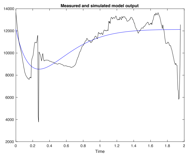
Figure E2: Measured (black) and simulated model (blue) output of control subject 1 with 27.6% best fit - omitted from the analysis.
