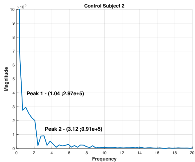
Figure F2: A FFT plot of control subject 2 using R^2 data.
