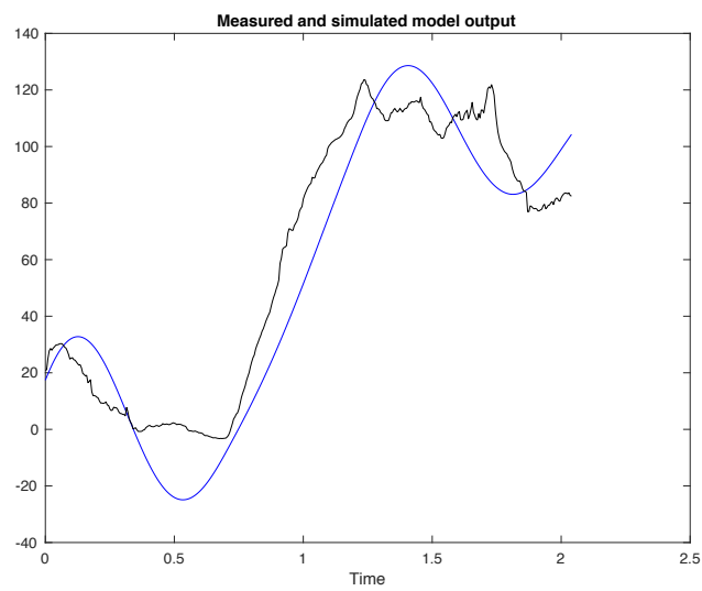
Figure C62: Measured (black) and simulated model (blue) output of control subject 8 with 64.5% best fit.
