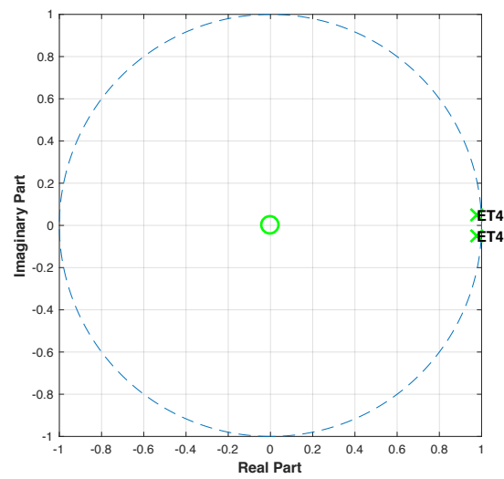
Figure C27: Pole-zero plot of ET patient 4 using X-axis data.
