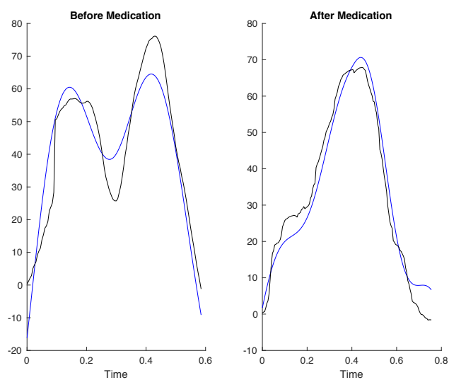
Figure D72: Measured (black) and simulated model (blue) output of PD patient 3 before and after medication with 60.6% and 79.8% best fit respectively.
