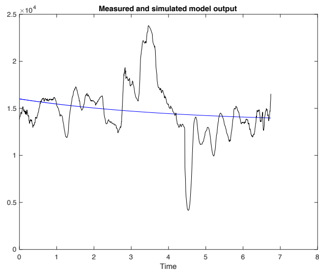
Figure E30: Measured (black) and simulated model (blue) output of ET patient 5 with 2.0% best fit - omitted from the analysis.
