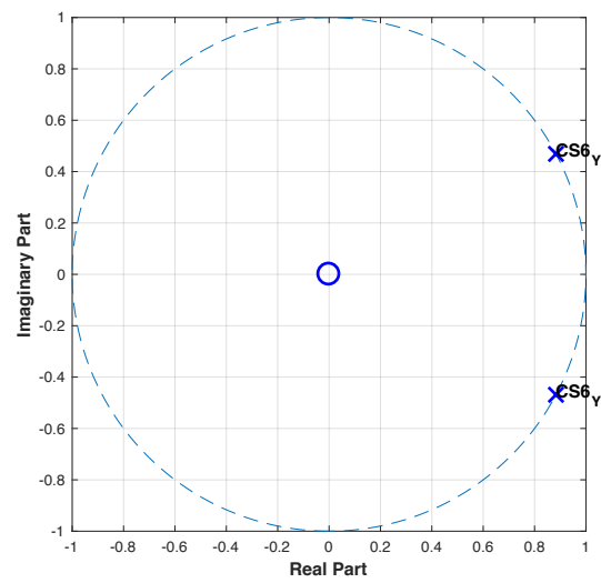
Figure D49: Pole-zero plot of control subject 6 using Y-axis data.
