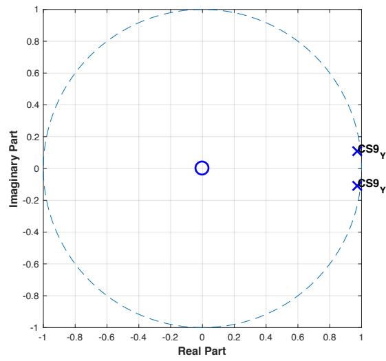
Figure D55: Pole-zero plot of control subject 9 using Y-axis data.
