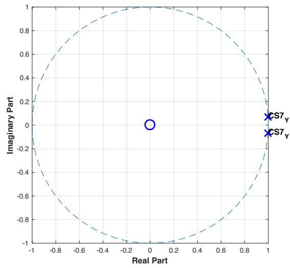
Figure D51: Pole-zero plot of control subject 7 using Y-axis data.
