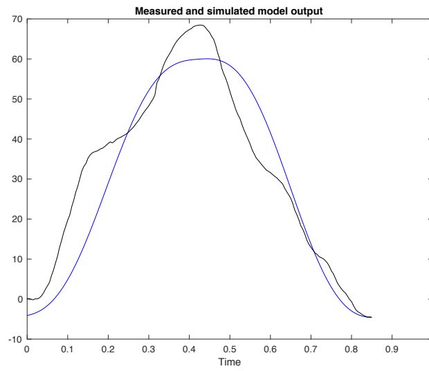
Figure D52: Measured (black) and simulated model (blue) output of control subject 7 with 62.5% best fit.
