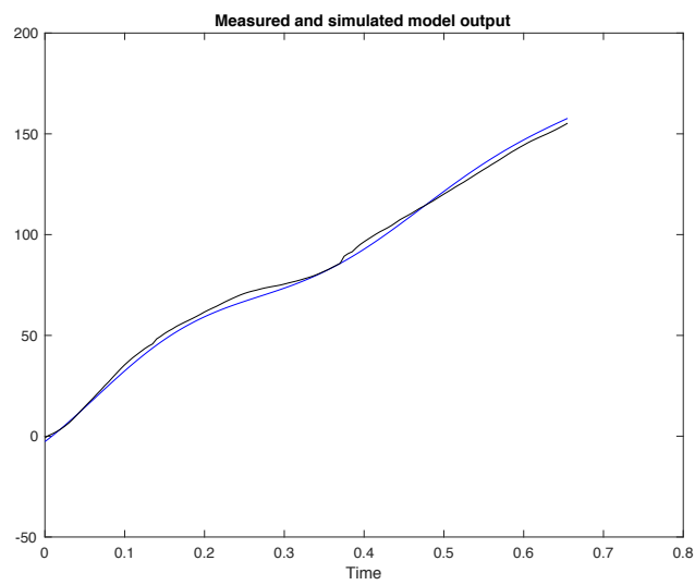
Figure D20: Measured (black) and simulated model (blue) output of control subject 10 with 94.3% best fit.
