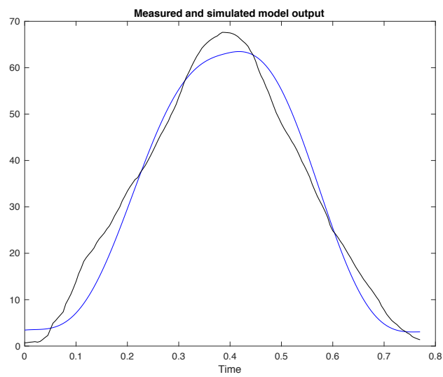
Figure D40: Measured (black) and simulated model (blue) output of control subject 1 with 81.4% best fit.
