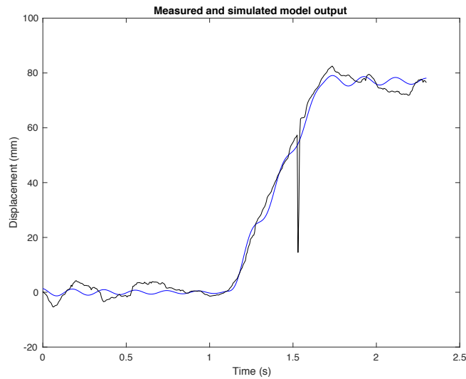
Figure 4.1.9: An example of a Y-axis measured data plotted against simulated output data from the step-function pattern with 90.2% best fit.
