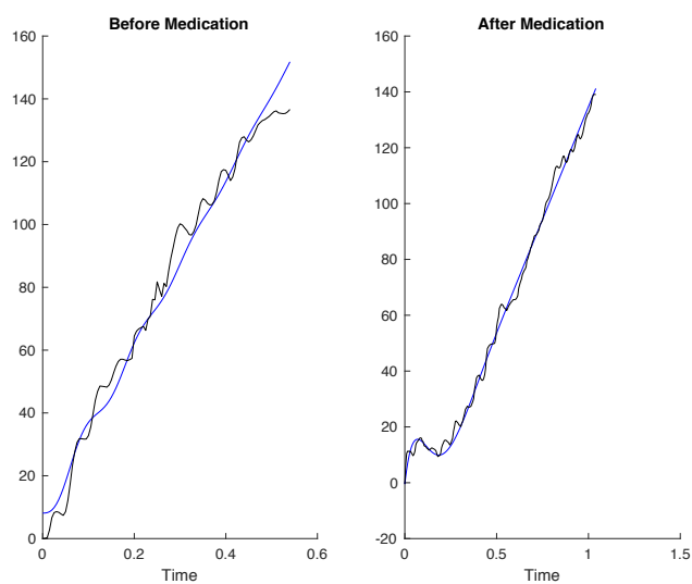
Figure D36: Measured (black) and simulated model (blue) output of PD patient 5 before and after medication with 86.2% and 93.6% best fit respectively.
