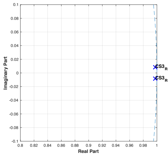
Figure E5: Pole-zero plot for control subject 3 using R^2 data.
