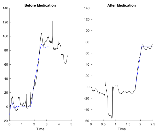
Figure C80: Measured (black) and simulated model (blue) output of PD patient 3 before and after medication with 77.5% and 55.7% best fit respectively.
