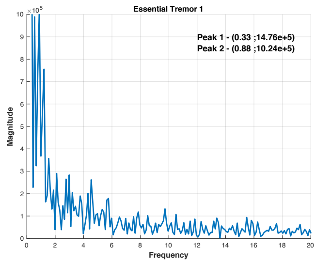
Figure F11: A FFT plot of ET patient 1 using R^2 data.
