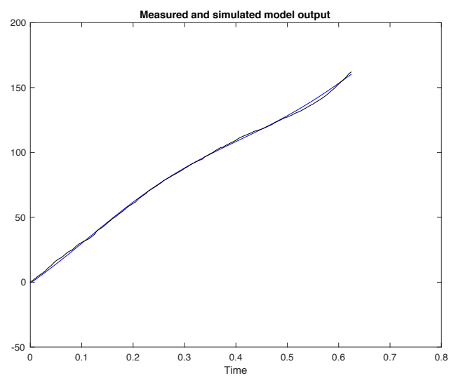
Figure D22: Measured (black) and simulated model (blue) output of ET patient 1 with 97.2% best fit.
