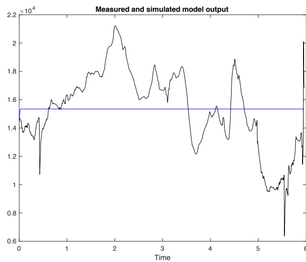
Figure E12: Measured (black) and simulated model (blue) output of control subject 6 with -1.3% best fit - omitted from the analysis.
