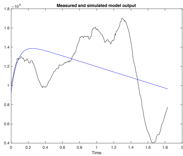
Figure E18: Measured (black) and simulated model (blue) output of control subject 9 with 7.1% best fit - omitted from the analysis.
