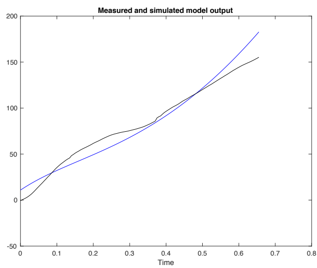
Figure D4: Measured (black) and simulated model (blue) output of control subject 2 with 76.5% best fit.
