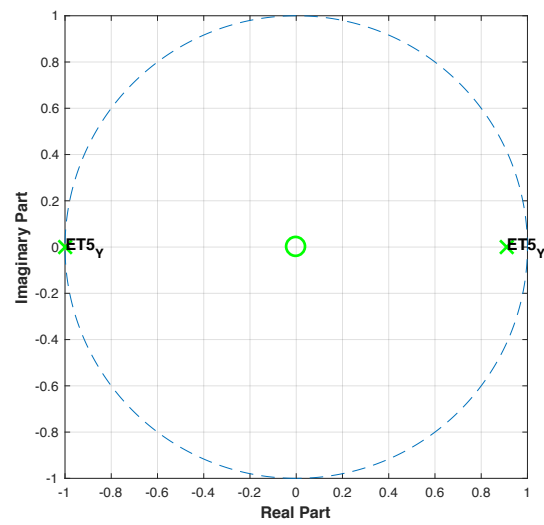
Figure D67: Pole-zero plot of ET patient 5 using Y-axis data.
