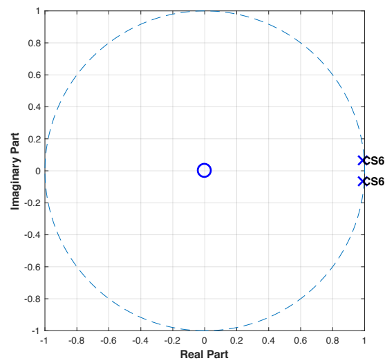
Figure D11: Pole-zero plot of control subject 6 using X-axis data.
