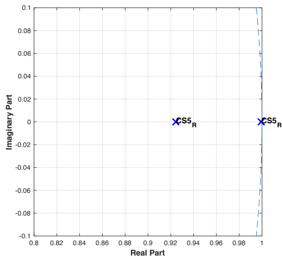
Figure E9: Pole-zero plot for control subject 5 using R^2 data.
