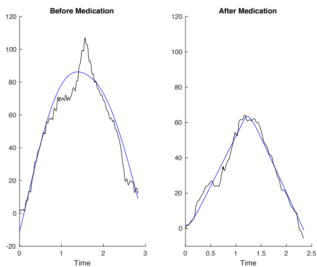
Figure D74: Measured (black) and simulated model (blue) output of PD patient 4 before and after medication with 71.3% and 82.5% best fit respectively.
