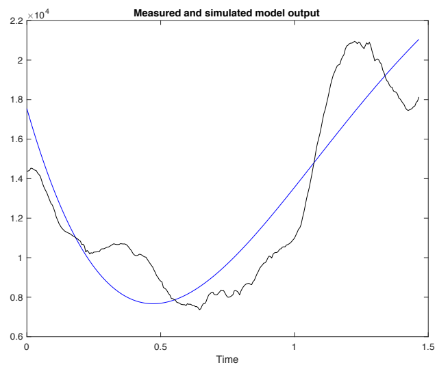
Figure E20: Measured (black) and simulated model (blue) output of control subject 10 with 55.1% best fit.
