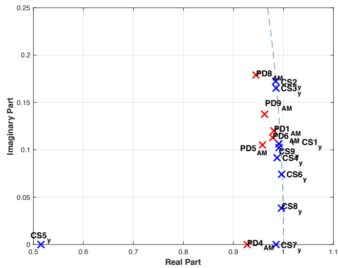
Figure 4.1.16: Pole-zero plot between control subjects (blue) and PD patients after medication (red) using Y-axis data - conjugate counterparts are mirror image.
