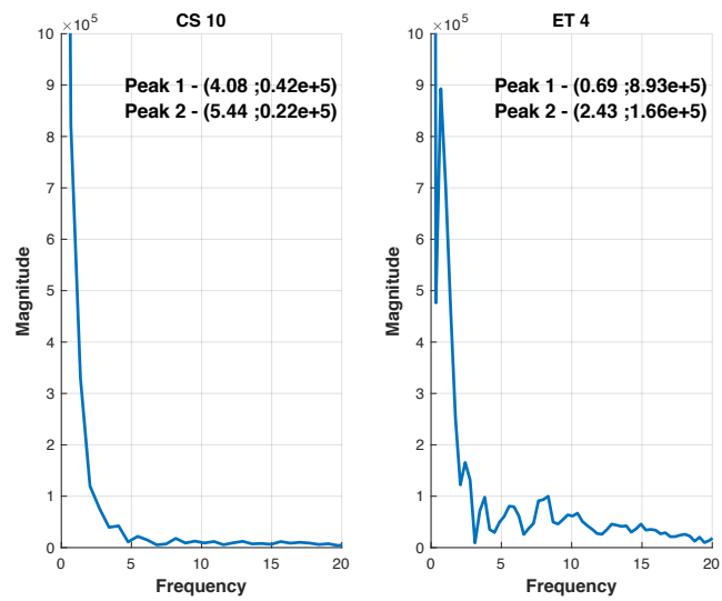
Figure F18: A comparison FFT plots between ET patient 4 and control subject 10 using R^2 data.
