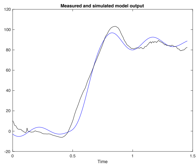
Figure C54: Measured (black) and simulated model (blue) output of control subject 4 with 86.2% best fit.
