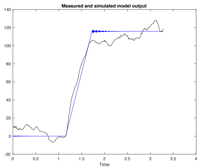
Figure C70: Measured (black) and simulated model (blue) output of ET patient 2 with - 3.7% best fit - omitted from the analysis.
