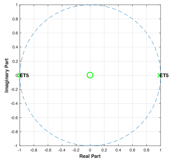
Figure C29: Pole-zero plot of ET patient 5 using X-axis data.
