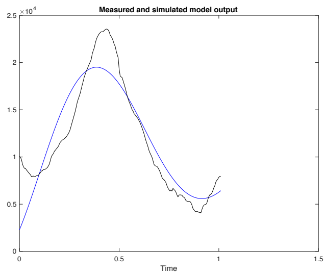
Figure E8: Measured (black) and simulated model (blue) output of control subject 4 with 59.3% best fit.
