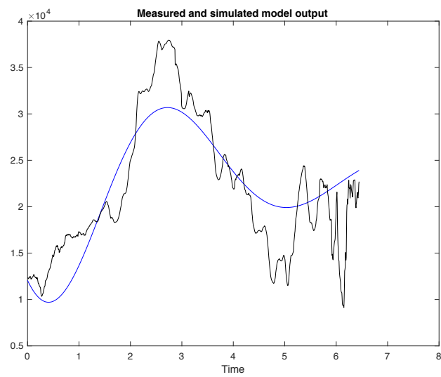
Figure E26: Measured (black) and simulated model (blue) output of ET patient 3 with 44.6% best fit - omitted from the analysis.
