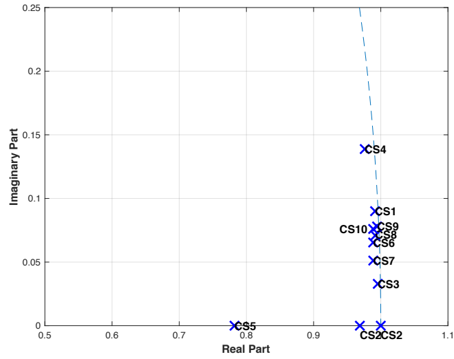
Figure 4.2.2: Combined X-axis data pole-zero plot for control subjects (blue) - conjugate counterparts are mirror image.
