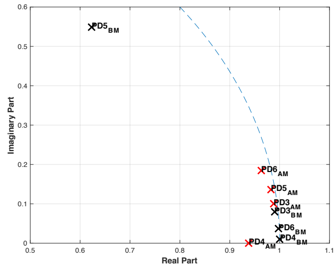
Figure 4.2.18: Pole-zero plot between PD patients before medication (black) and PD patients after medication (red) using Y-axis data - conjugate counterparts are mirror image.
