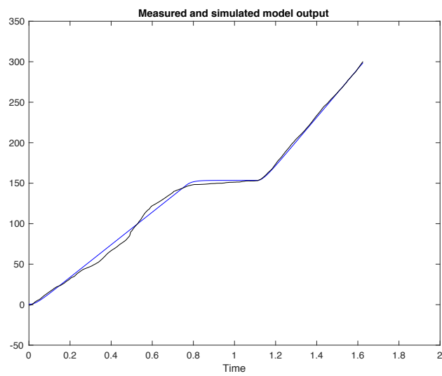
Figure C20: Measured (black) and simulated model (blue) output of control subject 10 with 95.0% best fit.
