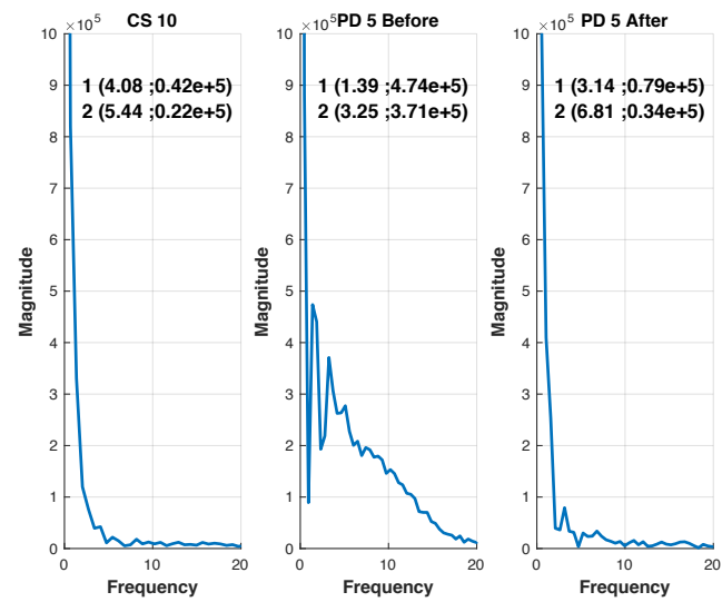
Figure F28: A comparison FFT plots between PD patient 5 (before and after medication) and control subject 10 using R^2 data.
