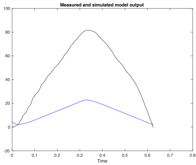
Figure D60: Measured (black) and simulated model (blue) output of ET patient 1 with - 54.4% best fit - omitted from the analysis.
