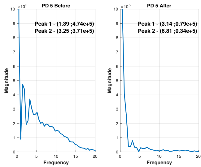
Figure F27: A FFT plot of PD patient 5 (before and after medication) using R^2 data.
