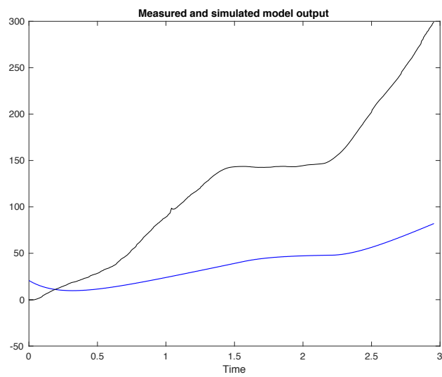
Figure C6: Measured (black) and simulated model (blue) output of control subject 3 with -34.3% best fit - omitted from the analysis.
