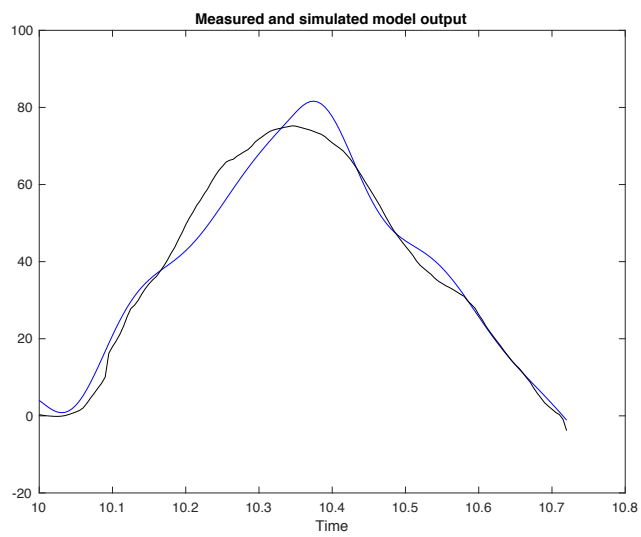
Figure D66: Measured (black) and simulated model (blue) output of ET patient 4 with 83.3% best fit.
