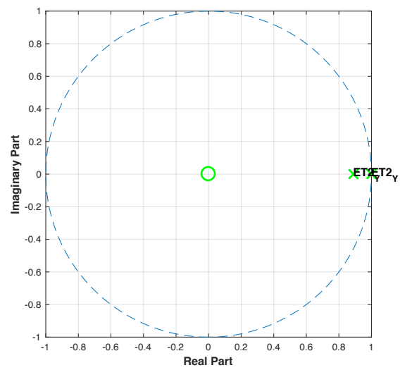
Figure D61: Pole-zero plot of ET patient 2 using Y-axis data.
