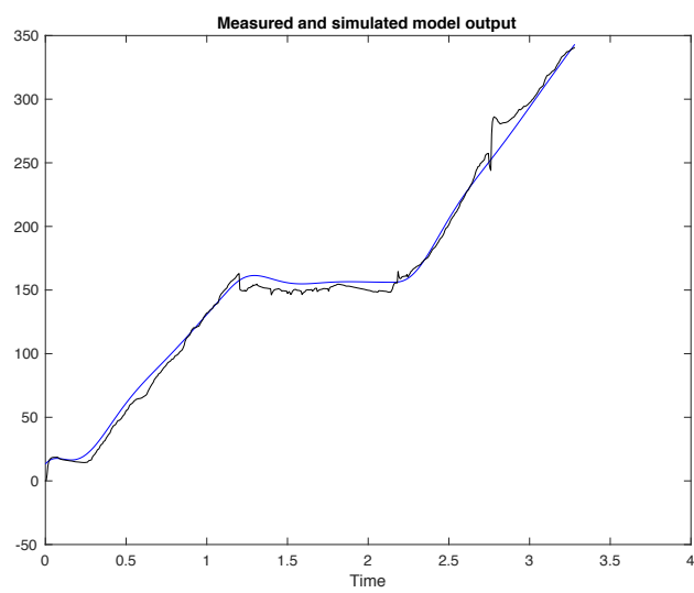
Figure C28: Measured (black) and simulated model (blue) output of ET patient 4 with 92.3% best fit.
