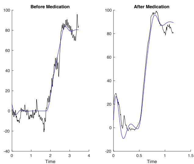
Figure C84: Measured (black) and simulated model (blue) output of PD patient 5 before and after medication with 82.1% and 84.6% best fit respectively.
