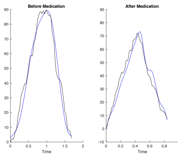
Figure D70: Measured (black) and simulated model (blue) output of PD patient 1 before and after medication with 81.5% and 76.3% best fit respectively.
