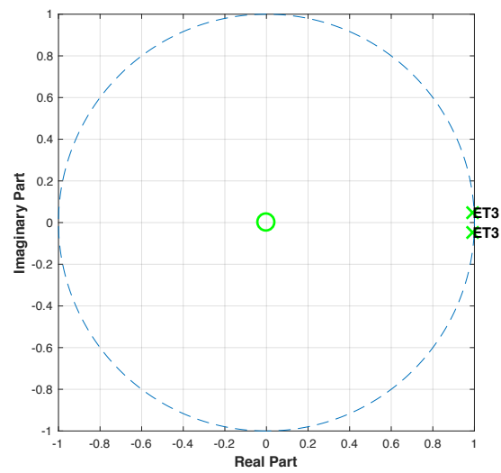
Figure C25: Pole-zero plot of ET patient 3 using X-axis data.
