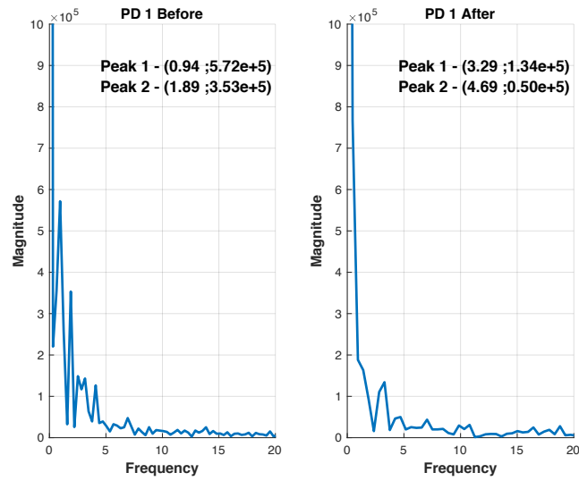
Figure 4.4.3: An example of a FFT plot of PD patient 1 (before and after medication) using R^2 data.
