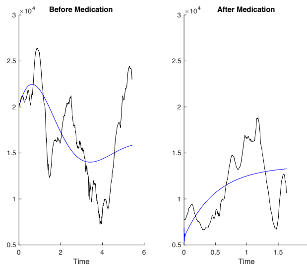
Figure E34: Measured (black) and simulated model (blue) output of PD patient 3 before and after medication with 21.3% and 16.7% best fit respectively - omitted from the analysis.
