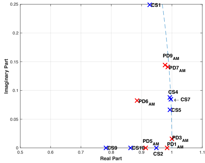
Figure 4.1.7: Pole-zero plot between control subjects (blue) and PD patients after medication (red) using X-axis data - conjugate counterparts are mirror image.
