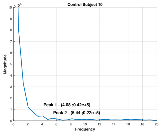
Figure F10: A FFT plot of control subject 10 using R^2 data.
