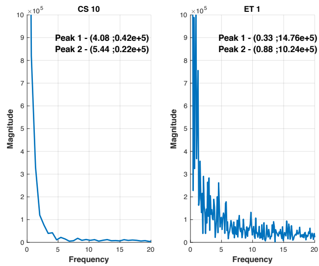
Figure F12: A comparison FFT plots between ET patient 1 and control subject 10 using R^2 data.
