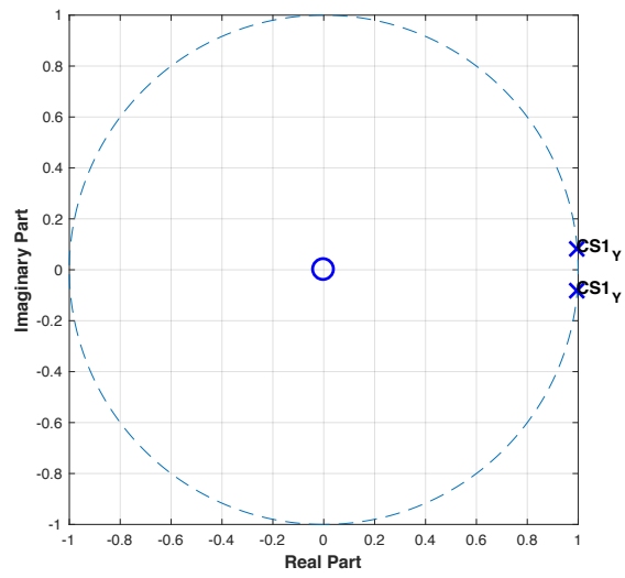
Figure D39: Pole-zero plot of control subject 1 using Y-axis data.
