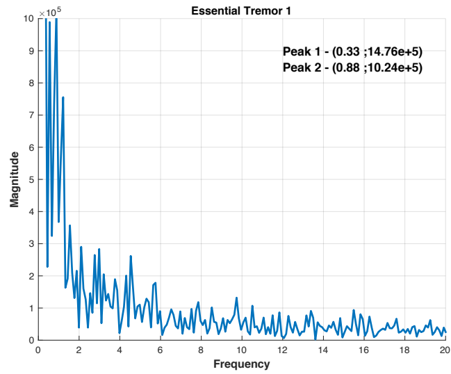
Figure 4.4.2: An example of a FFT plot of ET patient 1.
