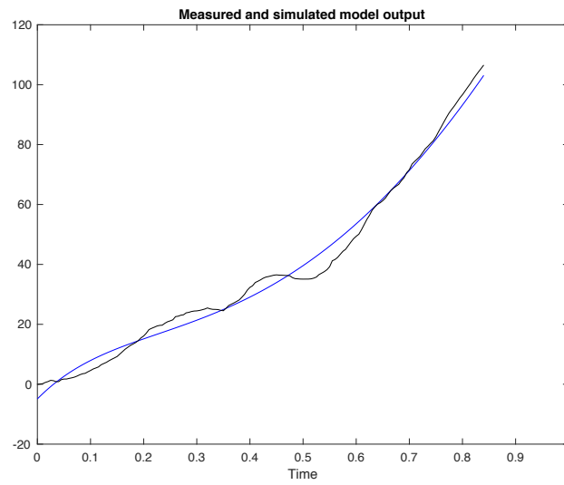
Figure D2: Measured (black) and simulated model (blue) output of control subject 1 with 89.2% best fit.
