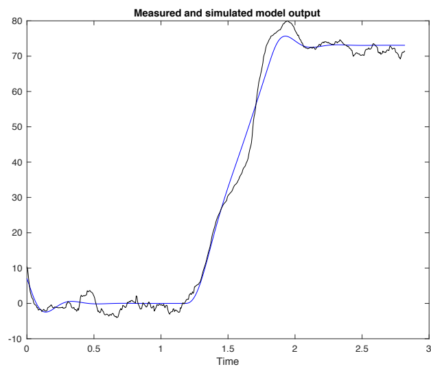
Figure C76: Measured (black) and simulated model (blue) output of ET patient 5 with 92.1% best fit.
