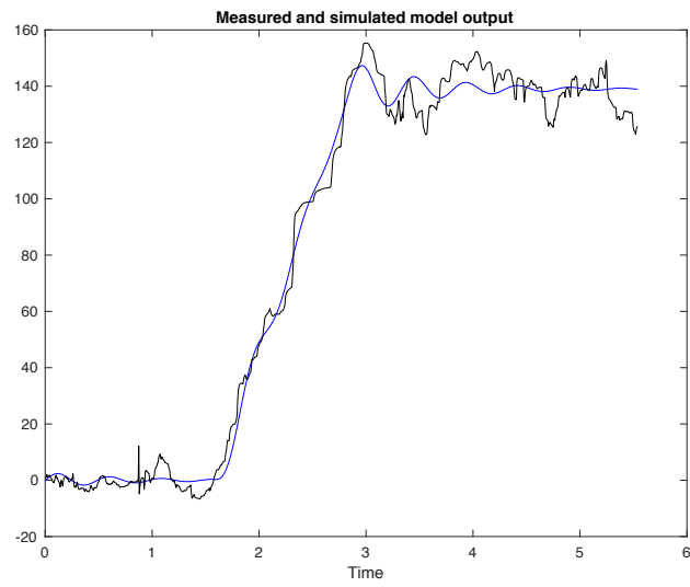
Figure C68: Measured (black) and simulated model (blue) output of ET patient 1 with 90.5% best fit.
