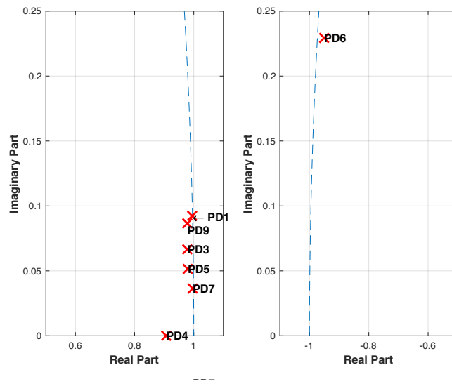
Figure 4.1.12: Combined Y-axis data pole-zero plot for PD patients before medication (red) - conjugate counterparts are mirror image.
