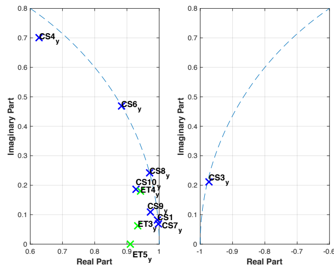
Figure 4.2.15: Pole-zero plot between control subjects (blue) and ET patients (green) using Y-axis data - conjugate counterparts are mirror image.
