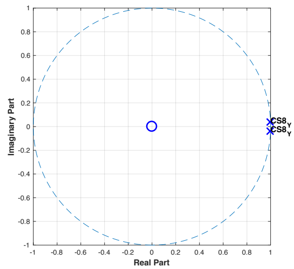
Figure C61: Pole-zero plot of control subject 8 using Y-axis data.
