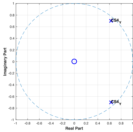
Figure D45: Pole-zero plot of control subject 4 using Y-axis data.
