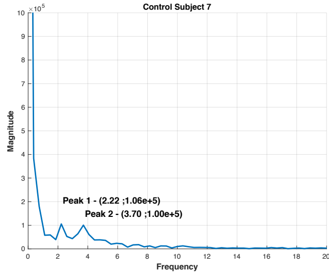
Figure 4.4.1: An example of a FFT plot of a 'good' control subject.
