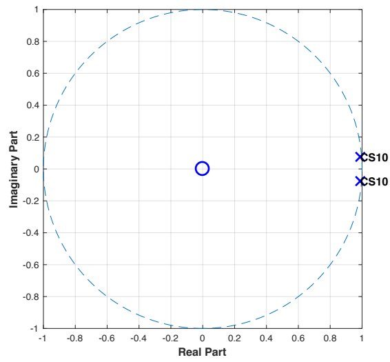
Figure D19: Pole-zero plot of control subject 10 using X-axis data.
