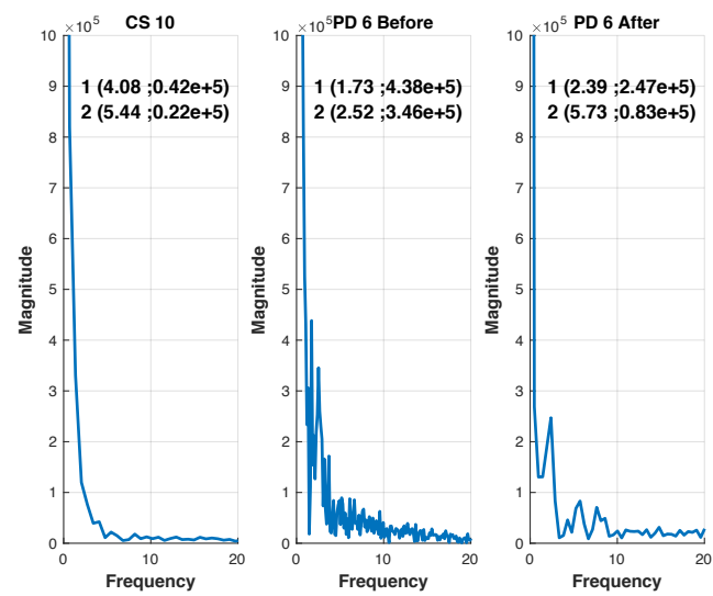
Figure F30: A comparison FFT plots between PD patient 6 (before and after medication) and control subject 10 using R^2 data.
