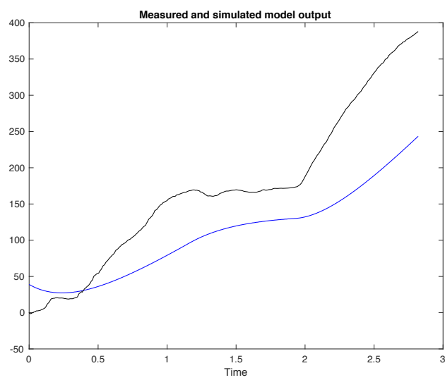
Figure C30: Measured (black) and simulated model (blue) output of ET patient 5 with 24.9% best fit - omitted from the analysis.
