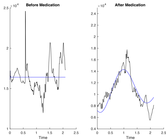
Figure E32: Measured (black) and simulated model (blue) output of PD patient 1 before and after medication with -9.9% (omitted from the analysis) and 50.8% best fit respectively.
