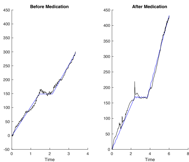
Figure C42: Measured (black) and simulated model (blue) output of PD patient 7 before and after medication with 90.2% and 89.3% best fit respectively.
