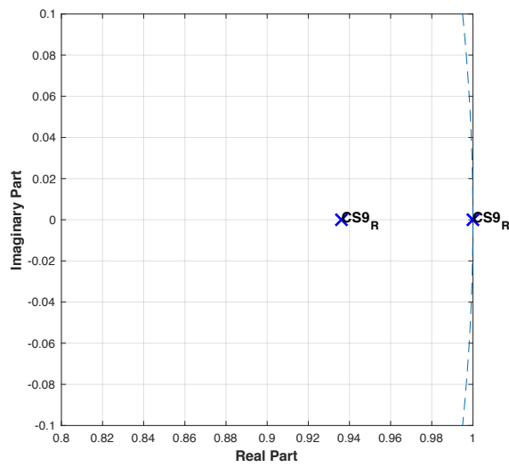
Figure E17: Pole-zero plot for control subject 9 using R^2 data.
