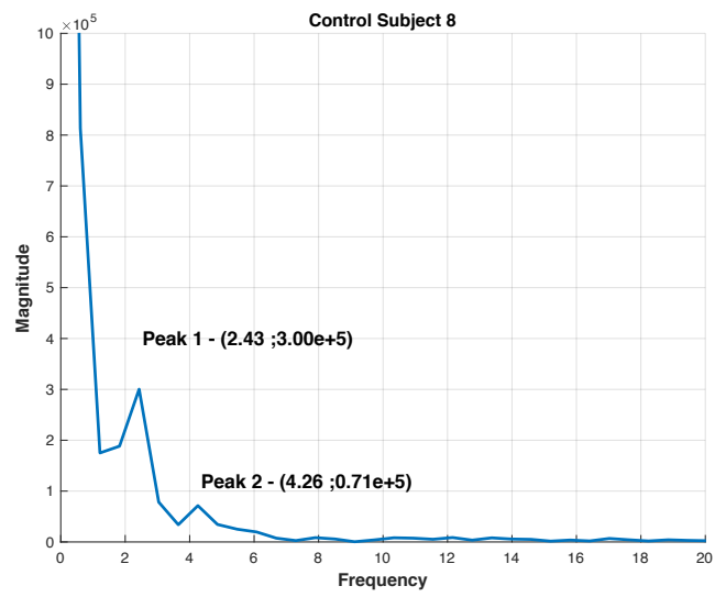
Figure F8: A FFT plot of control subject 8 using R^2 data.
