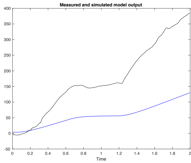
Figure C16: Measured (black) and simulated model (blue) output of control subject 8 with -25.5% best fit - omitted from the analysis.
