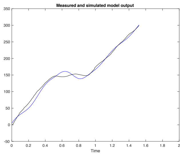
Figure C14: Measured (black) and simulated model (blue) output of control subject 7 with 88.8% best fit.
