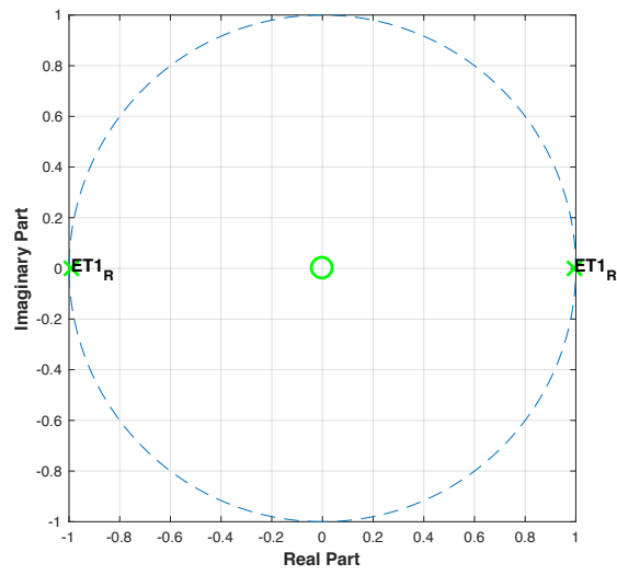
Figure E21: Pole-zero plot of ET patient 1 using R^2 data.
