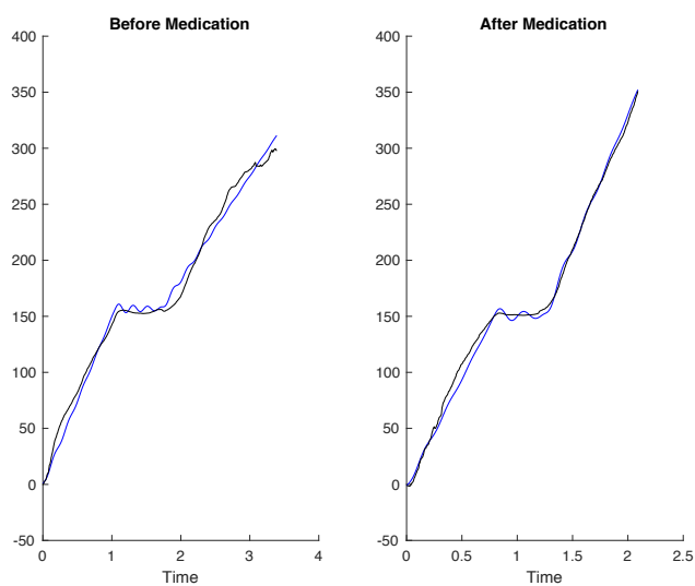
Figure C46: Measured (black) and simulated model (blue) output of PD patient 9 before and after medication with 89.9% and 93.5% best fit respectively.
