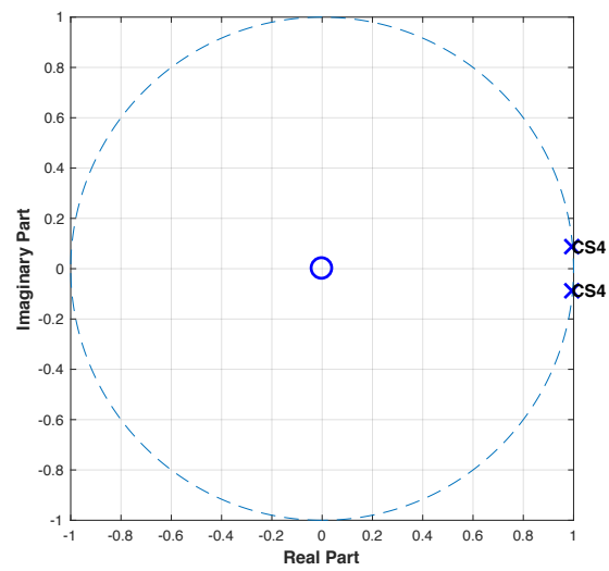
Figure C7: Pole-zero plot of control subject 4 using X-axis data.
