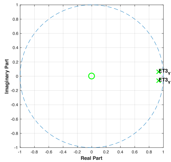
Figure D63: Pole-zero plot of ET patient 3 using Y-axis data.
