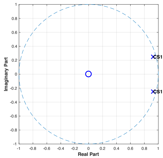
Figure C1: Pole-zero plot of control subject 1 using X-axis data.
