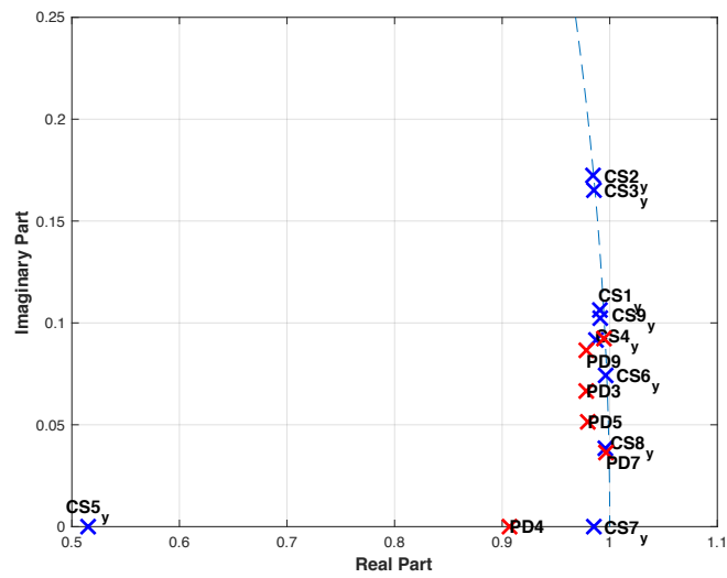
Figure 4.1.15: Pole-zero plot between control subjects (blue) and PD patients before medication (red) using Y-axis data - conjugate counterparts are mirror image.
