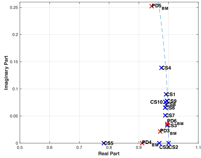
Figure 4.2.7: Pole-zero plot between control subjects (blue) and PD patients before medication (red) using X-axis data - conjugate counterparts are mirror image.
