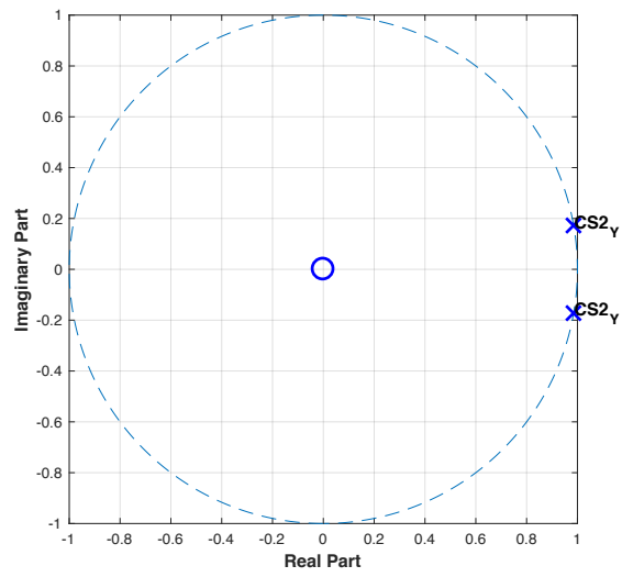
Figure C49: Pole-zero plot of control subject 2 using Y-axis data.
