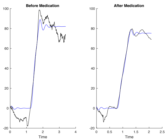
Figure C92: Measured (black) and simulated model (blue) output of PD patient 9 before and after medication with 80.0% and 89.3% best fit respectively.
