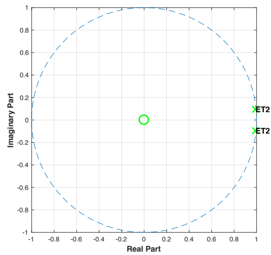
Figure D23: Pole-zero plot of ET patient 2 using X-axis data.
