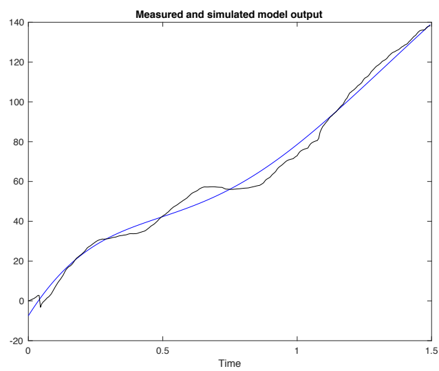
Figure D30: Measured (black) and simulated model (blue) output of ET patient 5 with 90.2% best fit.
