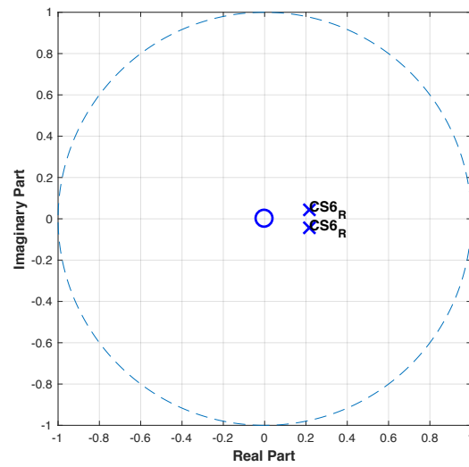
Figure E11: Pole-zero plot for control subject 6 using R^2 data.
