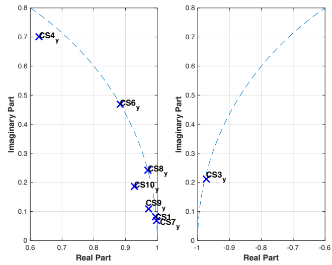
Figure 4.2.11: Combined Y-axis data pole-zero plot for control subjects (blue) - conjugate counterparts are mirror image.
