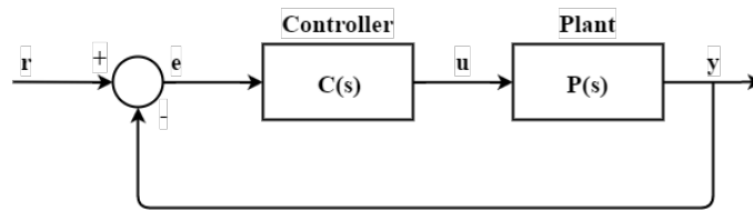
Figure 3.1.1: A diagram of a unity feedback system.
