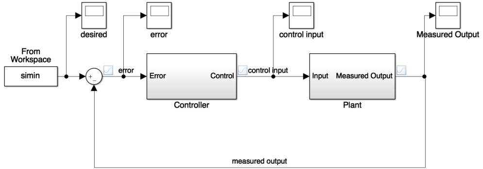
Figure 3.1.2: Simulink model of a PID.
