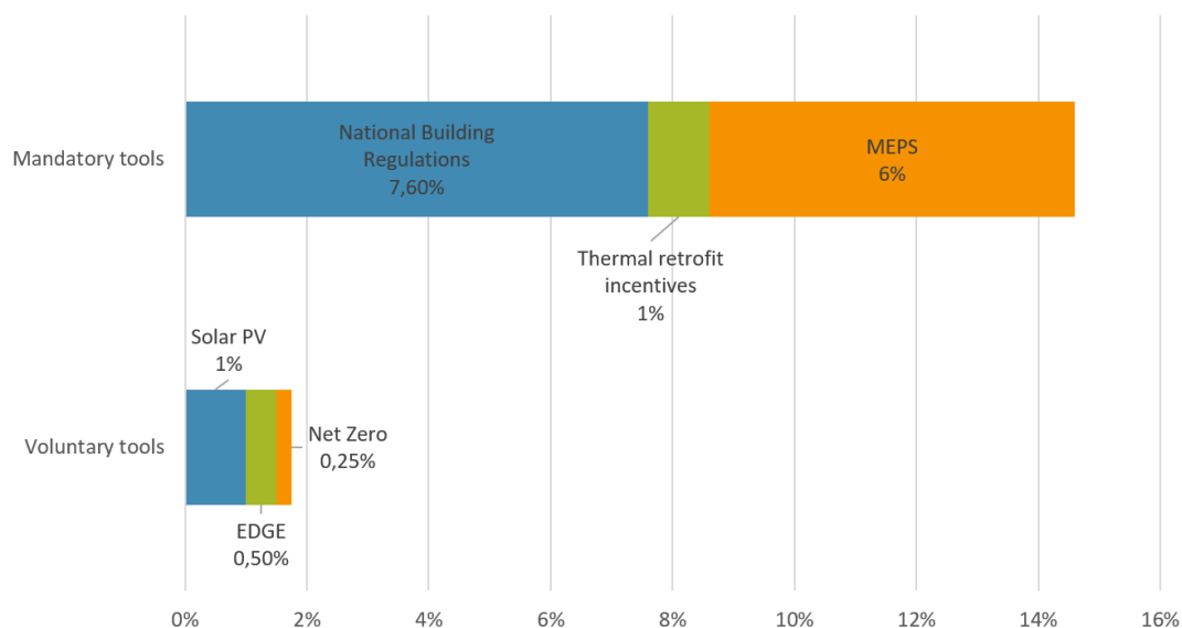
Figure 16 - Energy intensity reduction potential of different building efficiency tools commonly used in South Africa
