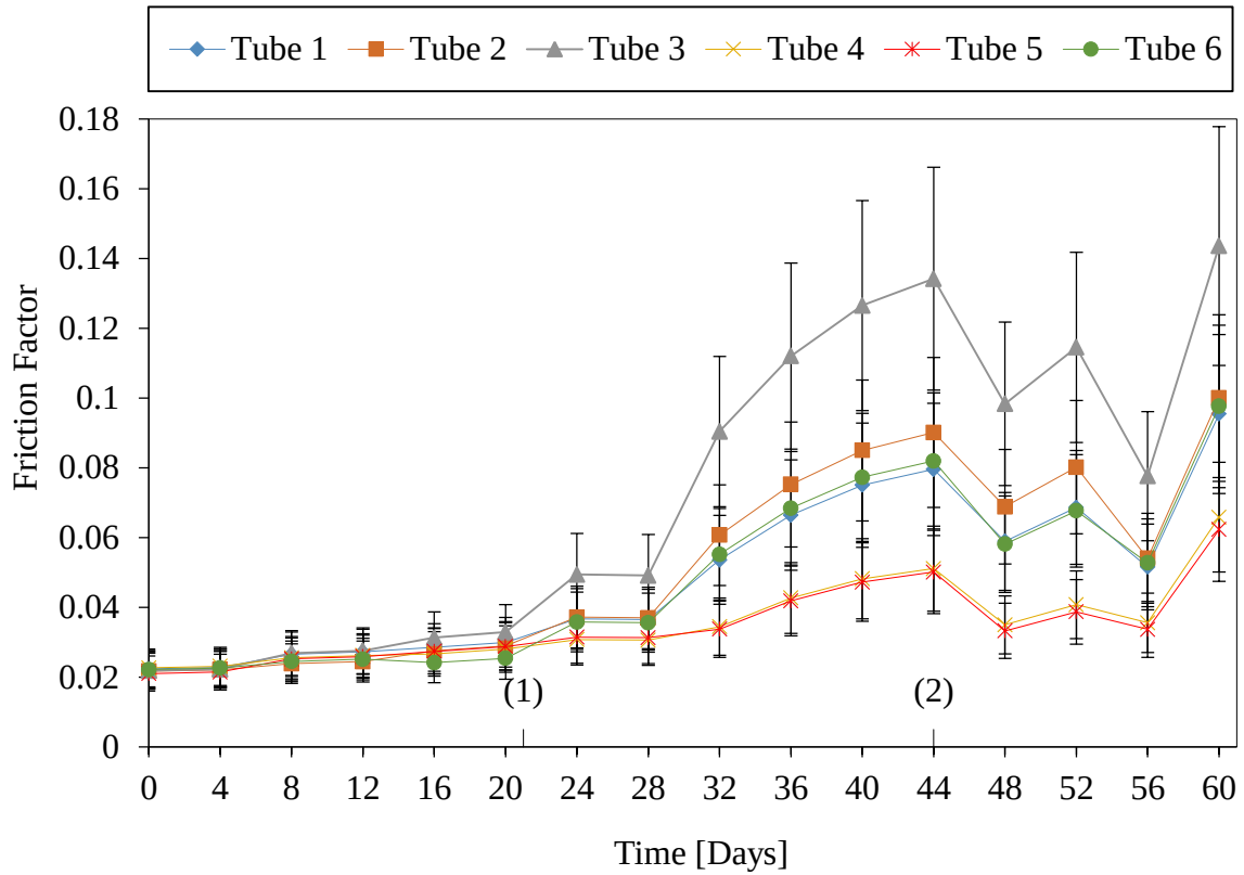
Figure 28: Measured friction factors for tube 1, 2, 3, 4, 5 and 6 during test 3 – (1) Plant dosed biocide – (2) Increase dosing concentration in tube 1, 2, 3 and 6
