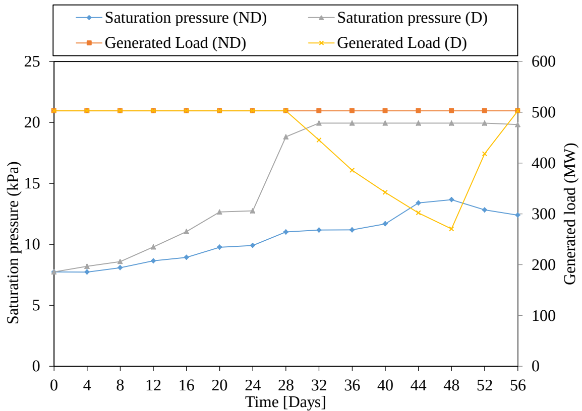
Figure 32: Generated load and actual condenser saturation pressure for test 1- (D) Dosed tube-6, (ND) Non dosed tube-4
