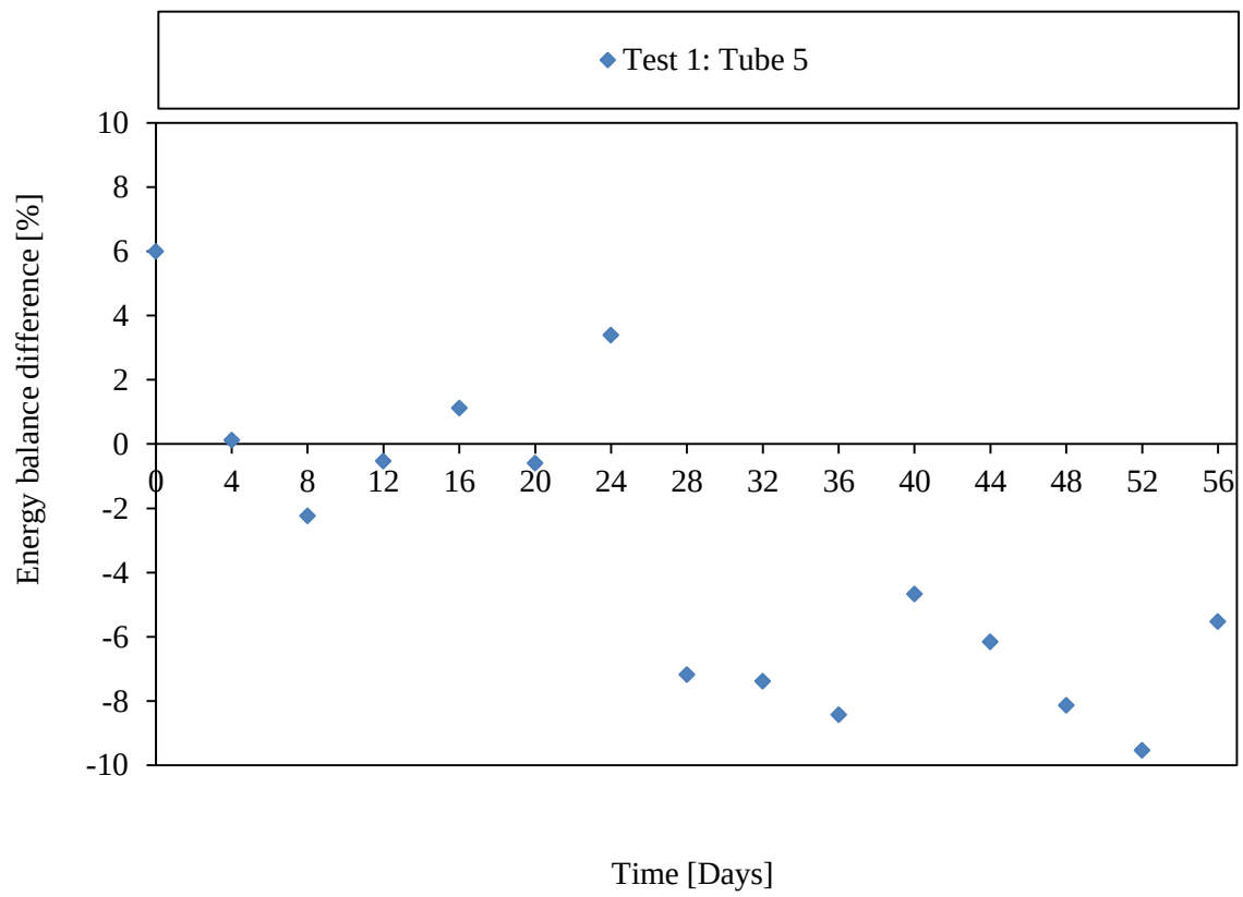
Figure 50: Difference in energy balance Equation (21) of Test 1: Tube 5
