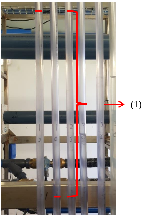
Figure 17: U-type manometer – (1) Pressure differential over the first condenser tube.
