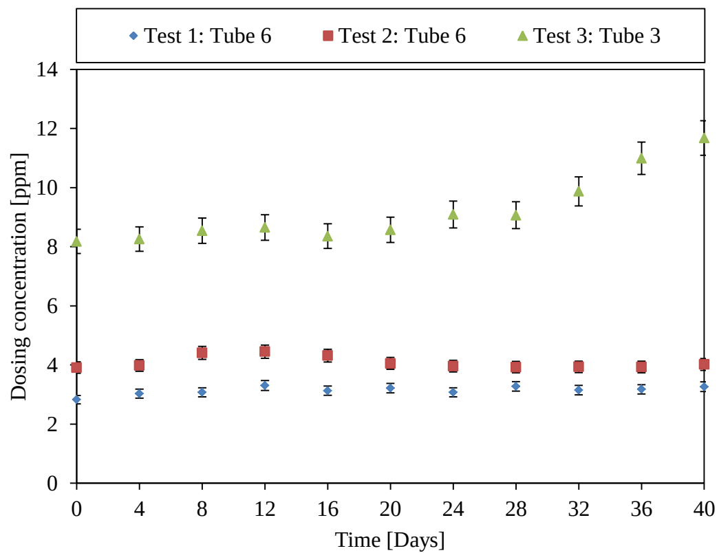
Figure 47: Bio-dispersant dosing concentration: Test 1: Tube 6 (3.1 ml/h), Test 2: Tube 6 (4.1 ml/h) and Test 3: Tube 3 (9.2 ml/h).
