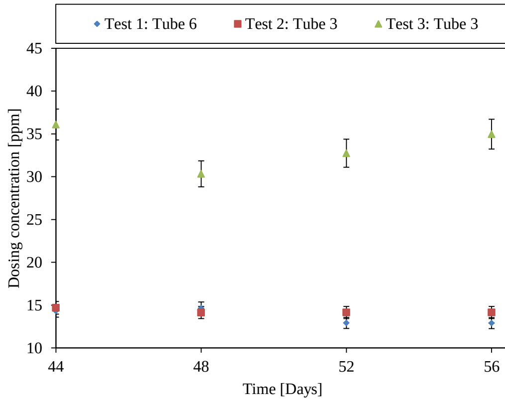
Figure 51: Bio-dispersant dosing concentration: Test 1: Tube 6 (13.6 ml/h), Test 2: Tube 3 (14.2 ml/h) and Test 3: Tube 3 (34.8 ml/h).
