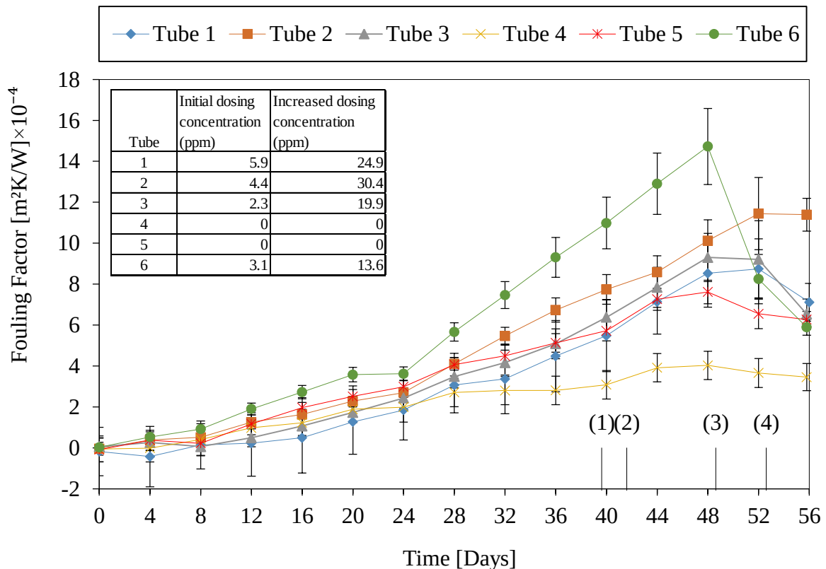
Figure 20: Measured fouling factors for tube 1, 2, 3, 4, 5 and 6 during test 1 – (1) Plant dosed biocide – (2) Increase dosing concentration in tube 1, 2, 3 and 6 – (3) Dosed NaOCl in strainers – (4) Dosed NaOCl in strainers
