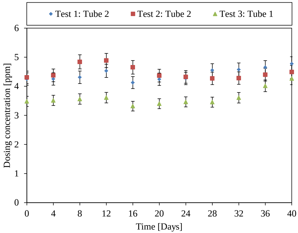
Figure 45: Bio-dispersant dosing concentration: Test 1: Tube 2 (4.4 ml/h), Test 2: Tube 2 (4.5 ml/h) and Test 3: Tube 1 (3.6 ml/h).
