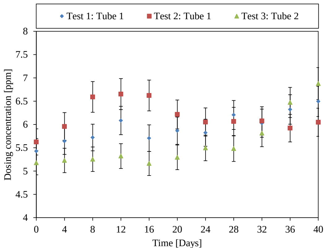
Figure 44: Bio-dispersant dosing concentration: Test 1: Tube 1 (5.9 ml/h), Test 2: Tube 1 (6.2 ml/h) and Test 3: Tube 2 (5.6 ml/h).
