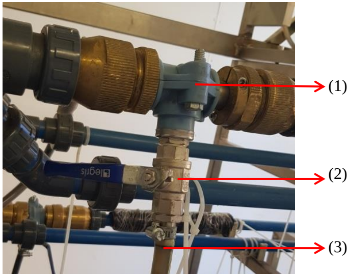
Figure 16: Pressure tapping – (1) Pipe saddle, (2) Isolating valve, (3) PVC hose to common manifold
