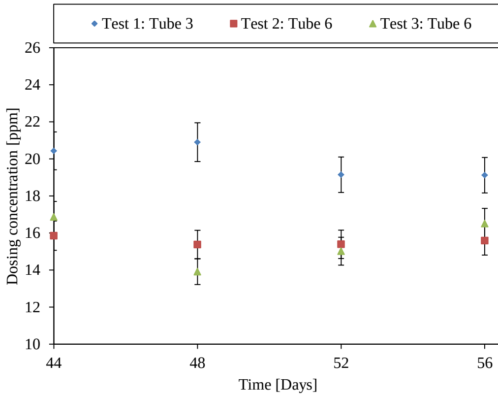
Figure 50: Bio-dispersant dosing concentration: Test 1: Tube 3 (19.9 ml/h), Test 2: Tube 6 (15.5 ml/h) and Test 3: Tube 6 (16.3 ml/h).
