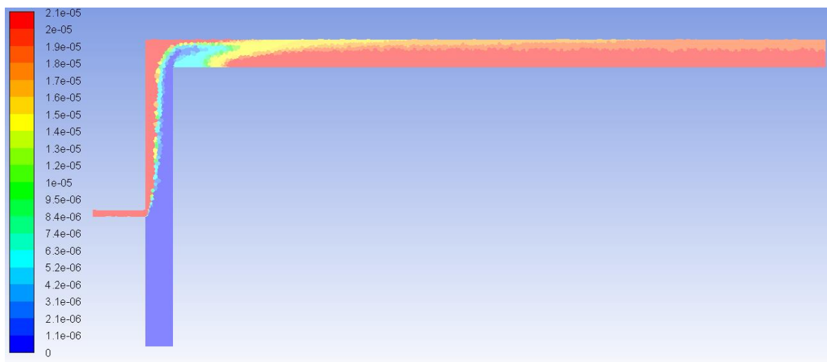
Figure 41: CFD results for a bio-dispersant flowrate of 1.24761 \times 10^{-5} kg/s (Final mixing concentration of 20 ppm). The scale indicates the bio-dispersant concentration in mg bio-dispersant per 1 L water.
