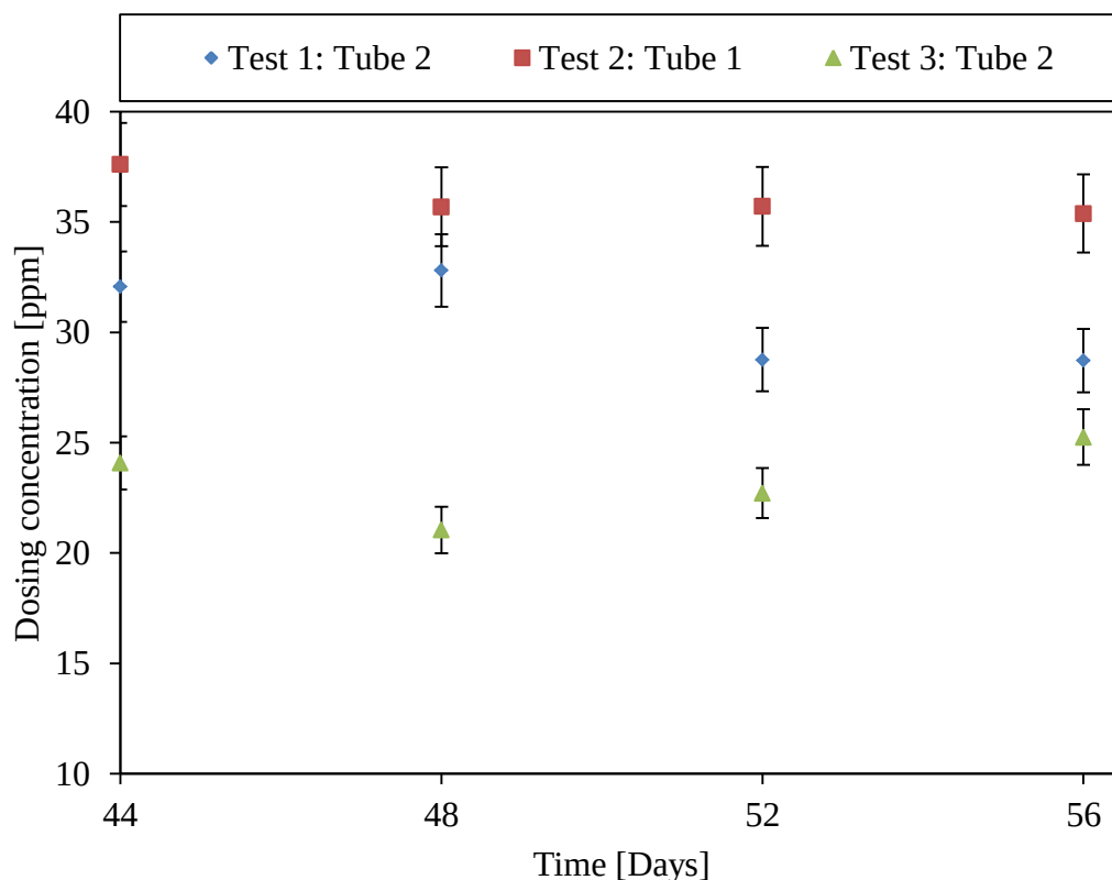
Figure 48: Bio-dispersant dosing concentration: Test 1: Tube 2 (30.4 ml/h), Test 2: Tube 1 (36 ml/h) and Test 3: Tube 2 (24.5 ml/h).
