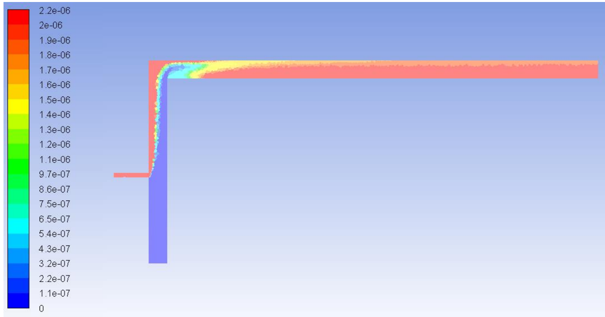
Figure 43: CFD results for a bio-dispersant flowrate of 1.24761 \times 10^{-6} kg/s (Final mixing concentration of 2 ppm). The scale indicates the bio-dispersant concentration in mg bio-dispersant per 1 L water.
