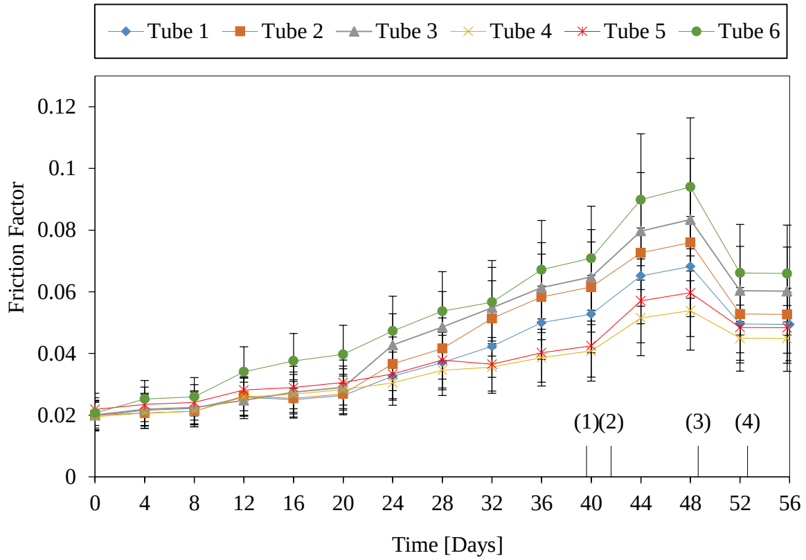
Figure 26: Measured friction factors for tube 1, 2, 3, 4, 5 and 6 during test 1 – (1) Plant dosed biocide – (2) Increase dosing concentration in tube 1, 2, 3 and 6 – (3) Dosed NaOCl in strainers – (4) Dosed NaOCl in strainers
