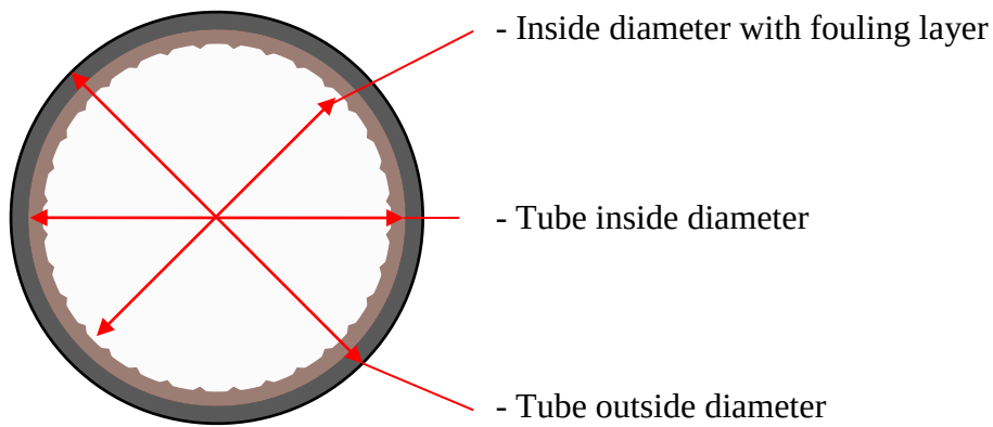
Figure 4: Schematic cross-sectional tube drawing showing the fouling layer.
