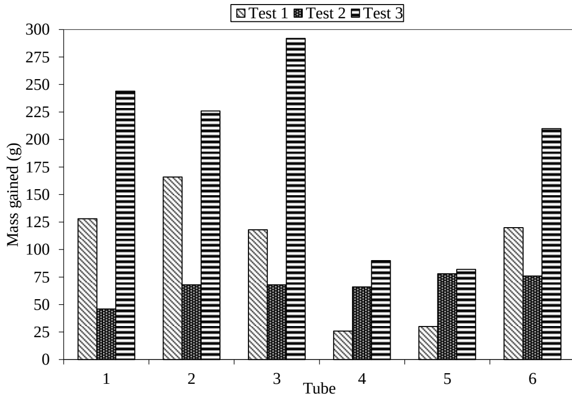
Figure 29: Mass gained for tube 1, 2, 3, 4, 5 and 6 during test 1, 2 and 3.
