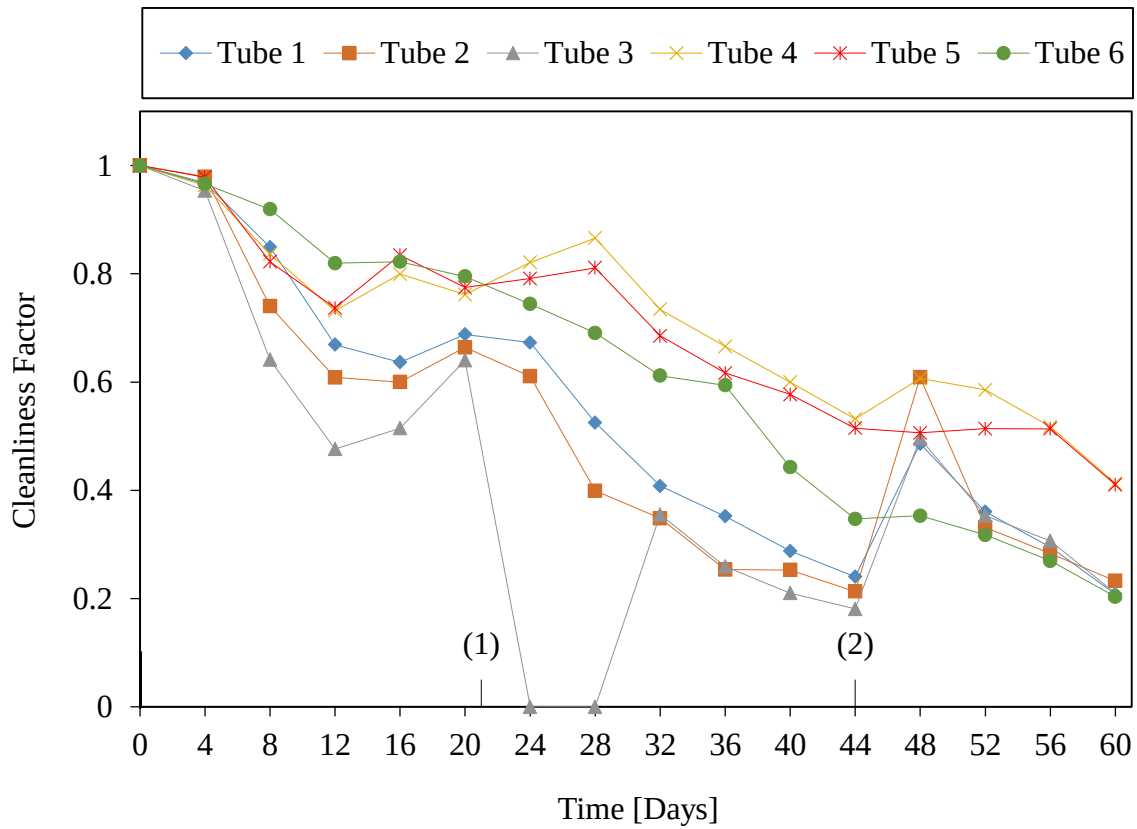
Figure 25: Calculated cleanliness factors for tube 1, 2, 3, 4, 5 and 6 during test 3 – (1) Plant dosed biocide – (2) Increase dosing concentration in tube 1, 2, 3 and 6
