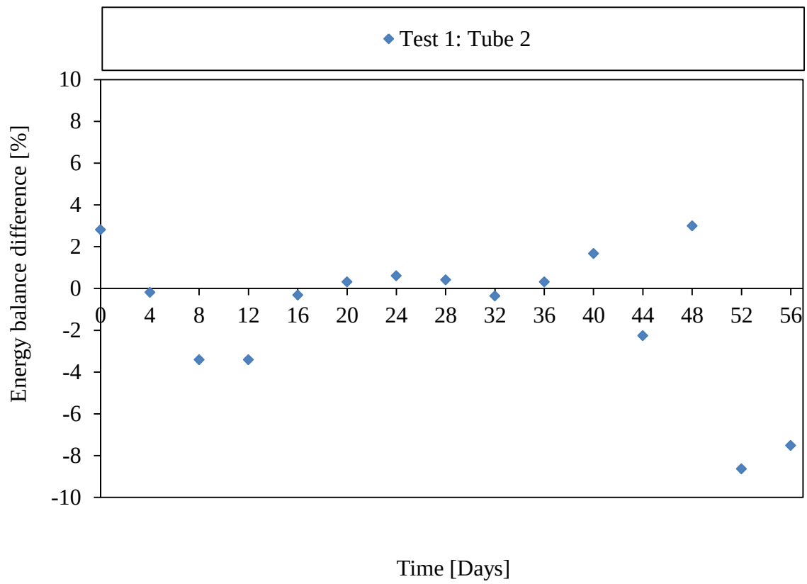
Figure 50: Difference in energy balance Equation (21) of Test 1: Tube 2
