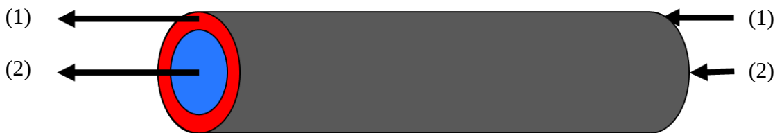
Figure 11: Water flow through annuli and titanium tube – (1) hot water flow, (2) cooling water flow
