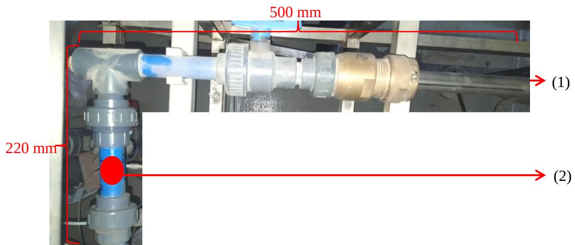
Figure 38: Cooling water tube section modelled – (1) Section where CFD was performed, (2) Proposed chemical injection point
