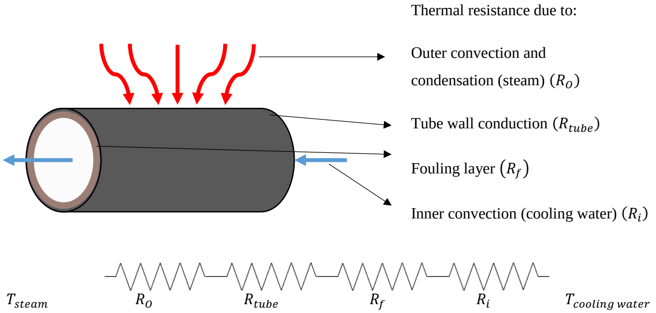
Figure 5: Thermal resistances for heat transfer from the hot to the cold fluid.
