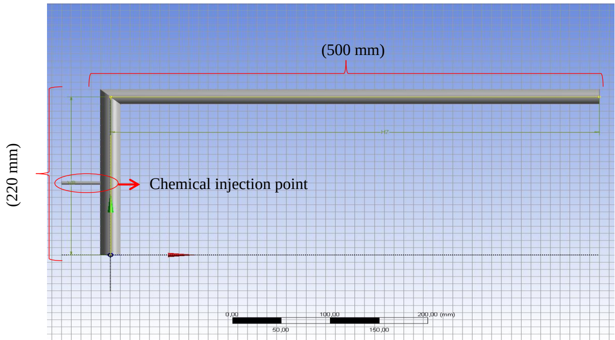
Figure 39: CFD geometry as per Figure 10.
