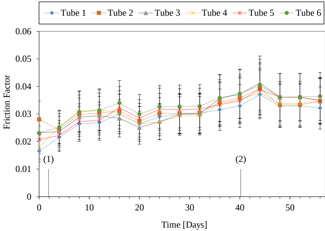
Figure 27: Measured friction factors for tube 1, 2, 3, 4, 5 and 6 during test 2 – (1) Plant dosed biocide – (2) Increase dosing concentration in tube 1, 2, 3 and 6
