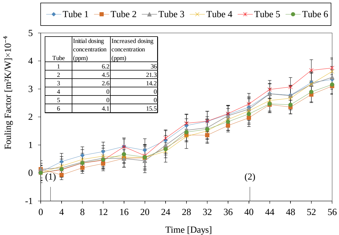
Figure 21: Measured fouling factors for tube 1, 2, 3, 4, 5 and 6 during test 2 – (1) Plant dosed biocide – (2) Increase dosing concentration in tube 1, 2, 3 and 6
