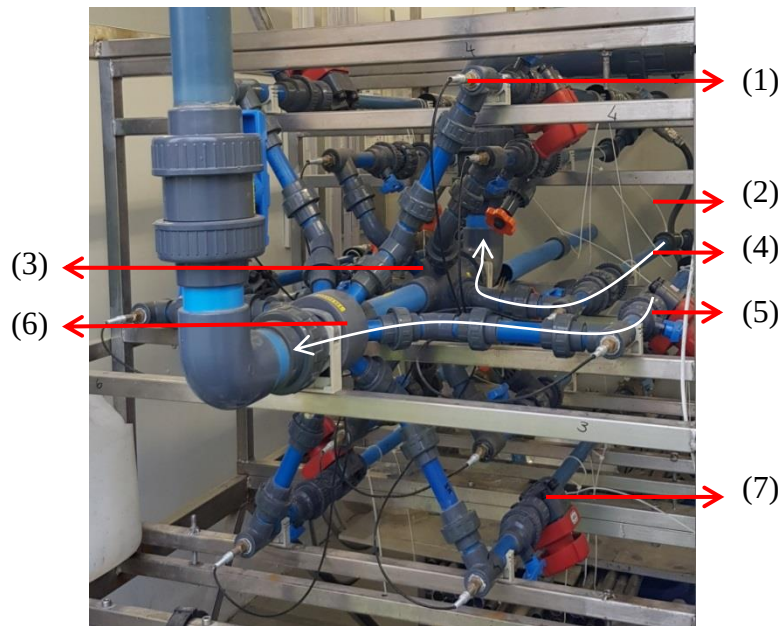
Figure 10: Layout of the test apparatus – (1) temperature probe, (2) polypropylene supports, (3) annulus manifold, (4) hot water flow direction, (5) cooling water flow direction, (6) cooling water manifold, (7) diaphragm valve
