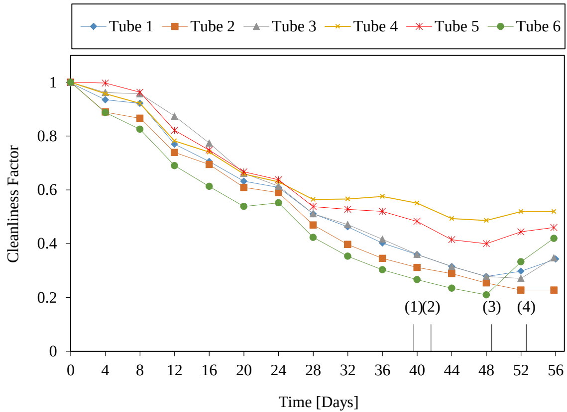
Figure 23: Calculated cleanliness factors for tube 1, 2, 3, 4, 5 and 6 during test 1 – (1) Plant dosed biocide – (2) Increase dosing concentration in tube 1, 2, 3 and 6 – (3) Dosed NaOCl in strainers – (4) Dosed NaOCl in strainers
