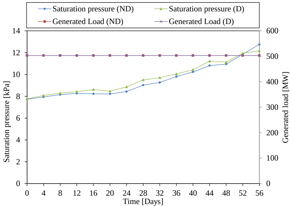
Figure 34: Generated load and actual condenser saturation pressure for test 2- (D) Dosed tube-1, (ND) Non dosed tube-4.
