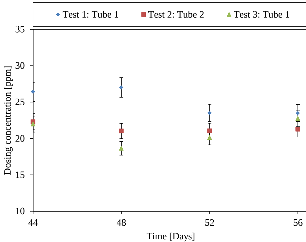
Figure 49: Bio-dispersant dosing concentration: Test 1: Tube 1 (24.9 ml/h), Test 2: Tube 2 (21.3 ml/h) and Test 3: Tube 1 (22 ml/h).
