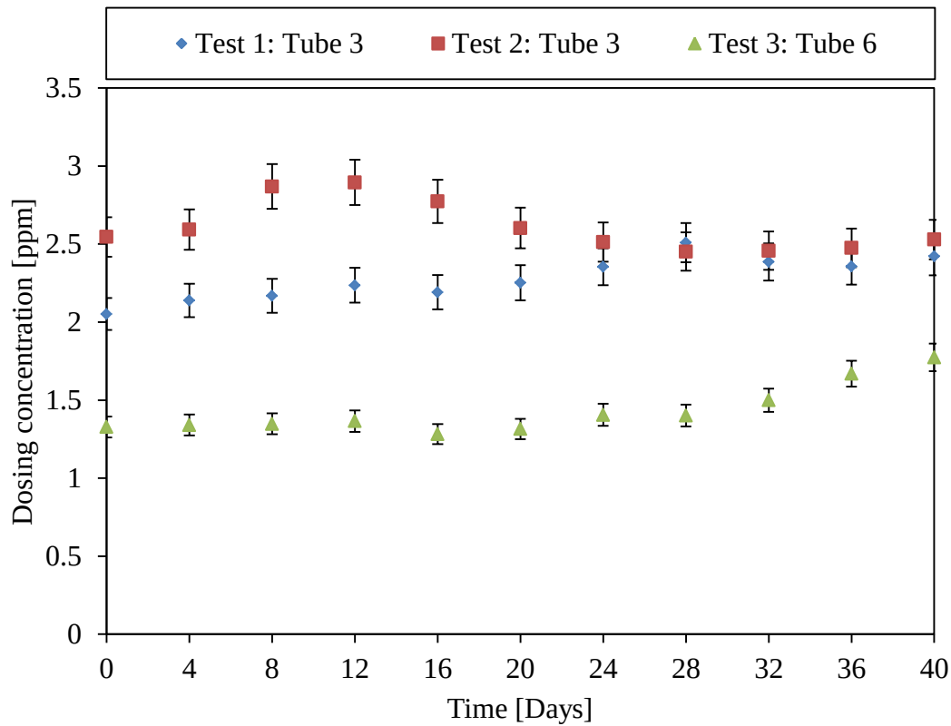
Figure 46: Bio-dispersant dosing concentration: Test 1: Tube 3 (2.3 ml/h), Test 2: Tube 3 (2.6 ml/h) and Test 3: Tube 6 (1.4 ml/h).
