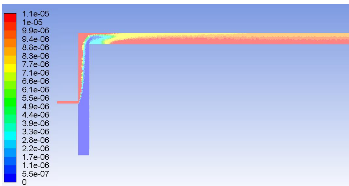
Figure 42: CFD results for a bio-dispersant flowrate of 6.238056 \times 10^{-6} kg/s (Final mixing concentration of 10 ppm). The scale indicates the bio-dispersant concentration in mg bio-dispersant per 1 L water.
