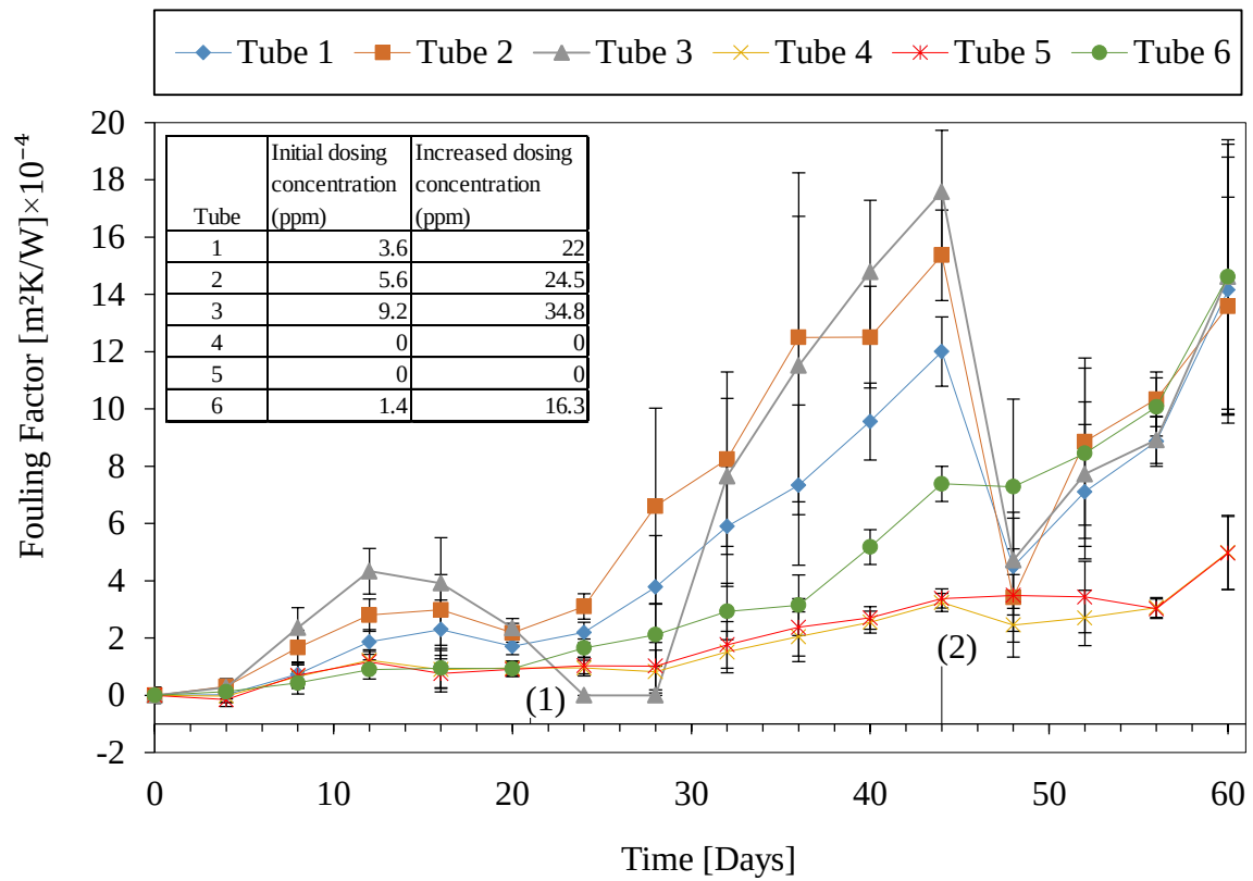
Figure 22: Measured fouling factors for tube 1, 2, 3, 4, 5 and 6 during test 3 – (1) Plant dosed biocide – (2) Increase dosing concentration in tube 1, 2, 3 and 6
