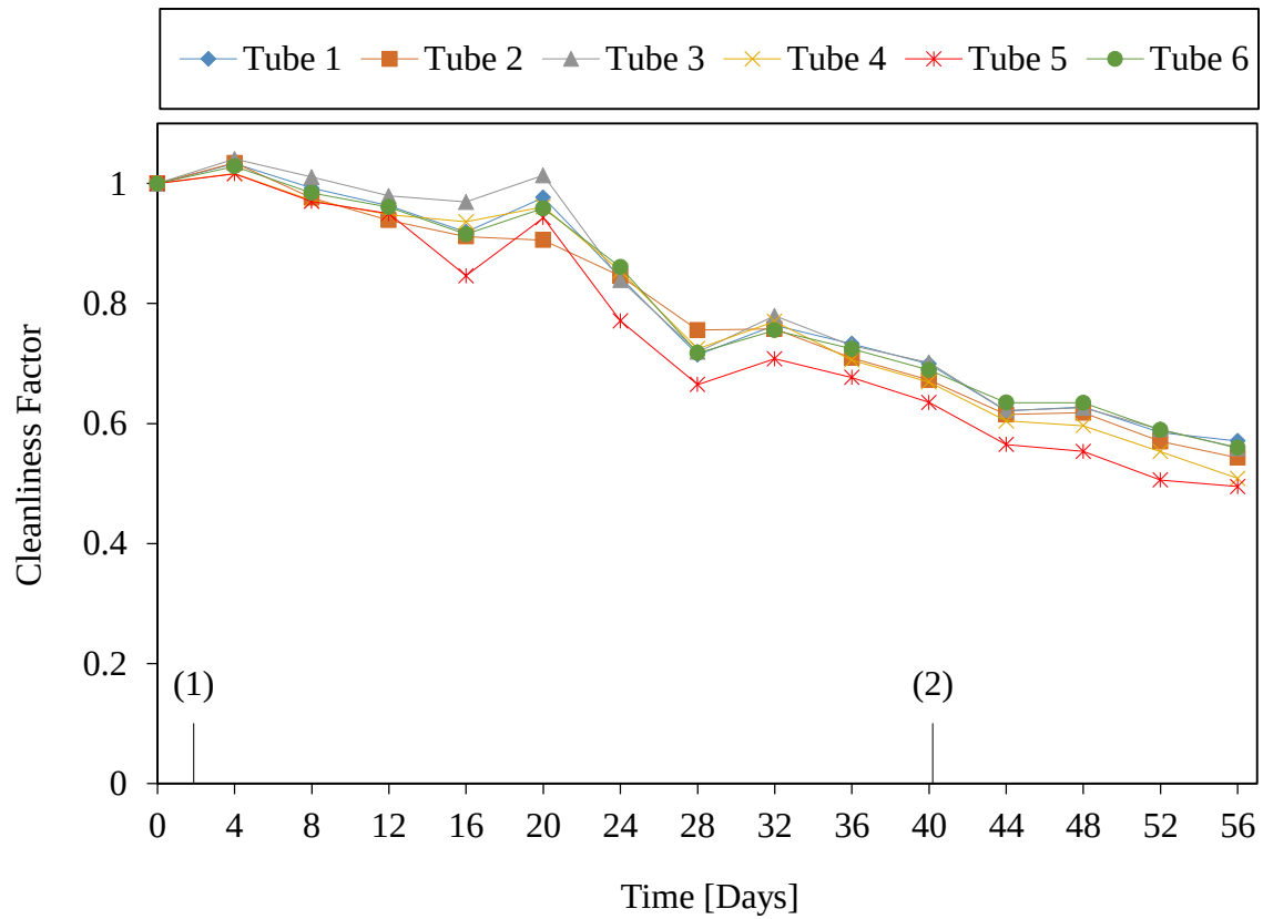
Figure 24: Calculated cleanliness factors for tube 1, 2, 3, 4, 5 and 6 during test 2 –(1) Plant dosed biocide –(2) Increase dosing concentration in tube 1, 2, 3 and 6
