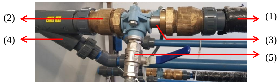
Figure 13: Layout of double pipe heat exchanger – (1) polyurethane insulation, (2) tube gland, (3) titanium condenser tube, (4) hot water jacket, (5) pressure tapping
