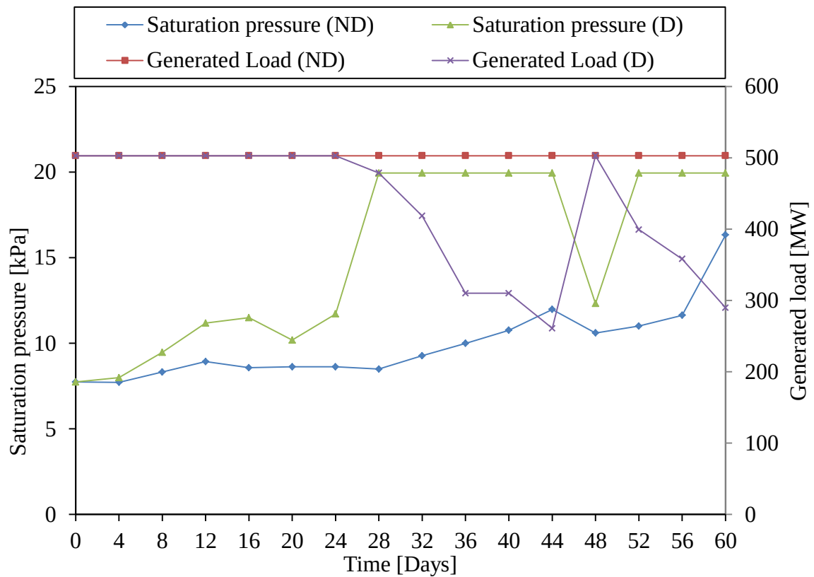
Figure 36: Generated load and actual condenser saturation pressure for test 3- (D) Dosed tube-3, (ND) Non dosed tube-4.
