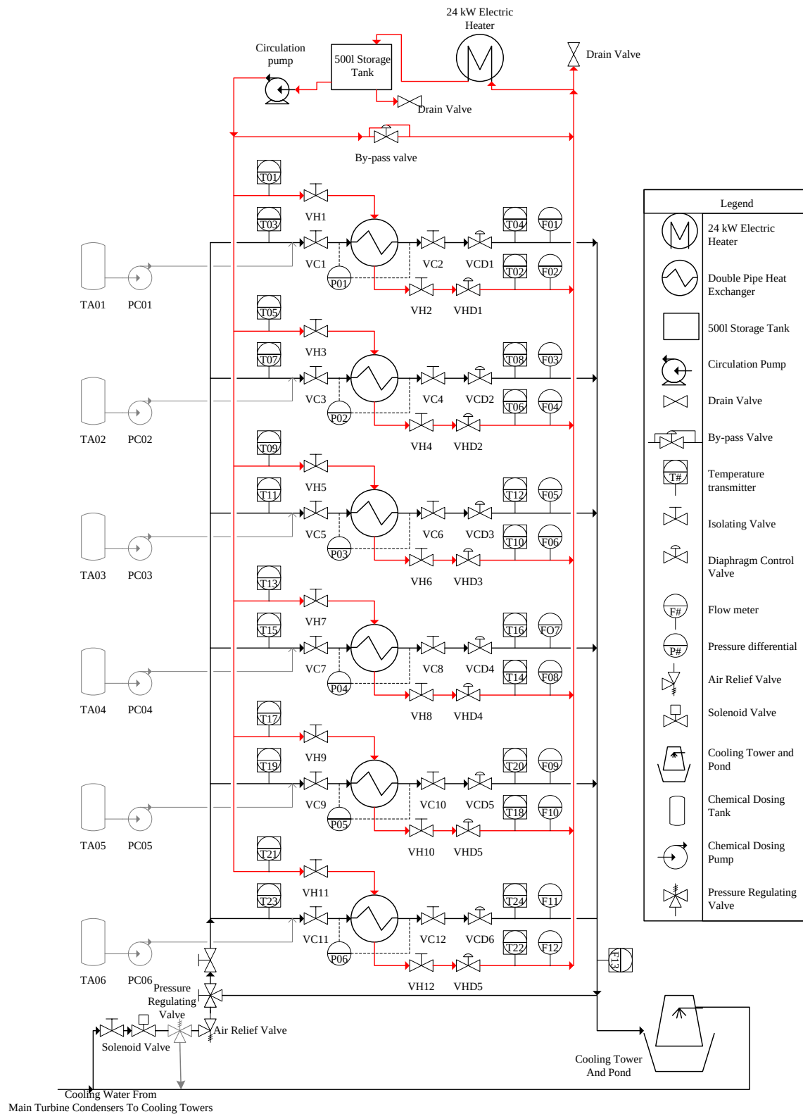
Figure 15: Piping and instrumentation diagram for the test apparatus.
