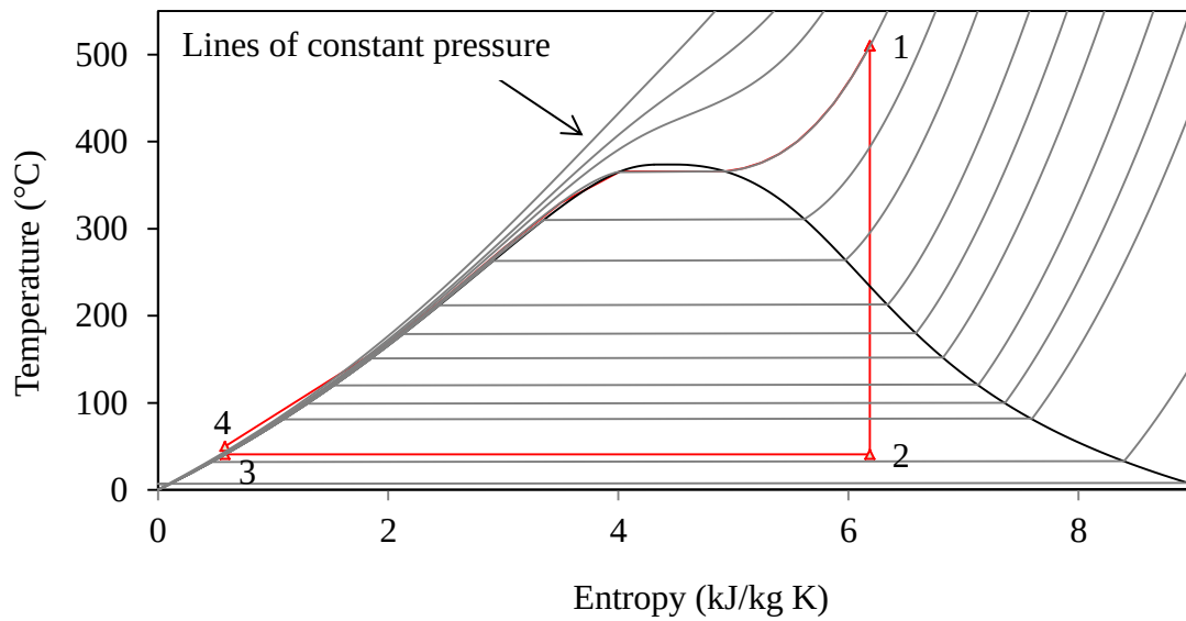
Figure 6: Rankine power cycle: Temperature – entropy diagram
