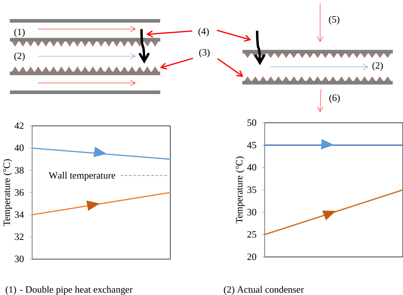
Figure 12: Heat transfer conditions compared in the double pipe heat exchanger and the actual condenser - (1) hot water flow, (2) cooling water flow, (3) fouling layer, (4) heat transfer, (5) steam, (6) condensate (Goodenough, 2017)
