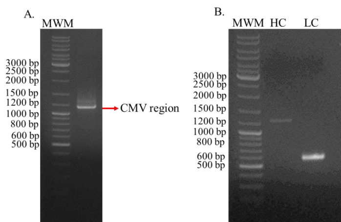
Figure 3.7: PCR amplification of the CMV promotor, and the antibody constant regions including the polyA tail. The DNA fragments were resolved on 0.8% agarose gels and visualised under UV light following ethidium bromide staining. The 1100 bp fragment indicates successful amplification of the CMV promoter region from the VRC_4196 plasmid vector (A). The DNA fragment above the 1200 bp MWM, and at the 600 bp MWM showed successful amplification of the heavy- and light-chain constant and polyA regions respectively (B). HC: heavy-chain constant region fragment containing poly-adenylation sequence, LC: light-chain constant region fragment containing poly-adenylation sequence. The constant and polyA regions were amplified from heavy- and light-chain plasmid vectors synthesized by GeneArt. The O'Gene Ruler DNA ladder #sm1173 (Thermo Fisher Scientific, Waltham, MA, USA) was used as the reference molecular weight marker (MWM), indicated as base pairs (bp) on the left.
