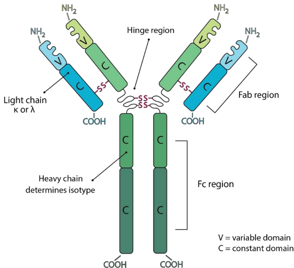
Figure 1.4: Schematic representation of the structure of an antibody. Image obtained from [147].
