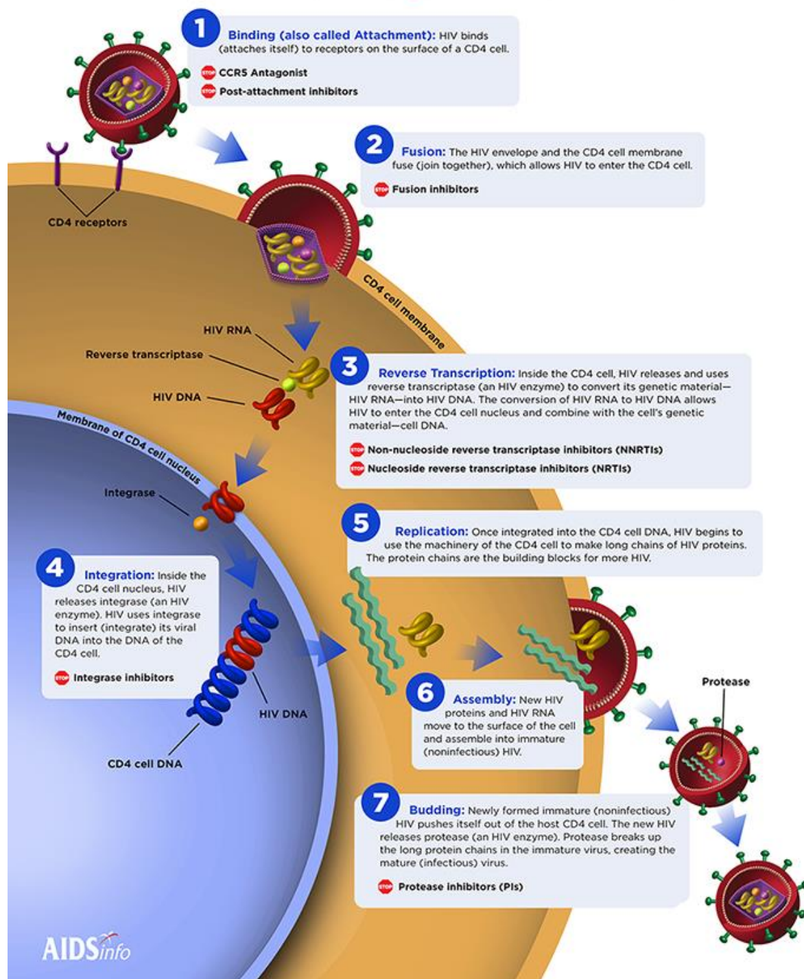
Figure 1.3: The HIV-1 viral life cycle, showing the seven stages of infection of a CD4 positive T cell. The targets of FDA approved antiretroviral drugs are also highlighted. Image obtained from [24].
