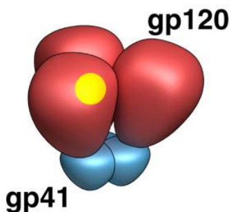
Figure 1.2: Schematic representation of the HIV-1 trimeric envelope glycoprotein made up of the non-covalently bound gp120 and gp41 subunits. Image obtained from [22].
