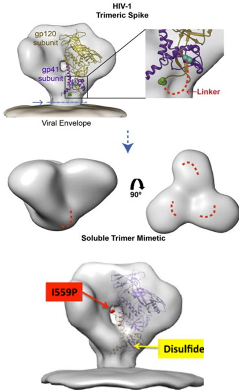
Figure 1.7: The native-like, soluble, trimeric conformation of SOSIP.664 gp140. The gp140 glycoprotein is cleaved into the gp120 and truncated gp41 subunits which are linked together through disulfide bonding. At residue 559 of gp41 there is a Ile-to-Pro change which improves trimerisation of Env. The MPER was cleaved until residue 664 increasing the solubility of Env. Image obtained from [200].
