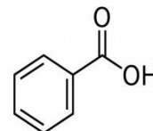
(iv) benzoic acid
