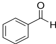
(iii) benzaldehyde
