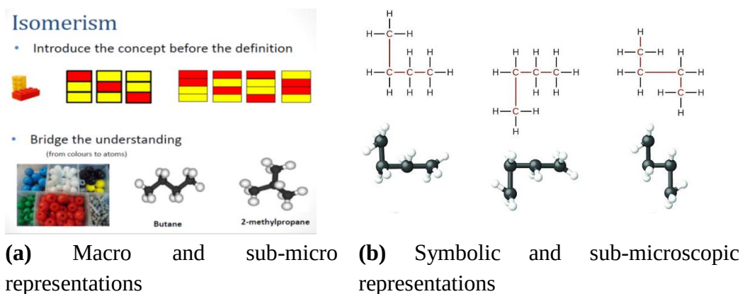
Figure 4.8: Three levels of representations for introducing isomerism
