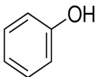
(i) phenol
