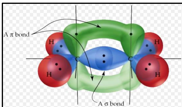
Figure 4.1: Pi and Sigma bonds in alkenes
