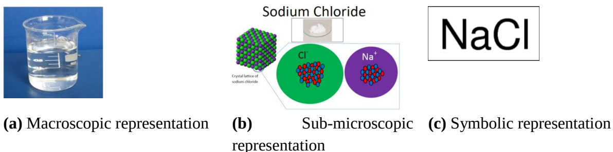
Figure 4.5: The three levels of representations
