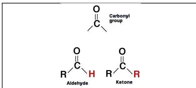
Figure 4.6: Difference and similarity between Aldehydes and Ketones
