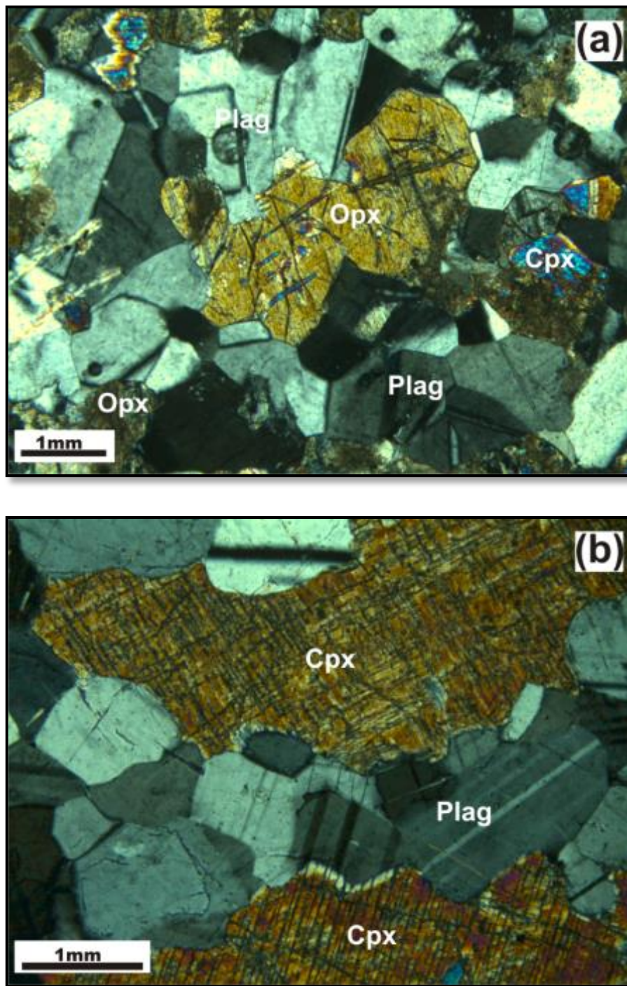
Fig. 4.10. Photomicrographs of (a) Micro norite with oikocrysts of orthopyroxene (Opx) with exsolution lamellae of clinopyroxene (Cpx) and plagioclase (Plag) in sample no. USM 1 under XPL (b) Micro gabbro with large oikocrysts of Cpx and cumulus plagioclase (Plag) in sample no. UNK 93-54 under XPL.
