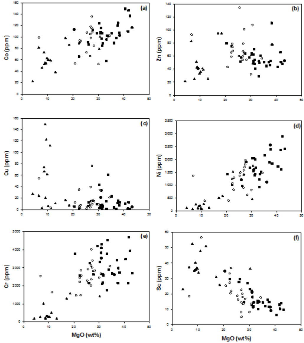
Fig. 6.5. Variation diagrams continued for trace elements plotted against MgO for the Unki xenolith samples. Closed squares (■) represent peridotites, open cycles (○) represent pyroxenites and closed triangles (▲) represent gabbros.
