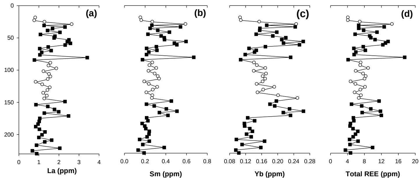
Fig. 5.8. Stratigraphic variation downhole of REE elements La, Sm, Yb and total (sum) REEs in the PAR 11 borehole. Open cycles (○) represent pyroxenite and closed squares (■) represent peridotites.
