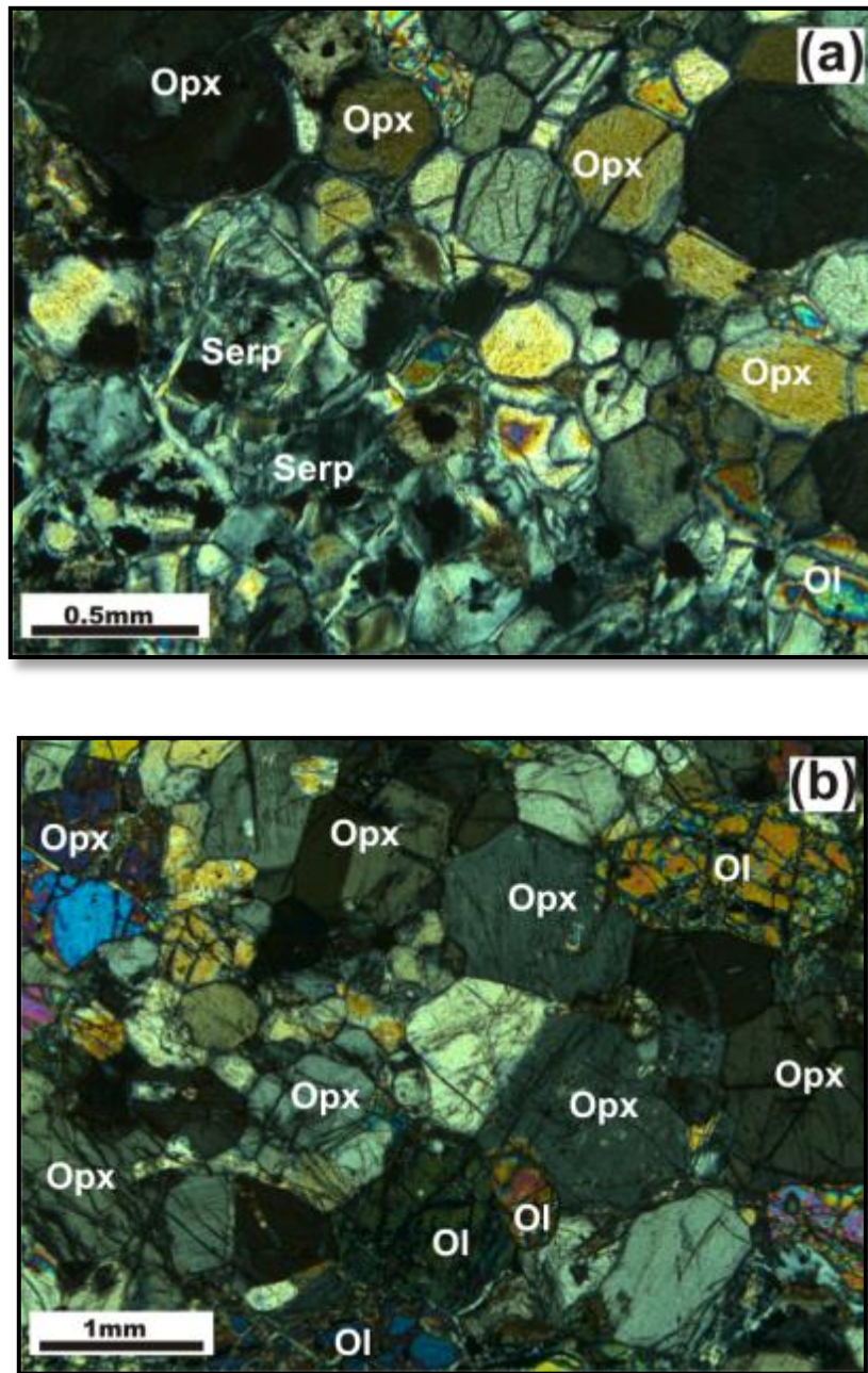
Fig. 4.4. Photomicrographs of harzburgites from the Selukwe xenolith suite. (a) Micro harzburgite with polygonal aggregates of orthopyroxene (Opx) and serpentinized (Serp) olivine grains and Olivine (Ol) in sample no. UNK 93-16 under XPL. (b) Medium grained harzburgite with polygonal aggregates of Opx and Ol central part of the thin section with minor spinel on the edges of the grains in sample no. UNK 93-26 under XPL.
