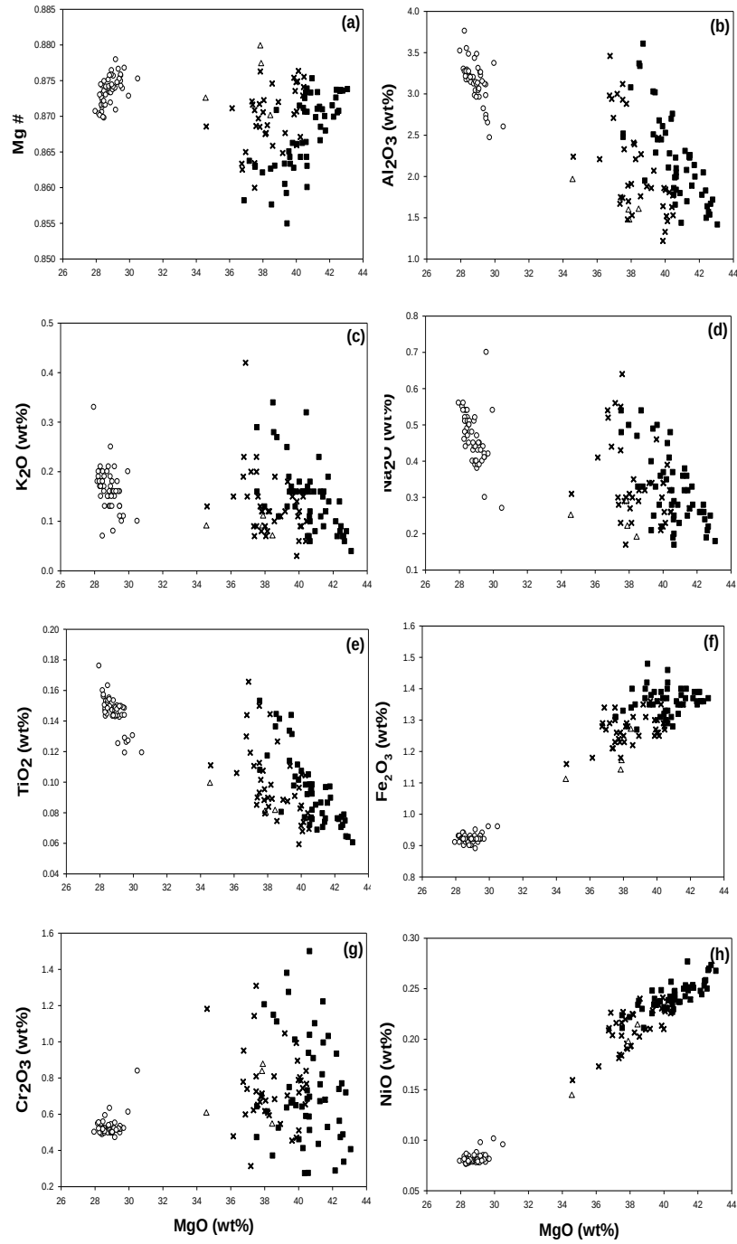
Fig. 5.3. Variation diagrams for major element oxides variation plotted against with MgO as an index of differentiation. Open cycles (○) represent pyroxenite, open triangles (Δ) represent olivine - pyroxenite, closed squares (■) represent dunites and (x) represent harzburgites.
