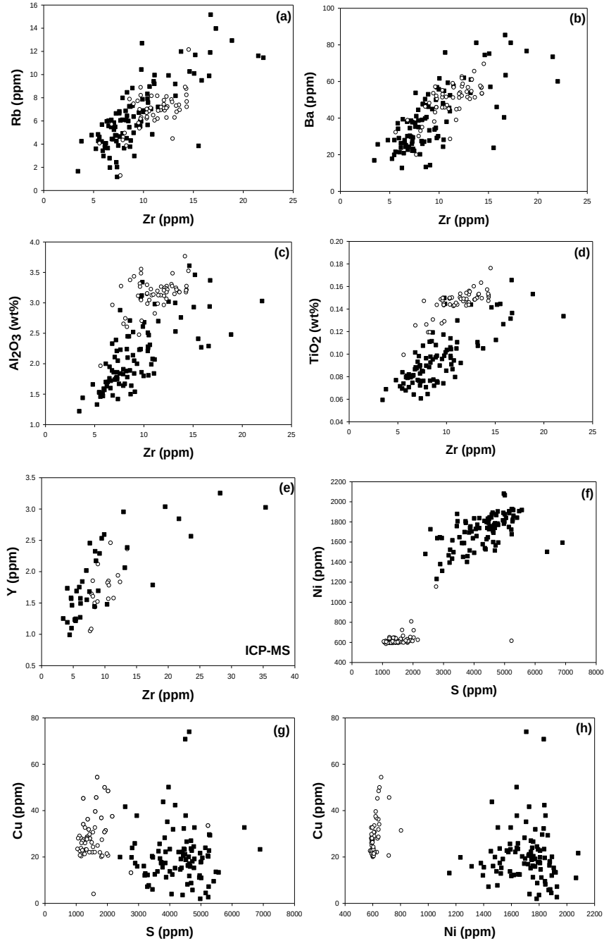
Fig. 5.7. Inter -element variation diagrams for trace elements (a) Rb vs Zr, (b) Ba vs Zr (c) Al 2 O 3 vs Zr, (d) Zr vs TiO 2 , (e) Zr vs Y, (f) Ni vs S, (g) Cu vs S, (h) Cu vs Ni. Open cycles (○) represent pyroxenite and closed squares (■) represent peridotites.
