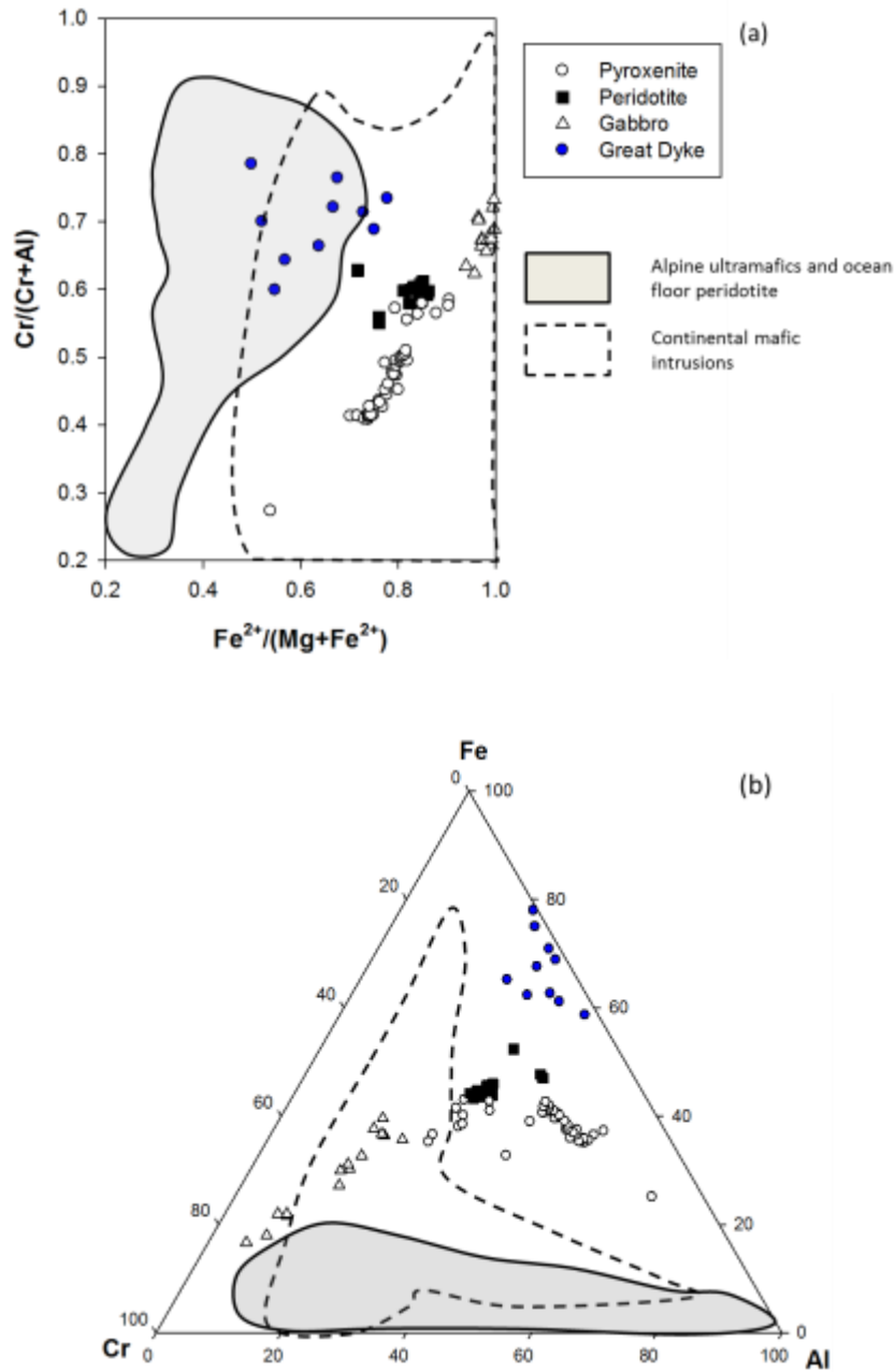
Fig. 8.7. Chromite variations for the xenolith suite in terms of the ratios (a) \text{Cr}/(\text{Cr}+\text{Al}) vs \text{Fe}^{2+}/(\text{Mg}+\text{Fe}^{2+}) (b) Plot of the trivalent cations \text{Al}^{3+} - \text{Cr}^{3+} - \text{Fe}^{3+} compared with Great Dyke (Wilson, 1982) chromitites, alpine ultramafics, ocean floor peridotite and continental mafic intrusions (Barnes and Roeder, 2001).
