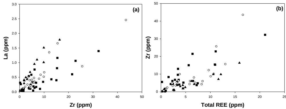
Fig. 6.7. Variations of (LREE) La (ppm) and Total REE (ppm) with incompatible element Zr (ppm) in the Unki xenolith suite Closed squares (■) represent peridotites, open cycles (○) represent pyroxenites and closed triangles (▲) represent gabbros.
