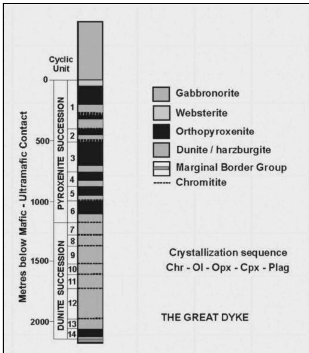
Fig 10.1. Crystallization sequence of the Great Dyke (Coghill et al. , 1993) as observed in the cyclic units of the Darwendale Subchamber. The order of crystallization in all five subchambers is chromite, olivine, orthopyroxene, clinopyroxene and plagioclase.
