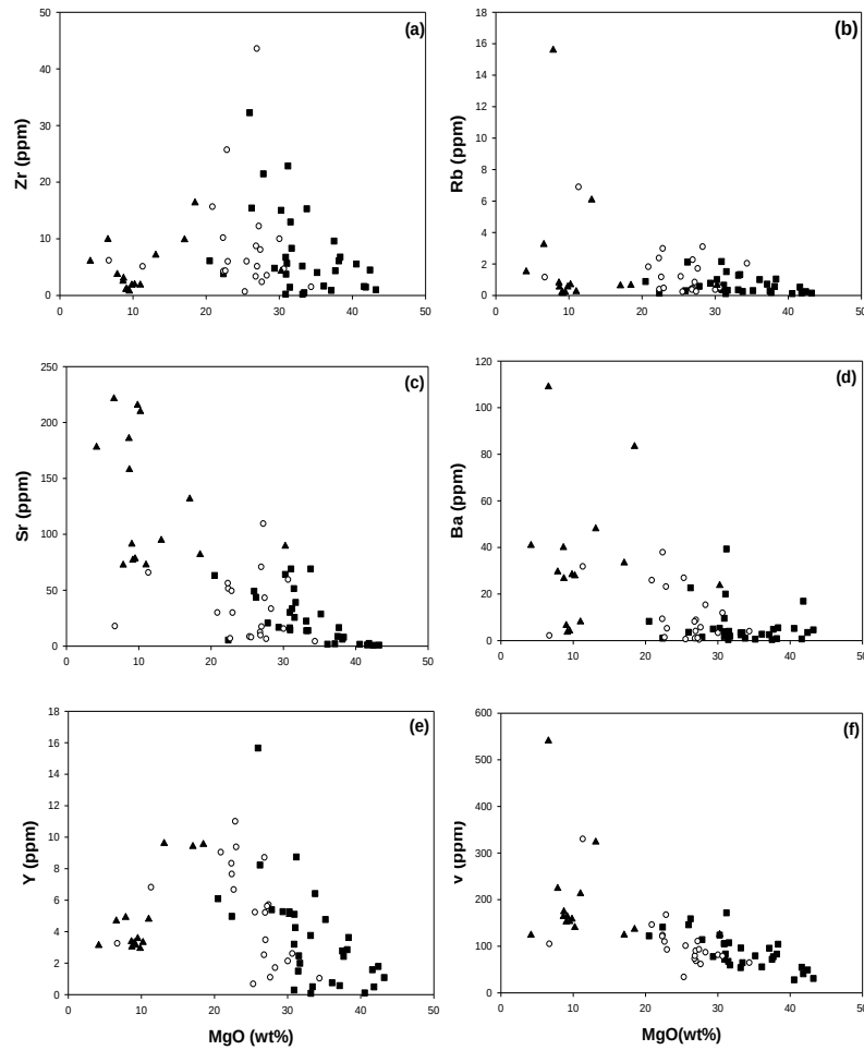
Fig. 6.4. Variation diagrams for trace elements plotted against MgO for the Unki xenolith samples. Closed squares (■) represent peridotites, open cycles (○) represent pyroxenites and closed triangles (▲) represent gabbros.
