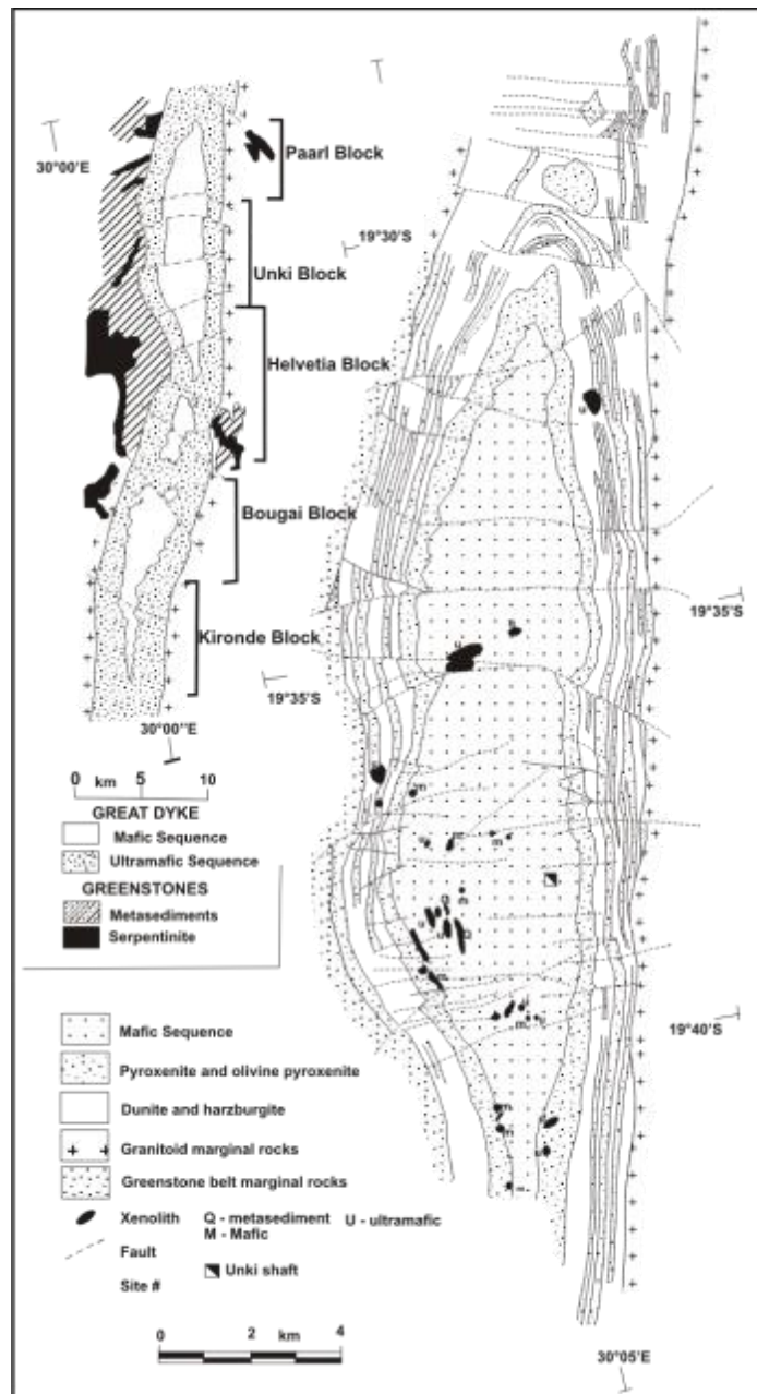
Fig. 2.1. The geology of the north-central zone of the Selukwe Subchamber. The simplified large- scale map shows the location of the Selukwe greenstone belt on the west contact of the subchamber. The various mining blocks are indicated. The map shown in greater detail is an outcrop and covers the Unki Block and parts of the Paarl and Helvetia Block. Also shown are fragments of xenolithic and autolithic suite (Wilson et al. , 2000a).
