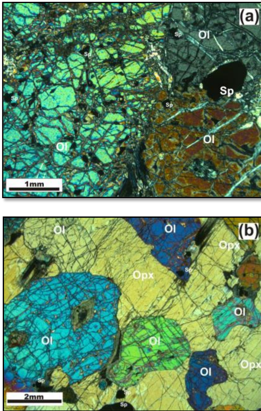
Fig. 4.1. (a) Photomicrograph of dunite with coarse crystals of olivine (Ol) enclosing fine crystals of spinel (Sp) in sample no. PAR 11-104 under XPL (b) Photomicrograph of harzburgite with large grains of olivine (Ol) enclosed in a large grain of orthopyroxene (Opx). There are fine grains of spinel (Sp) enclosed in the olivine in sample no. PAR 11-133 under XPL.
