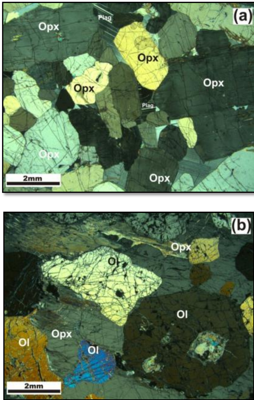
Fig. 4.2. (a) Photomicrograph of pyroxenite displaying tabular orthopyroxene (Opx) grains with well- developed triple junction points and postcumulus plagioclase (Plag) in sample no. PAR 11-53 under XPL. (b) Photomicrograph of olivine-pyroxenite with optically continuous orthopyroxene (Opx) enclosing and olivine (Ol) in sample no. PAR 11-149 under XPL. There are crystallized melt inclusions are within the olivine.
