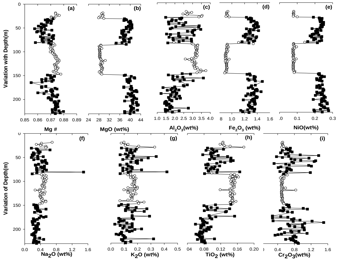
Fig. 5.4. Whole rock major element oxides variations with depth for the PAR 11 borehole. Open cycles (○) represent pyroxenite closed squares (■) represent peridotites.
