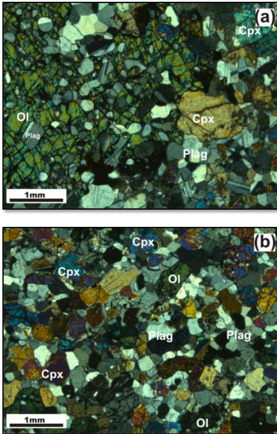
Fig. 4.12. Photomicrographs of (a) Micro-olivine gabbro with olivine (Ol), clinopyroxene (Cpx) and plagioclase (Plag). The large oikocryts of olivine encloses smaller grains of plagioclase in sample no. USM 4 under XPL (b) The micro olivine gabbro displays an equigranular texture in sample no. USM 66 under XPL.
