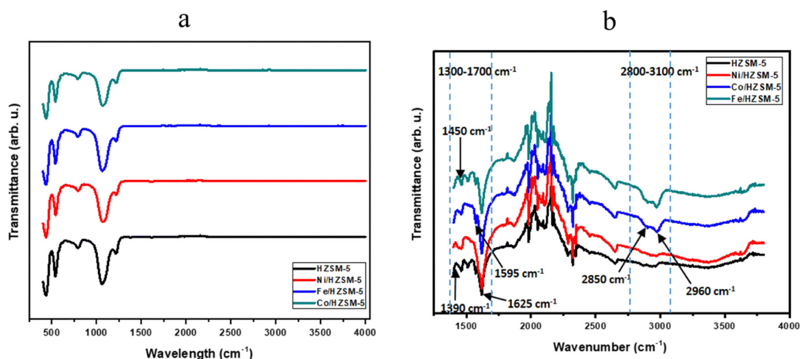
Fig. 9 FTIR spectra of coked metal doped HZSM-5 catalyst after the conversion of C_1 – C_3 alcohols to hydrocarbons at 350 °C and WSHV = 7 h -1 : (a) full spectral range (400–4000 cm^{-1} ) showing overall functional group vibrations; (b) expanded region (1300–3800 cm^{-1} ) highlighting characteristic bands associated with coke formation, including aliphatic, olefinic, and aromatic hydrocarbon species. Reproduced from ref. 42 with permission from Royal Society of Chemistry (RCS), copyright 2024.
