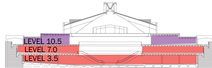
SECTION C-C
