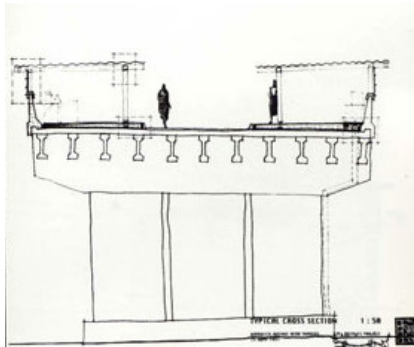
Fig 7.33 Warwick Junction market precinct, OMM Design Workshop market road bridge elevation (Courtesy OMM Design Workshop) Fig 7.34 Warwick Junction market precinct, OMM Design Workshop new multi market stalls section (Courtesy OMM Design Workshop)
