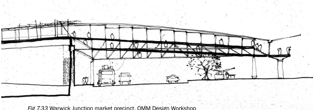
Fig 7.33 Warwick Junction market precinct, OMM Design Workshop market road bridge elevation (Courtesy OMM Design Workshop) Fig 7.34 Warwick Junction market precinct, OMM Design Workshop new multi market stalls section (Courtesy OMM Design Workshop)
