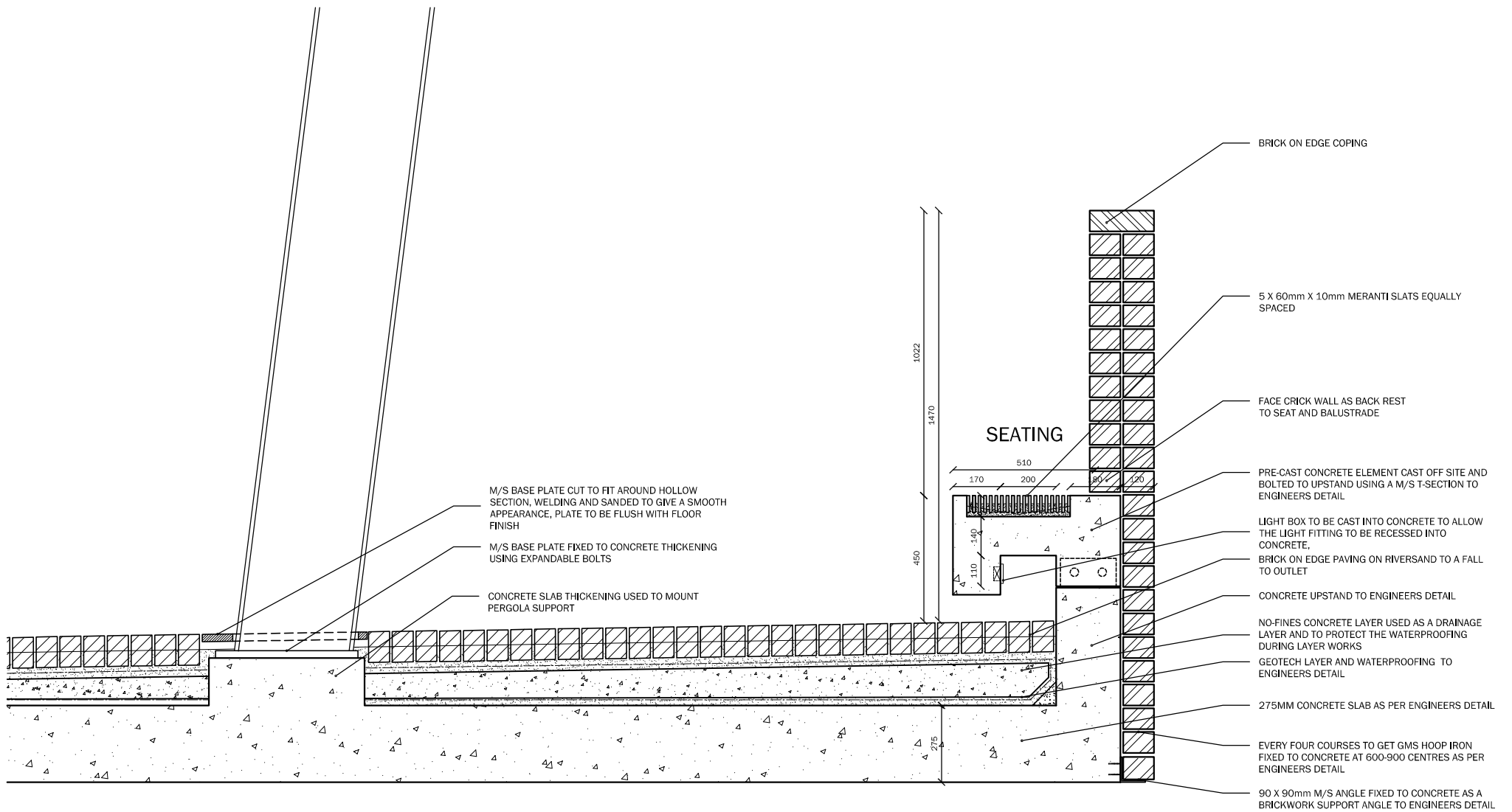
DETAIL SECTION SCALE 1:20
