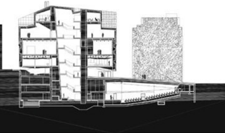
Fig 7.19 The Caixa Forum, Herzog and de Meuron Architects, 2008 section through plaza (Image @ Christian Richters, www.arcspace.com/architects )
