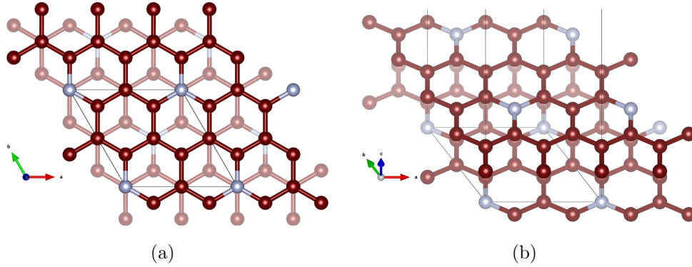
Figure 2.1: AB configuration for nitrogen incorporated graphene from (a) viewpoint perpendicular to the basal (b) rotated view. Carbon atoms maroon while nitrogen atoms are white.
