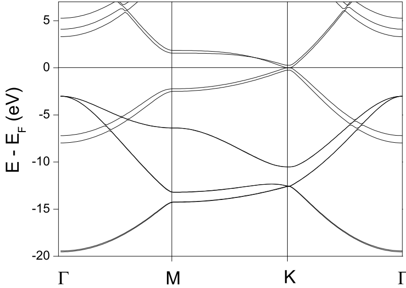
Figure 2.3: Band structure of pristine bilayer graphene in the AB stacking configuration.
