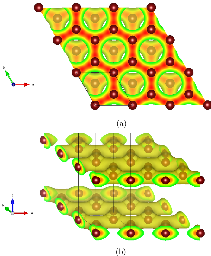
Figure 2.14: Charge density of pristine bilayer graphene in the AB configuration (a) view from above (b) viewed at an angle.
