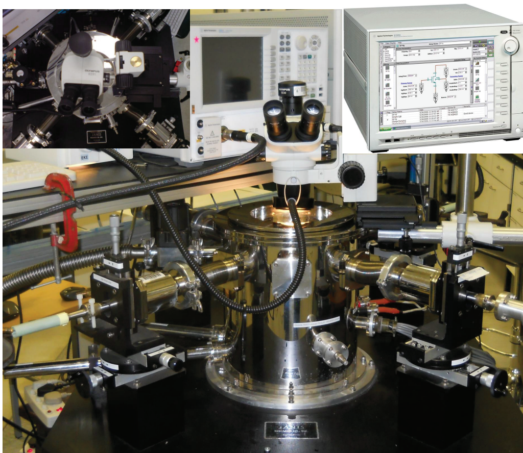
Figure 4.1: Janis micromanipulated probe station. Upper left inset: Viewed from above. Upper right inset: Agilent B1500A Semiconductor Device Analyser.
