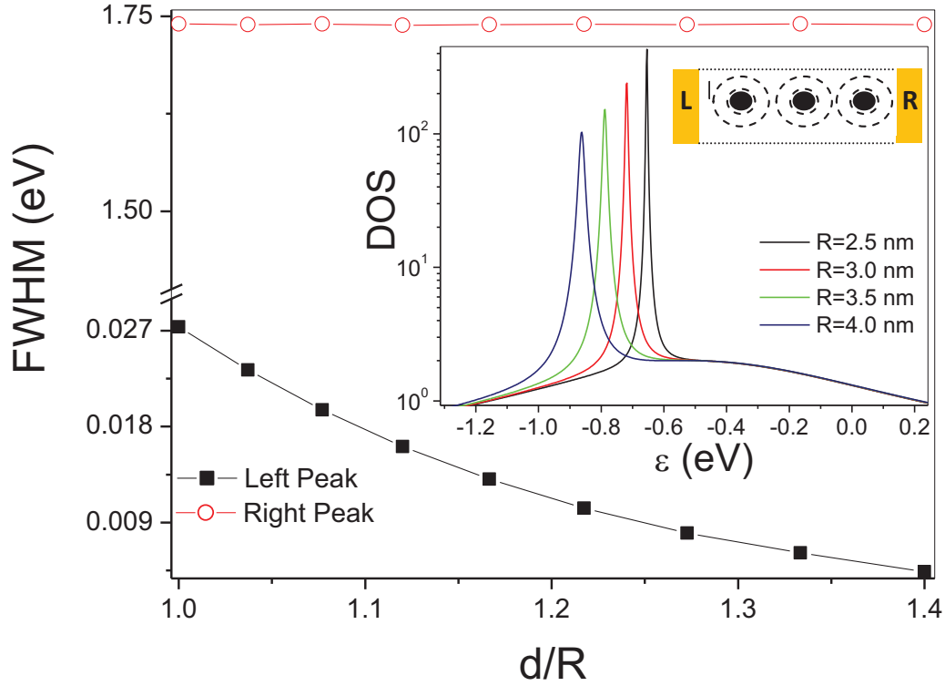
Figure 3.3: FWHM for the horizontal configuration with changing inter-cluster size, from 2.5 to 4 nm, as a function of the scaling factor d/R . Inset are the corresponding DOS spectra as a function of \epsilon .
