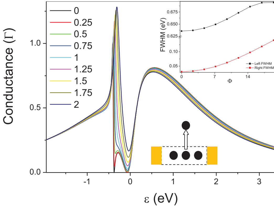
Figure 3.9: Conductance spectra as the central cluster is shifted vertically from the horizontal where each curve corresponds to a different vertical separation of the central cluster measured from the horizontal plane of the outer clusters, ranging from 0 to 2 nm. Inset is the FWHM of the DOS peaks as a function of the angle between the outer clusters and the central cluster.
