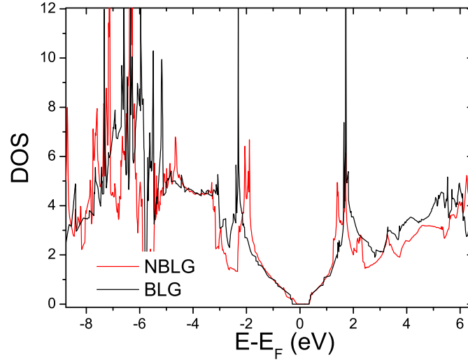
Figure 2.10: Density of states for pristine bilayer graphene (black) and nitrogen incorporated bilayer graphene (red) in the AB stacking configuration the nitrogen incorporated DOS shifted.
