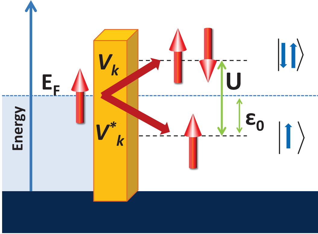
Figure 6.1: Schematic diagram of the Anderson single impurity model.
