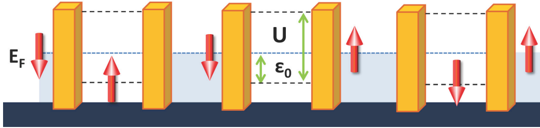
Figure 6.2: Schematic diagram of a conserved tunneling process within the Anderson impurity model.
