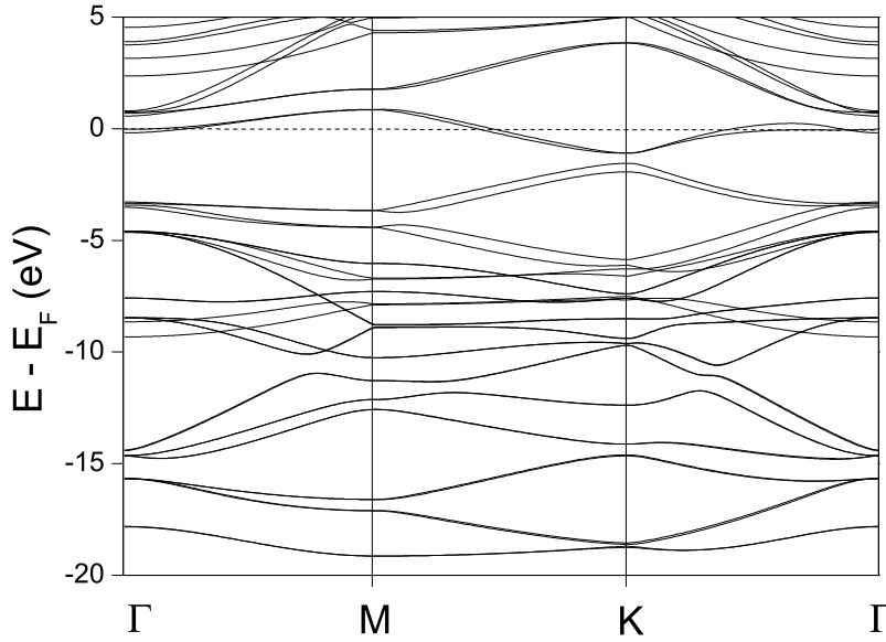
Figure 2.5: Band structure of nitrogen incorporated bilayer graphene in the AB stacking configuration.
