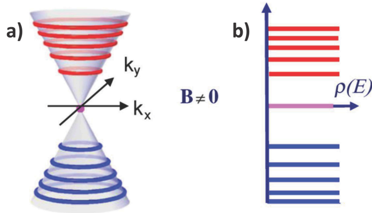
Figure 1.2: a) Landau levels represented on the Dirac cone of graphene under an external field. b) Schematic density of states under an applied field. Image from [16].
