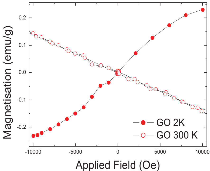
Figure 5.5: Hysteresis curves of GO at 300 K and 2 K indicating diamagnetism and ferromagnetism respectively.
