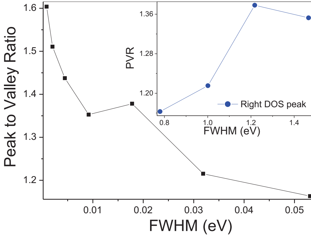
Figure 3.5: Peak to valley ratio of the resonant tunnelling feature as a function of the FWHM of the left (narrow) DOS peak. Inset: The corresponding curve as a function of the right (broad) DOS peak FWHM.
