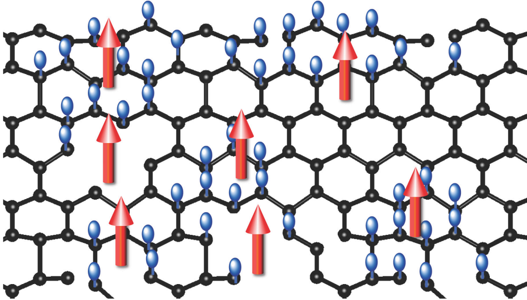
Figure 6.7: Schematic diagram of local moment formation in RGO. Local moments (red arrows) form at residual free radicals (blue spheres) which are attached to the basal graphene plane and vacancies in the lattice. Extended states may form in unfunctionalized graphene regions.
