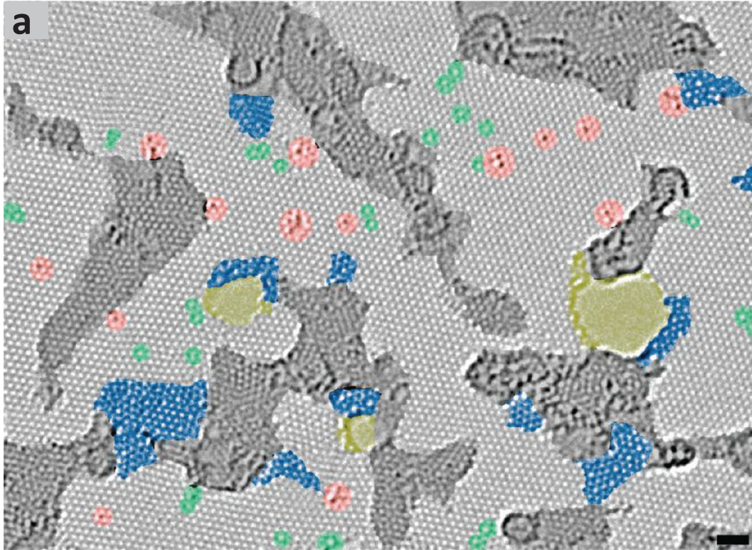
Figure 1.7: Atomic resolution transmission electron microscope image of reduced graphene oxide. The scale bar represents 1 nm . Dark grey regions represent residual functionalized regions and red regions represent individual adatoms. Blue regions represent regions dominated by topographical defects while green regions represent individual topographical defects. Vacancies are shaded yellow. Figure from [63].
