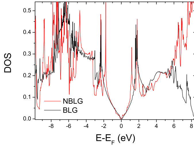
Figure 2.12: Comparison of density of states of AA stacked bilayer graphene (black) and nitrogen incorporated bilayer graphene (red) with the nitrogen incorporated shifted.
