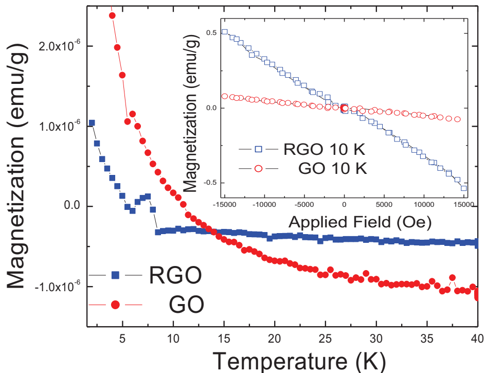
Figure 5.4: Magnetization as a function of temperature for GO and RGO. Inset is the magnetization of GO and RGO as a function of applied field at 10 K.
