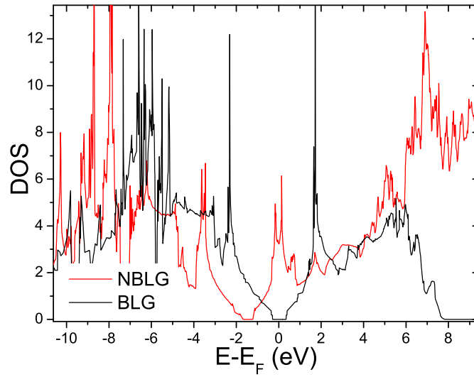
Figure 2.9: Density of states for pristine bilayer graphene (black) and nitrogen incorporated bilayer graphene (red) in the AB stacking configuration.
