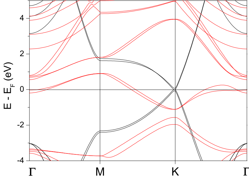
Figure 2.7: Comparison of the band structure of pristine (black) and nitrogen incorporated (red) bilayer graphene in the AB stacking configuration.
