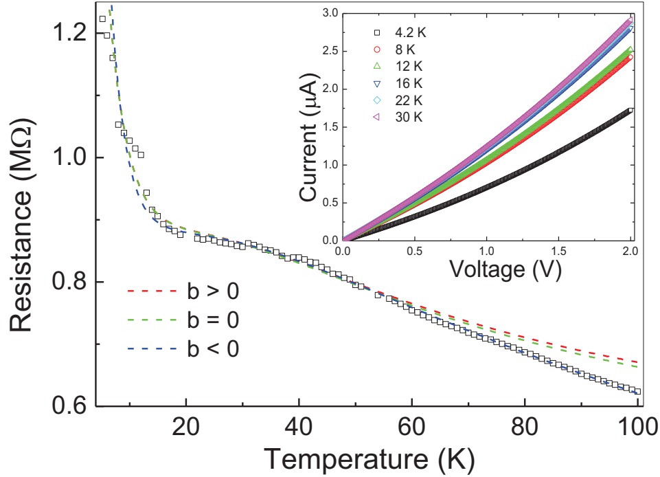
Figure 5.3: Resistance as a function of temperature in RGO. The dashed lines are fits to the data with the suggested model e.g. for b > 0 , b = 0 and b < 0 . Upper inset: Low temperature I - V measurements of RGO.
