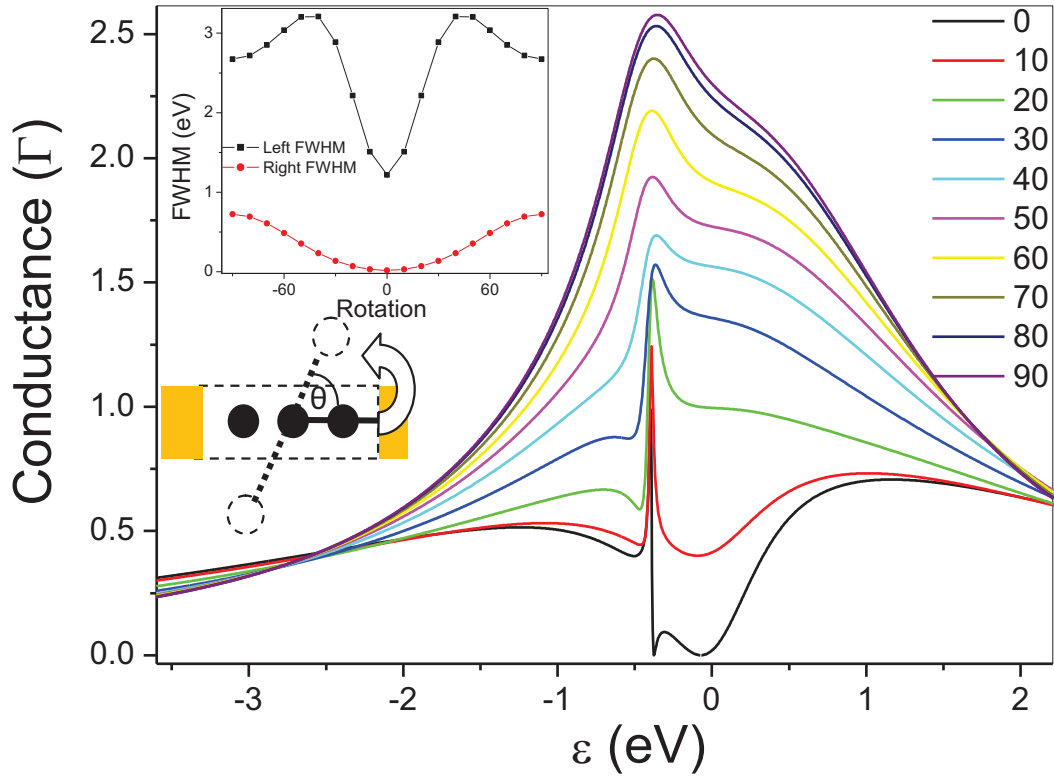
Figure 3.6: Conductance spectra as the horizontal configuration is rotated to the vertical configuration, each curve corresponds to a different angle measured from the horizontal. Inset is the FWHM of the corresponding DOS spectra as a function of the rotation angle from the horizontal.
