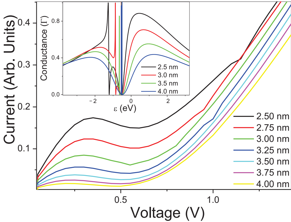
Figure 3.4: I - V curves for the horizontal configuration with changing inter-cluster separation, from 2.5 to 4 nm. Inset: the corresponding conductance spectra as a function of \epsilon .
