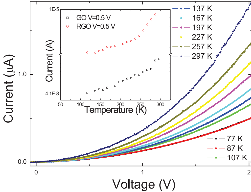
Figure 5.1: I - V measurements for GO. Inset: Current as a function of temperature for GO and RGO.
