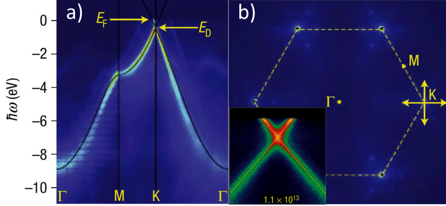
Figure 1.3: a) The band structure of graphene determined through angle-resolved photo-emission spectroscopy. b) Constant energy map of at the binding energy of the Dirac point, illustration the Brillouin zone of graphene. Image from [28].
