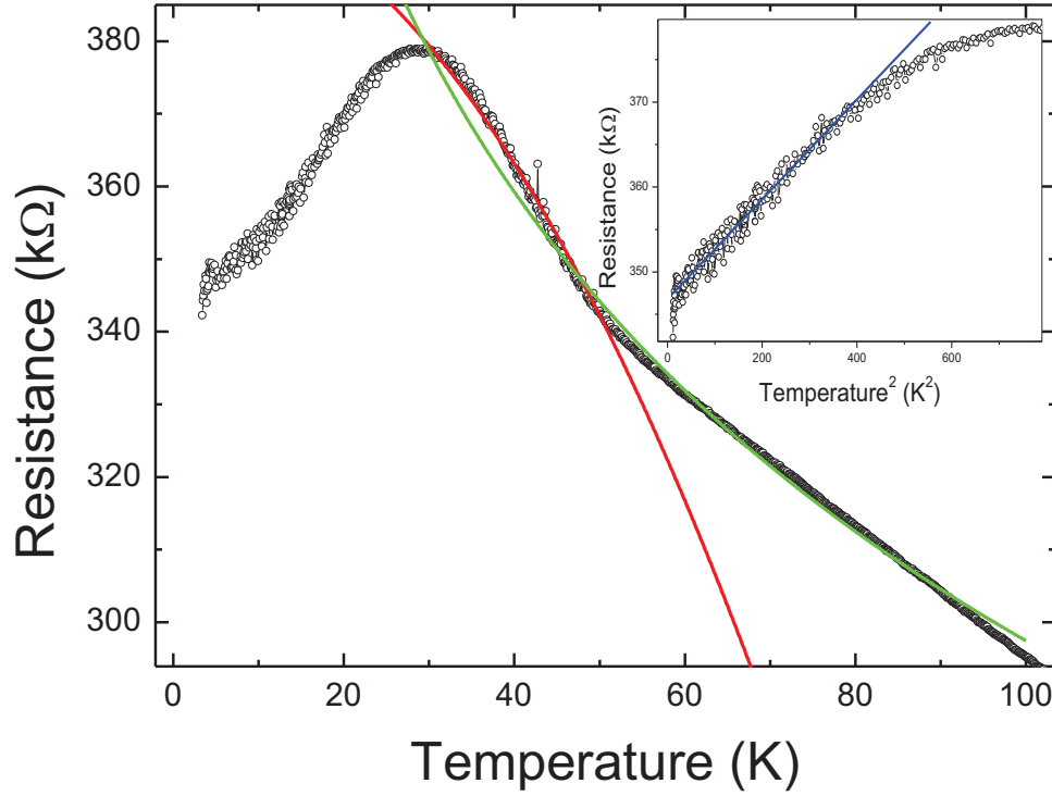
Figure 6.3: Resistance versus temperature of RGO. The solid red line is a fit to a quadratic temperature dependence while the green solid line is a fit to a logarithmic temperature dependence. Inset is the low temperature resistance plotted as a function of the temperature squared.
