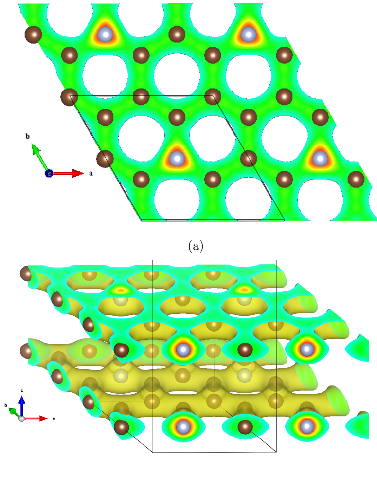
Figure 2.16: (a) Charge density of nitrogen incorporated bilayer graphene in the AA configuration. (b) Viewed at an angle
