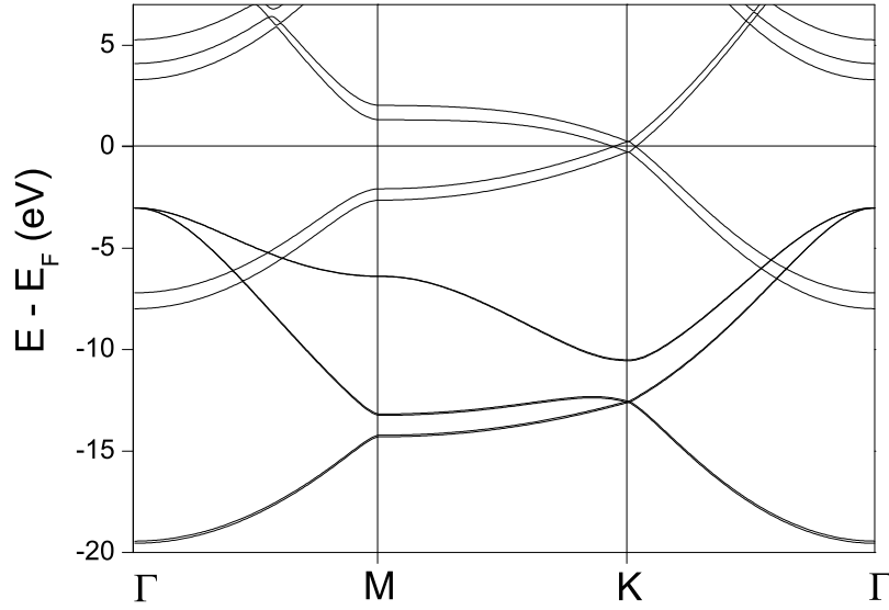
Figure 2.4: Band structure of pristine bilayer graphene in the AA stacking configuration.
