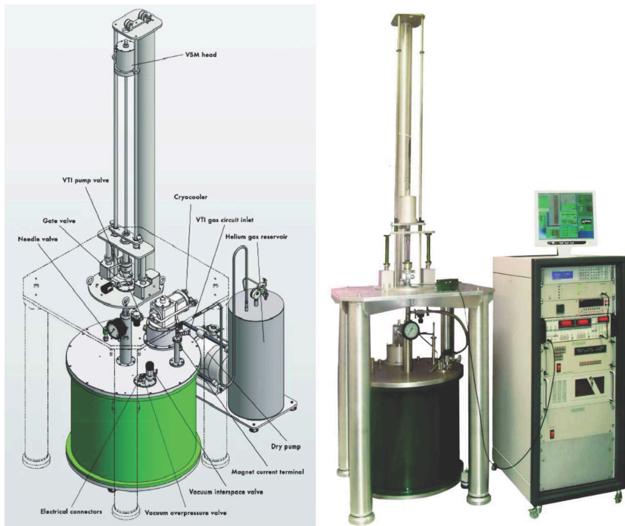
Figure 4.2: Cryogenic free measurement system.
