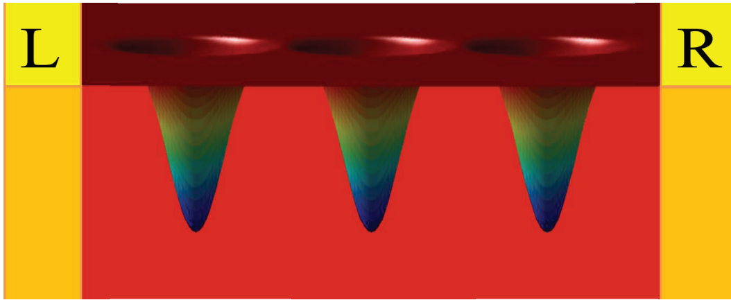
Figure 3.1: Schematic 3D diagram of the impurity cluster system including the leads and the 2D Gaussian potential. The regions in red indicate the high bandgap matrix while the multicoloured regions indicate the impurity cluster potential.
