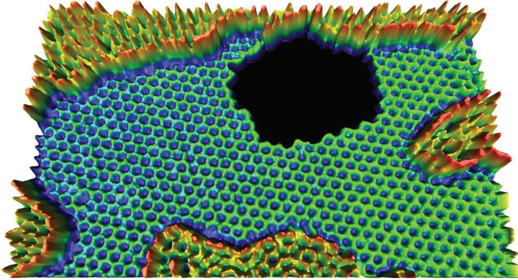
Figure 1.6: 3D image of the atomic structure of graphene with a vacancy. Image from [53]. In this study the rearrangement of carbon atoms at the edge of the vacancy was imaged in real time with an atomic resolution transmission electron microscope.
