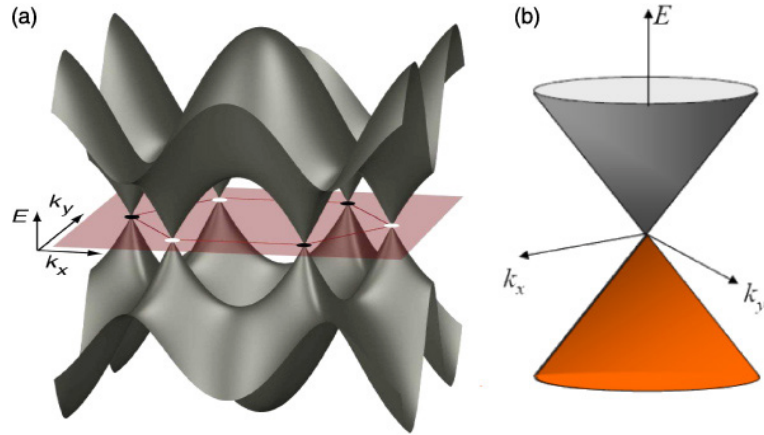
Figure 1.1: a) A 3D tight-binding band structure plot of graphene. b) The band structure in the region of the K points. Image from [15].
