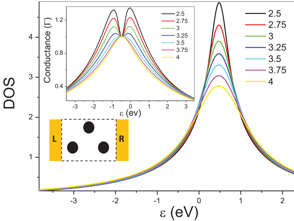
Figure 3.10: DOS spectra in the triangular configuration (equilateral) with increasing uniform inter-cluster separation from 2.5 nm to 4 nm. The corresponding conductance spectra are inset.
