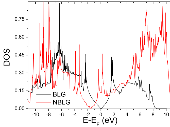
Figure 2.11: Density of states of AA stacked bilayer graphene (black) and nitrogen incorporated bilayer graphene (red).
