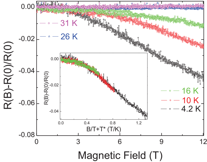
Figure 6.4: Magneto-resistance of RGO. Inset is the MR scaled with the characteristic temperature.
