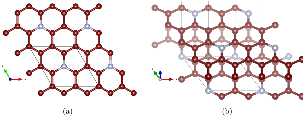
Figure 2.2: AA configuration for nitrogen incorporated graphene from (a) viewpoint perpendicular to the basal graphene plane and (b) a rotated view.
