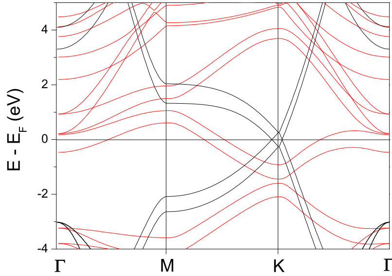
Figure 2.8: Comparison of the band structure of pristine (black) and nitrogen incorporated (red) bilayer graphene in the AA stacking configuration.
