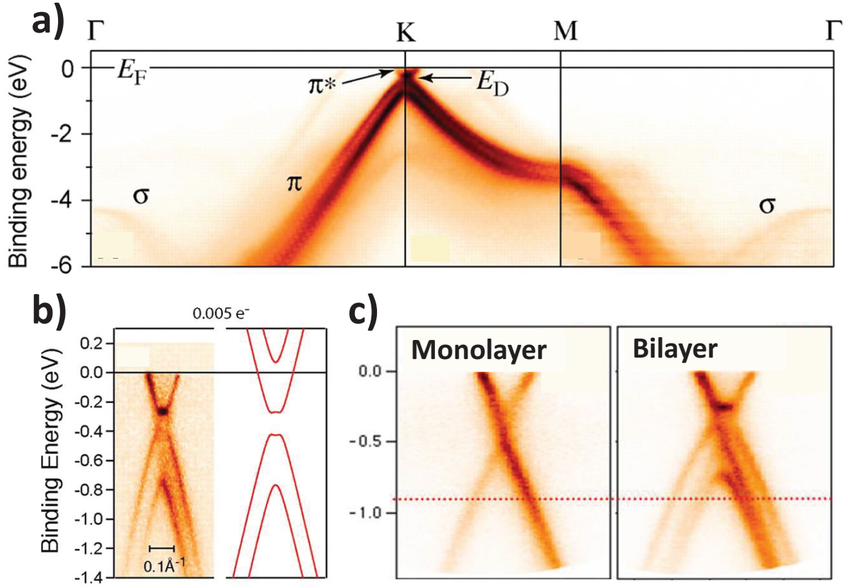
Figure 1.5: a) Band structure of bilayer graphene determined through angle-resolved photo-emission spectroscopy. b) Band structure close to the K point. c) Comparison of the band structure for monolayer and bilayer graphene close to the K point. Image from [26].
