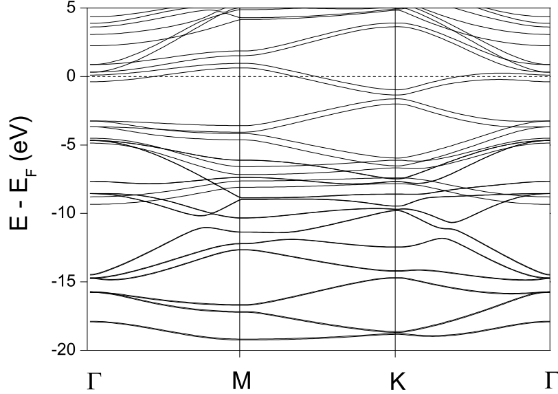
Figure 2.6: Band structure of nitrogen incorporated bilayer graphene in the AA stacking configuration.
