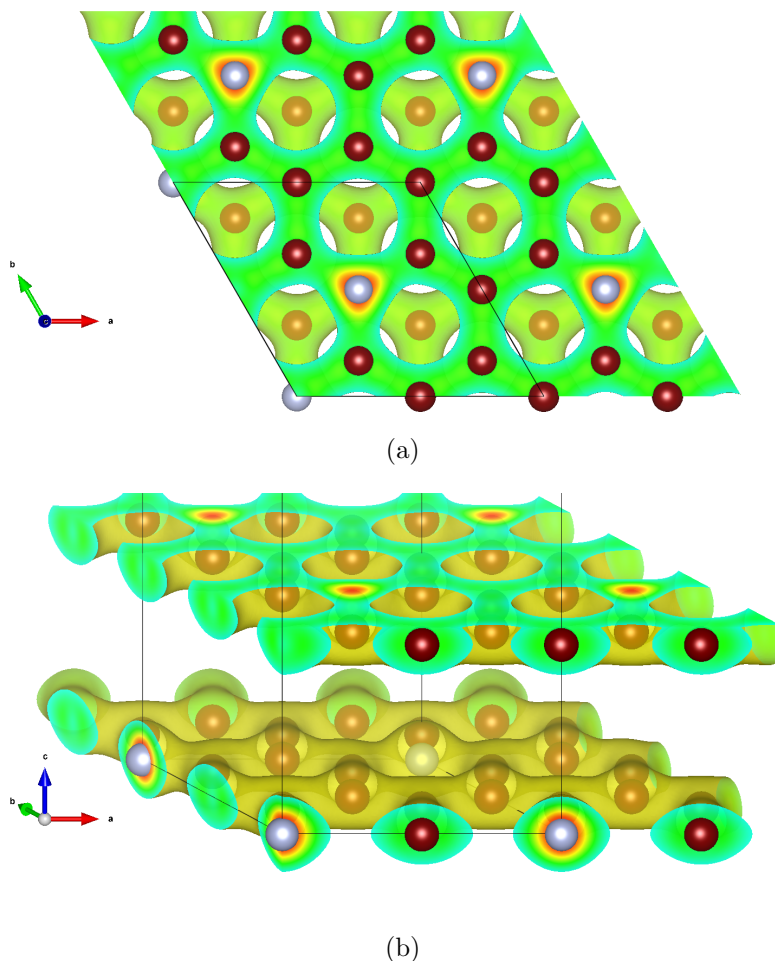
Figure 2.15: Charge density of nitrogen incorporated bilayer graphene in the AB configuration (a) view from above (b) viewed at an angle.
