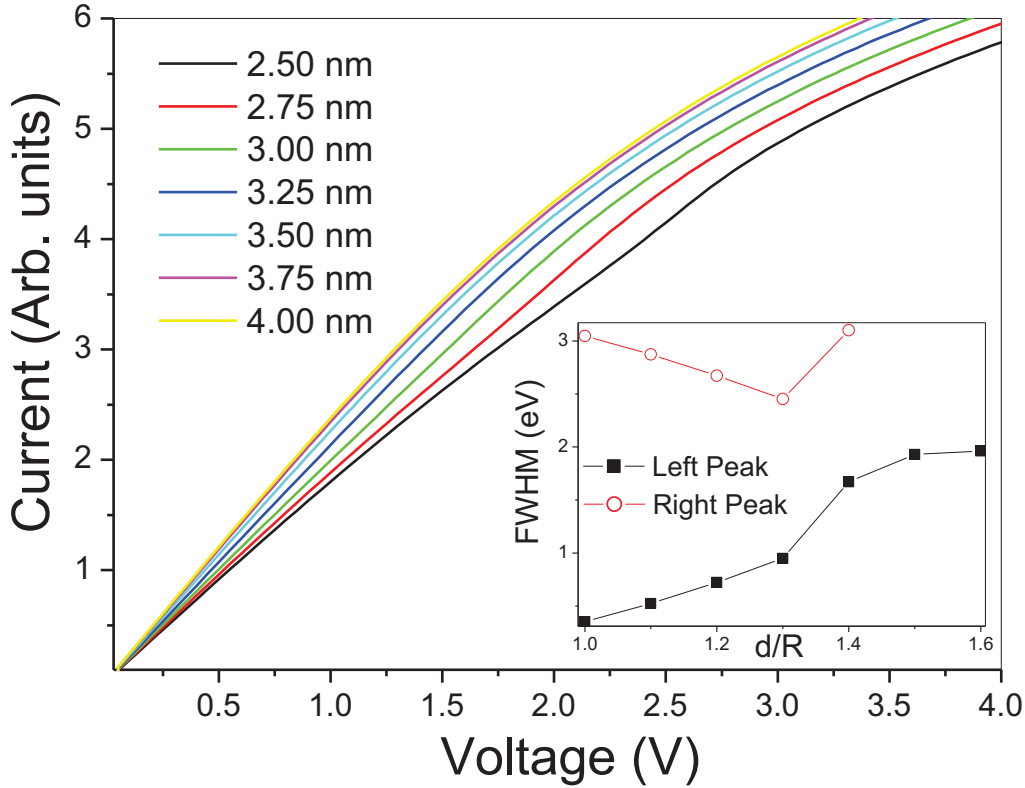
Figure 3.8: I-V curves for the vertical configuration with increasing vertical inter-cluster separation, from 2.5 to 4 nm. The FWHM of the corresponding DOS spectra as a function of the scaling factor d/R is inset.
