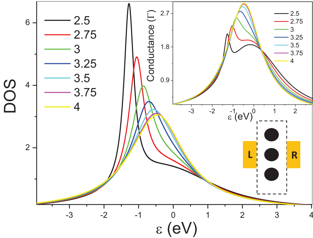
Figure 3.7: DOS spectra in the vertical configuration with changing inter-cluster separation, from 2.5 to 4 nm, as a function of \epsilon . Inset are the corresponding conductance spectra as a function of \epsilon .
