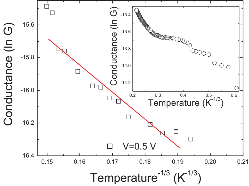
Figure 5.2: Logarithmic conductance of GO as a function of T^{-1/3} . Inset: the corresponding plot for RGO.
