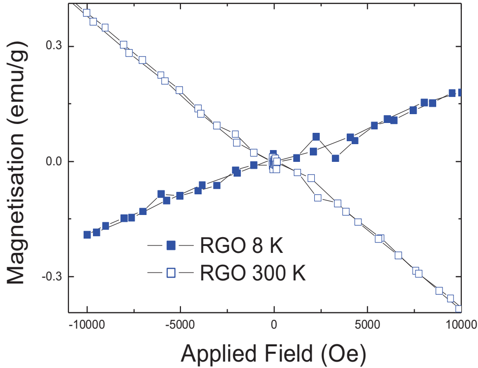
Figure 5.6: Hysteresis curves of RGO at 300 K and 8 K indicating diamagnetism and ferromagnetism respectively.
