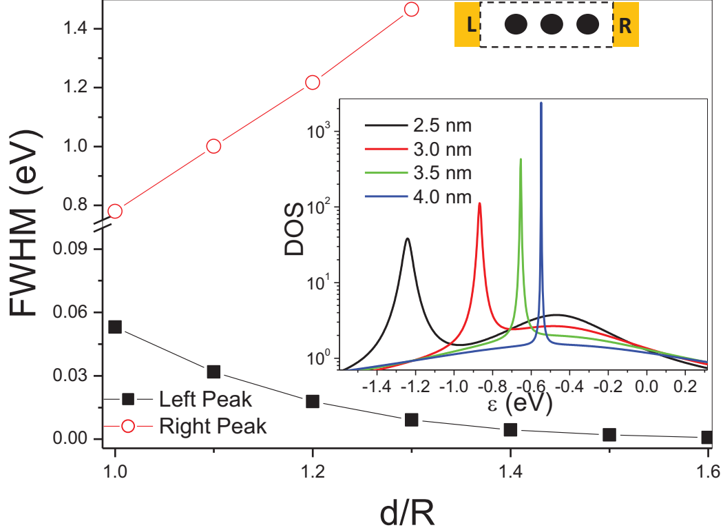
Figure 3.2: FWHM for the horizontal configuration with changing inter-cluster separation as a function of the scaling factor d/R defined as the ratio of inter-cluster separation to cluster size. Inset are the corresponding DOS spectra, for inter-cluster separations ranging from 2.5 to 4 nm, as a function of \epsilon = E_F - E (for all figures).
