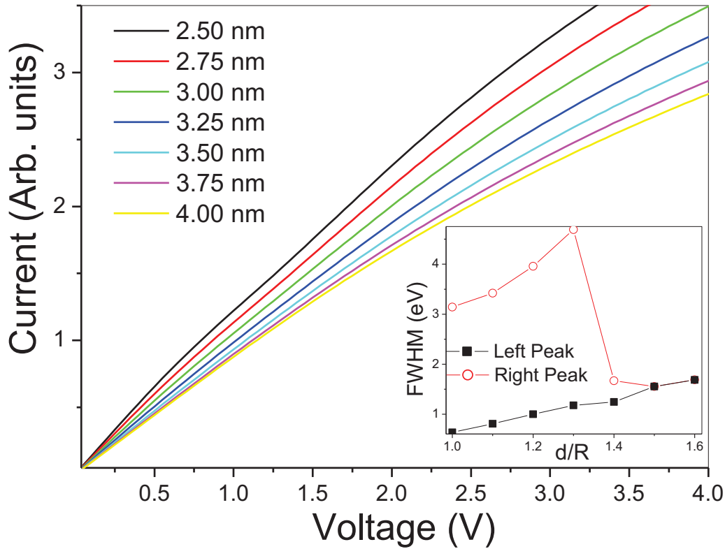
Figure 3.11: I-V curves for the triangular configuration (equilateral) with increasing inter-cluster separation, from 2.5 to 4 nm. The FWHM of the corresponding DOS spectra as a function of the scaling factor d/R is inset.
