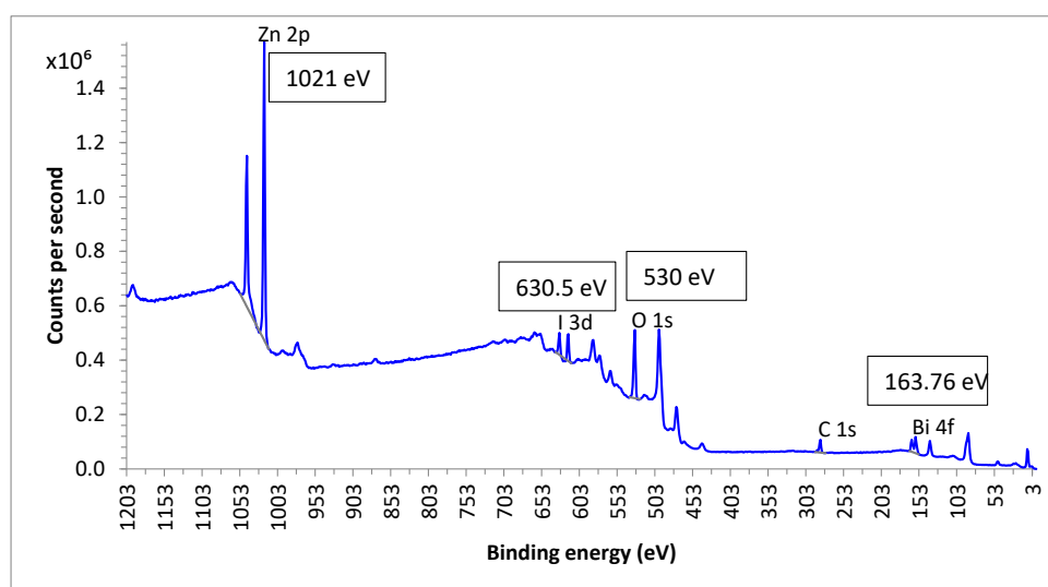
Figure 12. XPS spectra of the ZnO-[10%]BiOI heterojunction.
