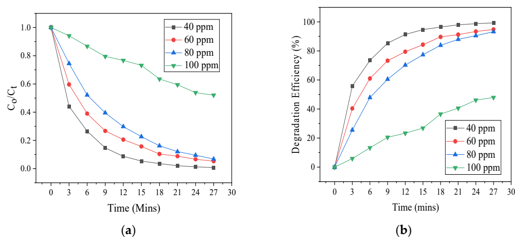
Figure 7. (a) Photodegradation of \text{SCN}^- at varying concentration (b) degradation efficiencies.
