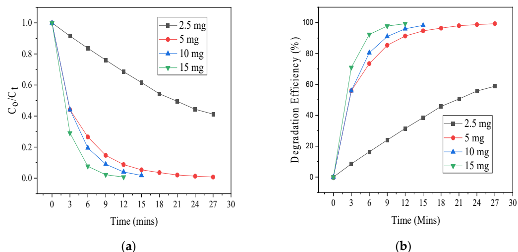
Figure 6. (a) Photodegradation of 40 ppm \text{SCN}^- at varying initial ZnO-[10%]BiOI dosage (b) photodegradation efficiencies.
