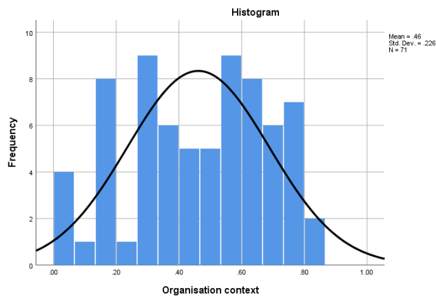
Figure 10: Philanthropic histogram
