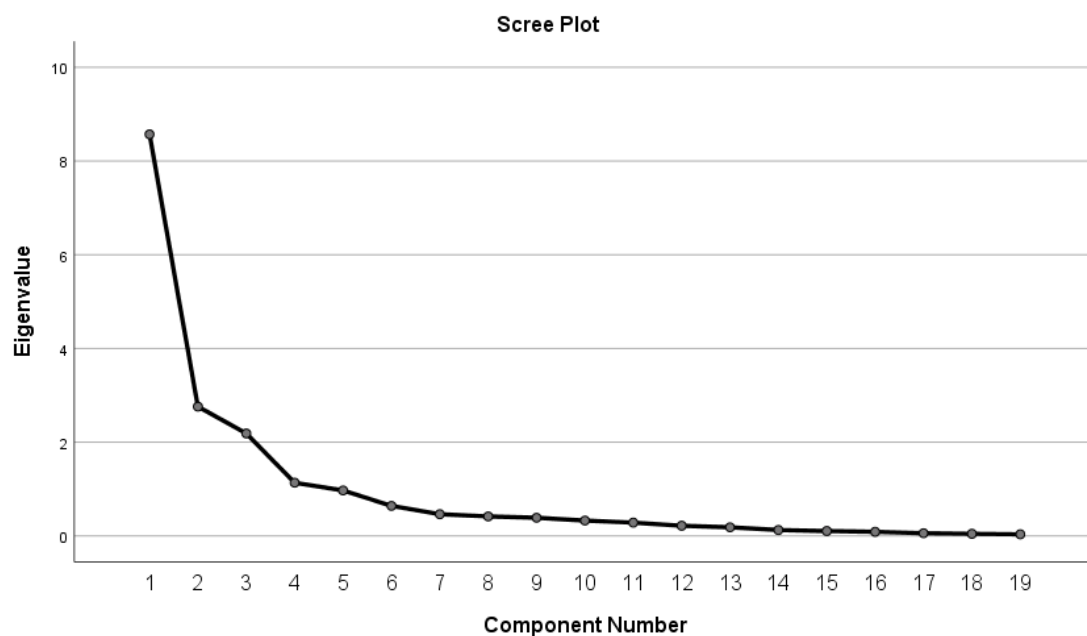
Figure 9:Scree plot
