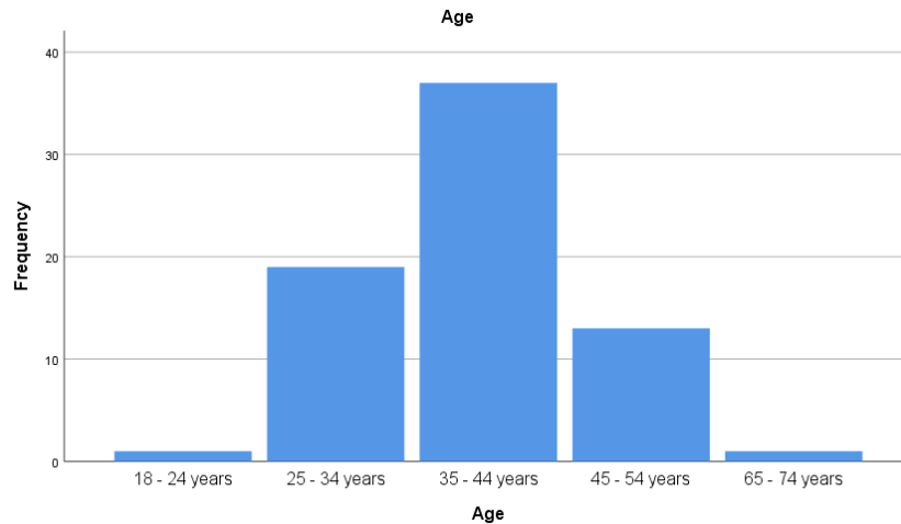
Figure 19: Age distribution
