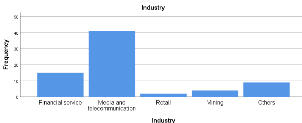
Figure 21: Industry distribution
