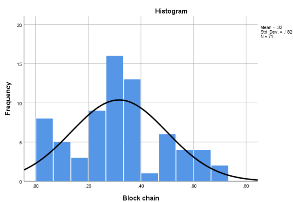
Figure 16: blockchain histogram
