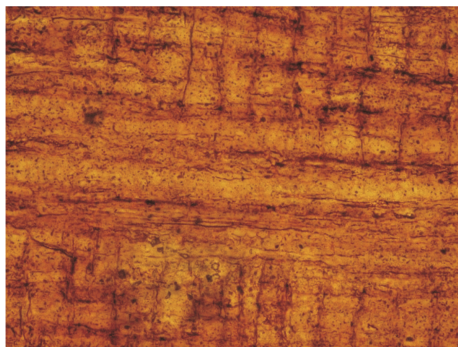
Figure 7. Photomicrographs of sample BP-16-1957. Top , a transverse section (ts) showing a growth ring with narrow latewood (thick-walled cells). Bottom , BP-16-1957 a radial longitudinal section (rls) with ghosts of biseriate, alternate bordered pits.
