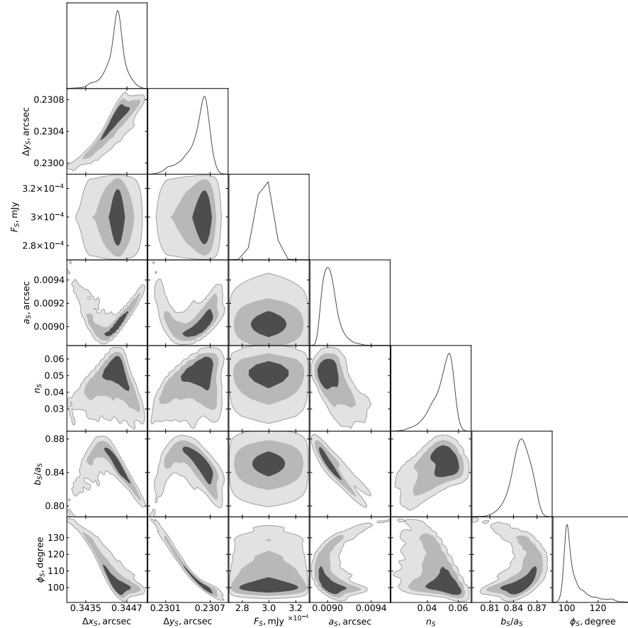
Figure 3. Source parameter degeneracy assuming the SIE ( \tilde{S}_V ) lens model. The contours show the 68%, 95%, and 98% confidence regions.
