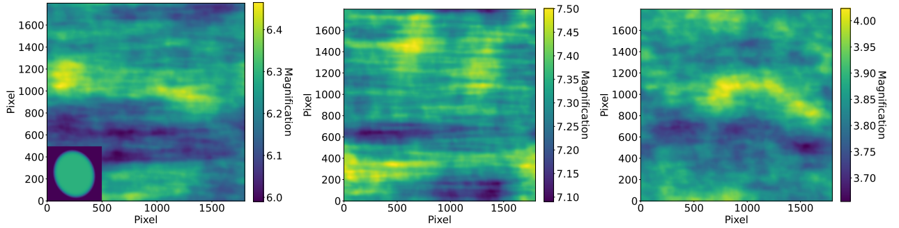
Figure 5. Representative magnification maps for image A, B, and C with f_{PBH} = 0.5 and \gamma = -1 after convolution with our best-fit Sérsic profile in Table 3. The shape of the source Sérsic profile is illustrated in the bottom left corner.
