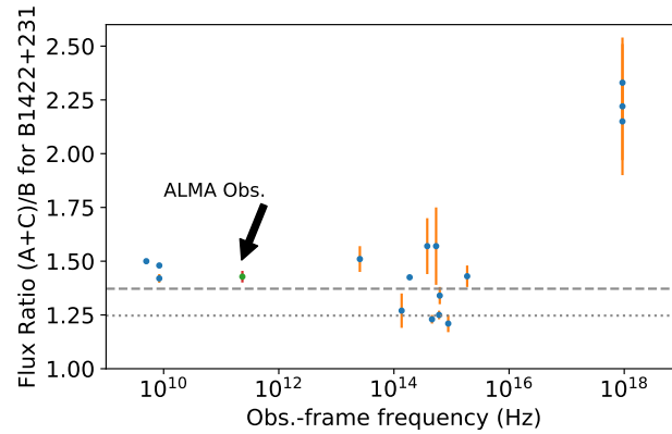
Figure 2. Flux density ratio anomalies as a function of observing frequency [51–53,55–57]. The orange error bars of flux density ratios are calculated from the individual lensed image flux densities and associated error bars reported in the literature, following the standard propagation of uncertainties. Our ALMA Band 6 observation labeled with an arrow shows a flux density ratio of (A+C)/B = 1.434 \pm 0.017 , consistent with measurements in radio and mid-infrared frequencies. The dotted and dashed horizontal lines show the predictions of the best-fit smooth lens model by Xu et al. [44], (A+C)/B = 1.247 and by Schechter et al. [58], (A+C)/B = 1.372 . Data points with large deviation from the horizontal lines exhibit large flux density ratio anomalies.
