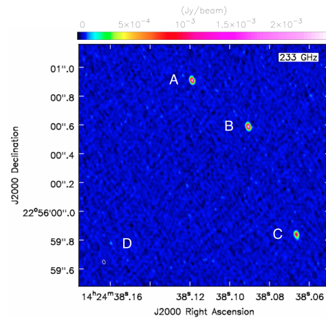
Figure 1. Naturally weighted ALMA Band 6 continuum map of B1422+231 at 233 GHz over a 7.5 GHz total bandwidth. The size of the restoring beam is 0.045'' \times 0.022'' , shown in the bottom-left corner. The rms noise level is 11 \mu\text{Jy beam}^{-1} . Four unresolved point sources are detected and labeled as images A, B, C, and D.
