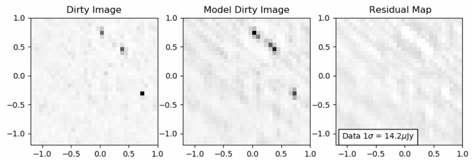
Figure 4. (Left): B1422+231 dirty image based on the calibrated ALMA Band 6 visibility data. (Middle): model dirty image based on the simulated visibilities for the best-fit SIE ( \tilde{S}_V ) lens model and Sérsic source profile. (Right): residual map with an estimated noise level. The coordinates are in units of arcsecs centered at the phase center in Table 1.
