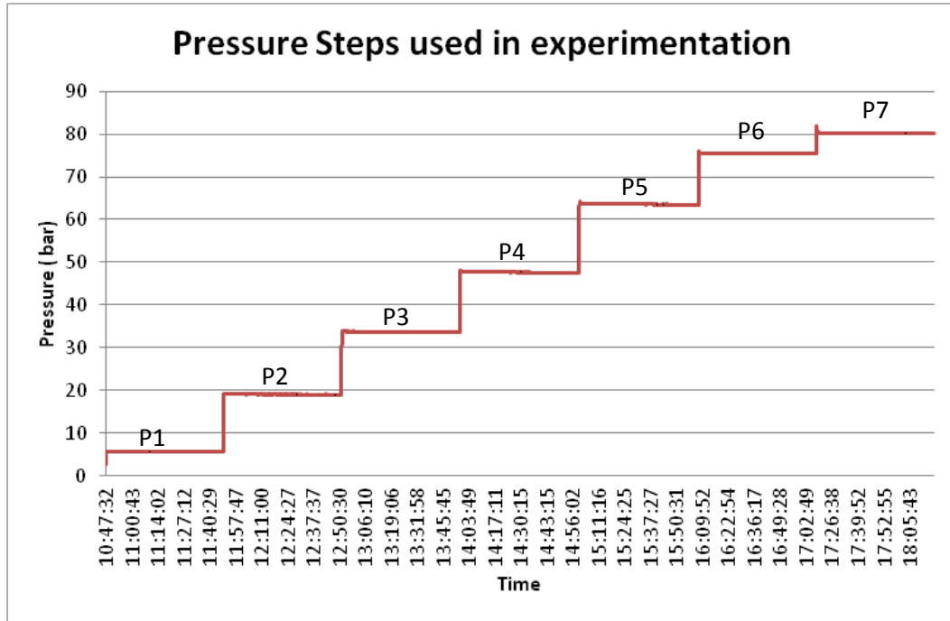
Figure 17: Plot of the pressure steps used in experimentation on the CO 2 adsorptive capacity of coal used in this research
