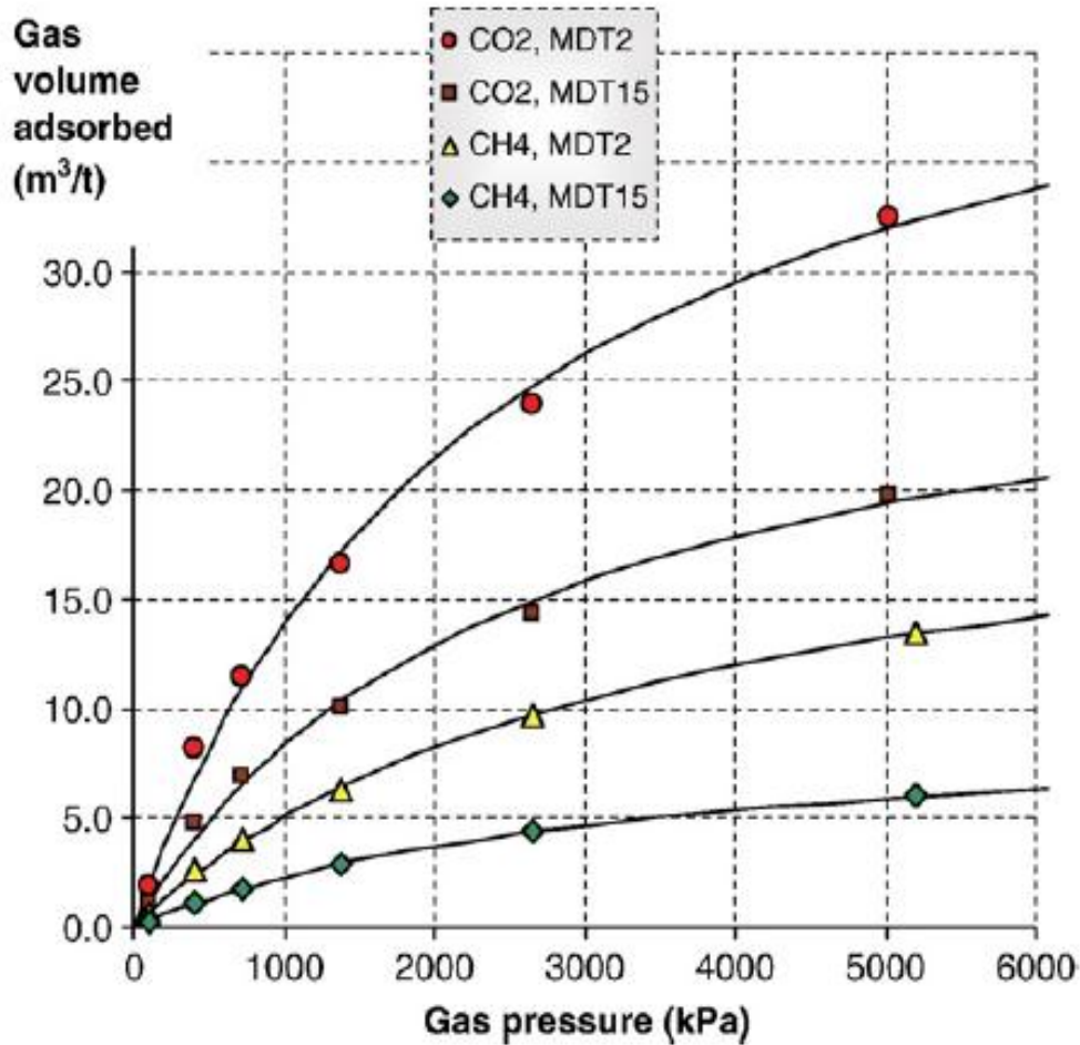
Figure 36: Adsorption curves generated in research on South African coal by Saghaei et al. (2008)
