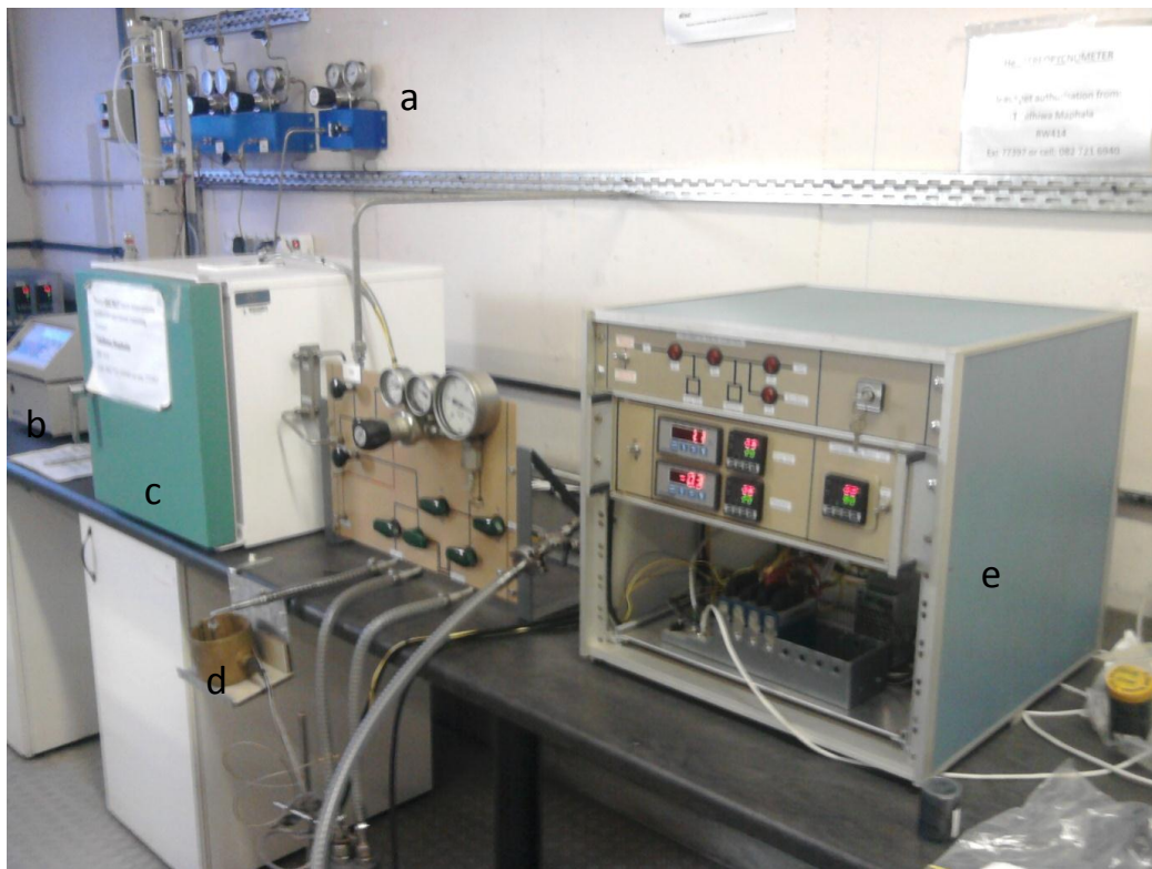
Figure 9: Picture of the laboratory adsorption equipment showing the pump, oven, degassing system, and the data logging system (see text for annotations)
