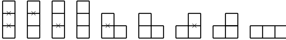
FIGURE 2. Bar graphs of cracked compositions of n = 3 .
