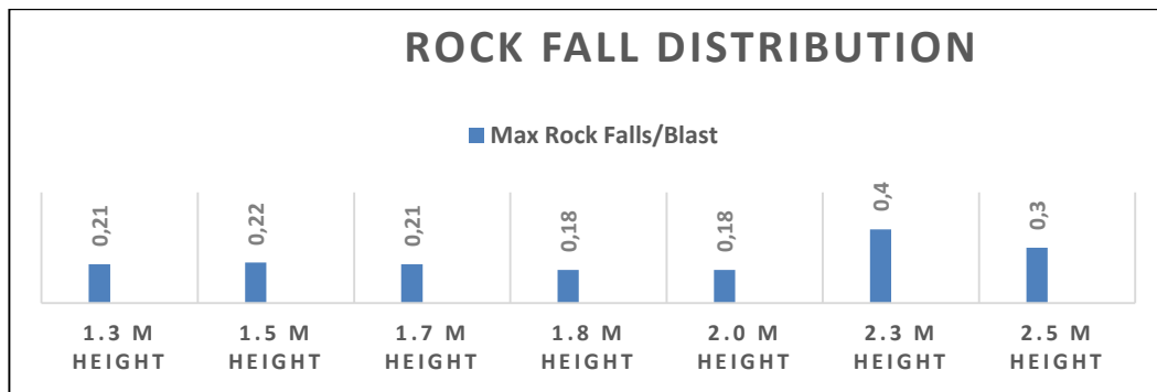
Figure 4.14: Rock fall distributions for the 2.5 m bolt length spaced at 1.5 m X 1.5 m for Scenario 2.
