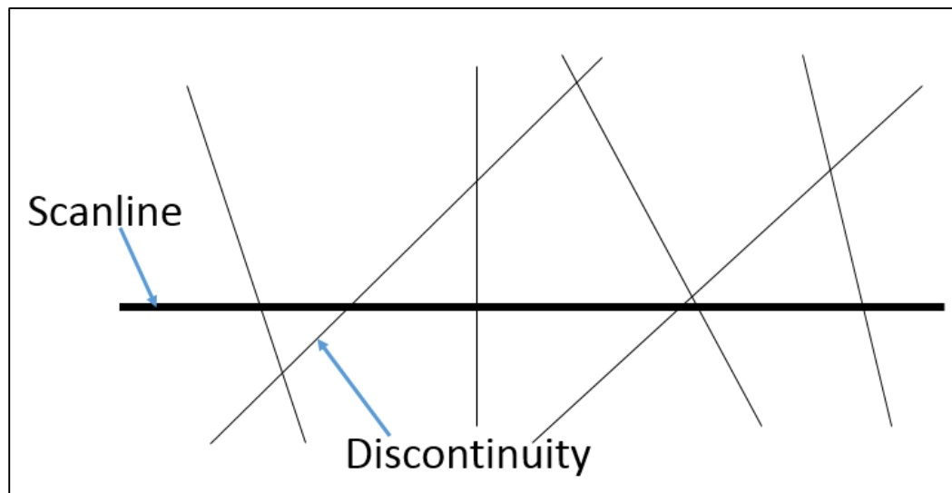
Figure 2.6: Discontinuity mapping in a scanline survey (after Priest and Hudson, 1981).
