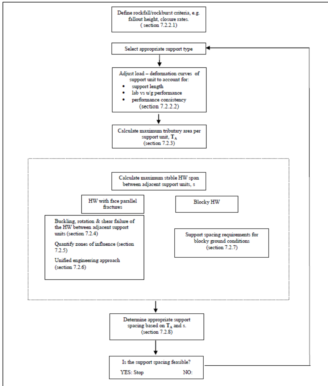
Figure 2.4: Flowchart outlining the principal design steps of support design methodology (after Daehnke et al. , 2001).
