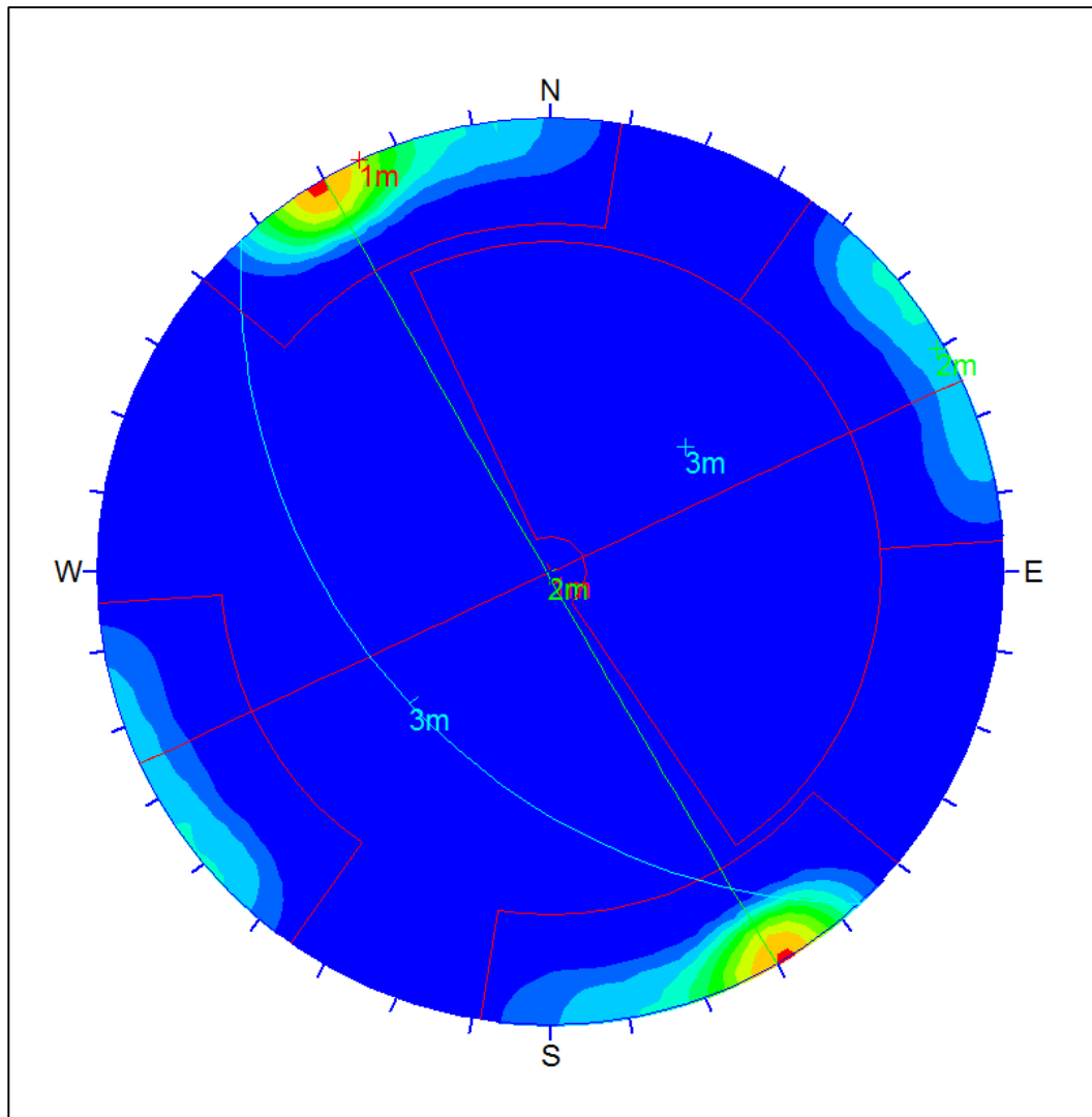
Figure 3.4: Lower hemisphere meridional stereonet projections showing the Dips program contour plot of joint poles and the manually evaluated sets shown by the great circle.
