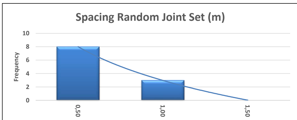
Figure 3.7: Joint spacing data of the random joint set indicating a negative exponential distribution.
