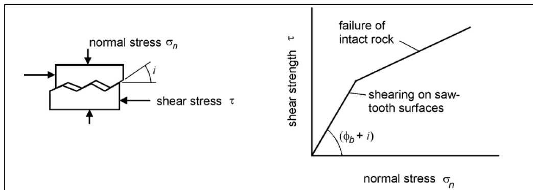
Figure 2.10: The illustration of Patton's experiment on shear strength of saw-tooth specimens (after Patton, 1966).
