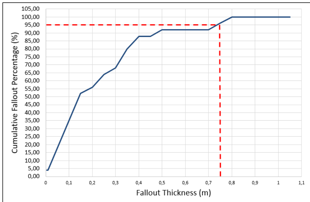
Figure 2.5: Cumulative fall out height graph for Mine A (after Daehnke et al., 1998, 2001).
