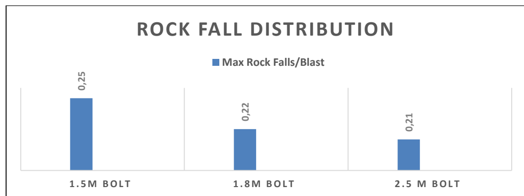
Figure 4.10: Rock fall distributions for the different bolt lengths at 1.5 m X 1.5 m spacing for Scenario 2, 1.7 m Triplet height.
