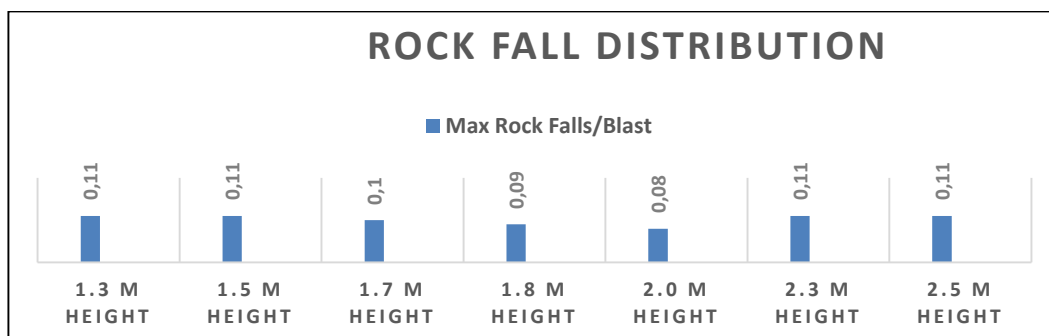
Figure 4.13: Rock fall distributions for the 2.5 m bolt length spaced at 1.5 m X 1.5 m for Scenario 1.
