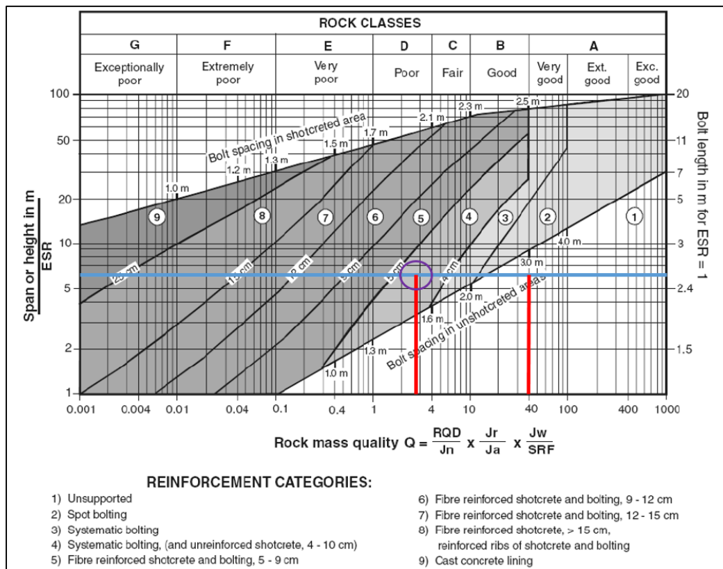
Figure 2.3: Tunnelling support guidelines indicating different support requirements at zones where the red and blue lines coincide (after Grimstad et al., 1993).
