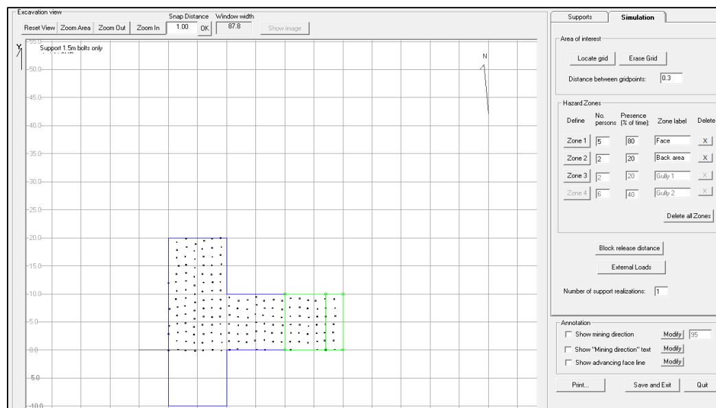
Figure 3.15: JBlock image of the excavation and the delineated hazard zone.
