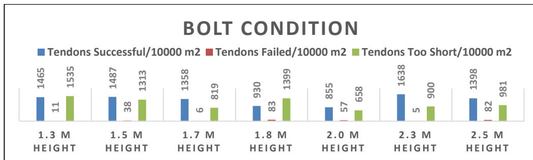
Figure 4.8: Contributing factors to bolt behaviours at various Triplets heights for Scenario 2.
