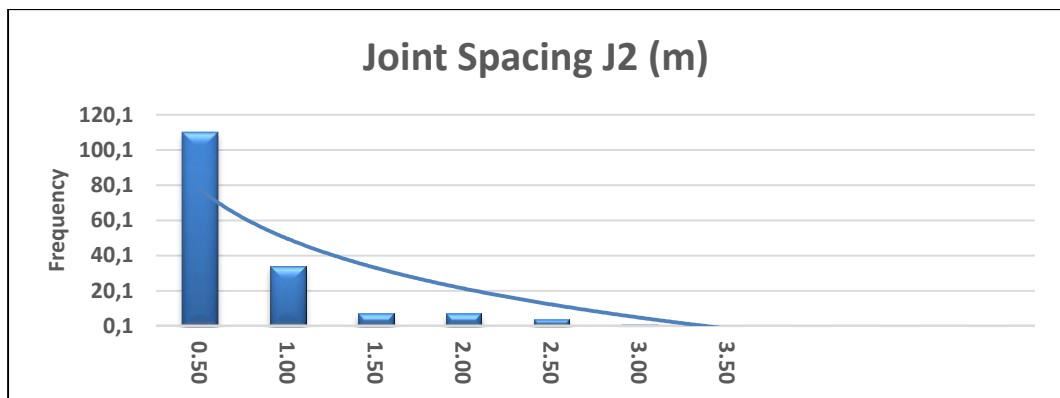
Figure 3.6: Joint spacing data of Joint set 2 indicating a negative exponential distribution.
