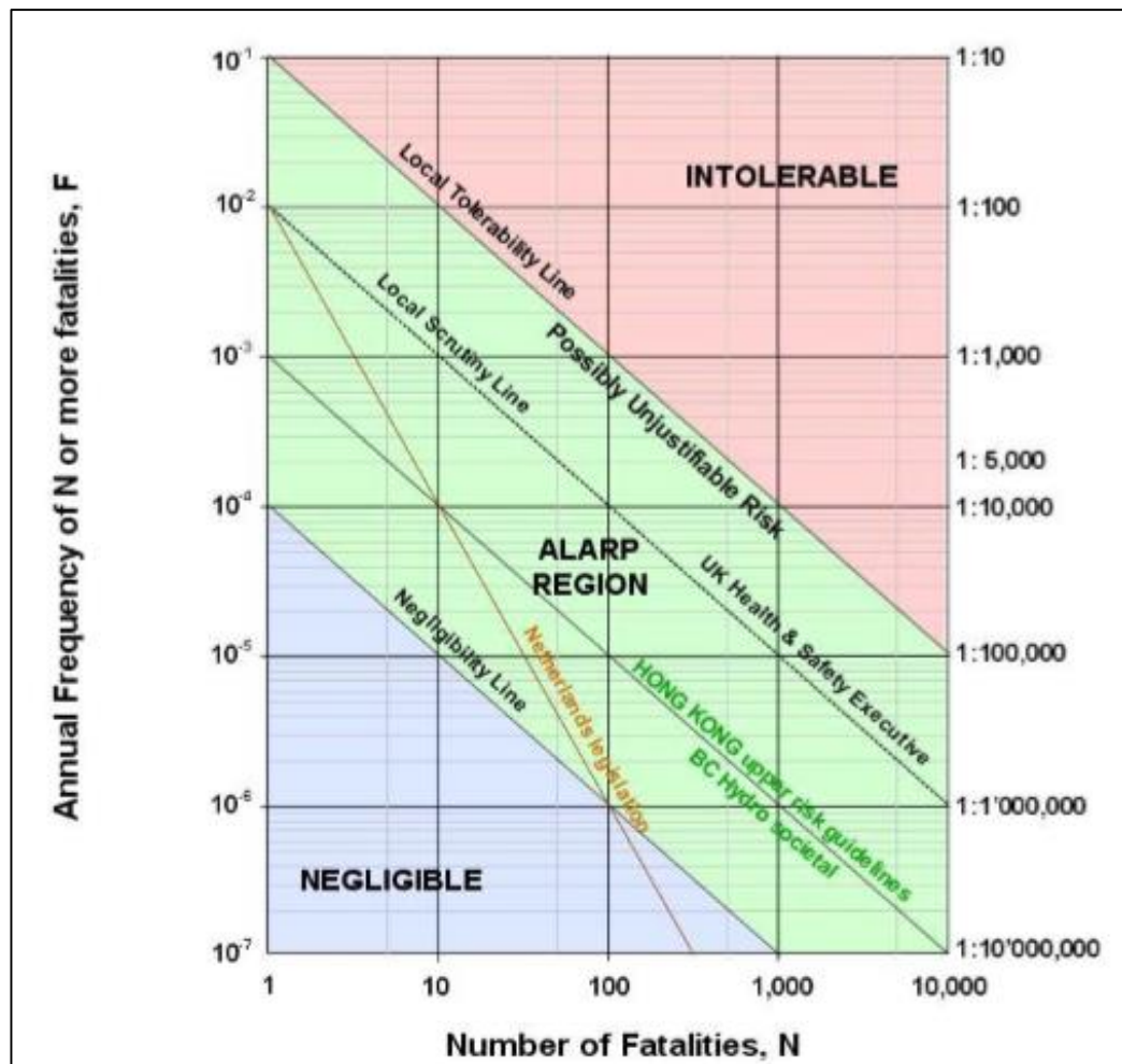
Figure 5.1: F-N graph for bench marking safety impact (Joughin et al., 2012a).
