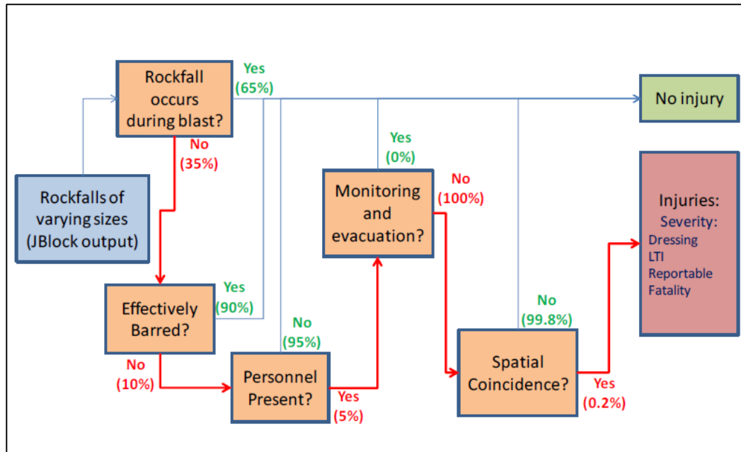
Figure 4.2: Event tree analysis for injuries (after Joughin et al. , 2012a).
