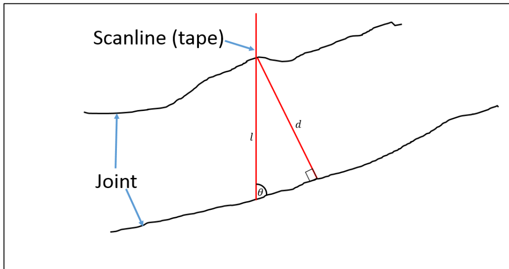
Figure 2.8: The illustration of joint spacing correction (Nezomba, 2012).
