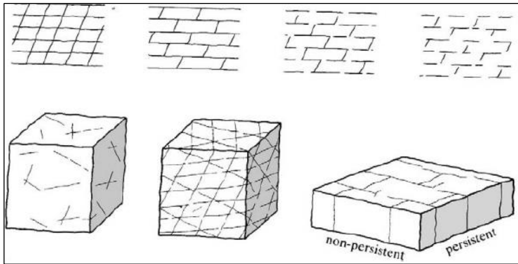
Figure 2.9: The illustration of the definition of persistence of discontinuity (Brady and Brown, 1993).
