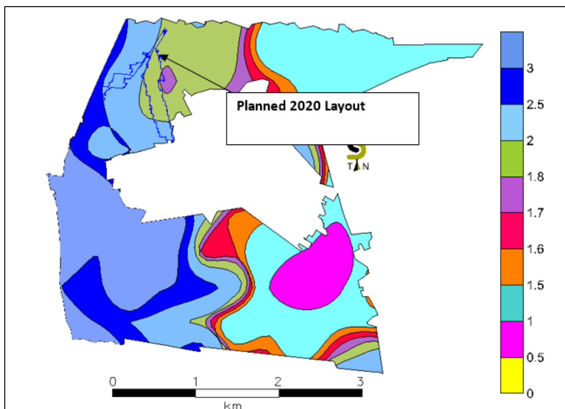
Figure 3.11: UG2 to Triplets layer isopachs (Kekana, 2018).
