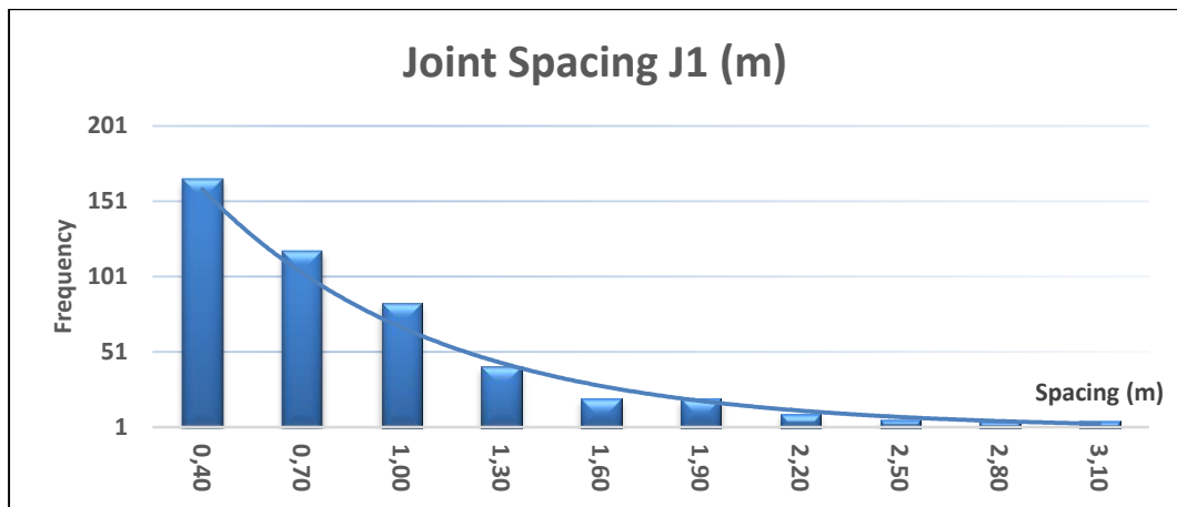
Figure 3.5: Joint spacing data of Joint set 1 indicating a negative exponential distribution.
