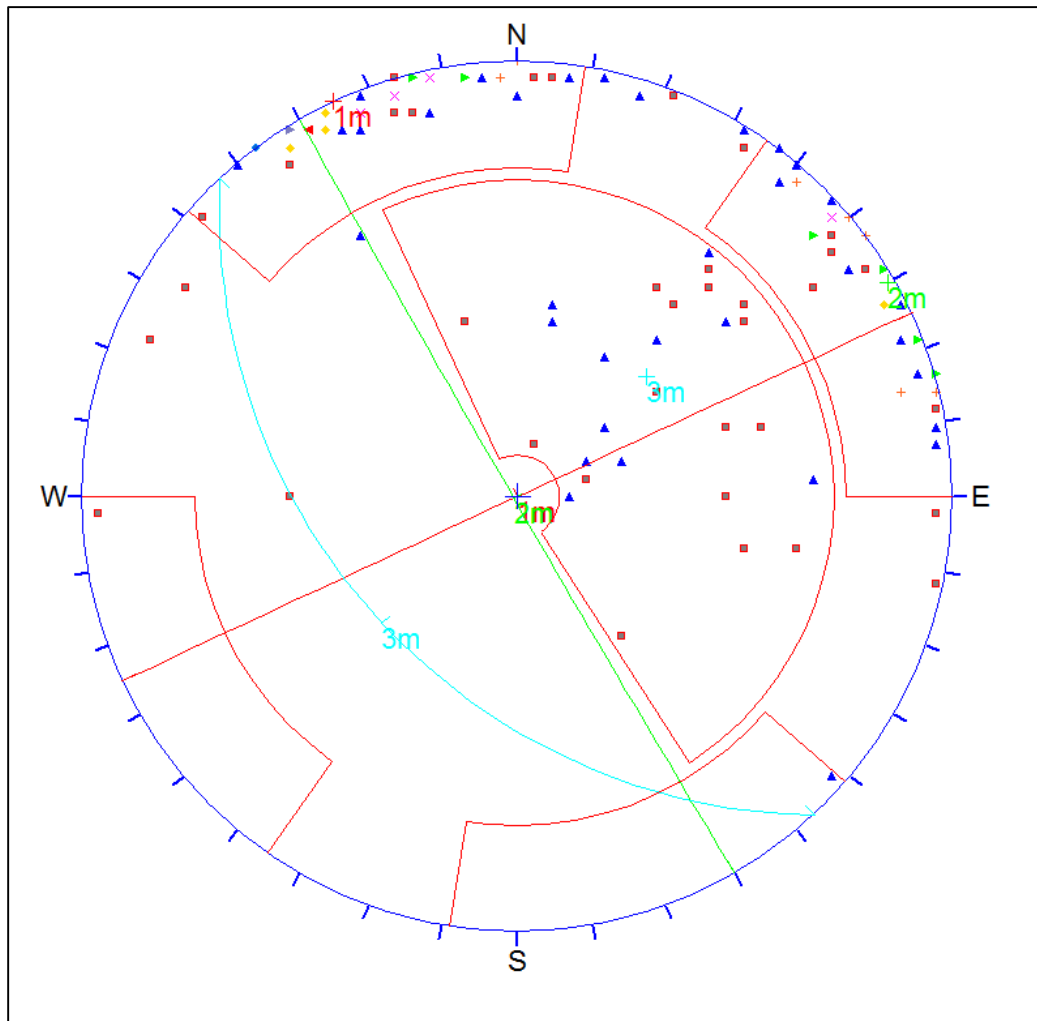
Figure 3.3: Lower hemisphere meridional stereonet projections of the mapped joint poles and the great circles of the manually evaluated sets using the Dips program.
