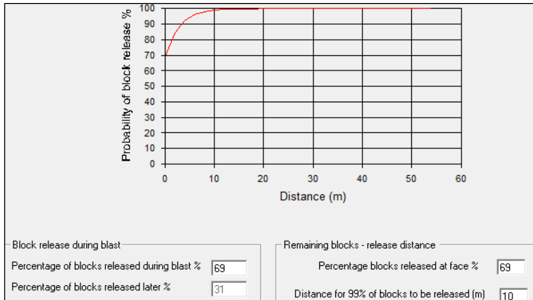
Figure 3.16: JBlock image of the keyblock release distance and probabilities.
