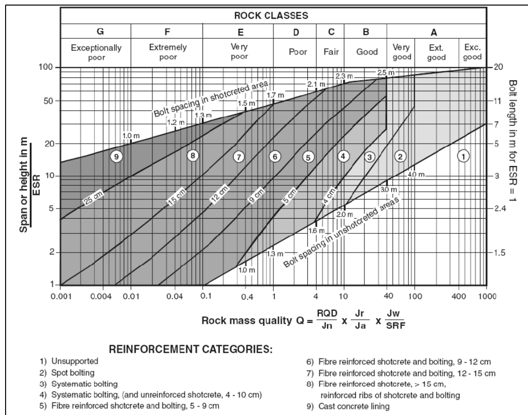
Figure 2.1: Tunnelling support guidelines (after Grimstad et al. , 1993).
