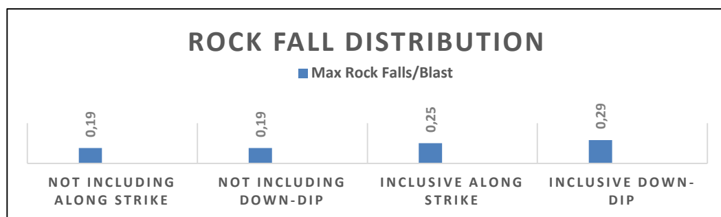
Figure 4.3: Rock fall distributions for both Scenarios.
