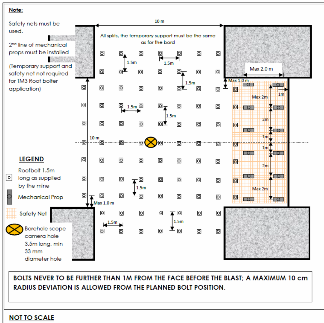
Figure 1.6: The support standard for the UG2 reef, (Sibanda, 2018).
