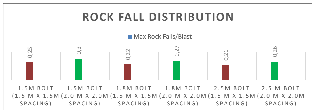
Figure 4.16: Rock fall distributions for three bolt lengths at different spacings for Scenario 2, (1.7 m Triplet height).
