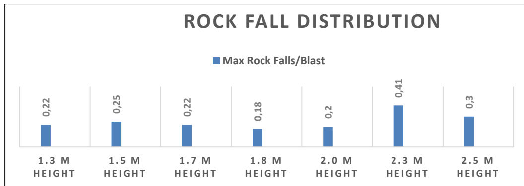
Figure 4.7: Rock fall distributions for the different Triplets heights for Scenario 2.
