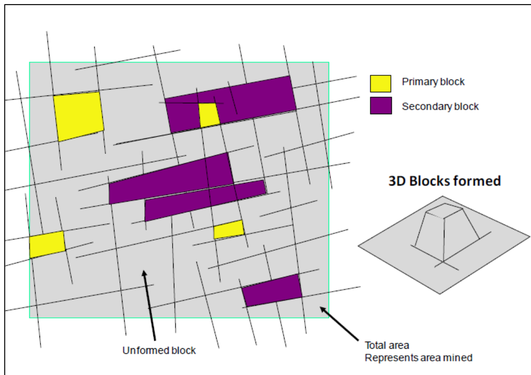
Figure 4.1: A plan view of a mining area indicating the trace of joints in the hangingwall with primary and secondary block formation (after Joughin et al., 2012b).
