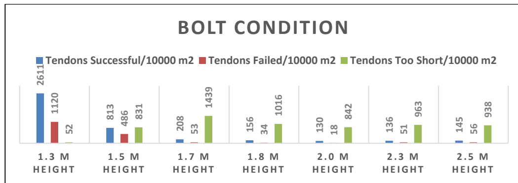
Figure 4.6: Contributing factors to bolt behaviours at various Triplets heights for Scenario 1.
