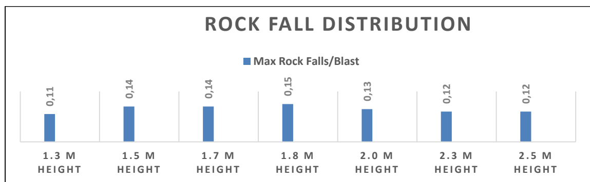
Figure 4.11: Rock fall distributions for the 1.8 m bolt length spaced at 1.5 m X 1.5 m for Scenario 1.
