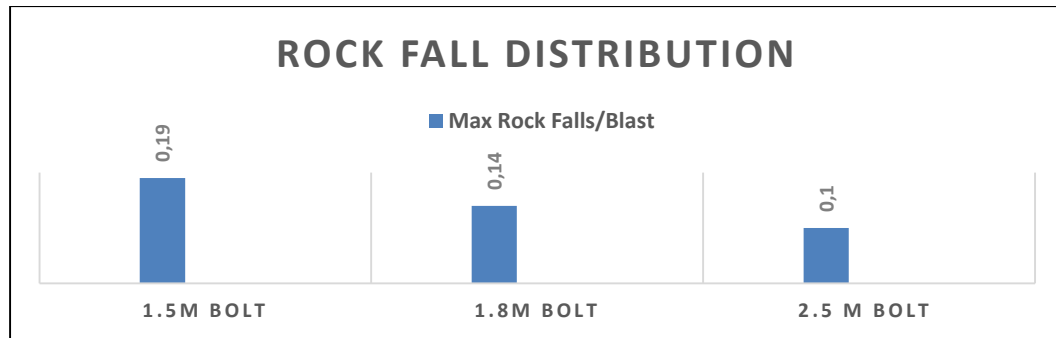
Figure 4.9: Rock fall distributions for various bolt lengths (1.5 m X 1.5 m spacing for Scenario 1, Triplets at 1.7 m).
