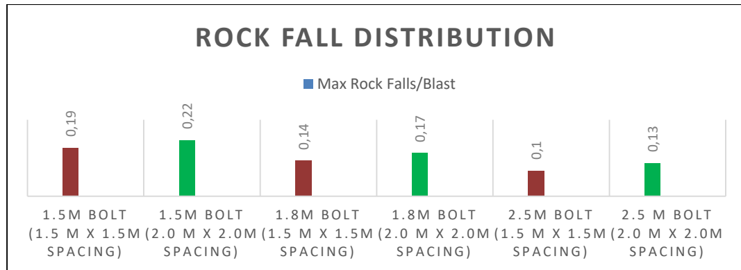
Figure 4.15: Rock fall distributions for three bolt lengths at different spacings for Scenario 1, (1.7 m Triplet height).
