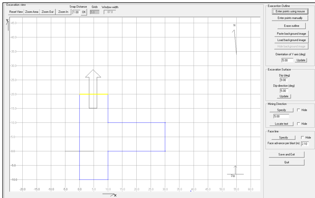
Figure 3.13: JBlock image of the excavation file for a panel along dip.
