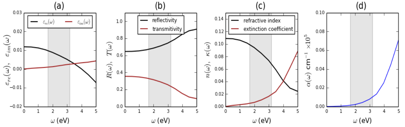
Figure 6.49: GW TiS 3 calculated frequency-dependent optical spectra (a) real \epsilon_{re}(\omega) and the imaginary \epsilon_{im}(\omega) parts of the dielectric function, (b) reflectivity R(\omega) and transmittivity T(\omega) , (c) refraction n(\omega) and extinction coefficient \kappa(\omega) and (d) absorption coefficient \alpha(\omega) . The visible range is shaded.
