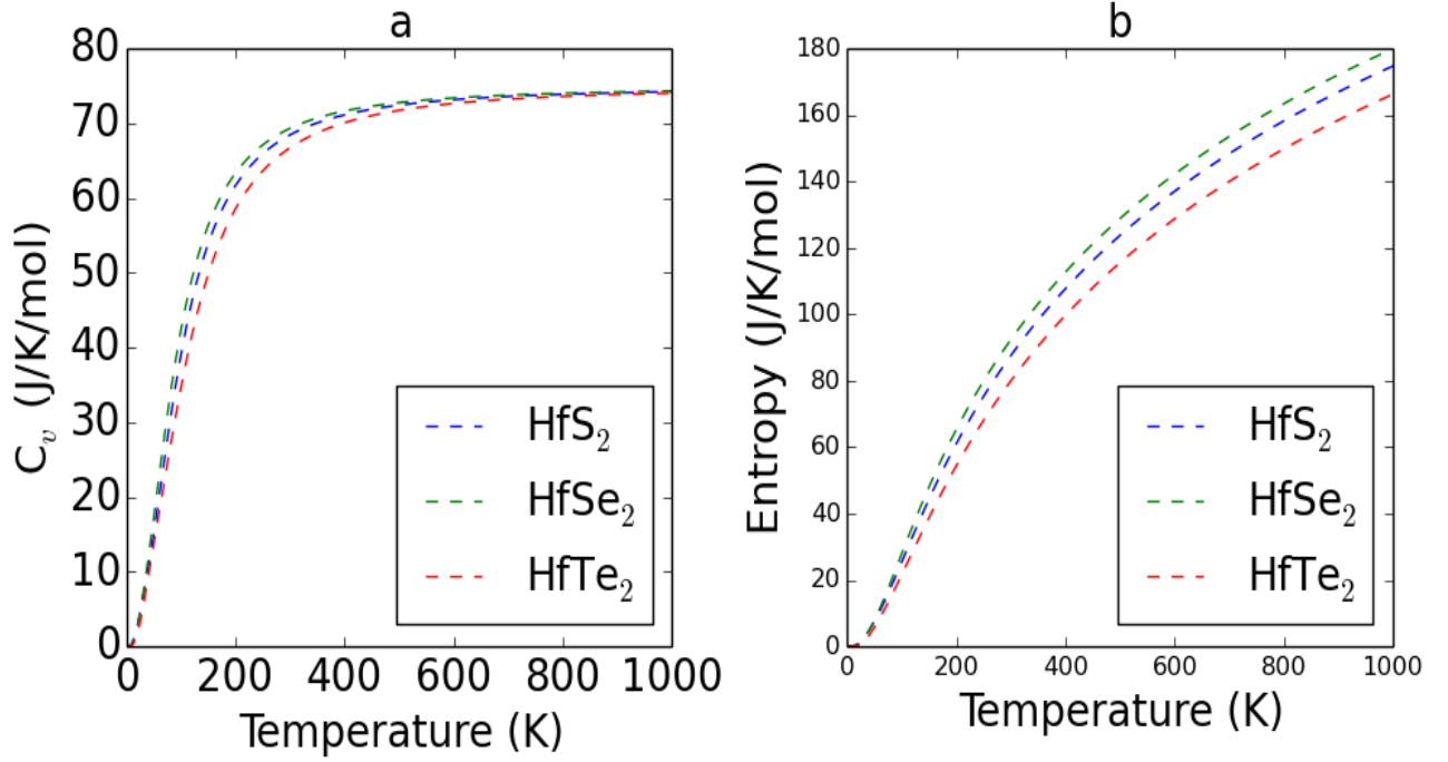
Figure 6.17: vdW-TS calculated specific heat capacity at constant volume and entropy for HfX 2 (X= S, Se and Te) structures.
