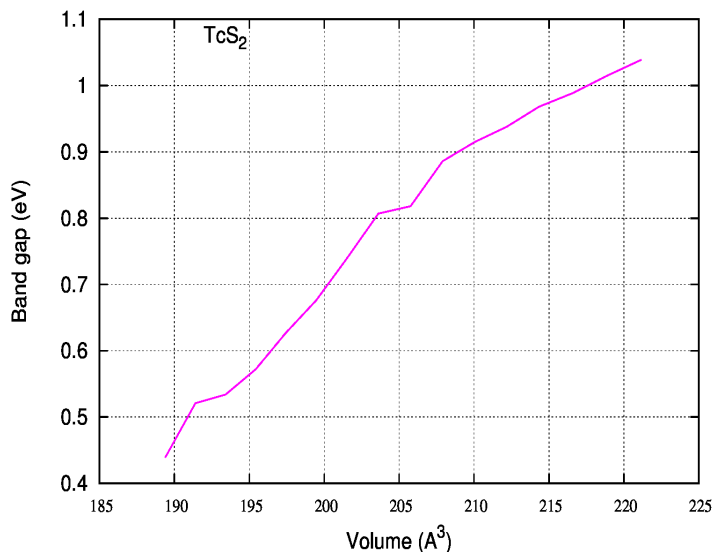
Figure 6.10: Band gap volume relationship in \text{TcX}_2 ( X = \text{S}, \text{Se} and \text{Te} ) calculated from vdW-D2 relaxed structure.
