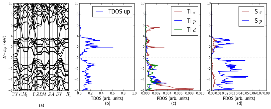
Figure 6.46: vdW-TS \text{TiS}_3 calculated electronic structure (a) band structure along high symmetry K-points, (b) spin projected TDOS, (c) PDOS of Ti(s,p,d) and (d) PDOS of S(s,p).
