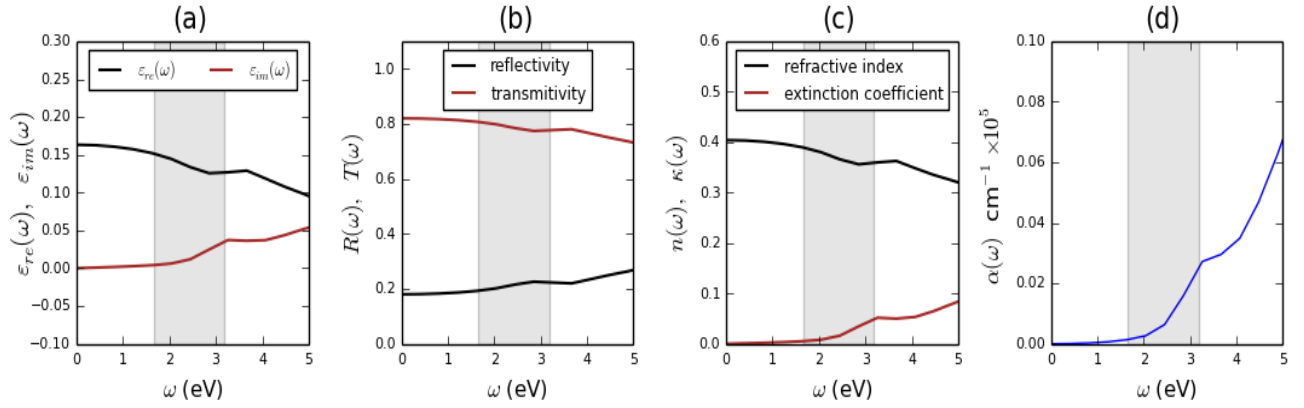
Figure 6.41: GW ZrS 3 calculated frequency-dependent optical spectra (a) real \epsilon_{re}(\omega) and the imaginary \epsilon_{im}(\omega) parts of the dielectric function, (b) reflectivity R(\omega) and transmittivity T(\omega) , (c) refraction \eta(\omega) and extinction coefficient \kappa(\omega) and (d) absorption coefficient \alpha(\omega) . The visible range is shaded.
