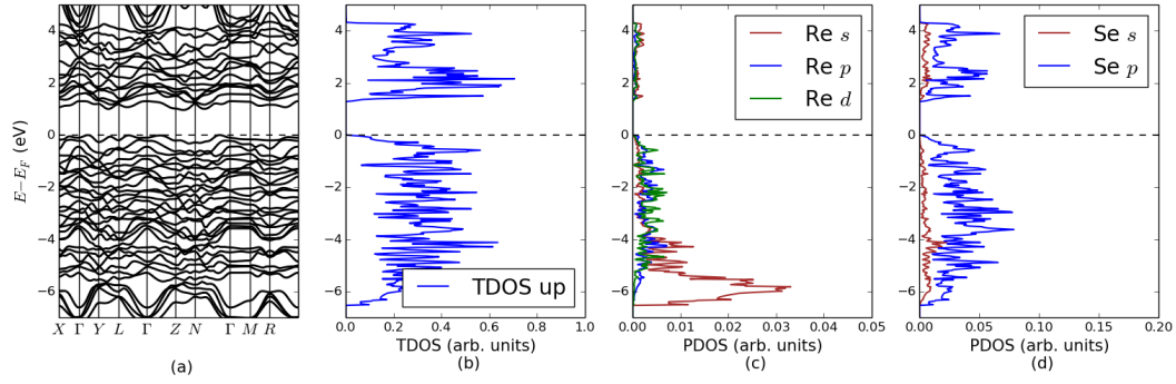
Figure 6.52: MBJ calculated ReSe 2 band structure (a) band structure along high symmetry K-points, (b) spin projected total density of states (TDOS), (c) partial density of states (PDOS) of Re(s,p,d) (d) PDOS of Se (s,p).
