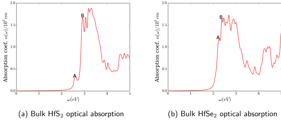
Figure 6.18: \text{HfX}_2 (X= S, Se) BSE calculated optical absorptions.
