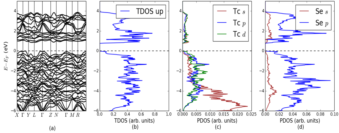
Figure 6.8: Calculated MBJ TcSe 2 calculated electronic structure (a) band structure along high symmetry K-points, (b) spin projected TDOS, (c) PDOS of Tc(s,p,d) and (d) PDOS of Se(s,p).
