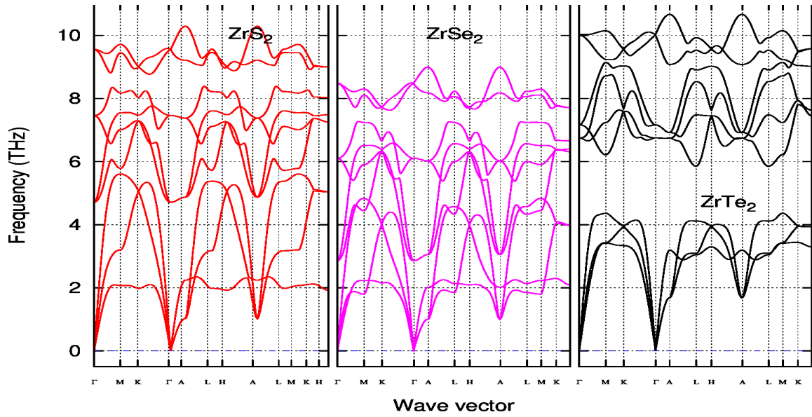
Figure 6.31: \text{ZrX}_2 phonon dispersion relation graph calculated using vdW-TS.
