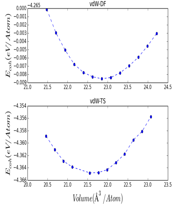
(b) \text{TiSe}_3 cohesive energy-volume graph calculated using (a) vdW-TS and (b) vdW-DF
