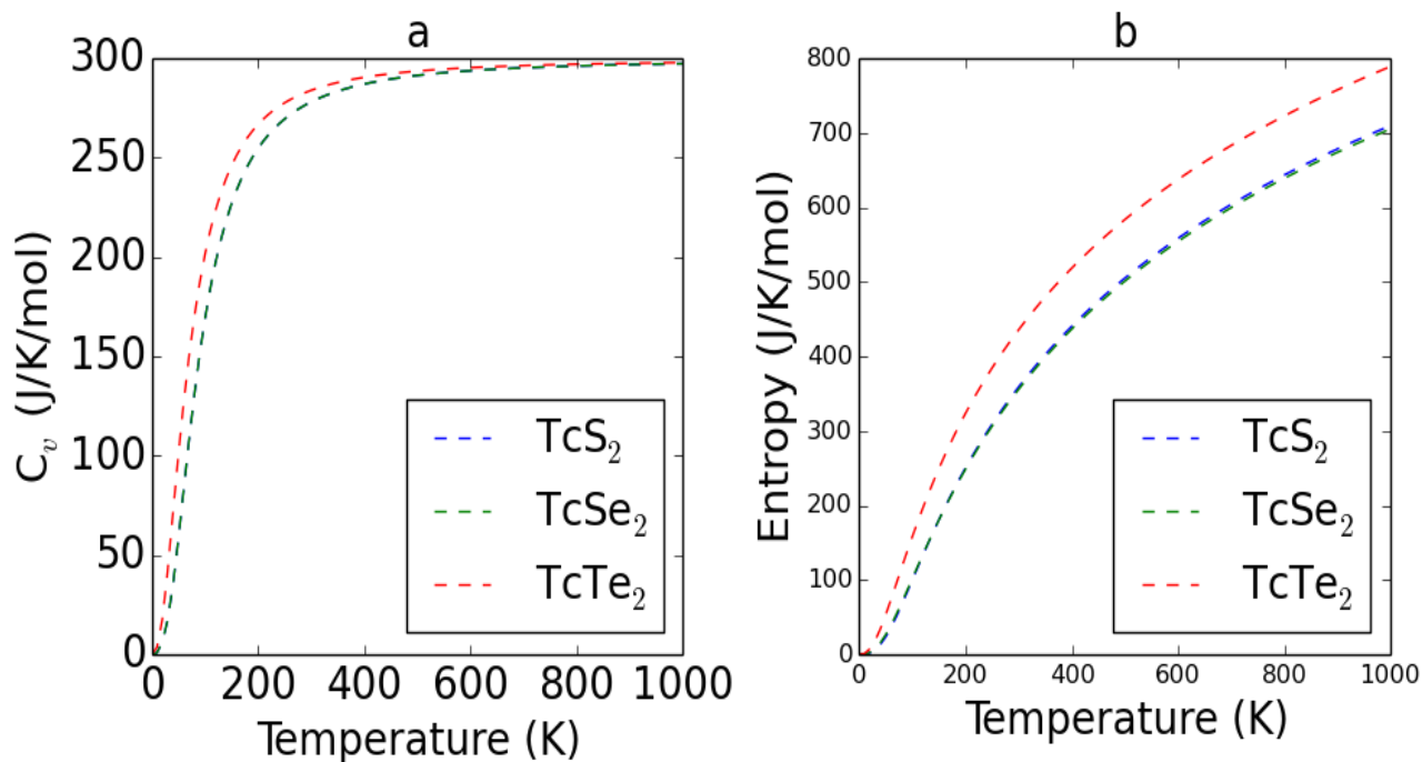
Figure 6.6: vdW-D2 calculated specific heat capacity at constant volume and entropy for the TcX 2 (X = S, Se and Te) structures.
