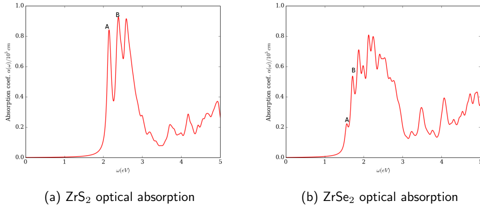
Figure 6.33: Optical absorptions for Monolayer \text{ZrX}_2 ( \text{X} = \text{S}, \text{Se} ) calculated at the BSE level.
