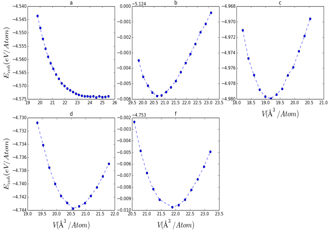
Figure 6.3: TcSe 2 cohesive energy-volume graph calculated using (a) PBE, (b) PBEsol, (c) vdW-TS, (d) DFT-D2 and (f) vdW-DF.
