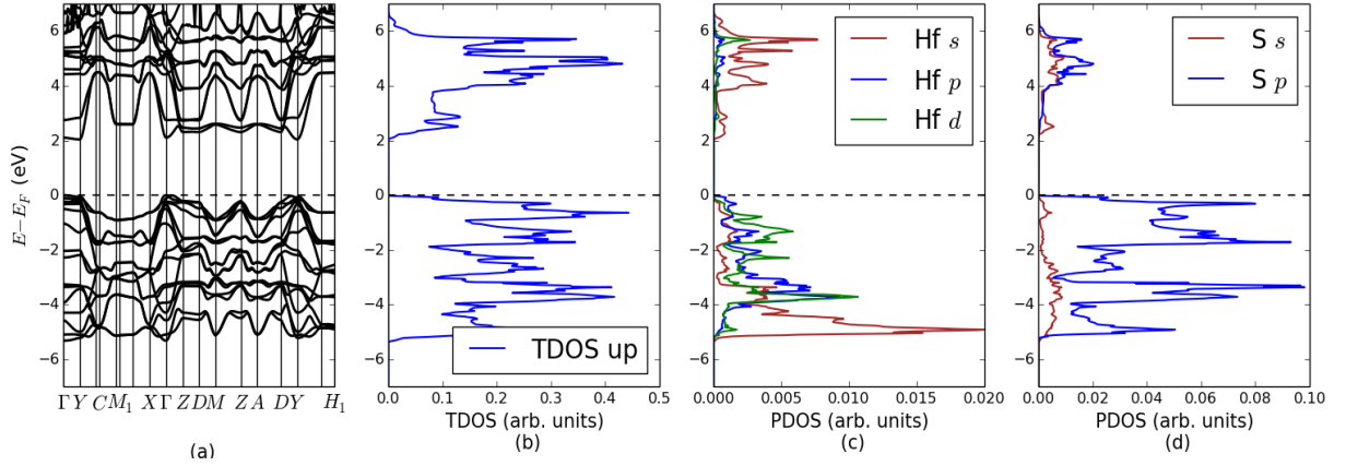
Figure 6.25: Calculated electronic properties of \text{HfS}_3 using MBJ functional band structure (a) band structure along high symmetry K-points, (b) spin projected TDOS, (c) PDOS of Hf(s,p,d) (d) PDOS of S (s,p).
