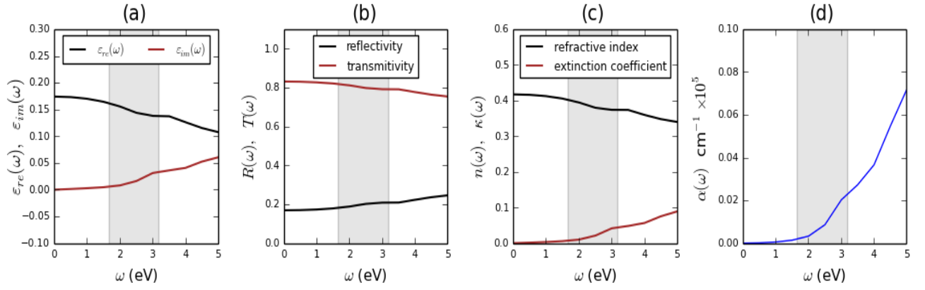
Figure 6.28: GW HfS 3 calculated frequency-dependent optical spectra (a) real \epsilon_{re}(\omega) and the imaginary \epsilon_{im}(\omega) parts of the dielectric function, (b) reflectivity R(\omega) and Transmittivity T(\omega) , (c) Refraction \eta(\omega) and extinction coefficient \kappa(\omega) and (d) absorption coefficient \alpha(\omega) . The visible range are shaded.
