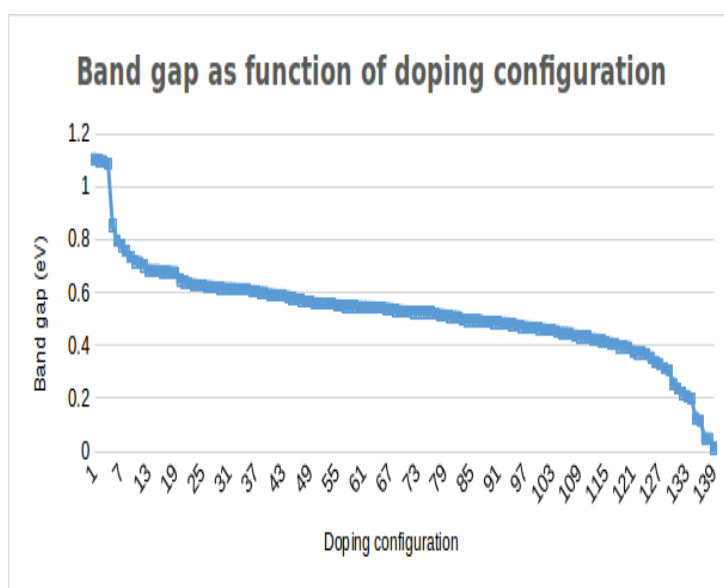
Figure 6.15: Band gap as a function of doping configuration for \text{TcS}_2 calculated with MBJ functional.
