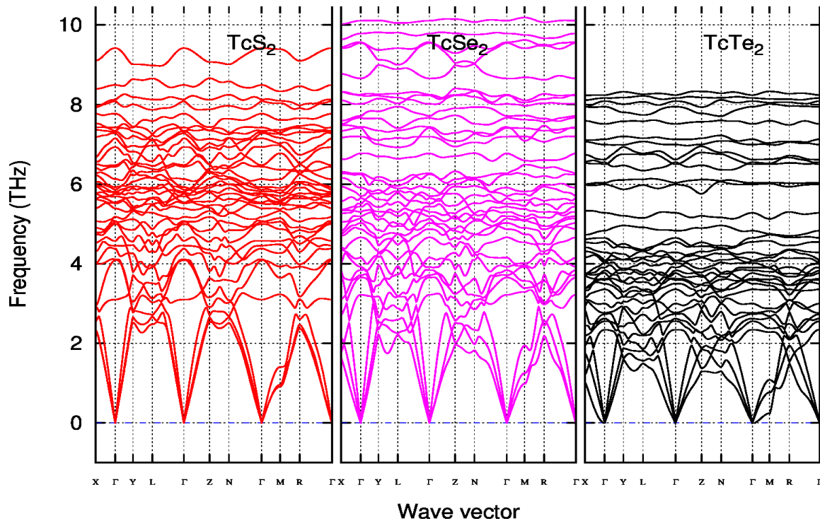
Figure 6.5: \text{TcX}_2 ( \text{X} = \text{S}, \text{Se} and \text{Te} ) phonon dispersion relation graph calculated using vdW-D2.
