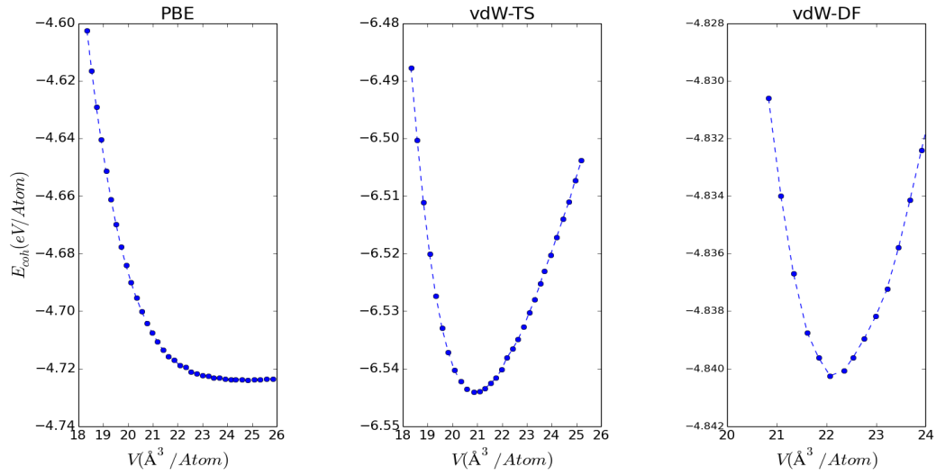
Figure 6.50: ReSe 2 cohesive energy-volume graph calculated using (a) PBE, (b) vdW-TS and (c) vdW-DF.
