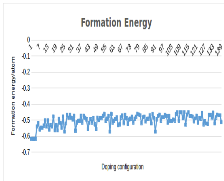
Figure 6.14: Formation energy per atom as a function of doping configuration.
