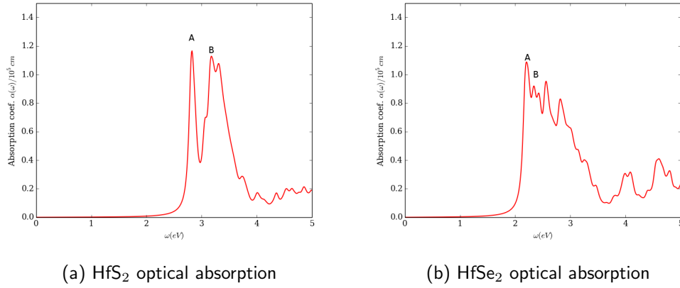
Figure 6.20: Monolayer \text{HfX}_2 ( X = \text{S}, \text{Se} ) BSE calculated optical absorptions.
