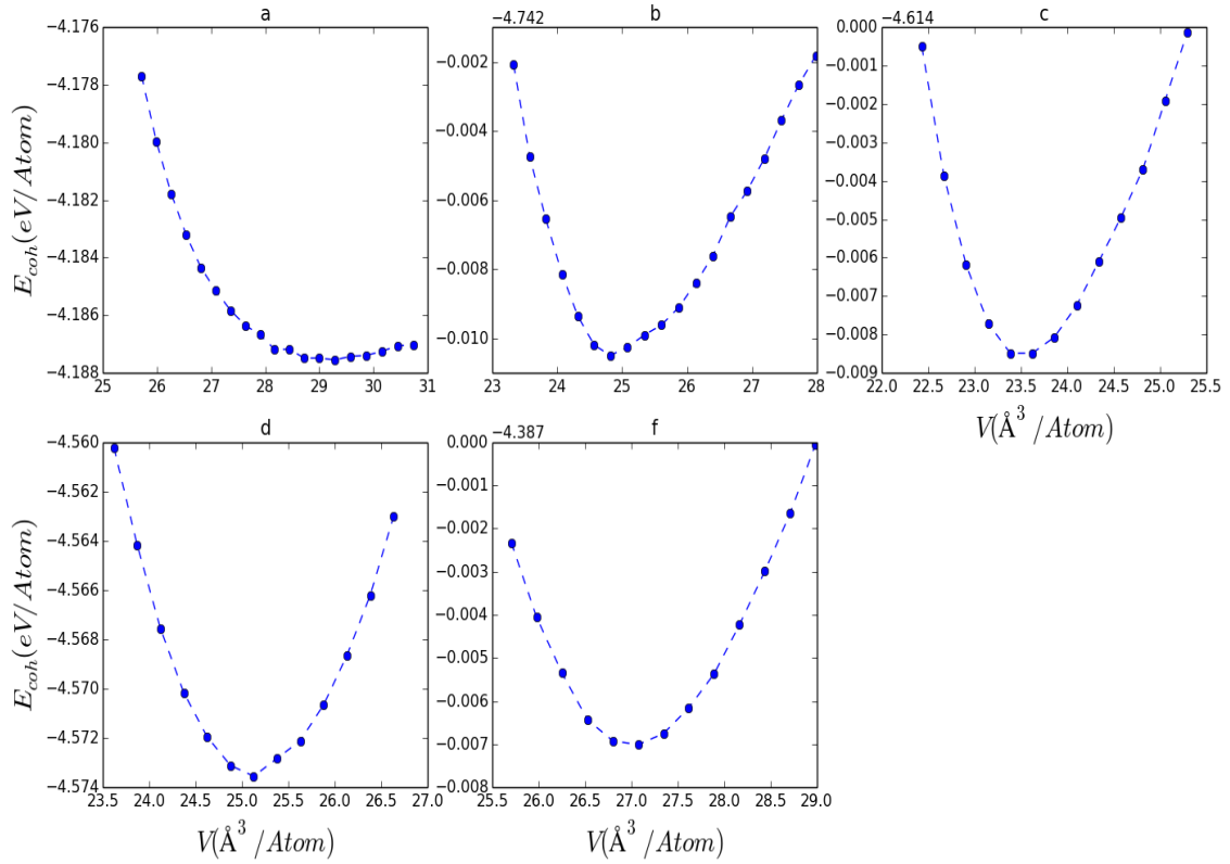
Figure 6.4: TcTe 2 cohesive energy-volume graph calculated using (a) PBE, (b) PBEsol, (c) vdW-TS, (d) DFT-D2 and (f) vdW-DF.
