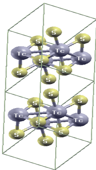
Figure 6.1: \text{TcS}_2 unit cell doubled in the Z-direction to show the layered structure.
