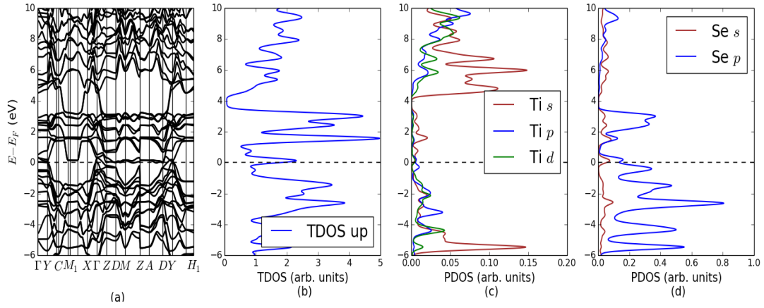
Figure 6.47: vdW-TS \text{TiSe}_3 calculated electronic structure (a) band structure along high symmetry K-points, (b) spin projected TDOS, (c) PDOS of Ti(s,p,d) and (d) PDOS of Se(s,p).
