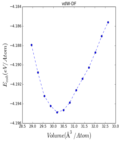
(c) \text{HfTe}_3 cohesive energy-volume graph calculated using (a) vdW-TS and (b) vdW-DF
