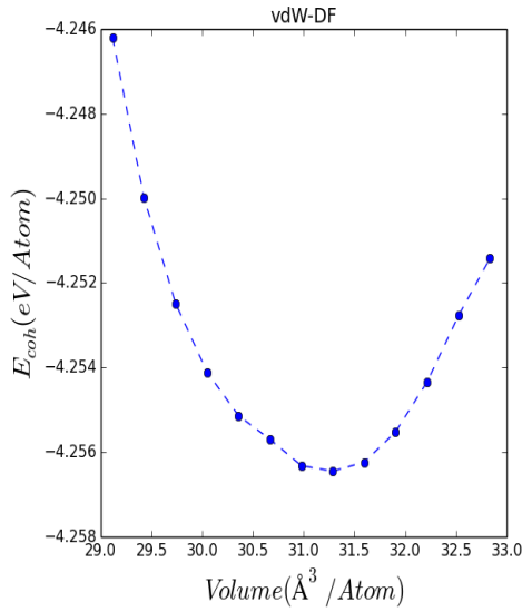
(c) \text{ZrTe}_3 cohesive energy-volume graph calculated using (a) vdW-TS and (b) vdW-DF
