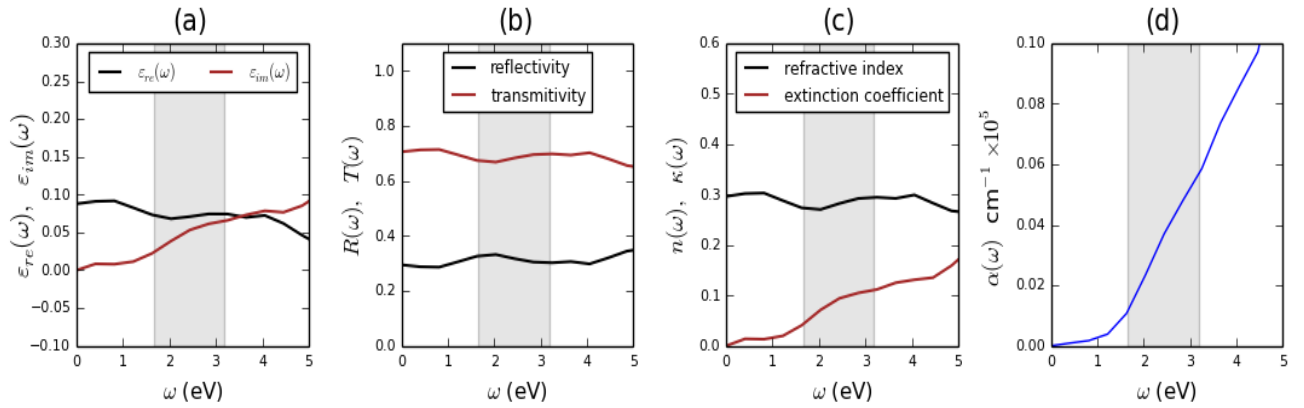
Figure 6.42: GW ZrSe 3 calculated frequency-dependent optical spectra (a) real \epsilon_{re}(\omega) and the imaginary \epsilon_{im}(\omega) parts of the dielectric function, (b) reflectivity R(\omega) and transmittivity T(\omega) , (c) refraction \eta(\omega) and extinction coefficient \kappa(\omega) and (d) absorption coefficient \alpha(\omega) . The visible range is shaded.
