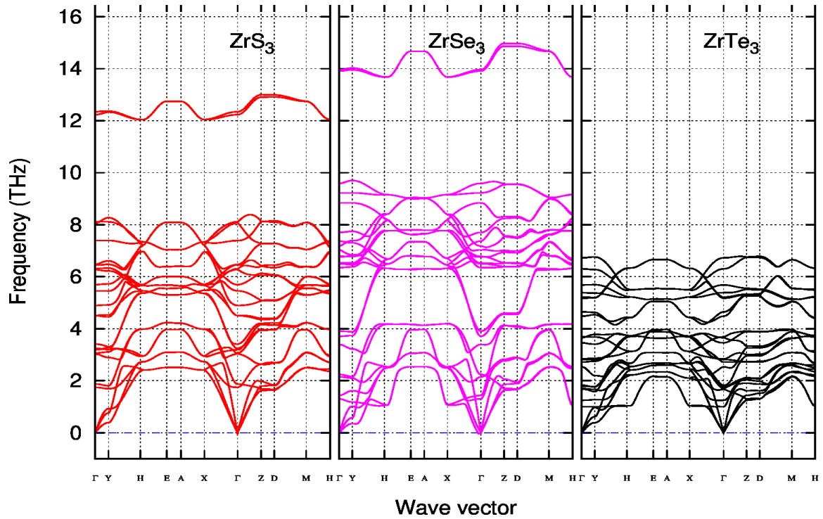
Figure 6.36: \text{ZrX}_3 phonon dispersion relation graph calculated using vdW-TS.
