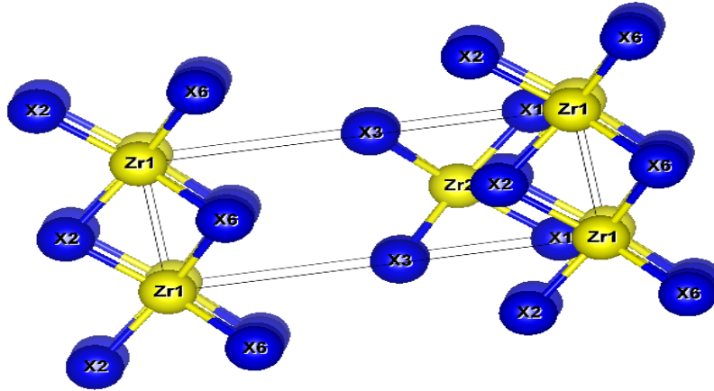
Figure 6.34: \text{ZrX}_3 structure.
