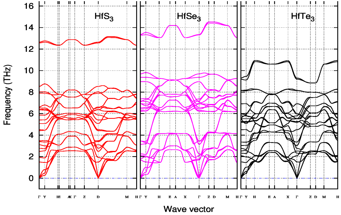
Figure 6.23: \text{HfX}_3 phonon dispersion relation graph calculated using vdW-TS.
