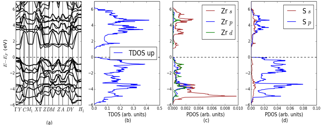
Figure 6.38: \text{ZrS}_3 vdW-TS calculated band structure (a) band structure along high symmetry K-points, (b) spin projected total density of states (TDOS), (c) partial density of states (PDOS) of Zr(s,p,d) (d) PDOS of S (s,p).
