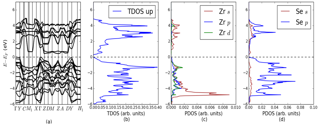
Figure 6.39: MBJ \text{ZrSe}_3 calculated band structure (a) band structure along high symmetry K-points, (b) spin projected TDOS, (c) PDOS of Zr(s,p,d) (d) PDOS of Se (s,p).
