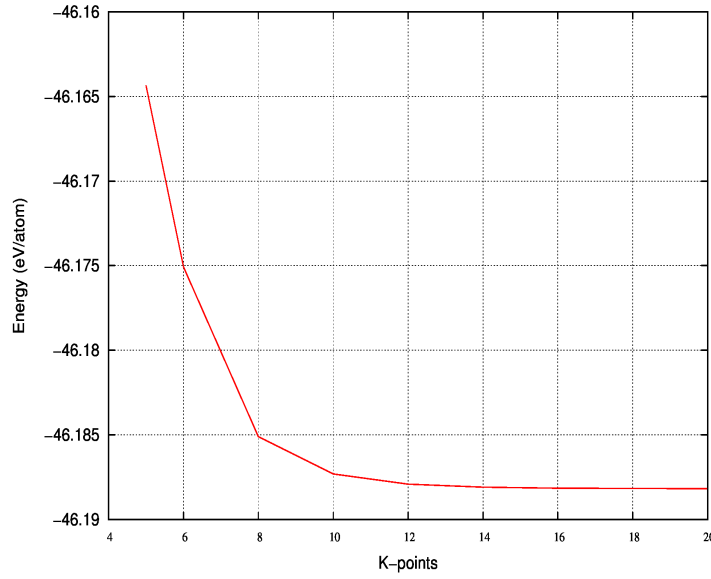
Figure 5.1: K point convergence.
