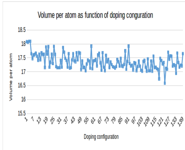
Figure 6.13: Structural volume per atom as a function of doping configuration.
