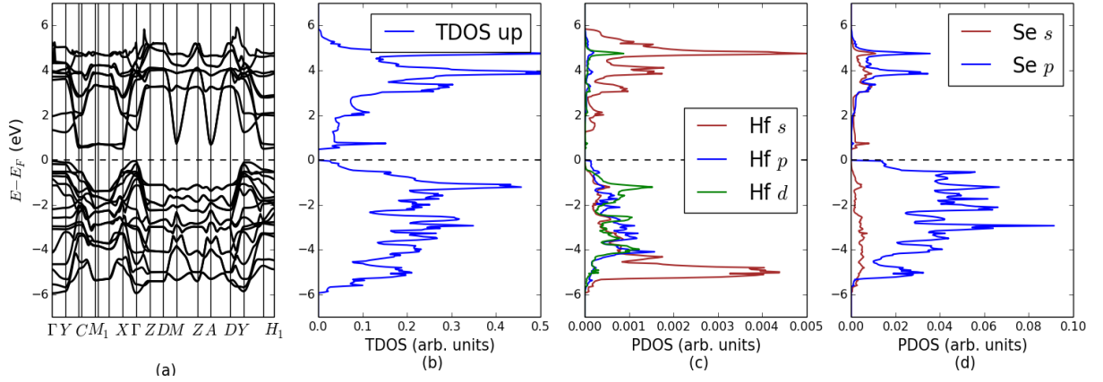
Figure 6.26: MBJ HfSe 3 calculated band structure (a) band structure along high symmetry K-points, (b) spin projected TDOS, (c) PDOS of Hf(s,p,d) (d) PDOS of Se (s,p).
