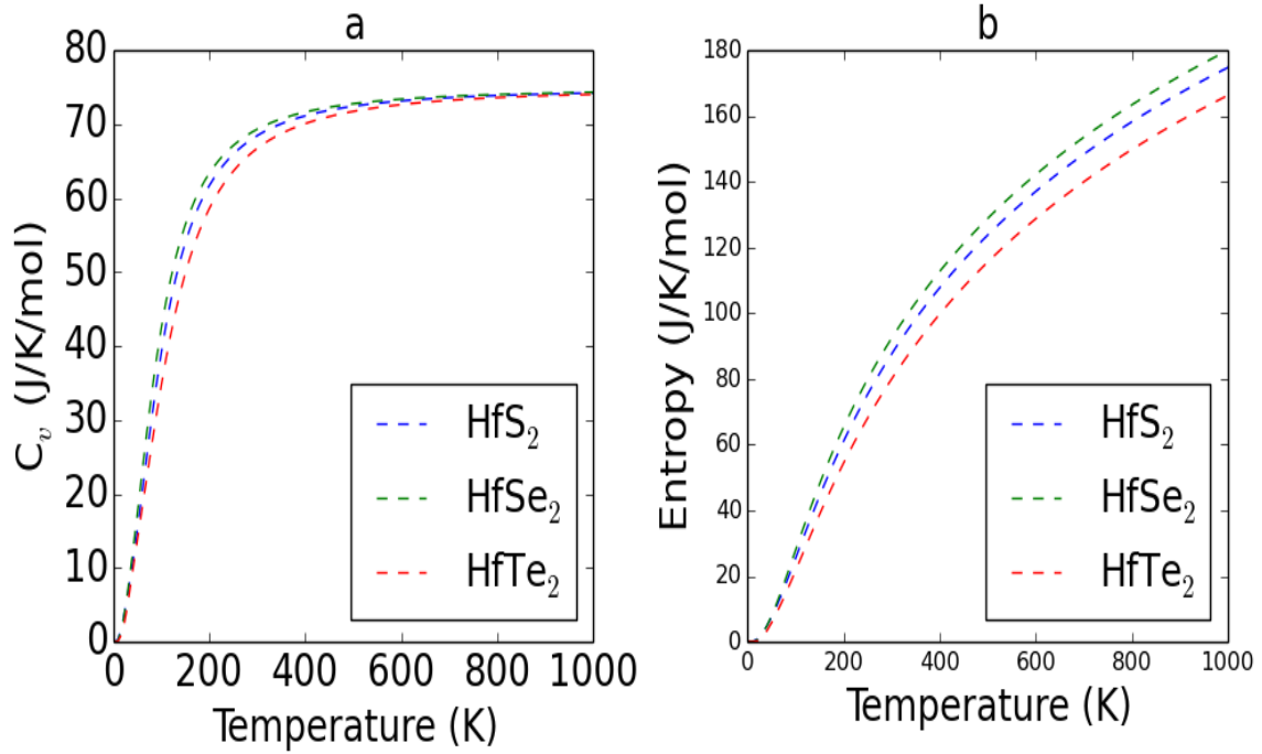
Figure 6.16: \text{HfX}_2 phonon dispersion relation graph calculated using vdW-TS.
