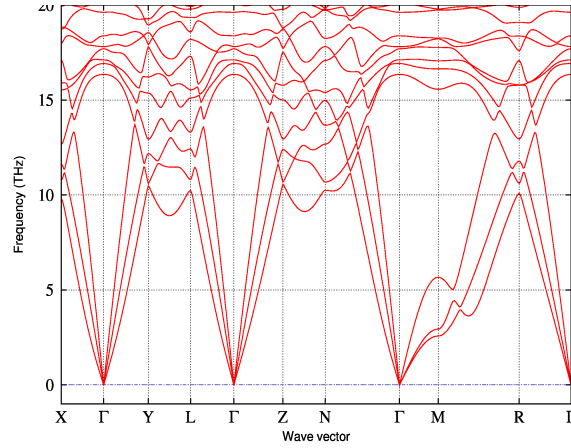
Figure 6.51: Phonon dispersion of ReSe 2 calculated using the vdW-TS relaxed structure.
