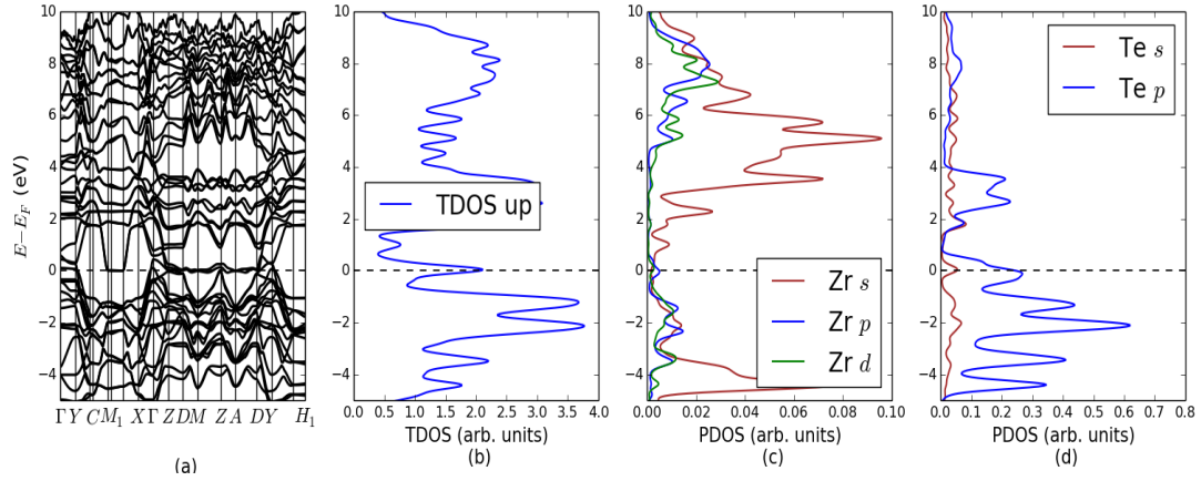
Figure 6.40: vdW-DF \text{ZrTe}_3 calculated band structure (a) band structure along high symmetry K-points, (b) spin projected TDOS, (c) PDOS of Zr(s,p,d) (d) PDOS of Te (s,p).
