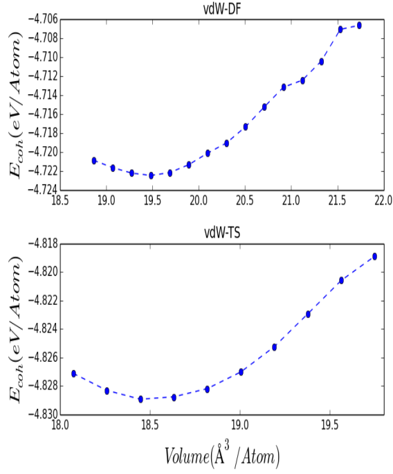
(a) \text{TiS}_3 cohesive energy-volume graph calculated using (a) vdW-TS and (b) vdW-DF
