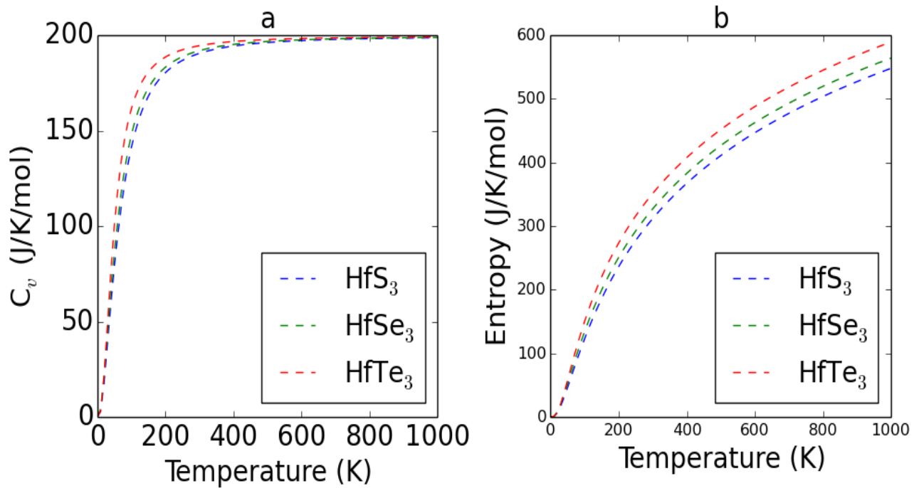
Figure 6.24: vdW-TS calculated specific heat capacity at constant volume and entropy for HfX 3 (X= S, Se and Te) structures.
