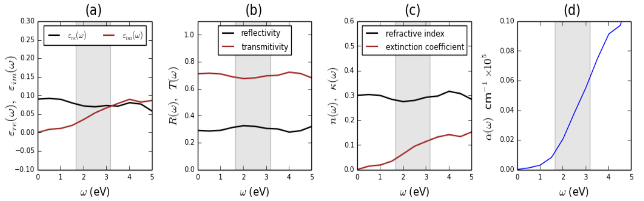
Figure 6.29: GW HfSe 3 calculated frequency-dependent optical spectra (a) real \epsilon_{re}(\omega) and the imaginary \epsilon_{im}(\omega) parts of the dielectric function, (b) reflectivity R(\omega) and transmittivity T(\omega) , (c) refraction \eta(\omega) and extinction coefficient \kappa(\omega) and (d) absorption coefficient \alpha(\omega) . The visible range is shaded.
