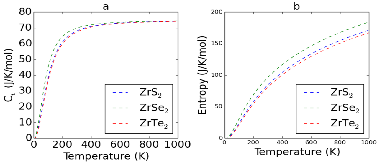
Figure 6.30: vdW-TS calculated Specific heat capacity at constant volume and entropy for the \text{ZrX}_2 ( \text{X} = \text{S}, \text{Se} and \text{Te} ) structures.
