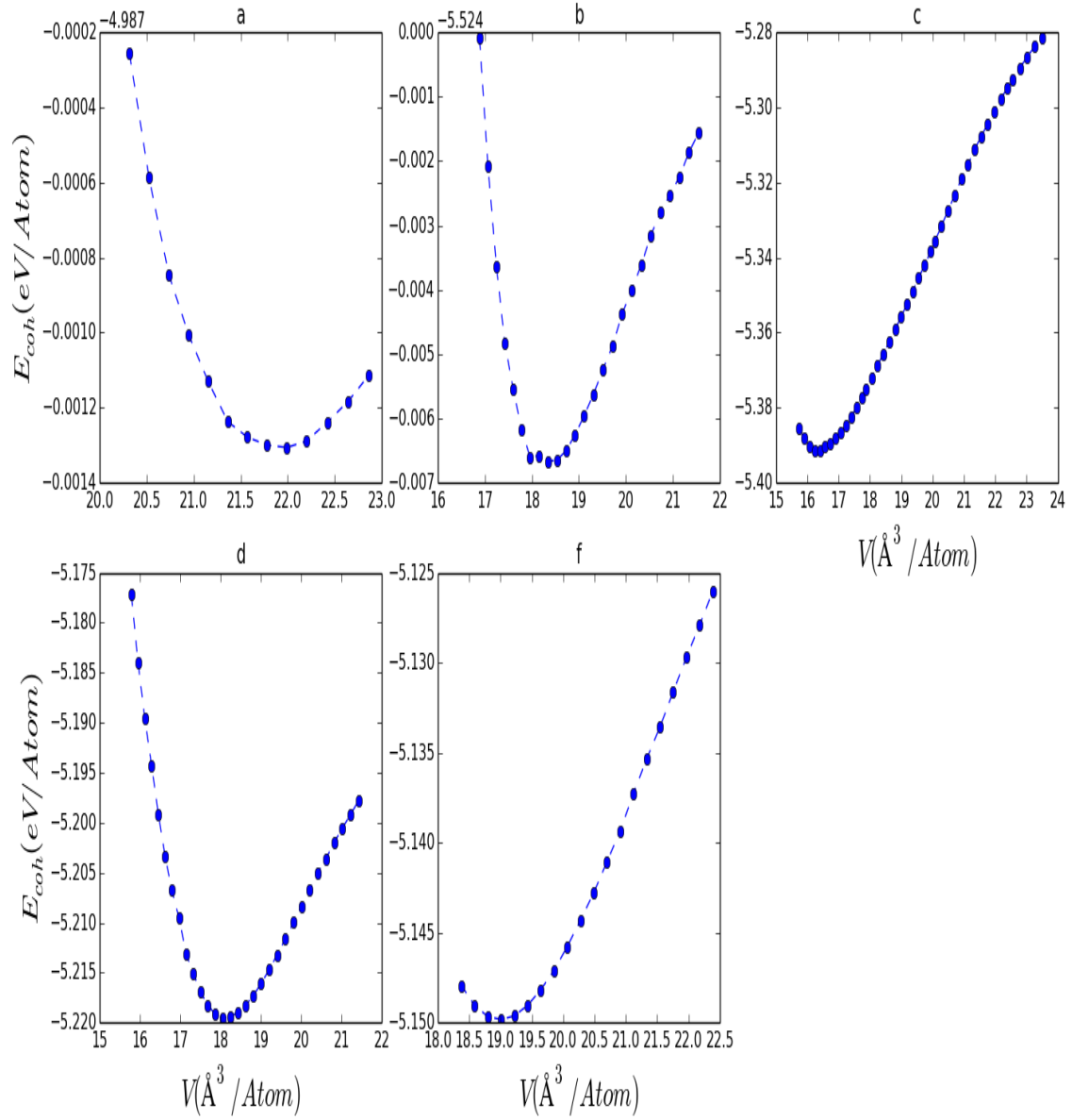
Figure 6.2: \text{TcS}_2 cohesive energy-volume graph calculated using (a) PBE, (b) PBEsol, (c) vdW-TS, (d) DFT-D2 and (f) vdW-DF.
