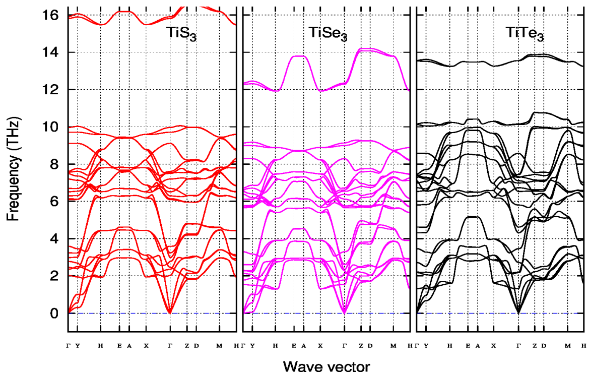
Figure 6.45: \text{TiX}_3 phonon dispersion relation graph calculated using vdW-TS.
