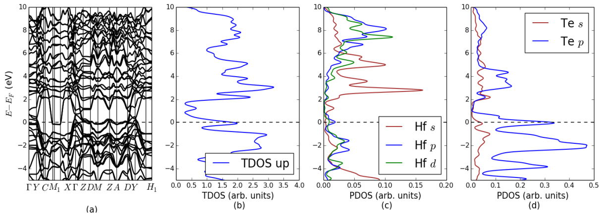
Figure 6.27: vdW-TS HfTe 3 calculated band structure (a) band structure along high symmetry K-points, (b) spin projected TDOS, (c) PDOS of Hf(s,p,d) (d) PDOS of Te (s,p).
