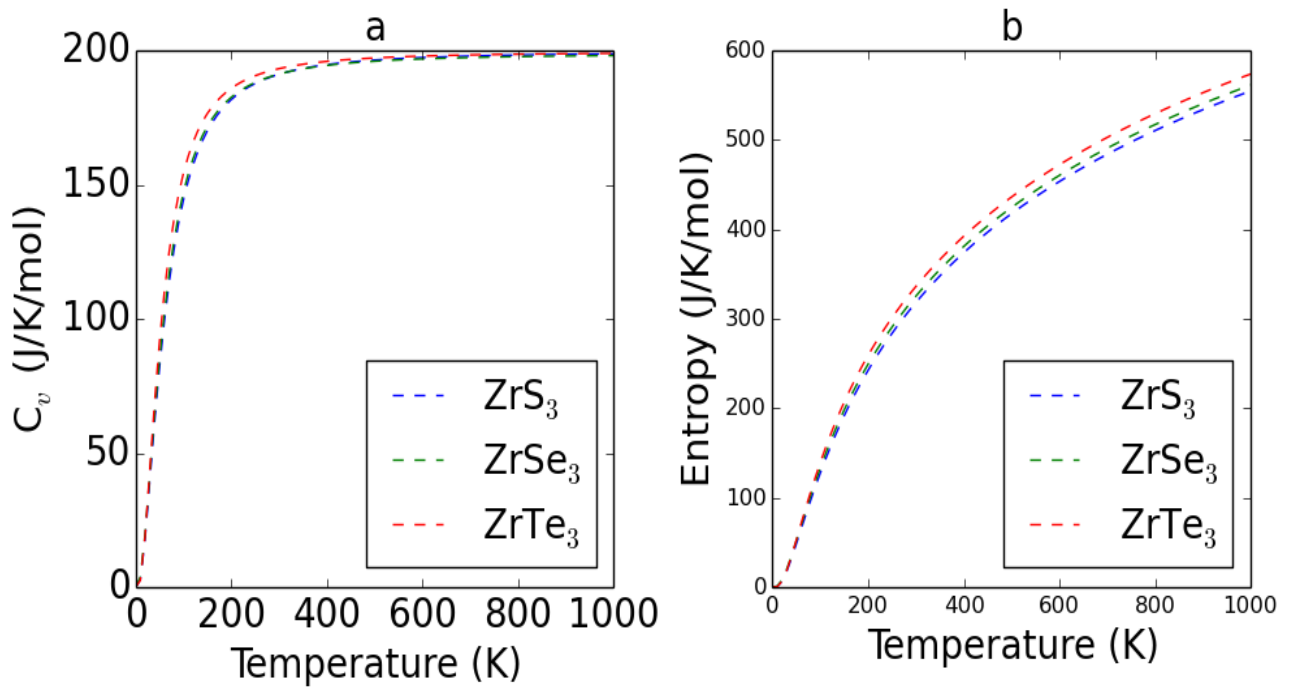
Figure 6.37: vdW-TS calculated specific heat capacity at constant volume and entropy for \text{ZrX}_3 (X= S, Se and Te) structures.
