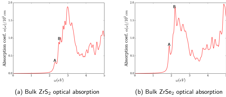
Figure 6.32: ZrX 2 (X= S, Se) BSE calculated optical absorptions.
