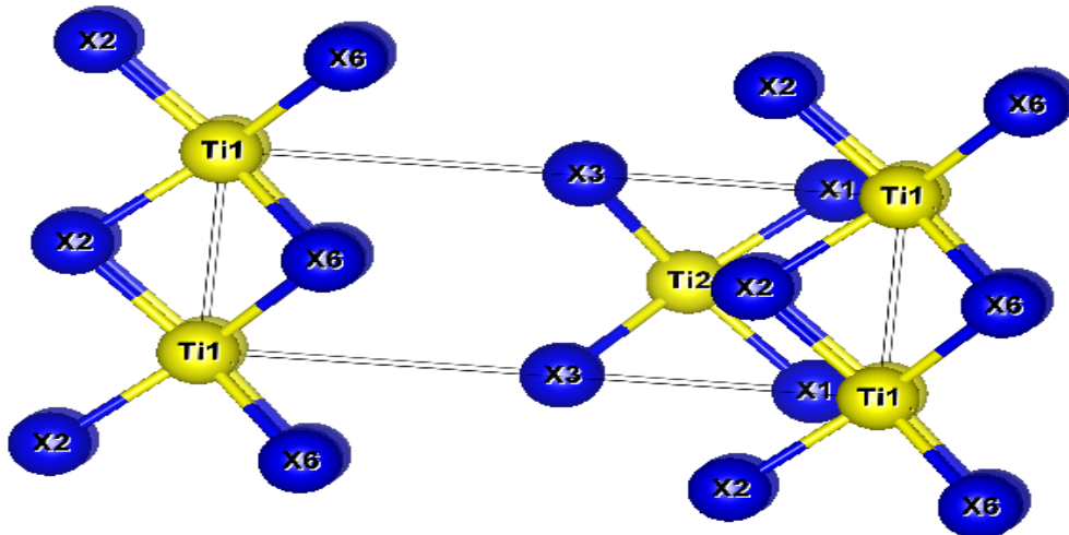
Figure 6.43: \text{TiX}_3 structure.
