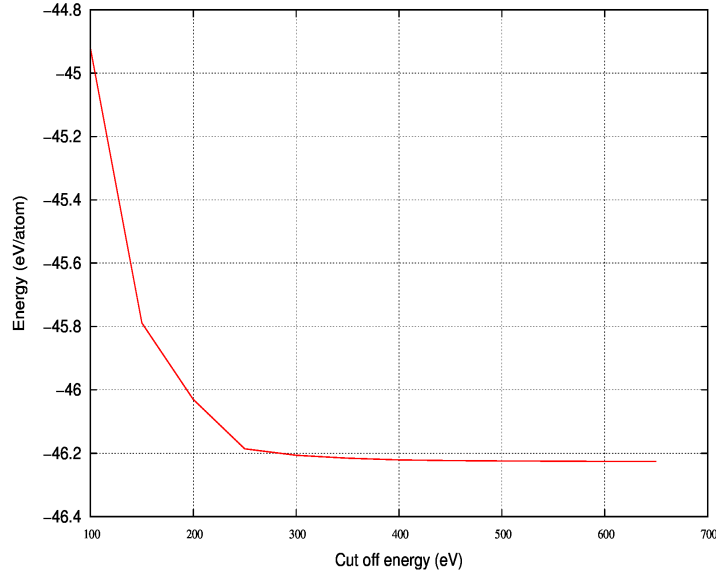
Figure 5.2: Cut-off energy convergence.
