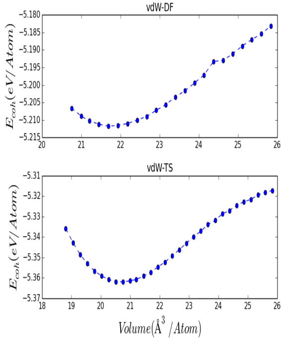
(a) \text{ZrS}_3 cohesive energy-volume graph calculated using (a) vdW-TS and (b) vdW-DF
