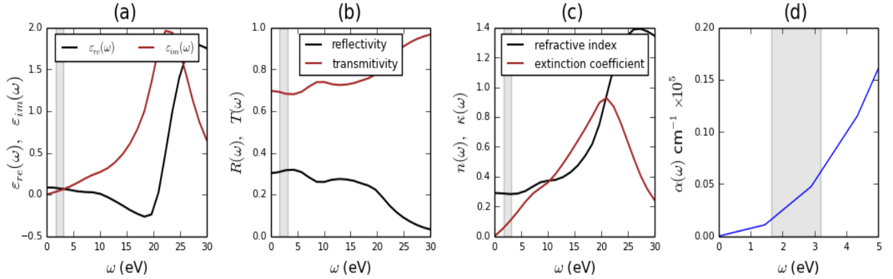
Figure 6.53: G_0W_0 ReSe 2 calculated frequency-dependent optical spectra (a) real \epsilon_{re}(\omega) and the imaginary \epsilon_{im}(\omega) parts of the dielectric function, (b) reflectivity R(\omega) and transmittivity T(\omega) , (c) refraction n(\omega) and extinction coefficient \kappa(\omega) and (d) absorption coefficient \alpha(\omega) . The visible range is shaded.
