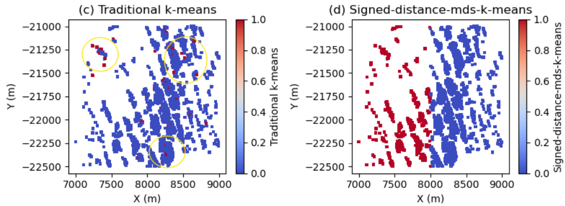
Figure 4.9: Cluster configuration c) Traditional K-means cluster layout showing cluster mixing. d) Signed-distance-mds-k-means cluster layout showing two distinct clusters.
