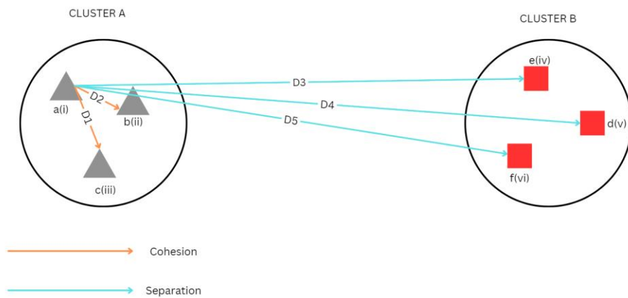
Figure 3.2: Simple graphical illustration of Silhouette calculations and the cluster selection criteria (1) Cohesion demonstrated by D1 and D2 (2) Separation demonstrated by D3, D4 and D5 adopted from Saputra et al. , (2020).
