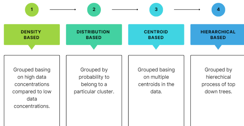
Figure 2.9: Types of clustering methods 1) Density method that develops clusters based on the concentrations of points 2) Distribution method that uses probability of belonging to determine clusters at used data concentration to determine clusters 3) Centroid methods that determines clusters by the a set number of centroids and closer points to centroids belong to a cluster 4) Hierarchical method where a top down decision tree is used to group data into clusters modified from Geeks for Geeks, (2024) .
