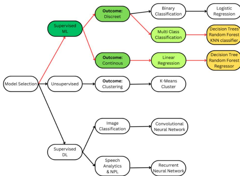
Figure 2.15: ML algorithm selection flow showing the step-by-step process of selecting a model fit for purpose.
