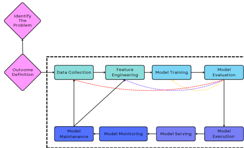
Figure 2.14: A simple ML modelling workflow that shows a summary of the process described above, the identification of problem and model outcome requirements are key in the use of ML models adopted from Andriy, (2019).
