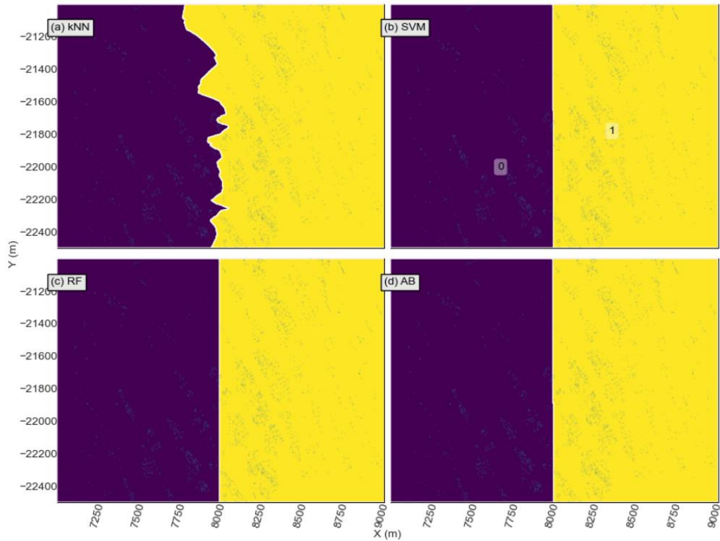
Figure 4.18: Domain boundaries generated by various ML algorithms a) kNN domain boundary b) SVM domain boundary c) RF domain boundary d) AB domain boundary.
