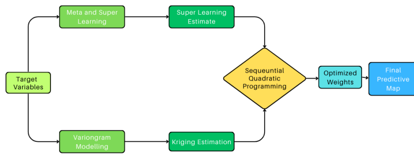
Figure 2.16: Simplified workflow of the combination of super learning and Kriging models for spatial estimation strategy. Illustration, reconstructed from (Erdogan Erten et al., 2022).
