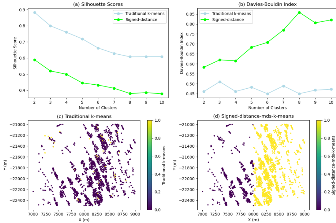
Figure 4.8: Cluster analysis a) Silhouette Scores b) Davies-Bouldin Index c) Traditional K-means clustering distribution d) Signed-distance-mds-K-means clustering distribution.
