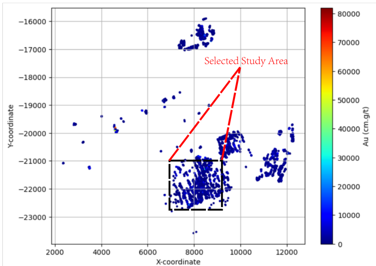
Figure 4.1: Outline of the selected study area (dotted black square) which was trimmed from the whole dataset because of the density of data points around the area.
