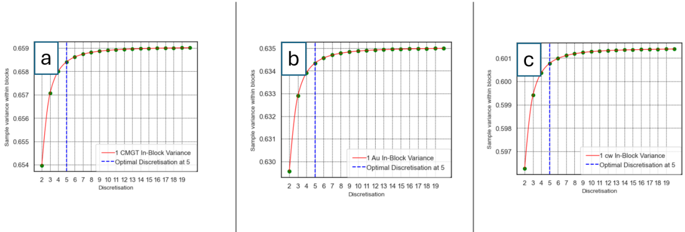
Figure 4.43: Block discretisation results per domain a) Domain 1 Au (cm.g/t) b) Domain 1 Au (g/t) c) Domain 1 CW (cm).
