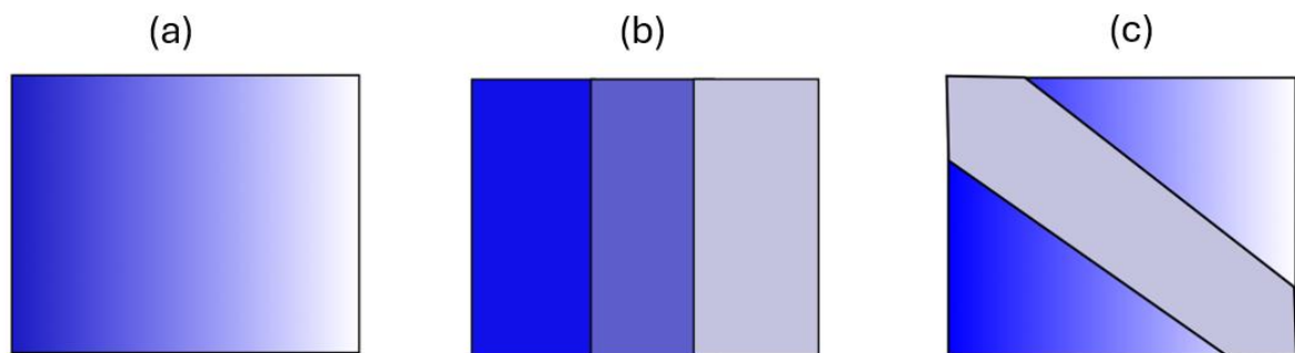
Figure 2.8: Common geological boundaries a) Soft boundary with no distinct break b) Hard boundaries showing hard breaks in between units c) A combination of both soft and hard boundaries which is more complicated to map modified from Kasmaee et al., (2019) .
