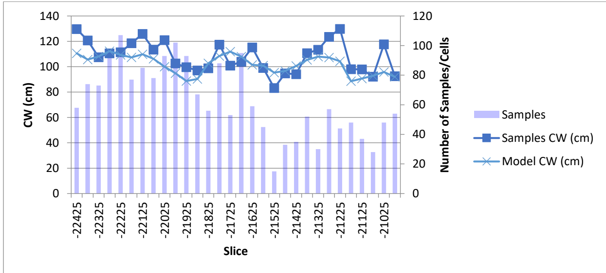
Figure 4.55: Y-axis swath plot showing the estimated values compared to actual grades along the N-S direction representing number of samples, samples CW (cm) and model CW (cm).
