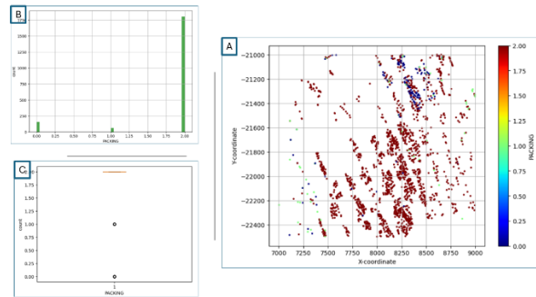
Figure A1: Packing graphical statistics and spatial distribution a) Spatial distribution of Packing values as shown in the study area, b) Histogram indicating frequency occurrence of Packing values.
