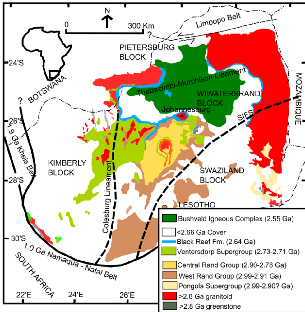
Figure 2.1: Geological Setting of the Witwatersrand Basin, shown are the structural lineaments of the Cotesburg magnetic lineament and Saddleback-Inyoka fault system (SIFS) that squeeze the basin and result in a semi elongated shape with a NE-SW orientation. Also, in shown is the Bushveld igneous complex located NE of the Witwatersrand basin modified from Frimmel & Nwaila, (2020) .
