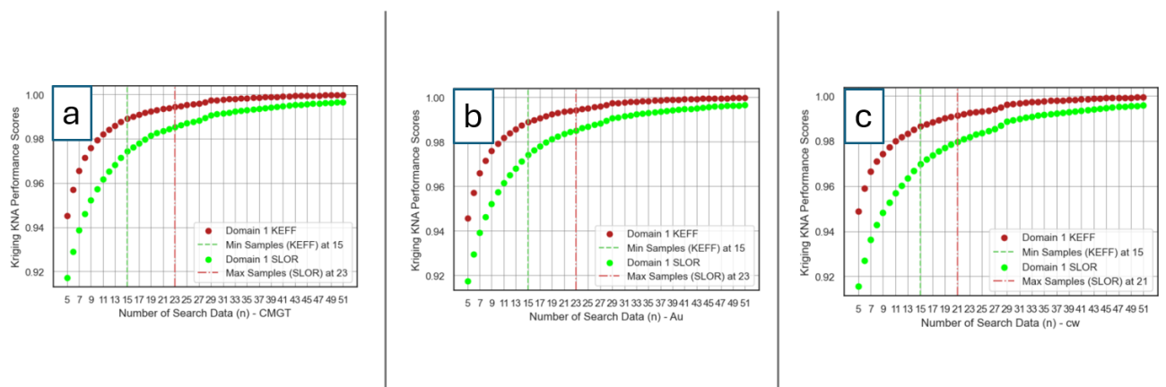
Figure 4.45: QKNA number of sample search selection a) Domain 1 Au (cm.g/t) minimum and maximum number of samples b) Domain 1 Au (g/t) minimum and maximum number of samples c) Domain 1 CW (cm) minimum and maximum number of samples.
