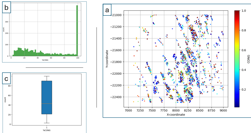
Figure 4.6: Conglomerate (%) graphical statistics and spatial distribution a) Spatial distribution of conglomerate (%) values as shown in the study area, b) Histogram indicating frequency occurrence of conglomerate (%) values c) Box plot showing well distributed conglomerate (%).
