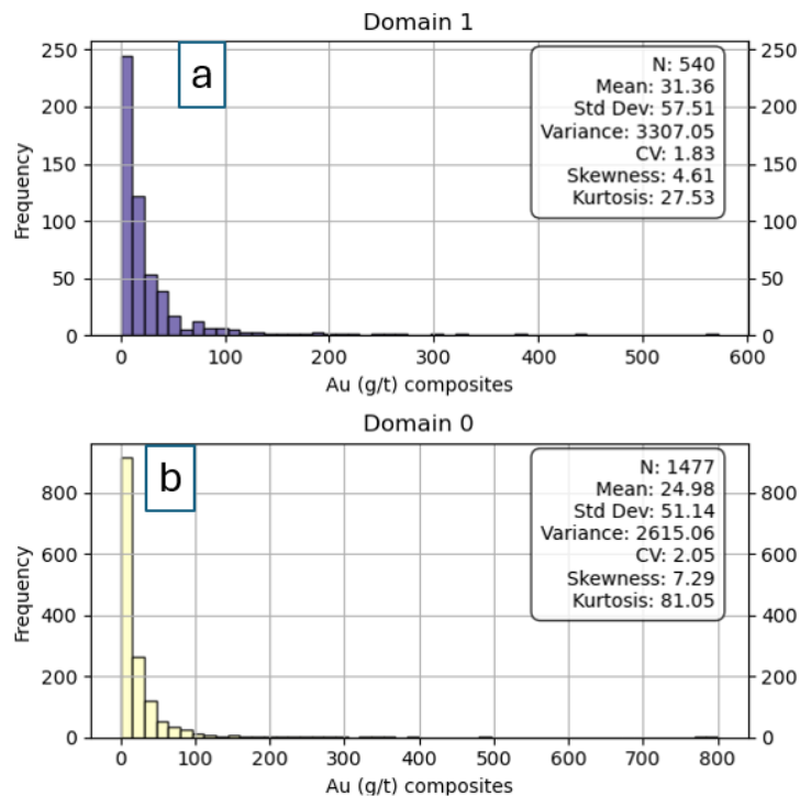
Figure 4.10: Histogram and summary statistics for individual domains a) Domain 1 b) Domain 0.
