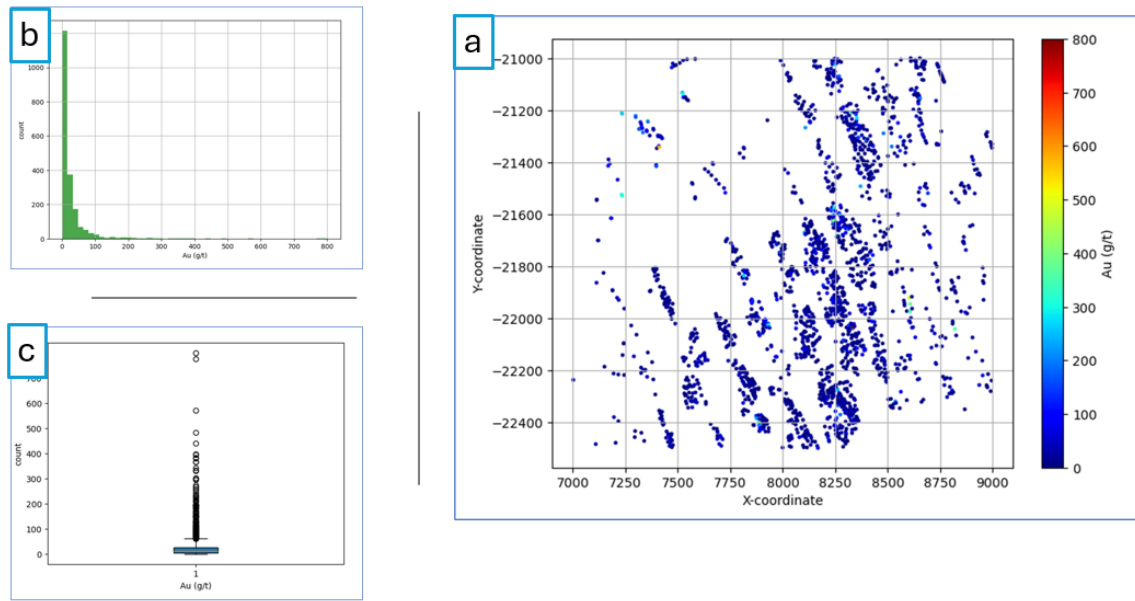
Figure 4.3: Au (g/t) graphical statistics and spatial distribution a) Spatial distribution of Au (g/t) values as shown in the study area, b) Histogram indicating frequency of the occurrence of Au (g/t) values c) Box plot showing the dispersion of outliers from the mean.
