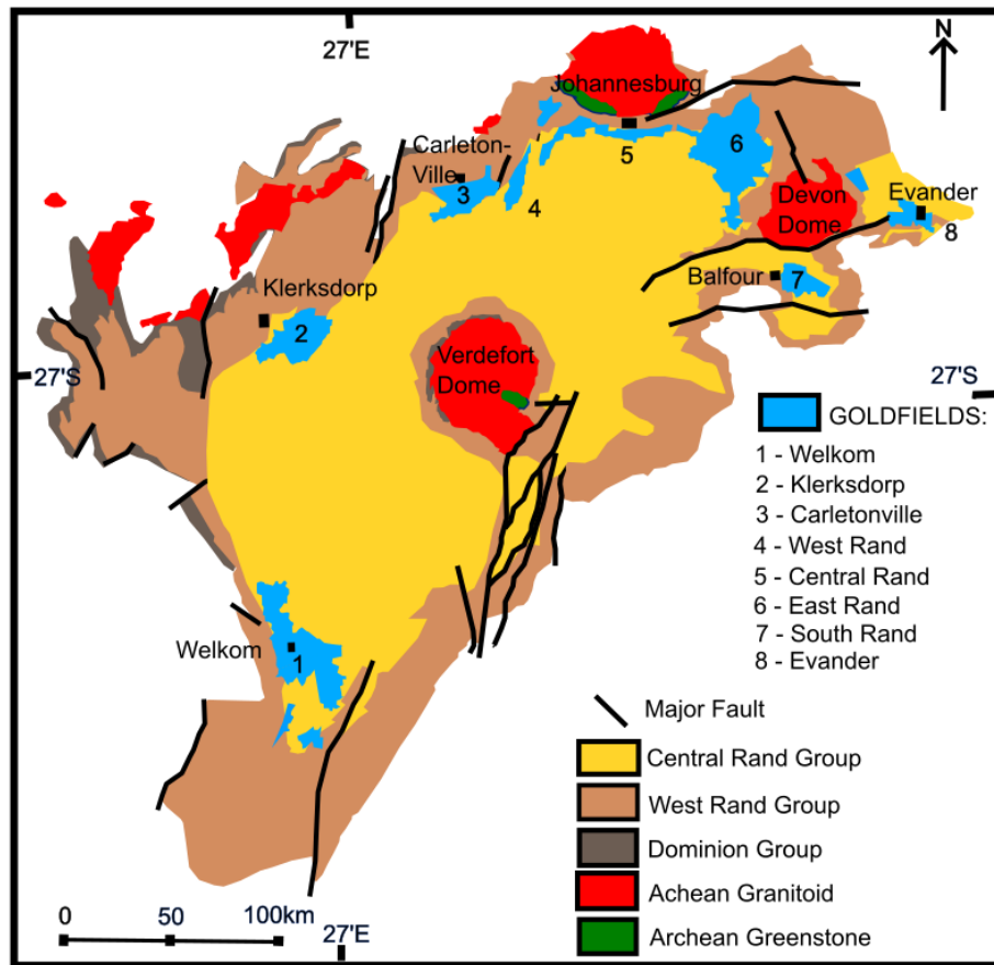
Figure 2.2: Witwatersrand Basin and the various Goldfields which occur in the contact regions between the older West Rand group of the Witwatersrand Supergroup and the younger Central Rand group 1) Welkom goldfield 2) Klerksdorp goldfield 3) Carletonville goldfield 4) West Rand goldfield 5) Central Rand goldfield 6) East Rand goldfield 7) South Rand goldfield 8) Evander goldfield modified from Frimmel & Nwaila, (2020) .
