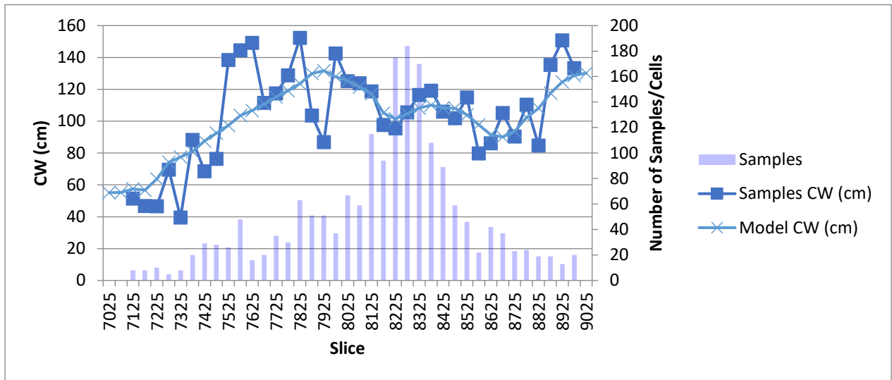
Figure 4.54: X-axis swath plot showing the estimated values compared to actual grades along the E-W direction representing number of samples, samples CW (cm) and model values CW (cm).
