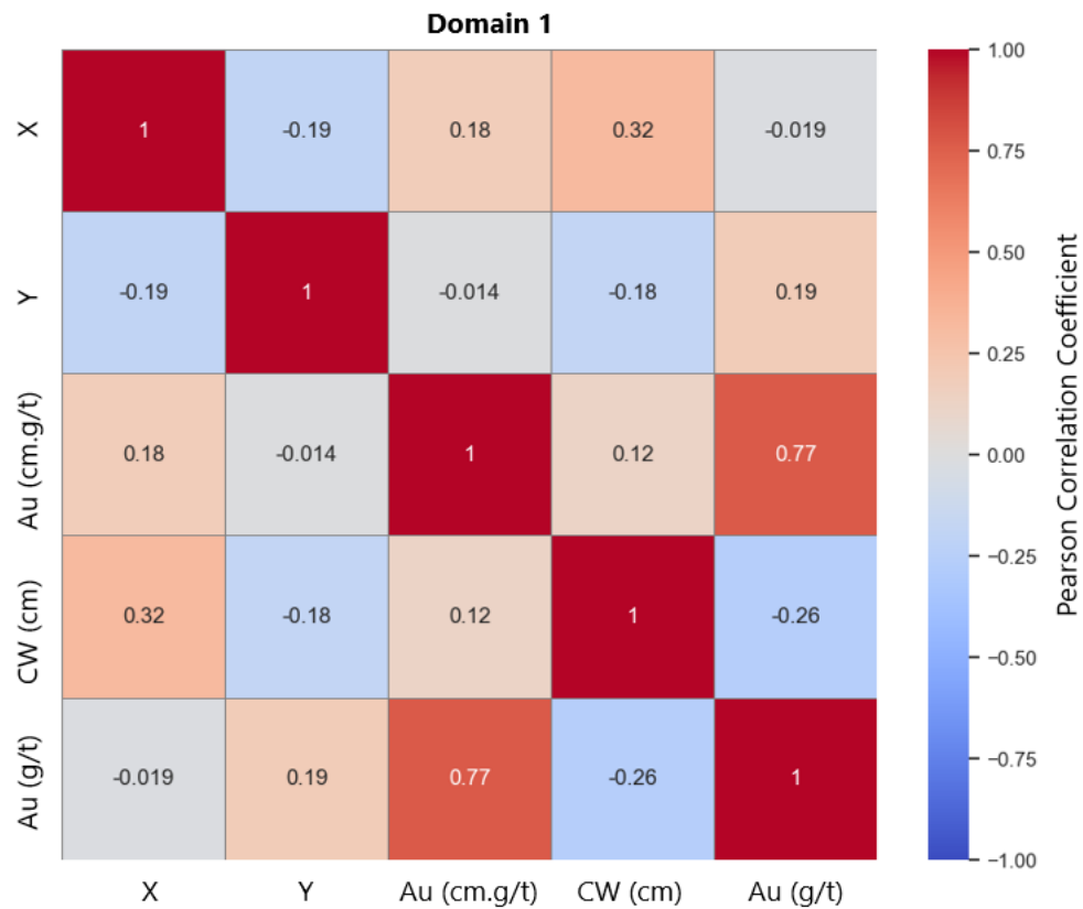
Figure 4.17: Pearson correlation heatmap of selected variables of interest Au (cm.g/t), Au (g/t) and CW (cm) and their spatial locations at Domain 1.
