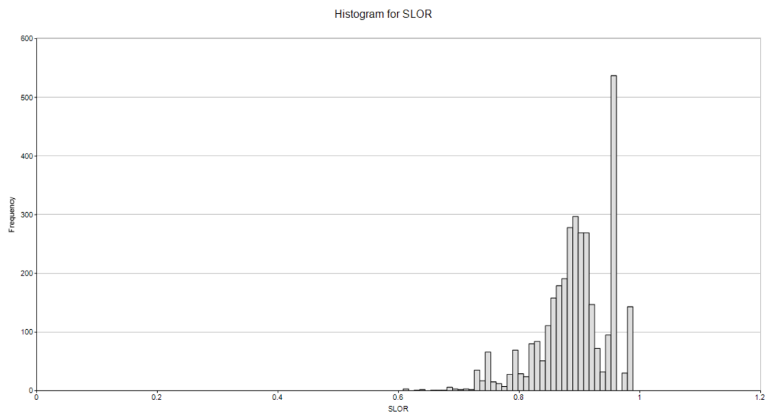
Figure 4.51: Histogram showing the SLOR distribution depicting a mixture of values across domains.
