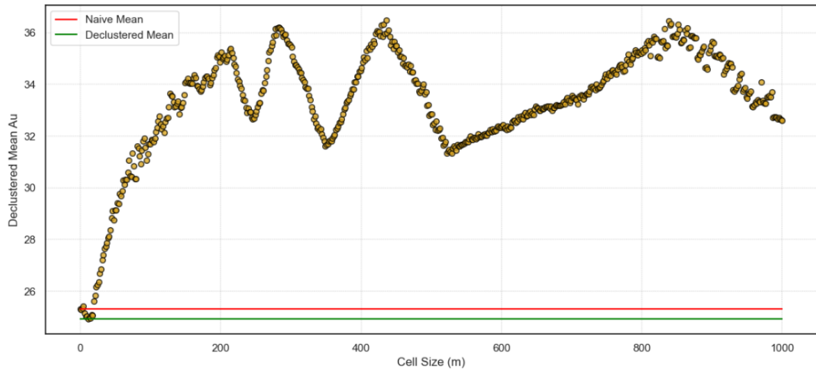
Figure 4.26: Cell size selection for Domain 0 Au (g/t) showing the minimum and maximum naïve and declustered mean corresponding to a cell size.
