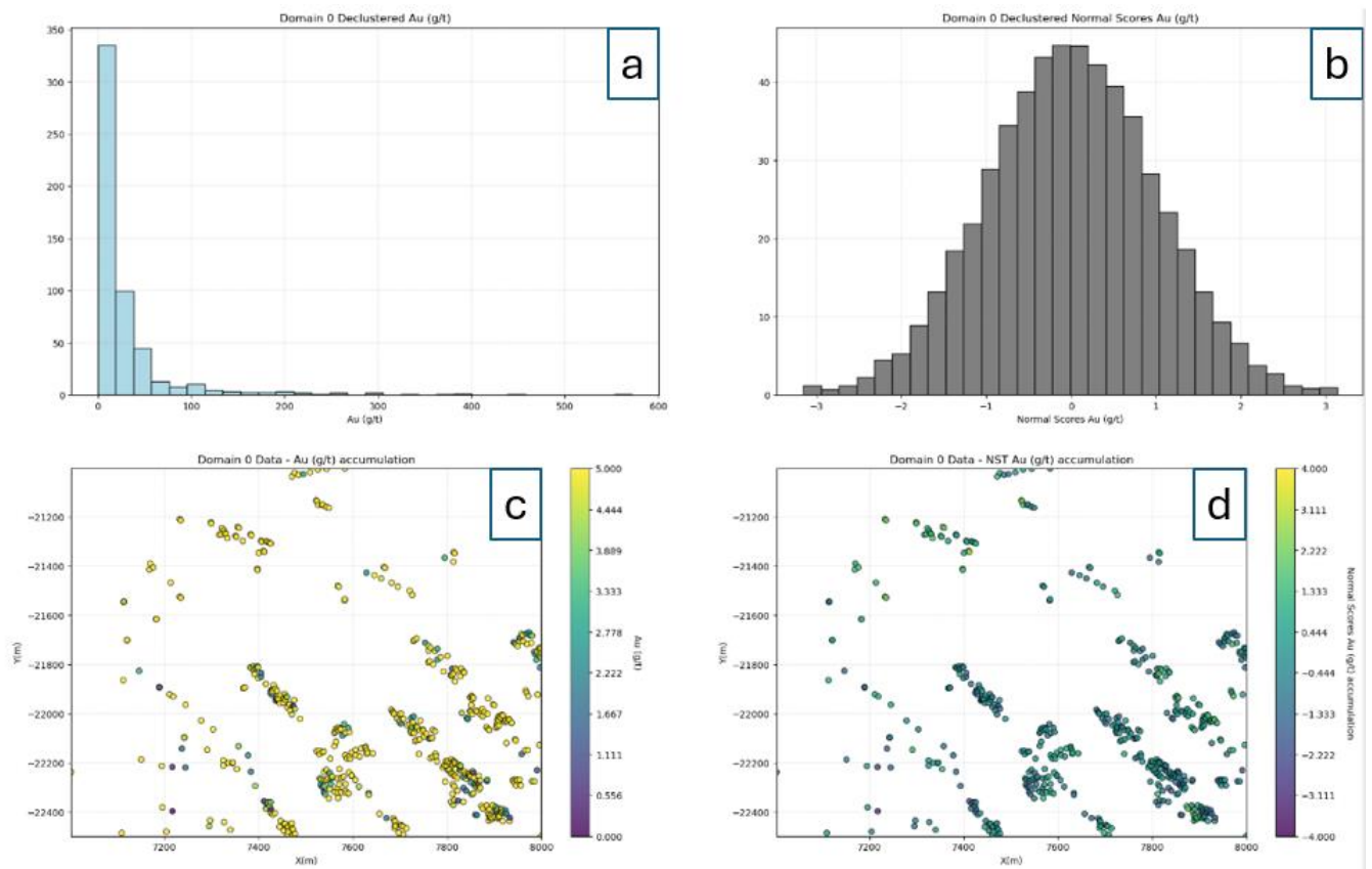
Figure 4.28: Domain 0 declustered Au (g/t) b) Domain 0 declustered normal score Au (g/t) c) Domain 0 declustered Au (g/t) spatial distribution d) Domain 0 normal score Au (g/t) spatial distribution.
