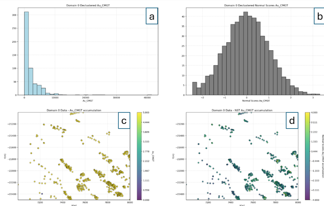
Figure 4.30: Domain 0 declustered Au (cm.g/t) b) Domain 0 declustered normal score Au (cm.g/t) c) Domain 0 declustered Au (cm.g/t) spatial distribution d) Domain 0 normal score Au (cm.g/t) spatial distribution.
