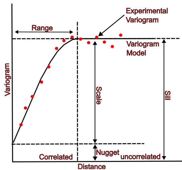
Figure 2.12: Semi variogram structure showing the sill, range and the nugget. It also shows the area of correlation and uncorrelated area that are regions beyond continuity adopted from Bohling, (2005).
