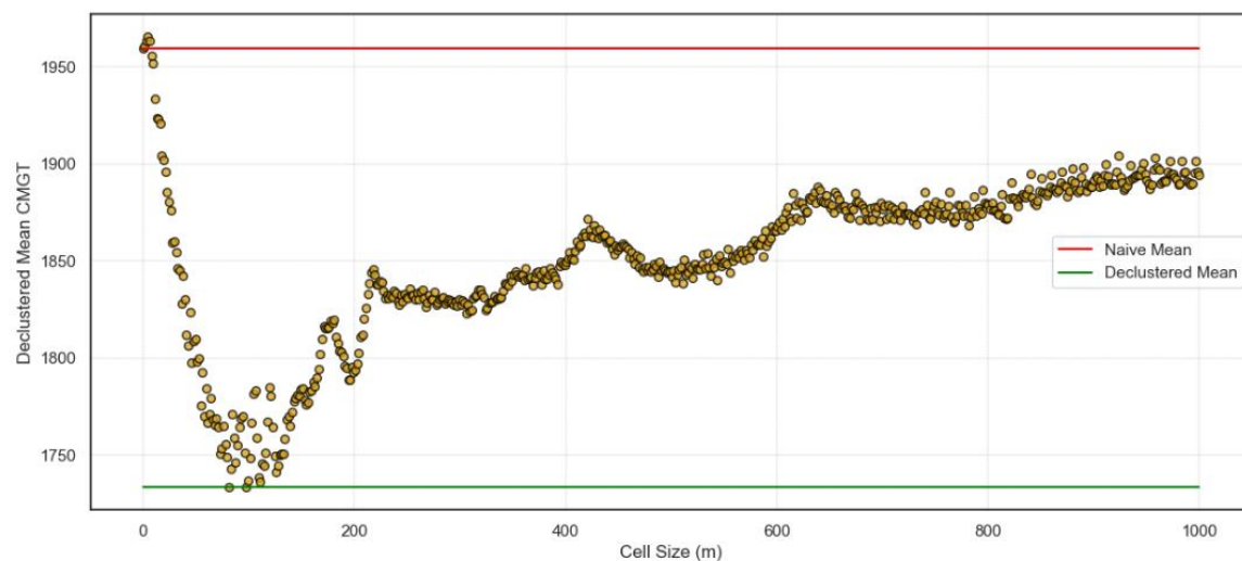
Figure 4.23: Cell size selection for Domain 1 Au (cm.g/t) showing the minimum and maximum naïve and declustered mean corresponding to a cell size.
