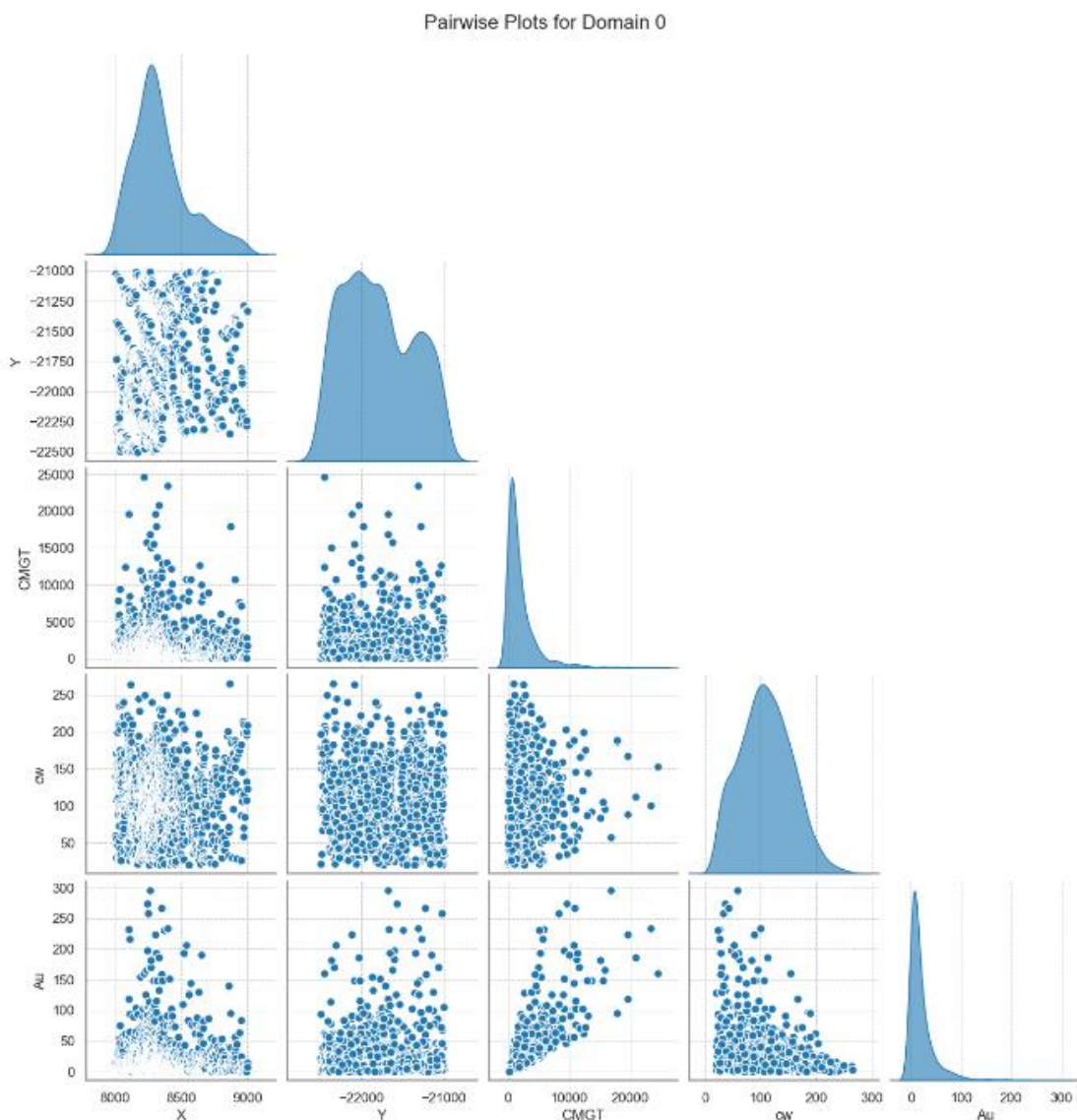
Figure 4.14: Pairwise plots for all the selected variables of interest in Domain 0.
