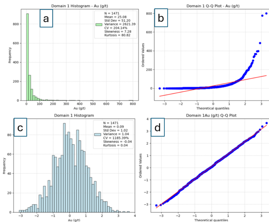
Figure 4.38: Domain 1 Au (g/t) histogram b) Domain 1 Q-Q Au (g/t) plot c) Domain 1 Au (g/t) treated data histogram d) Domain 1 Au (g/t) treated data Q-Q plot.
