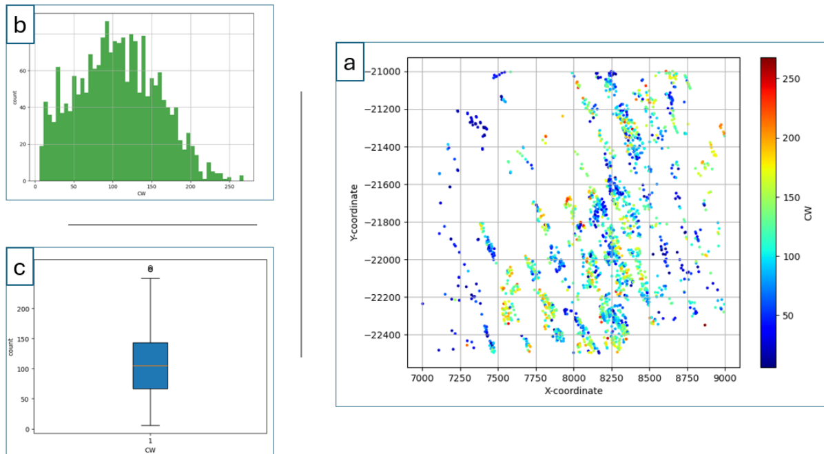
Figure 4.5: CW (cm) graphical statistics and spatial distribution a) Spatial distribution of CW (cm) values as shown in the study area, b) Histogram indicating frequency occurrence of CW (cm) c) Box plot showing a balanced occurrence of high and low CW values.
