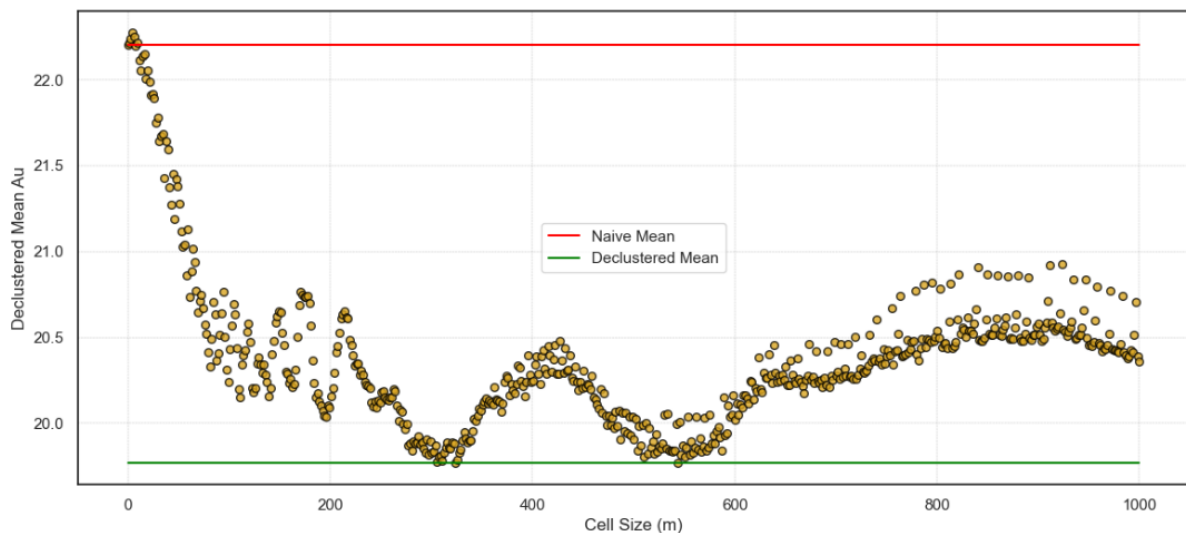
Figure 4.27: Cell size selection for Domain 1 Au (g/t) showing the minimum and maximum naïve and declustered mean corresponding to a cell size.
