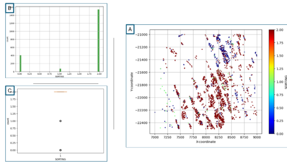
Figure A3: Sorting graphical statistics and spatial distribution a) Spatial distribution of Sorting values as shown in the study area, b) Histogram indicating frequency occurrence of Sorting values.
