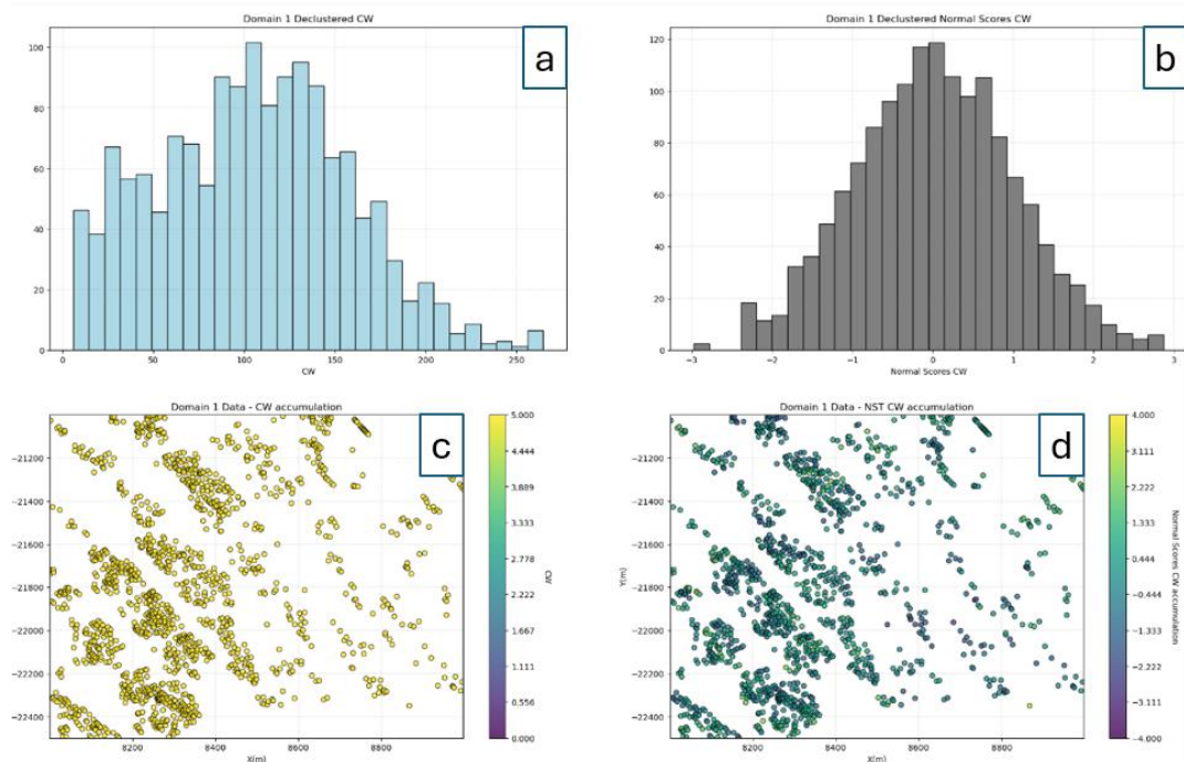
Figure 4.32: : Domain 1 declustered CW (cm) b) Domain 1 declustered normal score CW (cm) c) Domain 1 declustered CW (cm) spatial distribution d) Domain 1 normal score CW (cm) spatial distribution.
