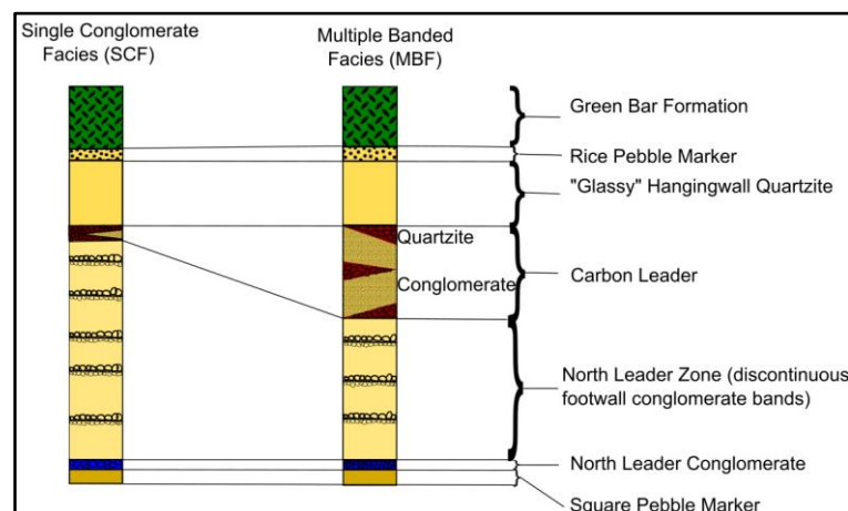
Figure 2.3: Carbon Leader Reef single conglomerate facies showing shorter and less diluted reef units on the (left) and, the multiple banded facies showing higher dilution and cyclic occurrences of individual bands modified from Shango Solutions (2007).
