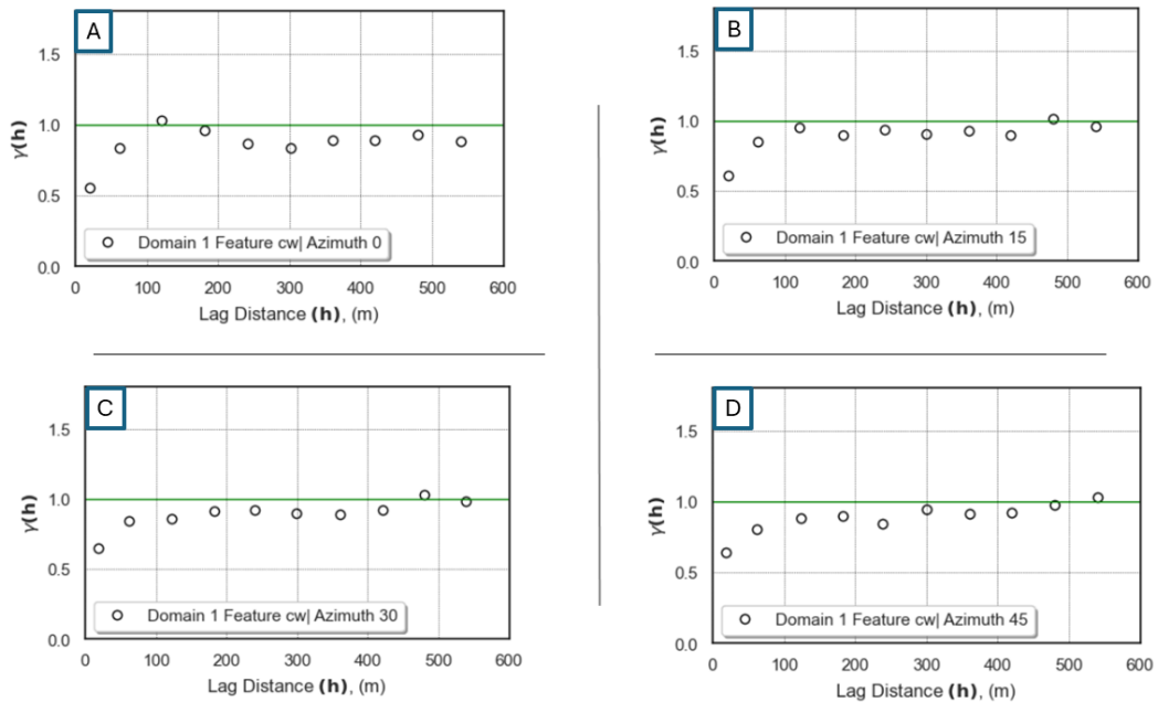
Figure B6: Experimental variograms a) Domain 1 CW (cm) azimuth 0 b) Domain 1 CW (cm) azimuth 15 c) Domain 1 CW (cm) azimuth 30 d) Domain 1 CW (cm) azimuth 45.
