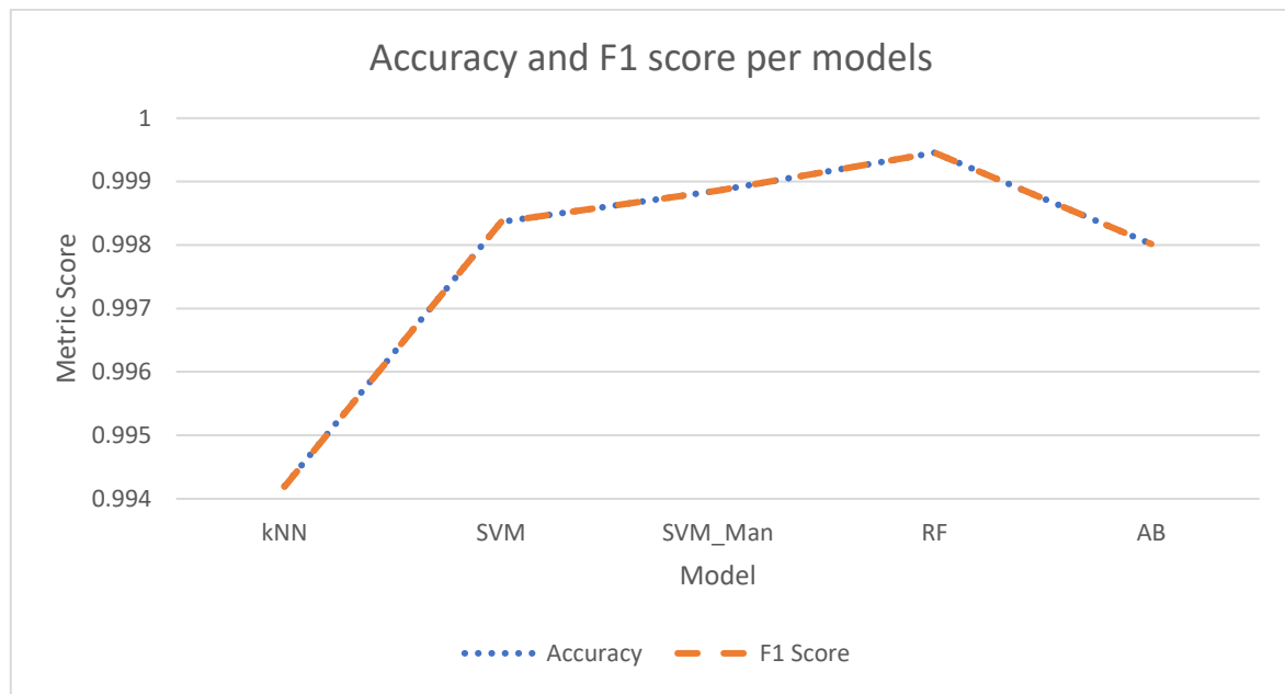
Figure 4.20: a) Line graph illustration of average Accuracy and F1 scores across the selected ML algorithms.
