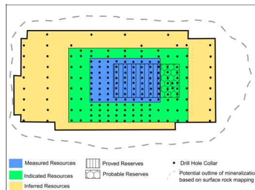
Figure 2.5: Mineral resources and reserves demarcation according to drill hole spacing confidence. Smaller drillhole spacing increases confidence from resources to reserves modified from Jowitt and McNulty (2021).
