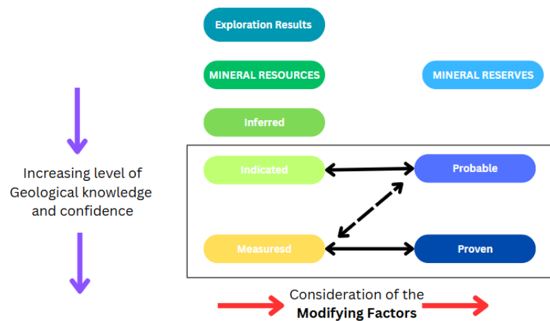
Figure 2.4: Categorisation of resources and reserves indicating the transitional considerations between the two in internationally recognised reporting standards modified from (CRIRSCO, 2024; SAMREC, 2016).
