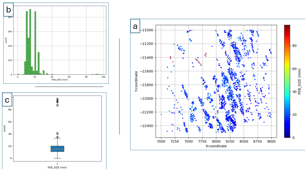
Figure 4.7: Pebble size (mm) graphical statistics and spatial distribution a) Spatial distribution of Pebble size (mm) values as shown in the study area, b) Histogram indicating frequency occurrence of Pebble size (mm) values c) Box plot showing the distribution of pebble sizes which are concentrated around 20 mm and a few high values.
