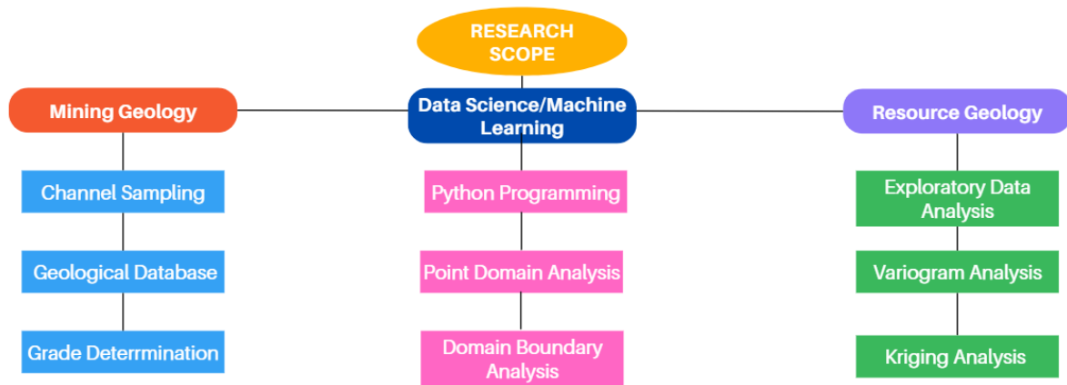
Figure 1.2: An outline indicating the levels of this research and the synergy of different geoscience fields. It includes mining geology (left), showing the onsite sampling type used in data collection, data management and storage and the grade determination methods. Data science (middle) involves the use of Python as baseline computing language to do clustering and classification of domains. Resource geology (right) involves the use of traditional geostatistics workflows that includes data pre-processing, quantitative Kriging analysis, ordinary Kriging, estimation and post estimation.
