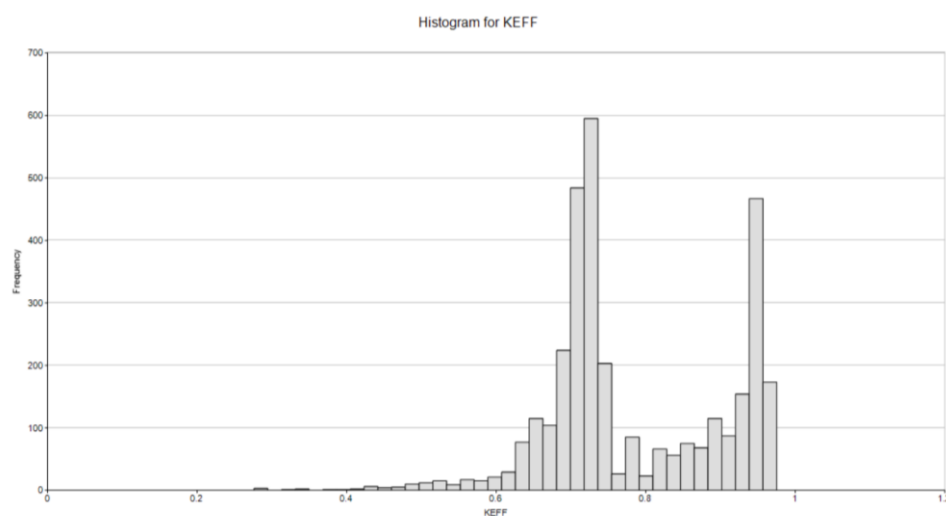
Figure 4.49: Histogram showing the KEFF distribution depicting a bimodal distribution.
