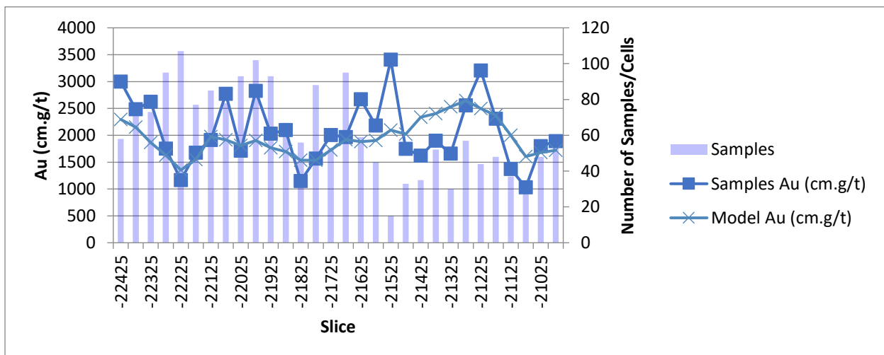
Figure 4.53: Y-axis swath plot showing the estimated values compared to actual grades along the N-S direction representing number of samples, samples Au (cm.g/t) and model Au (cm.g/t).
