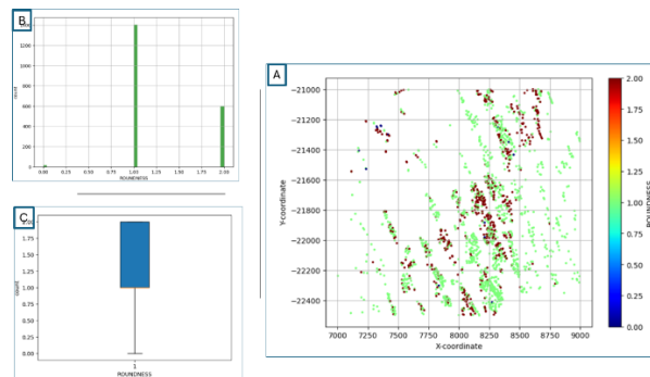
Figure A2: Roundness graphical statistics and spatial distribution a) Spatial distribution of Roundness values as shown in the study area, b) Histogram indicating frequency occurrence of Roundness values.
