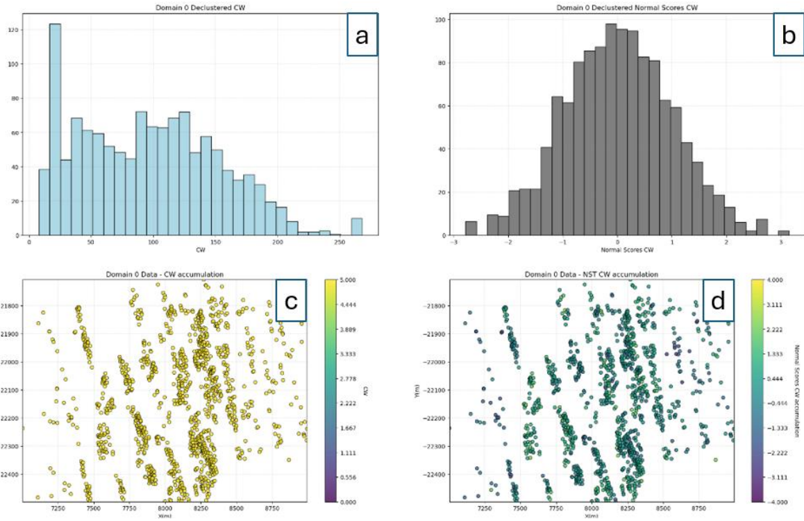
Figure 4.29: Domain 0 declustered CW (cm) b) Domain 0 declustered normal score CW (cm) c) Domain 0 declustered CW (cm) spatial distribution d) Domain 0 normal score CW (cm) spatial distribution.
