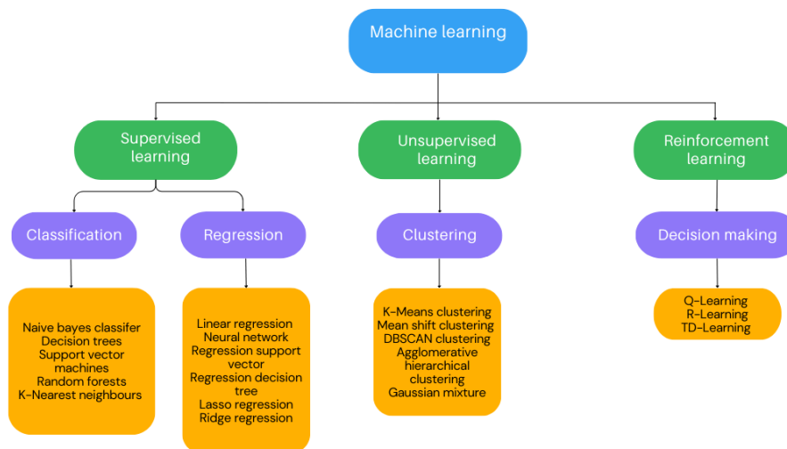
Figure 2.13: ML categories and their respective algorithms (orange boxes) 1) Supervised learning methods that used labelled data for learning 2) Unsupervised learning methods use unlabelled data and no human interaction (independent methods) 3) Reinforcement learning methods rely on learning based on cumulative rewards adopted from Ayodele, (2010) .
