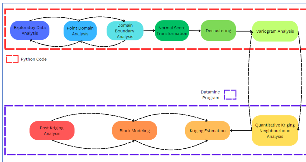
Figure 3.1: Simple graphical illustration of methodology steps and modelling environment used at each step.
