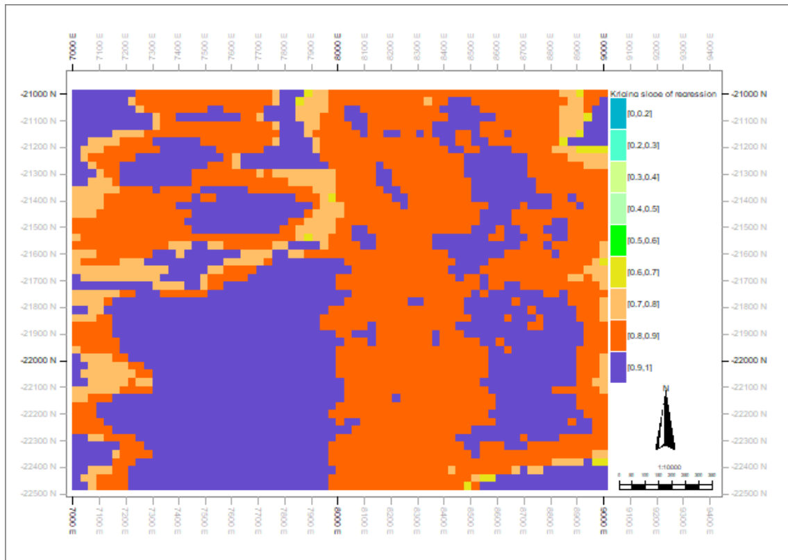
Figure 4.50: 2D map showing the spatial distribution of SLOR results.
