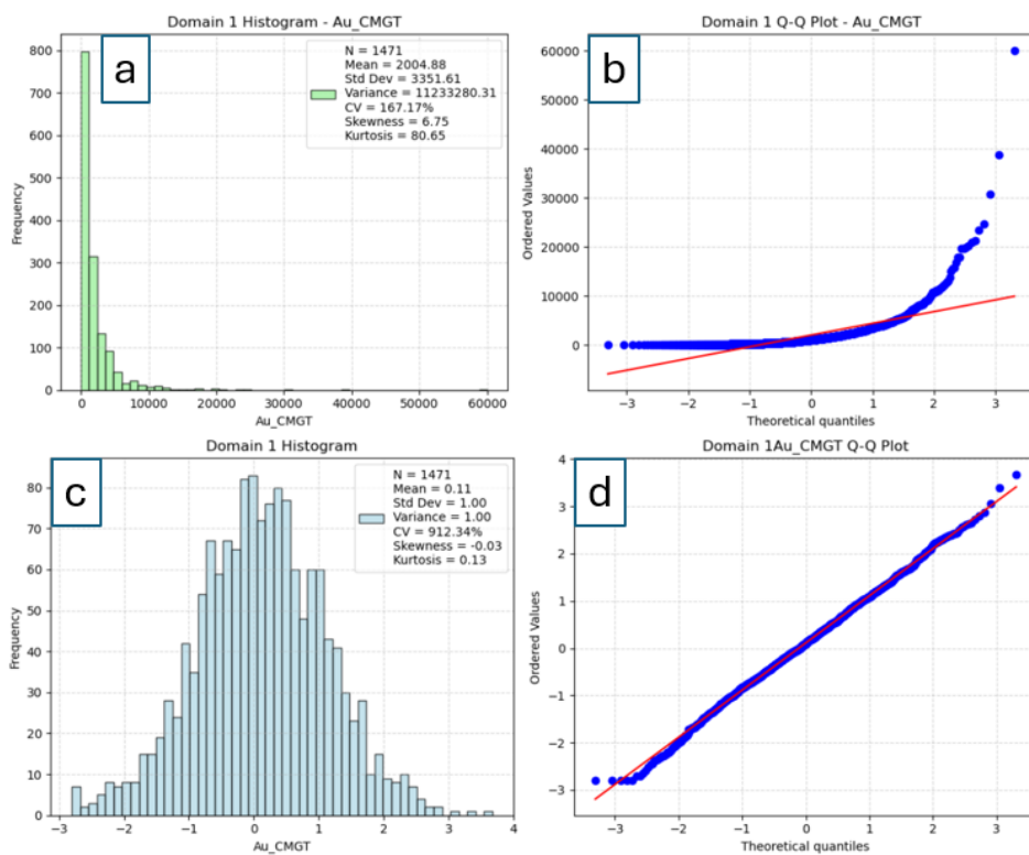
Figure 4.37: Domain 1 Au (cm.g/t) histogram b) Domain 1 Q-Q Au (cm.g/t) plot c) Domain 1 Au (cm.g/t) treated data histogram d) Domain 1 Au (cm.g/t) treated data Q-Q plot.
