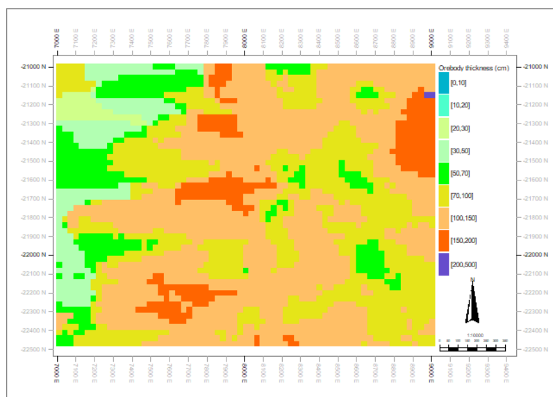
Figure 4.47: 2D map showing the spatial distribution of CW (cm) Kriging results.
