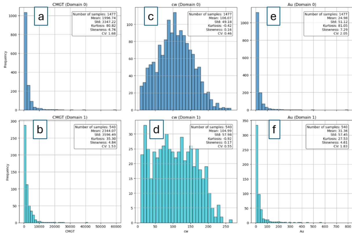
Figure 4.11: Feature histogram and summary statistics per domain a) Au (cm.g/t) Domain 0 b) Au (cm.g/t) Domain 1 c) CW (cm) Domain 0 d) CW (cm) Domain 1 e) Au (g/t) Domain f) Au (g/t) Domain 1.
