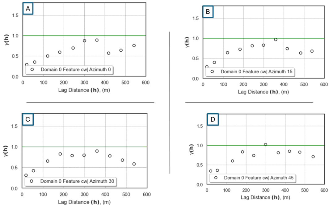
Figure B3: Experimental variograms a) Domain 0 CW (cm) Azimuth 0 b) Domain 0 CW (cm) azimuth 15 c) Domain 0 CW (cm) azimuth 30 d) Domain 0 CW (cm) azimuth 45.
