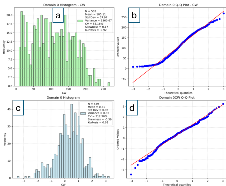
Figure 4.36: Domain 0 CW (cm) histogram b) Domain 0 Q-Q CW (cm) plot c) Domain 0 CW (cm) treated data histogram d) Domain 0 CW (cm) treated data Q-Q plot.
