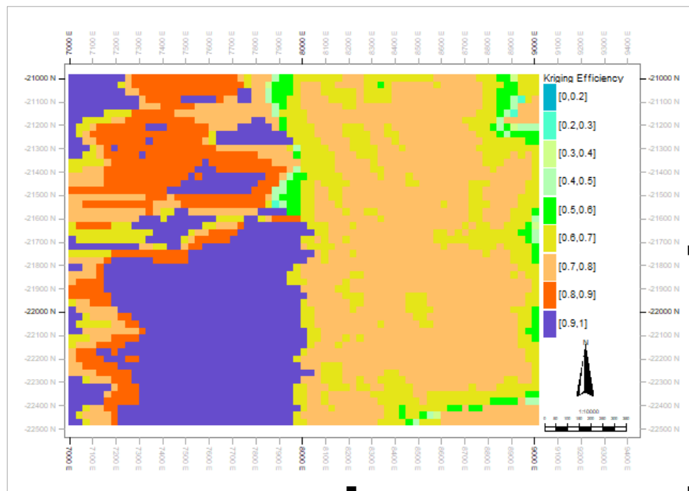
Figure 4.48: 2D map showing the spatial distribution of KEFF results.
