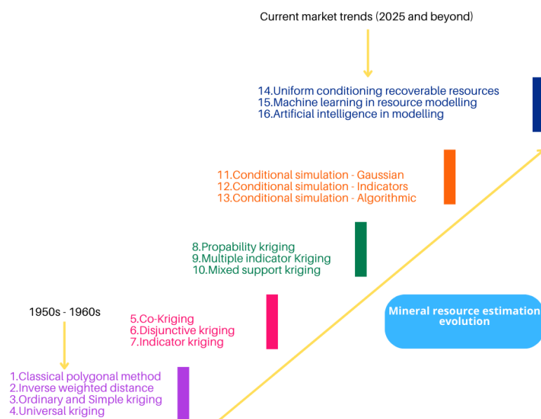
Figure 2.6: Evolution of mineral resource estimation methods/tools over time showing the older and simpler methods on the (lower left) and the recent and more sophisticated methods in the (top right) adapted from Dohm (2021) .
