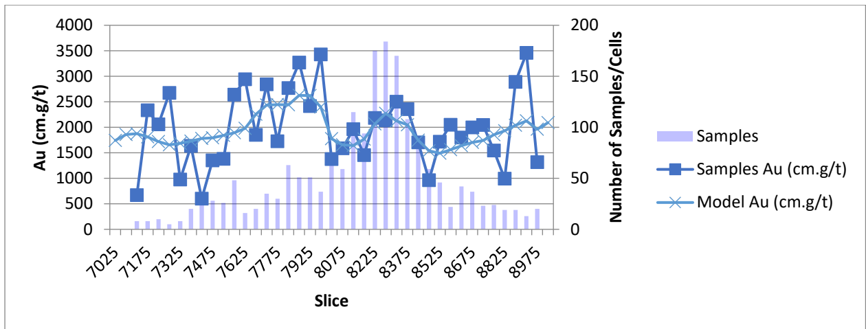
Figure 4.52: X-axis swath plot showing the estimated values compared to actual grades along the E-W direction representing number of samples, samples Au (cm.g/t) and model Au (cm.g/t).
