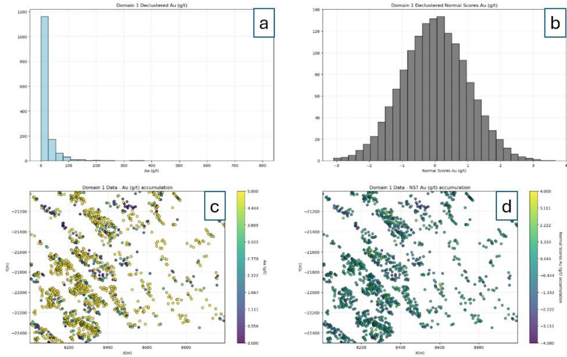
Figure 4.31: a) Domain 1 declustered Au (g/t) b) Domain 1 declustered normal score A (g/t) c) Domain 1 declustered Au (g/t) spatial distribution d) Domain 1 normal score Au (g/t) spatial distribution.
