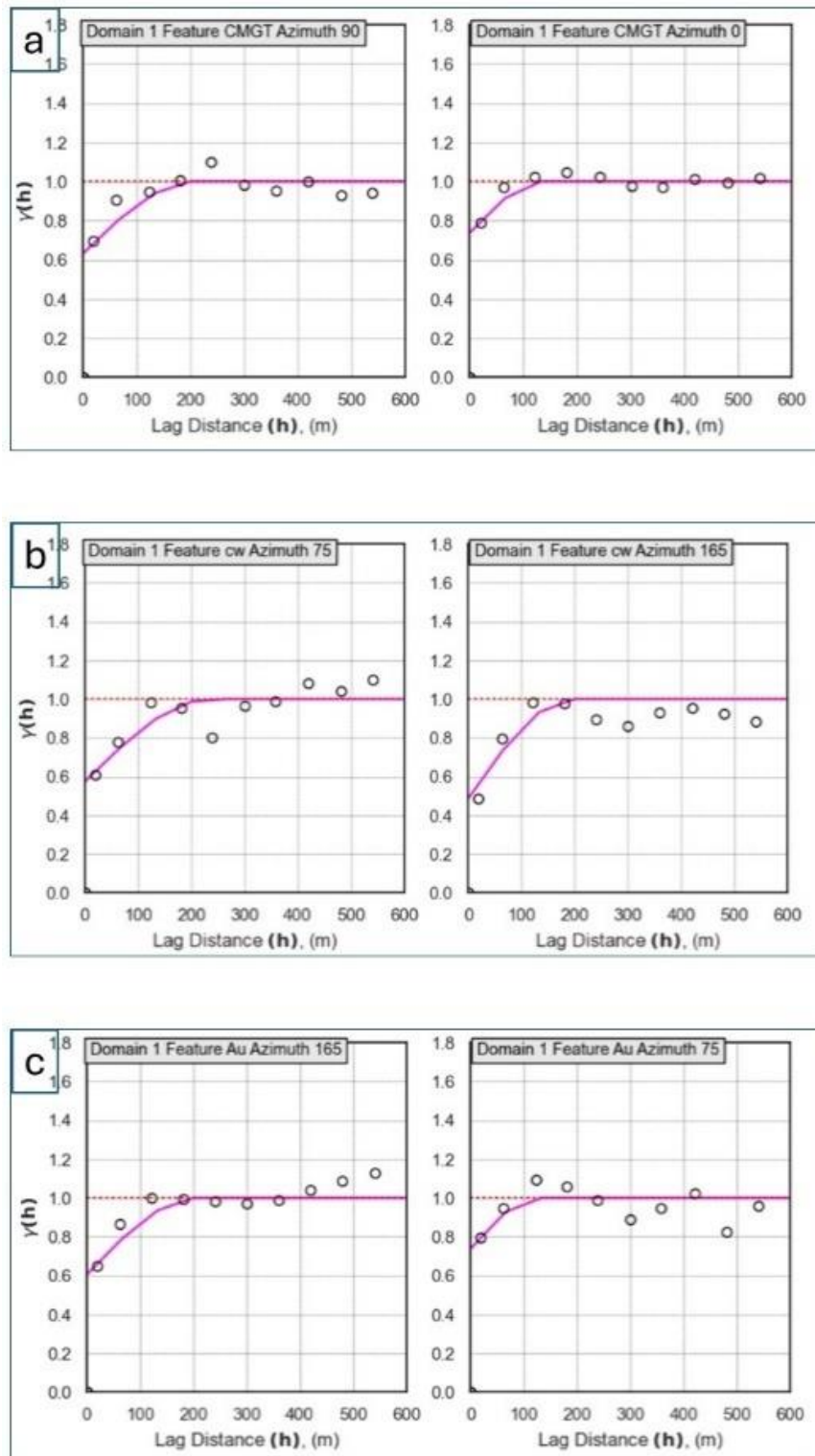
Figure 4.41: Fitted variogram model Domain 1 a) Au (cm.g/t) major angle 90 and minor angle 0 b) CW (cm) major angle 75 and minor angle 165 C) Domain 1 Au (g/t) major angle 165 and minor angle 75.
