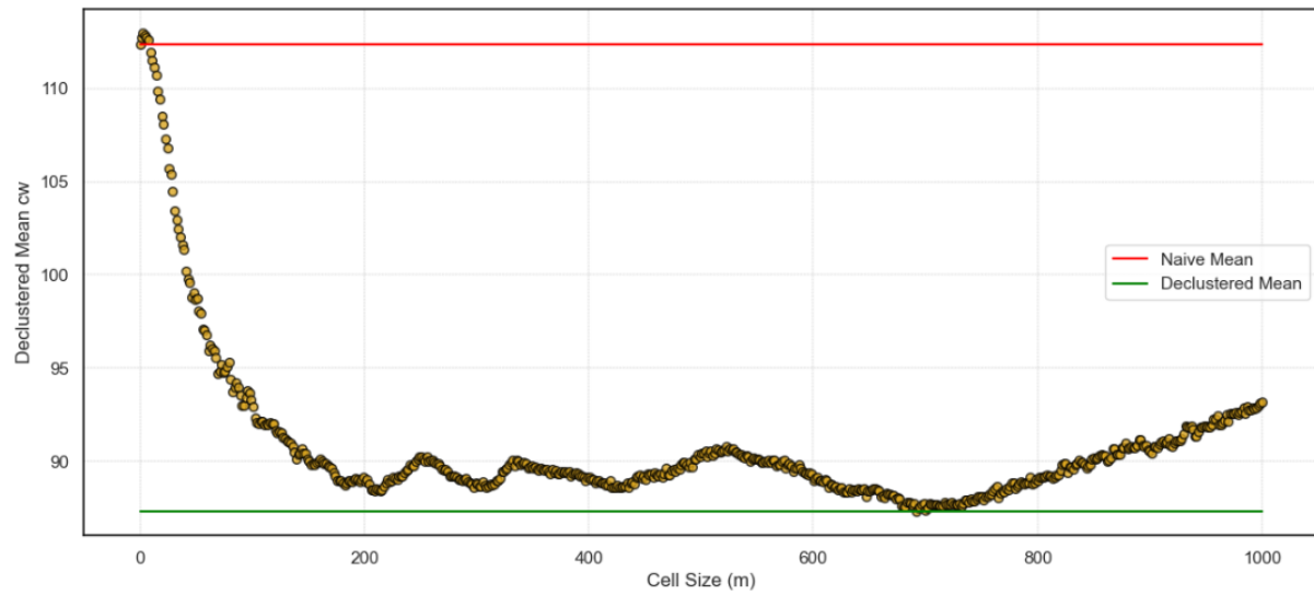
Figure 4.24: Cell size selection for Domain 0 CW (cm) showing the minimum and maximum naïve and declustered mean corresponding to a cell size.
