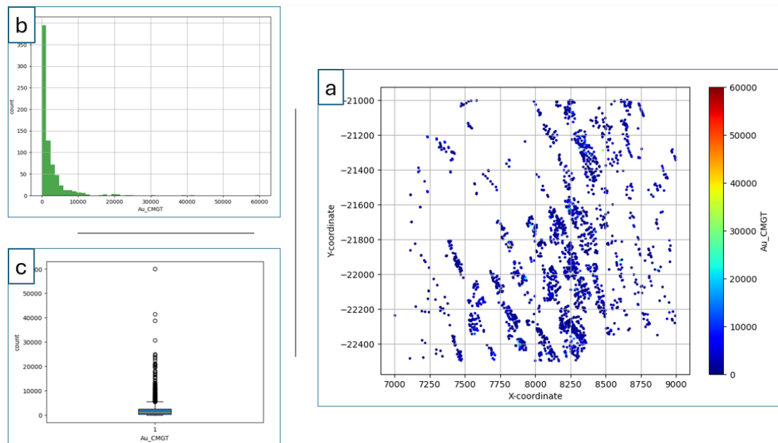
Figure 4.4: Au (cm.g/t) graphical statistics and spatial distribution a) Spatial distribution of Au (cm.g/t) values as shown in the study area, b) Histogram indicating frequency occurrence of Au (cm.g/t) values c) Box plot displaying the concentration of data around the mean and some outliers detected beyond that.
