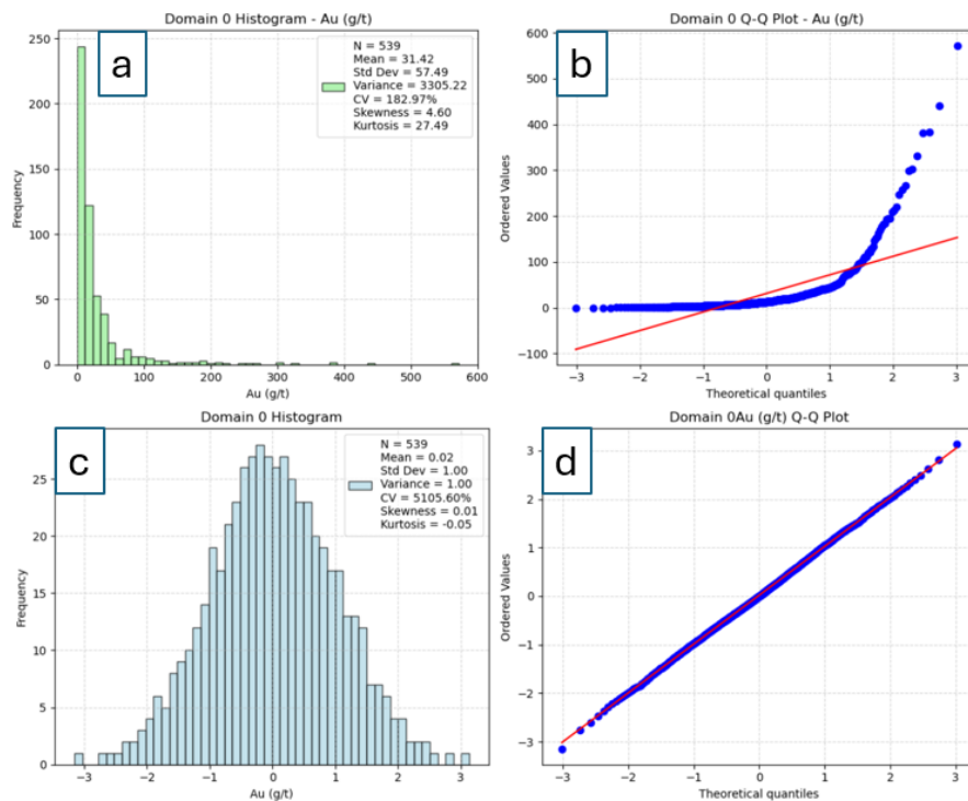
Figure 4.35: Domain 0 Au (g/t) histogram b) Domain 0 Q-Q Au (g/t) plot c) Domain Au (g/t) treated data histogram d) Domain Au (g/t) treated data Q-Q plot.
