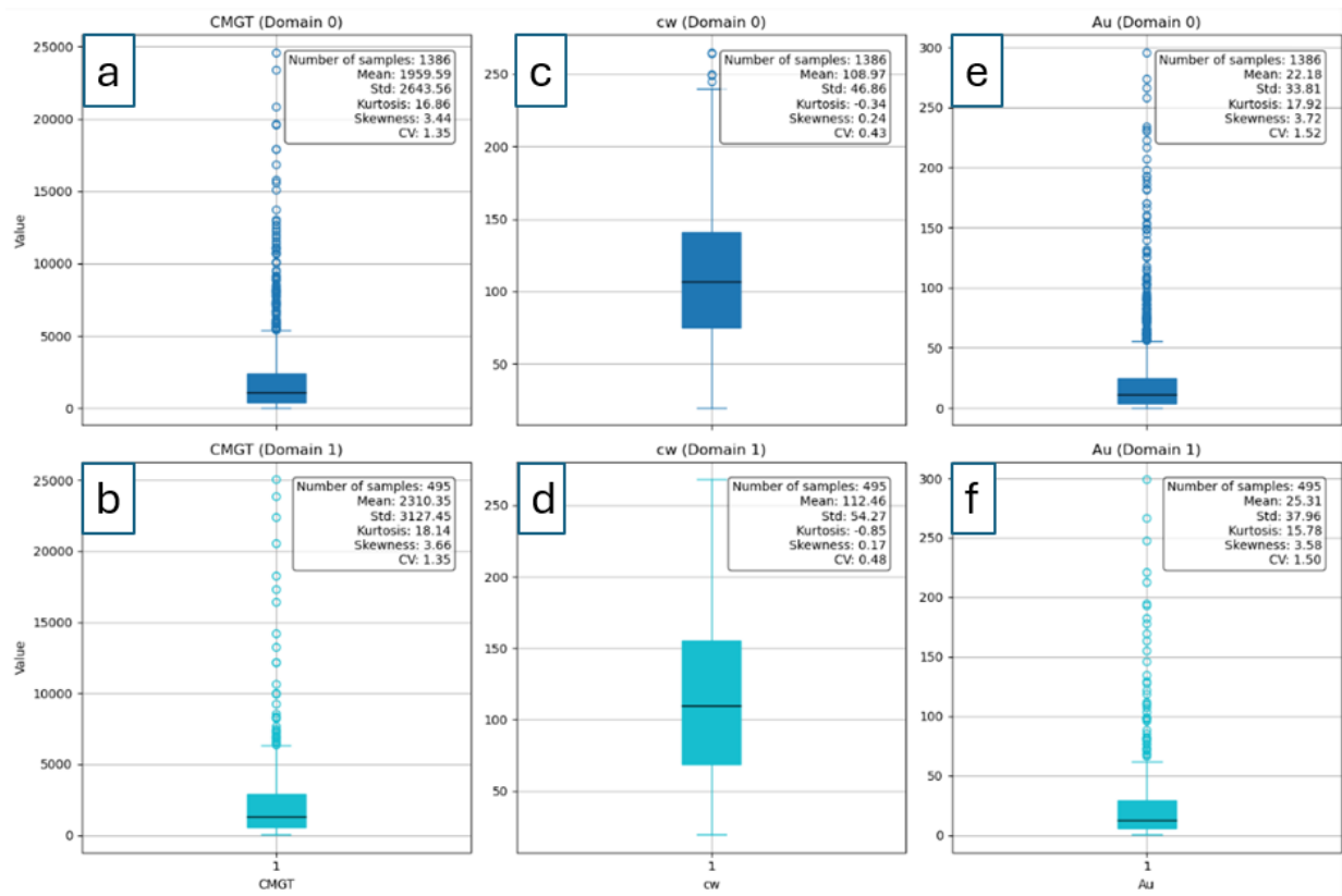
Figure 4.13: Outlier treated data represented as Whisker plots and summary statistics a) Au (cm.g/t) Domain 0 b) Au (cm.g/t) Domain 1 c) CW (cm) Domain 0 d) CW (cm) Domain 1 e) Au (g/t) Domain 0 f) Au (g/t) Domain 1.
