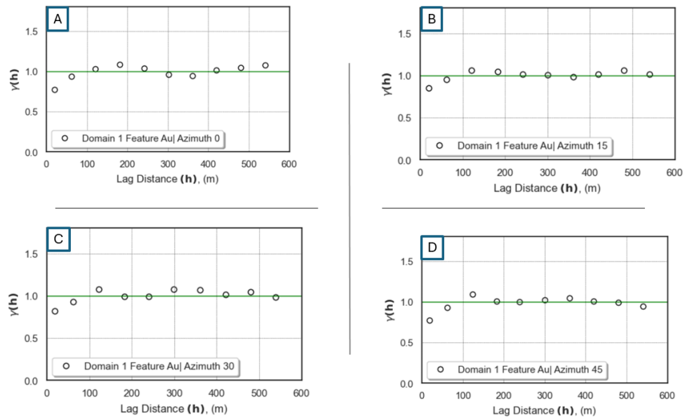
Figure B5: Experimental variograms a) Domain 1 Au (g/t) azimuth 0 b) Domain 1 Au (g/t) azimuth 15 c) Domain 1 Au (g/t) azimuth 30 d) Domain 1 Au (g/t) azimuth 45.
