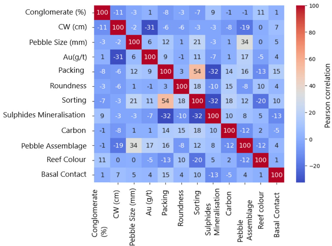
Figure 4.2: Feature correlation heat map showing the feature correlation from the primary dataset.
