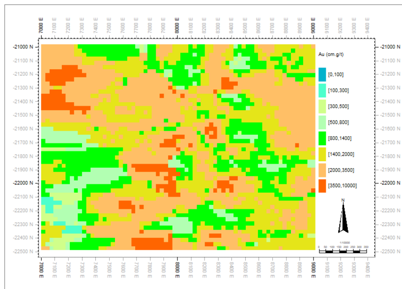
Figure 4.46: 2D map showing the spatial distribution of Au (cm.g/t) Kriging results.
