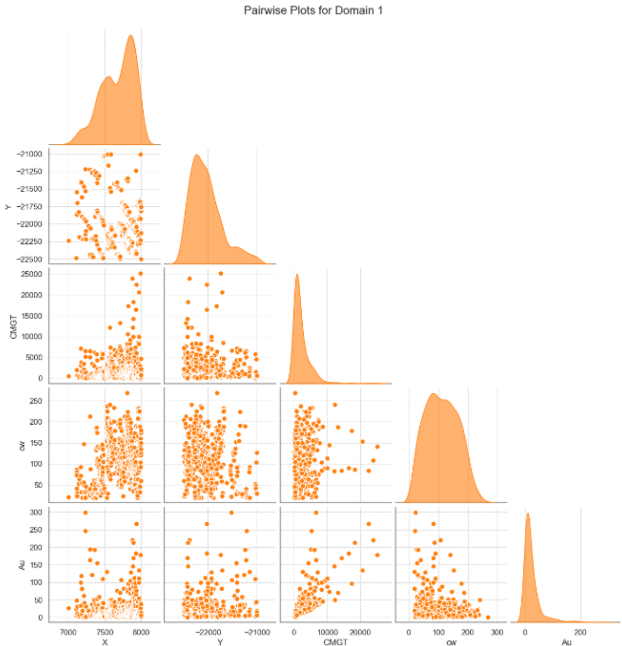
Figure 4.16: Pairwise plots for all the selected variables of interest in Domain 1.
