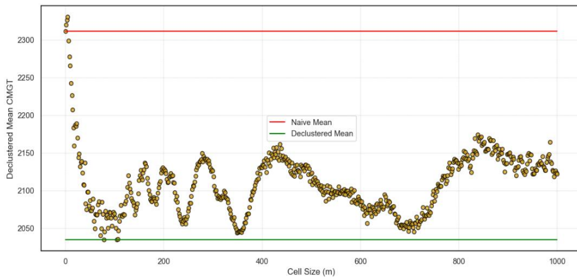
Figure 4.22: Cell size selection for Domain 0 Au (cm.g/t) showing the minimum and maximum naïve and declustered mean corresponding to a cell size.
