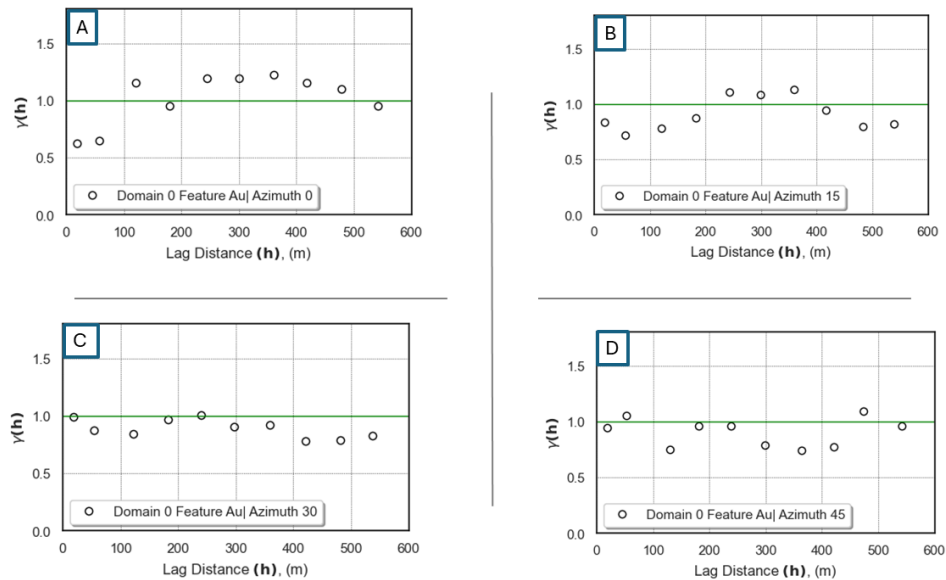
Figure B2: Experimental variograms a) Domain 0 Au (g/t) Azimuth 0 b) Domain 0 Au (g/t) Azimuth 15 c) Domain 0 Au (g/t) Azimuth 30 d) Domain 0 Au (g/t) Azimuth 45.
