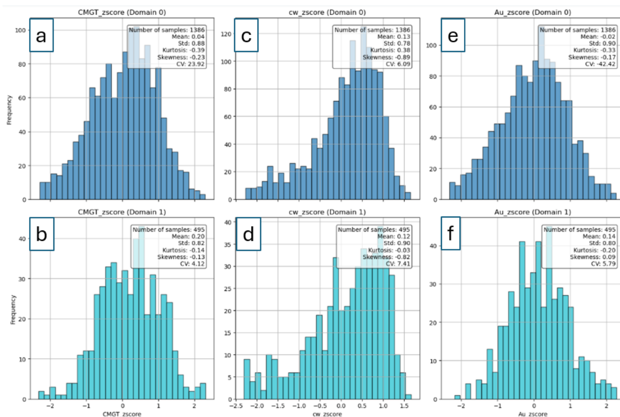
Figure 4.12: Feature Z-score histograms and the summary statistics per domain a) Au (cm.g/t) Z-score (Domain 0) b) Au (cm.g/t) Z-score (Domain 1) c) CW (cm) Z-score (Domain 0) d) CW (cm) Z-score (Domain 1) e) Au (g/t) Z-score (Domain 0) f) Au (g/t) Z-score (Domain 1).
