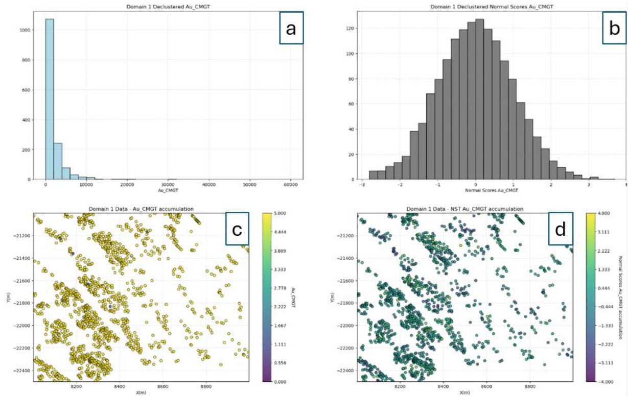
Figure 4.33: Domain 1 declustered Au (cm.g/t) b) Domain 1 declustered normal score Au (cm.g/t) c) Domain 1 declustered Au (cm.g/t) spatial distribution d) Domain 1 normal score Au (cm.g/t) spatial distribution.
