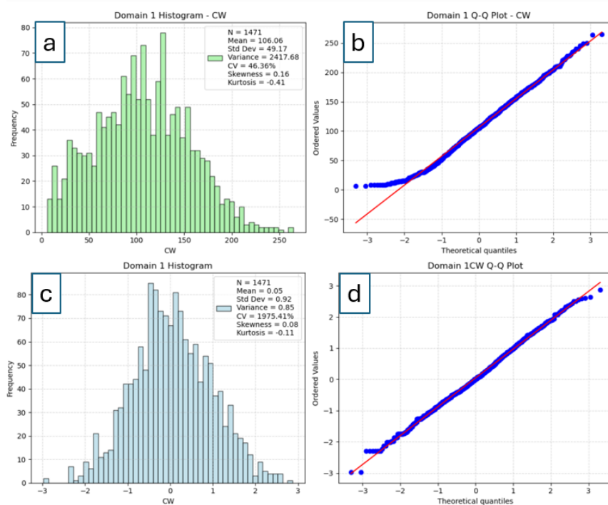
Figure 4.39: Domain 1 CW (cm) histogram b) Domain 1 Q-Q CW (cm) plot c) Domain 1 CW (cm) treated data histogram d) Domain 1 CW (cm) treated data Q-Q plot.
