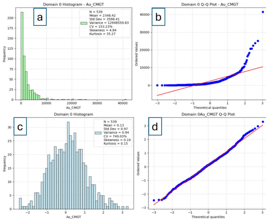
Figure 4.34: a) Domain 0 Au (cm.g/t) histogram b) Domain 0 Q-Q Au (cm.g/t) plot c) Au (cm.g/t) treated data histogram d) Au (cm.g/t) treated data Q-Q plot.
