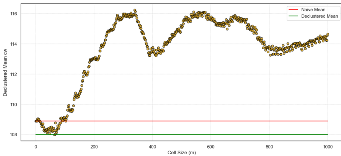
Figure 4.25: Cell size selection for Domain 1 CW (cm) showing the minimum and maximum naïve and declustered mean corresponding to a cell size.
