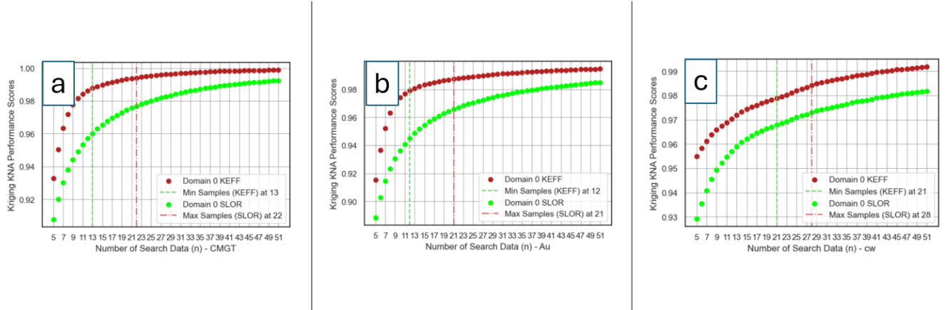
Figure 4.44: Quantitative Kriging neighbourhood a) Domain 0 Au (cm.g/t) minimum and maximum number of samples b) Domain 0 Au (g/t) minimum and maximum number of samples c) Domain 0 CW (cm) minimum and maximum number of samples.
