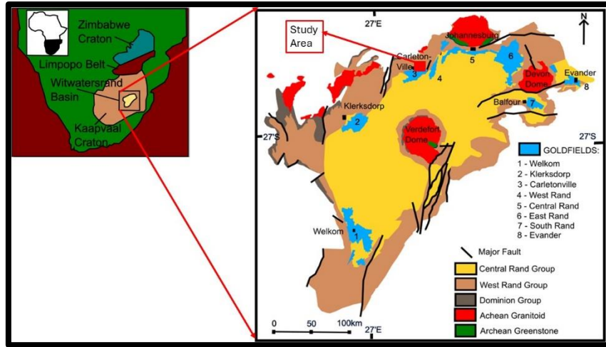
Figure 1.1: Location of the study area in Southern African(left) and a simplified geological map of the Witwatersrand Basin and associated goldfields (right). The red polygon corresponds to the location of the study area. Note the younger sequences covering the Witwatersrand Basin have been removed, figure modified from Frimmel & Nwaila, (2020) .
