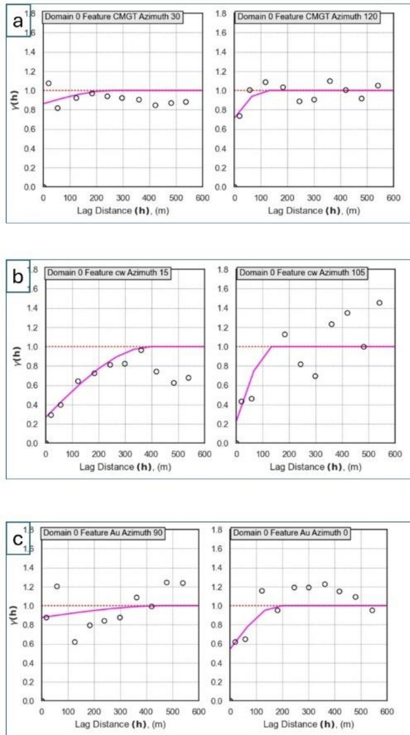
Figure 4.40: Fitted Variogram Model Domain 0 a) Domain 0 Au (cm.g/t) major angle 30 and minor angle 120 b) Domain 0 CW (cm) major angle 15 and minor angle 105 C) Domain 0 Au (g/t) major angle 90 and minor angle 0.
