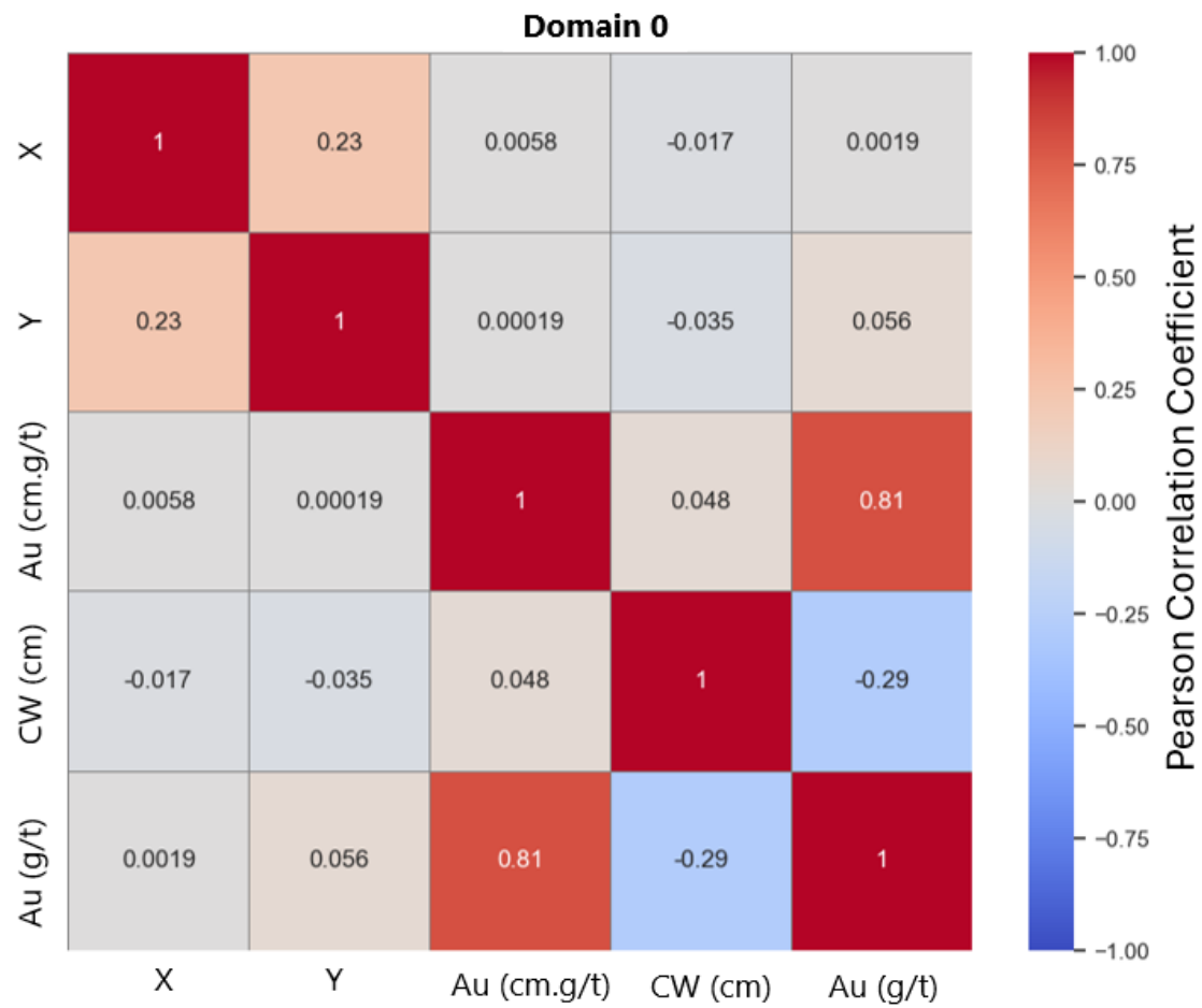
Figure 4.15: Pearsons's correlation heatmap of selected variables of interest Au (cm.g/t), Au (g/t) and CW (cm) and their spatial locations (Domain 0).
