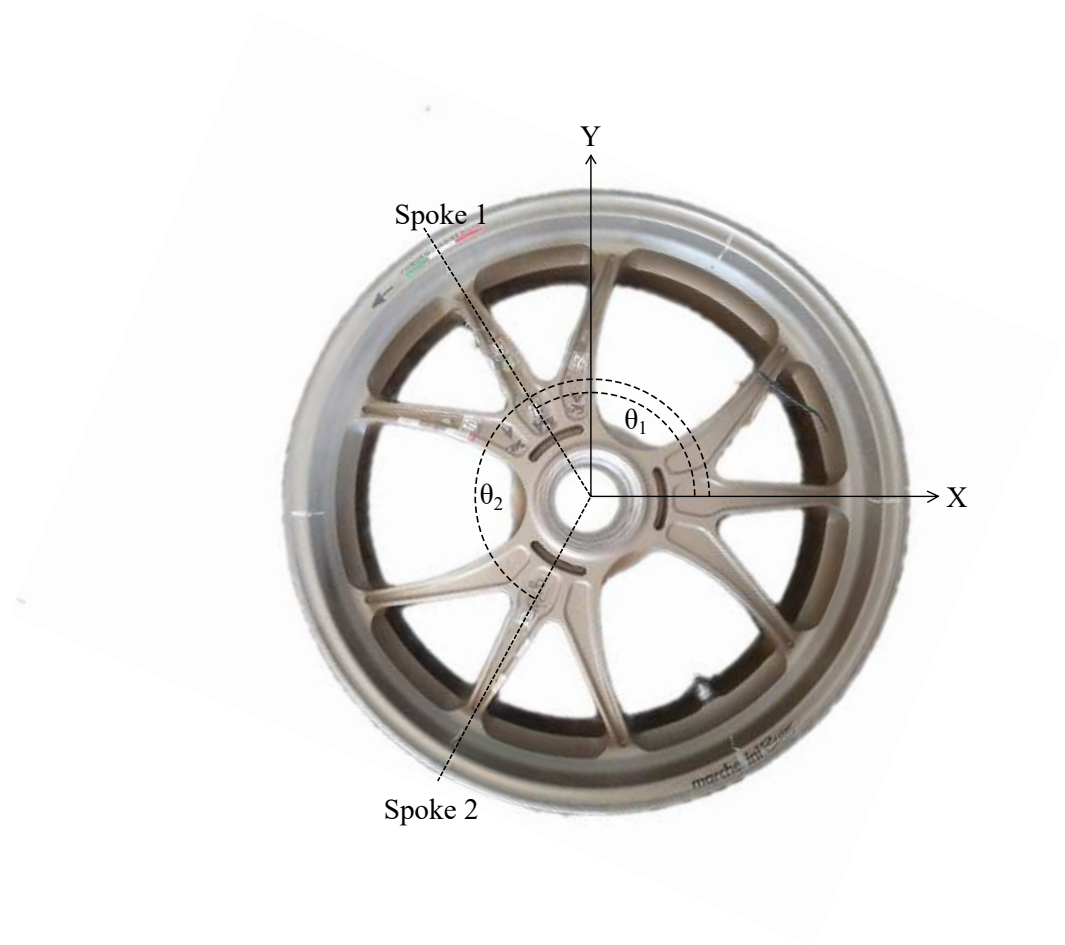
Figure 4.3: Relative orientations of primary and secondary spokes of 9 spoke ORW
