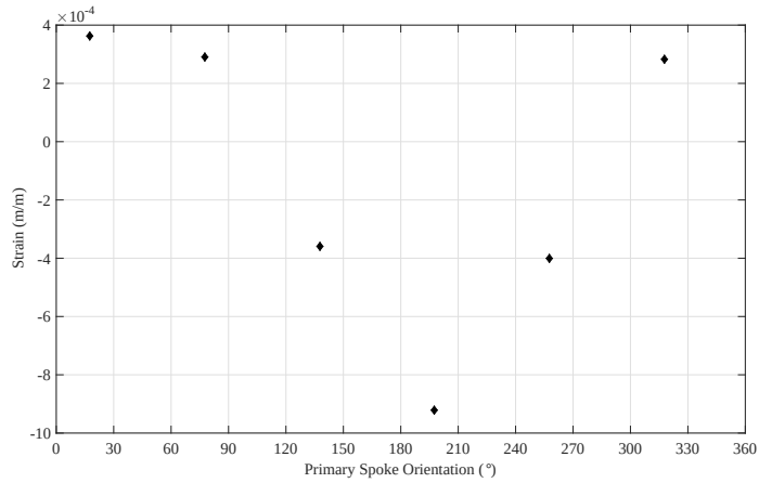
(c) 7 Spoke FW under bending load of 1\,100 \text{ N} \cdot \text{m} at x = 102 \text{ mm}
