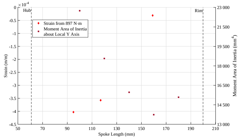
(a) 9 Spoke ORW under bending load of 897 \text{ N} \cdot \text{m} at \theta = 120^\circ
