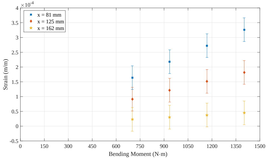
Figure 4.1: Strain versus load for 5 Spoke CRW under bending load case with \theta = 45^\circ
