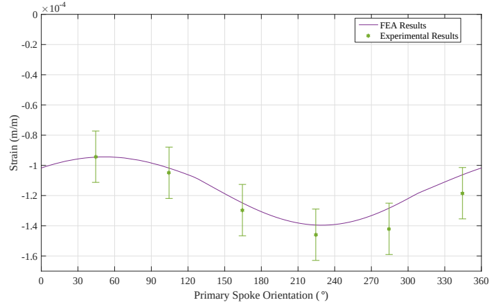
(b) 5 Spoke CRW under torsional load of 736 \text{ N} \cdot \text{m} at x = 123 \text{ mm}
