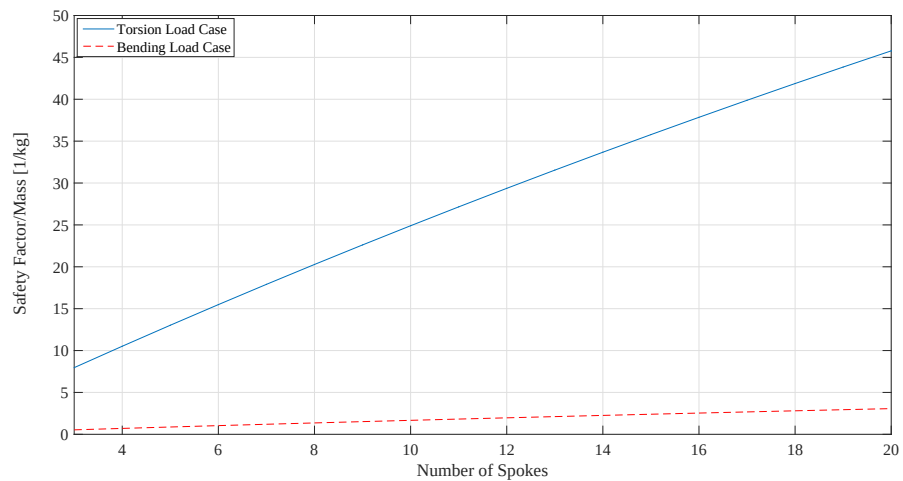
(b) Number of spokes versus ASME factor of safety normalised with the mass of the wheel
