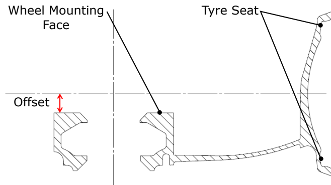
Figure 3.2: Offset direction of motorcycle wheel
