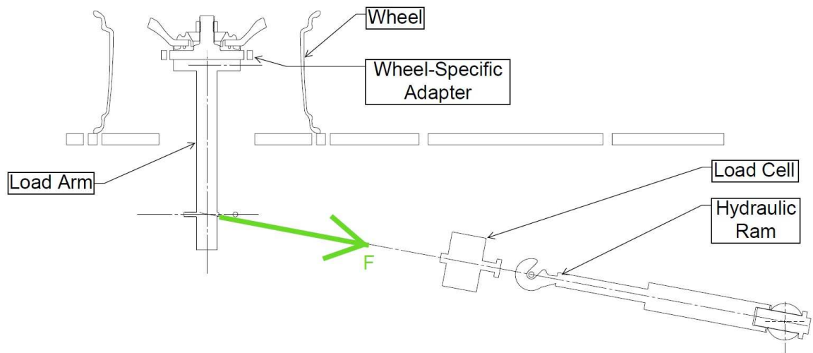
Figure 3.5: Bending stiffness test rig
