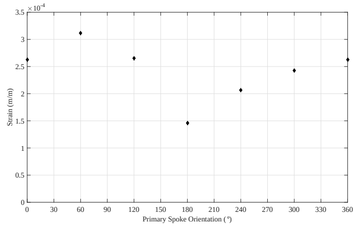
(c) 7 Spoke FW under torsional load of 515 \text{ N} \cdot \text{m} at x = 100 \text{ mm}
