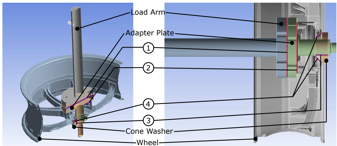
Figure 5.4: Full test rig simulation with connections
