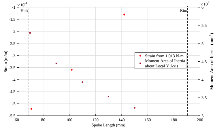
(c) 7 Spoke FW under bending load of 1\,037 \text{ N} \cdot \text{m} at \theta = 138^\circ
