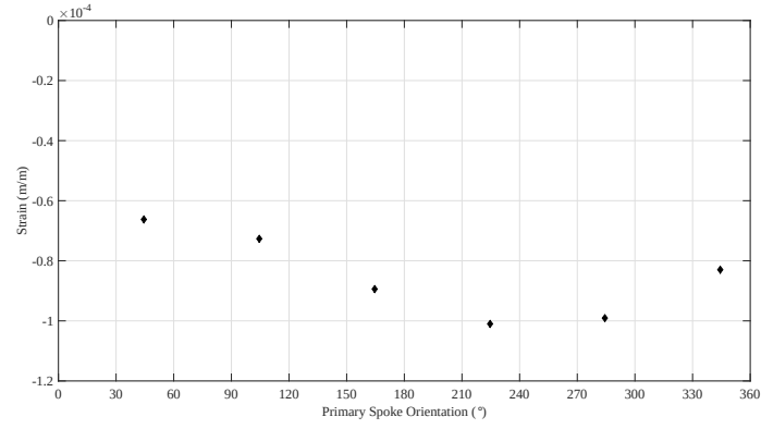
(b) 5 Spoke CRW under torsional load of 515 \text{ N} \cdot \text{m} at x = 123 \text{ mm}
