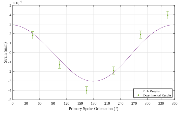
(b) 5 Spoke CRW under bending load of 1\,402\text{ N} \cdot \text{m} at x = 125\text{ mm}
