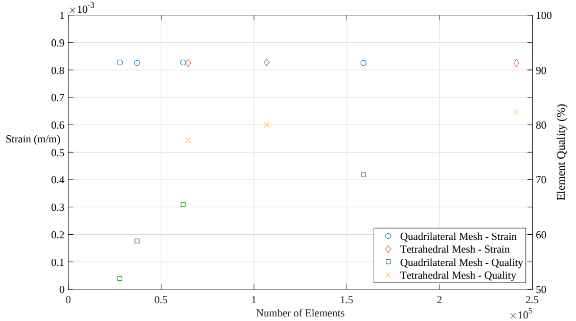
Figure 5.2: Strain and element quality versus number of elements
