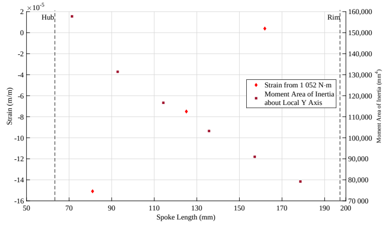
(b) 5 Spoke CRW under bending load of 1\,052 \text{ N} \cdot \text{m} at \theta = 105^\circ
