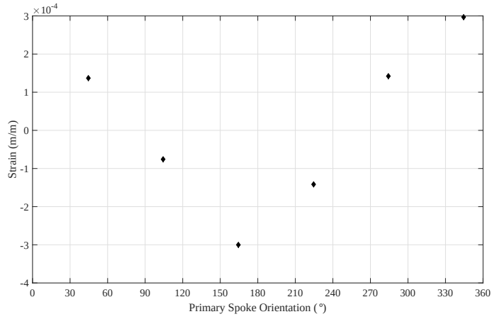
(b) 5 Spoke CRW under bending load of 1\,052 \text{ N} \cdot \text{m} at x = 125 \text{ mm}
