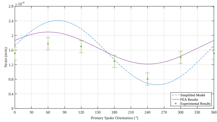
(c) 7 Spoke FW under torsional load of 736 \text{ N} \cdot \text{m} at x = 100 \text{ mm}
