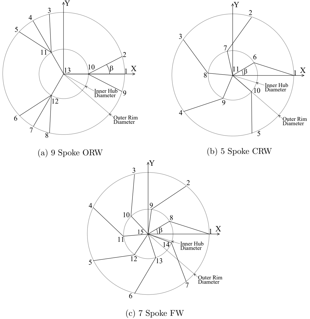
Figure 7.1: Diagram of elements and nodes of simplified model with \theta = 0^\circ
