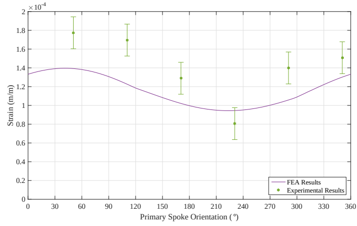
(a) 9 Spoke ORW under torsional load of 736 \text{ N} \cdot \text{m} at x = 80 \text{ mm}
