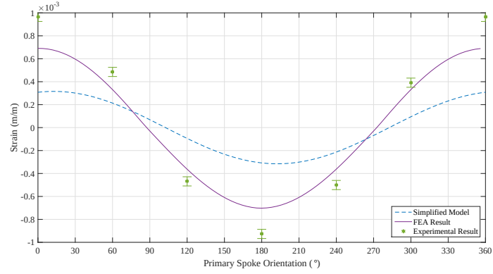
(a) 9 Spoke ORW under bending load of 1\,195\text{ N} \cdot \text{m} at x = 117\text{ mm}
