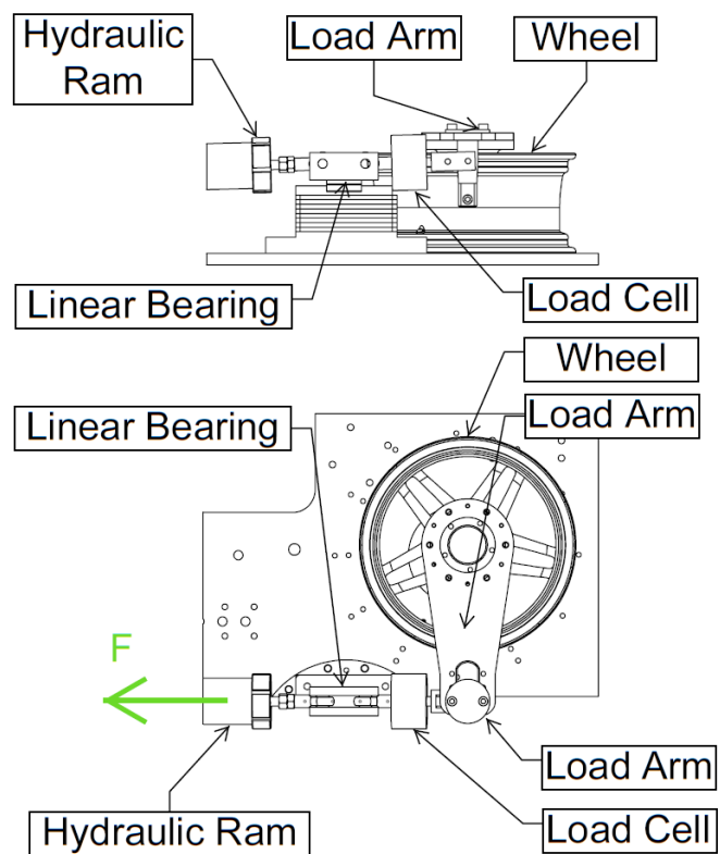
Figure 3.6: Torsional stiffness test rig
