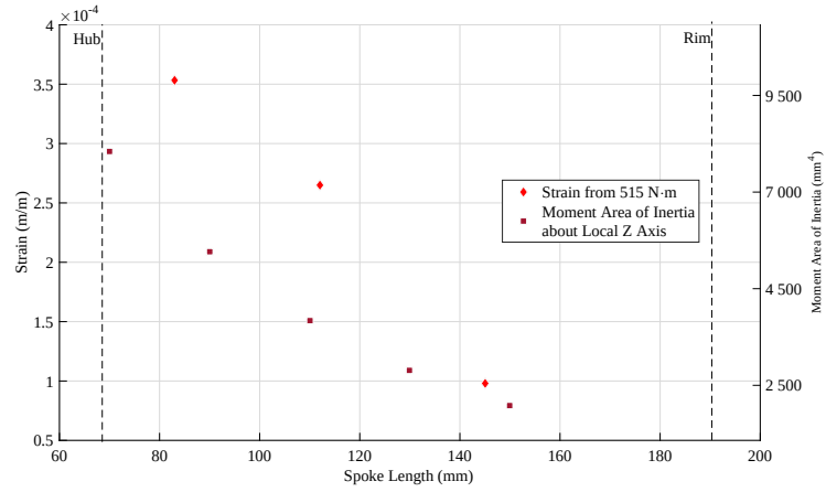
(c) 7 Spoke FW under torsional load of 515 \text{ N} \cdot \text{m} at \theta = 180^\circ
