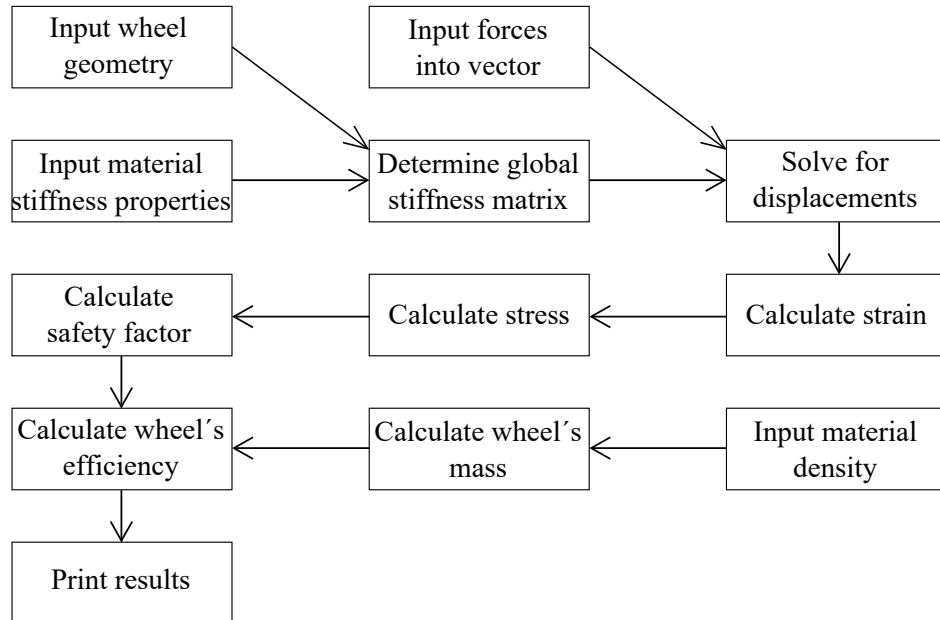
Figure 6.1: Simplified model data flow
