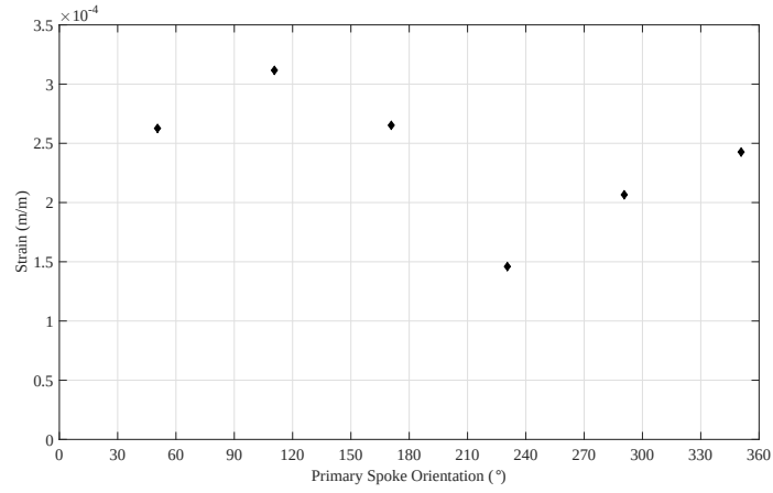
(a) 9 Spoke ORW under torsional load of 515 \text{ N} \cdot \text{m} at x = 80 \text{ mm}
