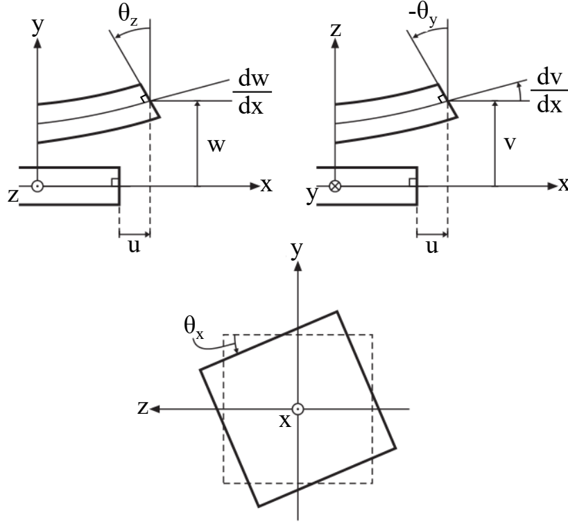
Figure 6.4: Kinematic constraints for a Euler-Bernoulli beam
