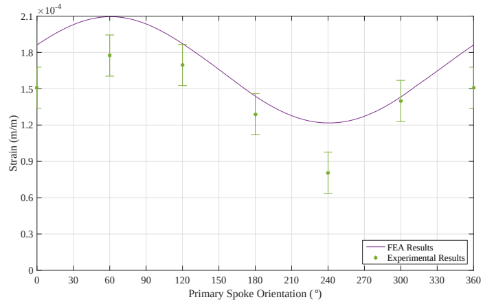
(c) 7 Spoke FW under torsional load of 736 \text{ N} \cdot \text{m} at x = 100 \text{ mm}
