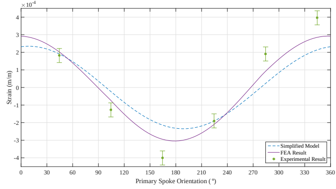
(b) 5 Spoke CRW under bending load of 1\,340\text{ N} \cdot \text{m} at x = 125\text{ mm}
