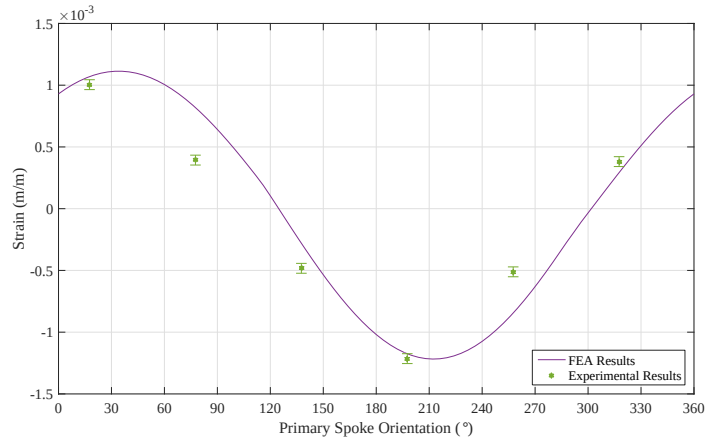
(c) 7 Spoke FW under bending load of 1\,340\text{ N} \cdot \text{m} at x = 102\text{ mm}
