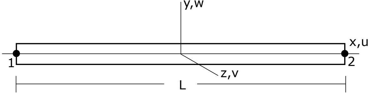
Figure 6.3: 3D Euler-Bernoulli beam element
