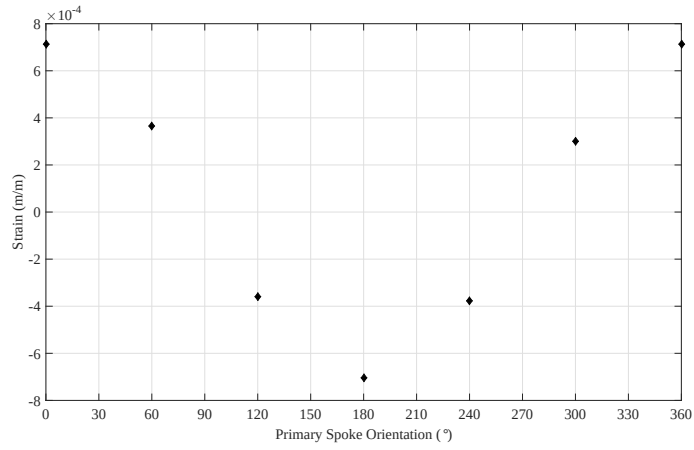
(a) 9 Spoke ORW under bending load of 897 \text{ N} \cdot \text{m} at x = 117 \text{ mm}
