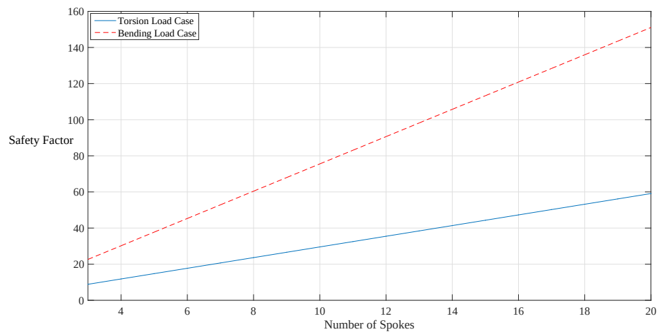
(a) Number of spokes versus ASME factor of safety
