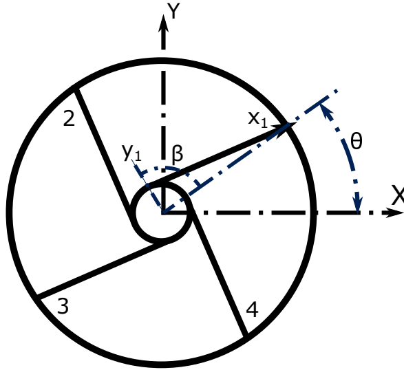
Figure 6.2: Simplified model coordinate system
