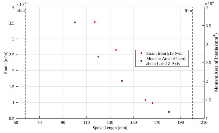
(a) 9 Spoke ORW under torsional load of 515 \text{ N} \cdot \text{m} at \theta = 171^\circ
