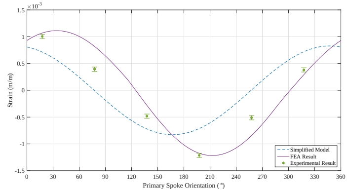
(c) 7 Spoke FW under bending load of 1\,402\text{ N} \cdot \text{m} at x = 102\text{ mm}
