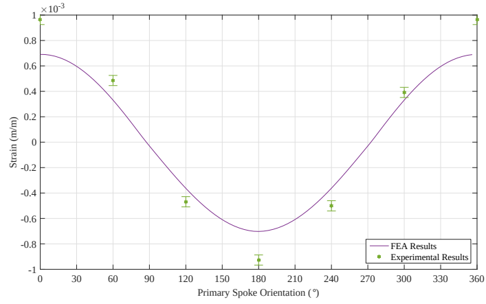
(a) 9 Spoke ORW under bending load of 1\,195\text{ N} \cdot \text{m} at x = 117\text{ mm}
