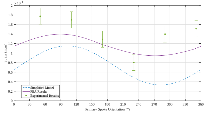
(a) 9 Spoke ORW under torsional load of 736 \text{ N} \cdot \text{m} at x = 80 \text{ mm}
