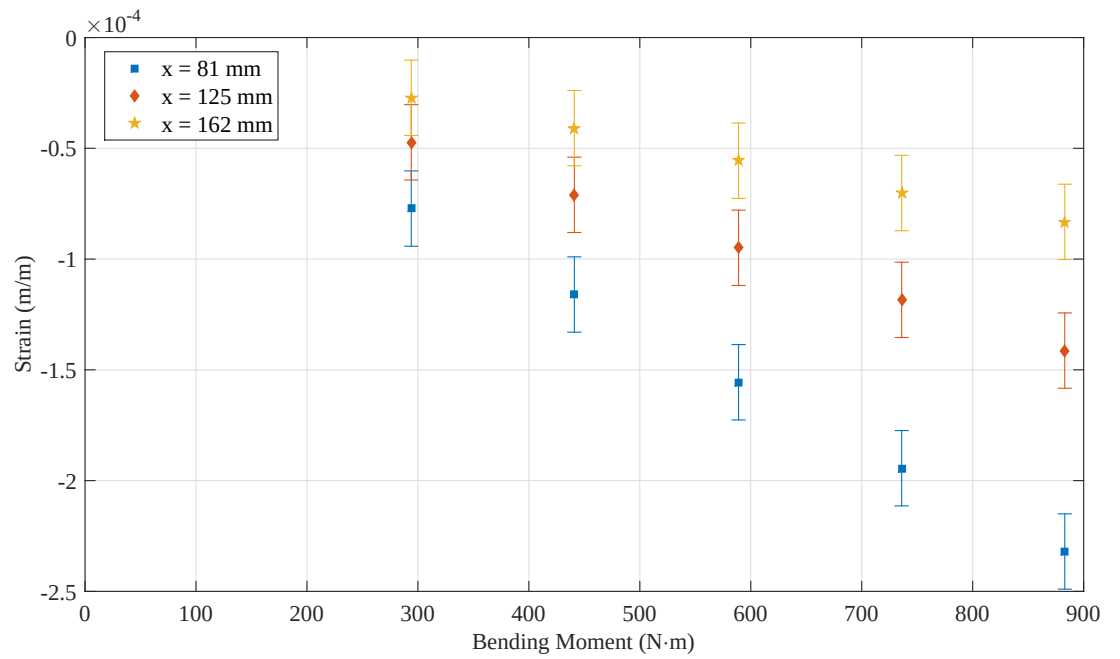
Figure 4.2: Strain versus load for 5 Spoke CRW under torsional load case with \theta = 60^\circ
