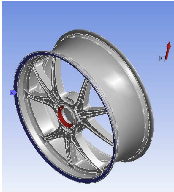
Figure 5.3: Simplified boundary conditions
