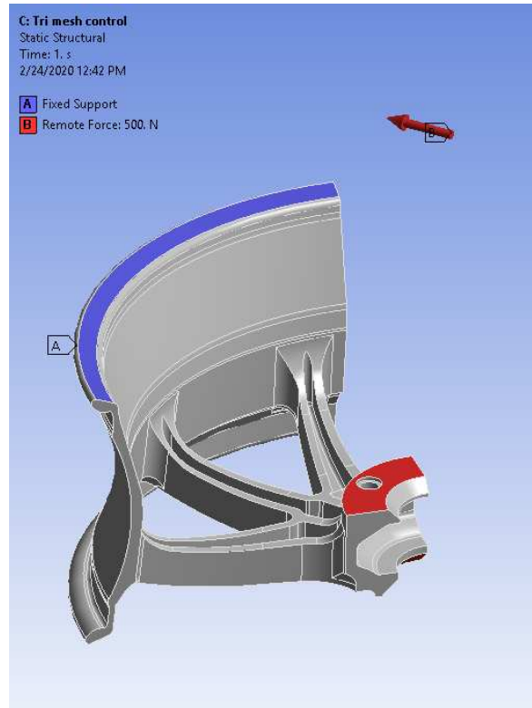
Figure 5.1: Geometry used in mesh independence study
