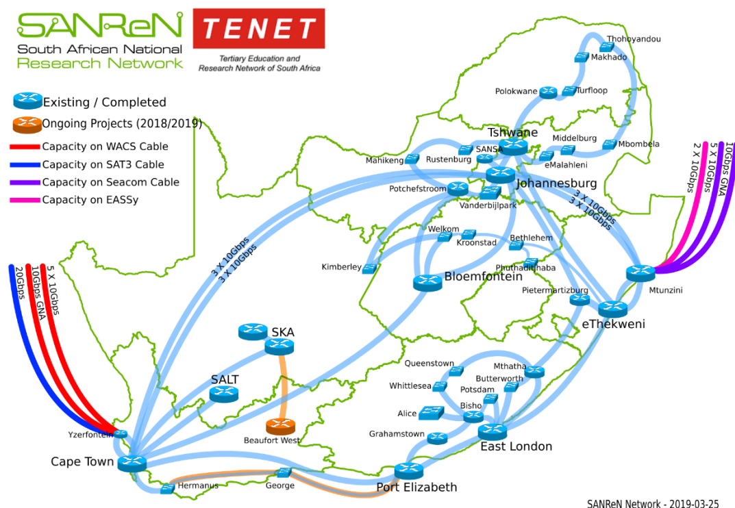
Figure 4.2. SA NREN Backbone Map indicating International Capacity
