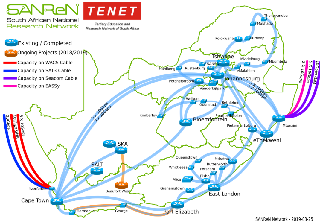
Figure 1.6. SA NREN Backbone Map indicating International Capacity (Source: SANReN (2019))
