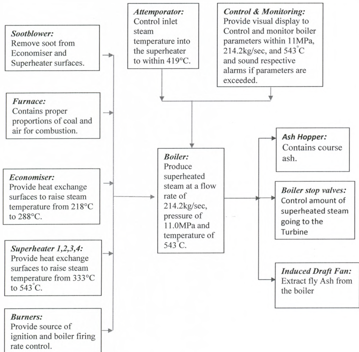
Figure 4-4 Boiler System Functional Block diagram.
