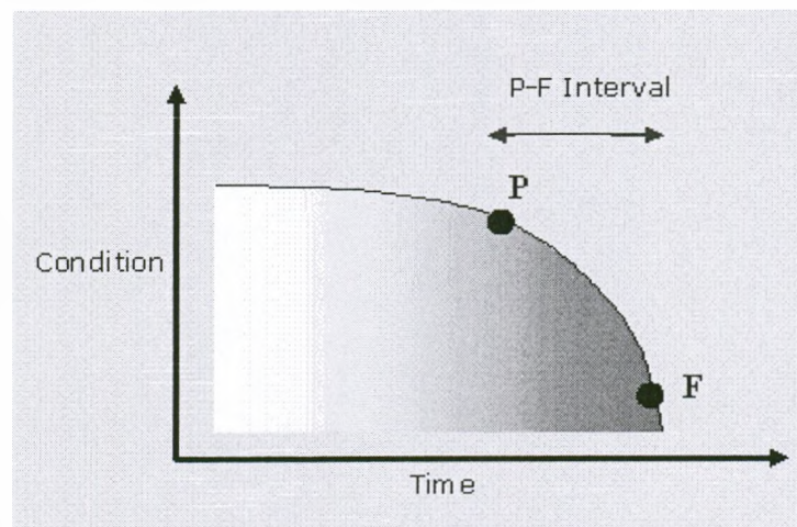
Figure 4-10 P-F curve.
