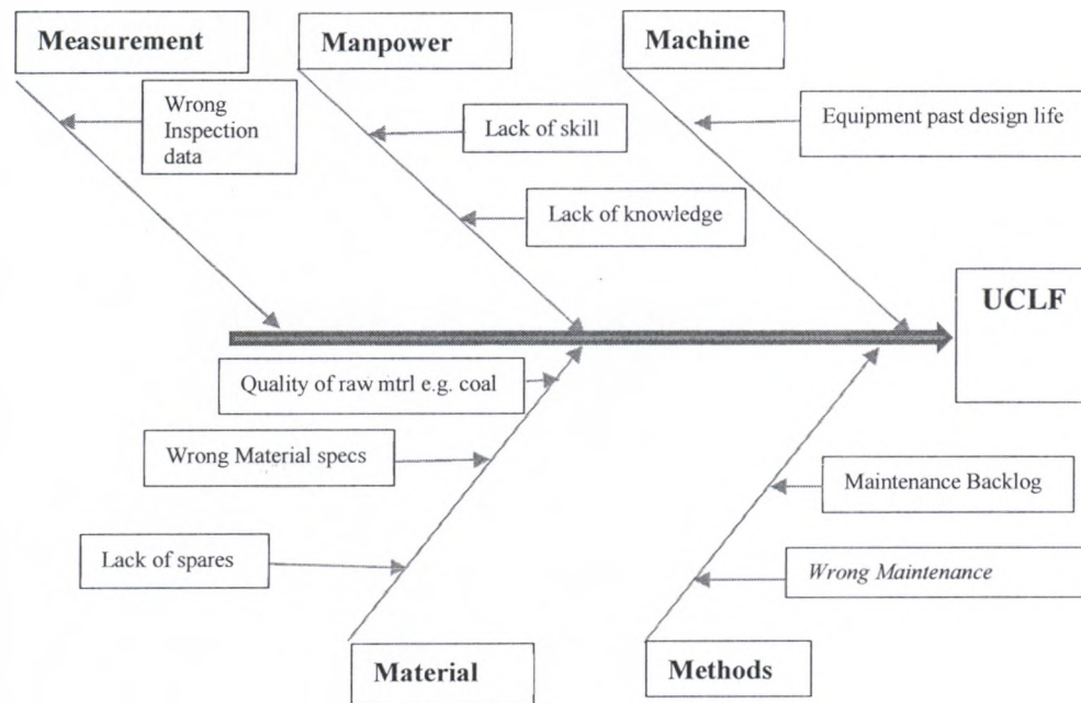
Figure 1-3 UCLF Fish bone diagram.
