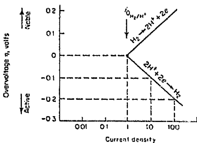
Figure 2.27: Overvoltage versus current density. 1
