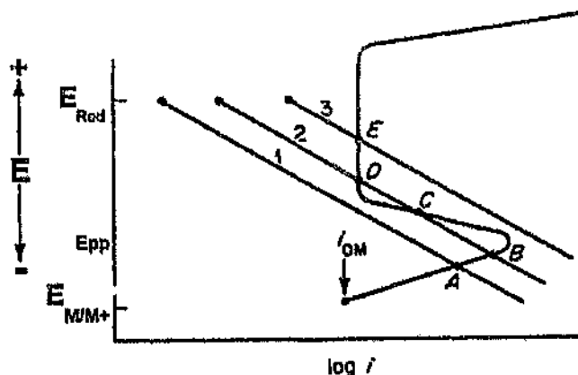
Figure 2.33: Requirements for cathodic modification 1
