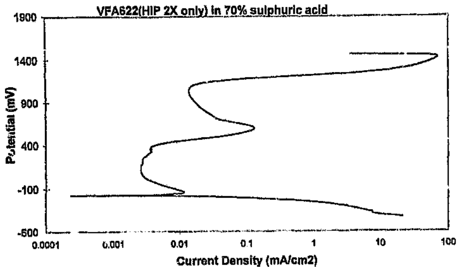
Figure 4.87: Corrosion scan for VFA622, HIPped twice. A distinct anodic loop is present with two minima in the passive region.
