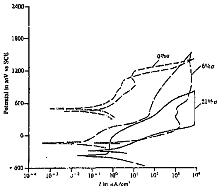
Figure 2.47: Anodic pitting polarisation curves of duplex alloy SAF2205 with various sigma phase contents exposed to 3.5% NaCl solution at 25°C. 53
