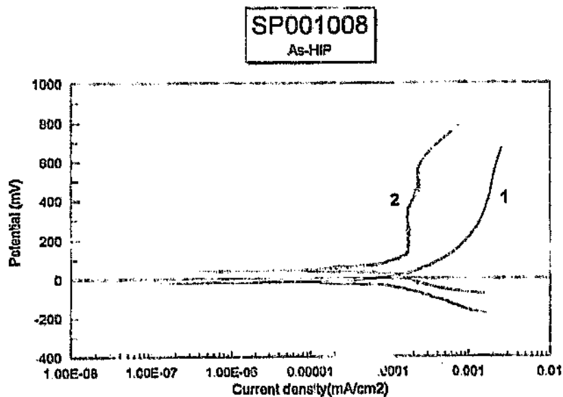
Figure 4.77: Corrosion scan for SP001008, as-HIPped. Spontaneous passivation in the test medium. The first scan in Figure 4.78 is inconsistent, and should be ignored.
