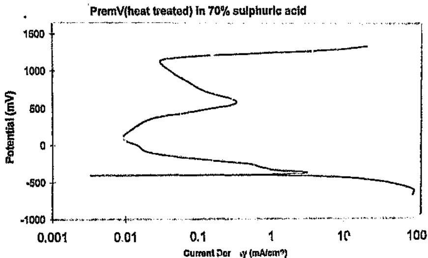
Figure 4.85: Corrosion scan for PremV, heat treated.
