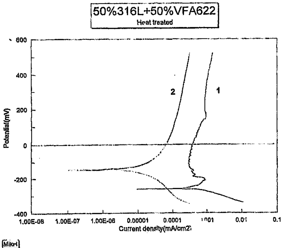
Figure 4.82: Corrosion scan for 50% 316L + 50% VFA622, heat treated. A small active loop followed by passivation at increasing potential was observed in the first scan. In the second scan, the material passivated spontaneously. A large difference in the E_{\text{corr}} values of the two scans was observed.
