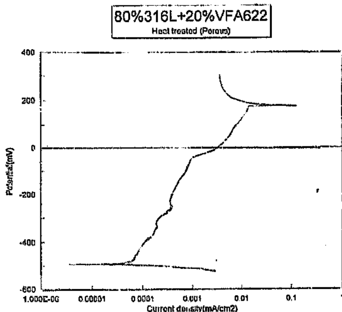
Figure 4.83: Corrosion scan for 80% 316L+20% VFA622, heat treated.
