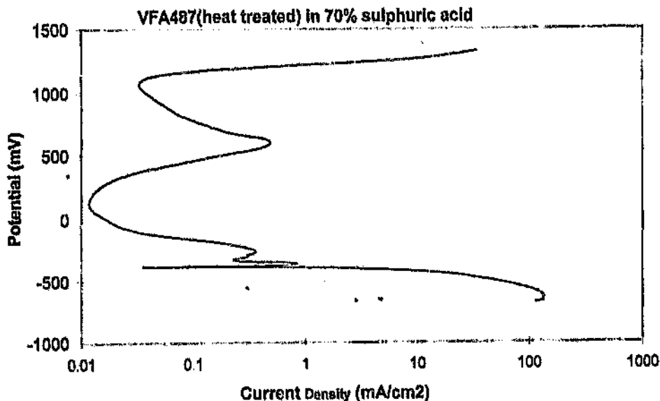
Figure 4.86: Corrosion scan for VFA487, heat treated.
