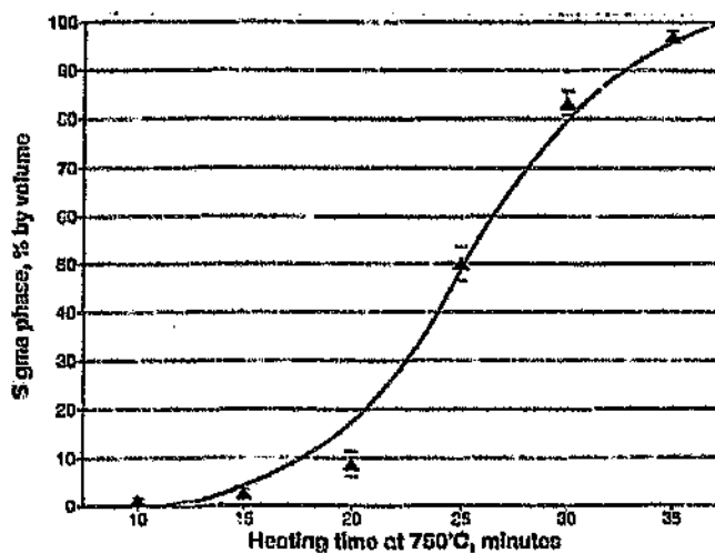
Figure 2.9: The rate of sigma phase formation in a 6Ni-40Cr-Fe as-cast alloy at 750°C. 21
