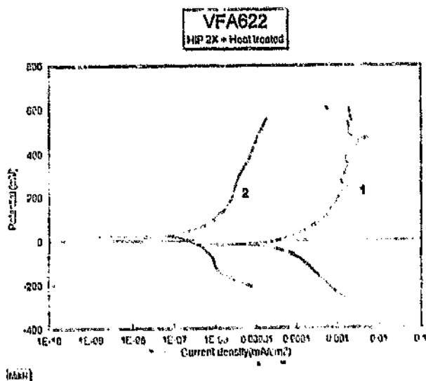
Figure 4.76: Corrosion scan for VFA622, HIPped(twice)+ heat treated. Spontaneous passivation in the test media.
