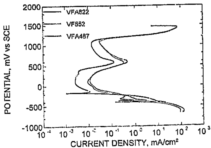
Figure 12. Potentiodynamic behaviour of three alloys in 70% H 2 SO 4 at 50°C. The alloy with ruthenium (VFA622) shows considerably greater resistance to corrosion.
