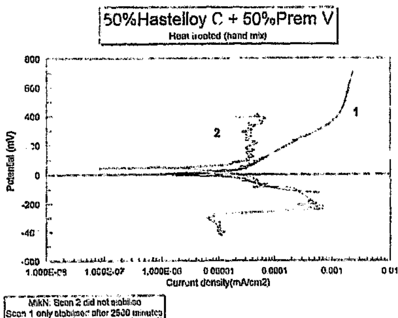
Figure 4.84: Corrosion scan for 50% Hastelloy C + 50% Prem V, heat treated.
