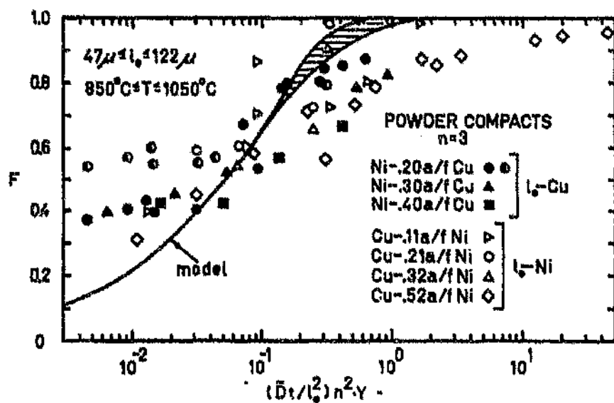
Figure 2.56: Comparison of data from two alloy systems (Ni-Cu) and (Cu-Ni) with model predictions. 64
