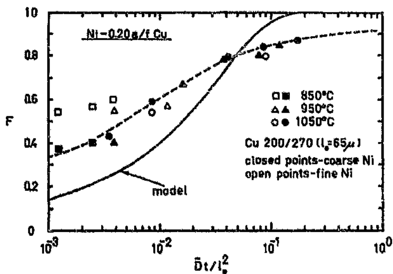
Figure 2.55: Comparison of experimental F data on Ni-0.20Cu compacts with model predictions. 64
