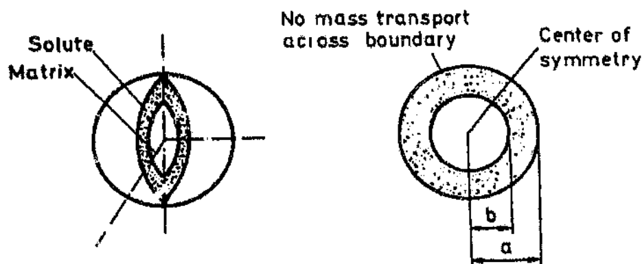
Figure 2.57: Larsson's model of homogenisation. 66
