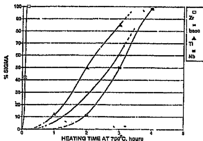
Figure 2.13 The rate of sigma formation at 750°C in the as-cast alloys containing 2%Mo and 2%Ni, with different stabilisers. 21
