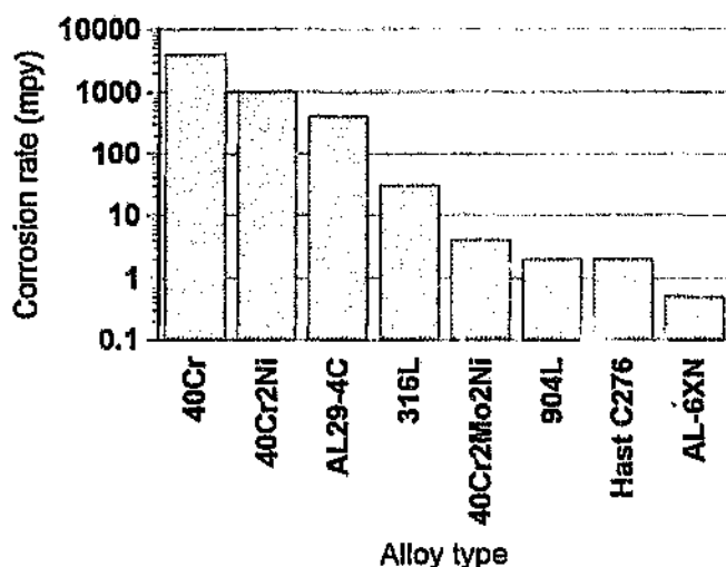
Figure 2.37: General corrosion rates of Fe-40Cr alloys and commercial stainless steels in 10% H 2 SO 4 at 30°C. 3
