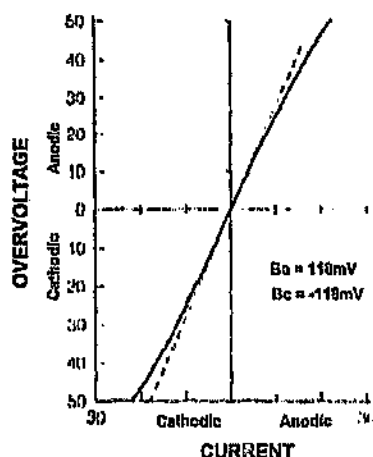
Figure 2.34: Linear region in cathodic and anodic polarisation curves. 17
