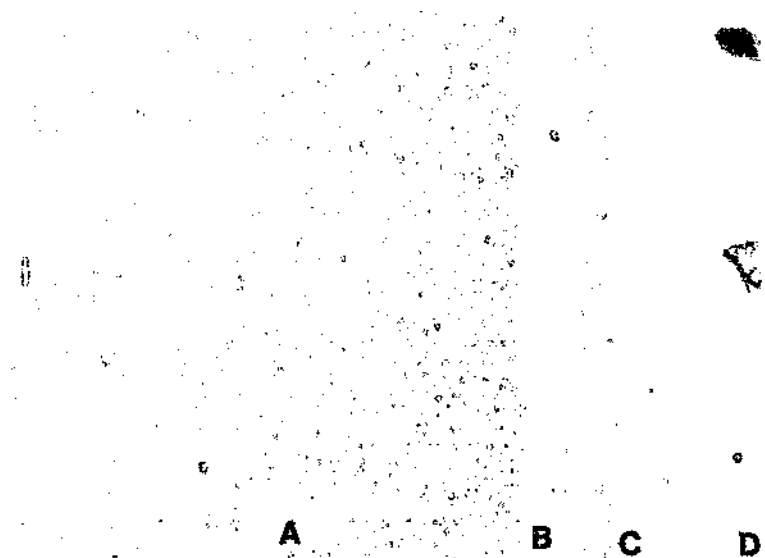
Figure 4.40: Extra-milled VFA543 (SP001012), (As-HIPped), Murakami etch, (200X), optical image.
