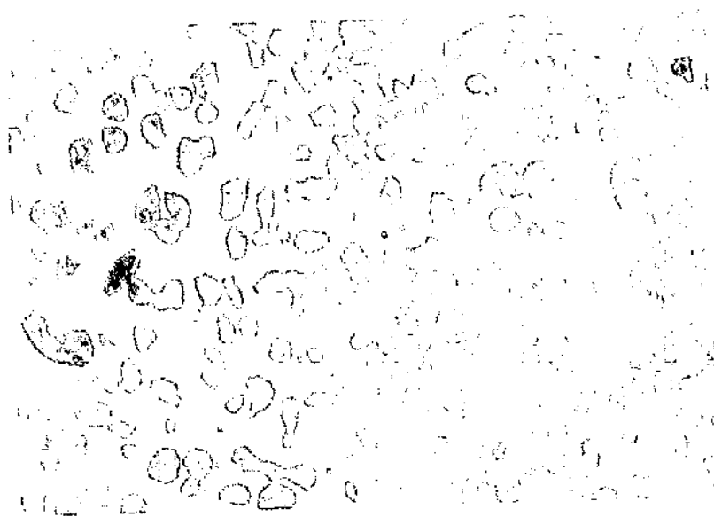
Figure 4.54: (80% 316L+20% VFA622), As-HIP (25X), HCl etch , optical image. Well distributed ferrite (dark) particles within an austenite (316L) matrix.
