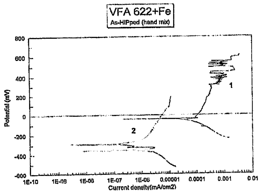
Figure 4.79: Corrosion scan for VFA622 + Fe, as-HIPped. Spontaneous passivation with unusual behaviour in the first scan of Figure 4.79.
