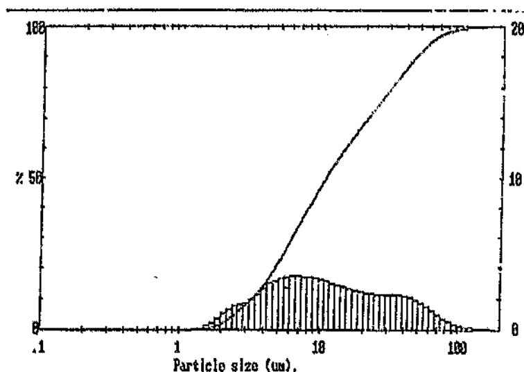
Figure 4.6: Particle size distribution of Fe powder.
