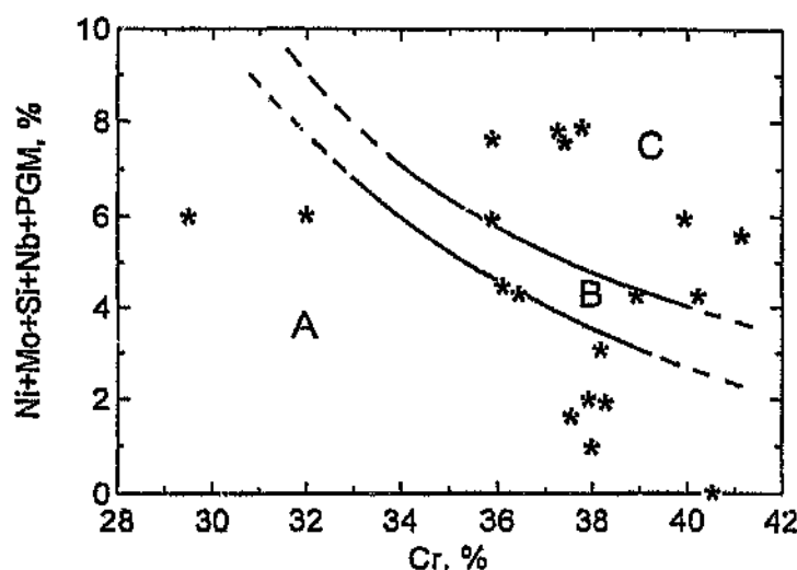
Figure 5.4: Diagram illustrating the effect of composition on the properties of the alloys. A - takes too long to convert to powder, B - Comes out of HIP as ferrite, C - comes out of HIP as sigma phase. 78
