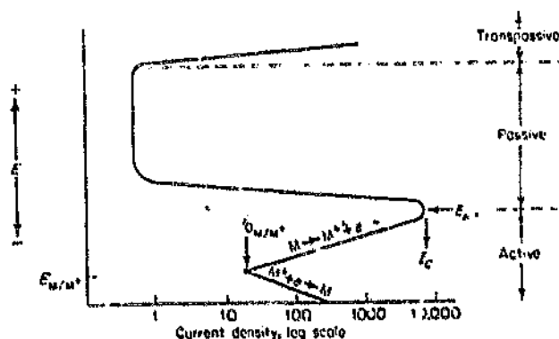
Figure 2.30: Typical anodic dissolution behaviour of an active-passive metal. 1
