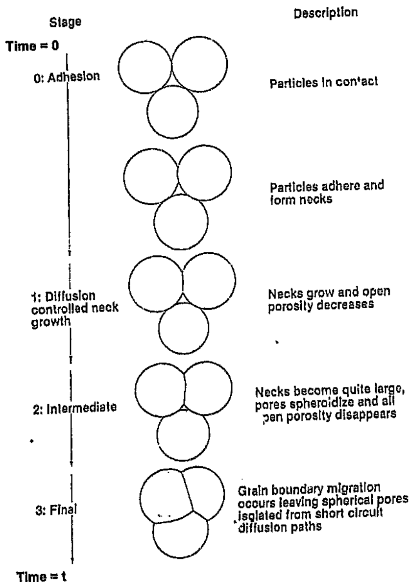
Figure 5.3: Plastic deformation of spherical powders particles during HIPping. 34
