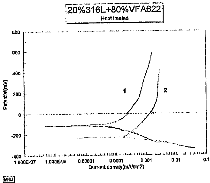
Figure 4.81: Corrosion scan for 20% 316L+80% VFA622, heat treated. Spontaneous passivation with a large variation in E_{corr} .
