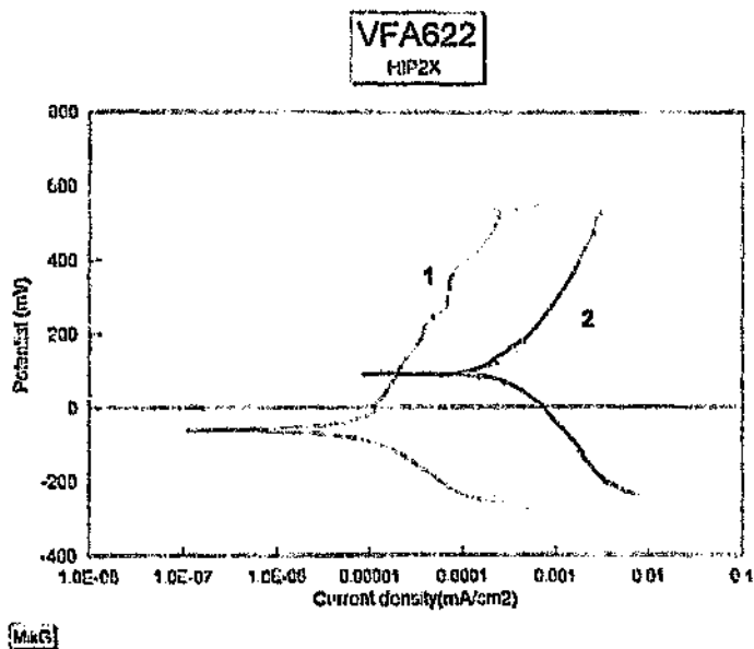
Figure 4.75: Corrosion scan for VFA622, HIPped(2X). Spontaneous passivation occurred in both scans.
