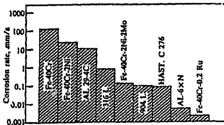
Figure 2.5: Corrosion rate (mm per annum) of several alloys in 10% H_2SO_4 at 30°C. 25
