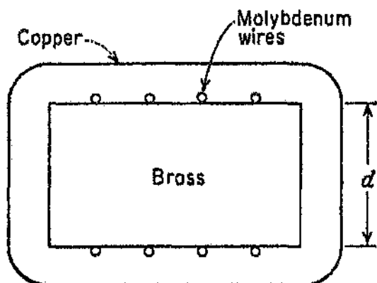
Figure 2.49: Diffusion couple used by Kirkendall. 58
