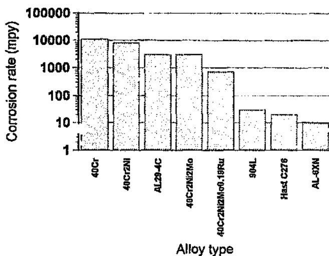
Figure 2.38: General corrosion rates of Fe- 40Cr alloys and commercial stainless steels in 10% H_2SO_4 +100ppm KSCN at 40°C. 3
