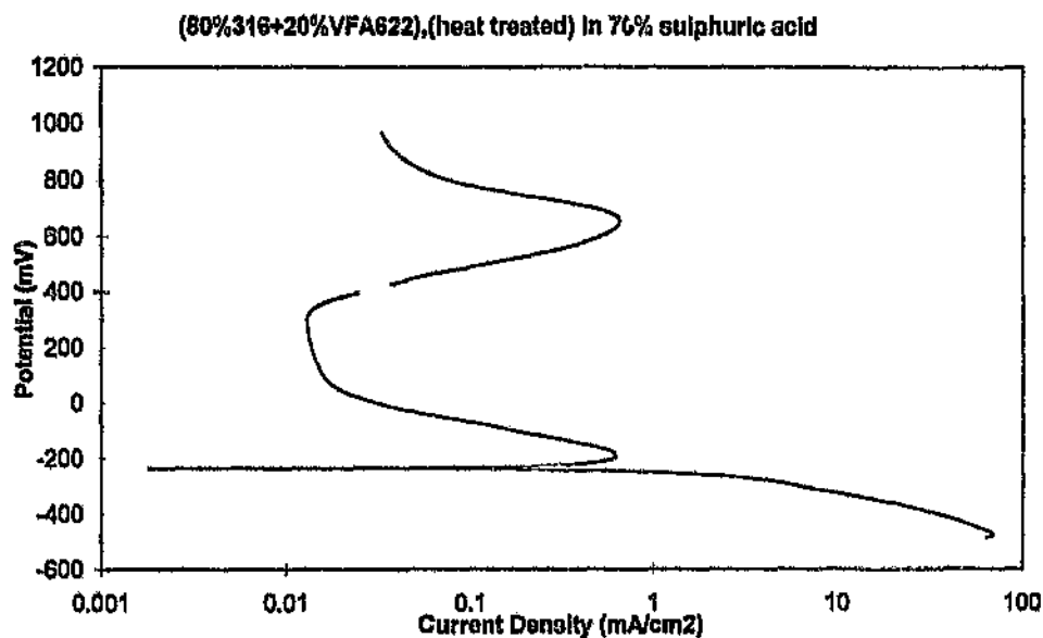
Figure 4.91: Corrosion scan for 80% 316 + 20% VFA622 (Heat-treated).
