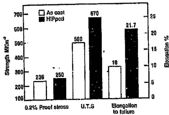
Figure 2.22: Illustrative comparison of material properties: as-cast and cast+HIPped. 34
