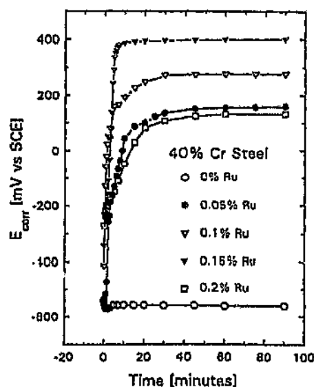
Figure 2.43: Open circuit corrosion potential variations with time of Fe-40%Cr-Ru alloys in 10% H 2 SO 4 at 25°C. 51
