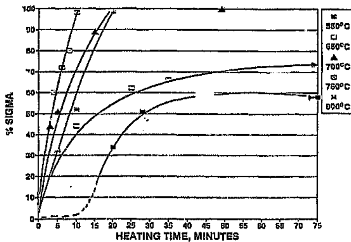
Figure 2.10: The rate of sigma phase formation in hot rolled 4Mo-39Cr-Fe at various temperatures. 21
