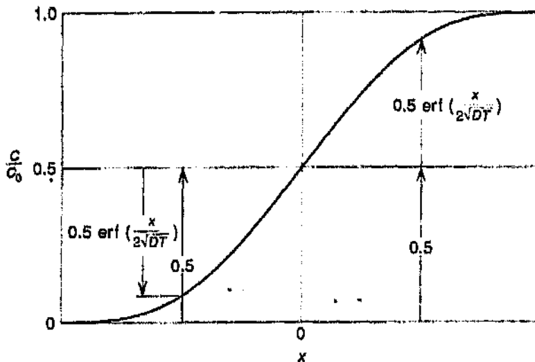
Figure 2.50: Normalised concentration profile produced by diffusion in an infinite diffusion couple. 55
