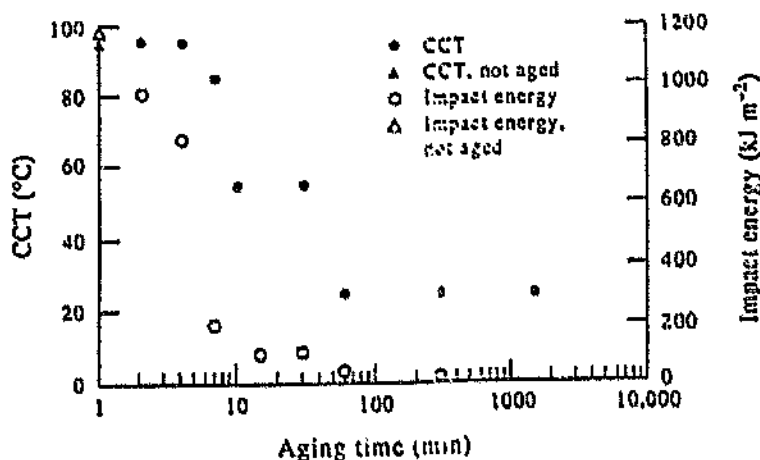
Figure 2.45: Critical crevice corrosion temperature (CCT) and impact value as a function of ageing time (i.e. increasing sigma content). 52
