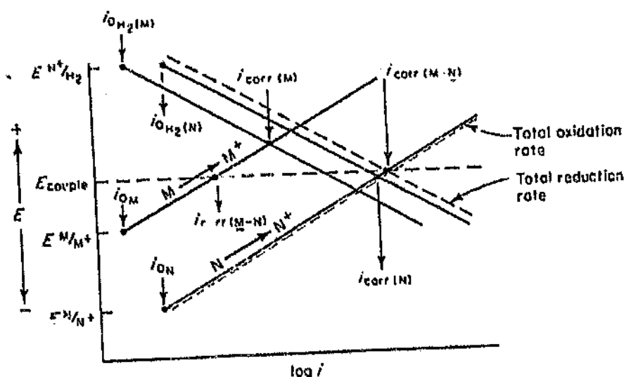
Figure 2.32: Galvanic couple between two corroding metals. 1
