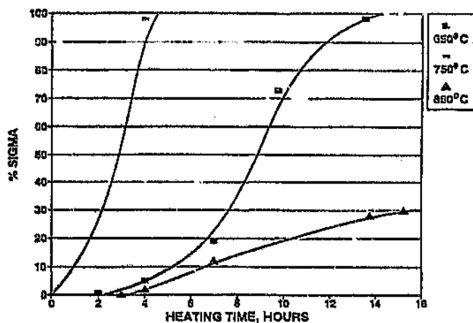
Figure 2.12: The rate of sigma phase formation in as-cast 2Ni-2Mo-39Cr-Fe at various temperatures. 21
