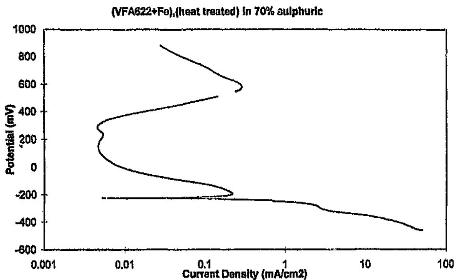
Figure 4.90: Corrosion scan for VFA622+Fe (Heat-treated).
