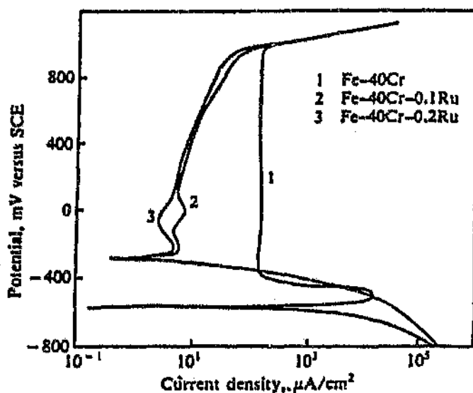
Figure 2.7: The effect of cathodic modification of Fe-40Cr with Ru in 0.5M \text{H}_2\text{SO}_4 . 25
