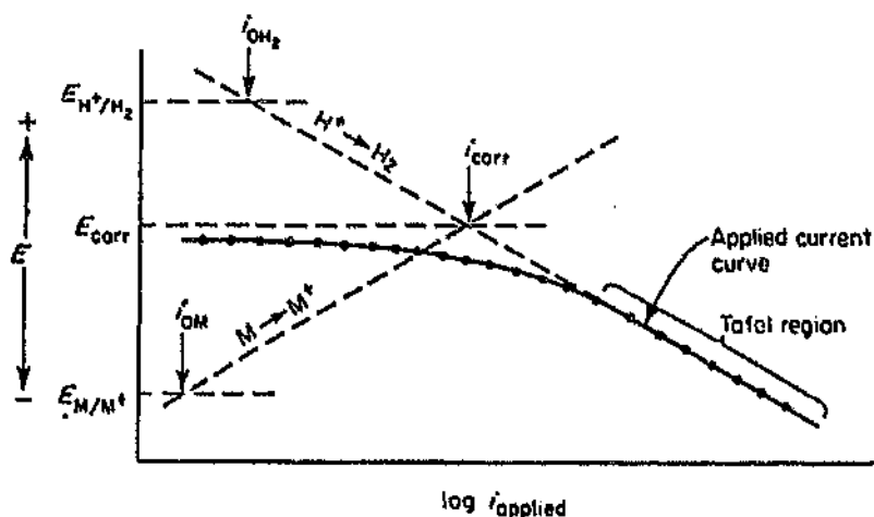
Figure 2.35: Applied current cathodic polarisation curve of a corroding metal showing Tafel extrapolation. 1
