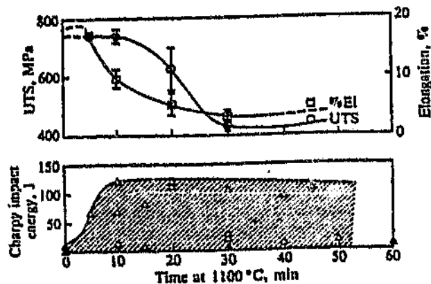
Figure 2.3: Mechanical properties of the warm-worked Fe-40Cr-2Ni-2Mo alloy as a function of SHT time at 1100°C. 25
