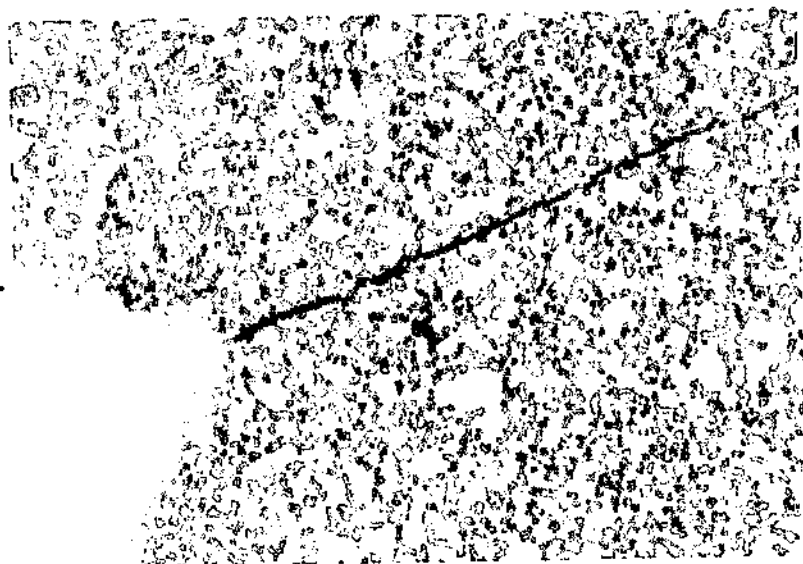
Figure 4.39: Extra milled VFA543 (SP001012), (As-HIPped), HCl etch, (500X), optical image.
