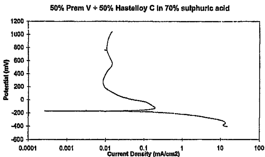
Figure 4.92: Corrosion scan for 50% Prem V + 50% Hastelloy C (Heat-treated). A distinct anodic loop is observed. The alloy remained passive up to an overpotential of 1000mv.
