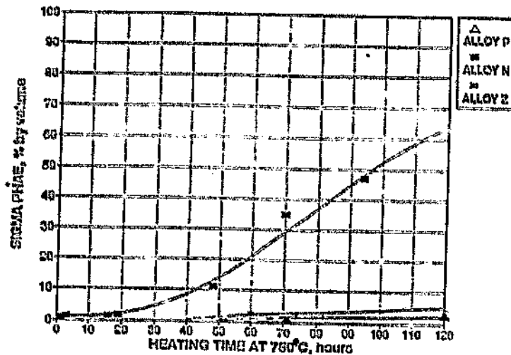
Figure 2.15 Formation of sigma phase in hot rolled alloys P (Al+Nb stabilised), N (Al+Zr stabilised) and Z (Al stabilised) at 750°C. 21
