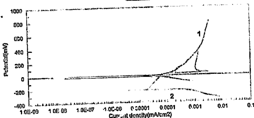
Figure 4.73: Corrosion scan for VFA487, as-HIPped. Spontaneous passivation. The second scan is non-representative due to poor electrical connection.
