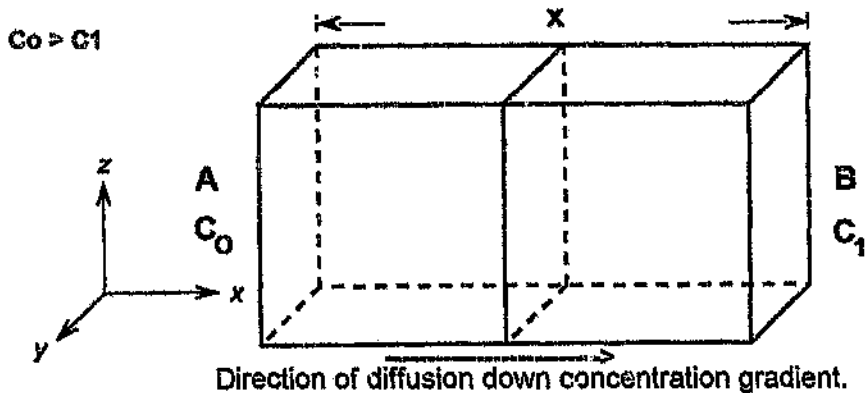
Figure 2.48: Basis for derivation of Fick's first law. 53
