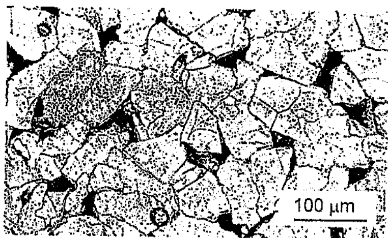
Figure 7. Porous microstructure of material produced during the HIP cycle in the absence of effective pressurization (VF420)
