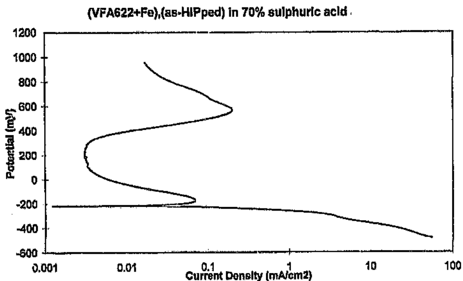
Figure 4.89: Corrosion scan for VFA622+Fe (As-HIPped).
