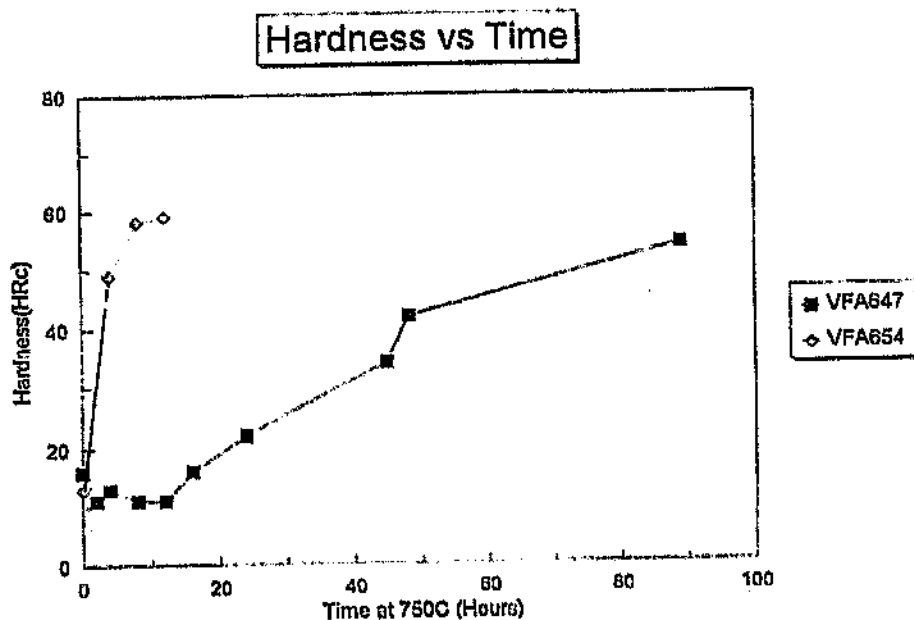
Figure 4.8: Hardness vs time at 750°C.
