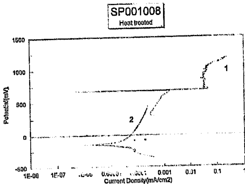
Figure 4.78: Corrosion scan for SP001008, heat treated
