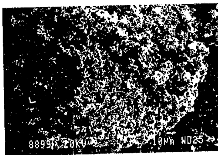
Figure 4.5: Detail of FeCr-Al agglomerate (SEM image in secondary electron mode).
