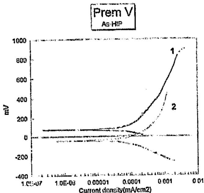
Figure 4.71: Corrosion scan for Prem V, as-HIPped. Spontaneous passivation in Figures 4.71-4.72.
