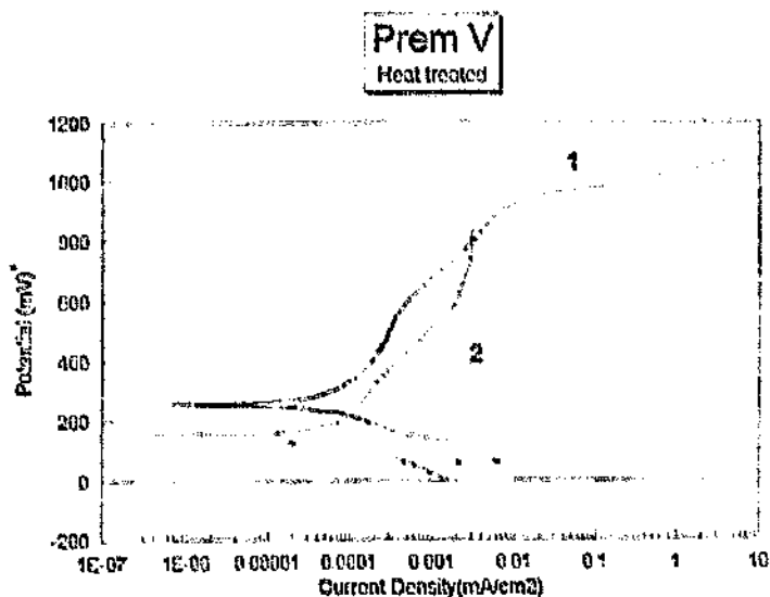
Figure 4.72: Corrosion scan for Prem V, heat treated.
