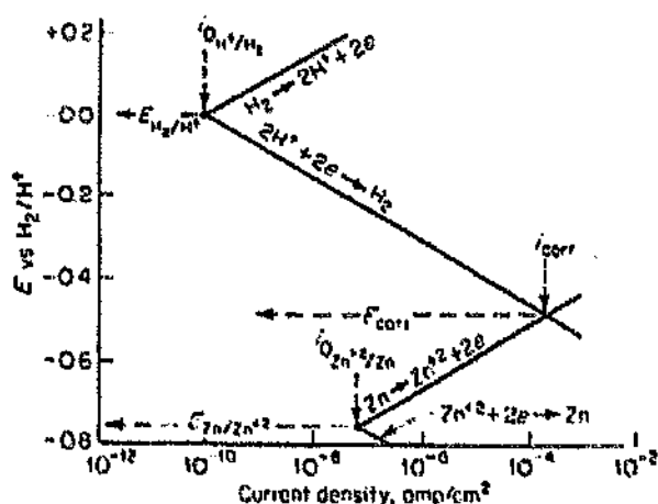
Figure 2.28: Electrode kinetic behaviour of Zn in acid solution. 1
