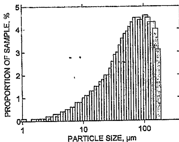
Figure 3. Particle size distribution of minus 170 \mu\text{m} fraction of powder produced by 30 seconds of milling in a Sieb mill (VF543).
