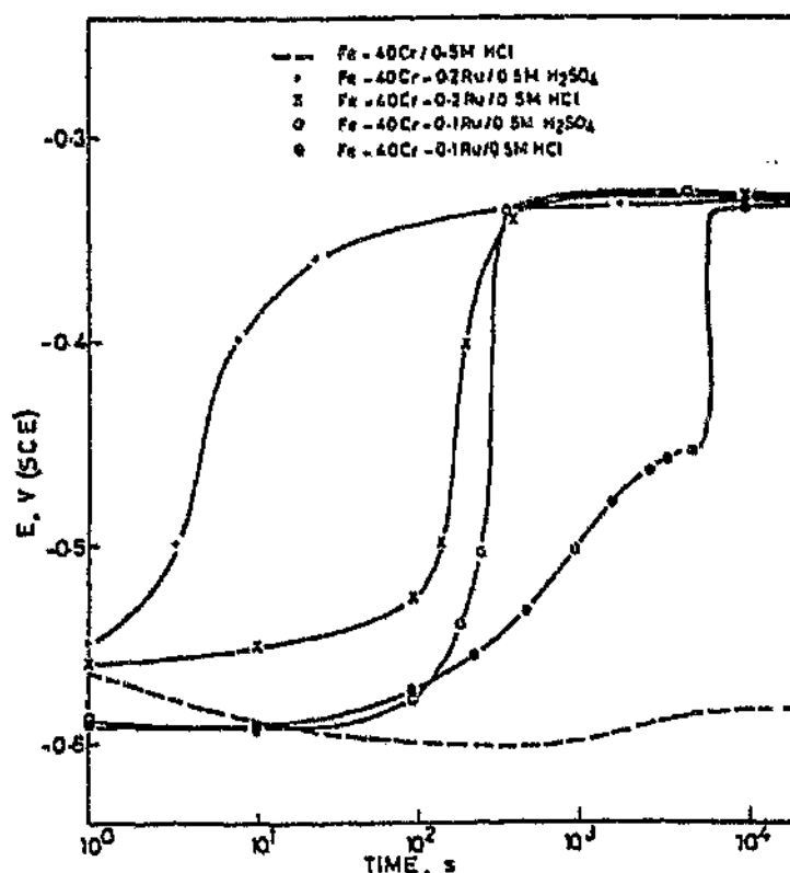
Figure 2.36: Potential-time curves for Fe-40Cr-Ru alloys displaying spontaneous passivation in 0.5M acids at 25°C. 27
