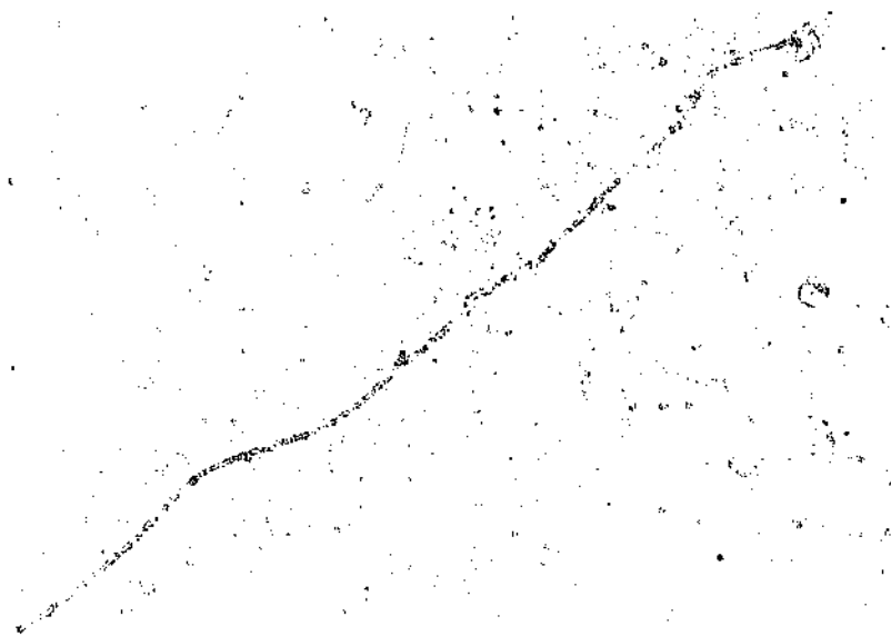
Figure 4.14: VFA417, (annealed 1100°, HCl etch, (200X), optical image. Large crack running through sigma-ferrite microstructure, with a higher number of particles near the crack.
