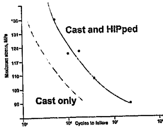
Figure 2.21: Comparison of material properties: as-cast and cast+HIPped. The material is Al-7 wt% Si alloy L99. 34
