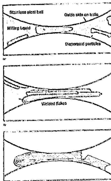
Figure 2.26: Cold welding of particles during ball milling 11
