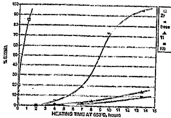
Figure 2.14 The rate of sigma phase formation at 650°C in the as-cast alloys containing 2%Mo and 2%Ni, with different stabilisers. 21
