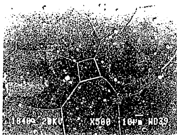
Figure 8. Microstructure of alloy VF552 in the HIPped and solution-annealed condition, showing a recrystallized ferritic matrix, and a network of oxide and carbonitride precipitates that outlines the original particle boundaries.
