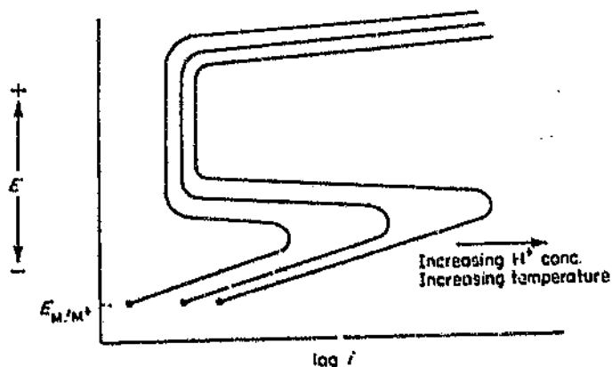
Figure 2.31: The effect of temperature and acid concentration on passivation. 1
