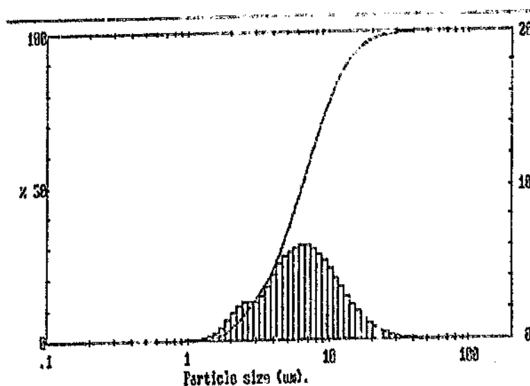
Figure 4.7: Particle size distribution of SP001008 (Extra Fe)
