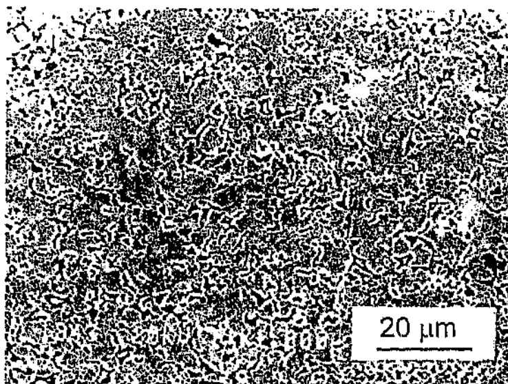
Figure 9. Microduplex mixture of ferrite and sigma phase produced by HIPping ultra-fine sigma powder (much of the sigma has been etched out in this micrograph).
