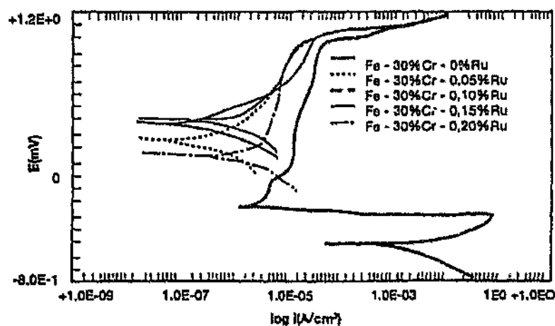
Figure 2.41: Potentiodynamic responses of Fe-30%Cr-Ru alloys in 10% H_2SO_4 at 25^\circ C . 51
