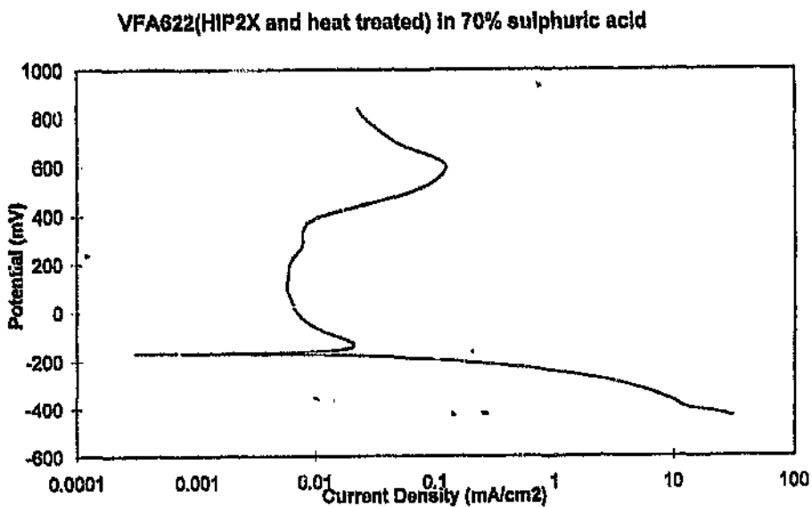
Figure 4.88: Corrosion scan for VFA622, HIPped twice- heat treated. A distinct anodic loop is present with two minima in the passive region.
