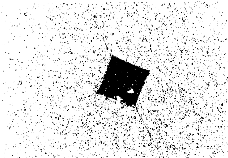
Figure 4.38: Extra-milled VFA543 (SP001012), (As-HIPped), HCl etch, (100X), optical image.
