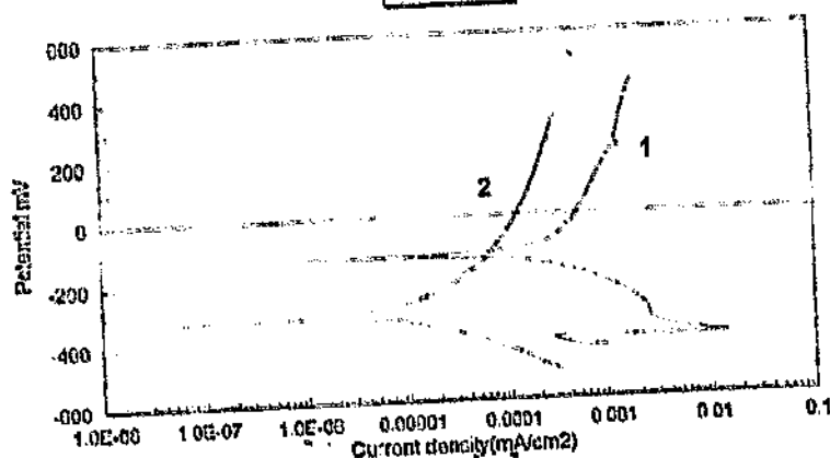
Figure 4.74: Corrosion scan for VFA487, heat treated. Spontaneous passivation in both scans.
