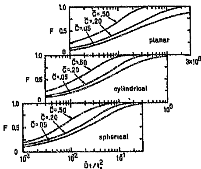
Figure 2.53: Homogenisation behaviour of planar, cylindrical and spherical pellets in terms of the degree of interdiffusion F , as a function of normalised homogenisation time, for various mean compositions, \bar{C} .
