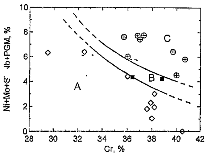
Figure 13. Diagram illustrating the effect of composition on the properties of the alloys, A - takes too long to convert to powder, B - comes out HIP as ferrite, C - comes out of HIP as sigma phase.
