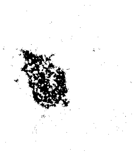
Figure 4.49: (20% 316L+80% VFA622), As-HIP (200X), HCl etch , optical image.
