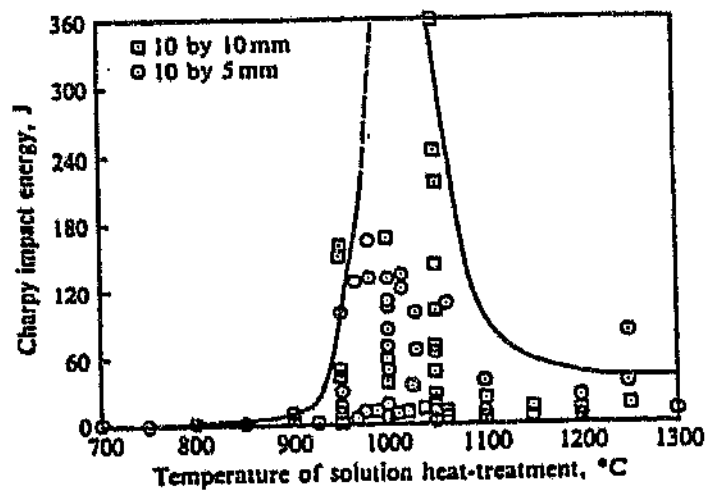
Figure 2.2: The effect of SHT (solution heat treatment) temperature on the room temperature Charpy toughness of Fe-40%Cr alloys. 25
