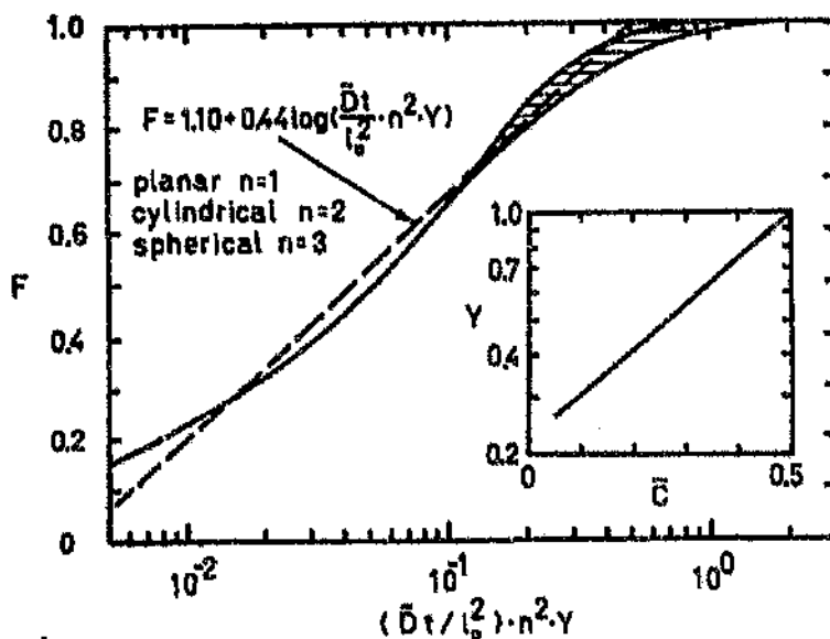
Figure 2.54: Normalised degree of interdiffusion F as a function of D_1 , t , l_0 , n and Y . 64
