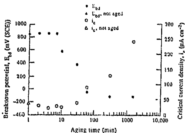
Figure 2.44: Breakdown potential ( E_{bd} ) and critical current density ( i_c ) as a function of ageing time (i.e. increasing sigma content). 52
