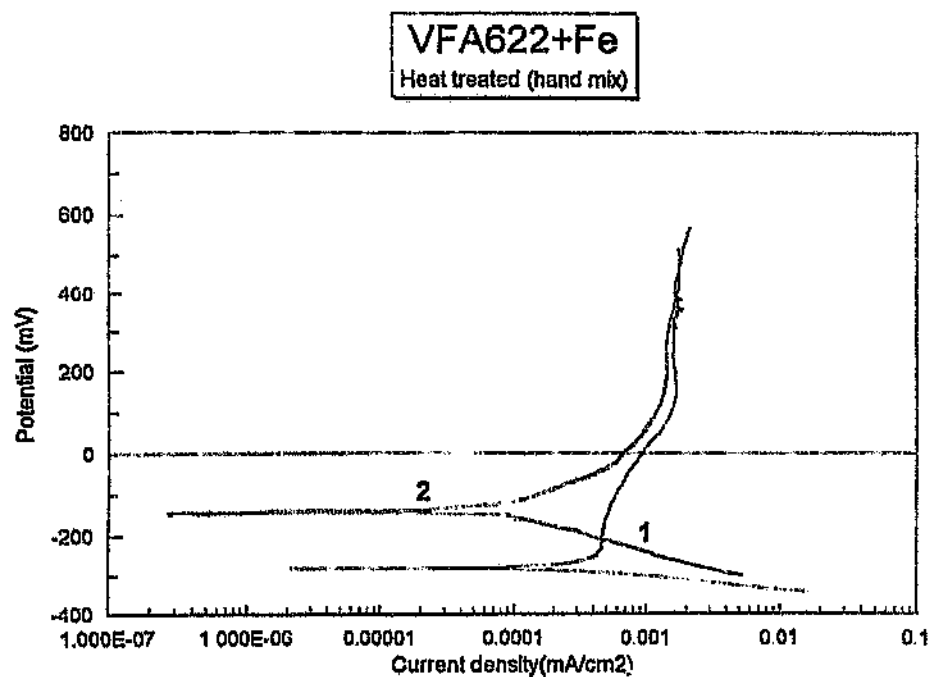
Figure 4.80: Corrosion scan for VFA622 + Fe, heat treated. Spontaneous passivation in the test medium.
