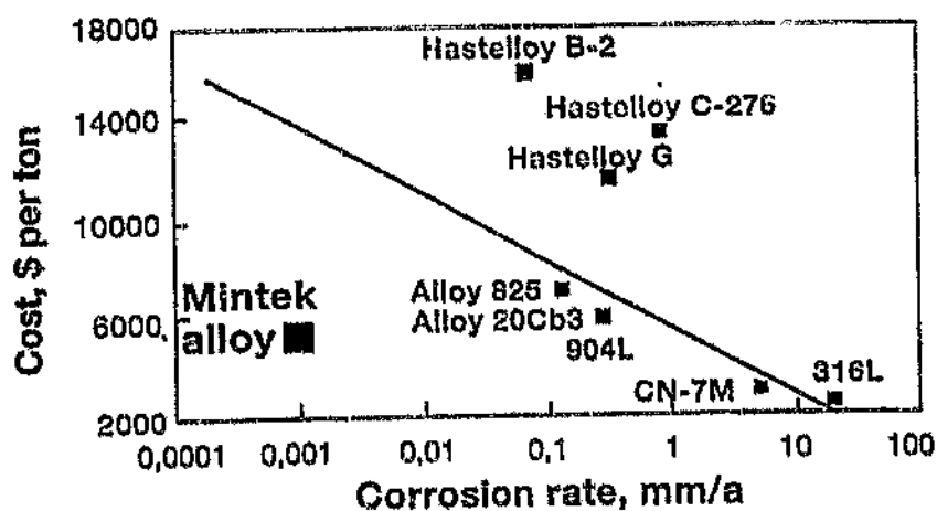
Figure 2.19: Cost-life comparisons in boiling 10% (by mass) sulphuric acid. 21
