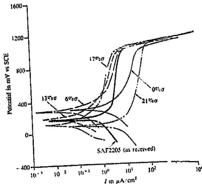
Figure 2.46: Potentiodynamic responses for SAF2205 duplex stainless steel with various sigma phase contents at 10% \text{H}_2\text{SO}_4 at 25^\circ\text{C} . 53
