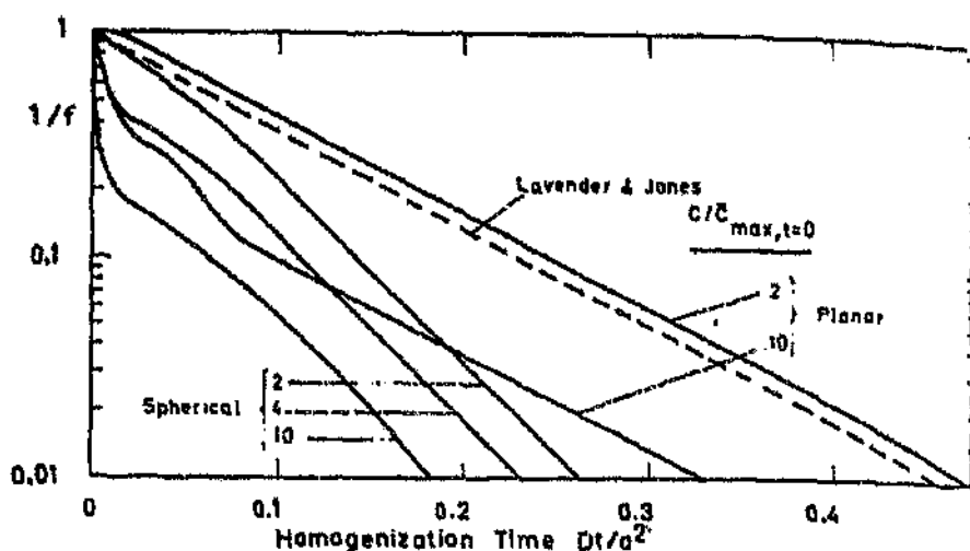
Figure 2.59: Comparison between predicted homogenisation behaviour based on the equation of Lavender and Jones and Larsson's study. Numbers on the curves show surface concentrations at \frac{Dt}{a^2} = 0 . 66
