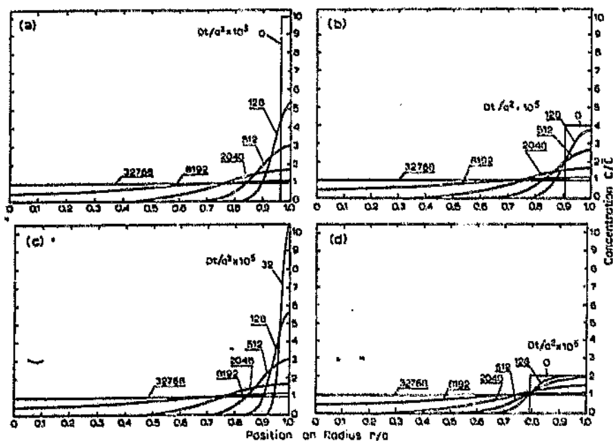
Figure 2.58: Concentration profiles along radius of sphere after various homogenisation times. Relative starting surface concentrations were: (a)10, (b)4, (c) \infty , (d)2. 10
