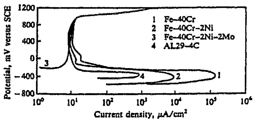
Figure 2.6: Potentiodynamic curves (against the standard calomel electrode) for the corrosion of four superferritic alloys in 10% \text{H}_2\text{SO}_4 . 25
