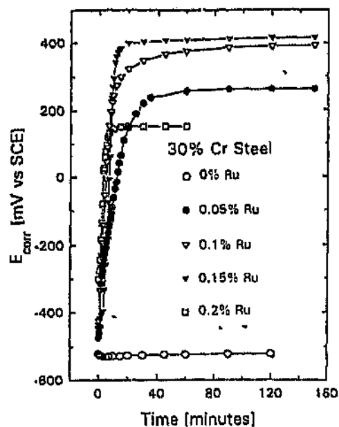
Figure 2.42: Open circuit corrosion potential variations with time of Fe-30%Cr-Ru alloys in 10% H_2SO_4 at 25^\circ C . 51
