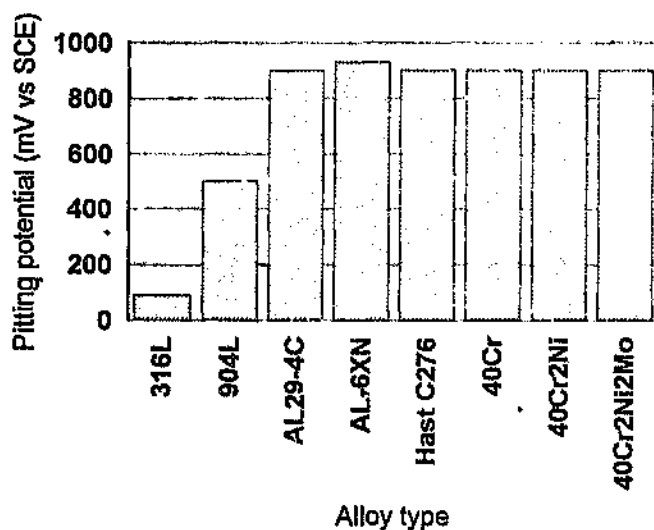
Figure 2.39: Pitting potentials of 40Cr-Fe alloys and commercial stainless steels in 3%NaCl at 60°C. 3
