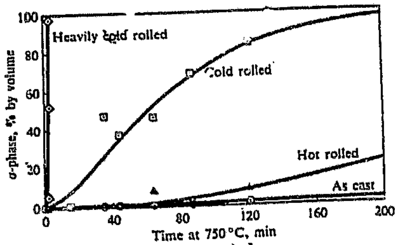
Figure 2.17 The effect of prior mechanical work on the formation of sigma phase in 2Ni-2Mo-40Cr-Fe 22
