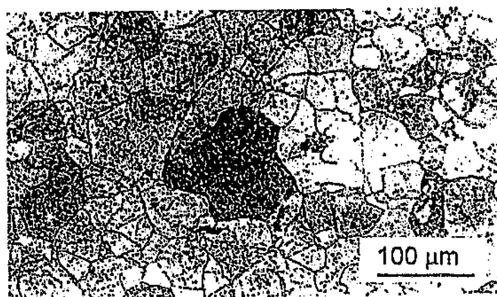
Figure 6. Typical angular microstructure of sigma phase produced by a single HIP cycle conducted on highly alloyed material (VF417).
