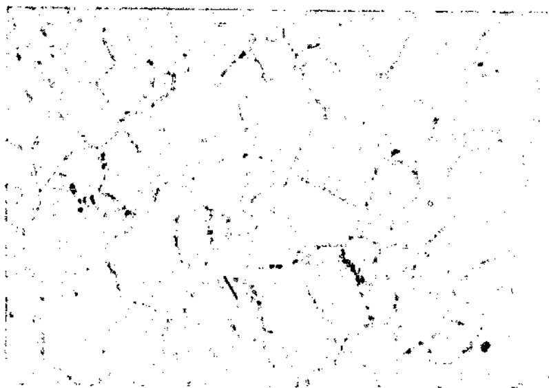
Figure 4.25: PremAlloy V, (annealed 1100°C), HCl etch, (200X), optical image. General ferritic microstructure with a number of dark grey inclusions. The inclusions were analysed with EDS techniques.
