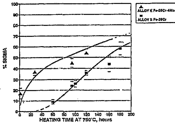
Figure 2.11: The rate of sigma formation in warm rolled (300°C) alloys K(4Mo-29Cr-Fe) and S(39Cr-Fe). 21
