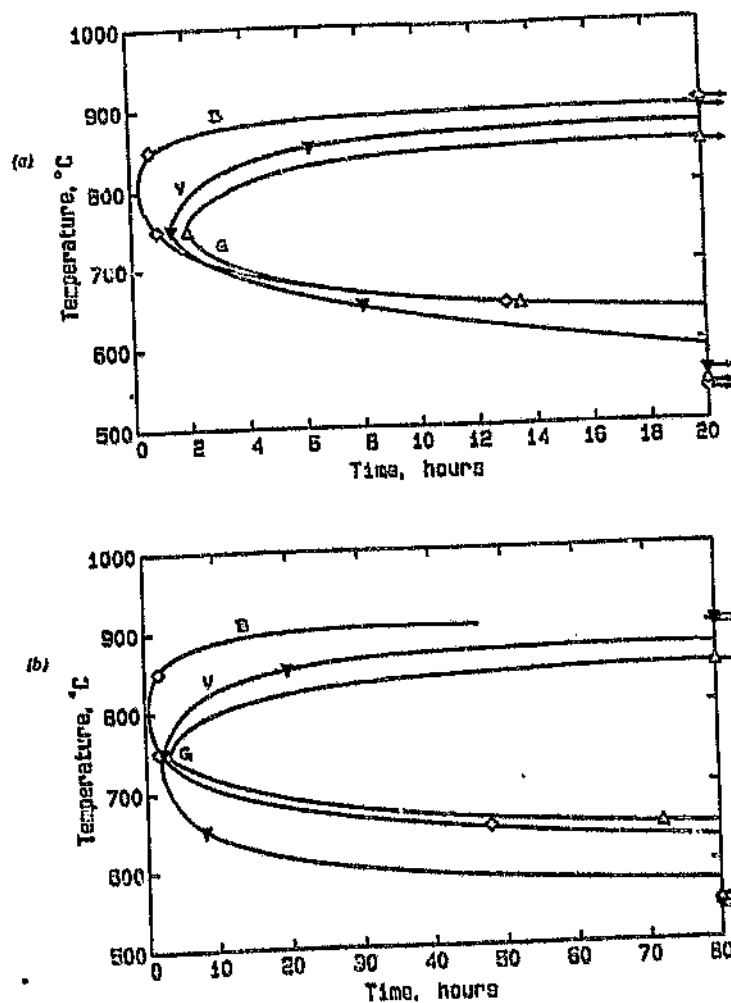
Figure 2.18. Time-temperature-transformation diagrams for the formation of sigma in as-cast unstabilised (V), Nb stabilised (G), Ti stabilised (B) alloys. 21 (a) 10% sigma (b) 50% sigma
