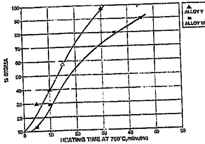
Figure 2.16 Formation of sigma phase in hot rolled 2%Mo and 2%Ni containing alloys V (unstabilised) and W (0.05% nitrogen) at 750 °C 21
