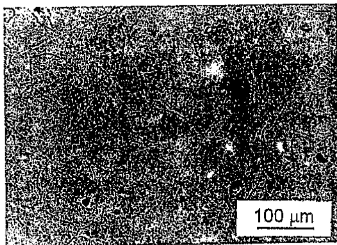
Figure 11. Microstructure of alloy VFA622, after a solution anneal and quench showing ferrite grains with intergranular precipitation of carbide and nitride precipitates.
