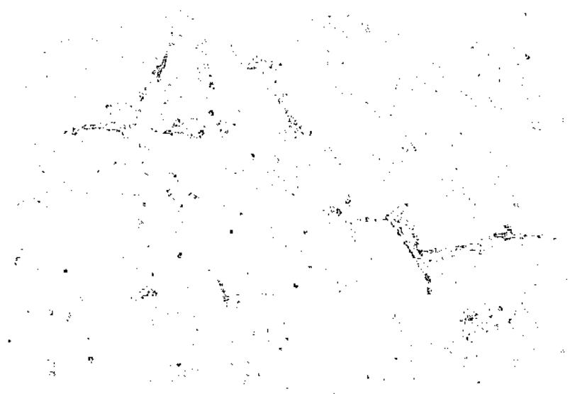
Figure 4.20: VFA423, (annealed 1100°C), HCl etch, (200X), optical image. Residual sigma in ferrite matrix.
