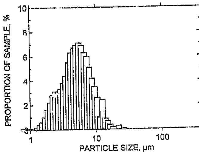
Figure 4. Particle size distribution of powder produced from Sieb mill product by a further 24 hours of milling in a ball mill (VFA 543).
