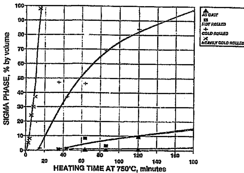
Figure 2.8: The effect of thermo-mechanical processing on sigma phase formation on alloy T15 at 750°C. 21
