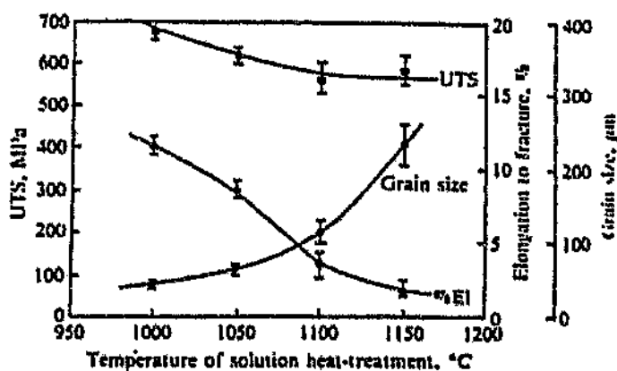
Figure 2.4: The effect of SHT temperature on the tensile properties of cold-worked Fe-40Cr-2Ni-2Mo. 25
