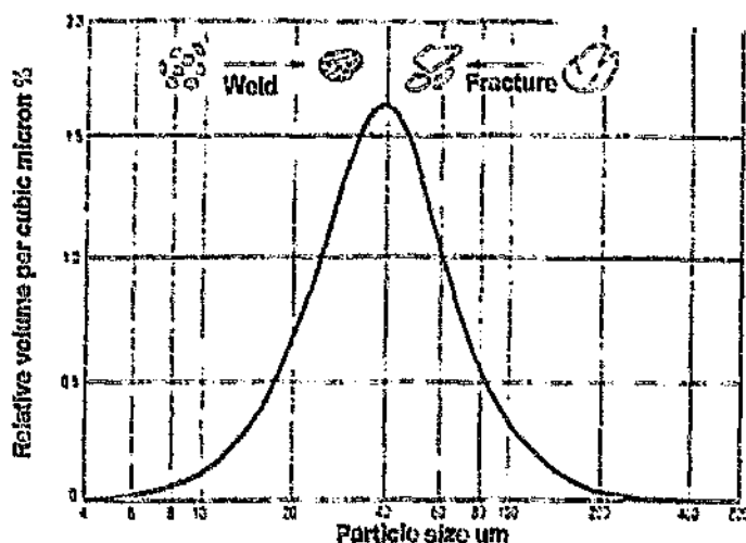
Figure 2.25: Narrow particle size distribution caused by tendency of small particles to weld and large particles to fracture. 11
