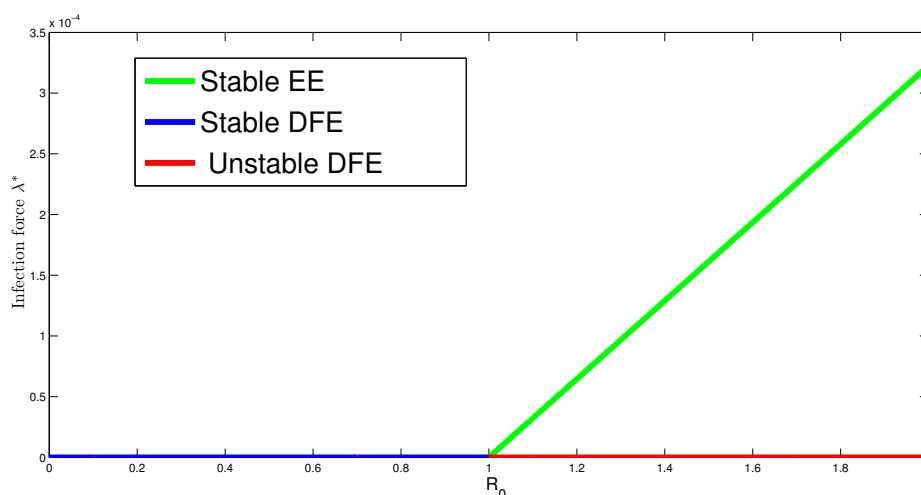
Figure 3. The forward bifurcation curve for the model system in (2.6) in the (\mathcal{R}_0, \lambda^*) plane.
