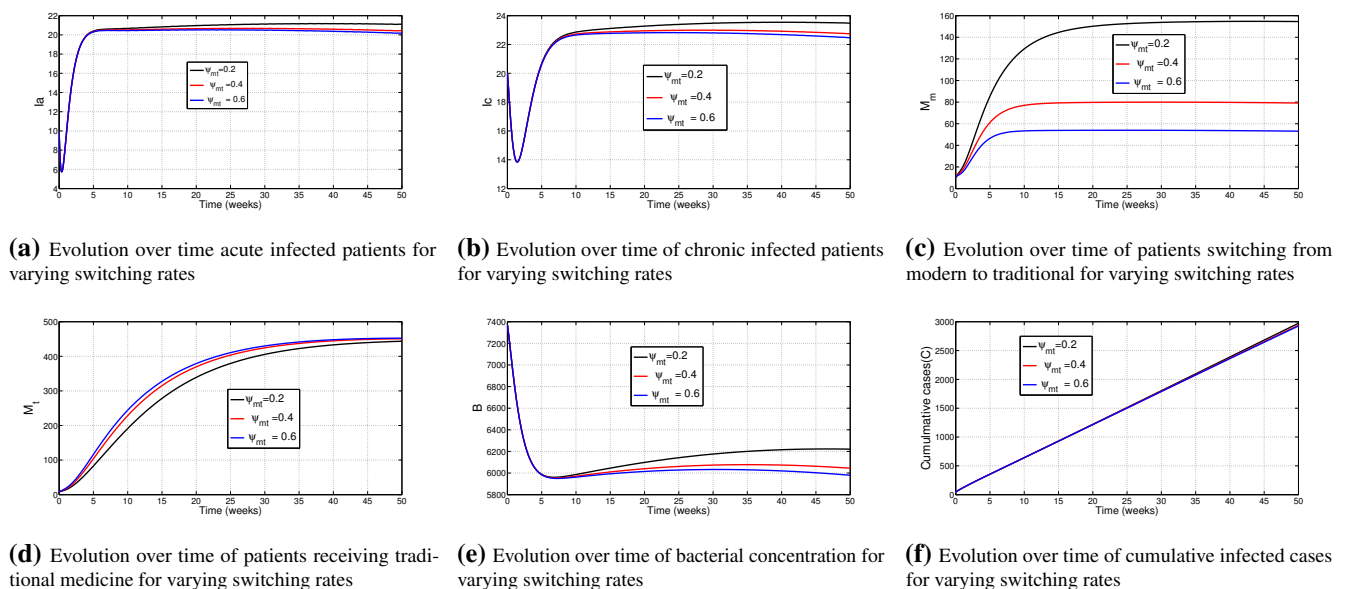
Figure 9. Importance of switching from modern to traditional treatment.
