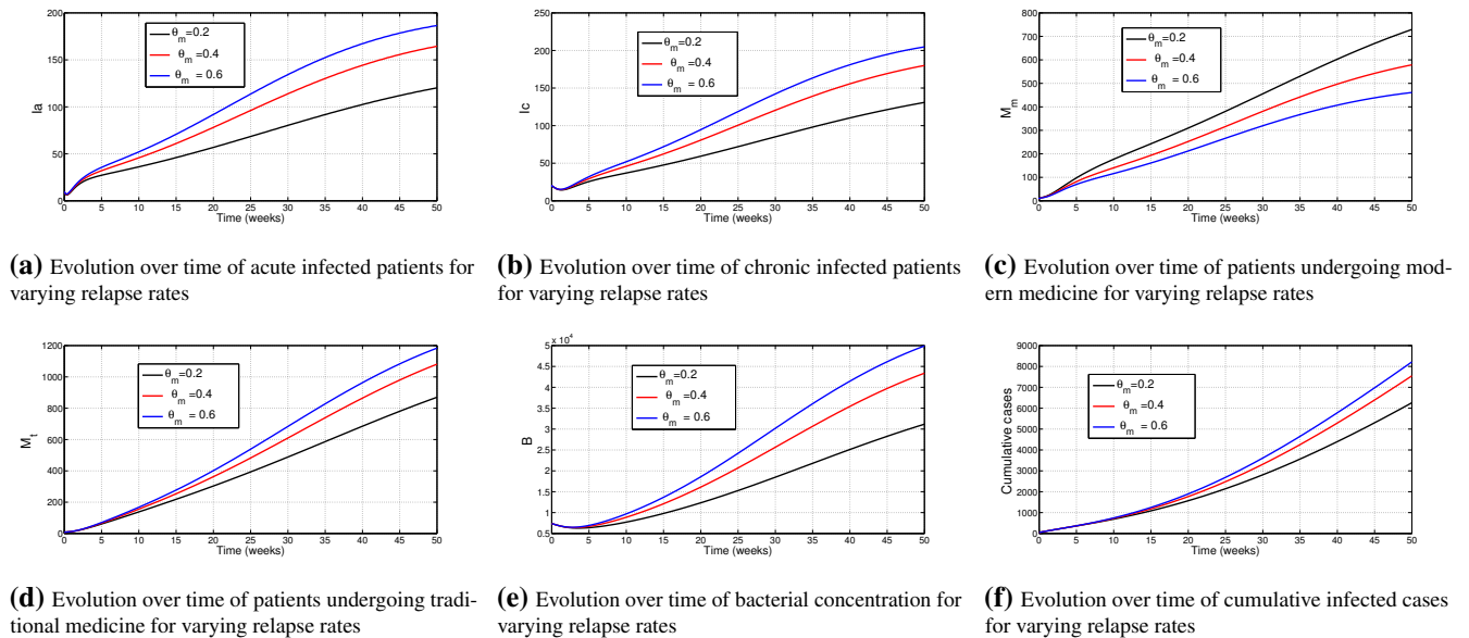
Figure 8. Influence of relapse on the model variables.
