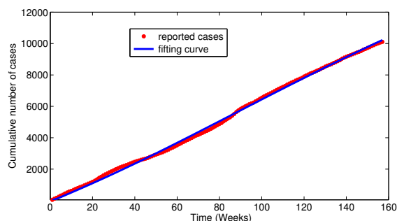
(a) Model fit on the cumulative number of cases per week between 30 December 2019 and 1 January 2023
