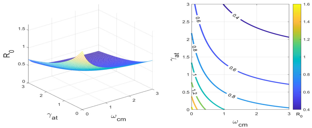
(a) Contour plot showing how R_0 depends on \gamma_{at} and \omega_{cm}
