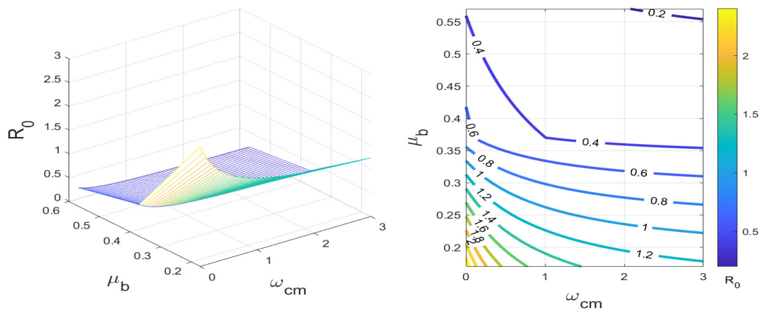
(b) Contour plot showing how R_0 depends on \mu_b and \omega_{cm}
