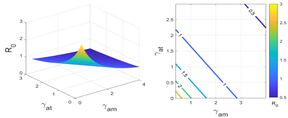
(c) Contour plot showing how R_0 depends on \gamma_{at} and \gamma_{am}
