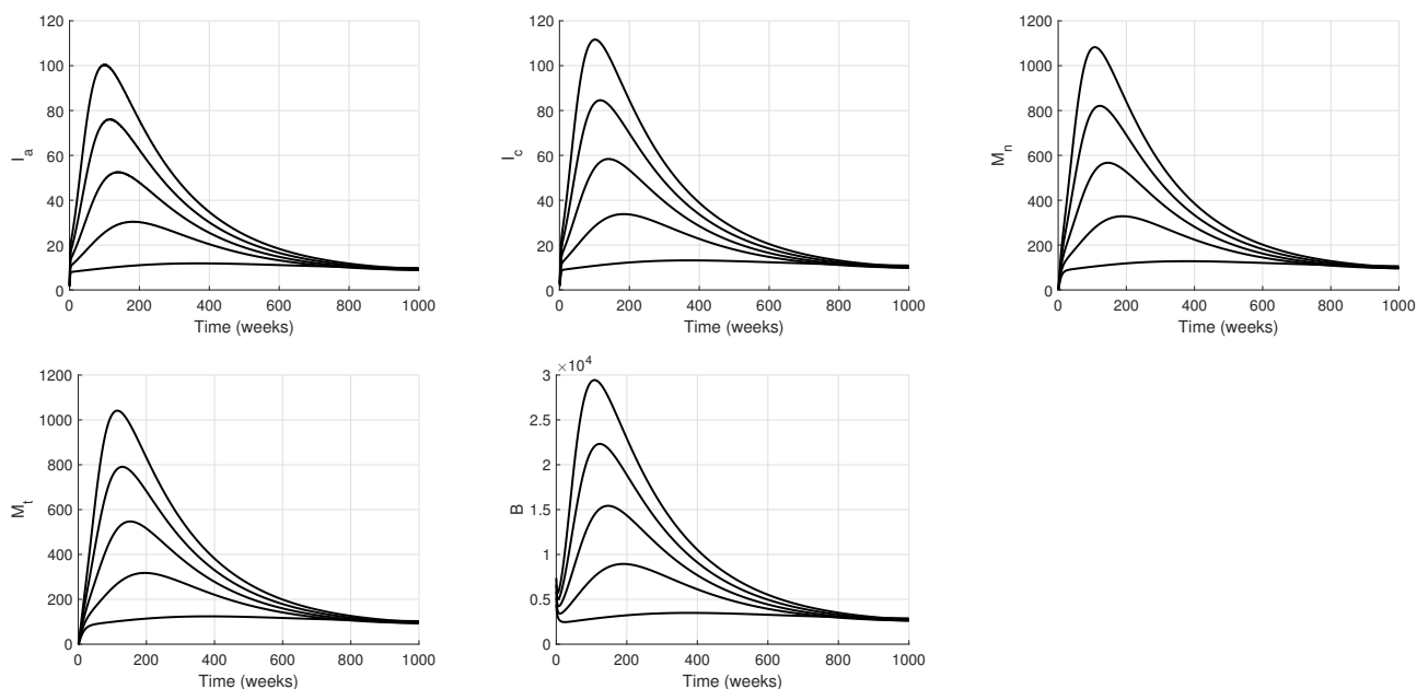
Figure 4. GAS of the EE. This figure is plotted with \theta_m = 0.097 . The other parameter values are as in Table 2. The value of \mathcal{R}_0 = 1.8 .
