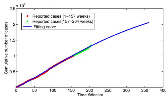
(b) Model validation and prediction on the dynamics of typhoid disease for the period up to November 2026
