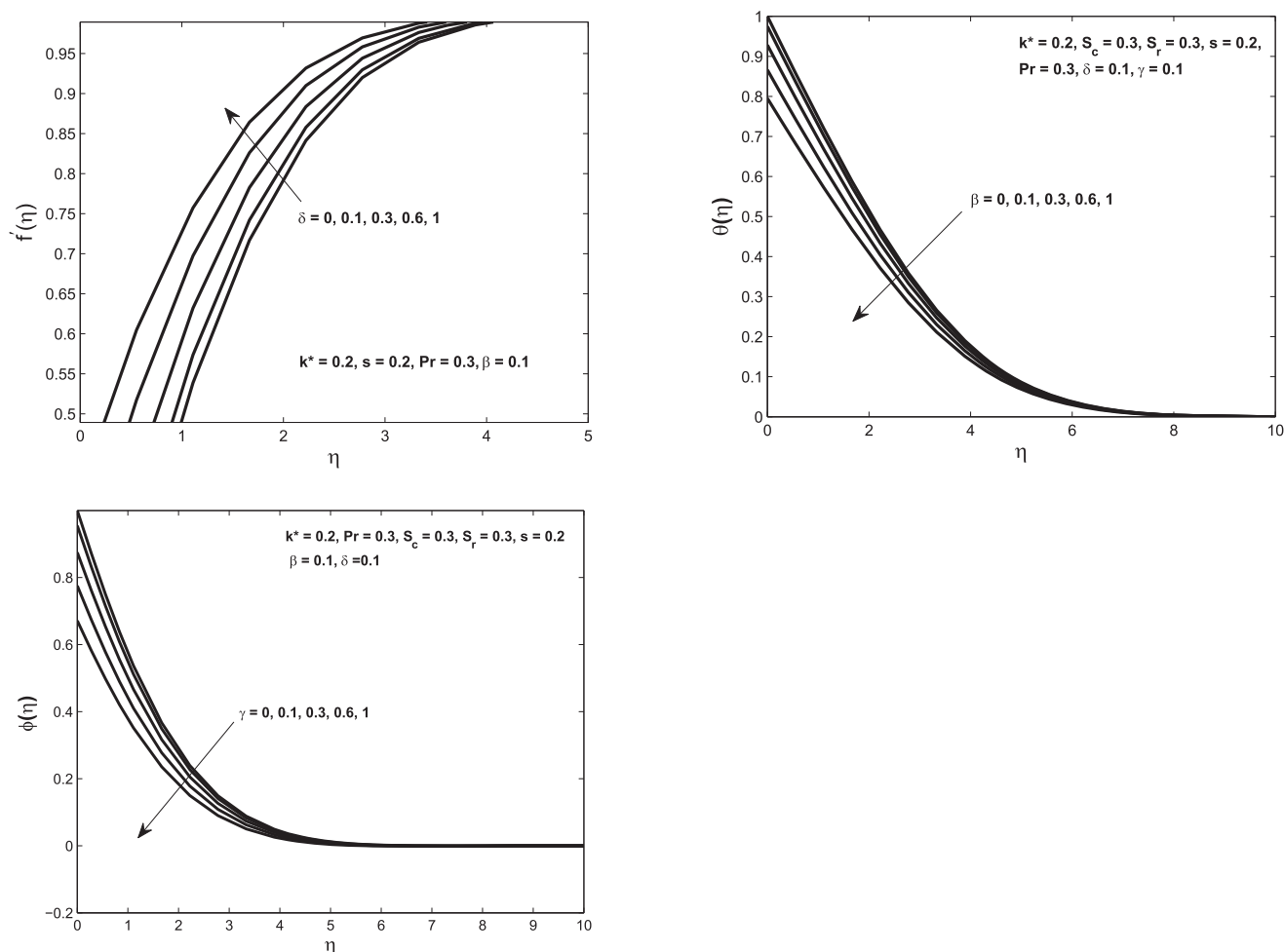
Fig. 3. Top left: Velocity profile f'(\eta) as a function of \eta ; Top right: Temperature profiles \theta(\eta) as function of \eta . Bottom left: Concentration profile \phi(\eta) as function of \eta . In all of these figures we vary velocity, thermal and concentration slip parameters for both slip and no-slip conditions.
