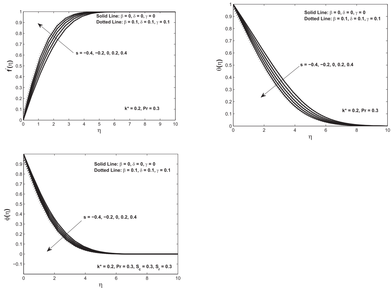
Fig. 4. Top left: Velocity profile f'(\eta) as a function of \eta ; Top right: Temperature profiles \theta(\eta) as function of \eta . Bottom left: Concentration profile \phi(\eta) as function of \eta . Here we vary the suction/blowing parameters for both slip and no-slip conditions.
