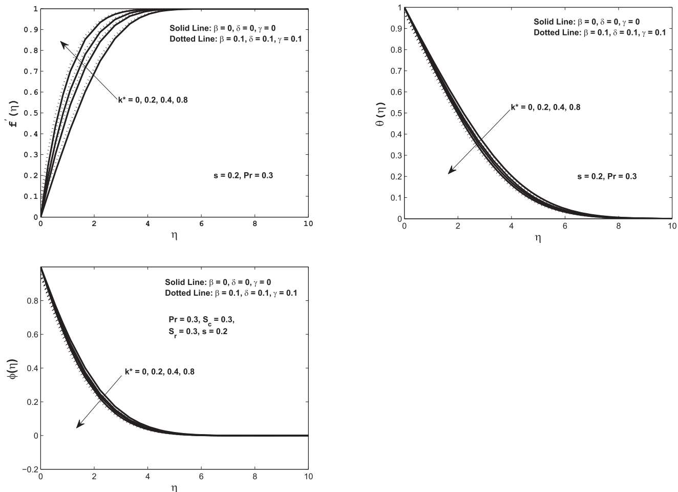
Fig. 2. Top left: Velocity profile f'(\eta) as a function of \eta ; Top right: Temperature profiles \theta(\eta) as function of \eta . Bottom left: Concentration profile \phi(\eta) as function of \eta . In all of these figures we vary permeability k^* with slip and no-slip conditions.
