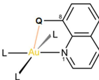
Figure 4.3. Diagram showing an example of the Au(III)\cdots Q interaction that would occur in our proposed metal-quinoline system.
