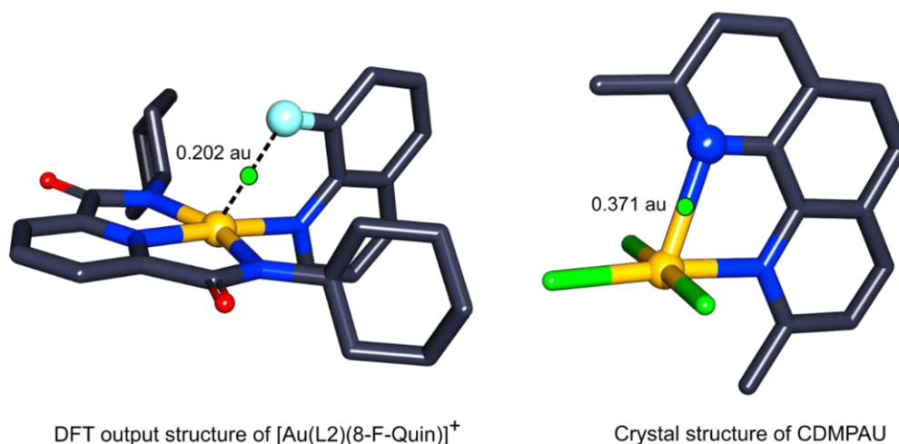
Figure 4.18. Diagram showing the structural differences between 5-coordinate \text{Au}(\text{III}) structures in the literature (CDMPAU) and a \text{Au}(\text{III}) structure that was analysed as part of this study. Hydrogen atoms have been excluded for visibility. The \rho(\text{Au}\cdots\text{F}) value for [\text{Au}(\text{L2})(8\text{-F-Quin})]^+ is 0.202 au and the \rho(\text{Au}\cdots\text{N}) value is 0.371 au.
