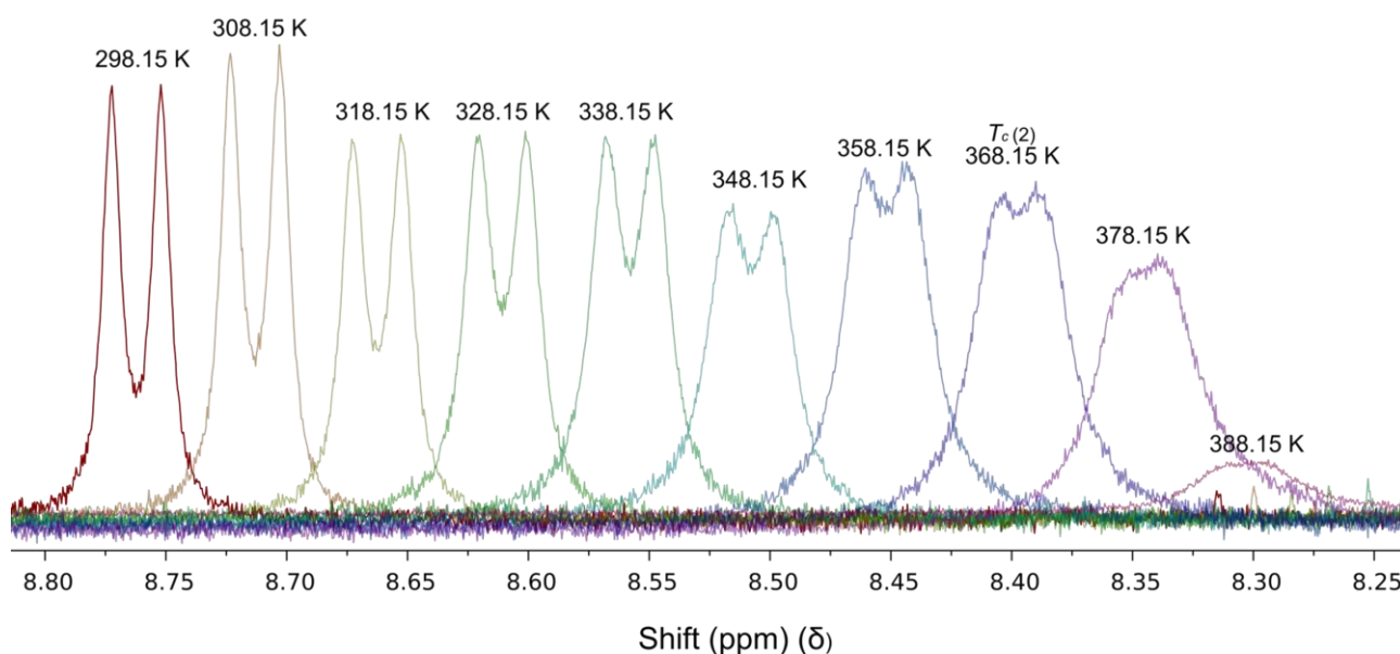
Figure 3.19. Variable temperature ^1\text{H} NMR spectra, taken at a constant concentration of 0.0228 M. The plot shows the downfield shift of the N-H amide peak. The temperature range for the experiment was 298.15 K to 388.15 K, with spectra recorded at 10 K intervals. The T_c(2) value is at 378.15 K.
