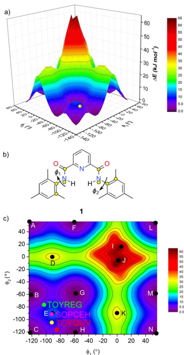
Figure 3.10. a) Three-dimensional plot showing the variation in the relative heat of formation, \Delta E , of 1 as a function of the torsion angles \phi_1 and \phi_2 . The angular coordinates locating the crystal structure are shown as a yellow sphere ( \phi_1 = -91.8^\circ , \phi_2 = -104.9^\circ , \Delta E = 8.8 \text{ kJ mol}^{-1} ).
