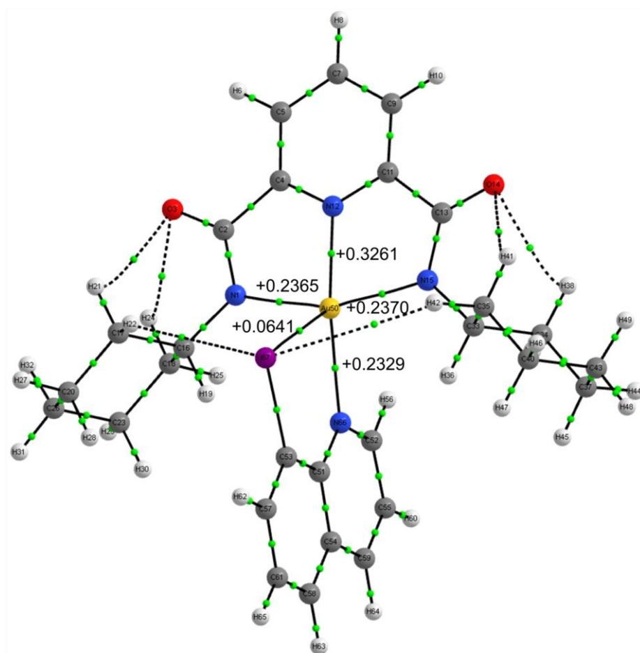
Figure 4.24. Example of the output of an AIM analysis on the [\text{Au}(\text{L2})(8\text{-l-Quin})]^+ structure. Bond critical points are rendered as green spheres, with \nabla^2\rho data labels displayed over selected bond critical points. All of the \nabla^2\rho values are positive, showing that the bonds are ionic in nature.
