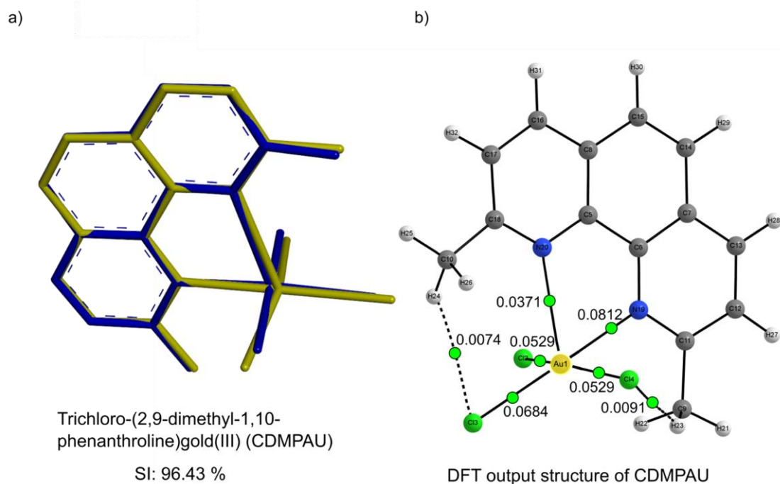
Figure 4.27. (a) Overlay of the DFT-calculated and crystal structure of CDMPAU. SI: 96.43%. Hydrogen atoms have been excluded for visibility. (b) DFT-calculated structure of CDMPAU with selected results of the AIM analysis. Selected bond critical points have been shown as green dots and their corresponding \rho values have been provided in Table 4.9.
