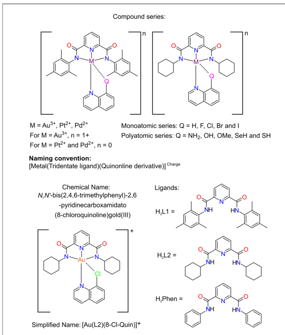
Figure 4.9. Diagram summarising the structures that were investigated, and the simplified naming convention that will be used throughout this dissertation.
