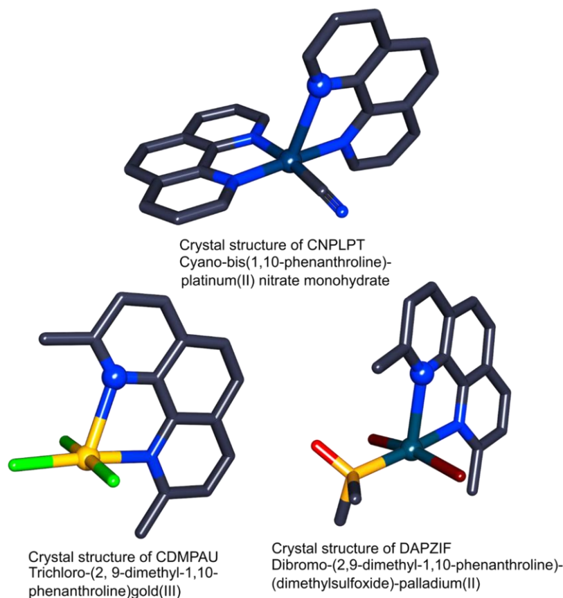
Figure 4.22. Selected examples from the literature of nominally 5-coordinate Au(III), Pt(II) and Pd(II) crystal structures. Hydrogen atoms have been excluded for visibility. The key question here is whether the axial M—N interaction behaves merely as an electrostatic interaction enforced by geometrical constraints of the phenanthroline ligand, or if sufficient electron density resides at a bond critical point for the interaction to be treated as a dative covalent bond. Structures are re-drawn from CSD codes: CNPLPT, CDMPAU and DAPZIF.
