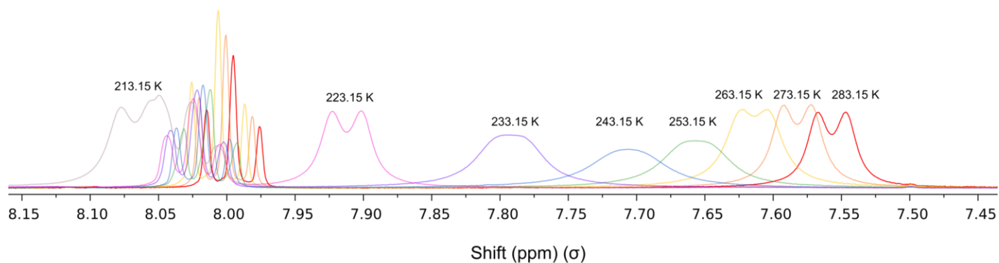
Figure 3.20. Variable temperature ^1\text{H} NMR spectra, taken at a constant concentration of 0.0228 M. The temperature range for the experiment was 288.15 K to 213.15 K, with spectra recorded at -10 K intervals. The plot shows the downfield shift of the N-Hamide peak.
