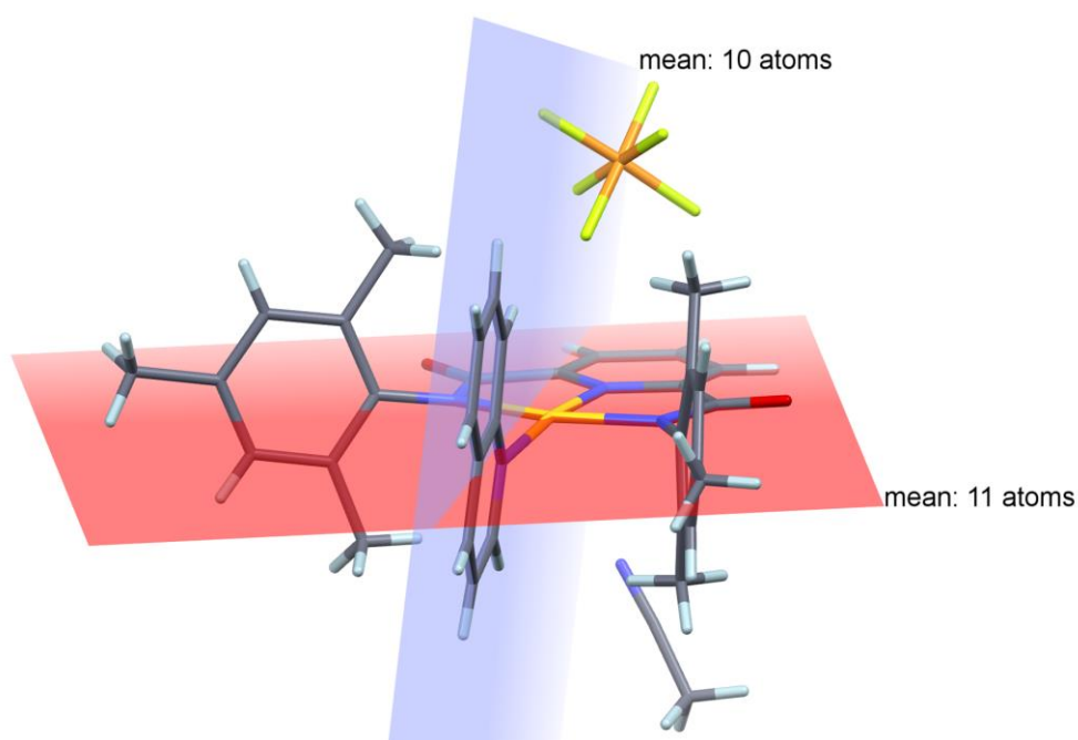
Figure 4.5. Diagram illustrating the least-squares planes between the metal-chelating 11-atom pincer ligand and the 10-atom quinoline ligand plane. The dihedral angle between the planes is 84.7°. The Au(III) ion and three N atoms of the pincer ligand lie approximately in the chelate plane (Au is displaced only 0.04 Å below the plane), while the quinoline N atom is displaced significantly below the plane (0.36 Å) giving it the appearance of a downward tilt.
