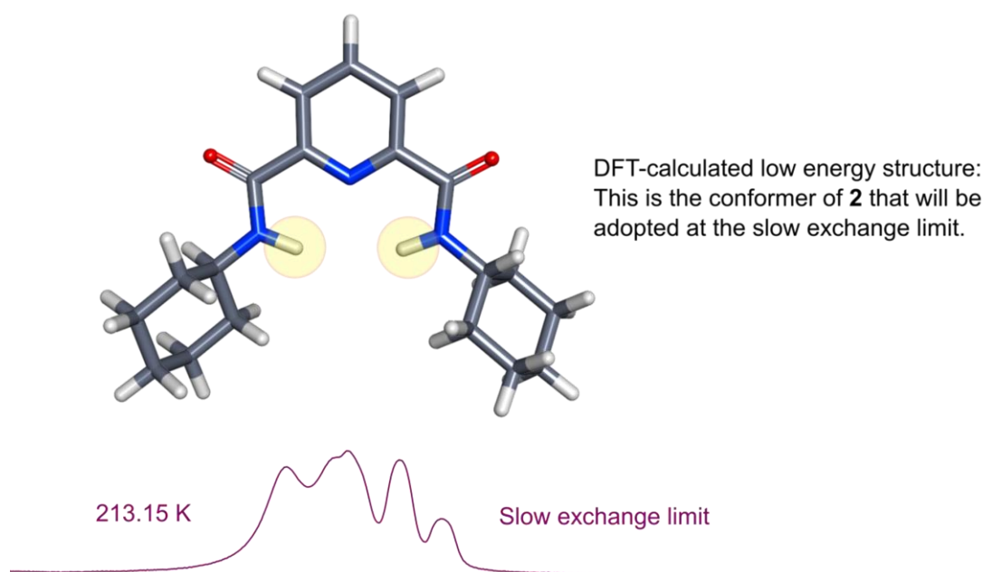
Figure 3.22. Low energy DFT calculated structure of 2 . At the slow exchange limit (213.15 K) this is likely the only conformer that will be adopted by the system.
