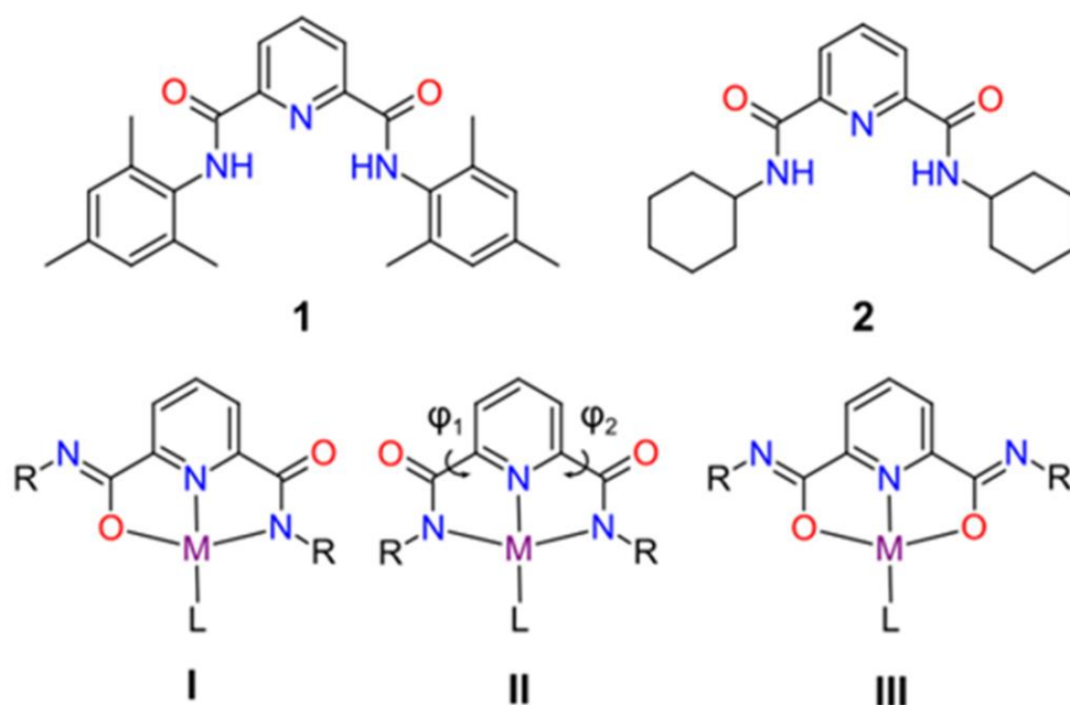
Scheme 3.1. Scheme depicting linkage isomers of N,N' -bis(2,4,6-trimethylphenyl)-2,6-pyridinedicarboxamide ( 1 ) and N,N' -bis(cyclohexyl)-2,6-pyridinedicarboxamide ( 2 ). Linkage isomers I to III result from rotations about \phi_1 and \phi_2 and resonance re-hybridization of the amide groups of the ligand. Linkage isomers are drawn for an arbitrary metal ion M with square planar geometry and a fourth ligand L.
