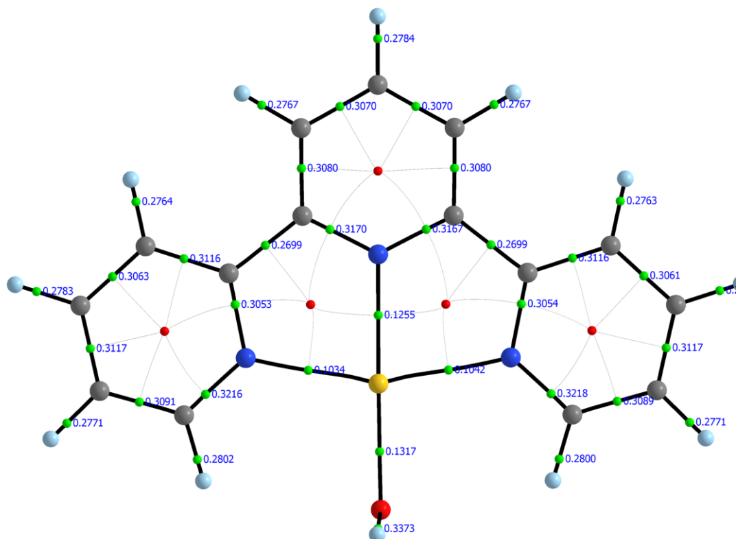
Scheme 4.1. The output of an AIM analysis performed on the structure of [Au(terpy)(OH)] 2+ , CSD code: BORSUY. Bond critical points are rendered as green spheres, with \rho data labels displayed over selected bond critical points. This structure was used to provide a suitable reference electron density for a substantially more covalent M-O coordination bond, enabling estimates of the % covalent character to be made in Tables 4.9-4.11.
