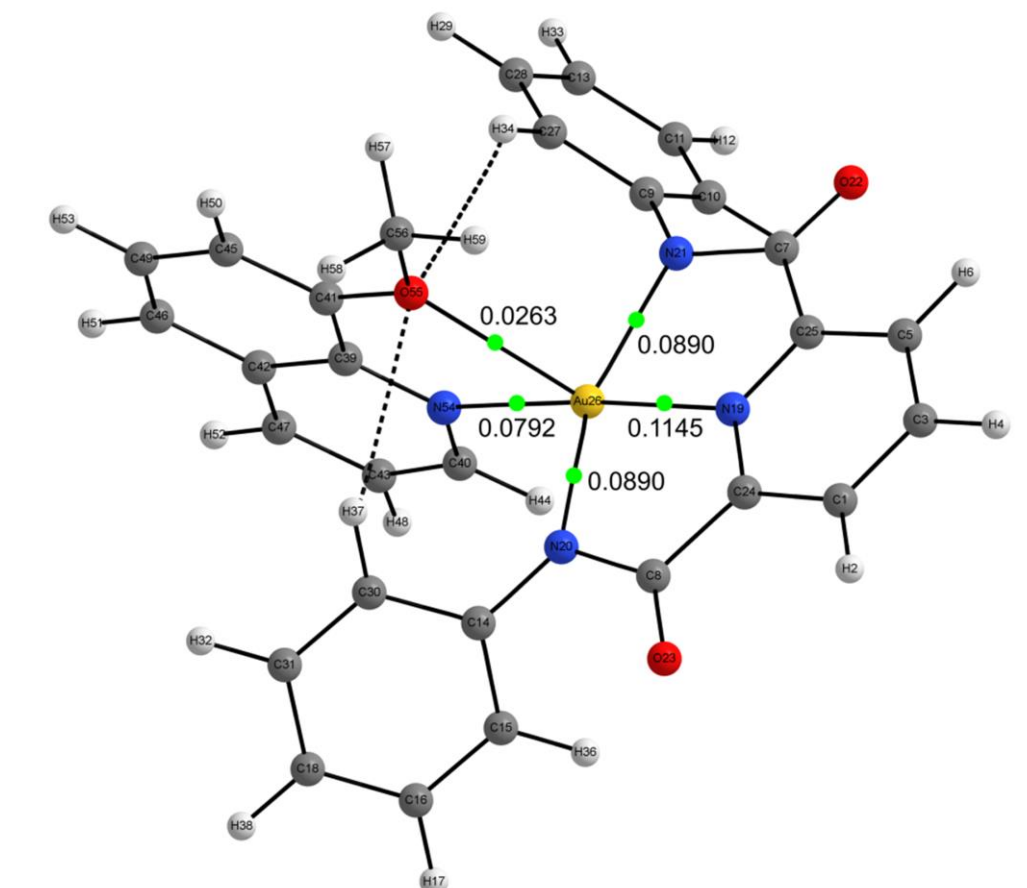
Figure 4.21. Image showing the output of an electron density analysis (AIM method; AIMAll software package) for [\text{Au}(\text{Phen})(8\text{-}[\text{OMe}]\text{-Quin})]^+ . The green dots denote selected bond critical points while the number (in atomic units, au) gives a measure of the predicted electron density of the BCP along the interaction.
