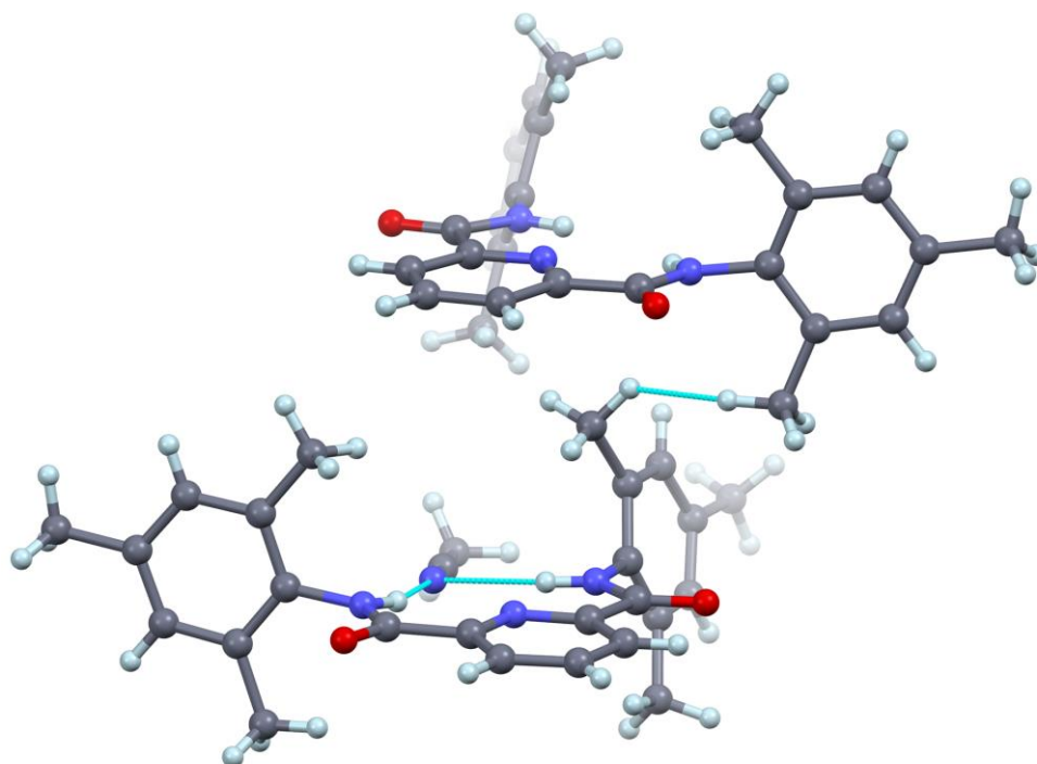
Figure 3.2 Diagram highlighting how intermolecular non-bonded contacts impact the dihedral angles of the mesityl rings in structure 1 .
