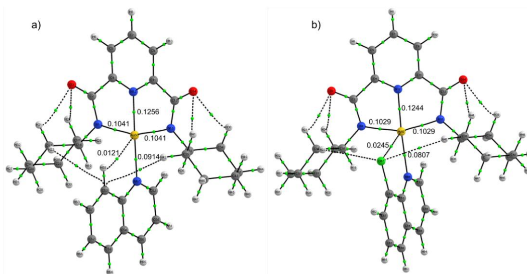
Figure 4.23. Examples of the output of AIM analysis on structures a) [\text{Au}(\text{L}2)(8\text{-H-Quin})]^+ and b) [\text{Au}(\text{L}2)(8\text{-Cl-Quin})]^+ . Bond critical points are rendered as green spheres, with p data labels displayed over selected bond critical points.
