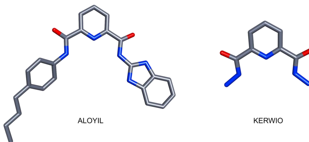
Figure 3.8: Crystal structures of ALOYIL and KERWIO. These are examples of literature pincer ligands, whose structure parameters closely match those of 1 and 2 .
