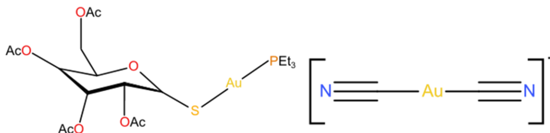
Figure 1.2. Diagram showing the structure of the Au(I) drugs Auranofin and [\text{Au}(\text{CN})_2]^- .
