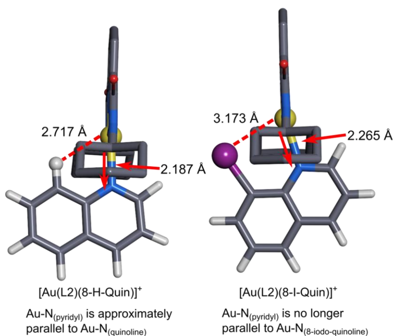
Figure 4.17. Diagram emphasising how M-N_{(\text{quin})} increases as M\cdots Q increases. N_{(\text{pyridyl})}-Au-N_{(\text{quinoline})} = 177.80^\circ and N_{(\text{pyridyl})}-Au-N_{(8\text{-iodo-quinoline})} = 164.62^\circ . Some hydrogen atoms have been excluded for visibility.
