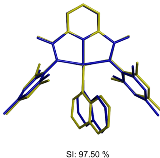
Figure 4.10b. A comparison between the DFT-calculated (yellow) and X-ray crystal structure (blue) of \text{Pd}(\text{L1})(8\text{-H-Quin}) . The DFT calculation was performed at the HSEH1PBE/SARC-ZORA/ 6-311G(d,p) level of theory. For the DFT calculation the SARC-ZORA basis set was used for the metal (Pd) and the 6-311G(d,p) basis set was used for light atoms (H, C, N, O). SI: 97.50%. Hydrogen atoms have been excluded for visibility.
