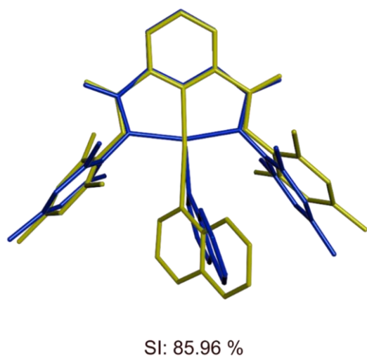
Figure 4.10a. A comparison between the DFT-calculated (yellow) and X-ray crystal structure (blue) of [\text{Au}(\text{L1})(8\text{-H-Quin})]^+ . The DFT calculation was performed at the HSEH1PBE/SARC-ZORA/ 6-311G(d,p) level of theory. For the DFT calculation the SARC-ZORA basis set was used for the metal (Au) and the 6-311G(d,p) basis set was used for light atoms (H, C, N, O). SI: 85.96%. Hydrogen atoms have been excluded for visibility.
