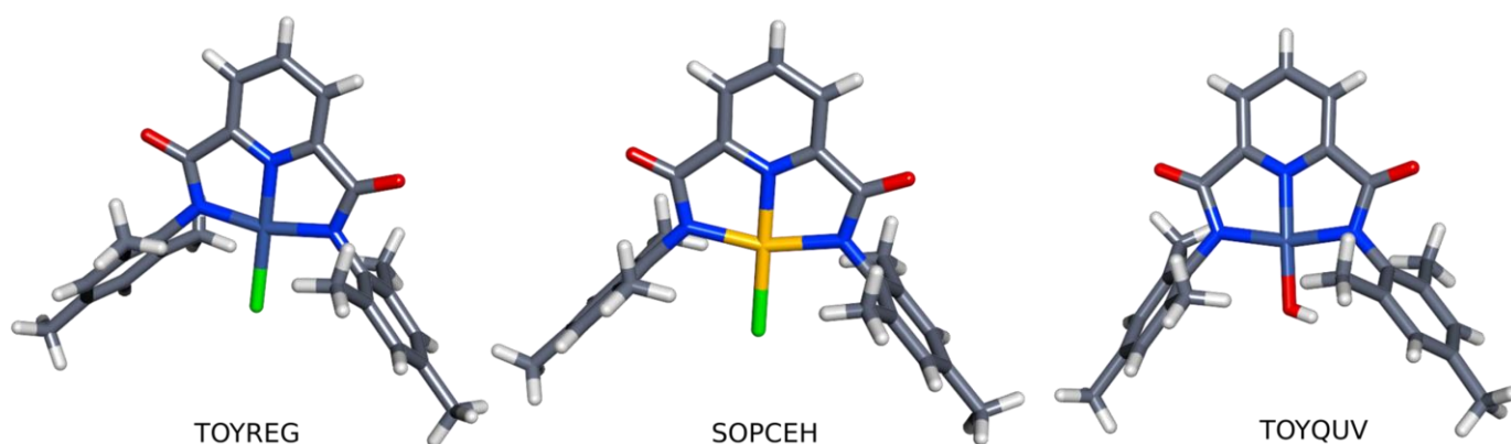
Figure 3.14. Crystal structures of TOYREG, TOYQUV and SOPCEH. TOYREG and TOYQUV are Ni(II) chelates of 1 and SOPCEH is a Au(III) chelate of 1 . The locations of the conformations of these structures on the surfaces shown in Figures 3.10 and 3.11 are indicated.
