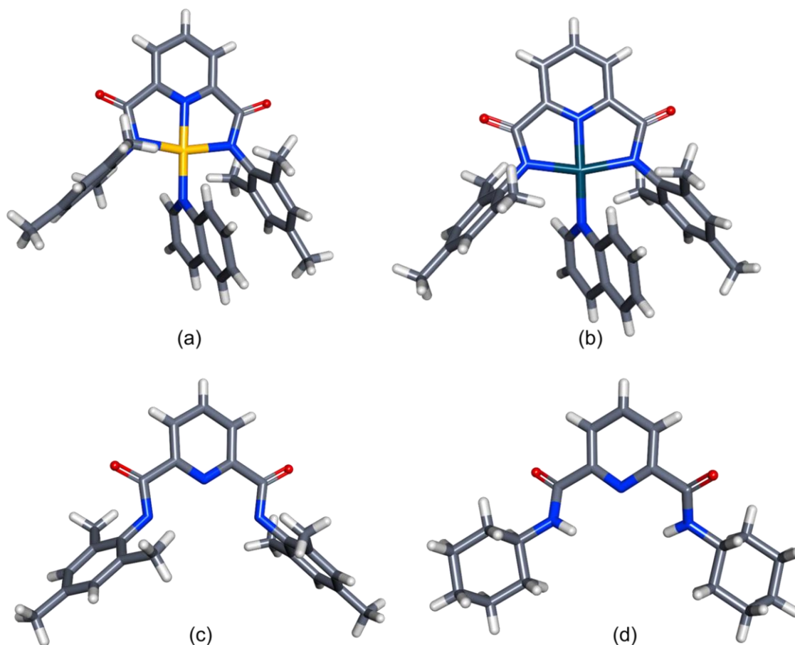
Figure 5.1. Diagram showing the compounds that have been synthesised during this dissertation. (a) N,N' -bis(2,4,6-trimethylphenyl)-2,6-pyridinecarboxamidato(quinoline)Au(III), (b) N,N' -bis(2,4,6-trimethylphenyl)-2,6-pyridinecarboxamidato(quinoline)palladium(II), (c) N,N' -Bis(2,4,6-trimethylphenyl)-2,6-pyridinedicarboxamide ( H_2L1 ) and (d) N,N' -Bis(cyclohexyl)-2,6-pyridinedicarboxamide ( H_2L2 ).
