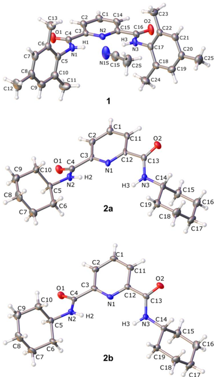
Figure 3.1: Thermal ellipsoid plots (50% probability surfaces) for the low-temperature X-ray structures of 1 and 2 . The atom numbering schemes are included. The structure of 2 comprises two independent molecules in the asymmetric unit (ASU); these are shown separately as 2a and 2b . Hydrogen atoms have been rendered as spheres of arbitrary radius.
