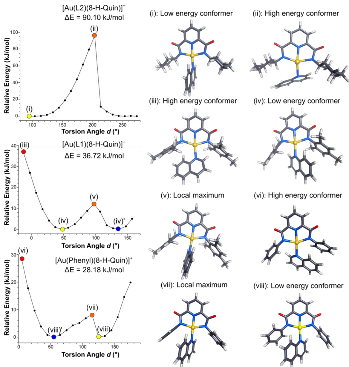
Figure 4.12. Diagram showing the energy profile of quinoline rotamers for [Au(L1)(8-H-Quin)] + , [Au(L2)(8-H-Quin)] + , [Au(Phenyl)(8-H-Quin)] + . The relative energy (kJ mol -1 ) of the conformer has been plotted against the quinoline ligand's torsion angle (°), d (see Figure 4.11 for torsion angle d ). Torsion angles: (i), 94.13°; (ii), 204.13°; (iii), -12.68°; (iv), 47.32°; (v), 97.32°; (vi), 4.63°; (vii), 54.63°; (viii), 114.63°. Note conformers or rotamers (viii)' and (iv)' are slightly higher energy structures, but can essentially be seen as being degenerate to conformers (viii) and (iv), respectively.
