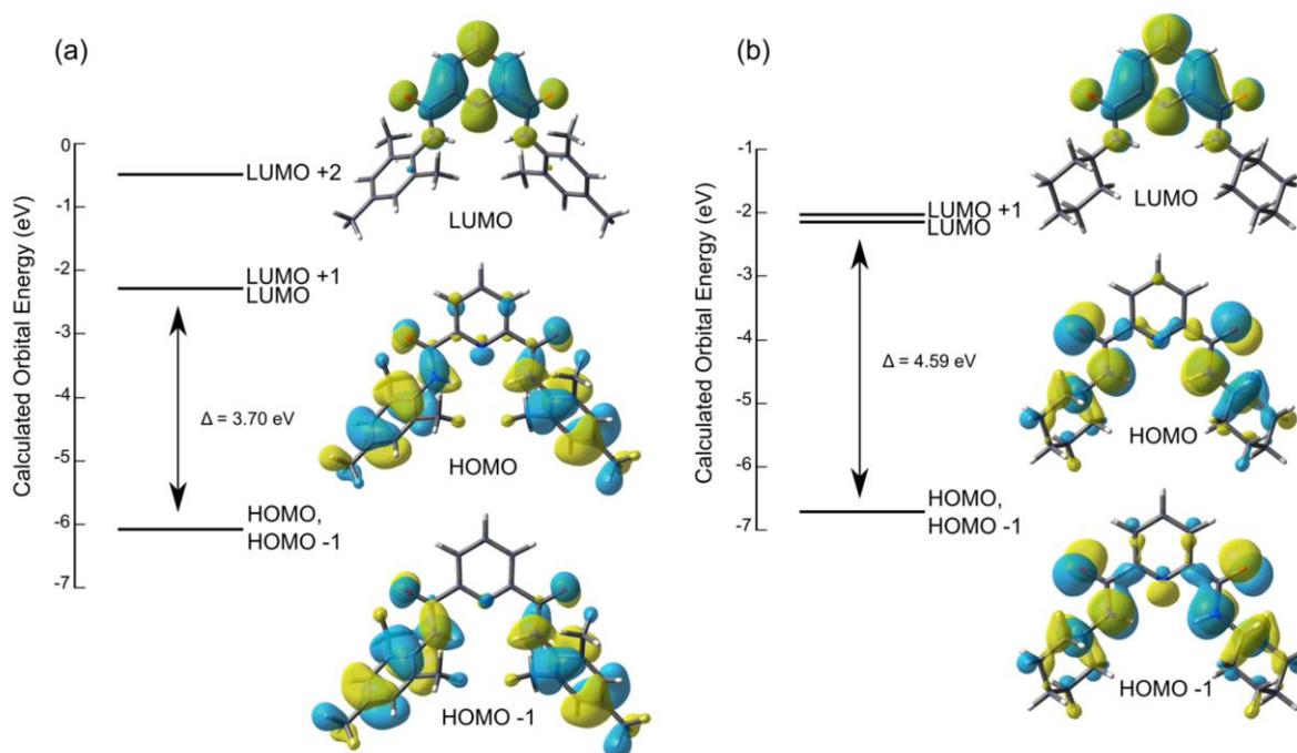
Figure 3.9. (a) DFT-calculated molecular orbital diagram for compound 1 . The HOMO-LUMO gap is 3.70 eV. (b) DFT-calculated molecular orbital diagram for compound 2 . The HOMO-LUMO gap is 4.59 eV.
