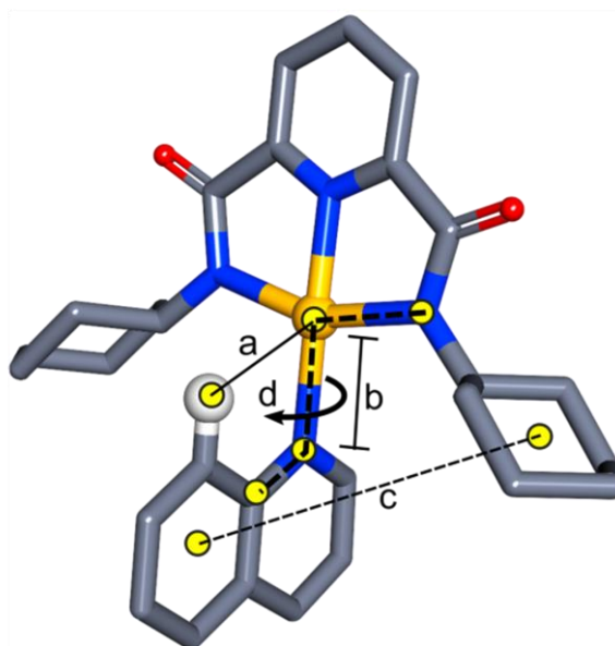
Figure 4.11. Diagram defining the main structural features that were systematically analysed for a series of Au(III) pincer complexes. The structure of [\text{Au}(\text{L2})(\text{Quin})]^+ has been used for illustration: (a) \text{M}\cdots\text{Q} distance, l ; (b) \text{M}-\text{N}_{(\text{Quin})} distance; (c) Inter-centroid distance; (d) Torsion angle defining the orientation of the quinoline ligand, d . The electron density at the bond critical point along a, \rho(\text{M}\cdots\text{Q}) , was obtained from AIMAll analysis of the final DFT-calculated geometry and electron density of the system; the location of the bond critical point (BCP) was structure-dependent.
