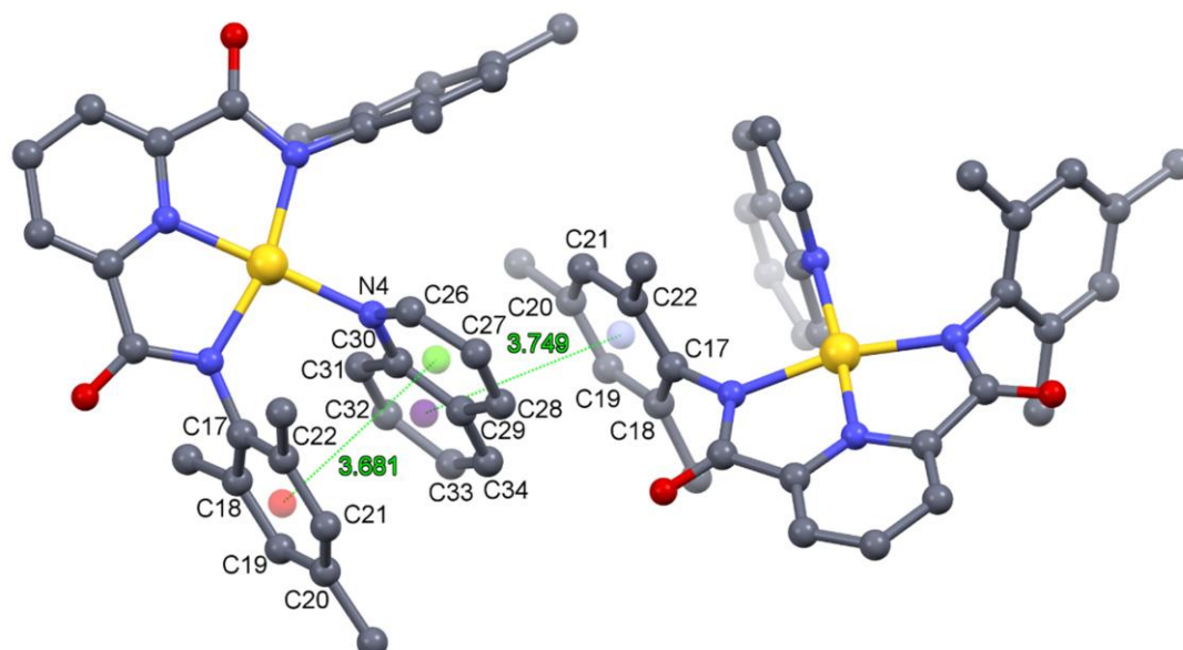
Figure 4.6. Partly labelled diagram illustrating the packing between two [Au(L1)(Quinoline)] + cations. The quinoline ligand of the left structure [symmetry code: x , y , z ] is \pi -stacked with the mesityl ring of the neighbouring molecule [symmetry code: -0.5+x , 0.5-y , z ] in the lattice. Ring centroids are illustrated as coloured spheres; distances between selected centroids are in Å. H atoms have been omitted for clarity.
