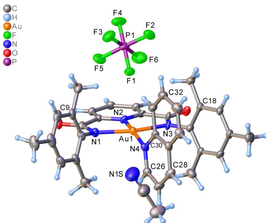
Figure 4.4. Thermal ellipsoid plot (30% probability surfaces) of the [\text{Au}(\text{L1})(\text{Quinoline})][\text{PF}_6] \cdot (\text{CH}_3\text{CN}) crystal structure showing selected atom labels from the crystallographic numbering scheme. Hydrogen atoms have been rendered as spheres of arbitrary radius.
