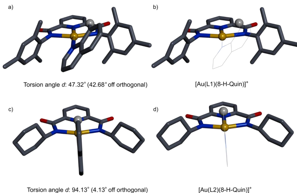
Figure 4.20. Diagram showing the variation in the orientation of the quinoline substituent. This has been quantified by examining torsion angle d for the conformers of the \text{Au}(L1) and \text{Au}(L2) series. Similar quinoline orientation trends are seen for the \text{Pd(II)} and \text{Pt(II)} congeners. For Parts b) and d), the quinoline group has been displayed as wire for visibility. All hydrogen atoms have been omitted for visibility, with the exception of hydrogen atoms that interact with the metal. Note that when torsion angle d = 90^\circ , the plane of the quinoline will be orthogonal to the \text{AuN}_4 square plane.
