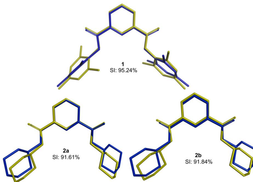
Figure 3.4: A comparison between the DFT-calculated (yellow) and the X-ray crystal structure (blue) of compounds 1 and 2 . The crystallographically-independent molecules of 2 are shown separately as 2a and 2b . Hydrogen atoms excluded for visibility. SI values: 1 : 95.24 % 2a : 91.61 % 2b : 91.84 %
