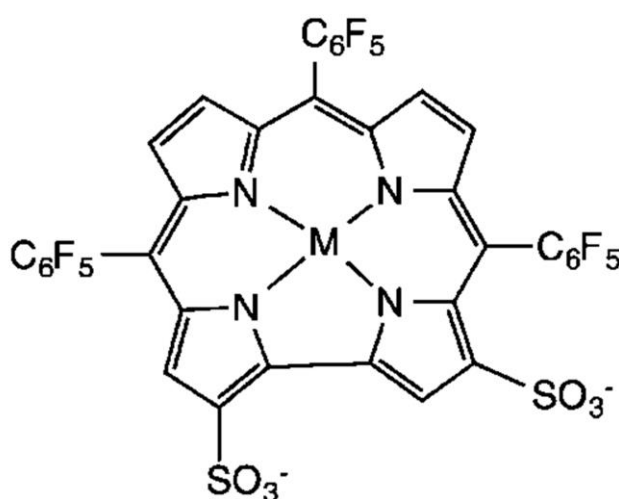
Figure 1.1. Diagram of a Au(III) corrole, synthesized by Teo et al. 9 This complex exhibited high cytotoxicity towards cisplatin-resistant cancer cells. In this case M = Au(III), but other suitable metals include: Fe, Mn, Al and Ga.
