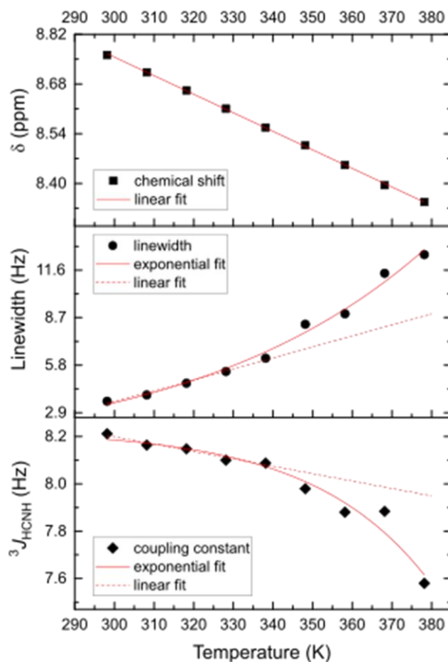
Figure 3.18. Plots of temperature vs ^3J_{\text{HCNH}} , linewidth and shift value for the variable temperature ^1\text{H} NMR experiment. This study was performed at a constant concentration of 0.0228 M.
