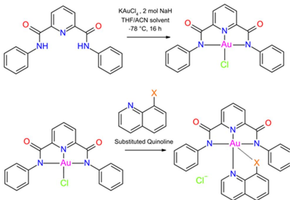
Figure 1.5. An example of a proposed synthesis ( Chapter 4 ) that was based on the synthesis done in the literature method outlined by Johnson et al. 12
