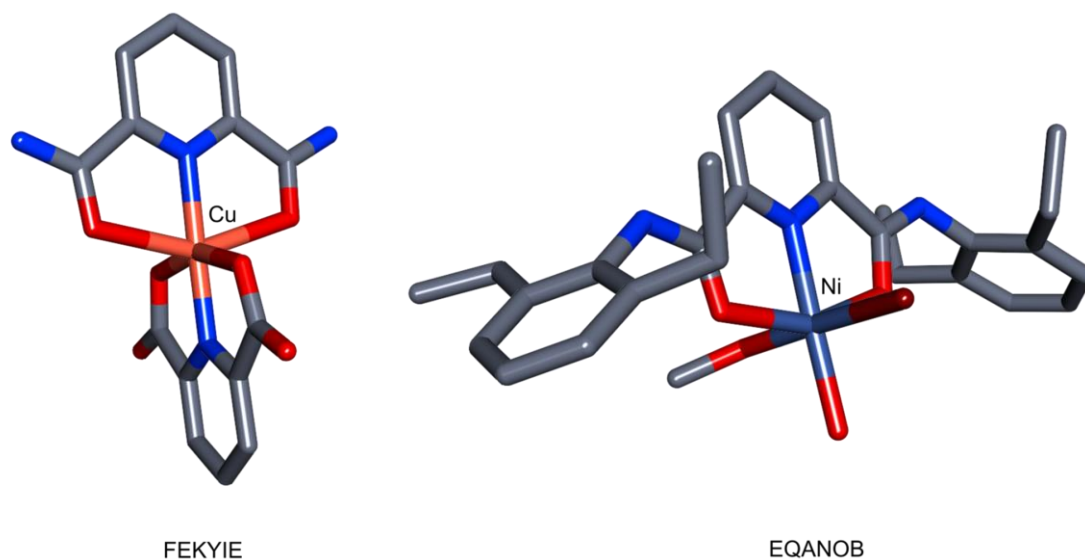
Figure 3.7: Crystal structures of EQANOB and FEKYIE. These are examples of coordination complexes which exhibit an exo|exo conformation (with respect to the amide group).
