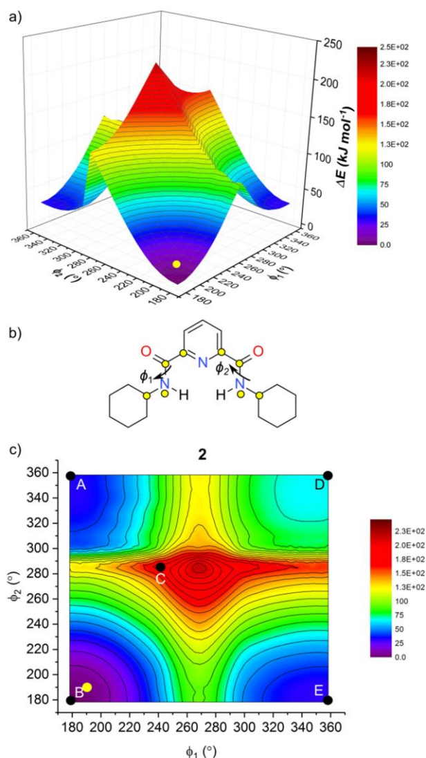
Figure 3.13. a) Three-dimensional plot showing the variation in the relative heat of formation, \Delta E , of 2 as a function of the torsion angles \phi_1 and \phi_2 . The angular coordinates locating the crystal structure are shown as a yellow sphere ( \phi_1 = 170.6^\circ , \phi_2 = -171.2^\circ , \Delta E = 1.7 \text{ kJ mol}^{-1} ).
