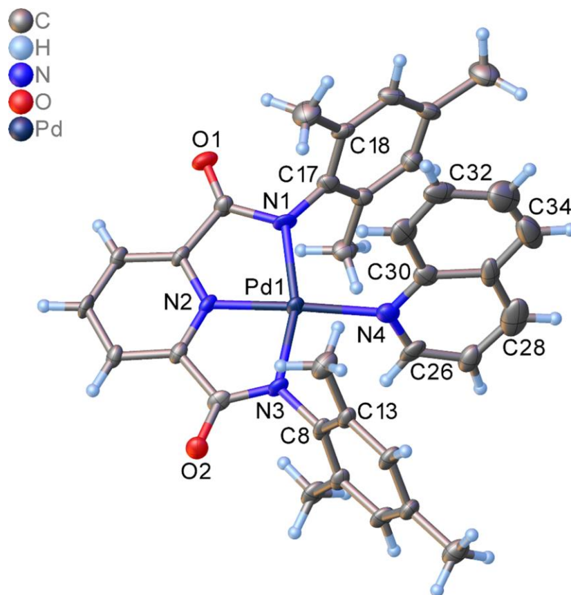
Figure 4.7. Thermal ellipsoid plot (25% probability surfaces, 296 K) of the Pd(L1)(Quinoline) crystal structure showing selected atom labels from the crystallographic numbering scheme. Hydrogen atoms have been rendered as spheres of arbitrary radius. Solvent (acetonitrile) is associated with the structure, but due to disorder and diffuse electron density was omitted using solvent masking in OLEX2. Two voids (each corresponding to 967.6 Å 3 ; 368.6 electrons) exist in the asymmetric unit at (0.000, 0.000, -0.986) and (0.500, 0.500, -0.402).
