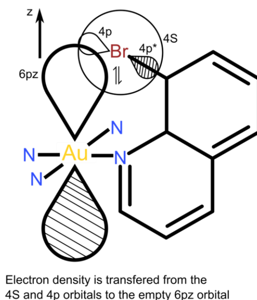
Figure 4.25. Diagram illustrating the nature of the side-on M\cdots Br interaction in the Au(Lx)(8-Br-Quin)]^+ structure. Electron density is transferred from the diffuse 4s orbital of Br into the 6p_z orbital of Au(III) .
