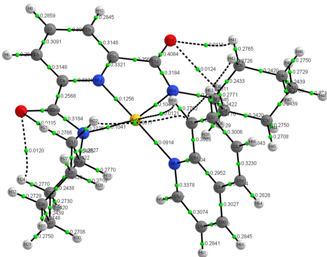
Figure 4.15. AIMAll output of the calculated structure of [\text{Au}(\text{L2})(8\text{-H-Quin})]^+ . The green dots are bond critical points and the number adjacent to the dots is the \rho value (electron density) at that point. In this case, the \rho(\text{M}\cdots\text{Q}) (where \text{Q} = \text{H} ) value is 0.0121 au.
