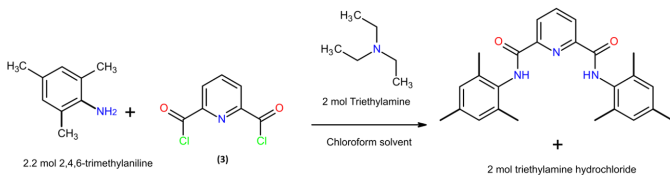
Figure 1.6. The proposed synthesis for ligands in this dissertation. The synthesis was based on the work of by Shimada et al. 57 as expounded in Chapter 3.
