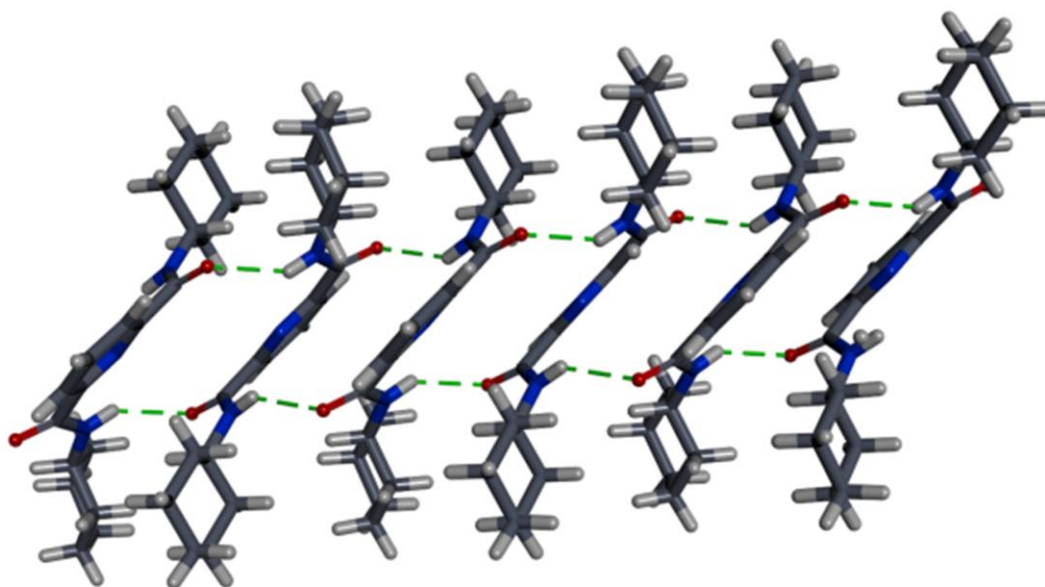
Figure 3.3. Packing diagram showing the intermolecular interactions between molecules of a dimer of 2 . Hydrogen bonds have been shown green. The distance of the O_{\text{(carbonyl)}} \cdots N_{\text{(amide)}} interaction alternates between 2.229 Å to 2.231 Å with each subsequent addition to the one-dimensionally bonded sequence.
