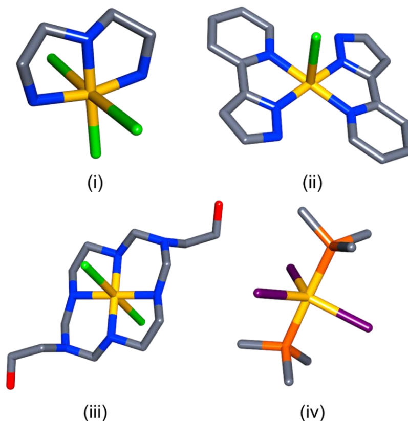
Figure 4.2. Diagram showing examples of structures obtained from the CSD, where the \text{Au(III)} ion is associated with non-coordinating, electron-rich groups. Hydrogen atoms have been omitted for visibility. Crystal structures of DODXID (i), NURYAB (ii), TEMMED (iii), and TUBBOH (iv) are shown.
