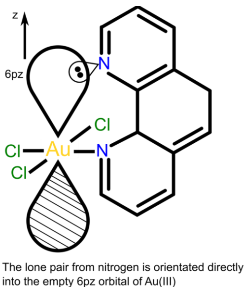
Figure 4.26. Diagram illustrating the ionic Au \cdots N interaction that is present in the CDMPAU structure. The 1,10-phenanthroline nitrogen is positioned so that the lone pair on the nitrogen is orientated into the 6p z orbital of Au(III).
