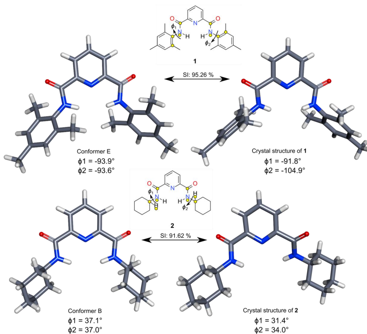
Figure 3.16. Conformational comparison between the global energy minimum conformer E (Scan 1, Figure 3.10), and the crystal structure of 1 , and the Conformational comparison between the global energy minimum conformer B (Scan 1, Figure 3.11) and the crystal structure of 2 .
