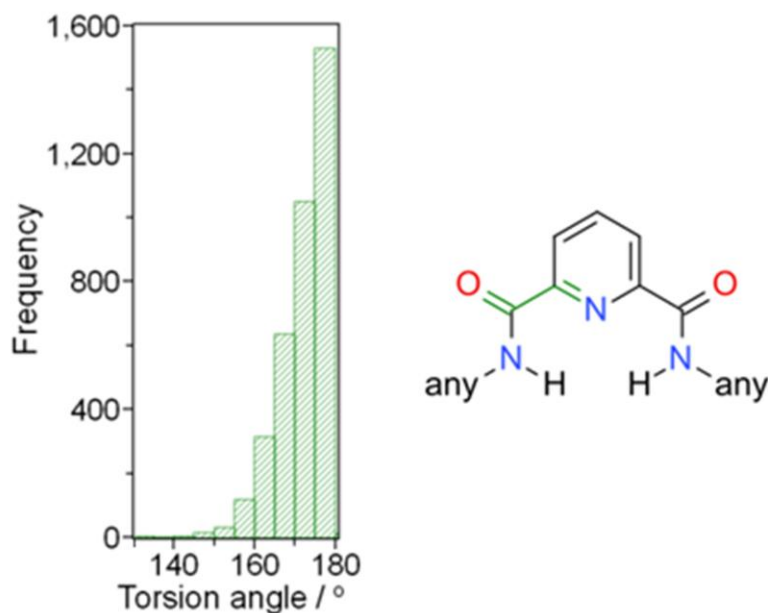
Figure 3.5. MOGUL search of the CSD (up to May 2017) mapping the range of N=C–C=O torsion angles (highlighted in green) in crystallographically characterized bis(amide)-pyridine pincer derivatives. Out of 3721 structures, only 6 have the highlighted torsion angle < 30°. The typical range is 140–180°, with the majority of structures exhibiting a torsion angle between 170–180°. The histogram has been constructed with a 5° bin width.
