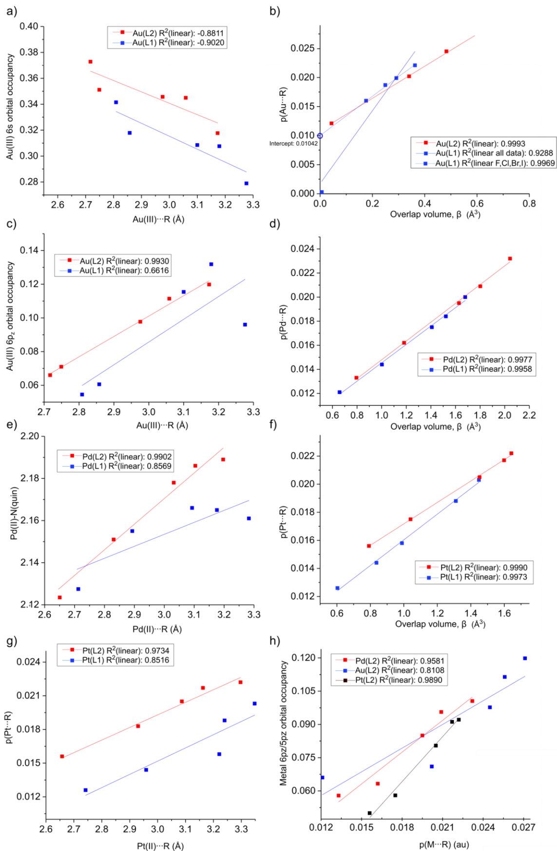
Figure 4.14. Plots of selected data from Table 4.7. These plots are discussed further in Section 4.3.5.1.
