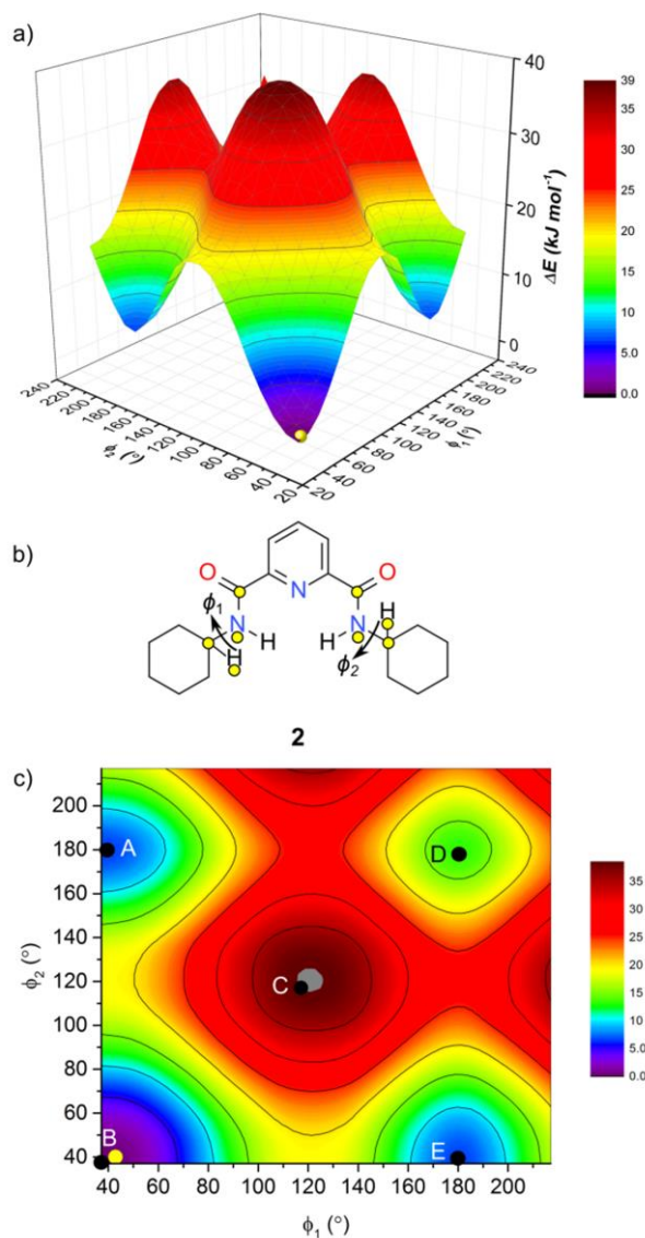
Figure 3.11. a) Three-dimensional plot showing the variation in the relative heat of formation, \Delta E , of 2 as a function of the torsion angles \phi_1 and \phi_2 . The angular coordinates locating the crystal structure are shown as a yellow sphere ( \phi_1 = 42.9^\circ , \phi_2 = 40.1^\circ , \Delta E = 0.1 \text{ kJ mol}^{-1} ).
