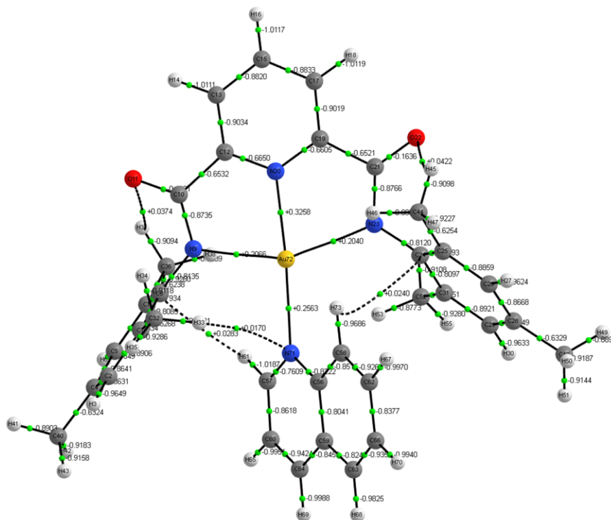
Figure 1.4. Example of an output of an Atoms in molecules (AIM) analysis (performed using the AIMAll software package). The bond critical points have been rendered as green spheres. Solid lines indicate formal bonding, while the dotted lines denote an electrostatic interaction. The numbers adjacent to the bond critical points are the Laplacian of the electron density ( \nabla^2\rho ). However this is just one of the many bond critical point properties that were calculated during the analysis; significantly, the \nabla^2\rho and the electron density ( \rho ) values are most relevant to this work.
