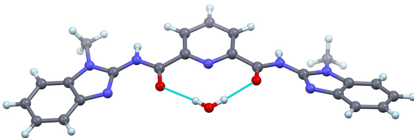
Figure 3.6. One of the independent molecules in the X-ray structure of MILHEV in which an exo|exo conformation for the bis(amide) system is stabilized by the two amide carbonyl oxygen atoms serving as H-bond acceptors to a water molecule.
