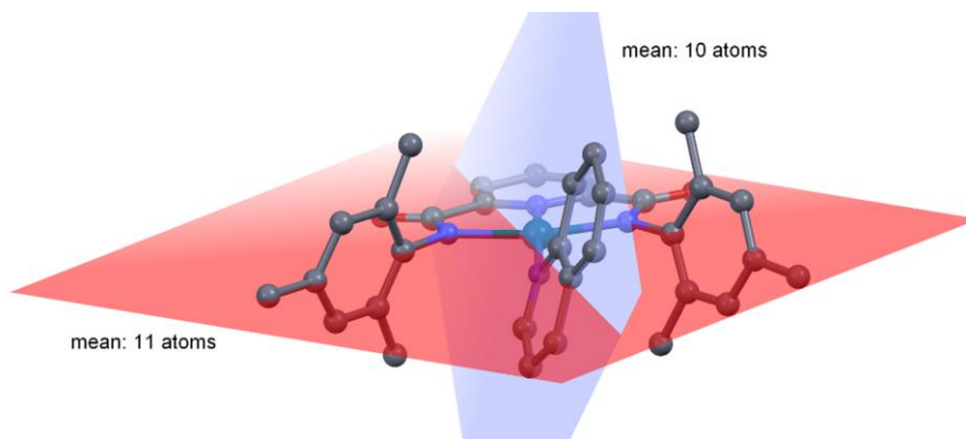
Figure 4.8. Diagram illustrating the least-squares planes between the metal-chelating 11-atom pincer ligand and the 10-atom quinoline ligand plane for Pd(L1)(Quinoline). The dihedral angle between the planes is 68.5°. The Pd(II) ion and three N atoms of the pincer ligand lie approximately in the chelate plane (Pd is displaced only 0.08 Å below the plane), while the quinoline N atom is displaced significantly below the plane (0.41 Å) giving it the appearance of a downward tilt. H atoms have been omitted for clarity.
