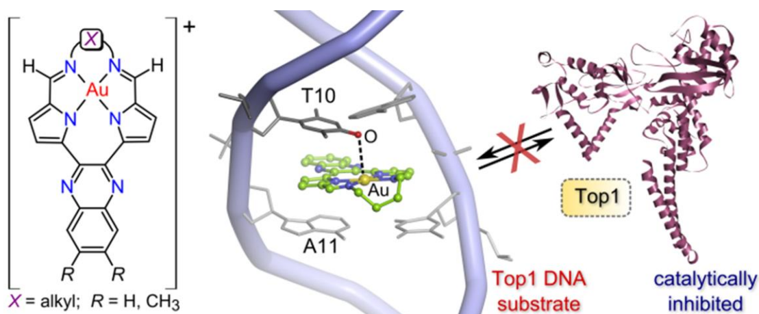
Figure 1.3. A diagram from a paper by Akerman et al. 11 showing that cytotoxic Au(III) macrocycles act as catalytic inhibitors of human topoisomerase I (Top 1). This study showed that this mechanism of action may be traced to the existence of a crucial Au(III)---O=C interaction with the carbonyl group of thymine in the TA base pair targeted by the metallodrug.
