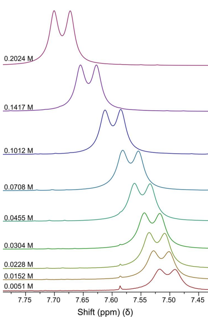
Figure 3.17. Variable concentration ^1\text{H} NMR spectra, taken at a constant temperature of 293.15 K. The plot shows the downfield shift of the N-H amide peak with increasing concentration.
