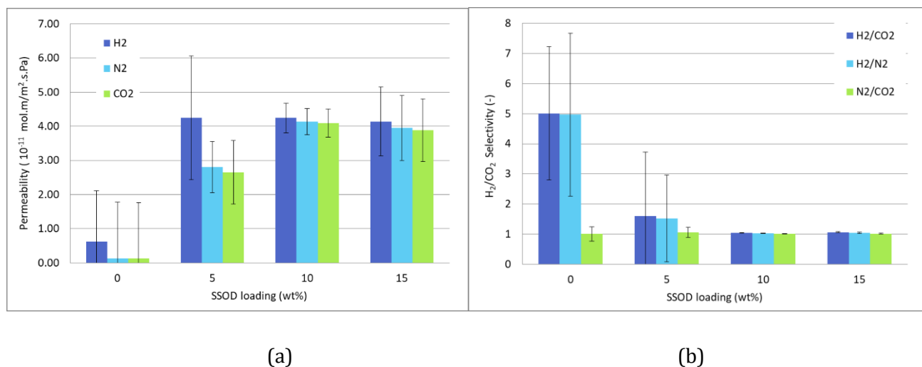
Figure 39: Effect of silica sodalite loading on membrane a) permeability and b) selectivity (1 Bar)
