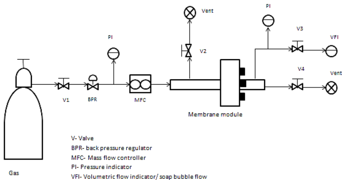
Figure 42: Schematic diagram of membrane gas separation rig
