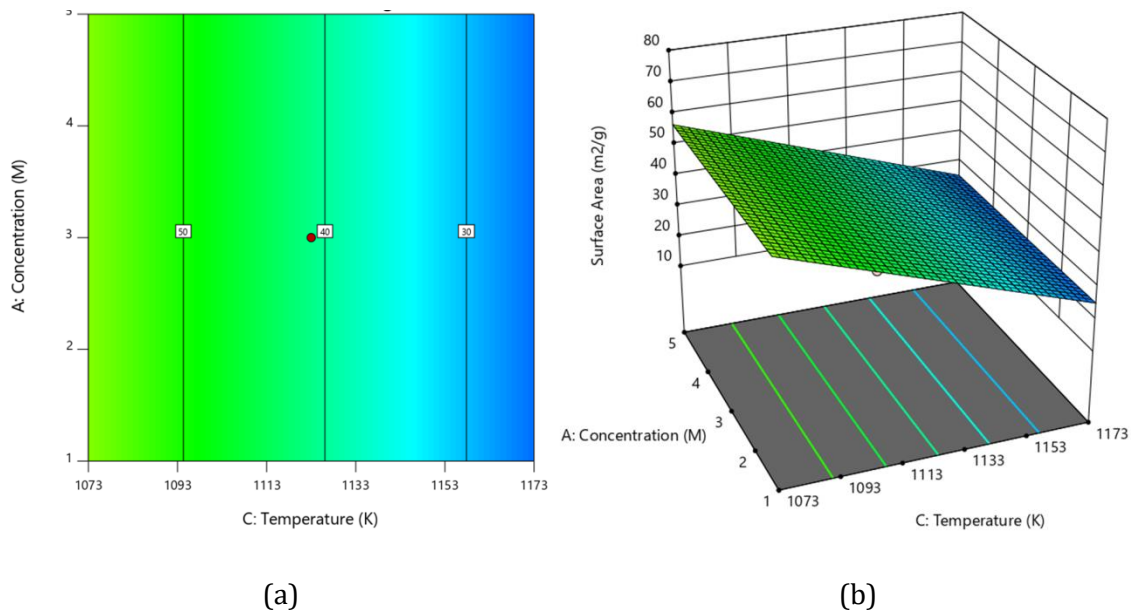
Figure 19: a) Contour and b) response surface plot for acid strength (A) and calcination temperature (C) at B= 95 min
