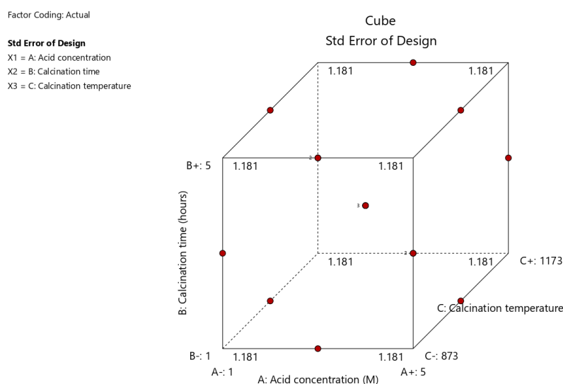
Figure 4: Design space for extended investigation
