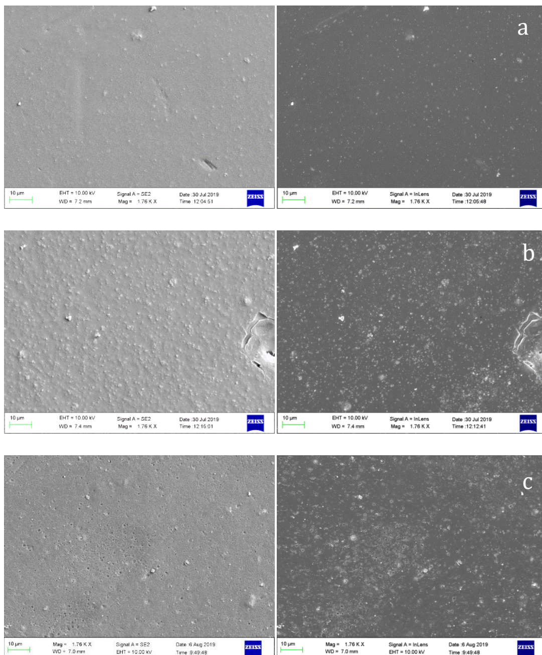
Figure 34: SEM images of membranes surface for SSOD/PSF MMM a) 5 wt. %; b) 10 wt. %; c) 15 wt. % (Mag=1.76 kX) under SE2 (left) and InLense (right) detection.
