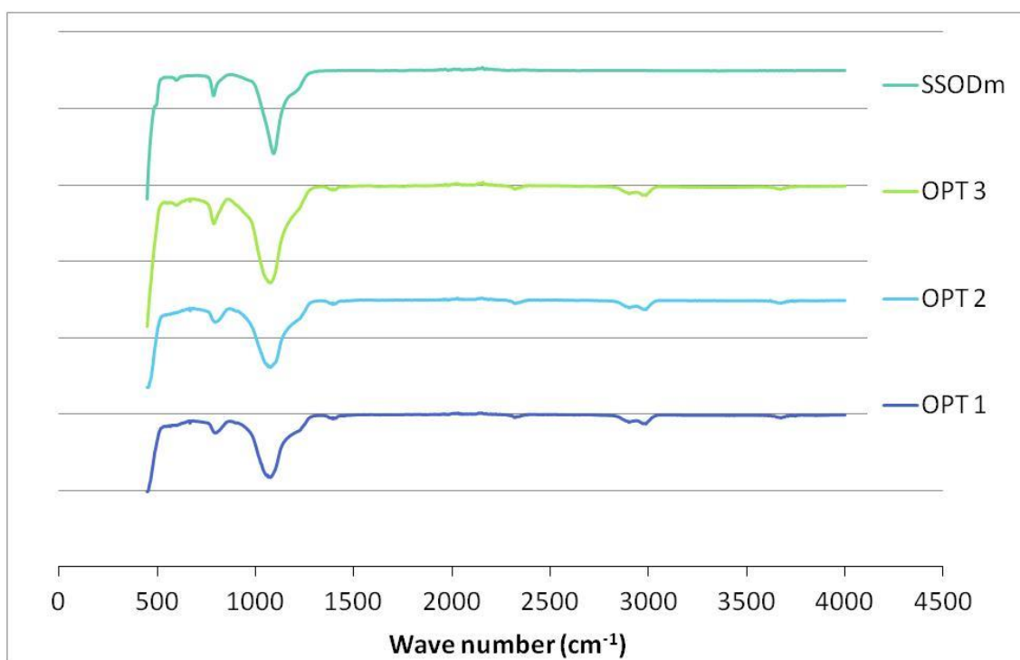
Figure 30: FTIR absorption spectrum for optimized silica sodalite
