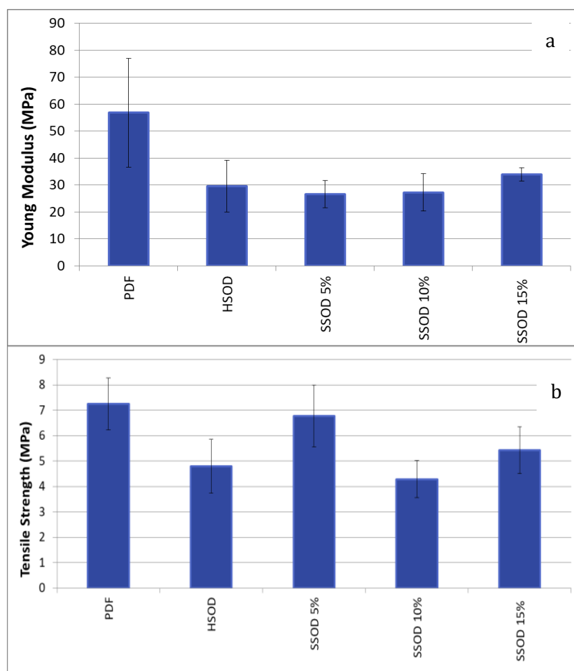
Figure 37: a) Young's Modulus and b) tensile strength for MMMs
