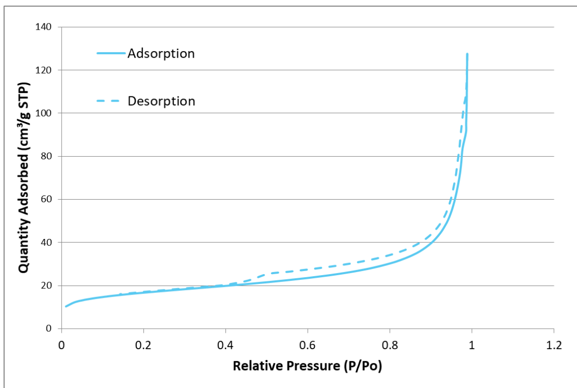
Figure 27: Adsorption isotherm for SSOD m
