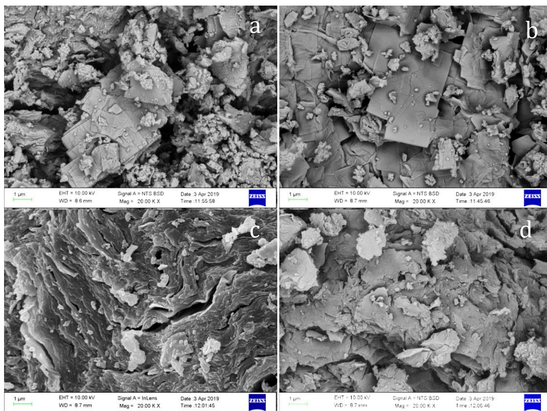
Figure 29: SEM imaging for optimized SSOD; a)OPT1; b)OPT2; c)OPT3 and d)SSODm
