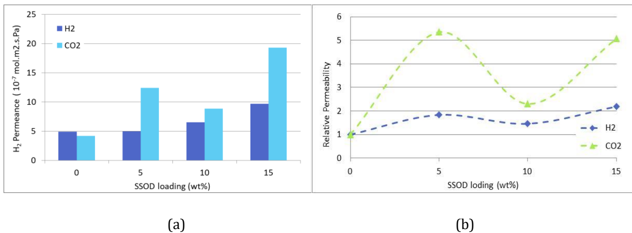
Figure 41: Effect of SSOD loading on a) permeance and b) relative permeability
