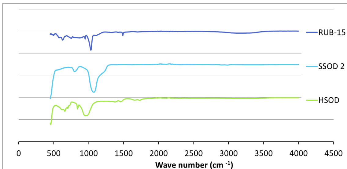
Figure 12: FTIR absorbance spectrum (a.u.) for synthesized samples (preliminary investigation)
