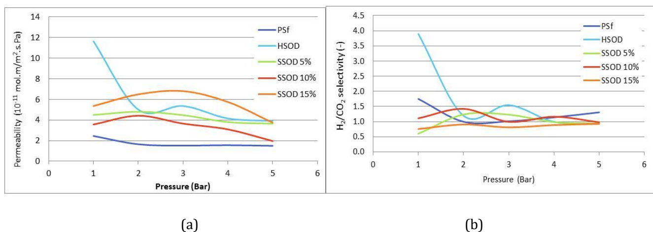
Figure 42: Effect of pressure on MMM a) permeability and b) selectivity
