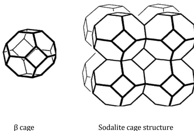
Figure 2: Sodalite framework (International Zeolite Association, 2007; Khajavi, et al., 2007)
