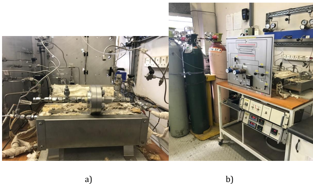
Figure 43: a) membrane module and b) gas separation rig
