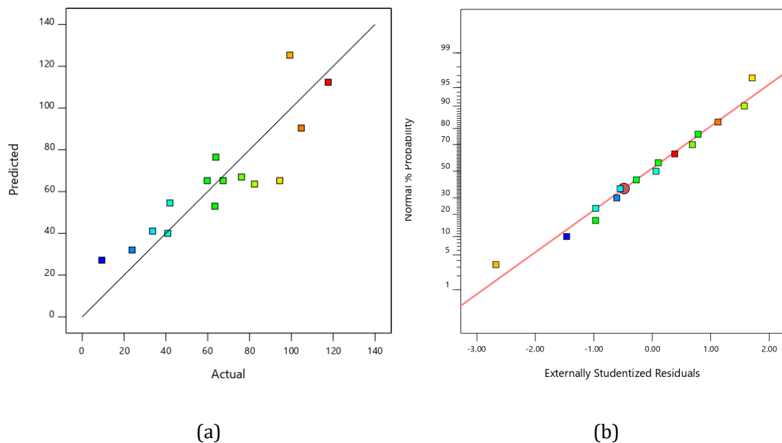
Figure 21: a) Predicted vs actual values; b) Normal plot of residuals
