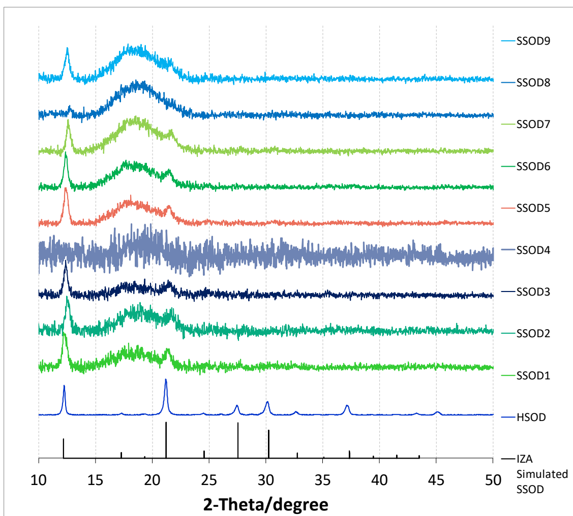
Figure 8: XRD patterns for sodalite samples synthesized in the preliminary investigation
