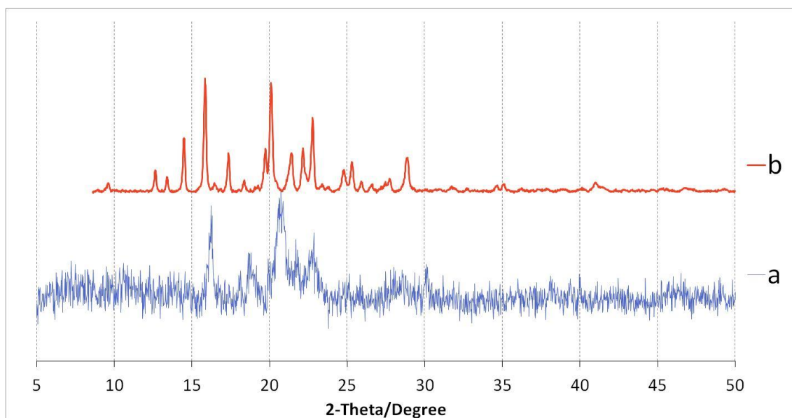
Figure 7: Powder X-ray diffraction patterns for RUB-15 synthesized in a) the preliminary study and b) the extended investigation
