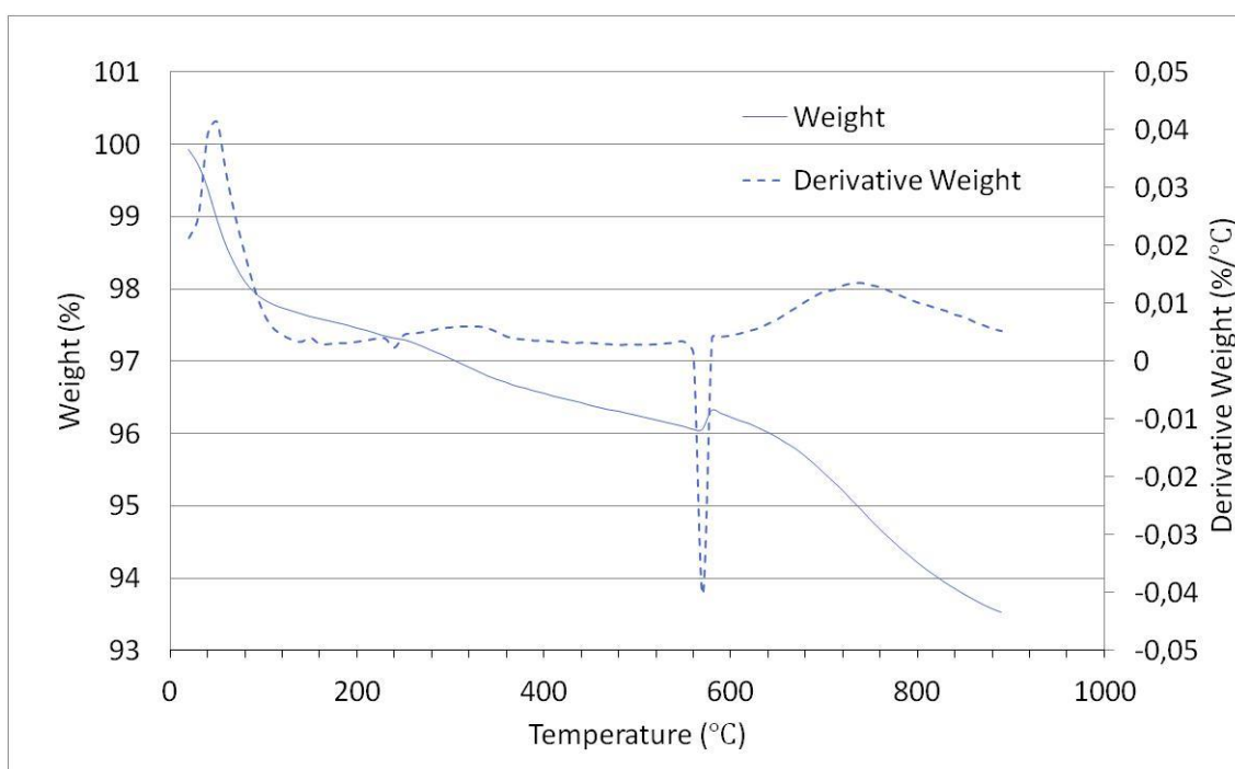
Figure 31: TGA results for SSODm
