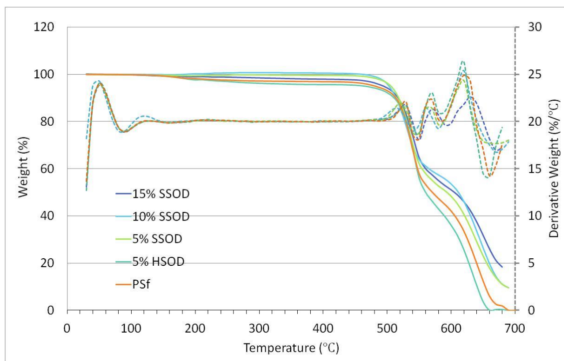
Figure 38: TGA weight (solid) and derivative weight (dashed) graphs for polysulfone mixed matrix membranes
