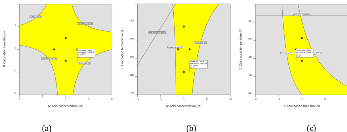
Figure 23: Overlay plots for model factors; a) A&B, b) A&C and c) B&C at optimum conditions
