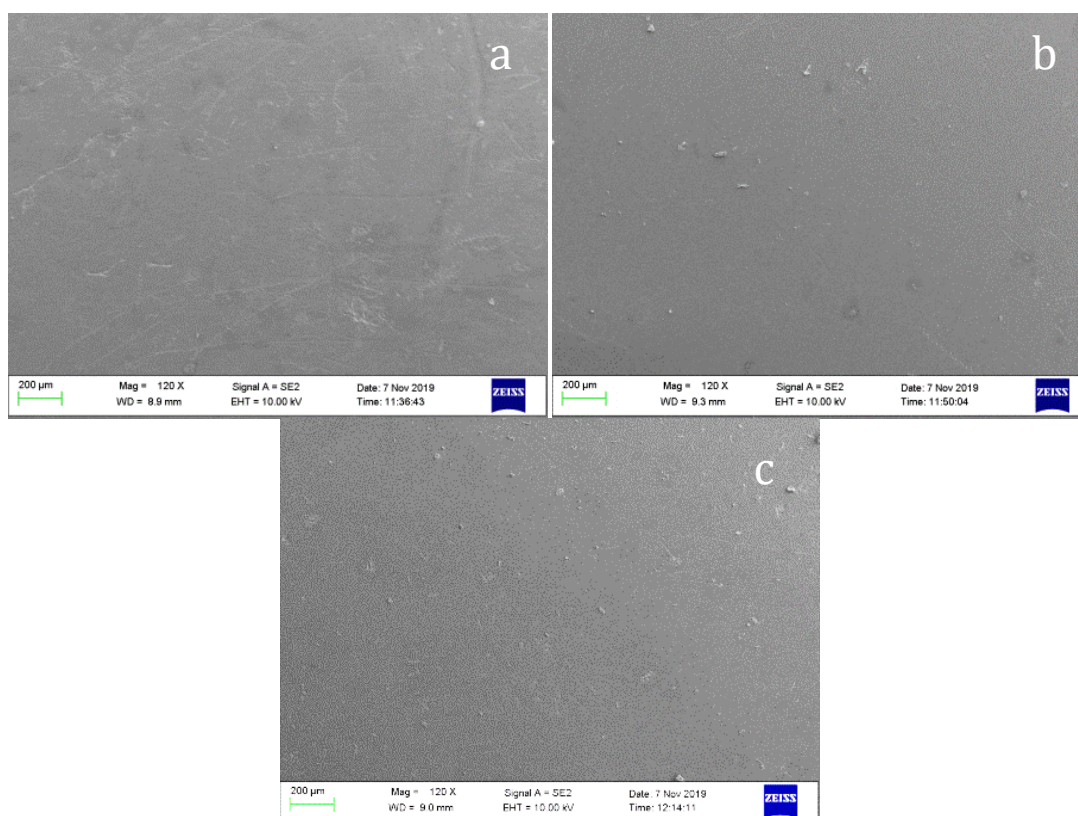
Figure 33: SEM images of membranes surface for a) purely PSF; b) 5wt. % HSOD/PSF ; c) 5wt. % SSOD/PSF MMM's (Mag =120 X)
