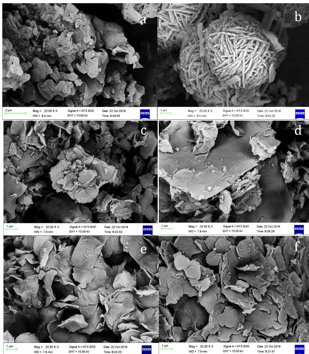
Figure 10: SEM imaging for synthesized samples a) RUB-15; b) HSOD; c) SSOD1; d) SSOD2; e) SSOD3; f) SSOD8
