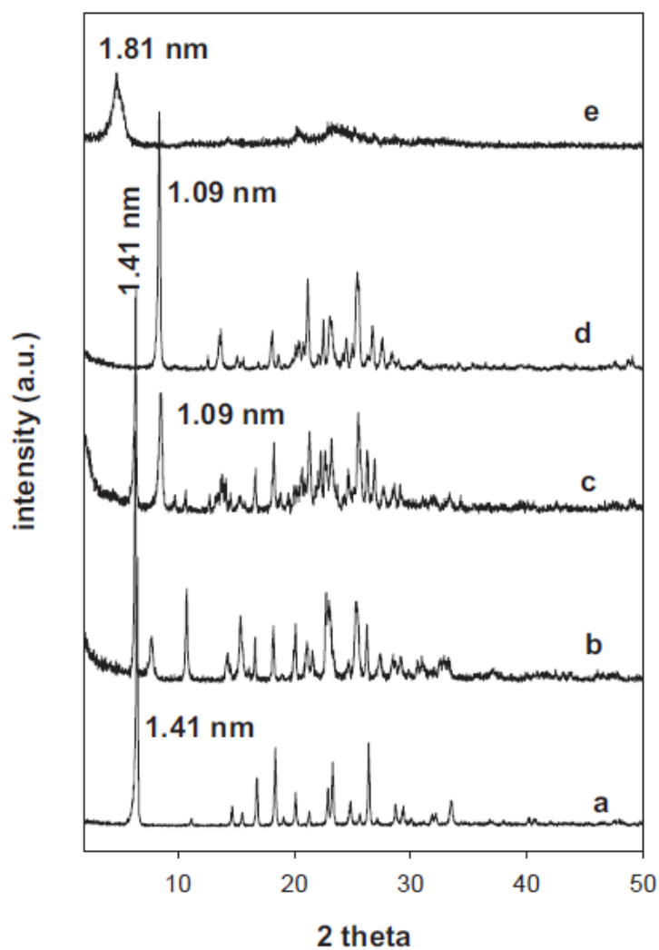
Fig. 2. Powder XRD of H-mag treated with TMAOH.5H 2 O at 150 °C with different amounts of water added. (a) sample 3 (b) sample 8, (c) sample 9, (d) sample 10, and (e) sample 11.
