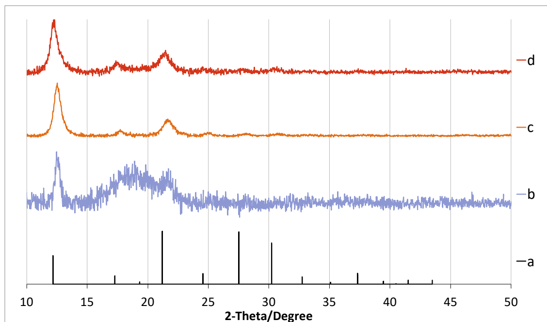
Figure 9: XRD pattern for a) simulated IZA standard; b) Preliminary investigation SSOD 2; c) SSOD 6; d) SSOD 9
