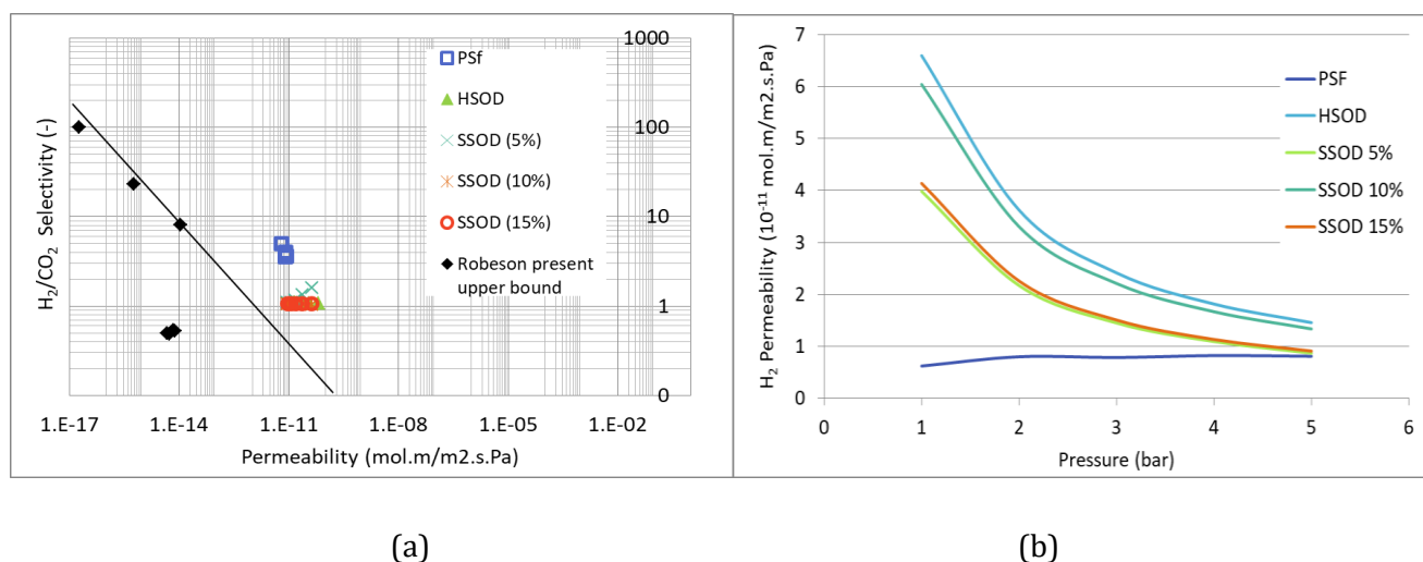
Figure 40: a) Robeson's H 2 /CO 2 boundary and b) Effect of pressure on H 2 permeability
