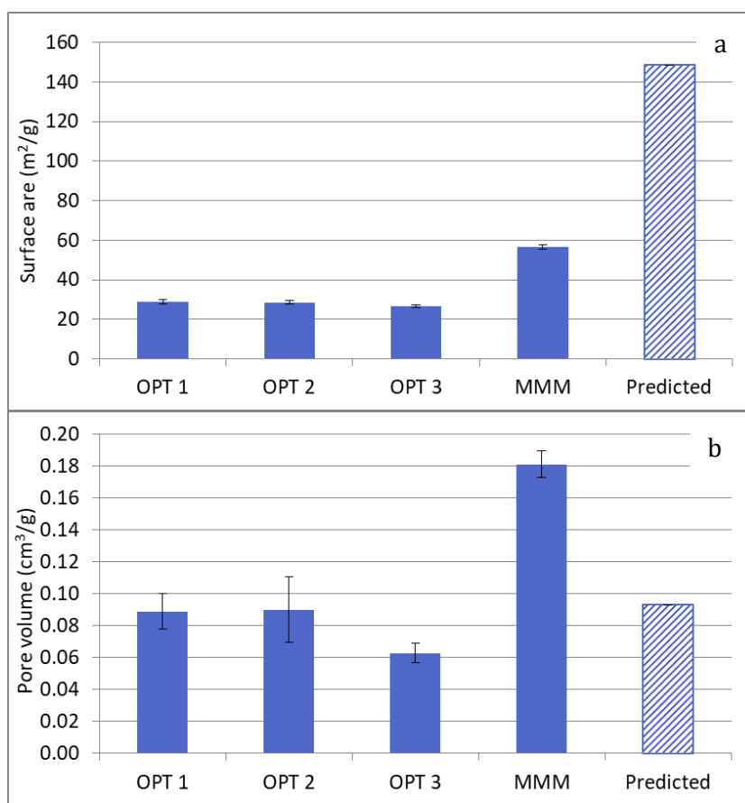
Figure 25: a) SA and b) PV results for optimized SSOD
