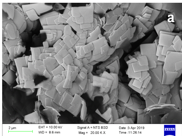
Figure B: SEM imaging for synthesized samples a)RUB-15; b)SSOD6; c)SSOD9; d)OPT1; e)OPT2; f)OPT3; g)OPT4
