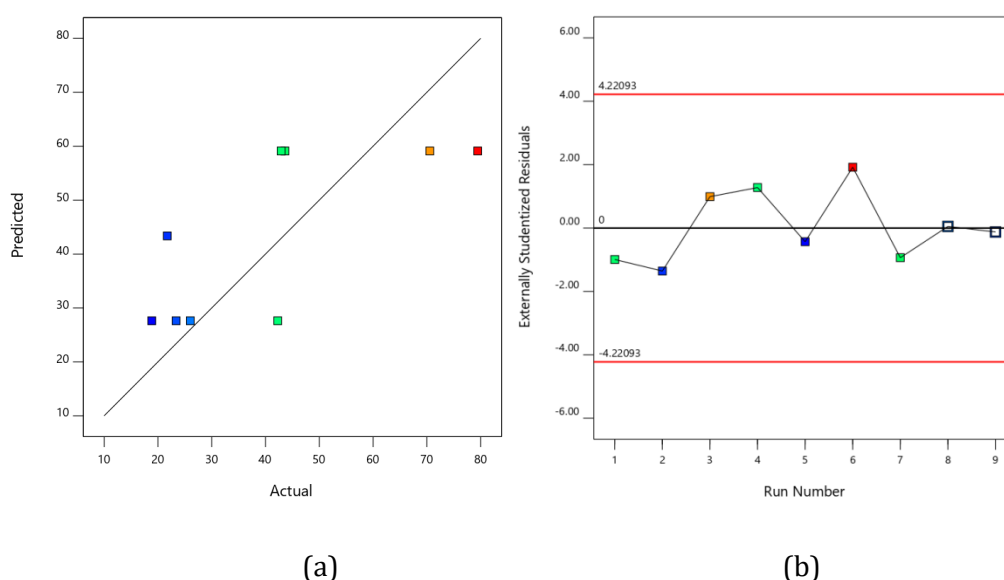
Figure 18: a) Predicted vs. run plot and b) Residual vs. run plot for SA model (factorial design)
