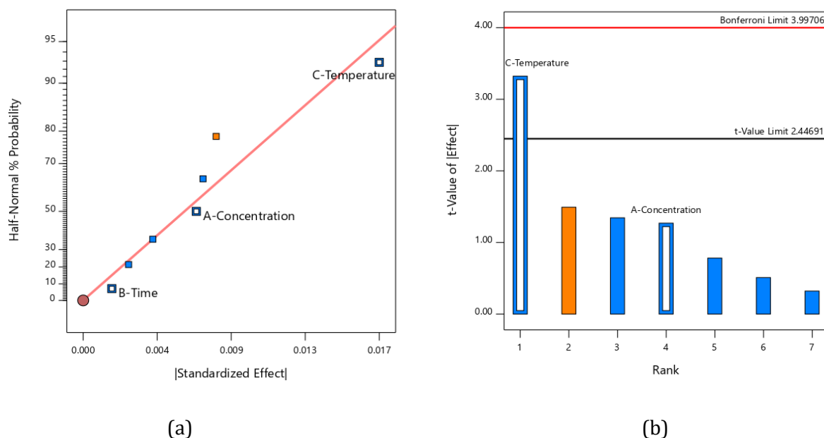
Figure 14: a) Half-Normal and b) Pareto chart for PV model (factorial design)
