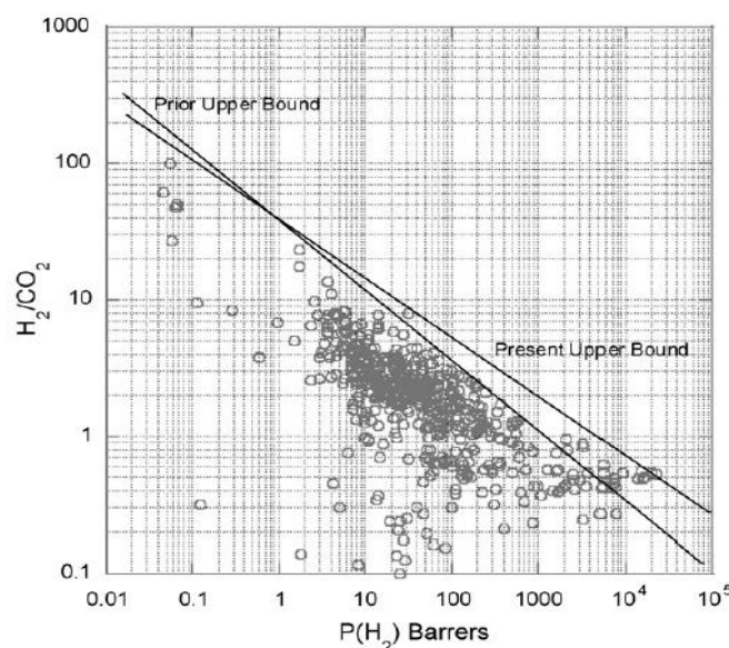
Figure 1: Upper bound correlation for H_2/CO_2 separation (Robeson, 2008)
