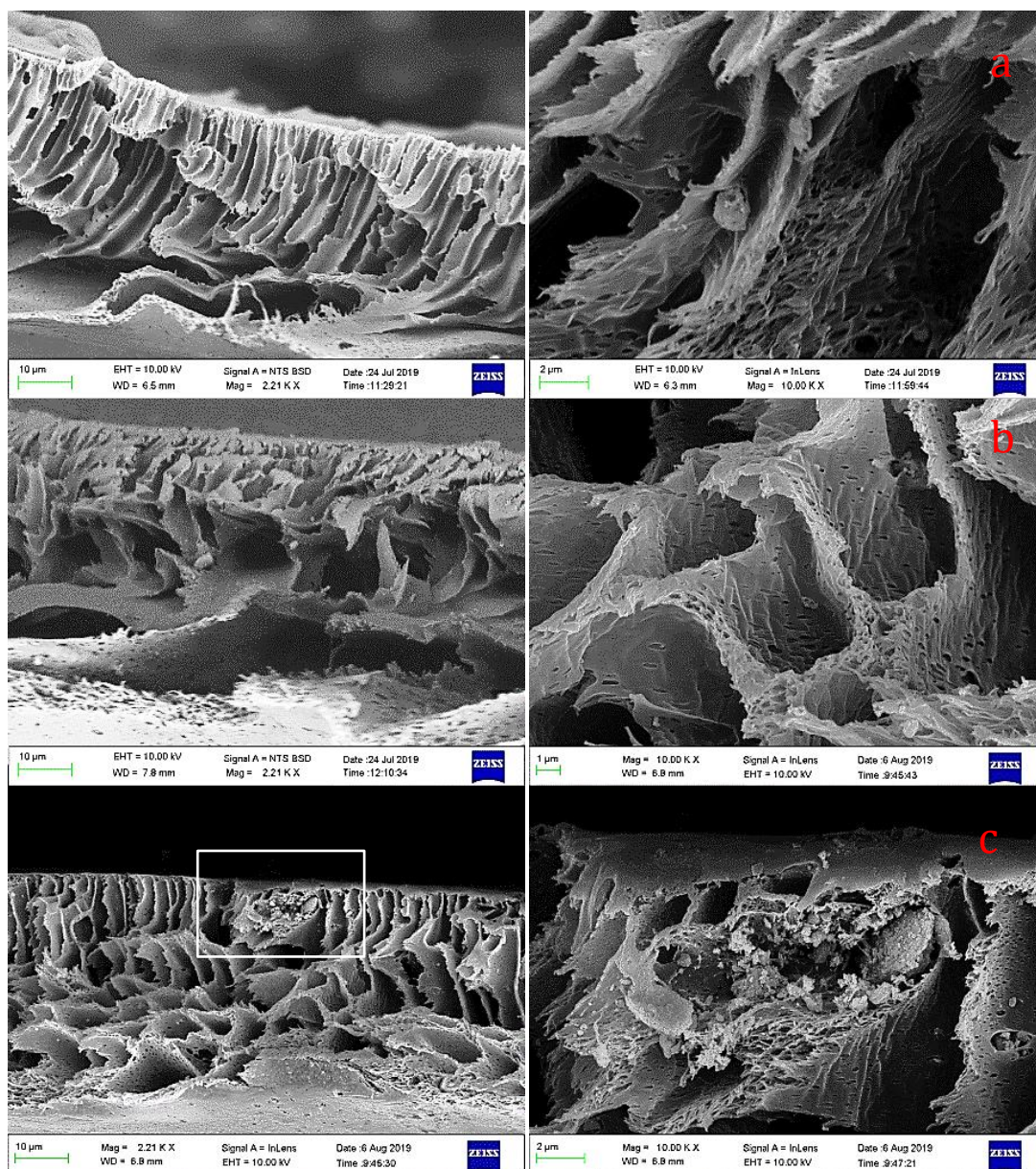
Figure 36: Cross-sectional view of SEM images for SSOD/PSF MMMs at a) 5wt. %; b) 10wt. %; c) 15wt. % at magnifications of 2.21 kX (left) and 10 kX (right), respectively.
