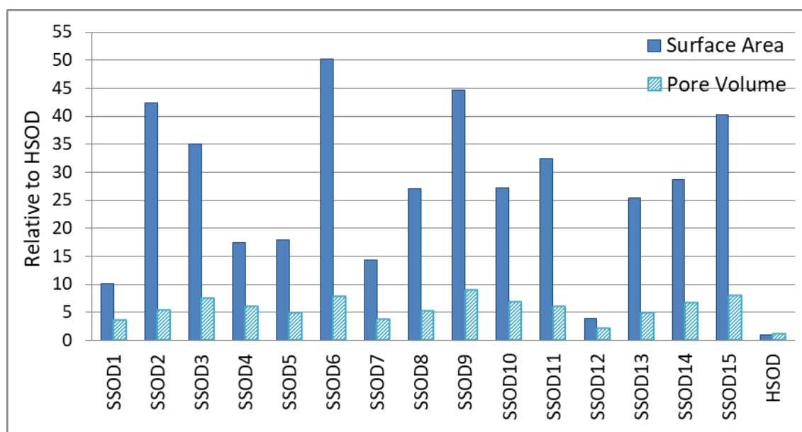
Figure 5: BET surface area and pore volume of SSOD relative to HSOD results
