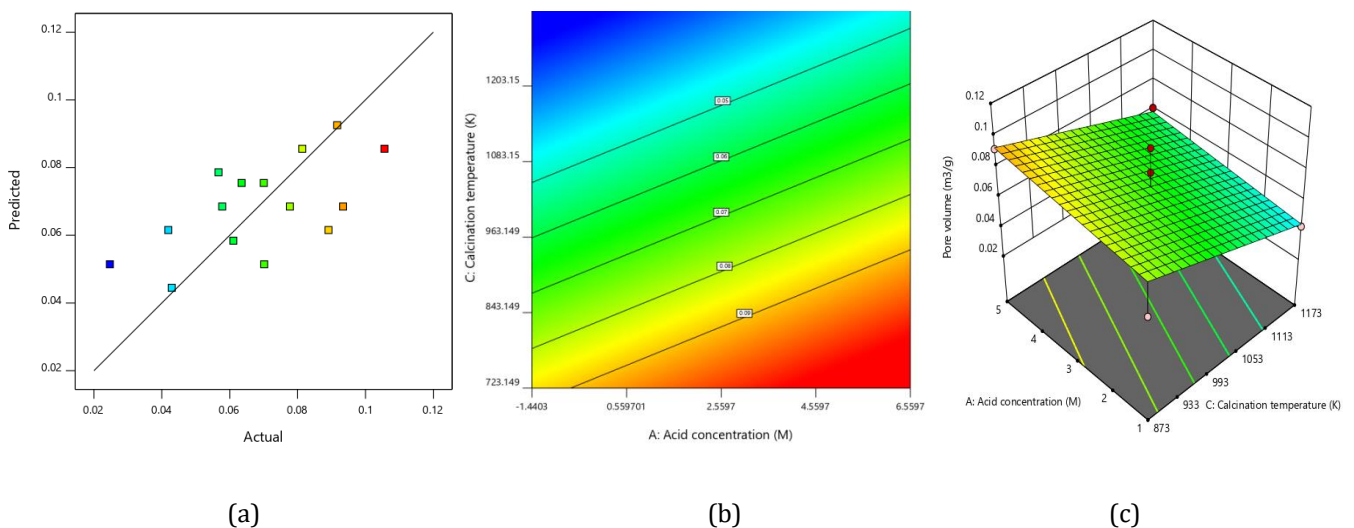
Figure 20: Model graphs a) Predicted vs actual results; b) 2D Contour plot of model terms A and C at B= 3h; c) 3D response surface for model terms A and C at B=3h
