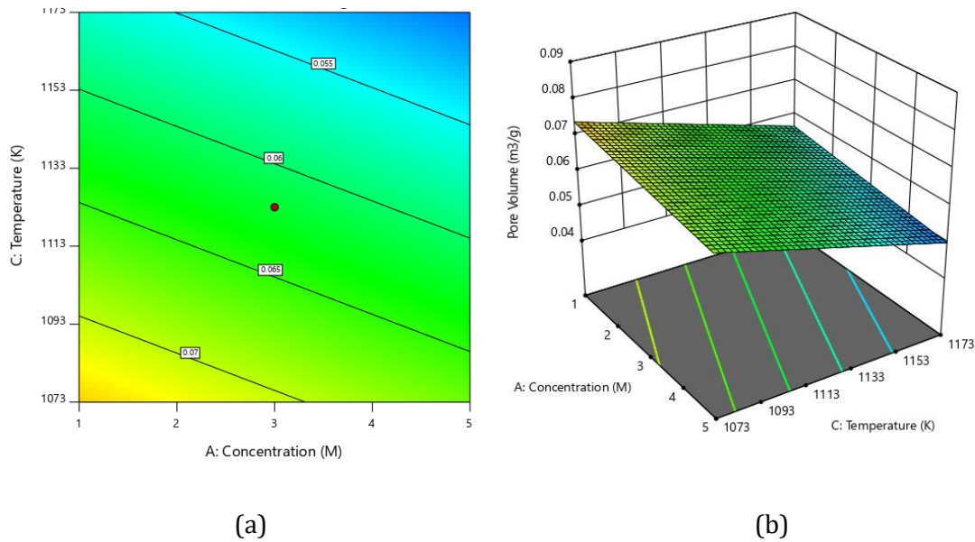
Figure 16: a) contour and b) response surface plot for acid strength (A) and calcination temperature (C) at B= 95 min
