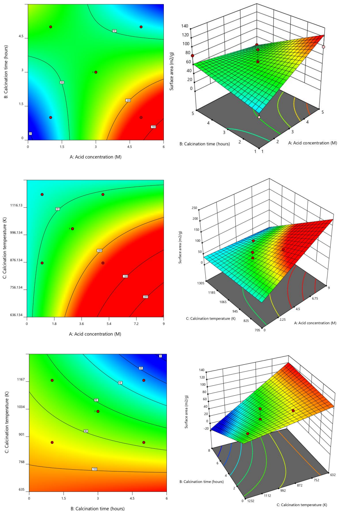
Figure 22: 2D contour plots and 3D response surfaces for model factors A, B and C (third factor not shown is at an intermediate level in each case).
