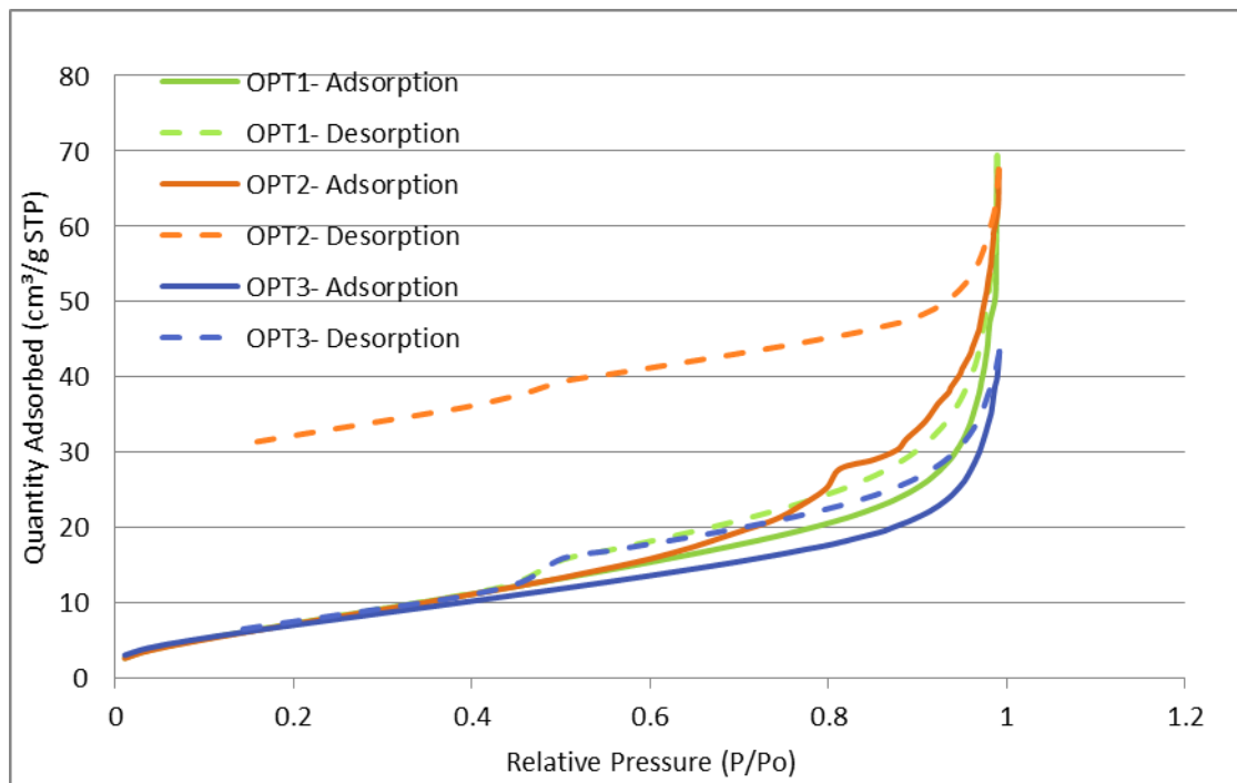
Figure 26: Adsorption isotherms for optimized SSOD
