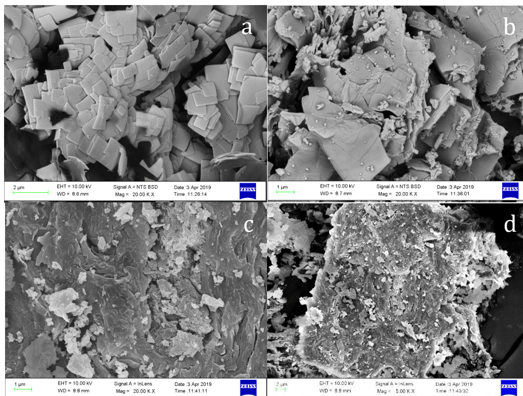
Figure 11: SEM imaging of synthesized samples; a) RUB-15; b) SSOD6; c) SSOD 9 (20kX) and d) SSOD 9 (5kX)
