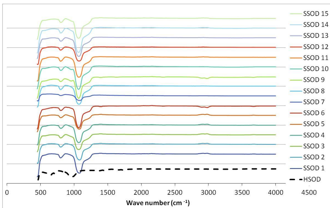
Figure 13: FTIR absorbance spectrum (a.u.) of synthesized sodalite (extended investigation)
