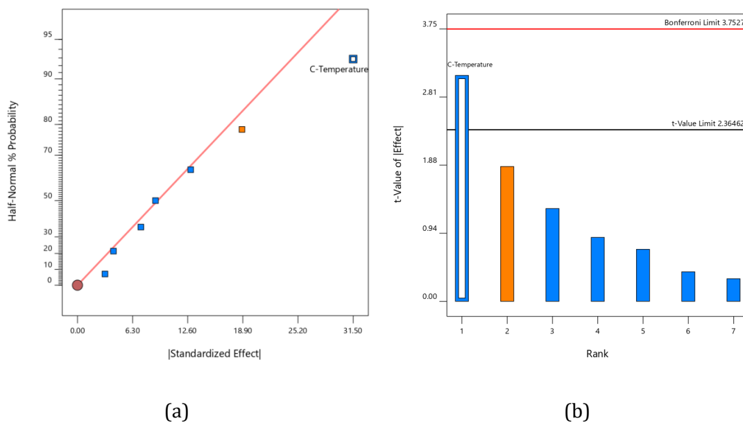
Figure 17: a) half-normal; b) Pareto plots for SA model
