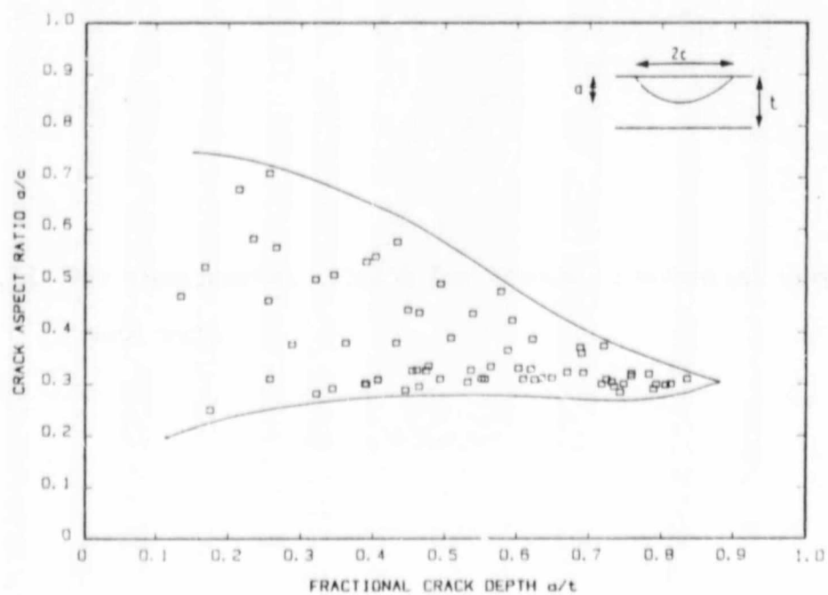
Figure 6.11 The experimental results obtained for the change in crack aspect ratio with fractional crack depth.
