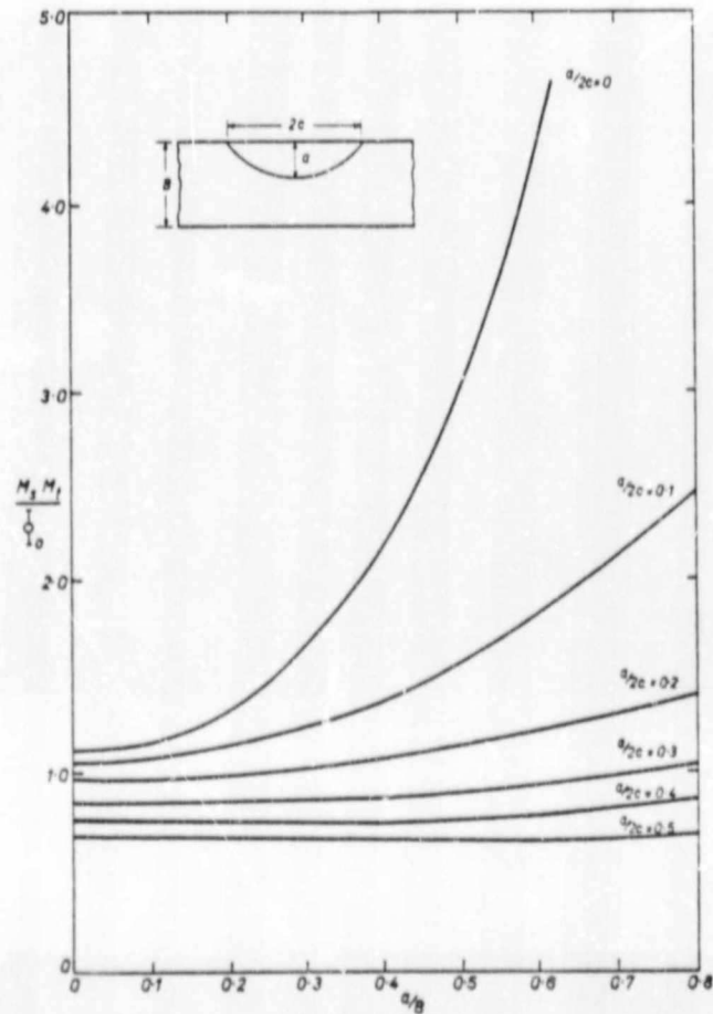
Figure 6.4 Variation of the magnification factor with crack depth for various surface-crack shapes (from (128)).
