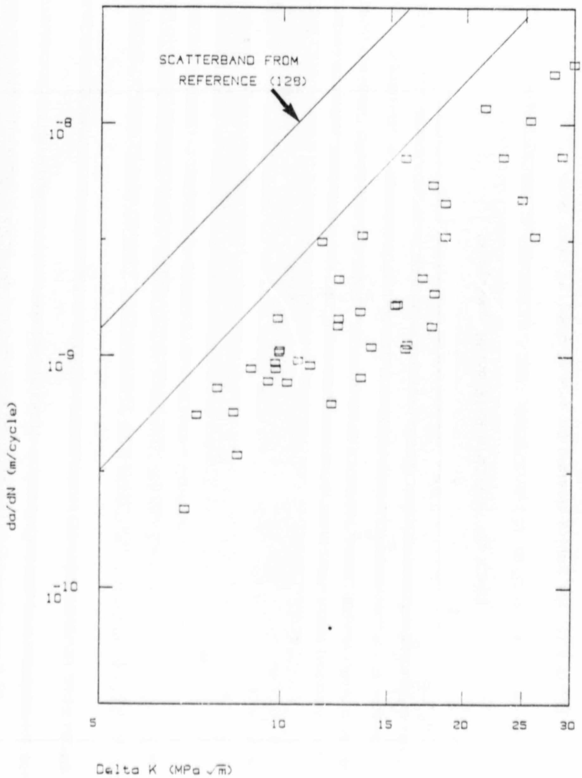
Figure 6.14 da/dN versus \Delta K for beachmarked specimens. These crack tip stress intensities were calculated from (128).
