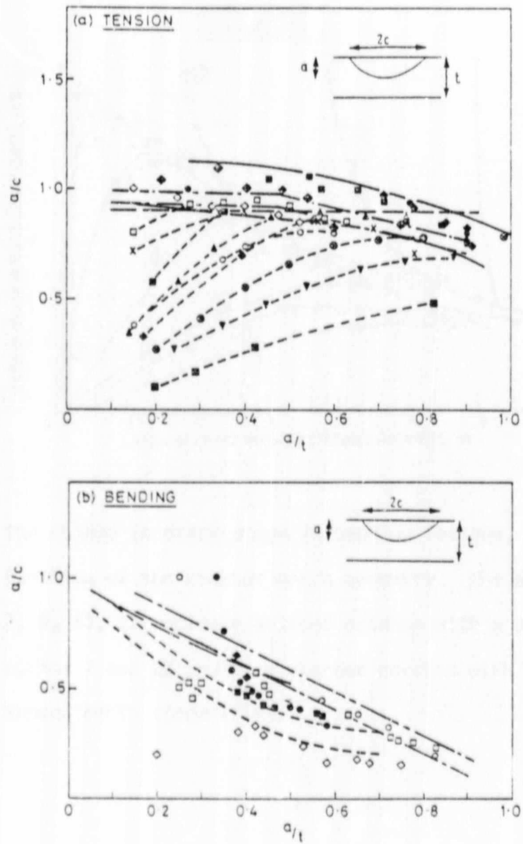
Figure 6.1 The development of crack shape under (a) direct tension and (b) pure bending. The different symbols refer to various data sources (see reference 115).
