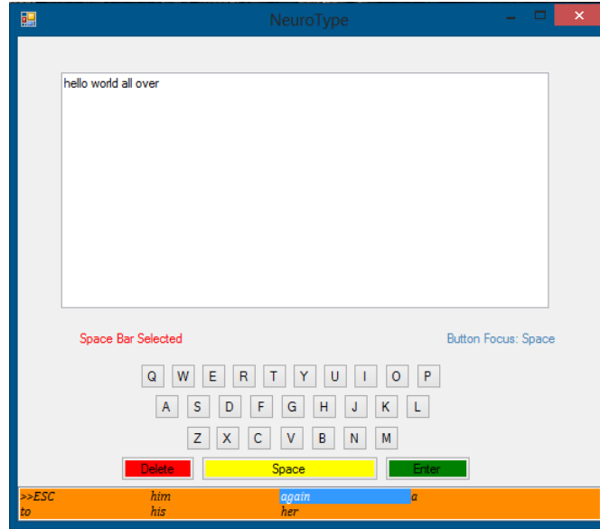
Figure 4.5: Text input GUI with predictive text functionality.
