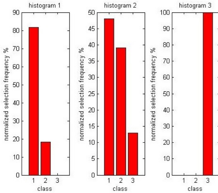
Figure 6.8: Confusion matrix results obtained using subj3 test data. The results indicate that the third mental task is inferred with 100% accuracy when the actual class label coincides with that class. A large proportion of the misclassification is attributable to the second mental task, in which the structure appears to not being learnt well by the LDCRF.
