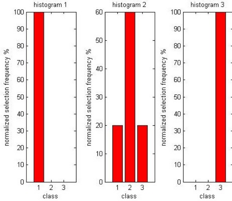
Figure 6.6: Confusion matrix results obtained using subj2 test data. The results indicate that both the first and third mental tasks are inferred with 100% accuracy when the actual class label coincides with any of those classes. Using Figure 6.7, it is clear that the classification error observed with the second mental task results is due only to the first two clusters in the data, beyond that the LDCRF produces error-free classification performance.
