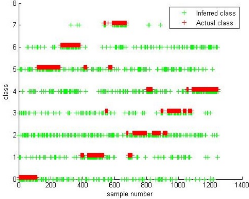
Figure 4.6: Temporal classification performance visualization tool.
