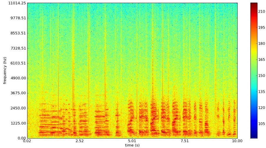
Figure 2.15: Graphical representation of a signal spectrogram. Along the vertical axis are frequency values, along the horizontal axis is time, and the colour bar represents the magnitude of the frequency component. With the three pieces of information it is possible to visualize the temporal evolution of the frequency components.
