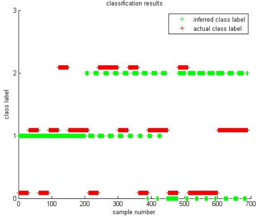
Figure 6.5: Temporal classification performance on Emotiv data for sub1. The plot represents the results obtained from the test data. The results obtained from sub2 are similar in form. The misalignment in the inferred and actual class labels indicated misclassification.
