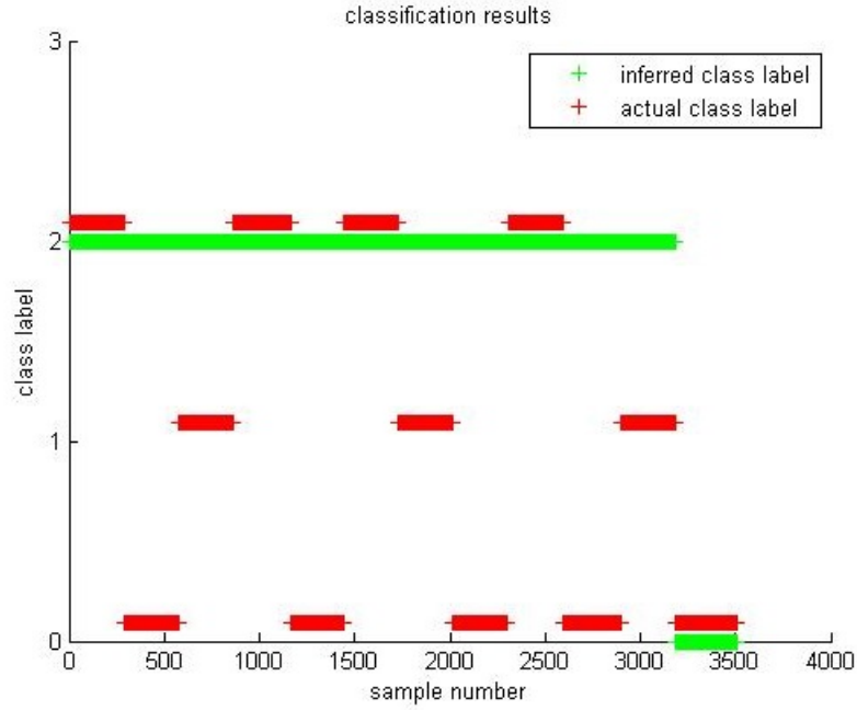
Figure 6.10: Temporal layout of classification results. The figure indicates that the model consistently infers the same class label for almost all data samples. It should also be noted that only two of the total three classes are inferred throughout the whole process.
