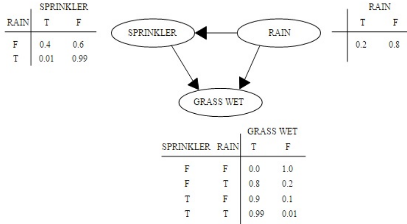
Figure 2.20: Probabilistic graphical model and associated disjoint conditional probability distributions.
