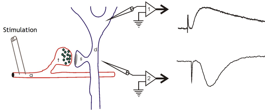
Figure 2.4: Measurement of neuron potential difference. Depending on the stimulation induced on a neuron that has synaptic coupling with another neuron, a measurable change in the potential difference is produced between two spatially separated locations in the receiving neuron. Charge is a conserved quantity, so the spatial distribution of the potential difference has to reflect the conservation. In the image, the potential differences are measured with respect to ground at two locations and differences in the plotted profiles illustrates the conservation of charge.
