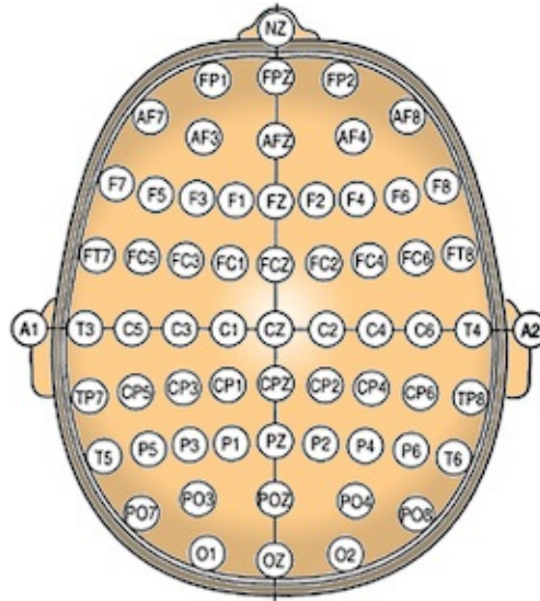
Figure 2.10: General montage template using the 10-20 electrode placement system. The topographical layout of the nodes is intended to provide full coverage on the scalp.
