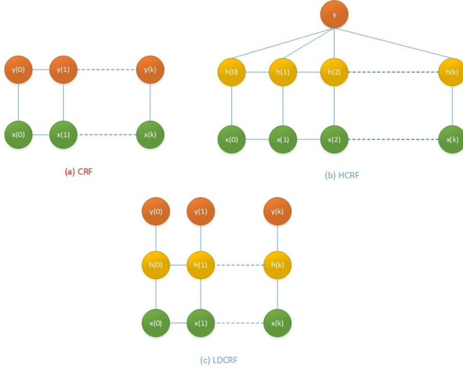
Figure 5.1: The evaluated discriminative probabilistic graphical models have blue labels. The CRF is shown for comparison purposes, and both the HCRF and LDCRF have been used in the experiments.
