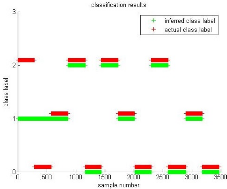
Figure 6.7: Temporal classification performance on BCI Competition data for subj2. The plot represents the results obtained from the test data. The misalignment in the inferred and actual class labels indicated misclassification
