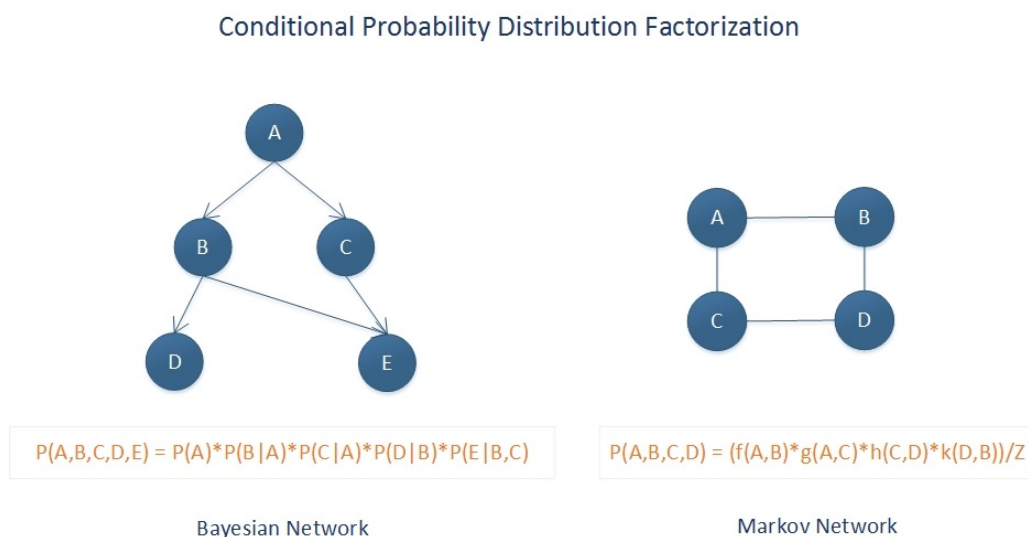
Figure 2.19: Bayesian and Markov probabilistic graphical models.
