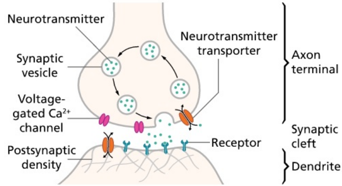
Figure 2.5: Neuro-transmitter mediated inter-neuron electric action potential transfer. The axon terminal is connected to the neuron that is the source of the action potential. The recipient of the action potential is neuron with the dendritic extension.
