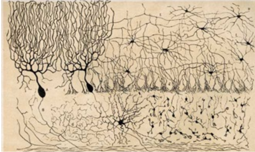
Figure 2.3: Schematics of biological neurons. Cell bodies that contain the nucleus are depicted using black bulbous dots. The long projections emanating from the cell body represent the axon of the neuron that transmits the action potential of that neuron to other neurons it is connected to. The short projections represent the dendrites of the neuron that receive action potentials from other neurons connected to it.
