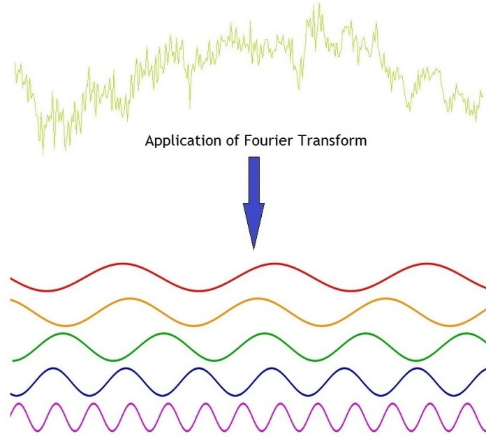
Figure 2.13: Illustration of the decomposition of a signal into its constituent signals. Points of similarity or dissimilarity are easily identifiable in the frequency domain.
