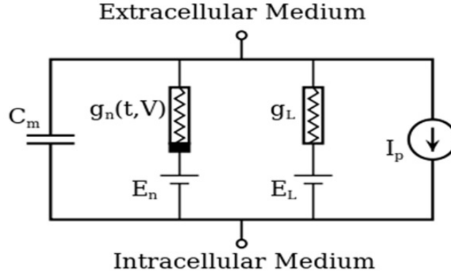
Figure 2.7: Schematic of the Hodgkin-Huxley model for action single neuron action potential. The model is based on biophysical modeling with certain physical attributes of a neuron represented by an electrical circuit that performs an analogous role in an electrical circuit.
