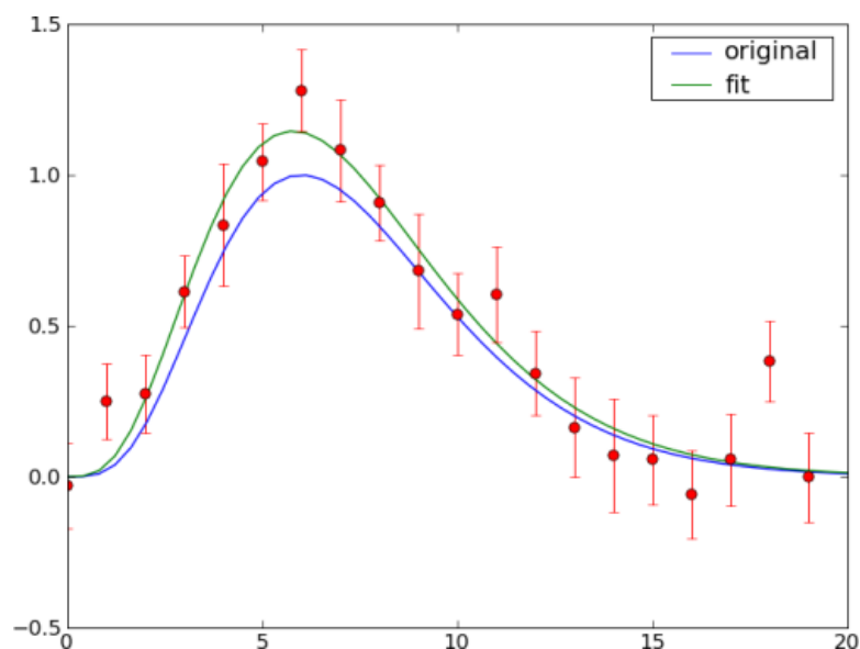
Figure 2.16: Function approximation with noisy data. The vertical lines on the data points represent error or variation in the measurement.
