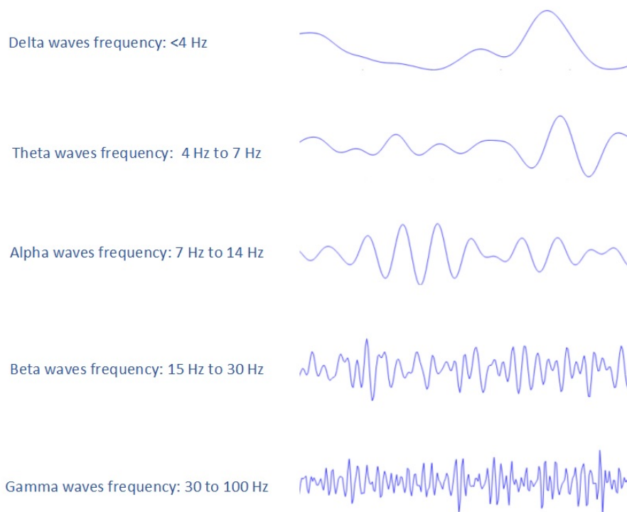
Figure 2.9: EEG signal decomposition into primary EEG bands. The frequency decompositions of the EEG signal represent the current categorization scheme. All except the gamma waves have been attributed to specific brain activity.
