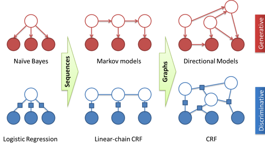
Figure 2.18: Graphical illustration of the structure of probabilistic graphical models.
