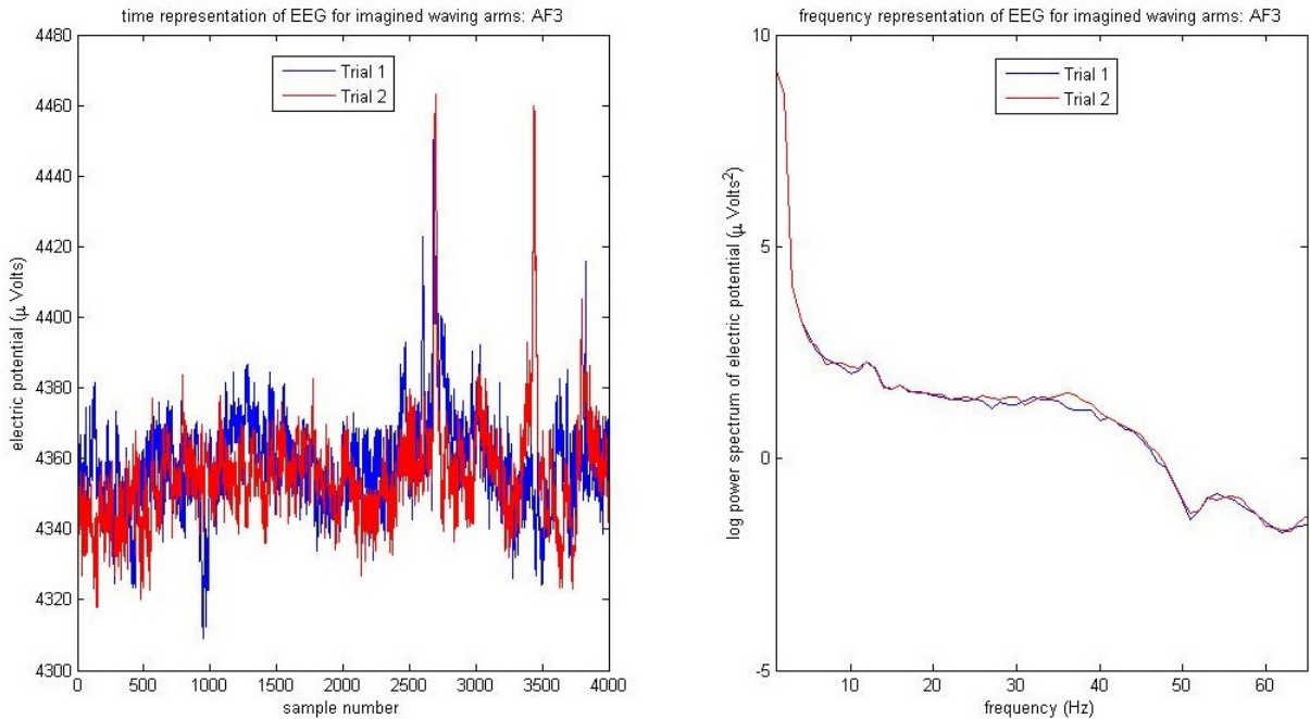
Figure 2.12: Illustration of the effect of the time-to-frequency domain transformation of a signal.
