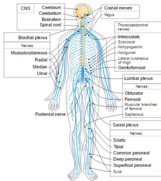
Figure 2.6: Schematic depicting long-range information processing in the nervous system. Not all nerves are directly connected to the brain with a single long-range connection. The spinal cord provides the relay mechanism that transmits action potentials to and from the brain. Concerning motor function, the connection that emanates from the brain terminates at a corresponding muscle. Concerning sensory function, the connections that emanate from sensory units such as tactile sensors on the skin terminate in the brain.
