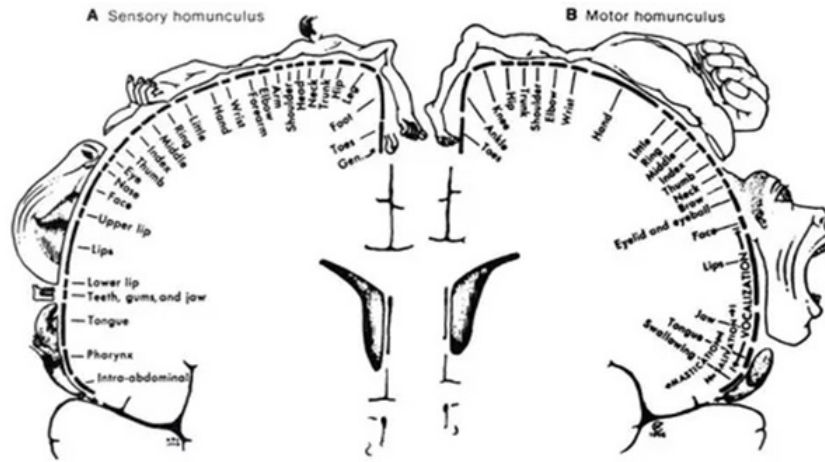
Figure 2.2: Cortical homunculus model for neural-tissue-to-body-part mapping. Varying amounts of neural tissue within a cortical region are dedicated to a particular body part. The spatial distribution of the tissue has a direct influence on the measurement of EEG activity corresponding to a particular region.
