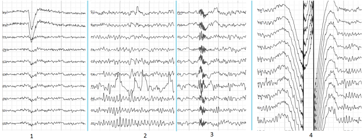
Figure 2.8: The samples of main types of artifacts in human EEG. 1 - Electrooculographic artifact caused by the excitation of eyeball’s muscles. 2 - Electrode’s artifact caused by bad contact between P3 electrode and skin. 3 - Swallowing artifact. 4 - Common reference electrode’s artifact caused by bad contact between reference electrode and skin.
