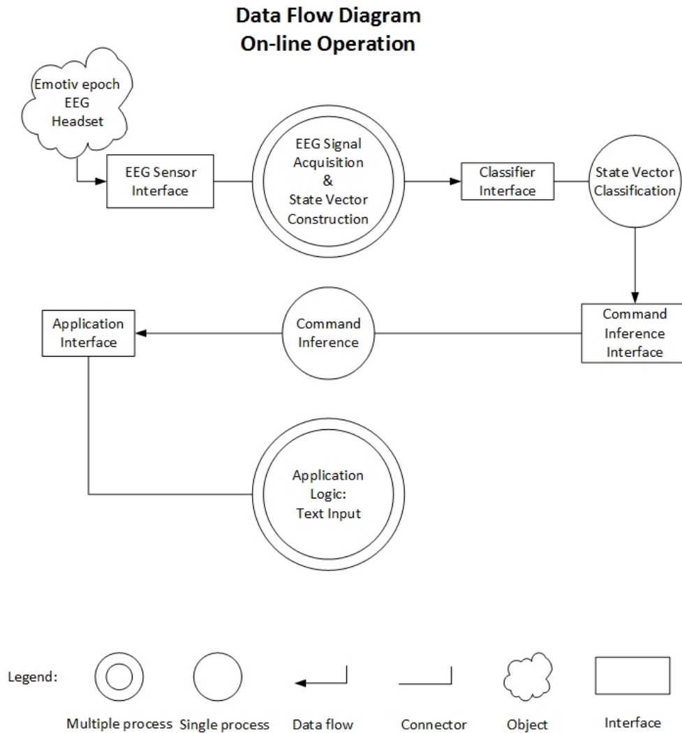
Figure 4.1: System design schematic with signal acquisition for on-line mode data-flow.
