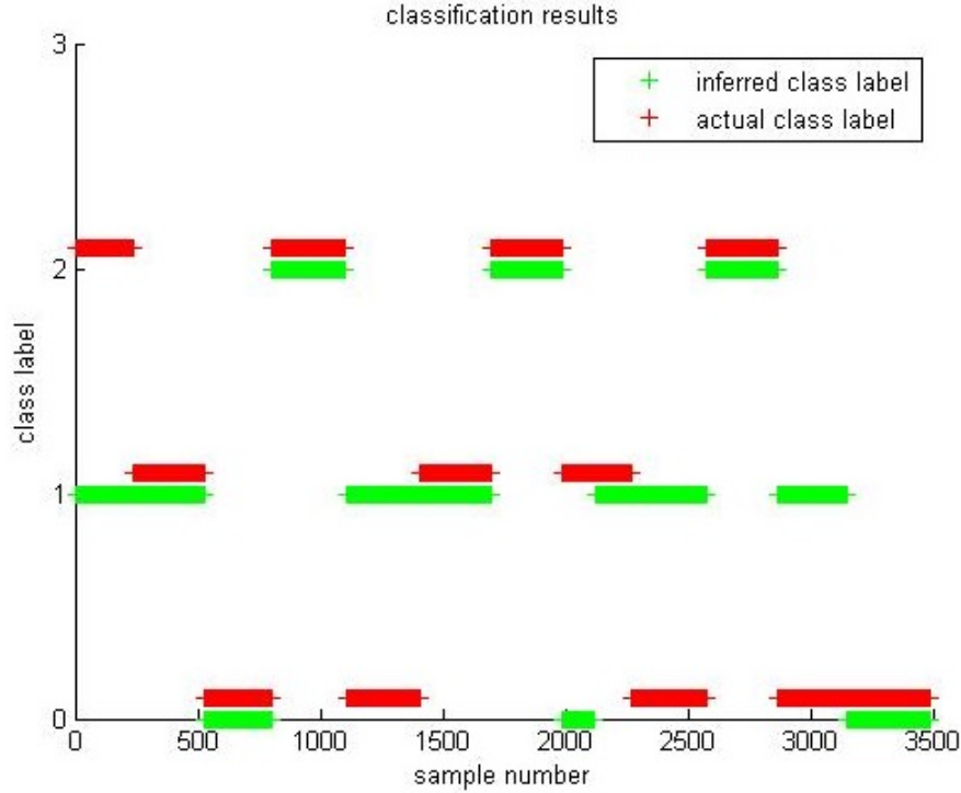
Figure 6.9: Temporal classification performance on BCI Competition data for subj3. The plot represents the results obtained from the test data. The misalignment in the inferred and actual class labels indicated misclassification
