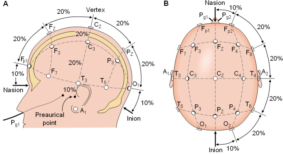
Figure 2.11: Illustration of the proportion marked 10-20 electrode placement system. The relative demarcation is designed such that differences in head sizes have a minimal influence on inter-subject comparative measurements.
