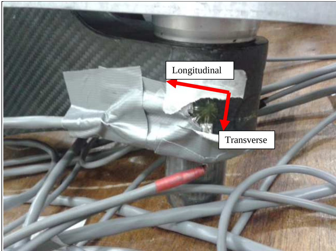
Figure 129. Strain Gauge 8.
