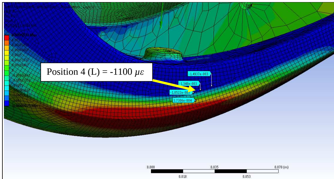
Figure 89. Strain distribution for Position 4 in the gauge longitudinal direction at 8000N.
