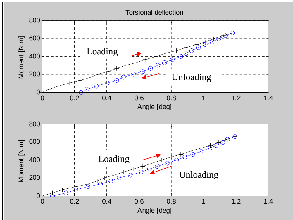
Figure 53. Torsional deflection of swingarm during loading and unloading during two torsional tests.
