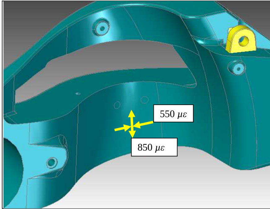
Figure 61. Maximum longitudinal and transverse strain at Position 3 during vertical loading.
