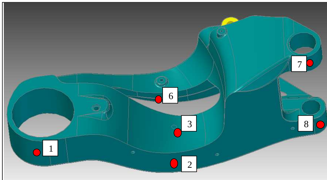
Figure 57. Strain Gauge measurement positions
