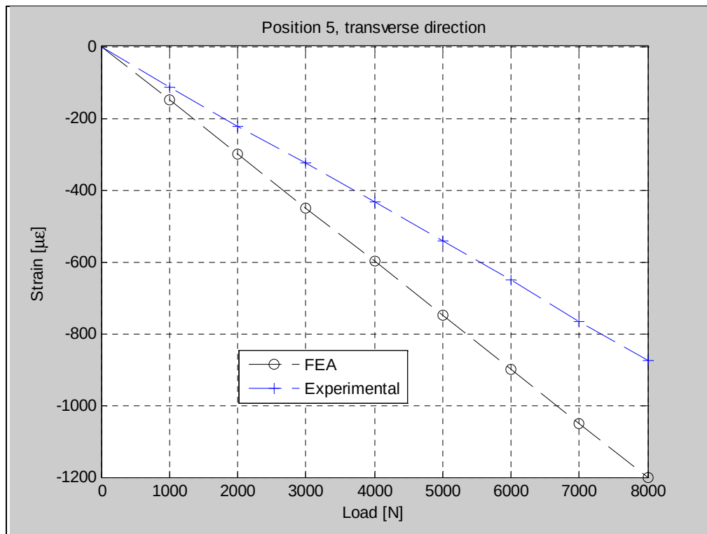
Figure 98. Comparison between FEA and experimental results at Position 5 in the gauge transverse direction.
