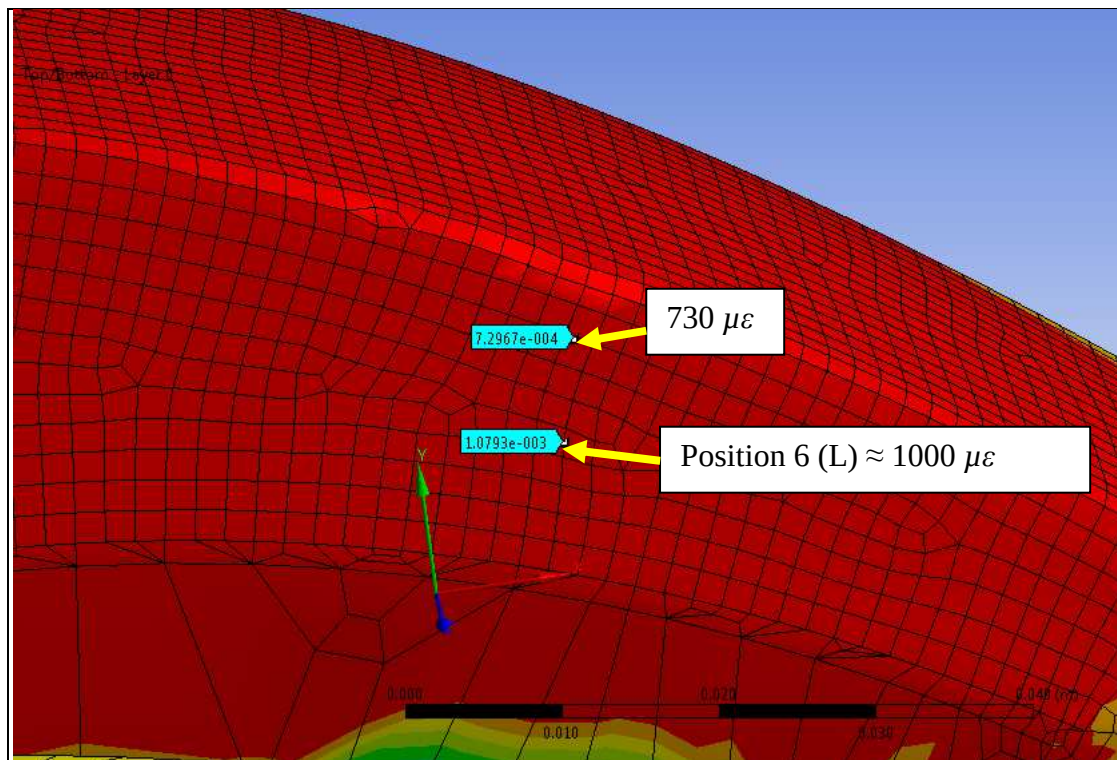
Figure 99. Strain distribution for Position 6 in the gauge longitudinal direction.
