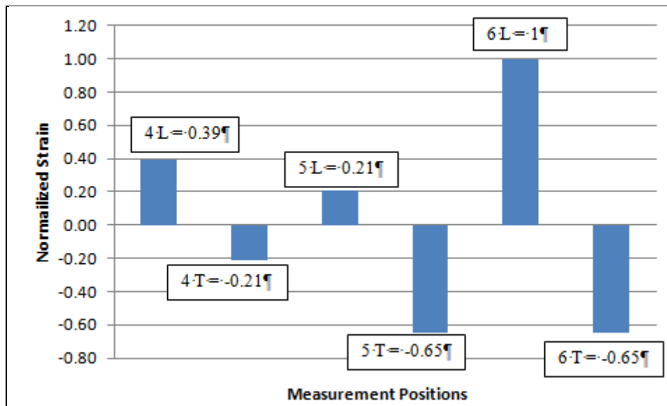
Figure 71. Normalized strain occurring on the top arm of the swingarm due to torsional loading.
