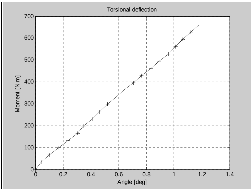
Figure 51. Torsional deflection of the swingarm.
