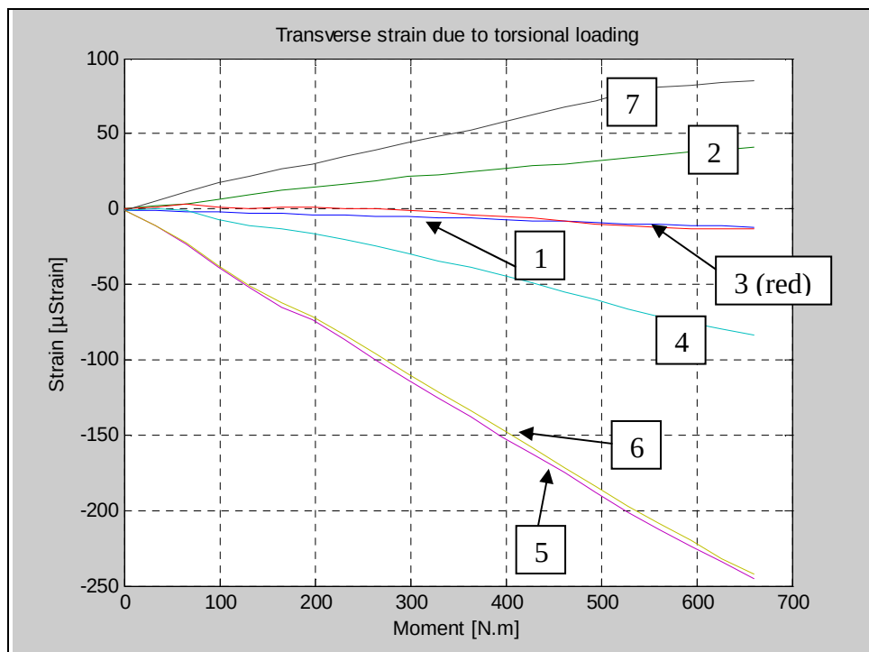
Figure 67. Strain in the transverse direction due to torsional loading.
