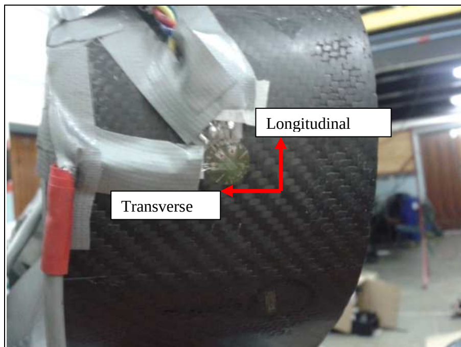
Figure 116. Strain Gauge 1.
