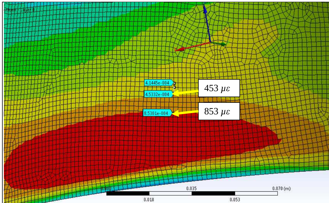
Figure 88. Position 3 in the transverse direction with axes rotated +2 degrees.
