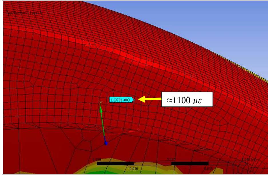
Figure 101. Longitudinal strain at Position 6 after adding three \pm 45^\circ plies.
