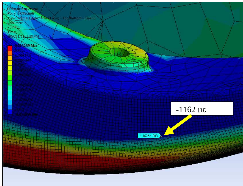
Figure 136. Position 4 with element size of 1 mm.
