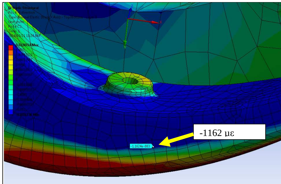
Figure 134. Position 4 with element size of 5 mm.
