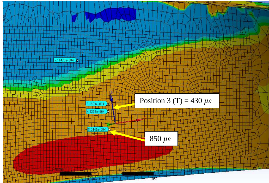
Figure 85. Close up of the strain distribution for Position 3 in the gauge transverse direction (vertical direction in the figure).
