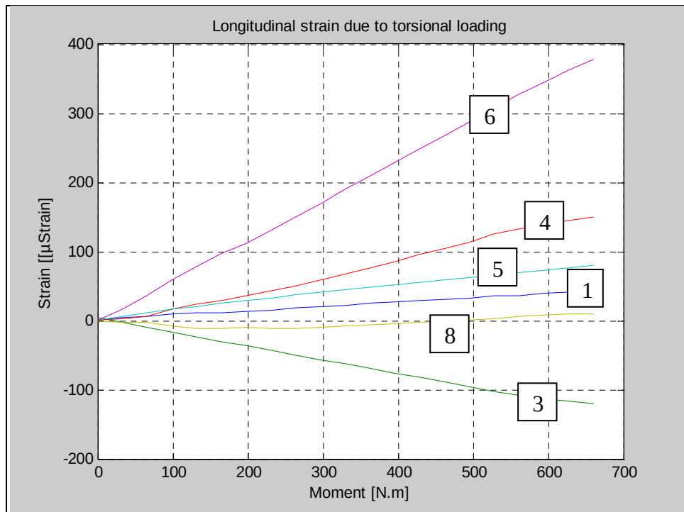
Figure 66. Longitudinal strain due to the torsional loading. Strain gauge positions are shown on the figure.
