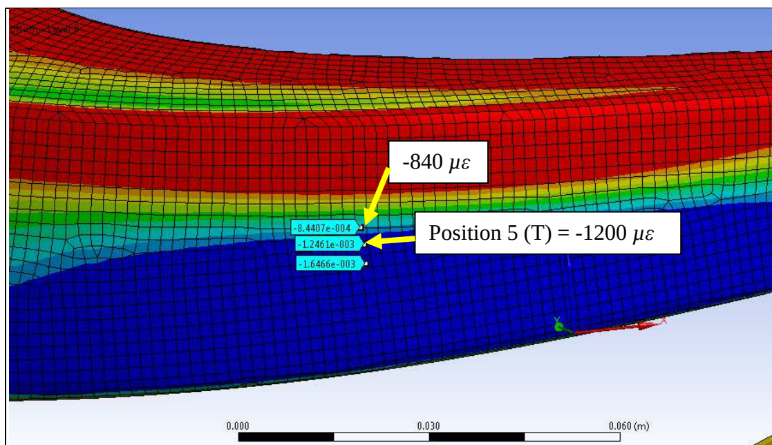
Figure 97. Strain distribution for Position 5 in the gauge transverse direction.
