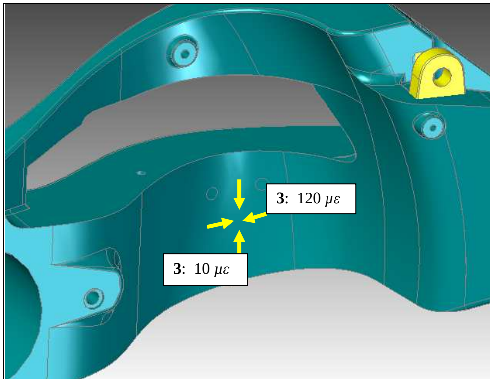
Figure 68. Maximum longitudinal and transverse strain at Position 3 during torsional loading.
