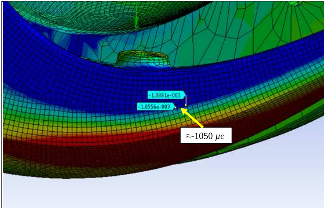
Figure 93. Updated longitudinal strain at Position 4 by adding 3 plies.
