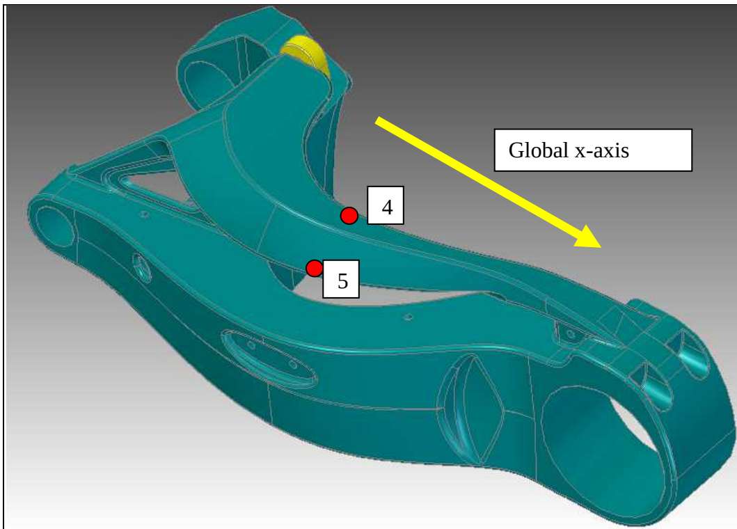
Figure 22. Strain gauge measurement positions.
