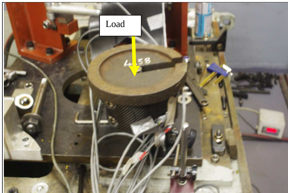
Figure 27. Rig setup for applying lateral loads in the global z-direction.
