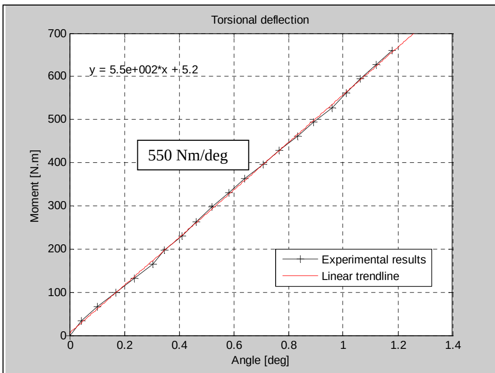
Figure 52. Torsional deflection of the swingarm showing the torsional stiffness coefficient of 550 Nm/deg.
