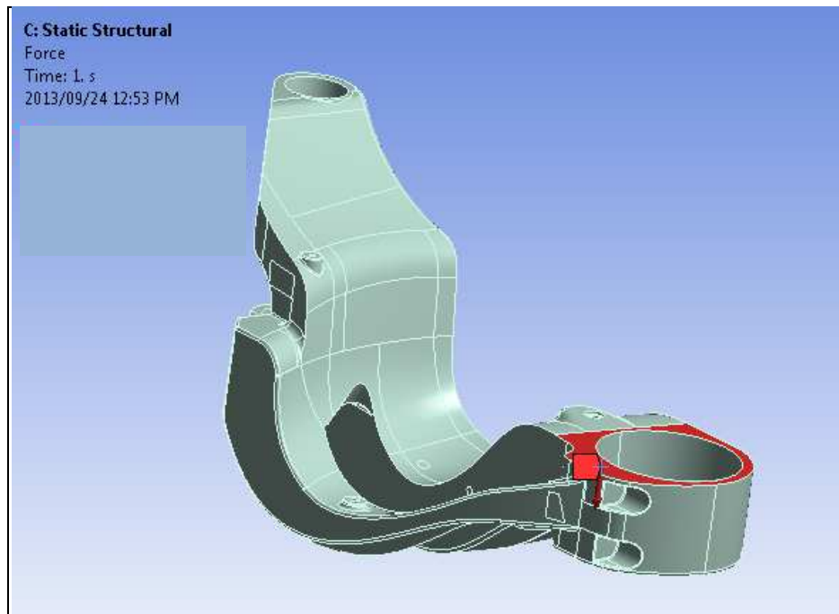
Figure 46. FE model subjected to a load in the motorcycle lateral direction.
