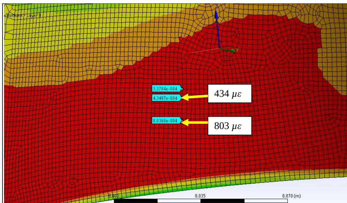
Figure 87. Position 3 in the transverse direction with axes rotated -2 degrees.
