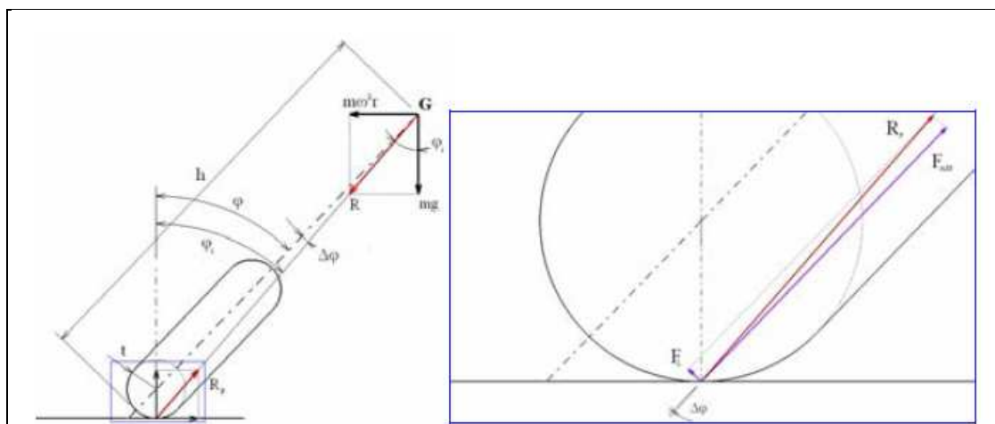
Figure 13. Loads acting on the swingarm during cornering assuming thick wheels [8].
