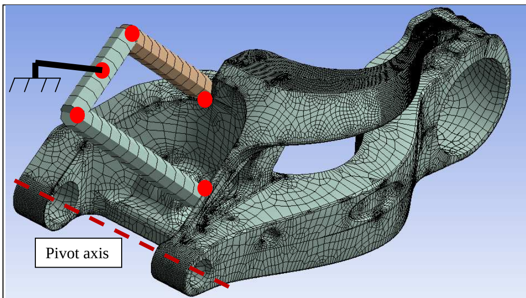
Figure 43. Finite element model of swingarm showing the rocker arm. The red dots indicate the positions of the revolute joints.
