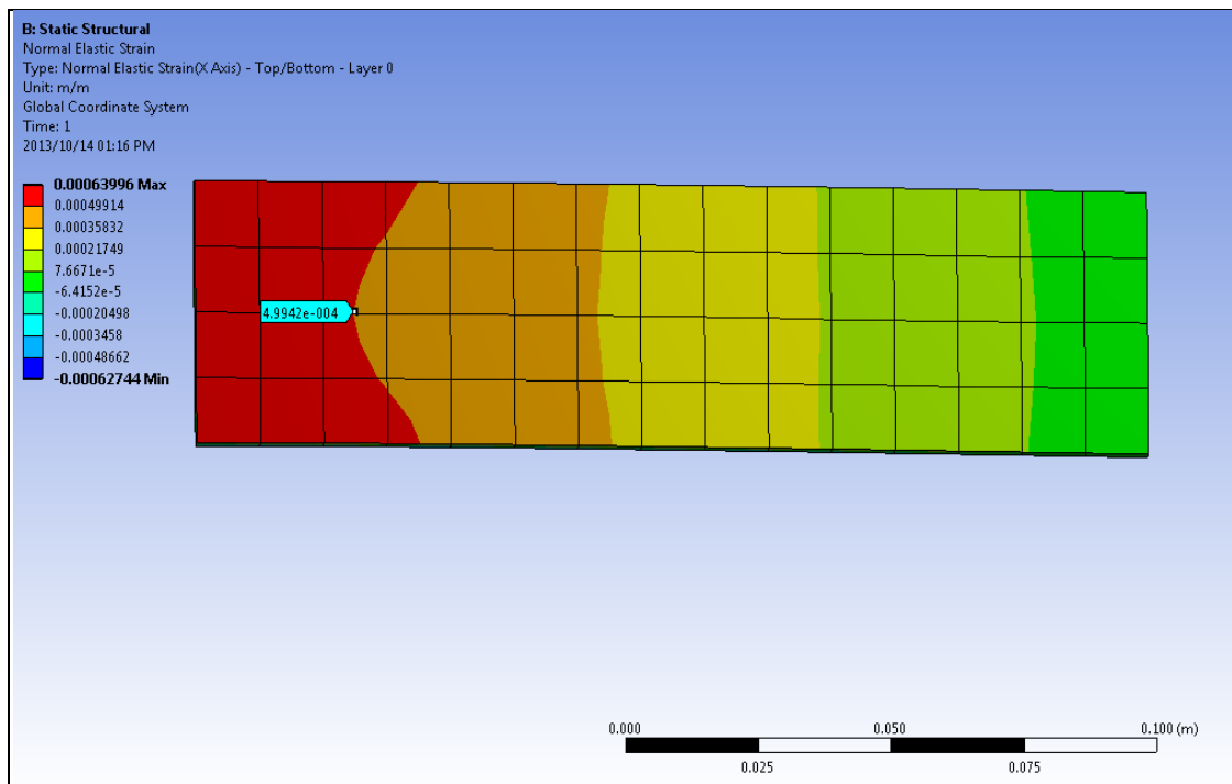
Figure 109. Longitudinal strain of 499 \mu\epsilon obtained from Ansys Composite.
