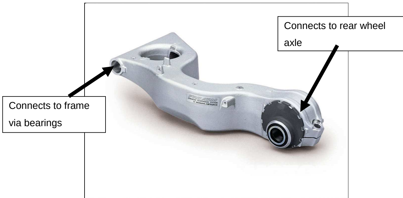
Figure 4. A single-sided swingarm [7].
