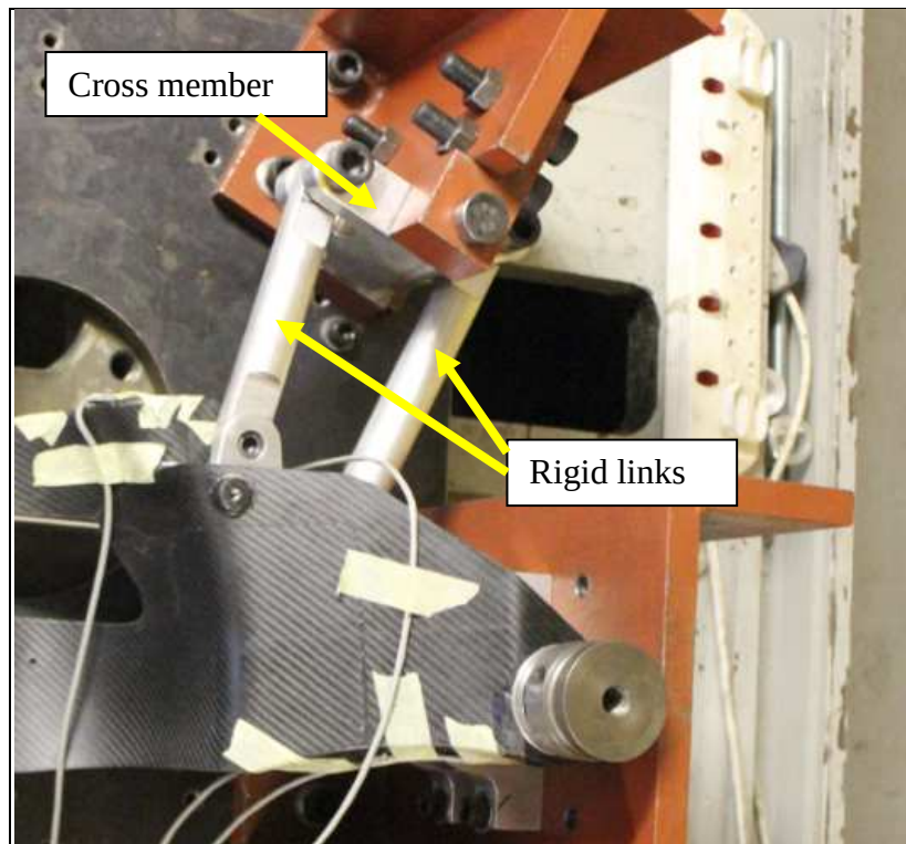
Figure 41. Rocker arm assembly.
