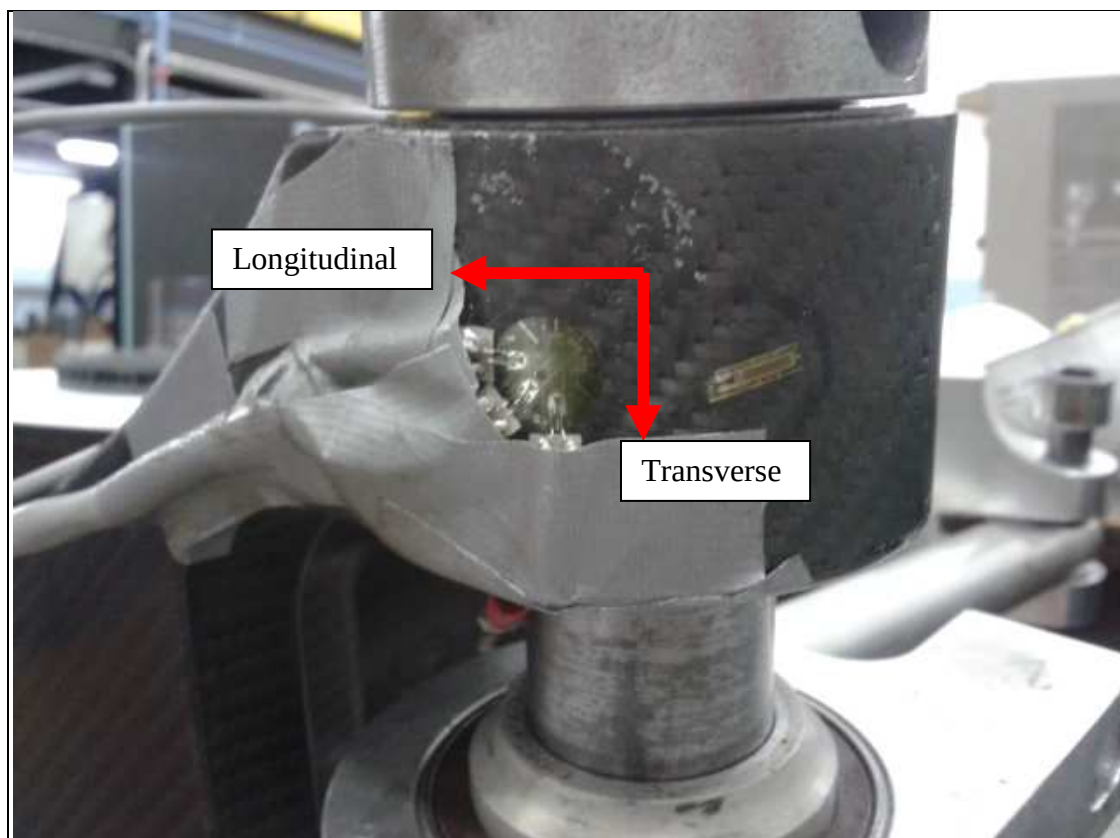
Figure 128. Strain Gauge 7.
