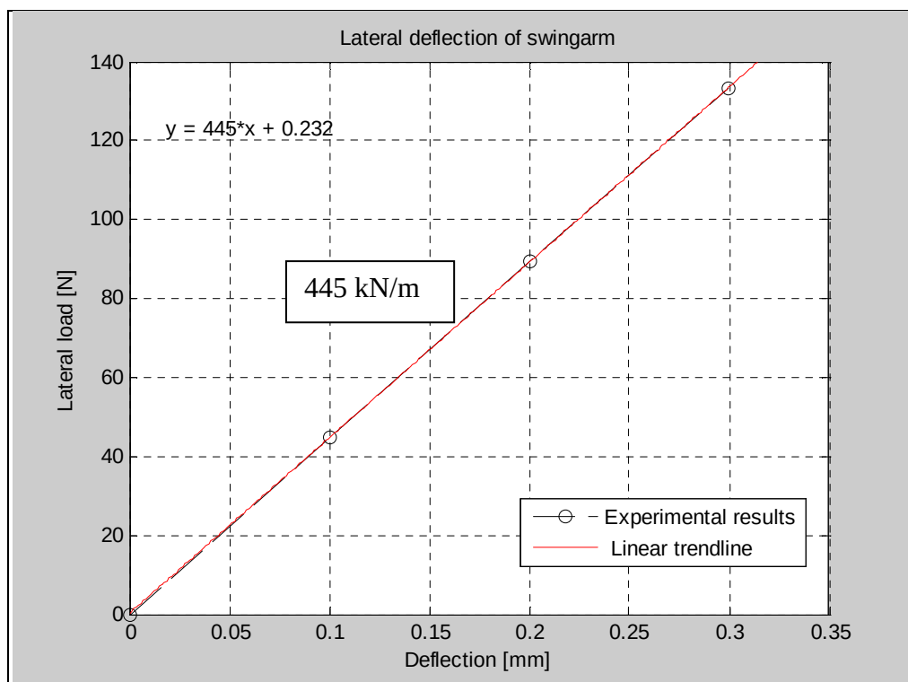
Figure 56. Lateral deflection of the swingarm showing the lateral stiffness coefficient of 445 kN/m.
