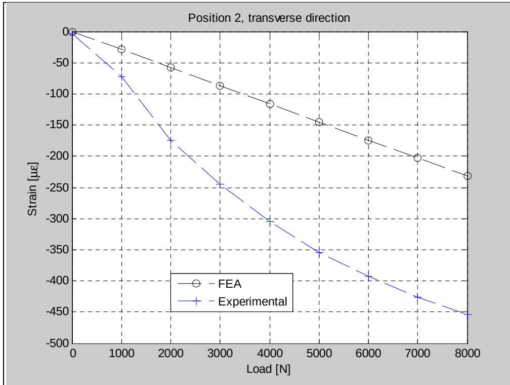
Figure 76. Comparison between FEA and experimental results at Position 2 in the gauge transverse direction.
