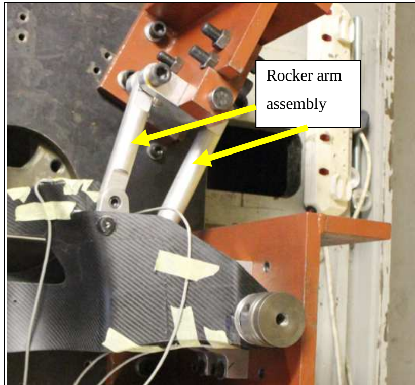
Figure 19. Connection from swingarm to rocker-arm.
