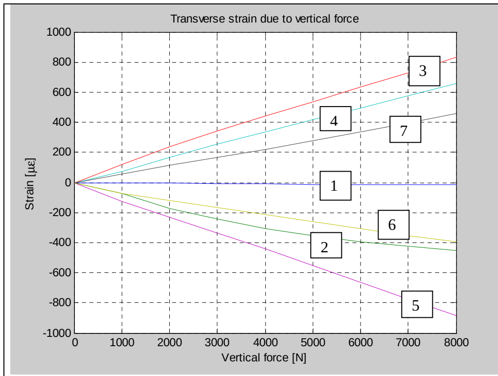
Figure 60. Transverse strain measured at positions 1 through 7.
