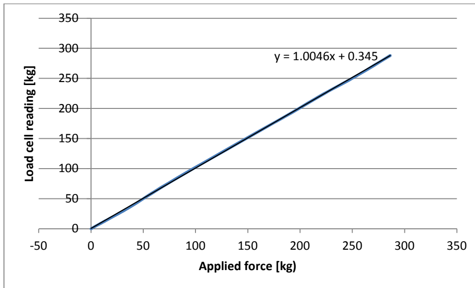
Figure 112. Calibration curve for the 50kN load cell.
