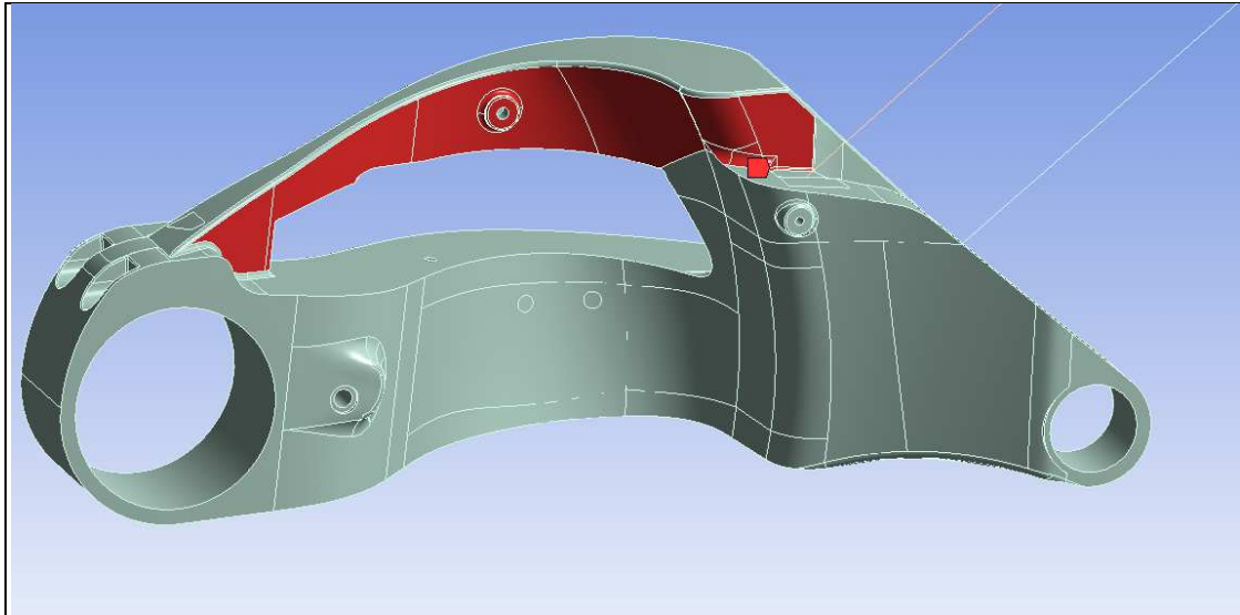
Figure 34. Inside zone of the top arm.
