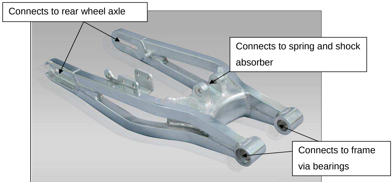
Figure 3. A double-sided swingarm [6].
