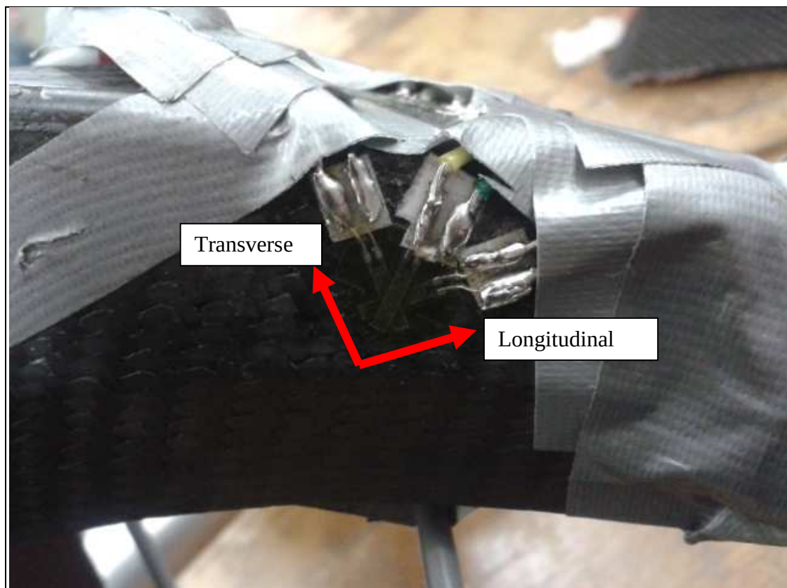
Figure 126. Strain Gauge 6.
