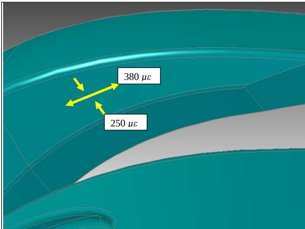
Figure 70. Maximum longitudinal and transverse strain at Position 6 during torsional loading.
