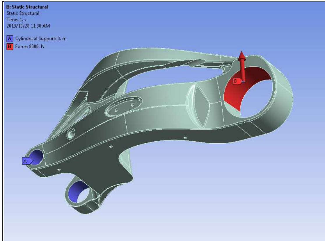
Figure 44. FE model showing constraints applied during vertical loading.
