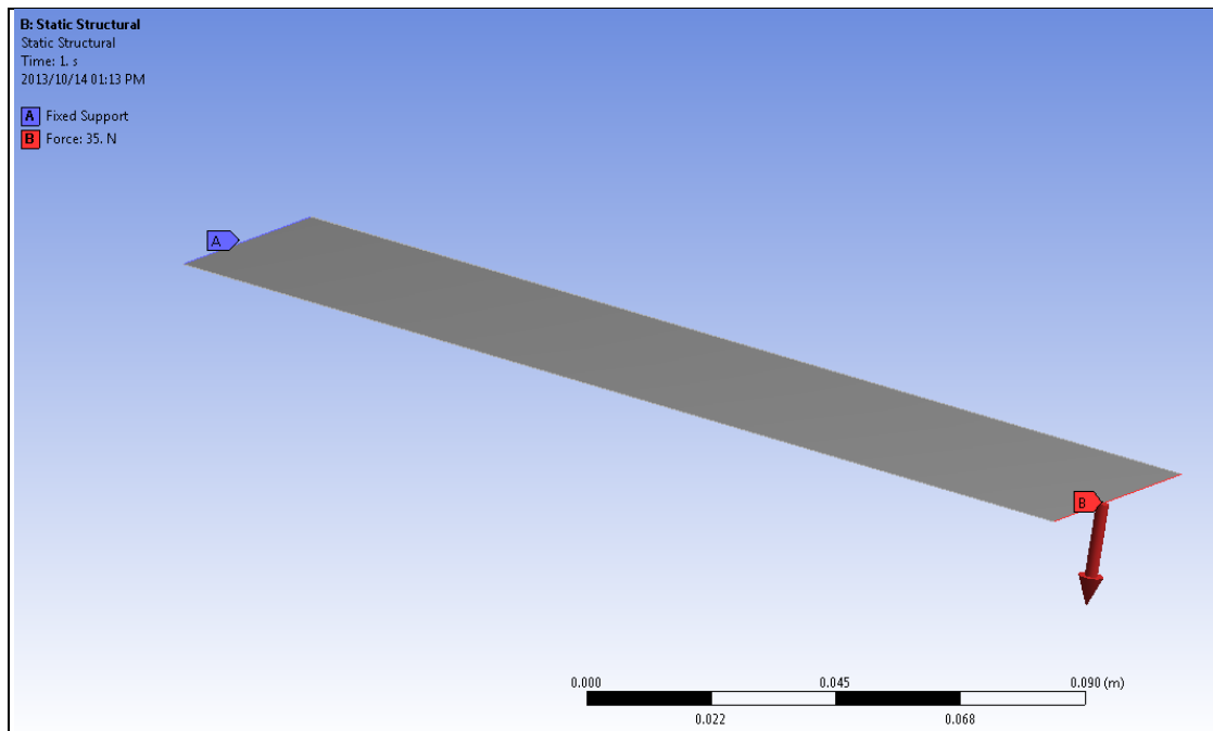
Figure 107. Constraints applied to the carbon fibre plate created in Ansys Composite.
