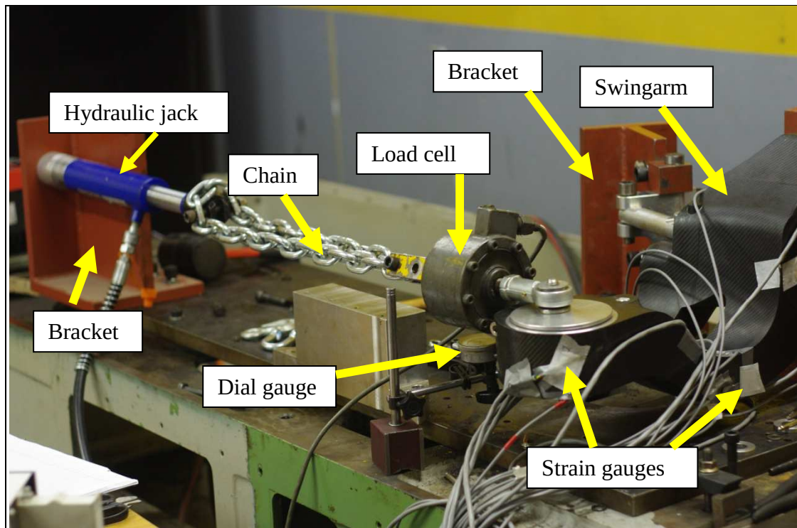
Figure 17. Test rig showing various components.
