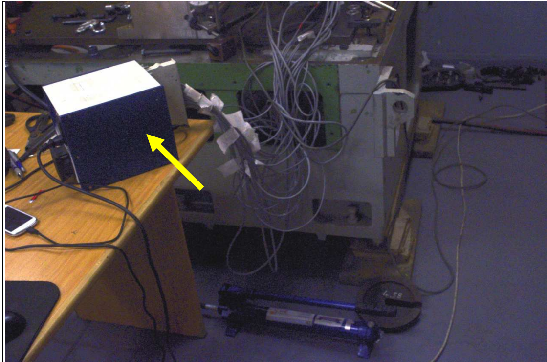
Figure 130. NI data acquisition system connected to the strain gauges on the swingarm.
