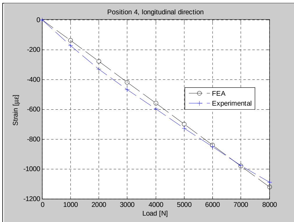
Figure 90. Comparison between FEA and experimental results at Position 4 in the gauge longitudinal direction.
