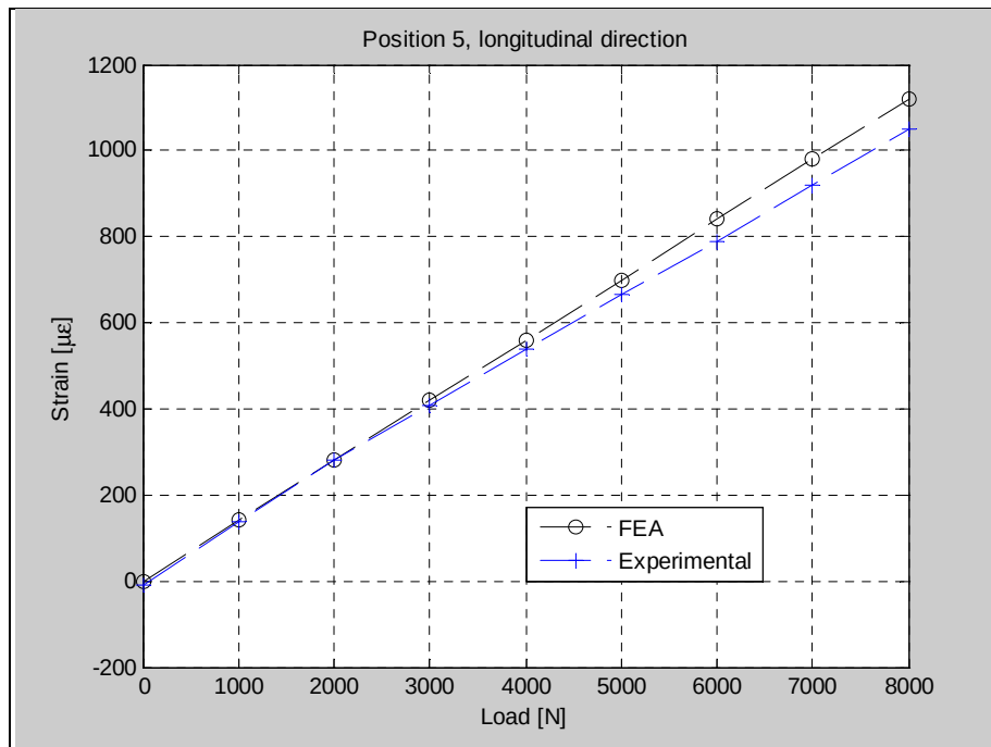
Figure 96. Comparison between FEA and experimental results at Position 5 in the gauge longitudinal direction.
