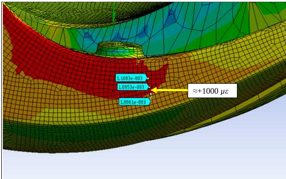
Figure 94. Updated transverse strain at Position 4 by adding 3 plies.
