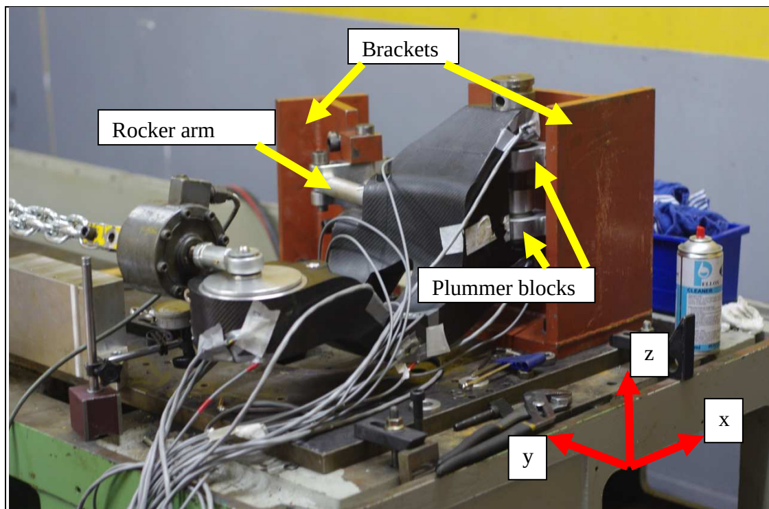
Figure 18. Test rig showing various components.
