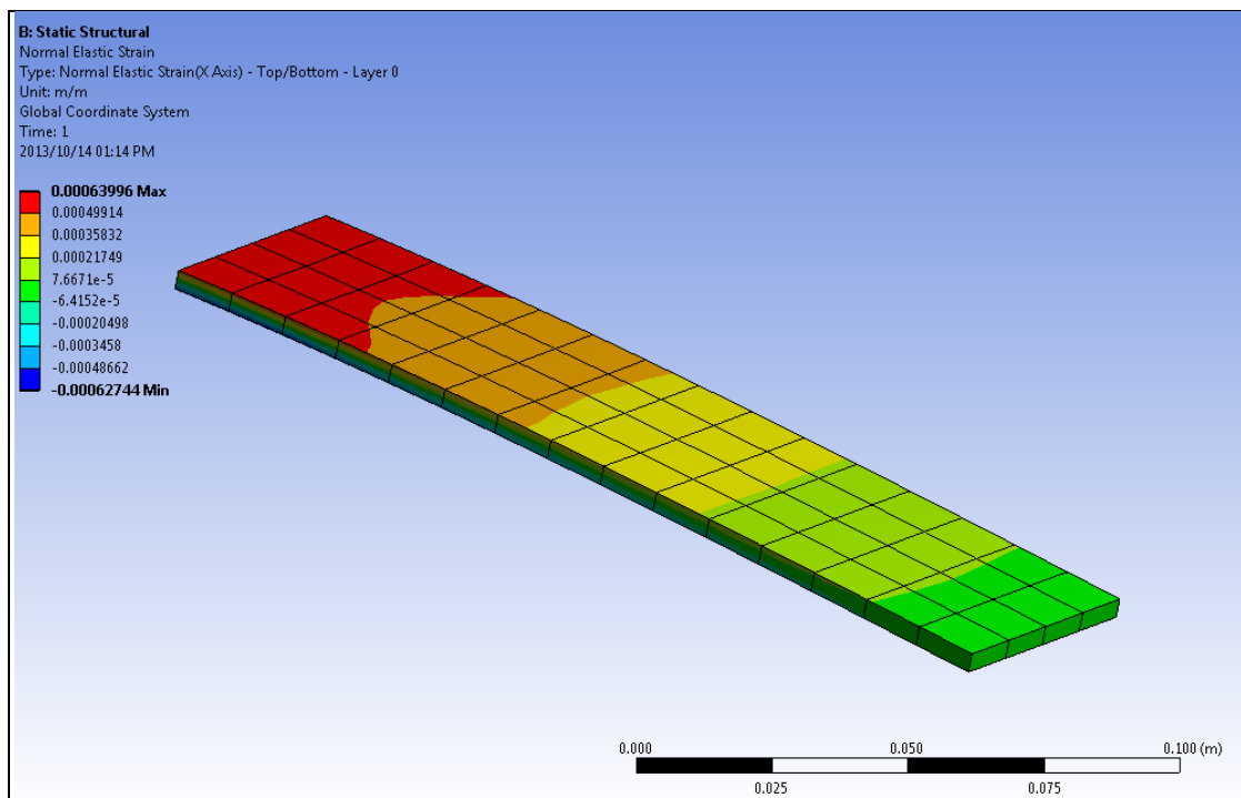
Figure 108. Graphical FEA results for the cantilever plate.
