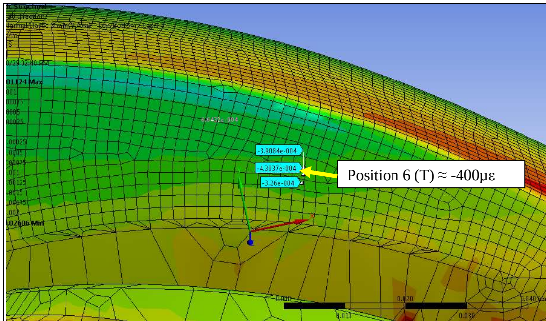
Figure 104. Strain distribution for Position 6 in the gauge transverse direction with the addition of 3 \pm 45^\circ plies.
