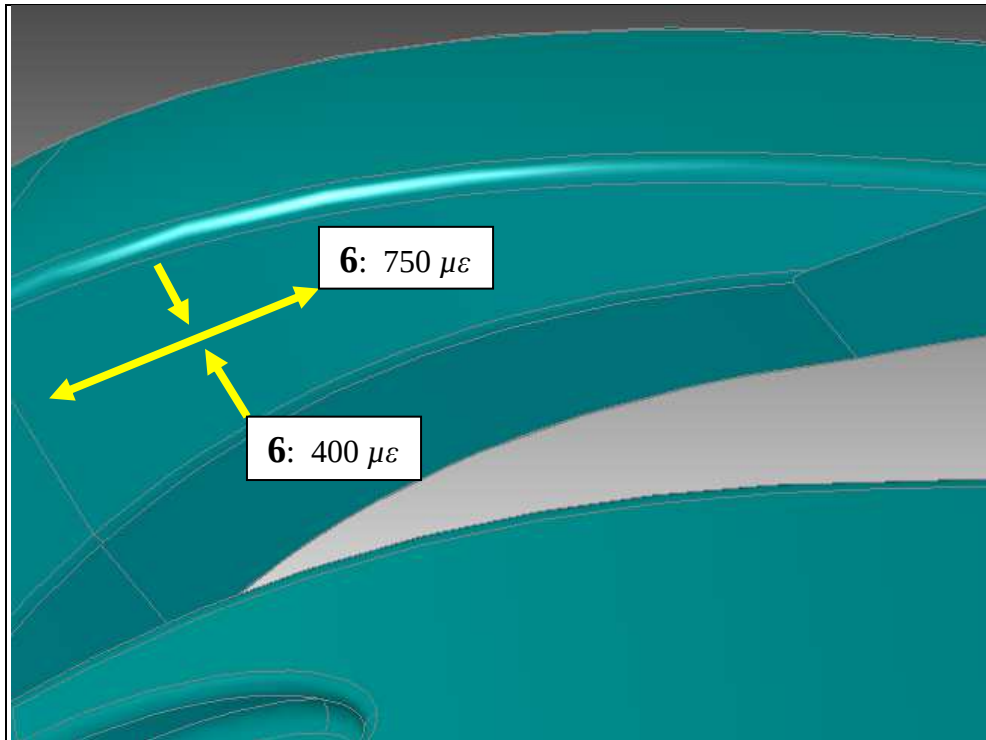
Figure 63. Maximum longitudinal and transverse strain occurring at Positions 6 during vertical loading.
