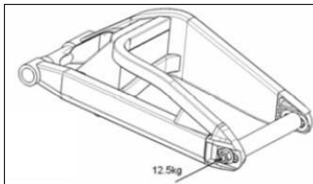
Figure 14. Lateral loading of the double-sided aluminium swingarm using spacer and spindle to simulate real loading conditions [8].
