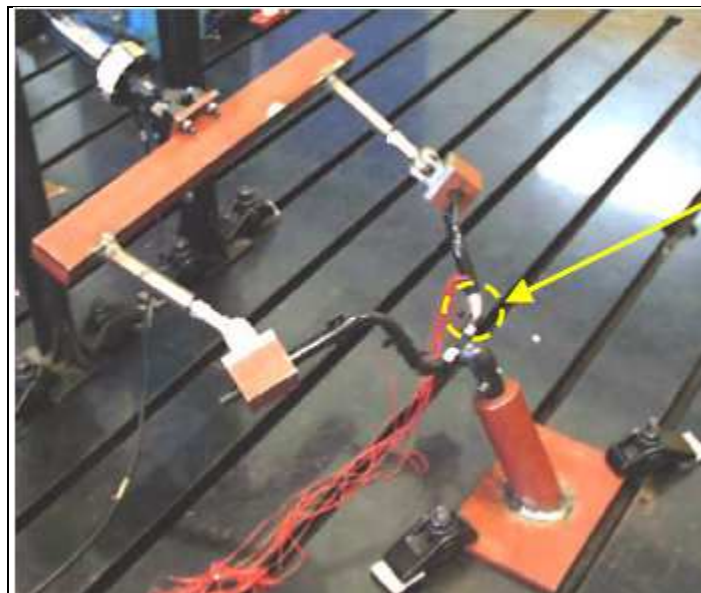
Figure 9. Durability test rig for motorcycle handlebars. [23]
