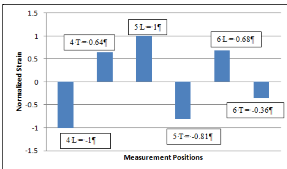
Figure 65. Normalized strain on the top arm of the swingarm due to vertical loading.
