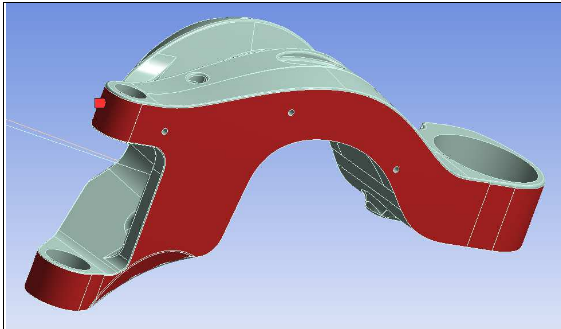
Figure 39. Underside zone of the bottom arm.
