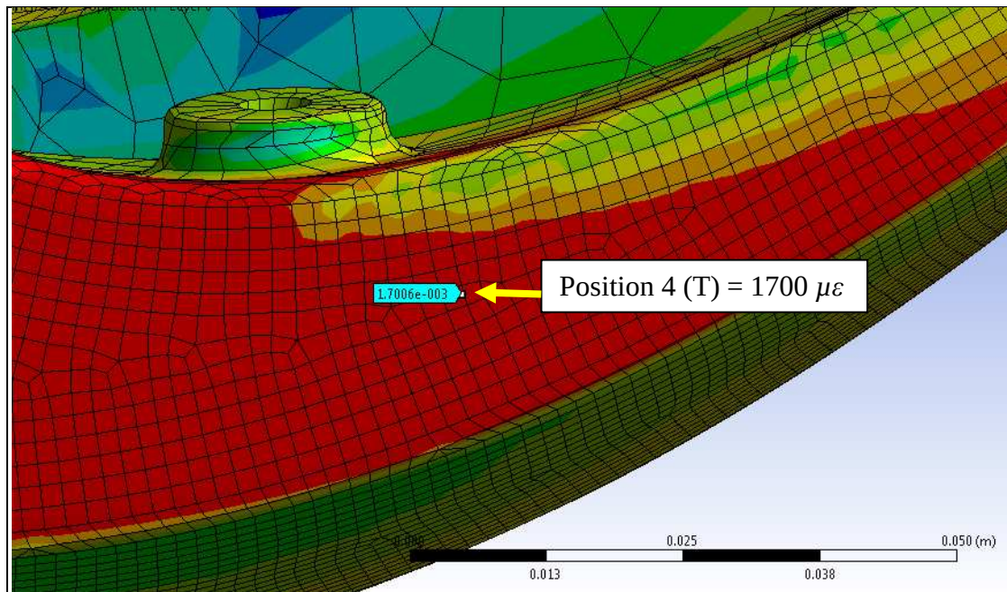
Figure 91. Strain distribution for Position 4 in the gauge transverse direction at 8000N.
