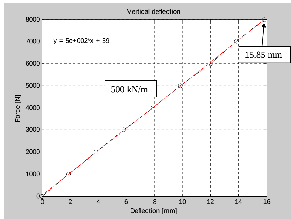
Figure 47. Vertical deflection of swingarm showing the vertical stiffness coefficient of 500 kN/m.
