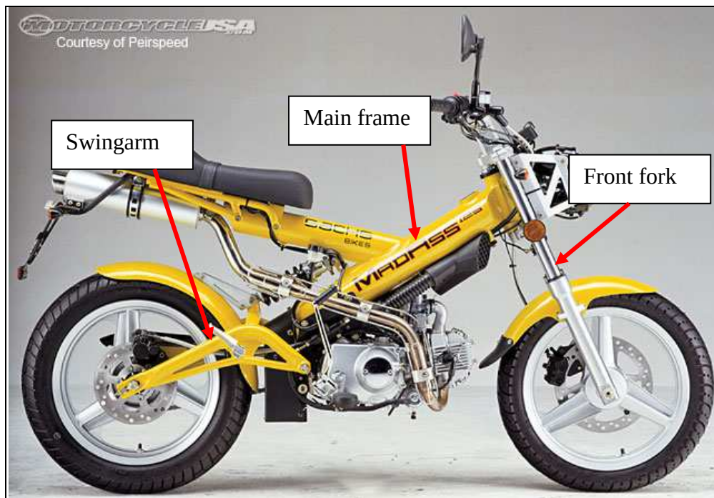
Figure 1. Example showing the main components of a motorcycle. [4]
