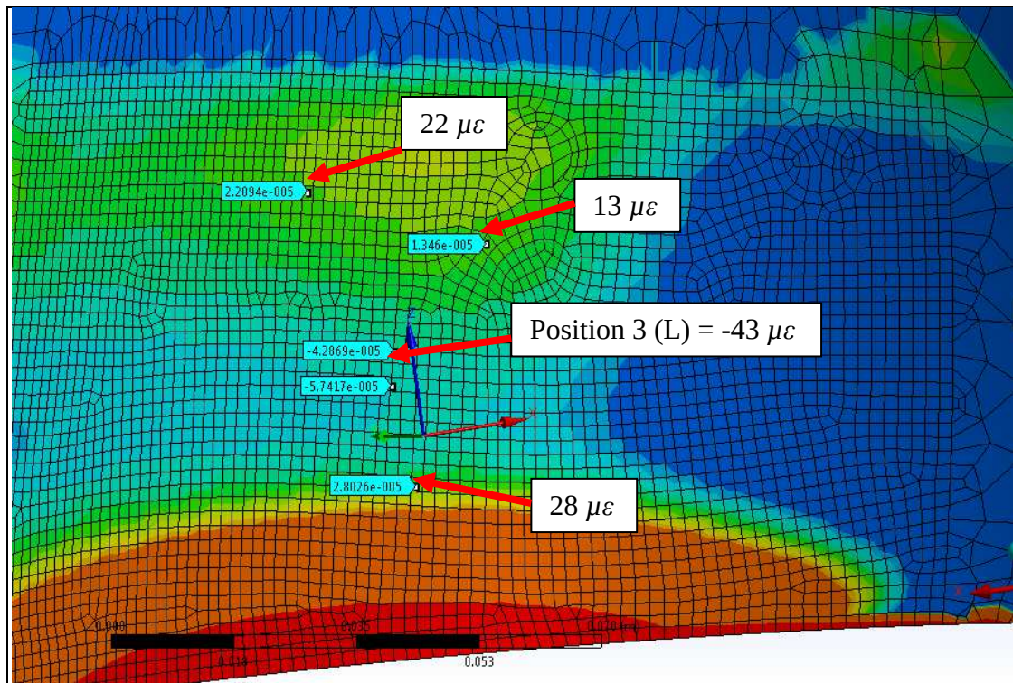
Figure 81. Close up of the strain distribution for Position 3 in the gauge longitudinal direction.
