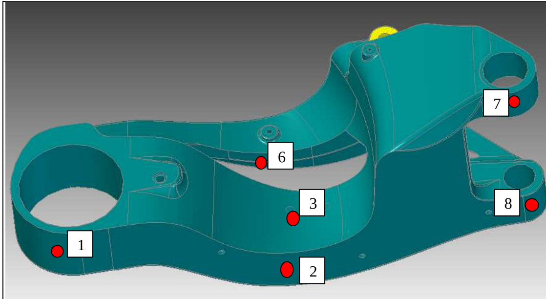
Figure 21. Strain gauge measurement positions.
