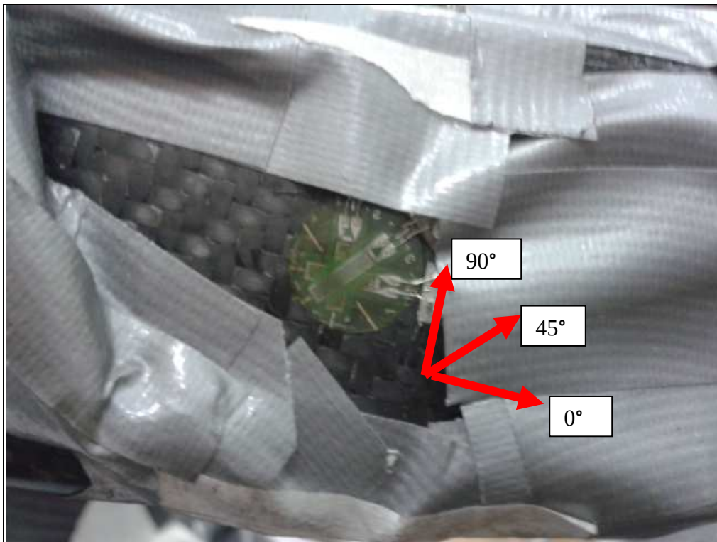
Figure 20. Rosette strain gauge.
