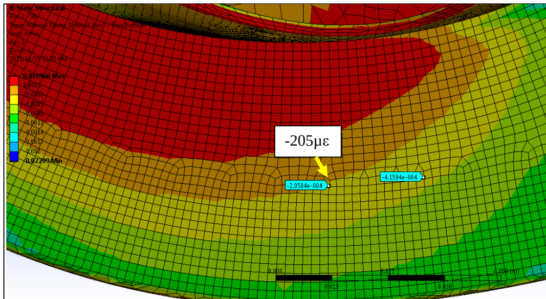
Figure 77. Position 2 in the transverse direction with the axes rotated -2 degrees.
