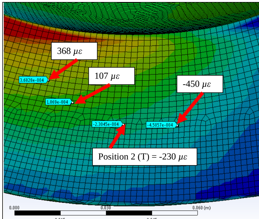
Figure 79. Close up of the strain distribution for Position 2 in the gauge transverse direction at vertical load of 8000 N
