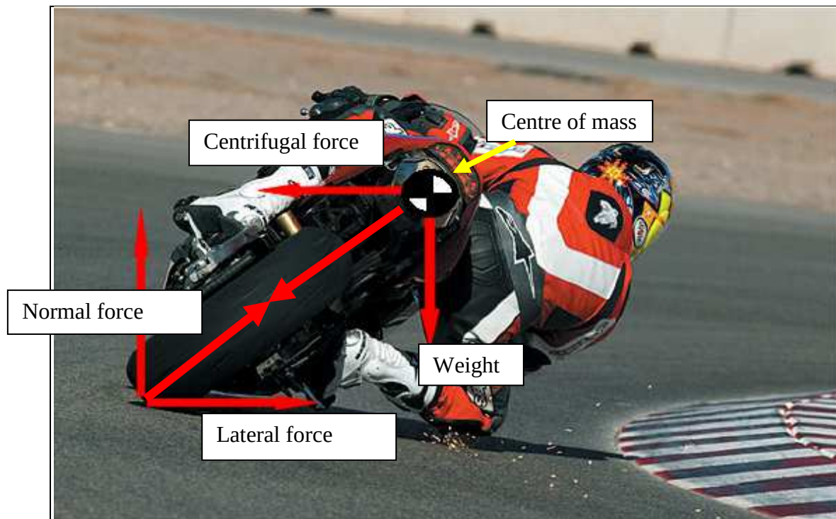
Figure 12. Loads acting on the swingarm during cornering assuming thin wheels [8].
