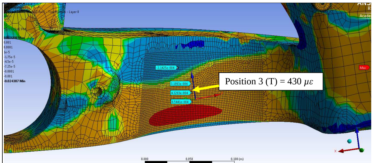
Figure 84. Strain distribution for Position 3 in the gauge transverse direction.
