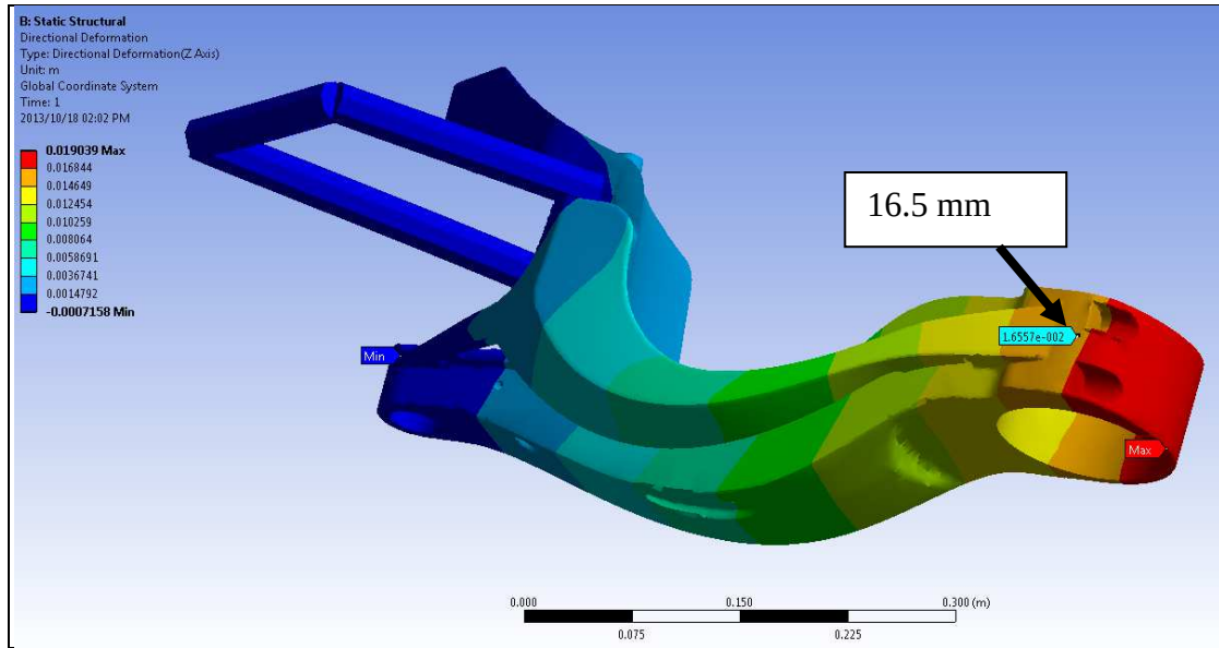
Figure 72. Vertical deflection at 8000N.
