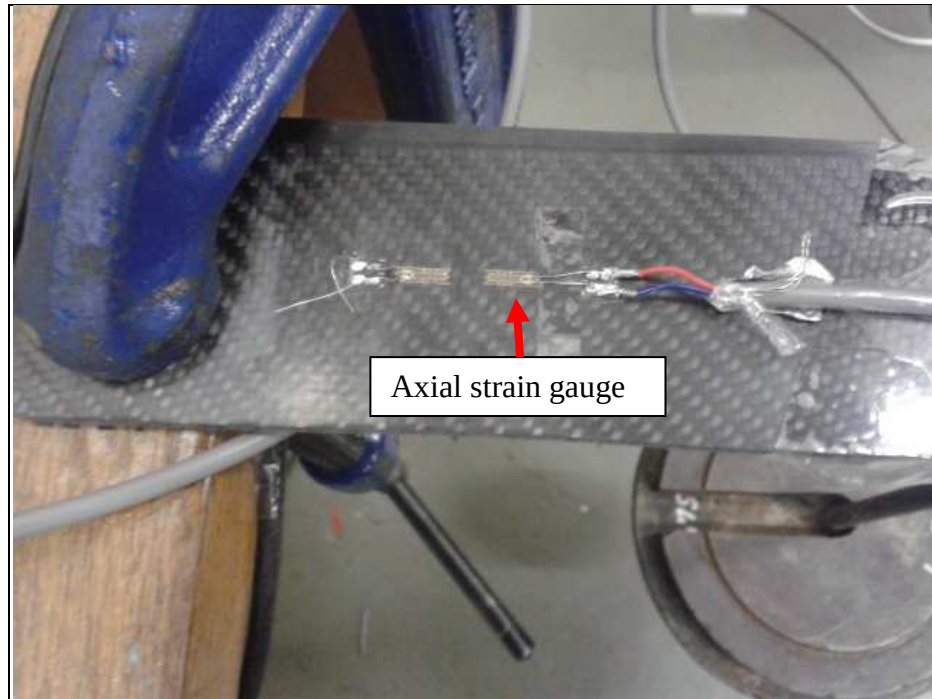
Figure 106. Axial strain gauge applied near the fixed end of the plate.
