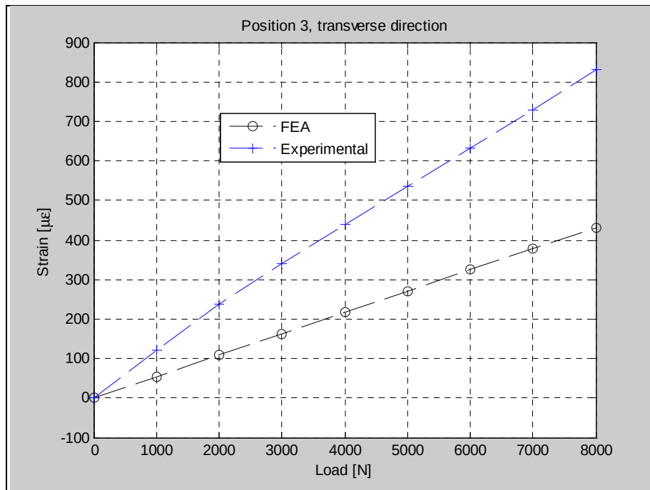
Figure 86. Comparison between FEA and experimental results at Position 3 in the gauge transverse direction.
