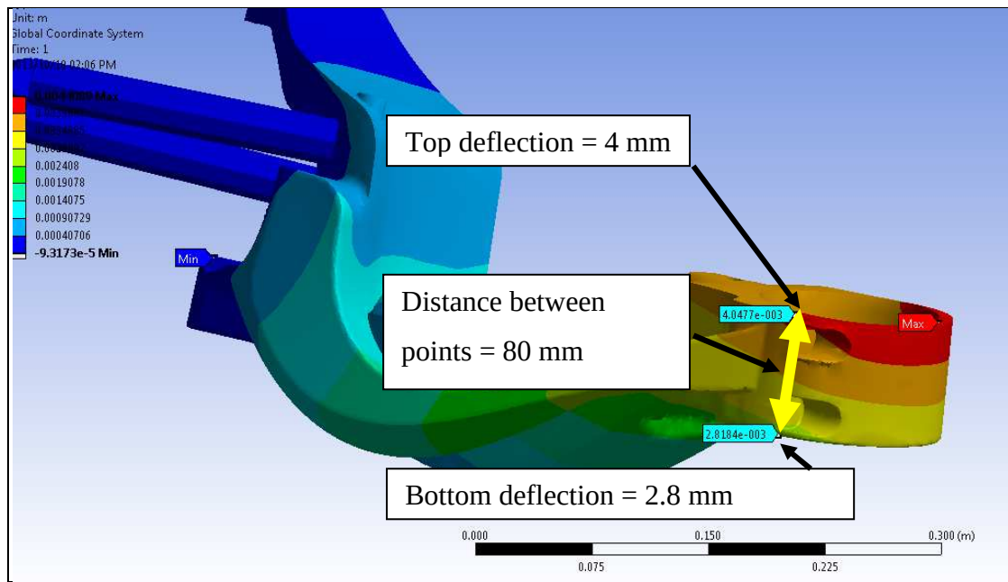
Figure 73. Deflection measured during maximum torsional loading of 2000 N and 680 Nm.
