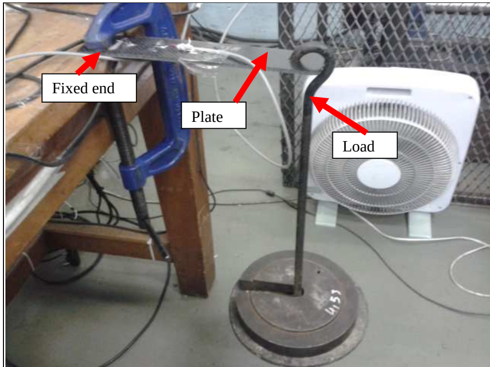
Figure 105. Rig setup for testing the carbon fibre plate.
