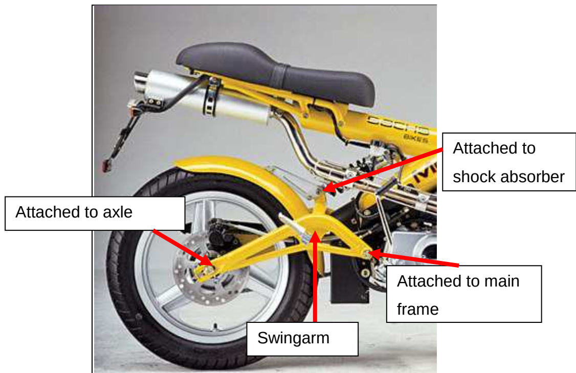
Figure 2. Example of the rear part of a motorcycle showing the swingarm. [4]
