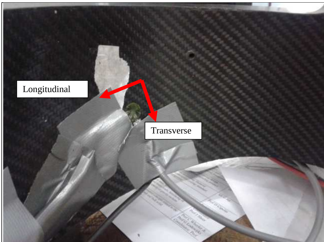
Figure 120. Strain Gauge 3.
