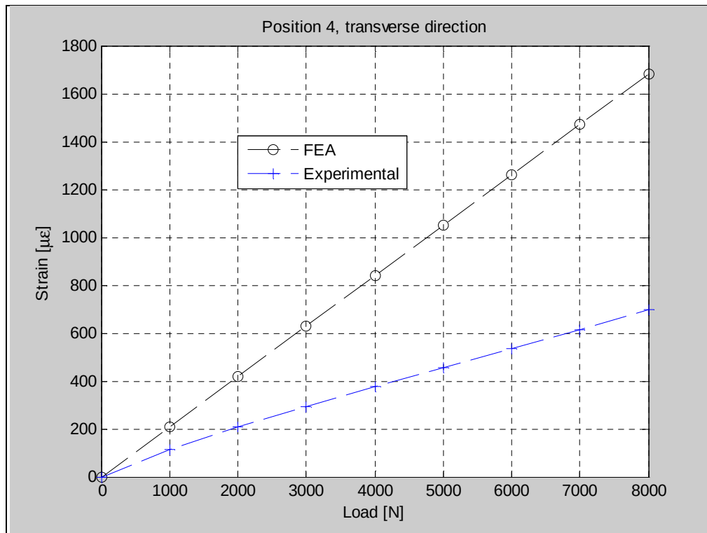
Figure 92. Comparison between FEA and experimental results at Position 4 in the gauge transverse direction.
