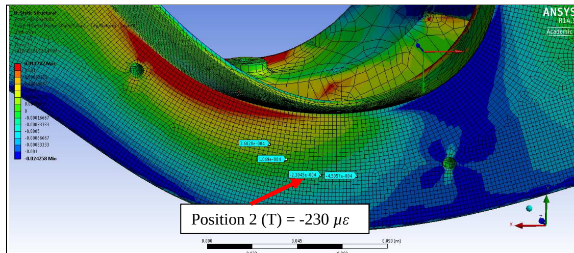
Figure 75. Strain distribution for Position 2 in the gauge transverse direction at vertical load of 8000 N.
