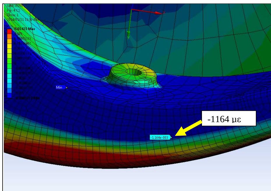
Figure 135. Position 4 with element size of 3 mm.
