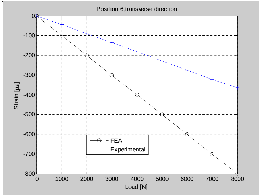
Figure 103. Comparison between FEA and experimental results at Position 6 in the gauge transverse direction.
