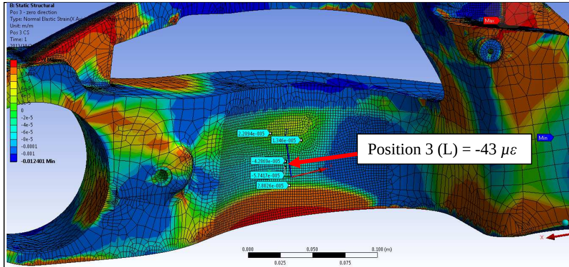
Figure 80. Strain distribution for Position 3 in the gauge longitudinal direction.
