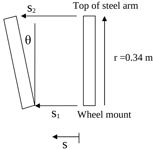
Figure 26. Schematic of deflection of steel arm during torsional loading.
