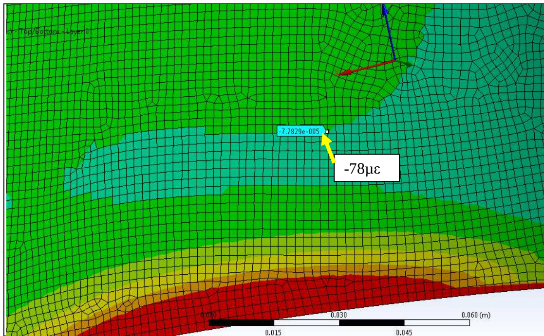
Figure 83. Strain at Position 3 in the longitudinal direction with the axes rotated +2 degrees.
