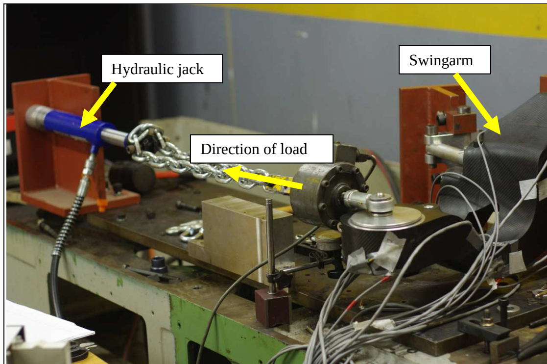
Figure 23. Swingarm test rig to apply vertical load.
