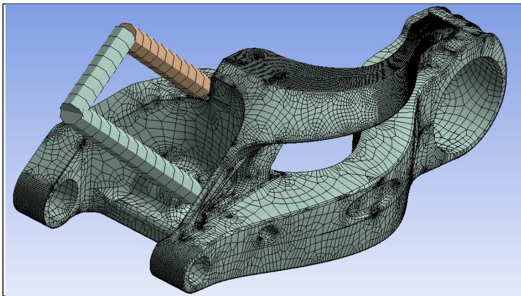
Figure 31. Finite element mesh on the swingarm
