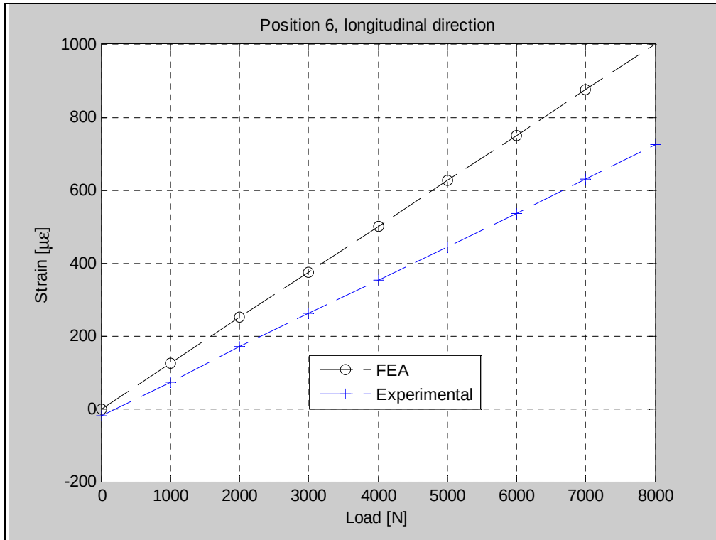
Figure 100. Comparison between FEA and experimental results at Position 6 in the gauge longitudinal direction.
