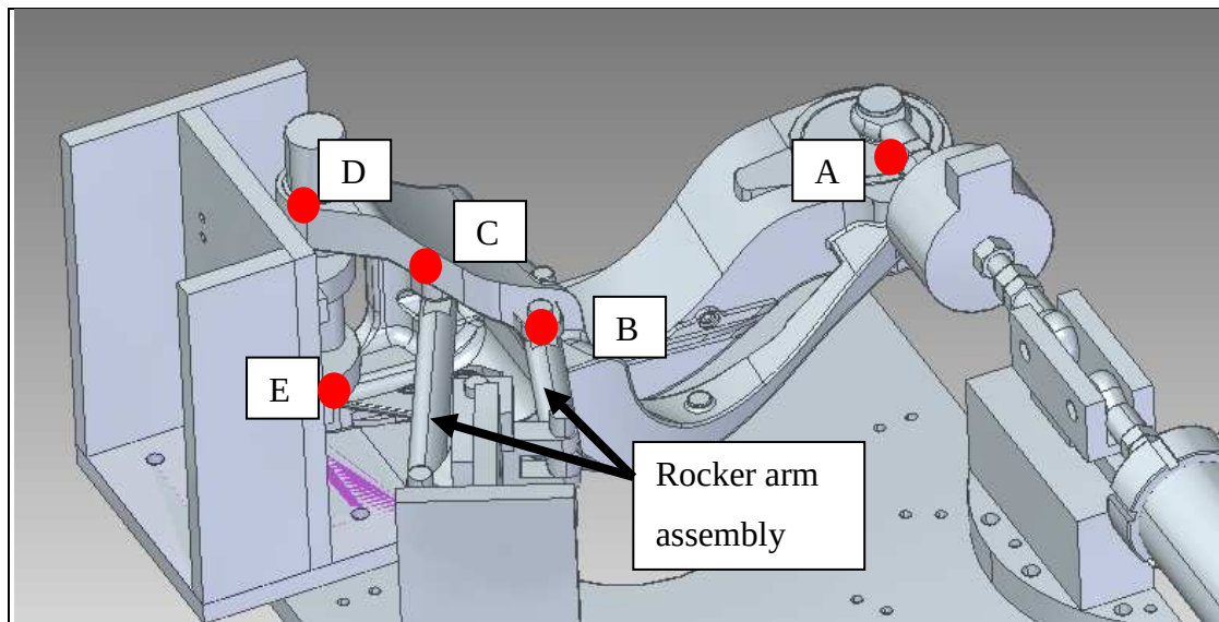
Figure 40. Positions of loading and constraints on the swingarm.
