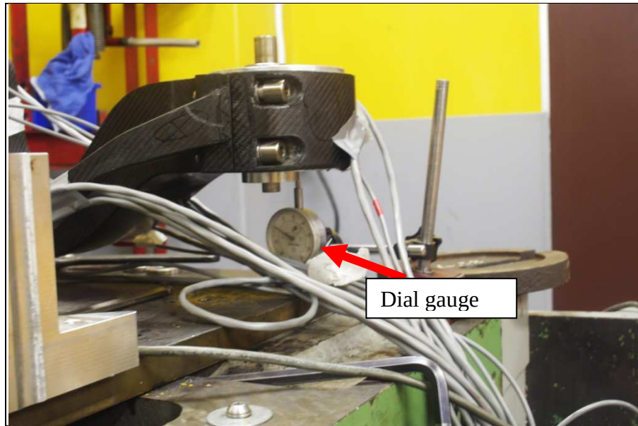
Figure 28. Position of dial gauge during lateral loading test measuring the lateral deflection.
