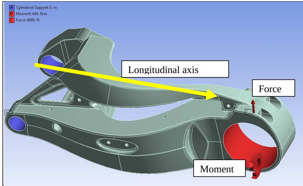
Figure 45. FE model subjected to a moment about the longitudinal x-axis and a force in the motorcycle vertical direction.
