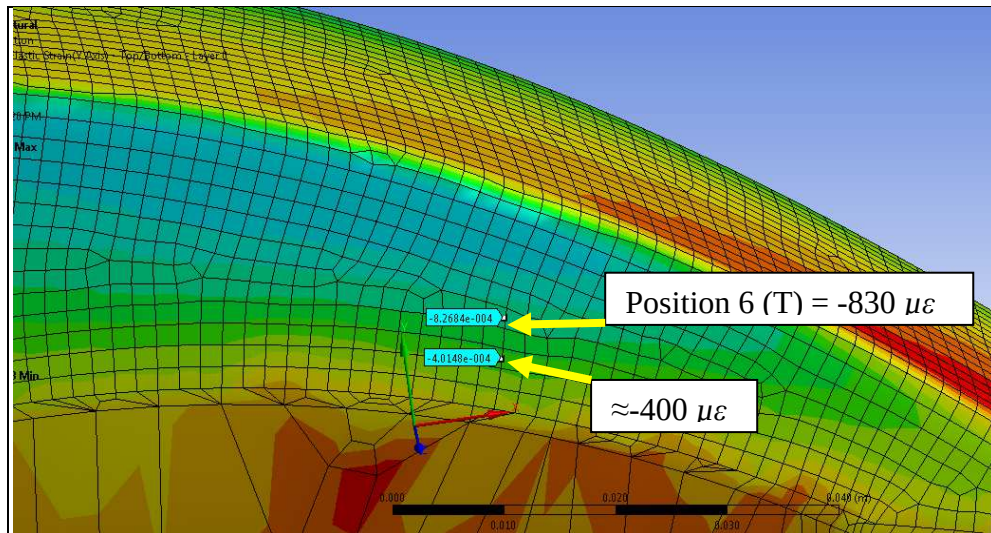
Figure 102. Strain distribution near Position 6 in the gauge transverse direction.
