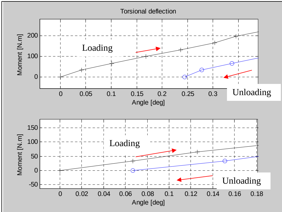
Figure 54. Torsional deflection during loading and unloading near the zero mark.
