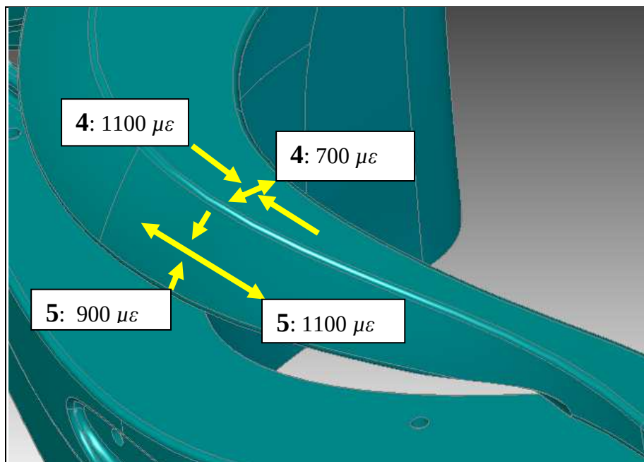
Figure 62. Maximum longitudinal and transverse strain at Positions 4 and 5 during vertical loading.
