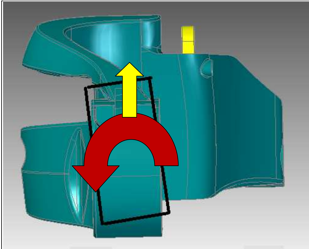
Figure 64. Schematic of the vertical and rotational translation of the swingarm during vertical loading.
