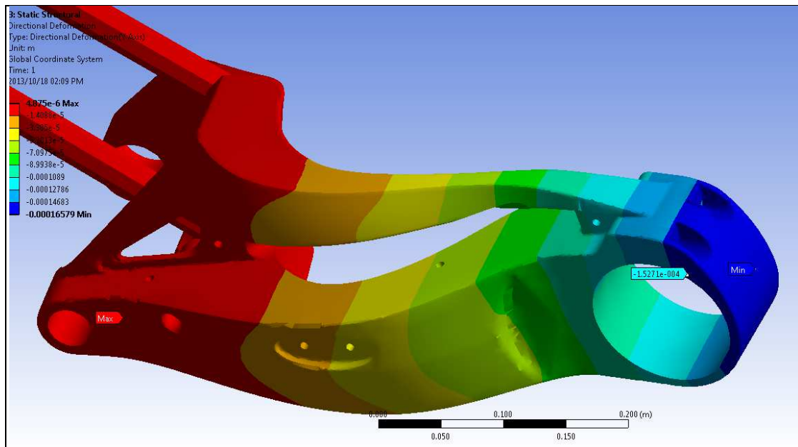
Figure 74. Lateral deflection under the 135 N load.
