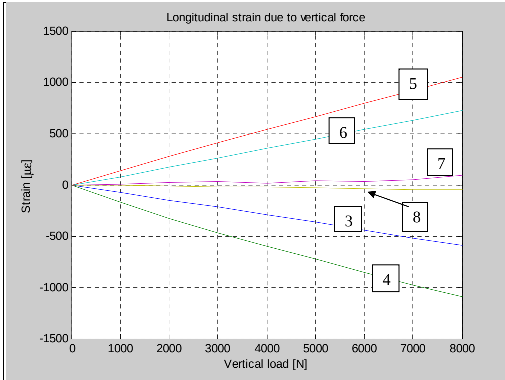
Figure 59. Longitudinal strain measured at positions 3 through 8.
