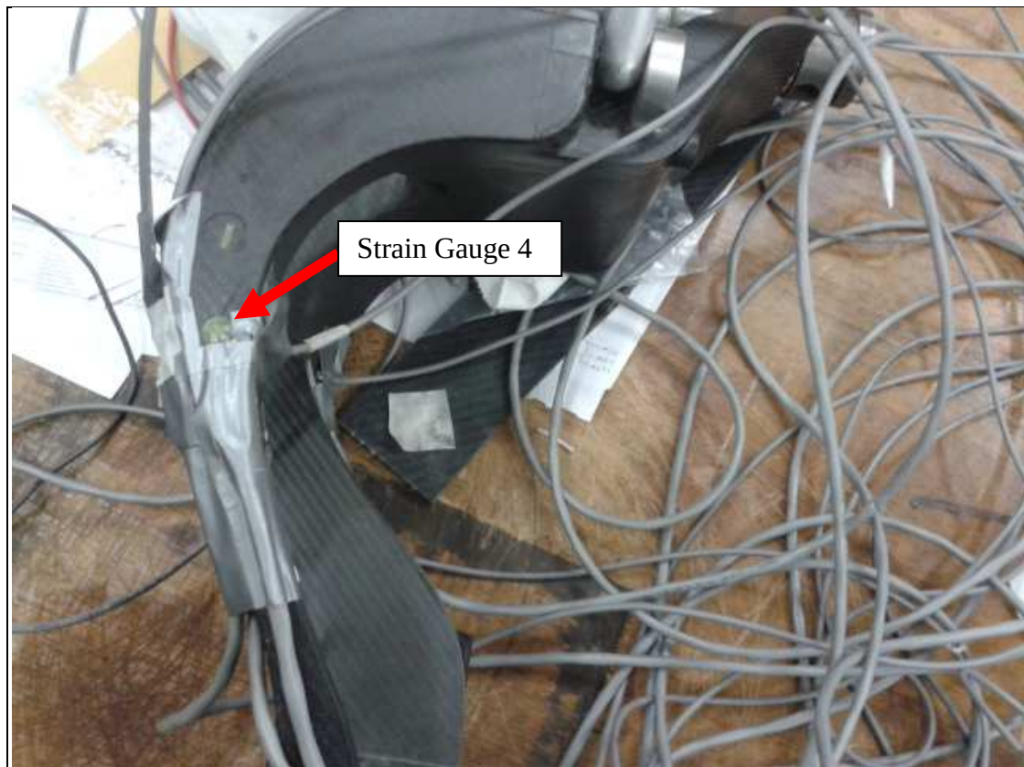
Figure 121. Strain Gauge 4.
