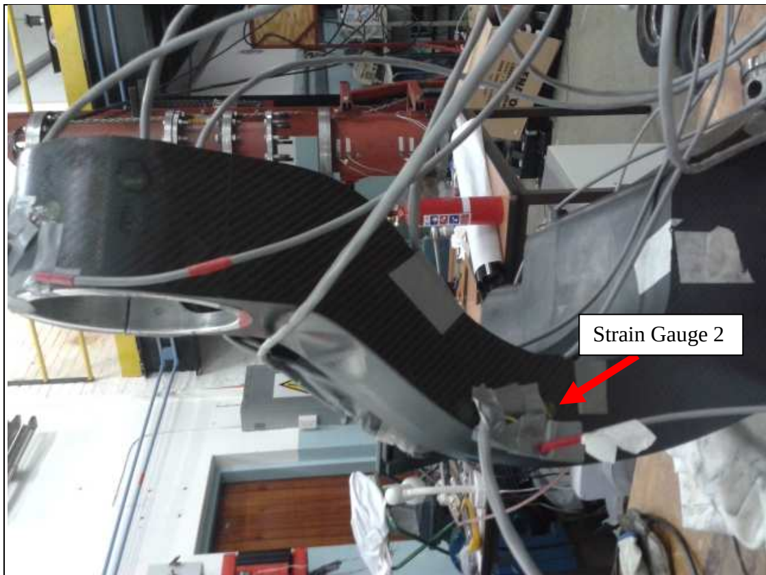
Figure 117. Strain Gauge 2.
