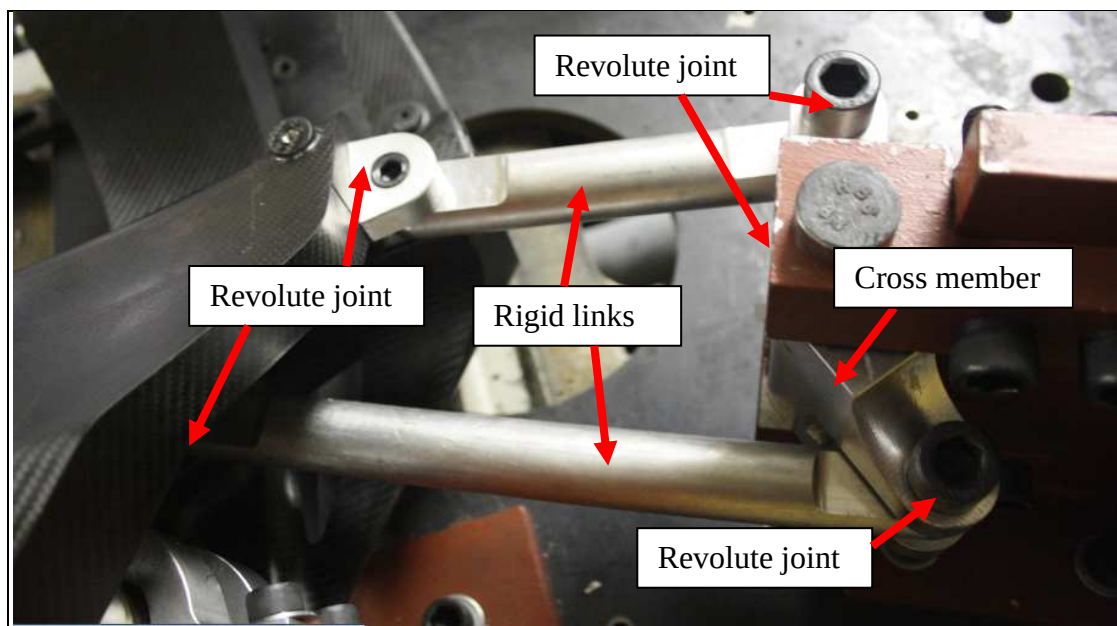
Figure 42. Rocker arm assembly.
