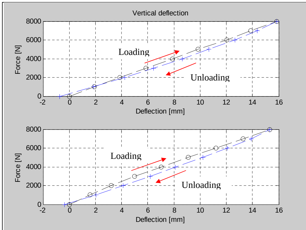
Figure 49. Deflection during loading and unloading of the swingarm
