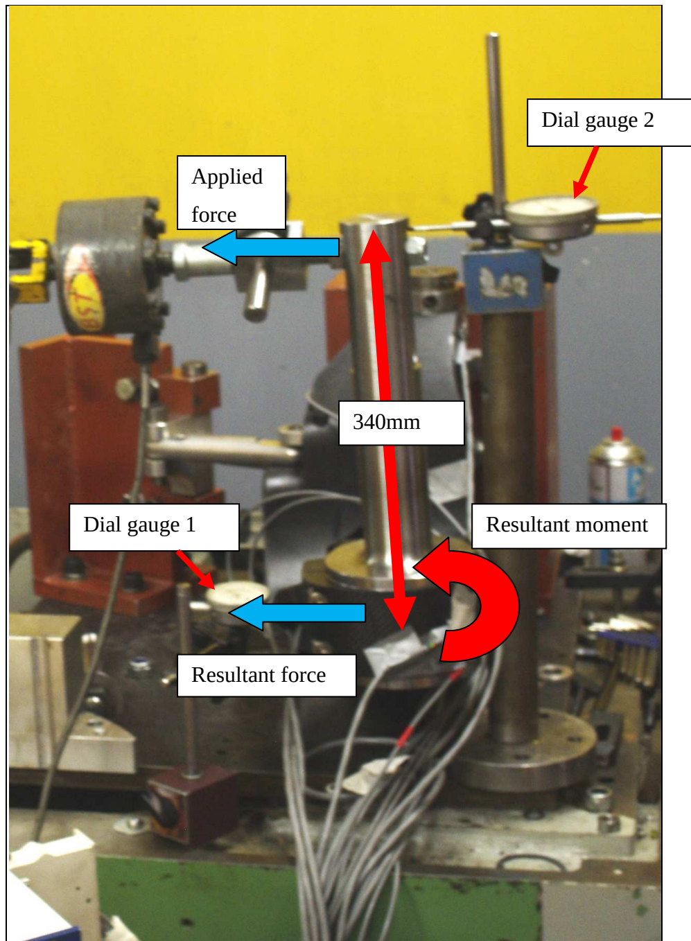
Figure 25. Test rig showing the steel arm used in the torsional test.
