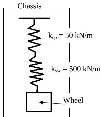
Figure 48. Schematic showing the rear spring and the swingarm as springs in series between the chassis and the wheel.
