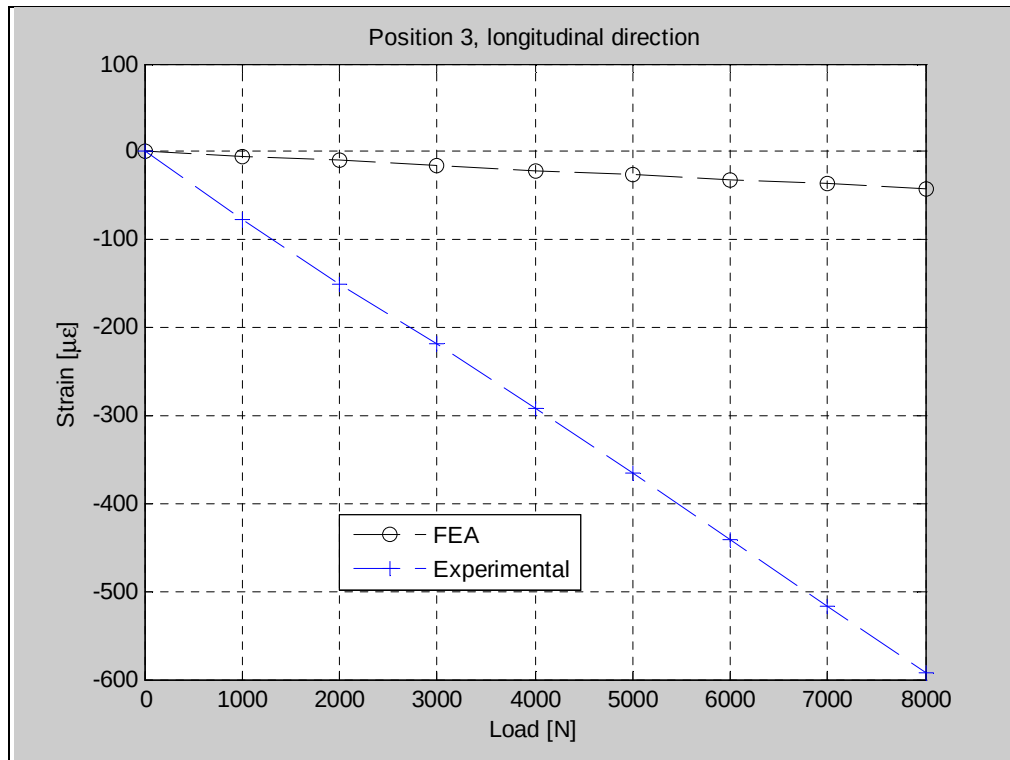
Figure 82. Comparison between FEA and experimental results at Position 3 in the gauge longitudinal direction.
