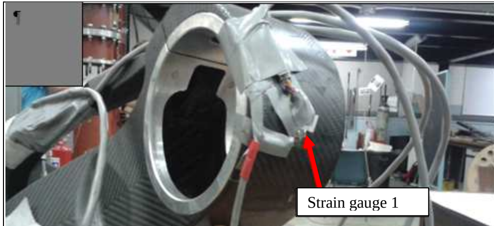
Figure 115. Strain Gauge 1
