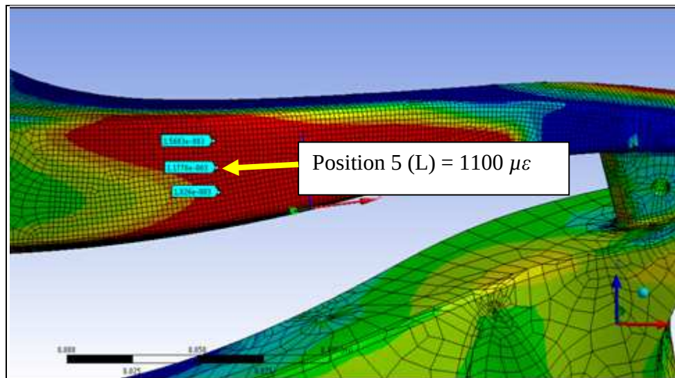
Figure 95. Strain distribution for Position 5 in the gauge longitudinal direction.
