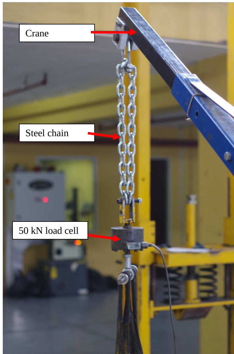
Figure 110. Top part of the load cell calibration rig showing the load cell attached to the portable crane via a steel chain.
