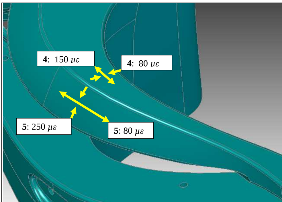
Figure 69. Maximum longitudinal and transverse strain at Positions 4 and 5 during torsional loading.
