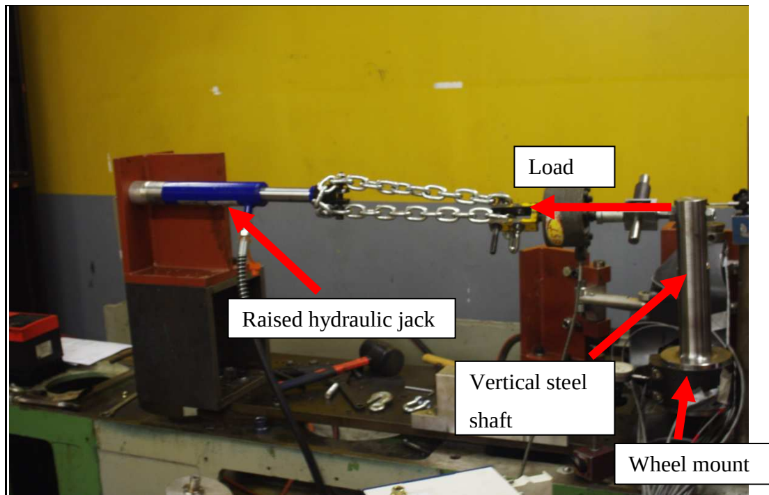
Figure 24. Rig setup to apply a torsional load on swingarm.
