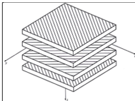
Figure 6. Example of carbon fibre composite sketch showing different layers orientated in different directions. [17]
