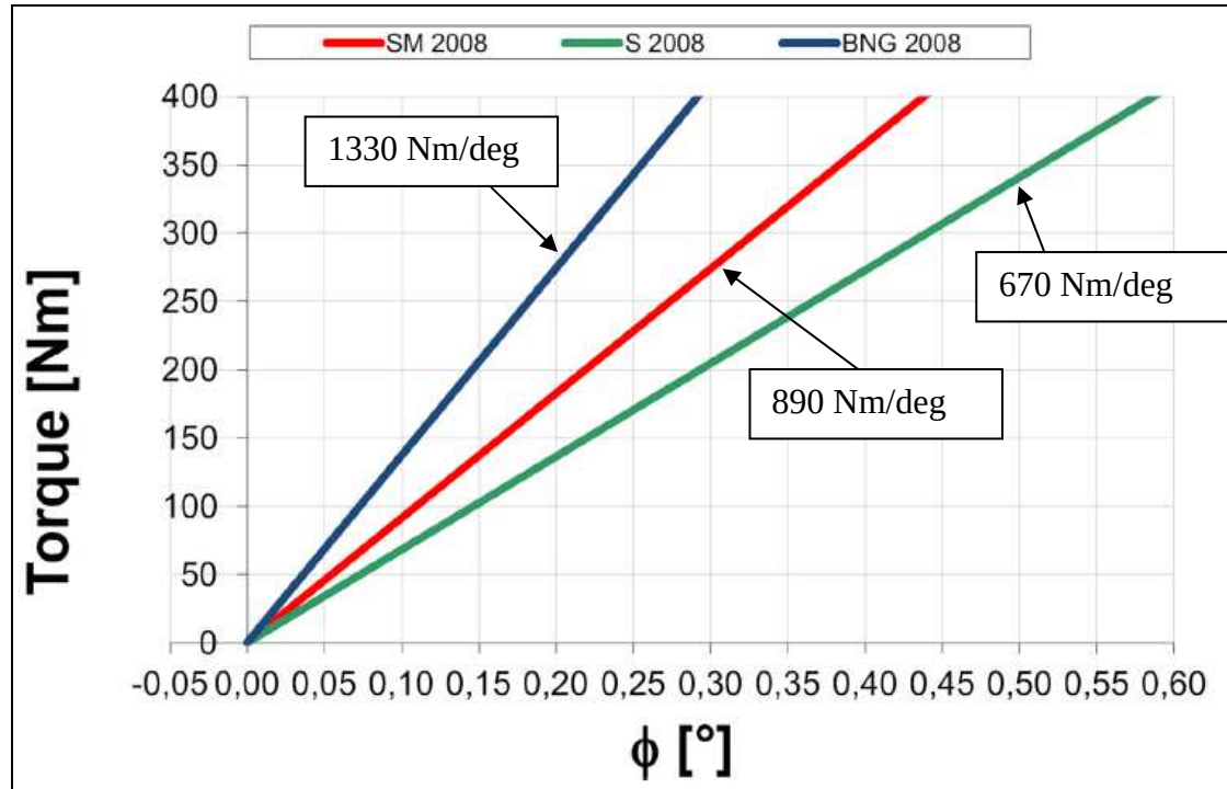
Figure 16. Torque-angle curves for three swingarms [5]
