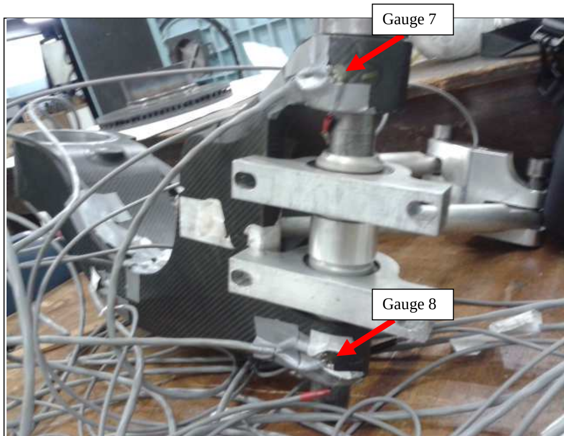
Figure 127. Strain Gauges 7 & 8.
