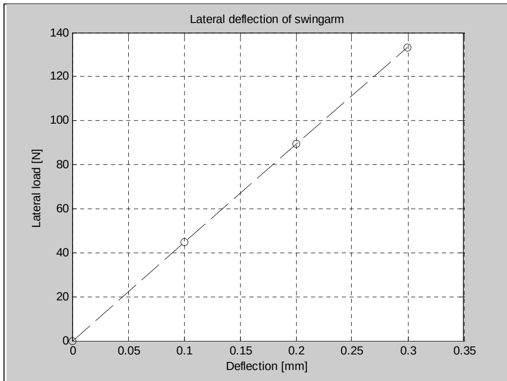
Figure 55. Lateral deflection of the swingarm.
