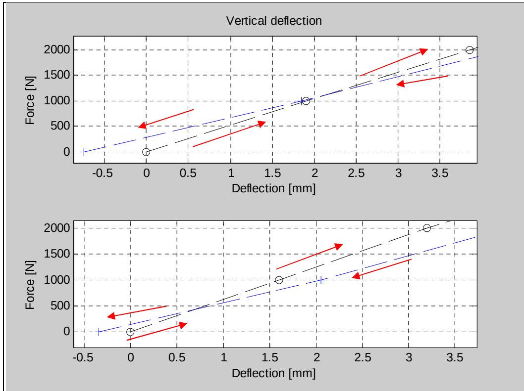
Figure 50. Deflection during loading and unloading near the zero load mark.
