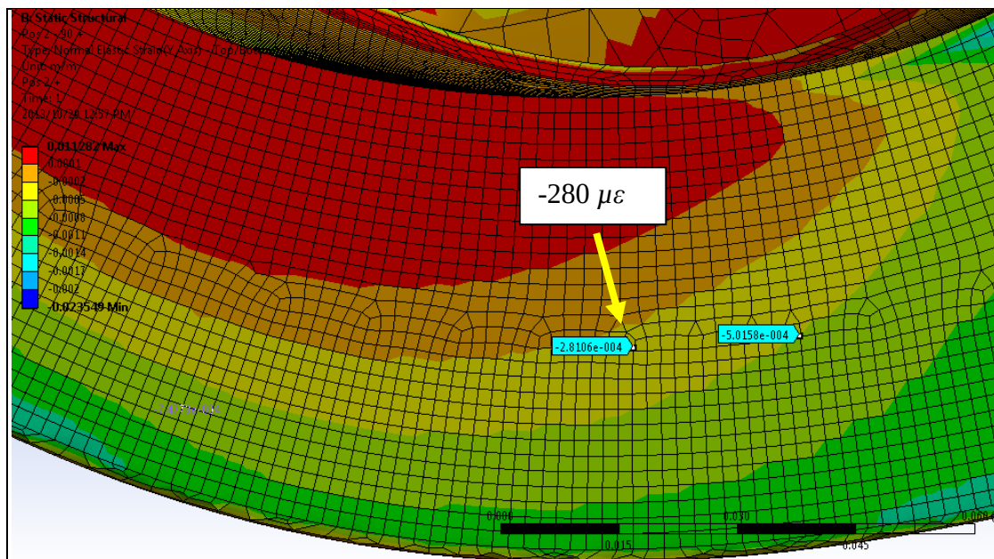
Figure 78. Position 2 in the transverse direction with the axes rotated +2 degrees.
