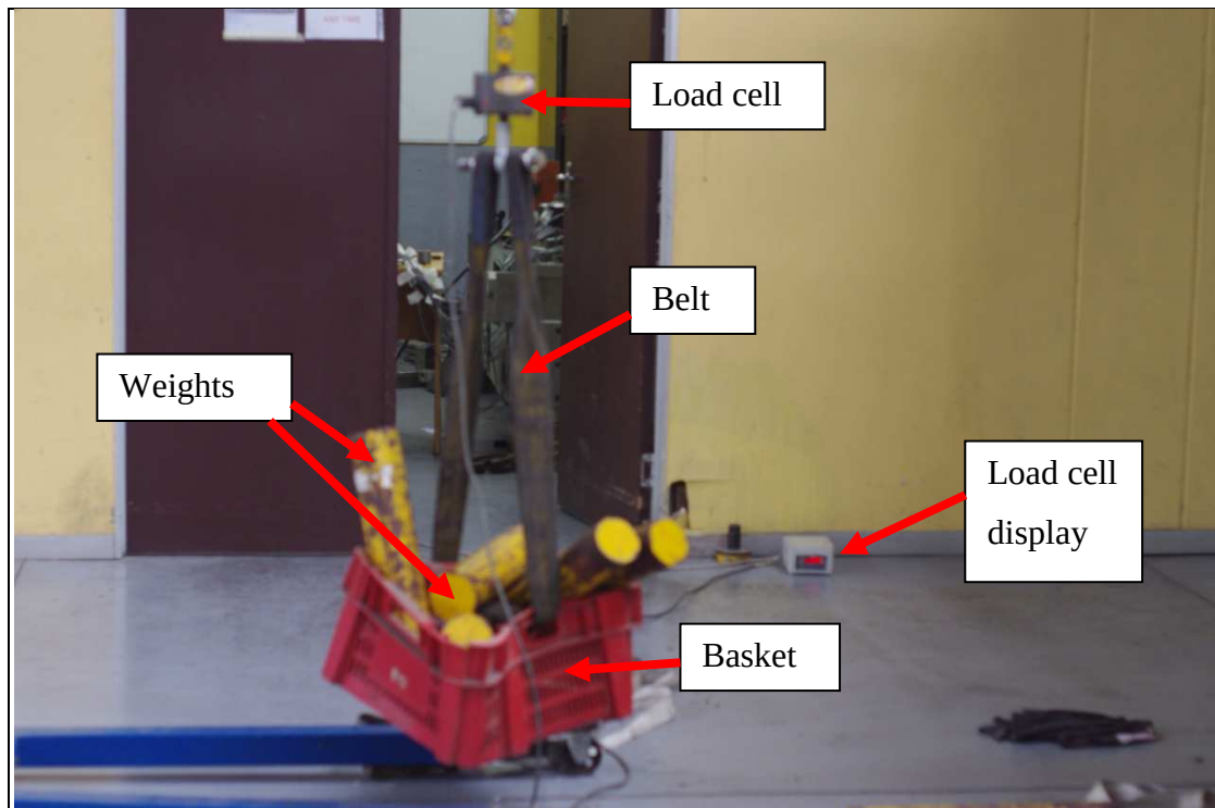
Figure 111. Basket carrying weights applying a load to the load cell.
