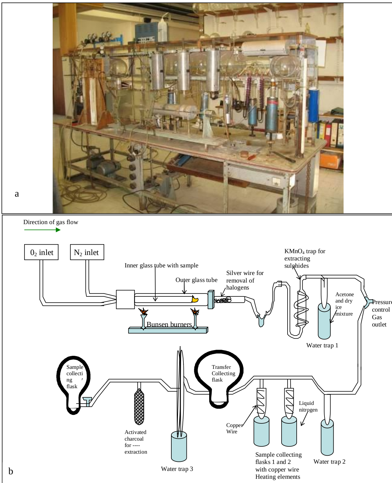
Figure 4.2 Photograph (a) and schematic diagram (b) of The Bench apparatus used for the purification and isolation of Carbon dioxide for carbon 14 analysis.
