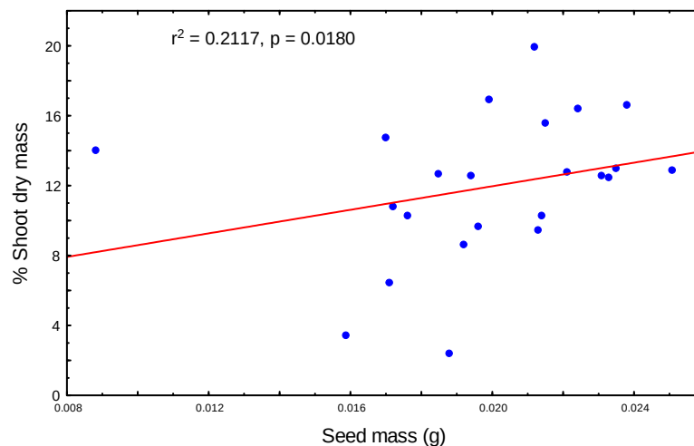
Figure 5.16. The relationship between seed mass and % allocation to shoot dry mass for seedlings of P. simplex (the outlier 0.008g/seed is shown) ( n=23 , p<0.05 ).
