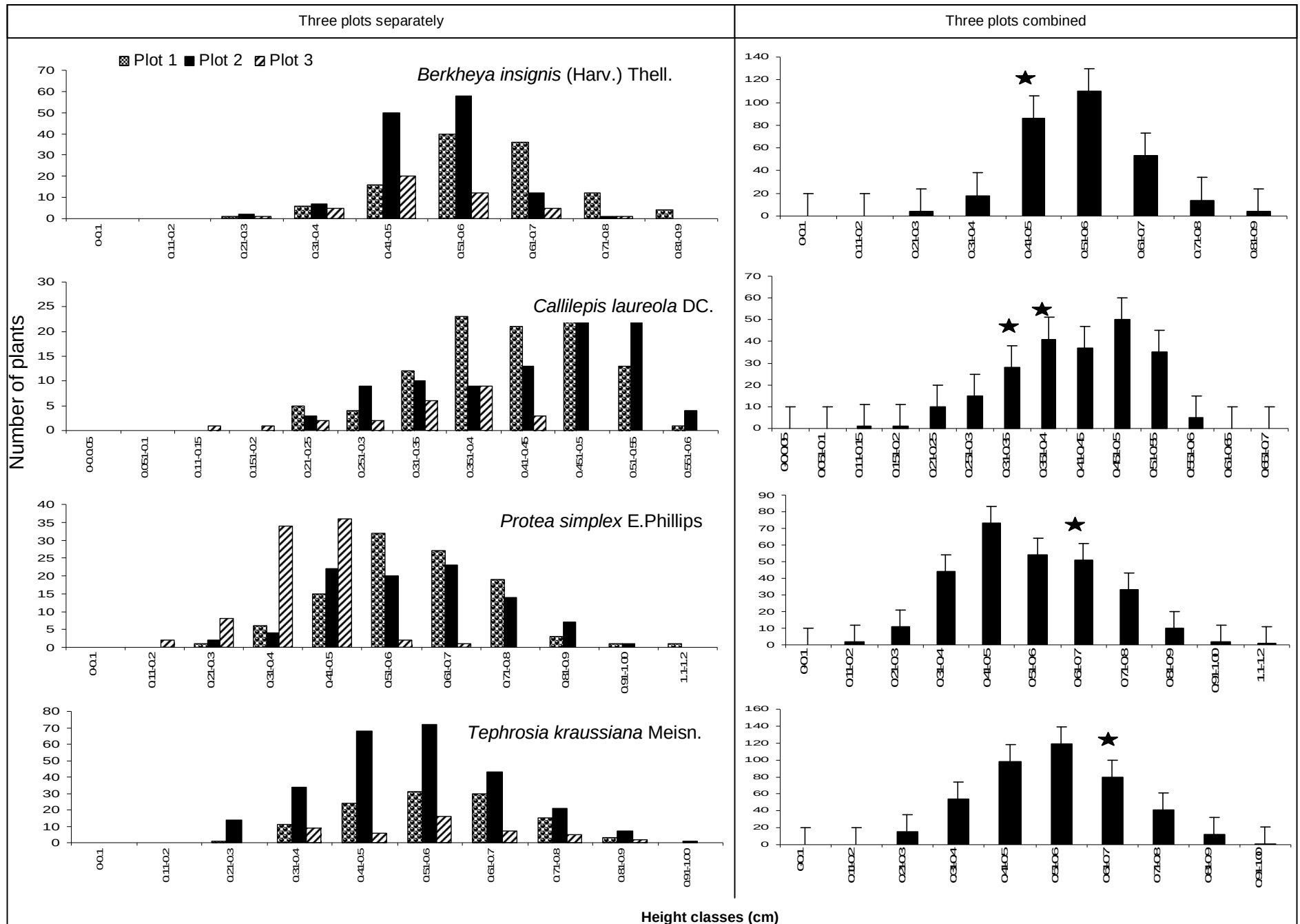
Figure 5.23. Distribution of the number of plants in each class showing height for B. insignis , C. laureola , P. simplex and T. kraussiana . Distributions were constructed for the 3 field plots separately and then for all 3 plots combined (mean \pm SE). ★ Indicates where the sizes of radiocarbon dated plants fall.
