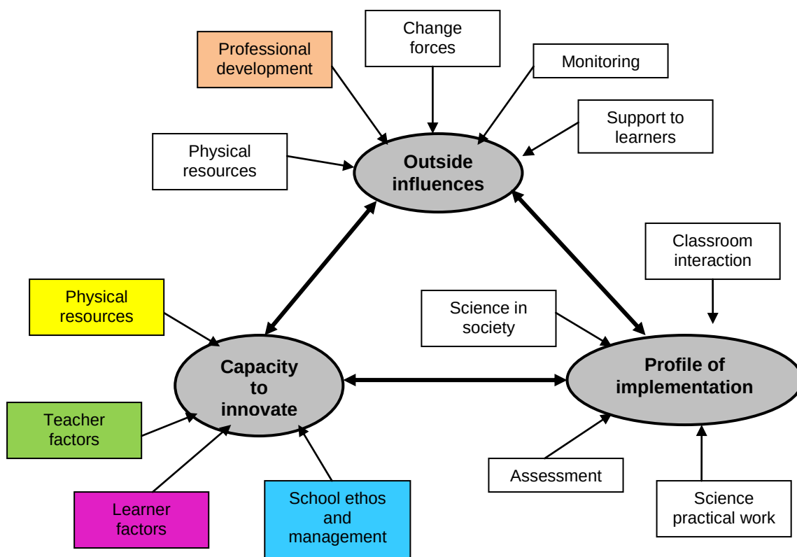
Figure 3.1: Rogan and Grayson's Theoretical Framework for curriculum implementation in developing countries (Rogan & Aldous, 2005, p. 314)
