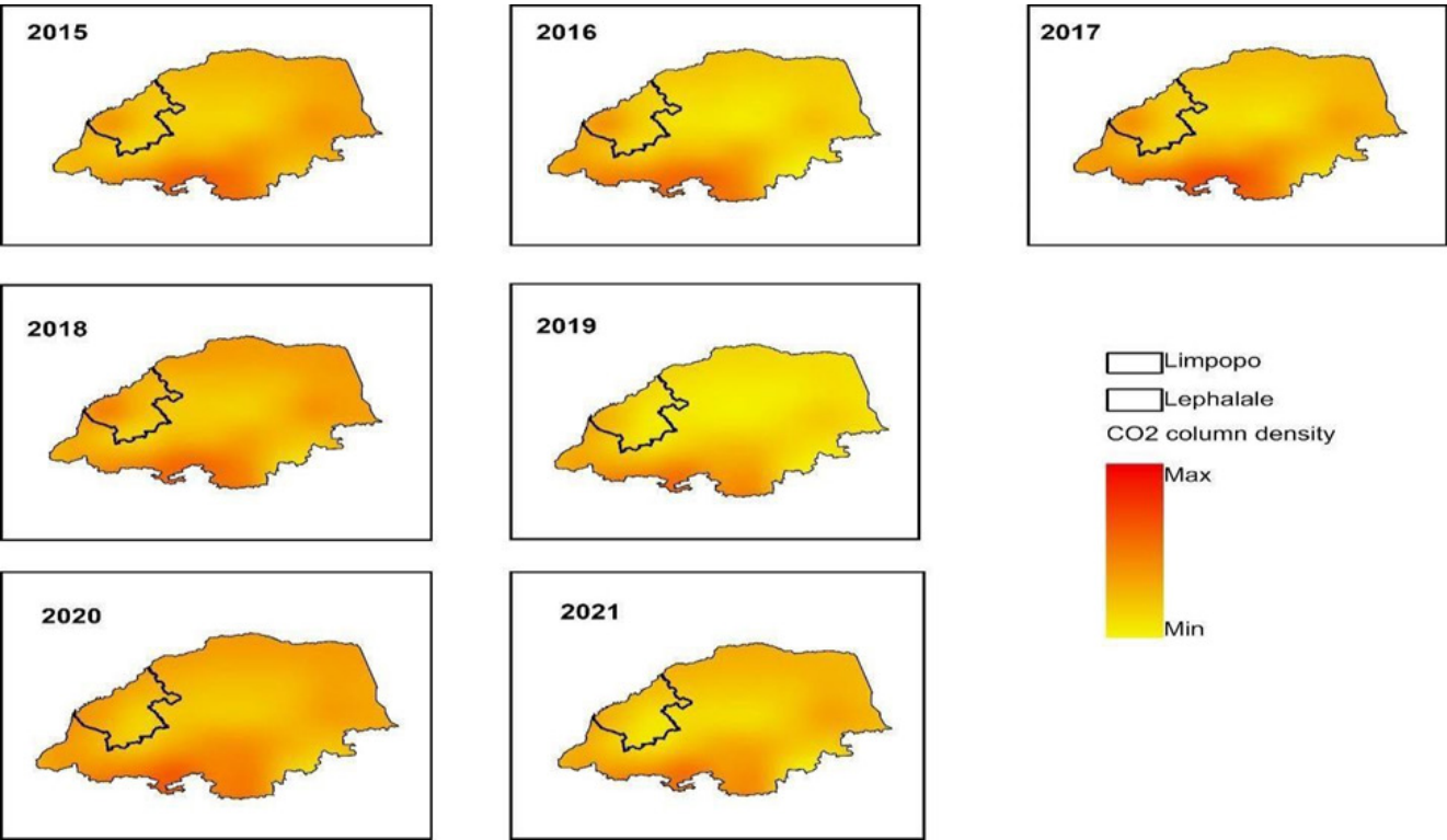
Figure 5: CO 2 column density (mol CO 2 /mol dry) trends over Lephalale from 2015-2021, as observed by GEOS-Chem.
