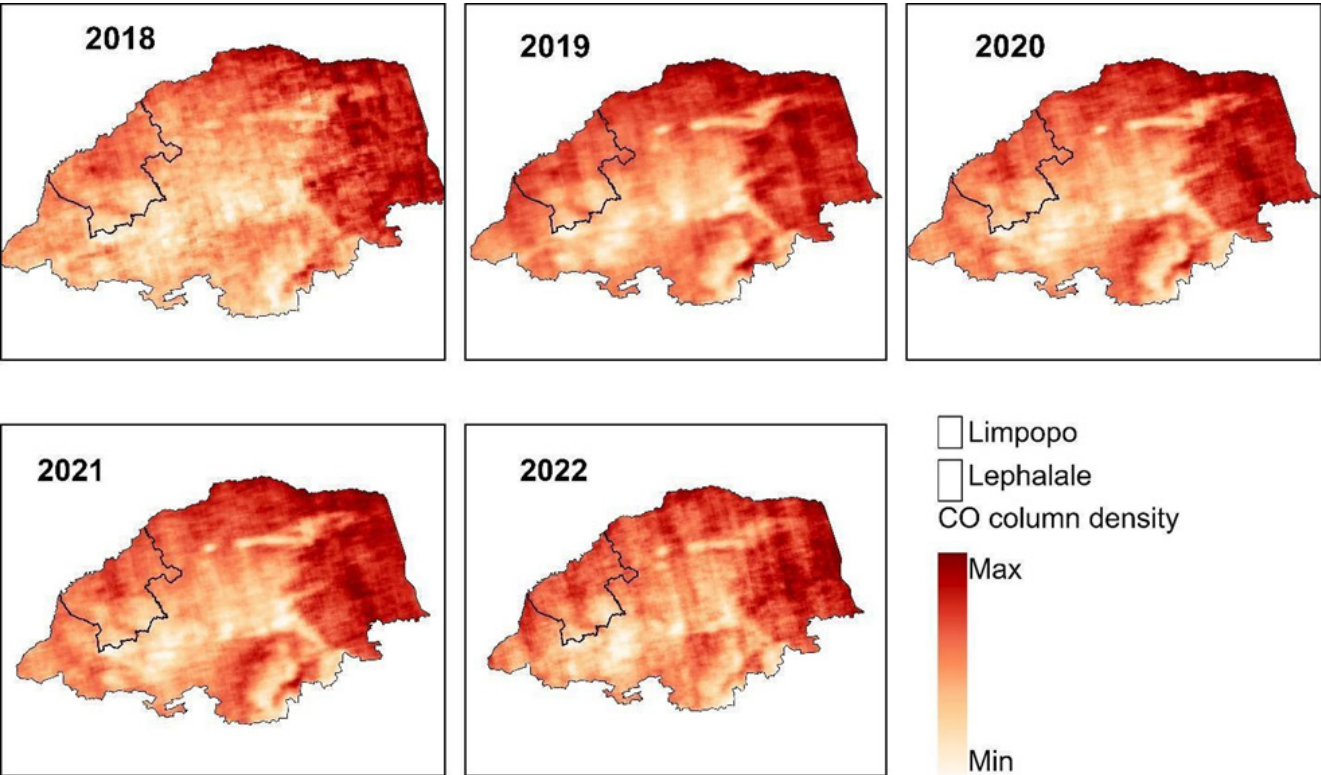
Figure 4: CO column density (mol/m 2 ) trends over Lephalale from 2018-2022 from Sentinel-5P.
