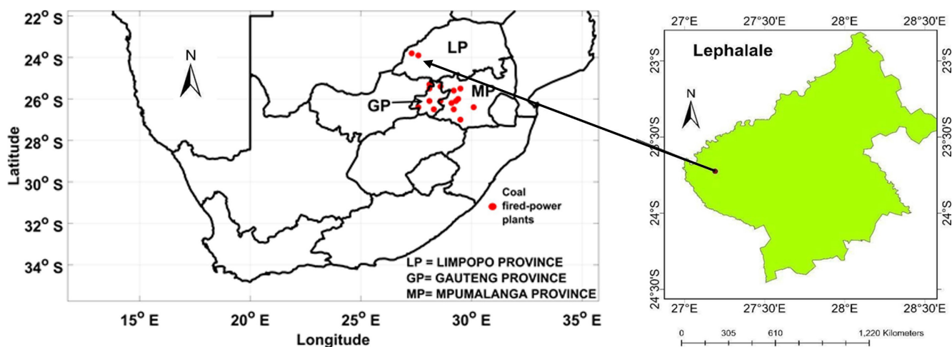
Figure 1: Map showing the coal-fired power stations that serve as \text{SO}_2 , \text{NO}_2 , CO and \text{CO}_2 emitters in Limpopo and South Africa
