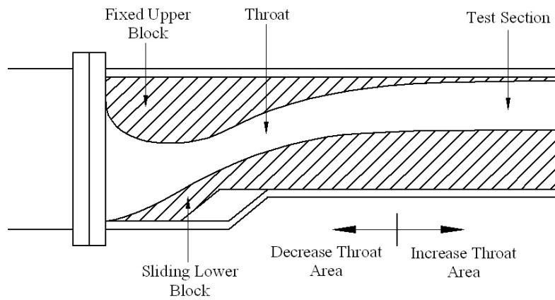
Figure 4.6: Schematic representation of the sliding block first throat
