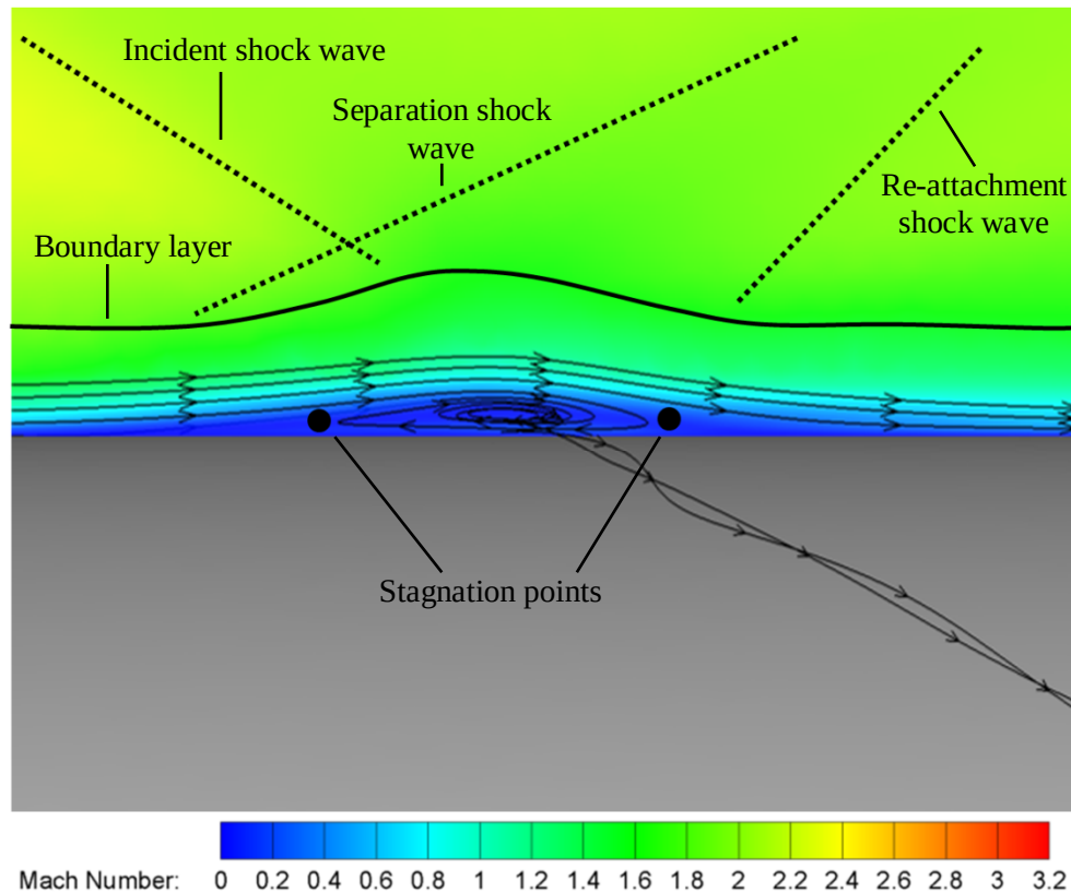
Figure 6.68: Superposition of the stagnation points and the flow within the separated region
