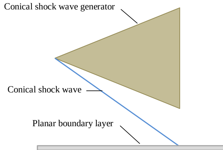
Figure 3.13: Schematic of a conical shock wave interacting with a planar boundary layer
