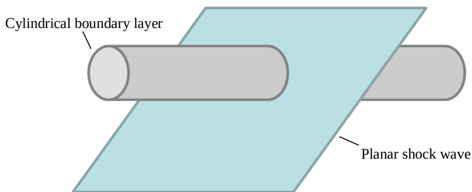
Figure 3.14: Schematic of a planar shock wave interacting with a cylindrical boundary layer
