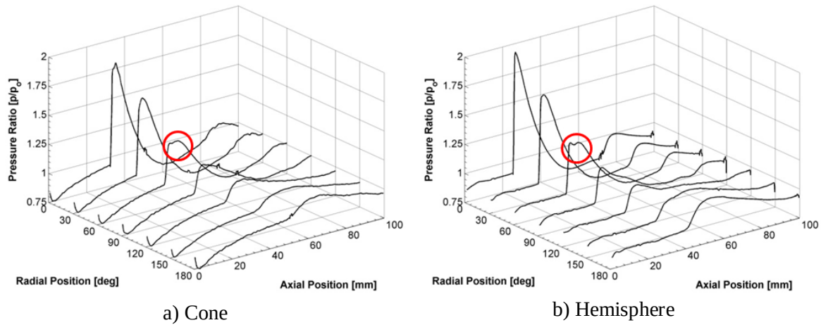
Figure 6.39: Secondary pressure bump location in pressure distribution curves
