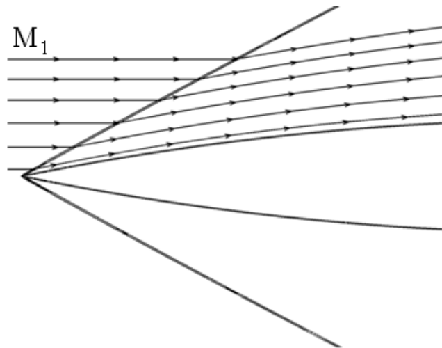
Figure 3.5: Supersonic flow past an ogive
