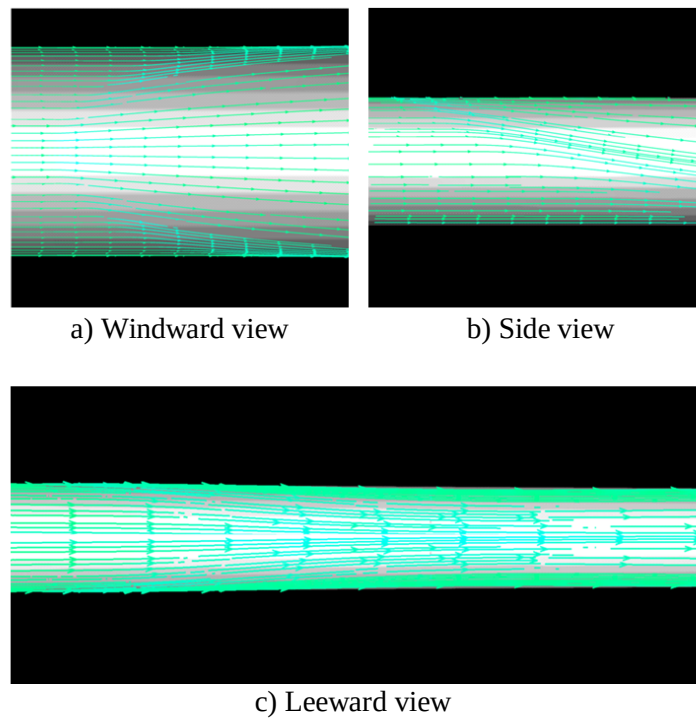
Figure 6.19: CFD Surface flow streamlines, Ogive
