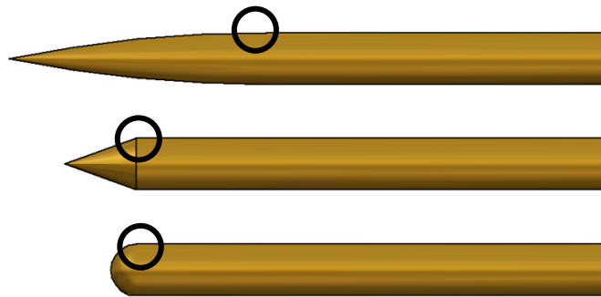
Figure 6.38: Intersection of nose profile and cylindrical section forming an expansion fan
