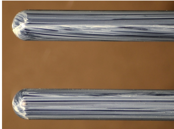
Figure 4.11: Oil surface flow mixture when applied to the models
