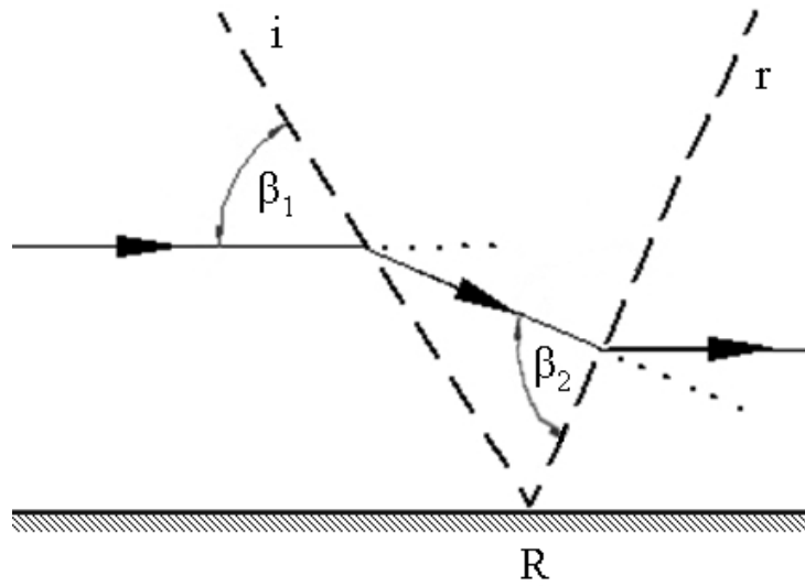
Figure 3.7: Regular reflection wave configuration
