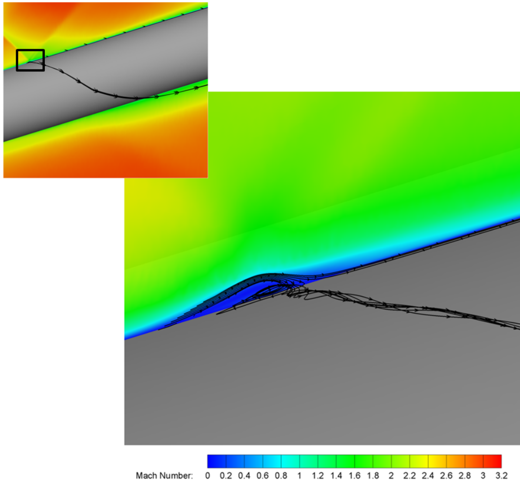
Figure 6.62: High resolution CFD streamlines within separated region, Hemisphere
