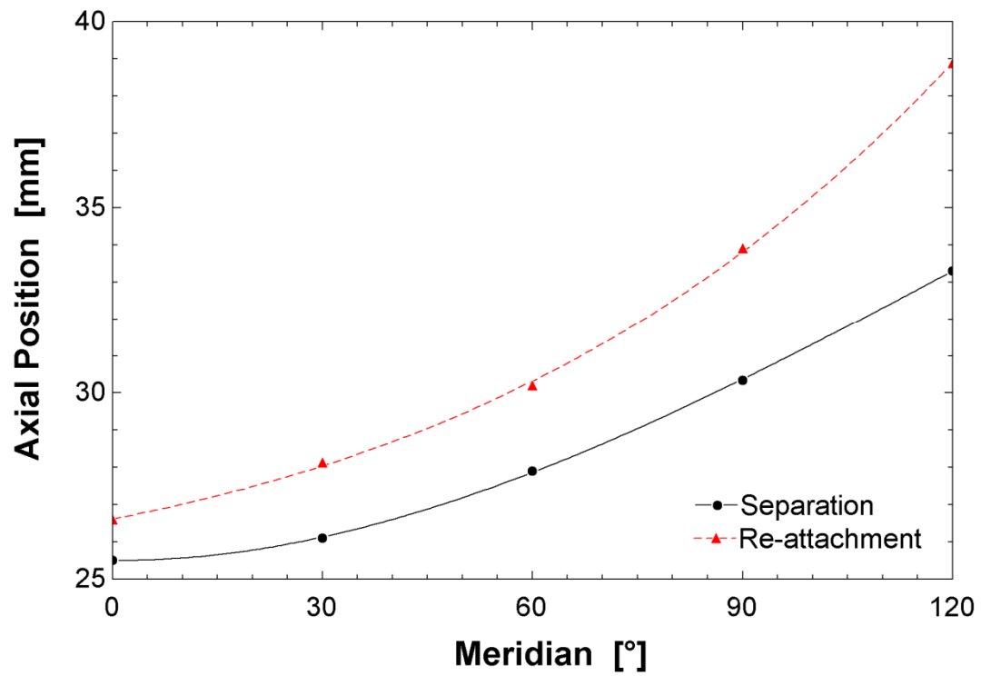
Figure 6.37: Separation and attachment co-ordinates for SWBLI, Hemisphere
