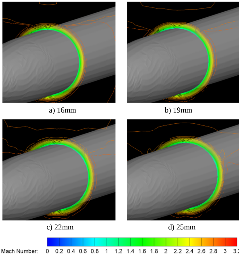
Figure 6.6: Mach number contour line plots transverse to the axis of the cylinder, Ogive (sub-captions indicate the axial distances from the nose)
