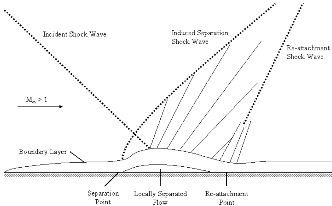
Figure 3.11: Anatomy of a SWBLI with separation
