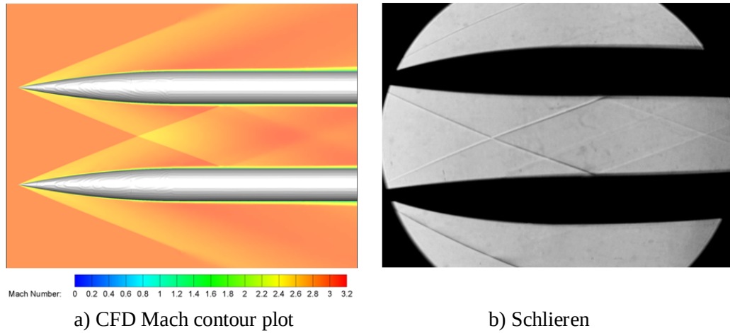
Figure 6.4: SWBLI on the 0° meridian, Ogive
