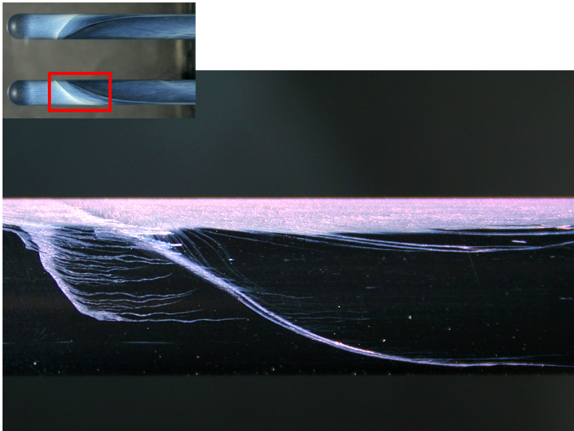
Figure 6.25: Oil surface flow within the separated region, Hemisphere
