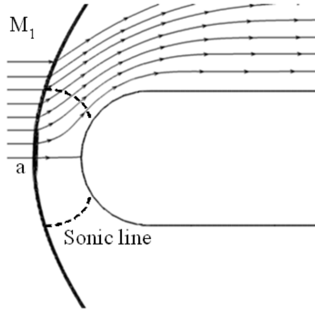
Figure 3.6: Supersonic flow past a hemisphere
