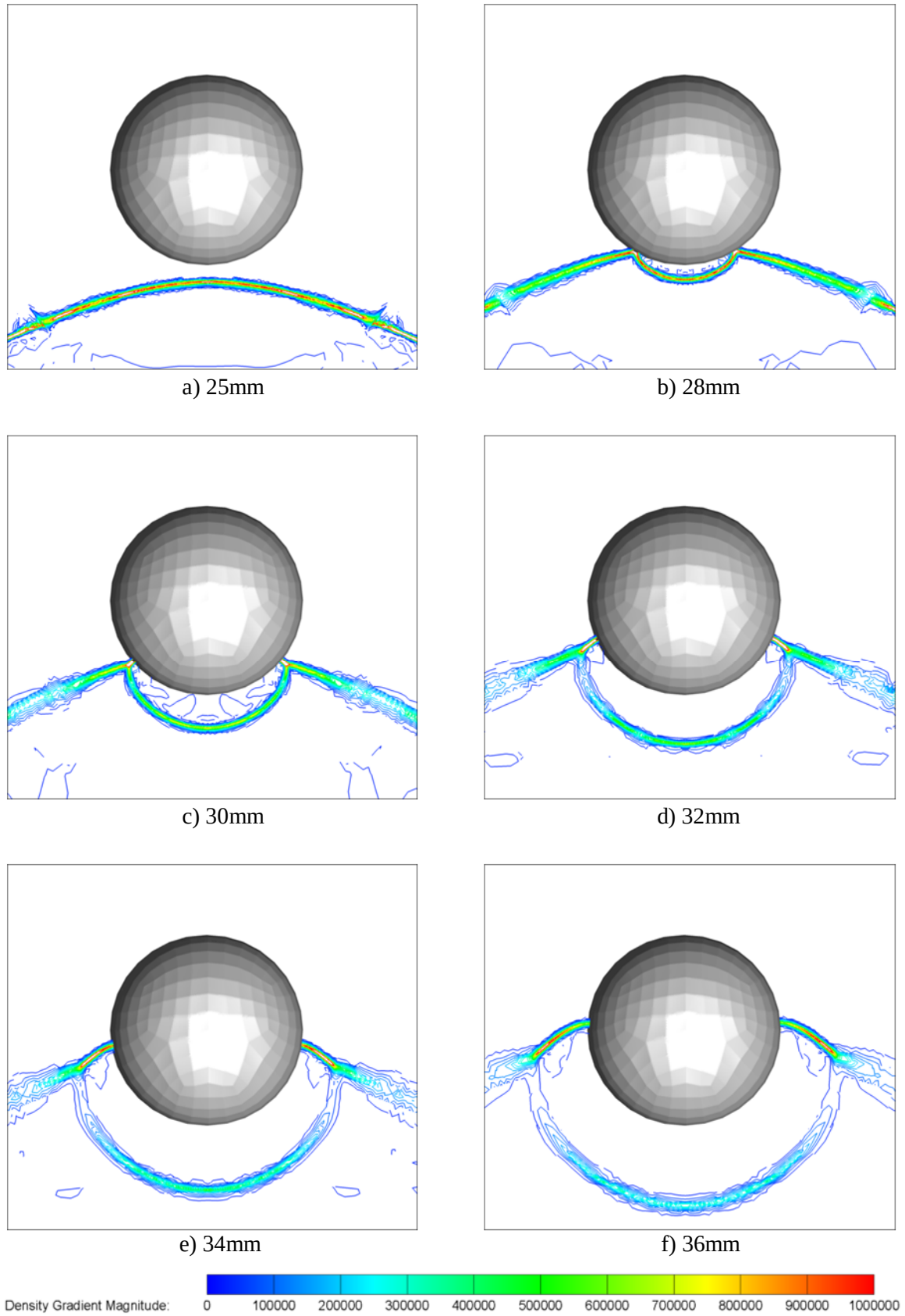
Figure 6.49: Inviscid simulation - density gradient contour lines
