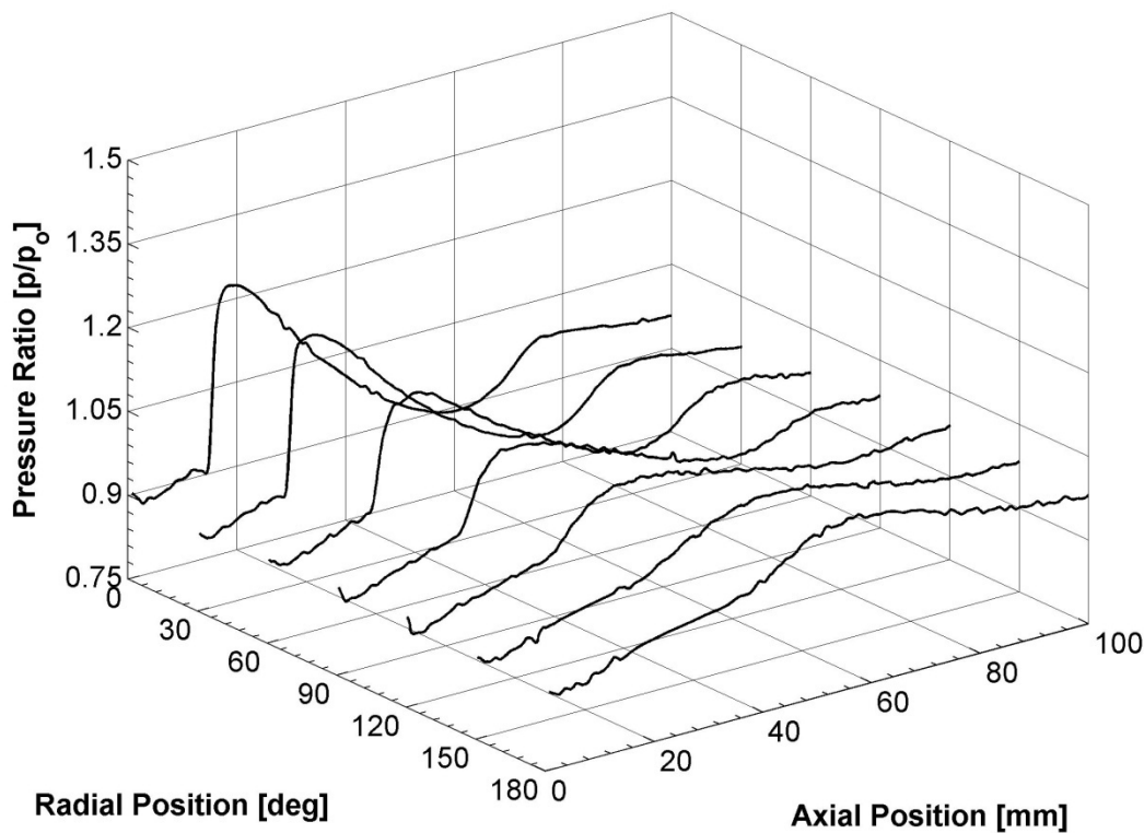
Figure 6.33: Surface pressure distribution, Ogive
