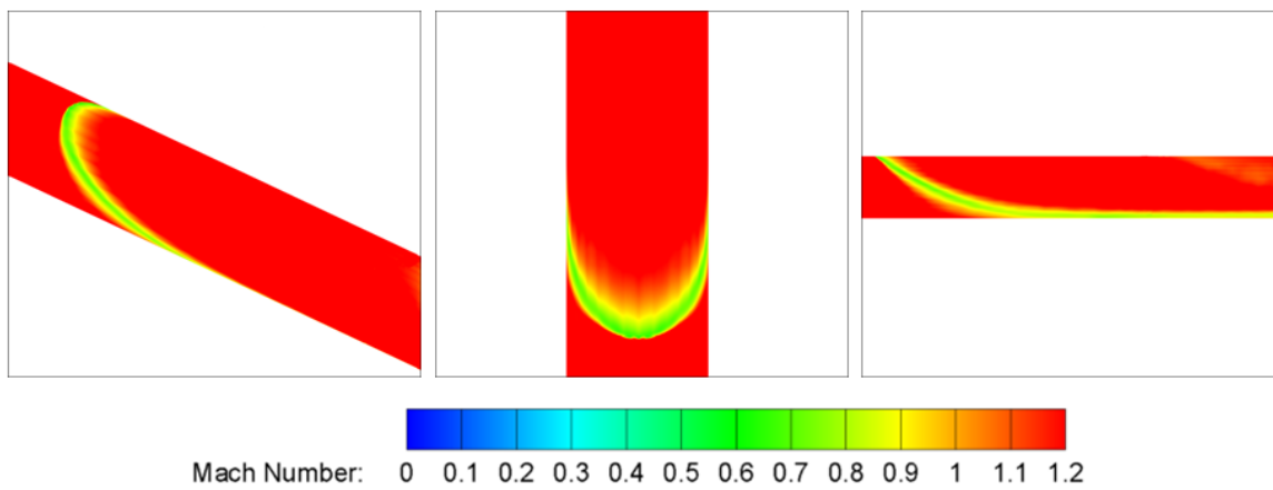
Figure 6.26: Surface flow visualisation, Hemisphere
