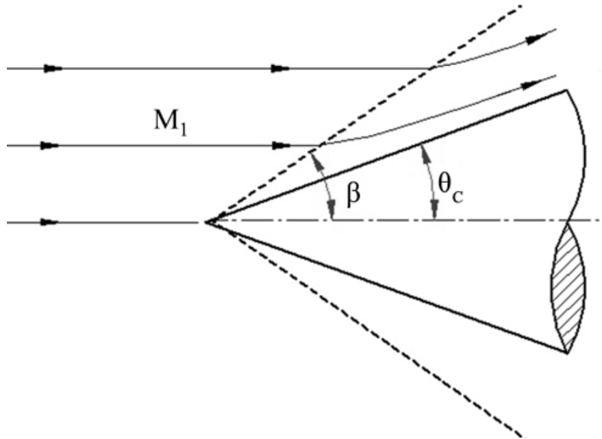
Figure 3.3: Supersonic flow past a cone
