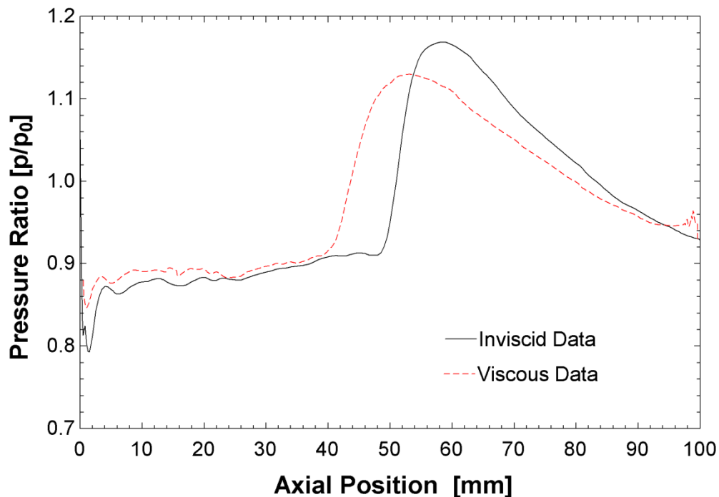
Figure 6.56: Lee-side (180° meridian) pressure distribution, Hemisphere
