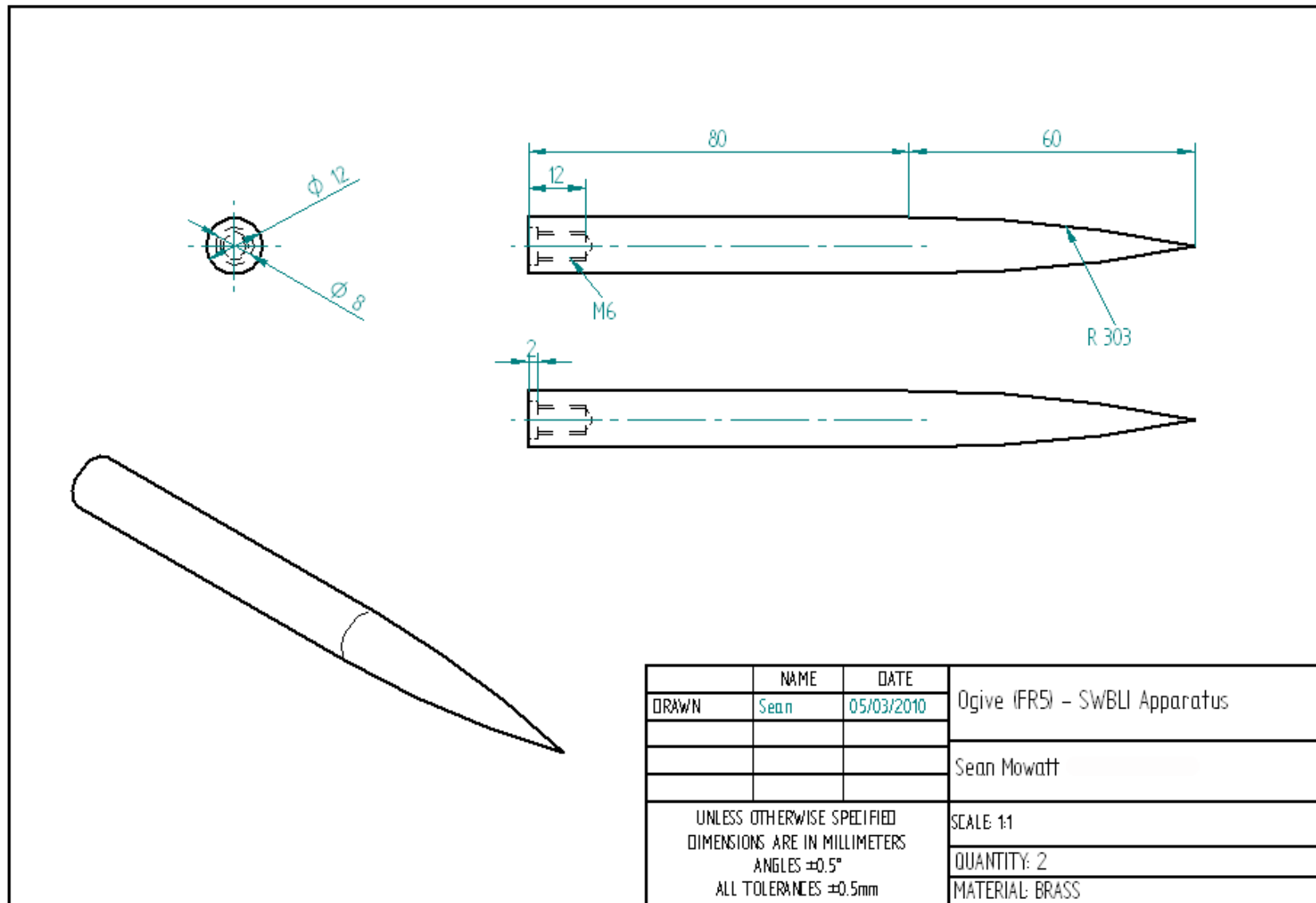
Figure C 1: Manufacturing drawings for the ogive SWBLI generator
