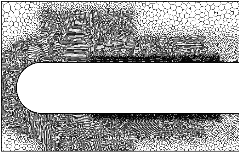
Figure 4.15: Star-CCM+ structured mesh
