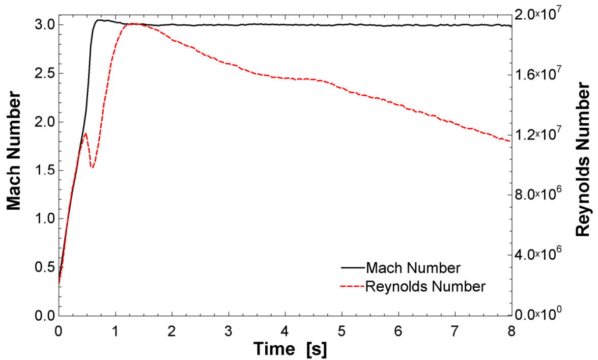
Figure A 9: Mach and Reynolds number variation during a wind tunnel test, Mach 3.0
