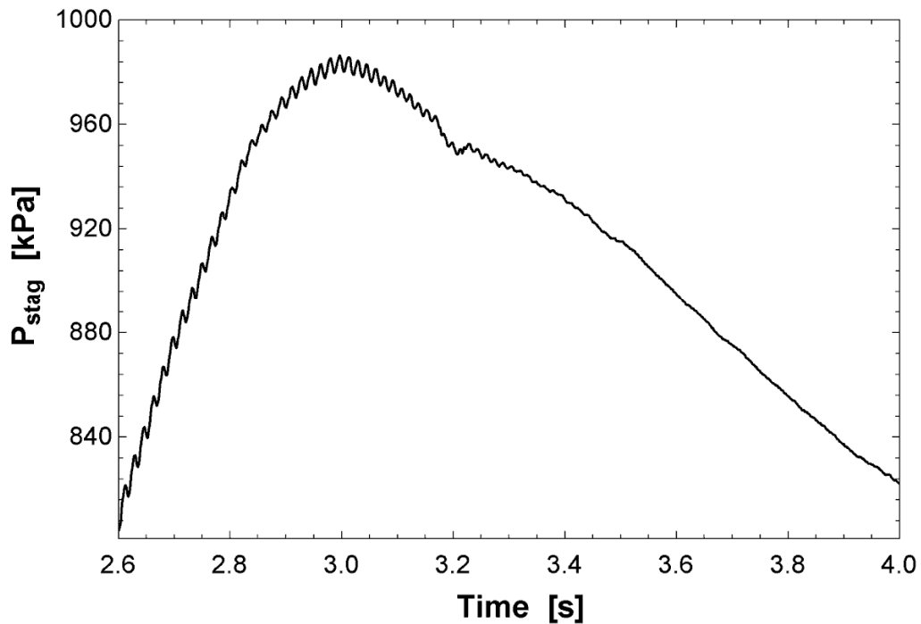
Figure A 6: Pressure trace showing vibration (August 2009)
