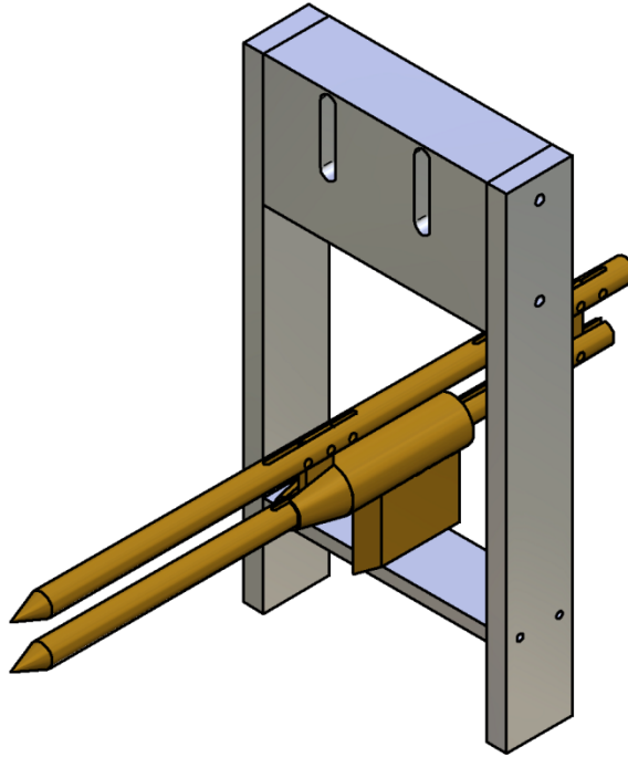
Figure 4.12: SWBLI generators and mounting bracket
