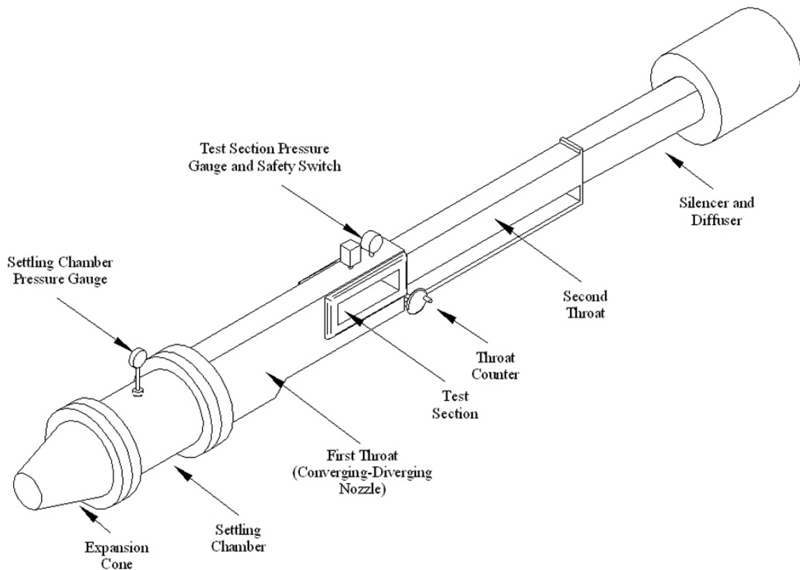
Figure 4.1: Schematic layout of the supersonic wind tunnel
