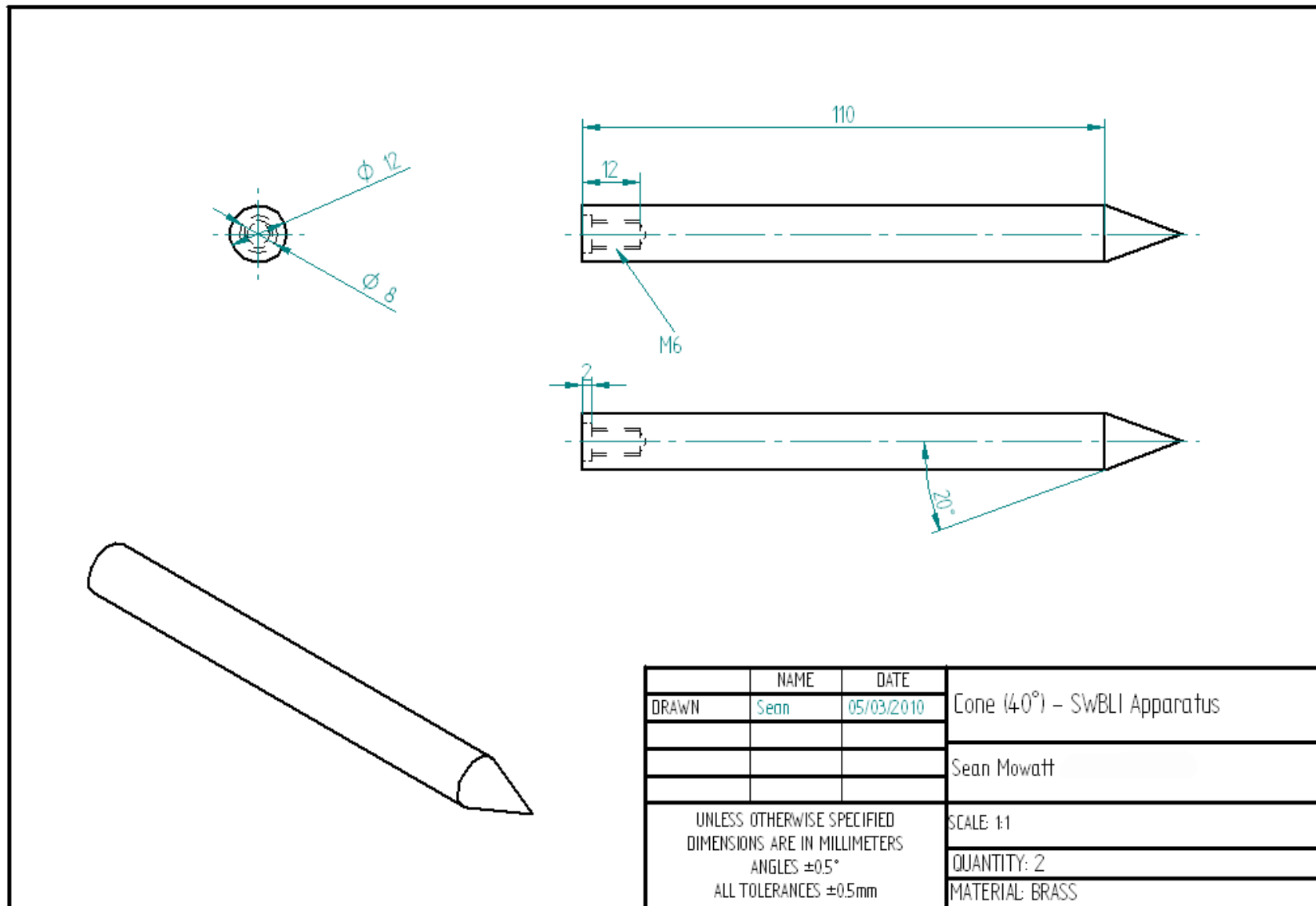
Figure C 2: Manufacturing drawings for the conical SWBLI generator
