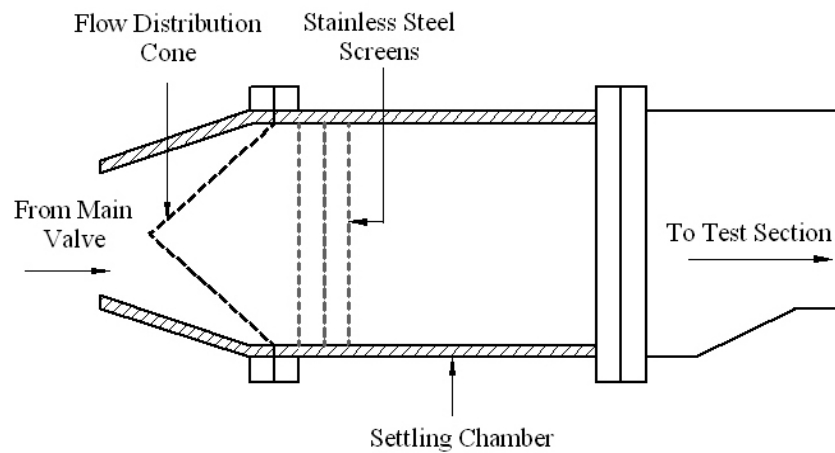
Figure 4.4: Sectional view of the settling chamber
