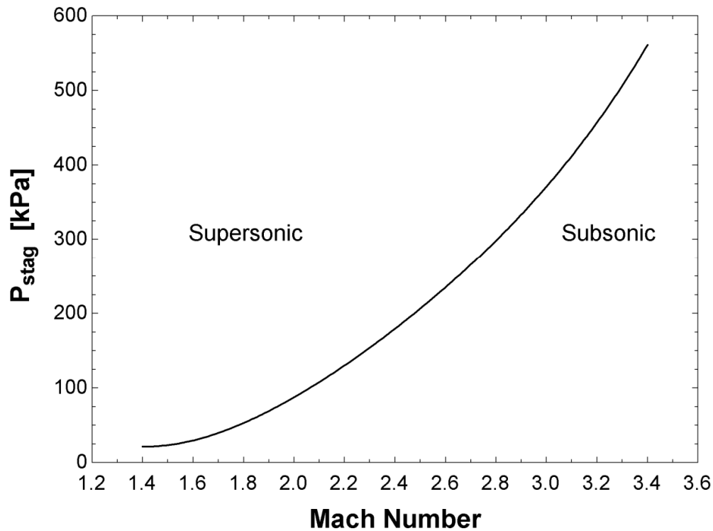
Figure 4.5: Minimum Stagnation Pressure Curve
