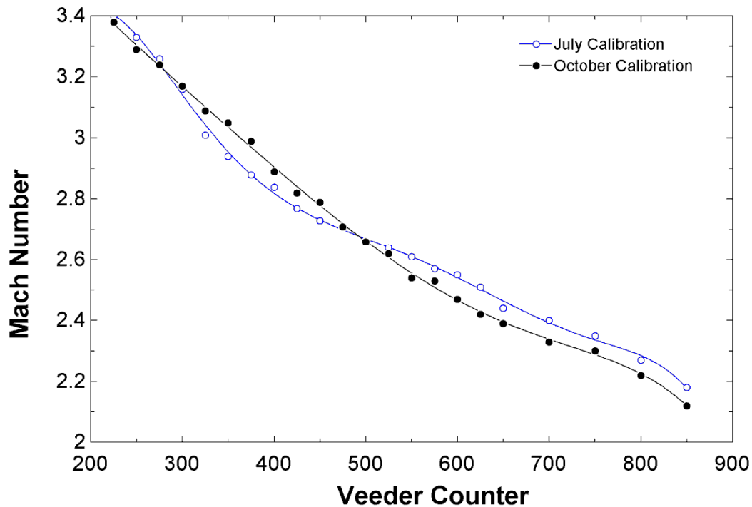
Figure A 4: Mach number – throat veeder counter calibration curves
