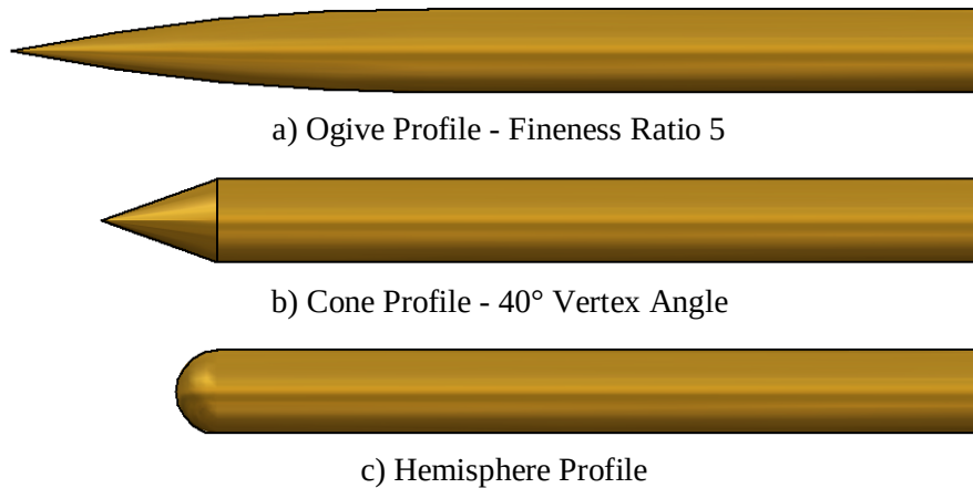
Figure 4.13: Shock wave generator profiles
