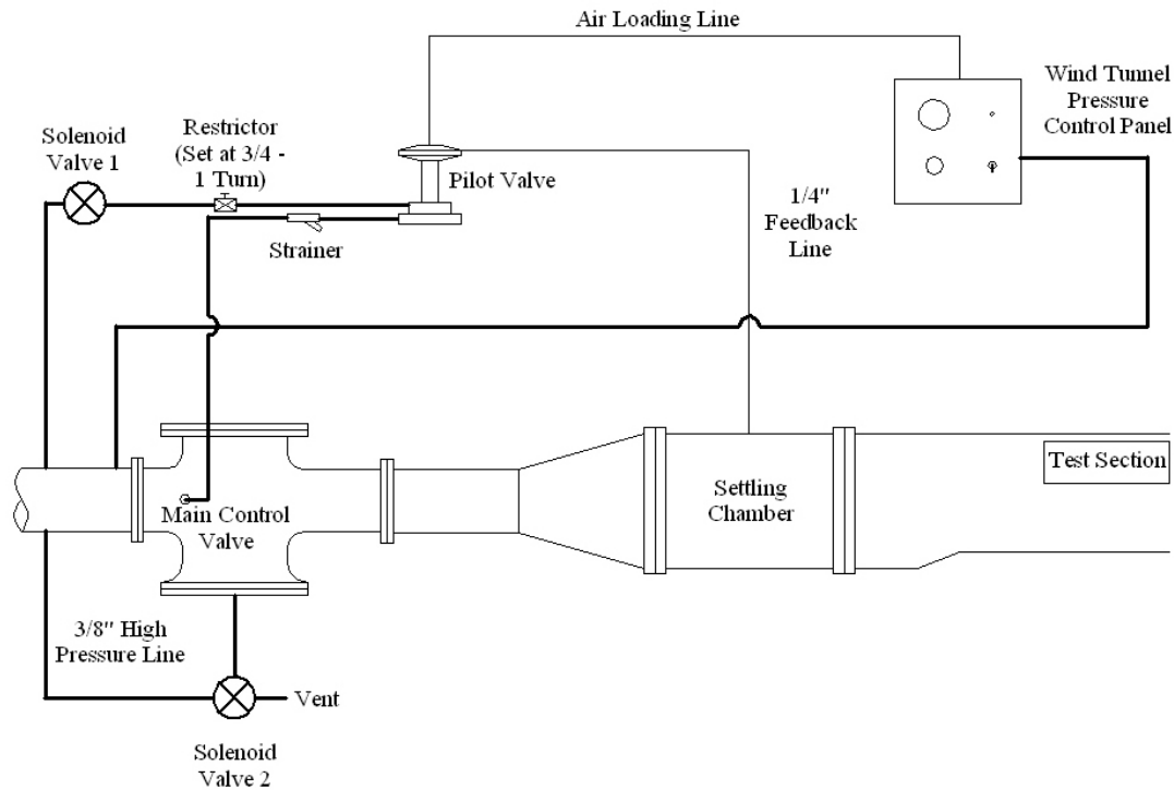
Figure 4.8: Pneumatic layout for the pressure control system
