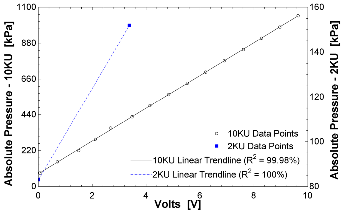
Figure 4.9: Pressure transducer calibration curve
