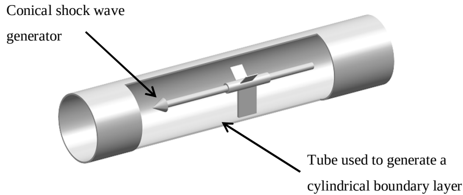
Figure 3.15: Experimental apparatus used by Kussoy et al (1980)
