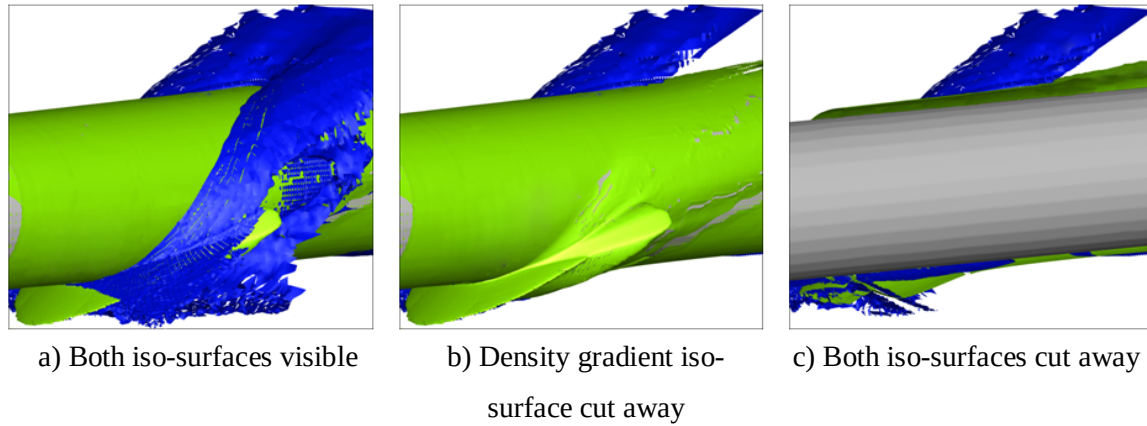
Figure 6.45: Sectioned iso-surfaces, Hemisphere
