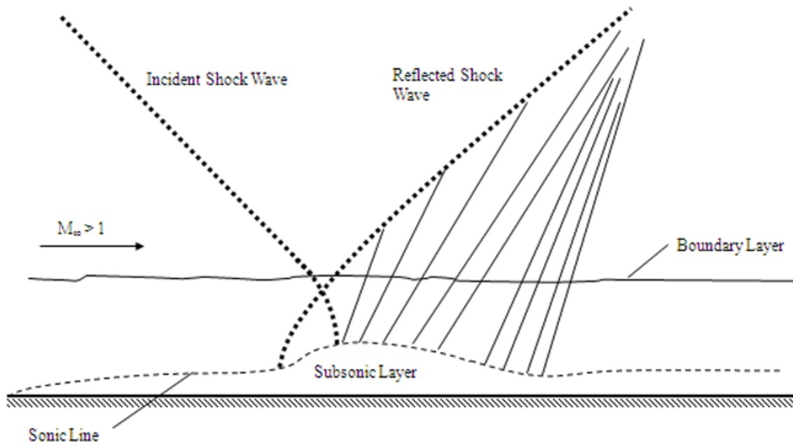
Figure 3.12: Anatomy of a SWBLI without separation
