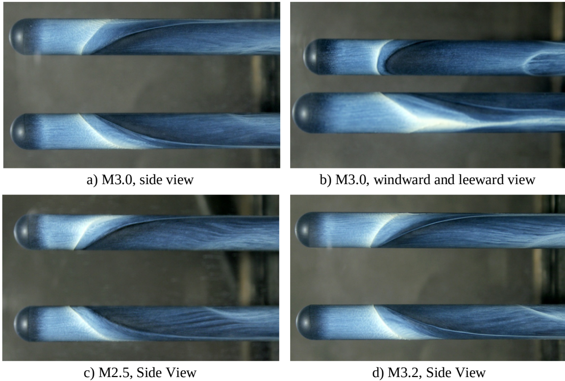
Figure 6.31: Oil surface flow visualisation during a blow down, Hemisphere
