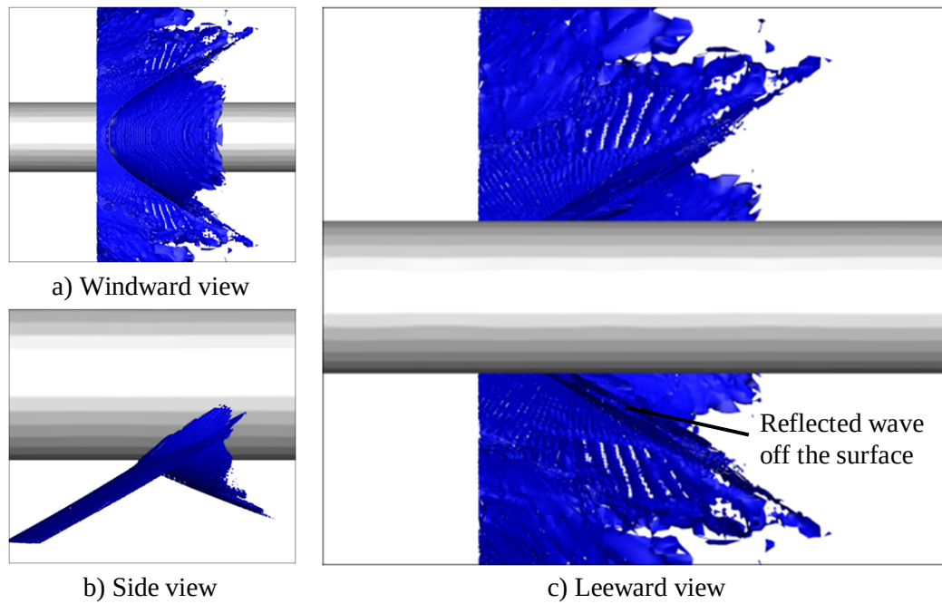
Figure 6.44: Viscous Simulation – Shock wave reflecting off surface of cylinder, Hemisphere
