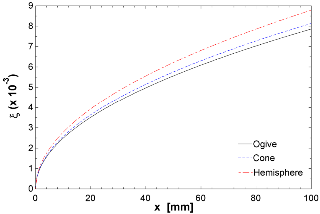
Figure 6.16: Variation of the nondimensional boundary layer parameter ( \xi ) along the length of the cylinder
