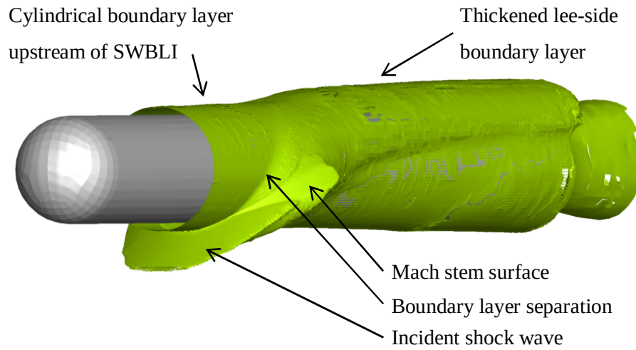
Figure 6.41: Annotated Mach Number ( M = 2.4 ) Iso-surface, Hemisphere
