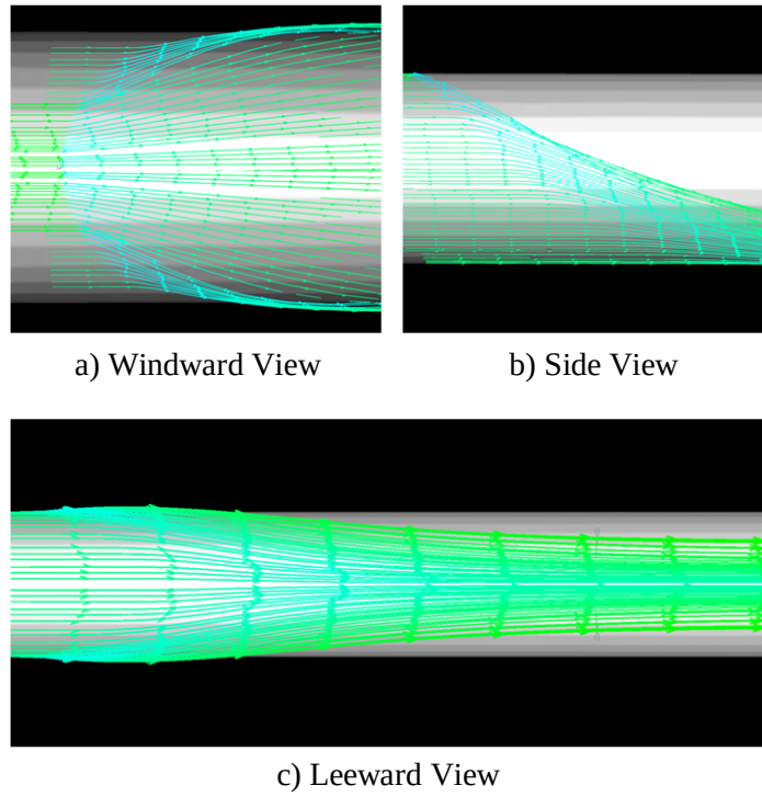
Figure 6.27: CFD Surface flow streamlines, Hemisphere
