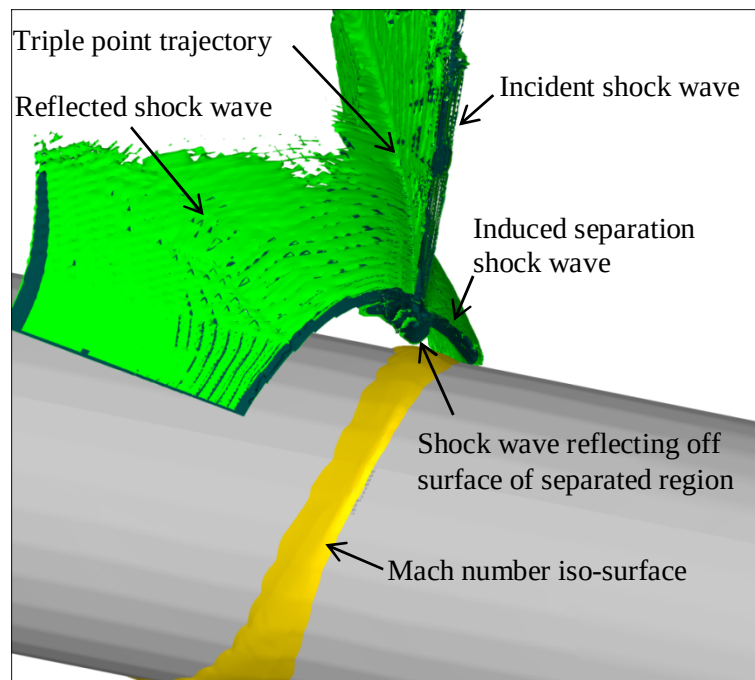
Figure 6.54: Viscous Simulation – annotated Mach number and density gradient iso-surfaces, Hemisphere, 30mm
