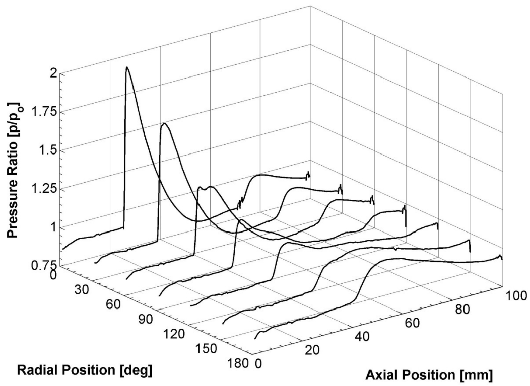
Figure 6.36: Surface pressure distribution, Hemisphere
