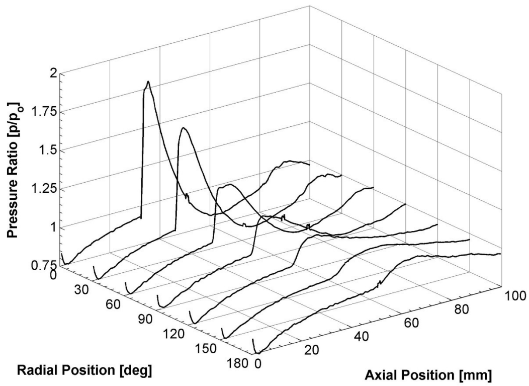
Figure 6.34: Surface pressure distribution, Cone
