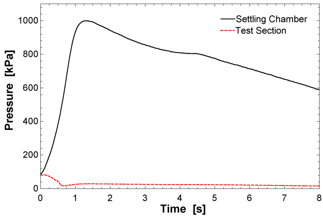
Figure 6.1: Settling chamber and test section pressure curves during a blow-down ( M = 3.0 )
