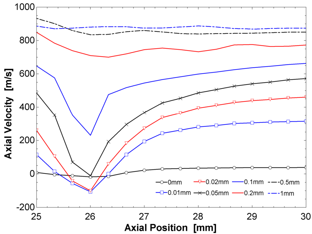
Figure 6.64: Axial velocity variation within the boundary layer in the immediate vicinity of the SWBLI, 0^\circ meridian, Hemisphere
