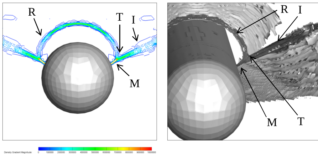
Figure 6.52: Inviscid Simulation – Annotated shock reflection structure, 32mm
