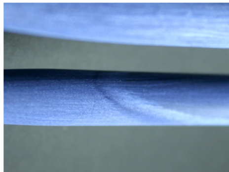
b) Windward view
