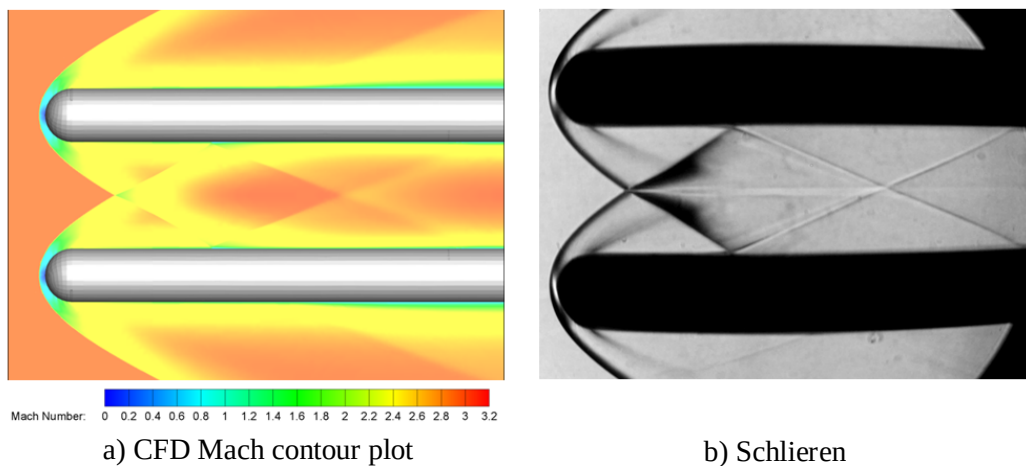
Figure 6.11: SWBLI on the 0^\circ meridian, Hemisphere
