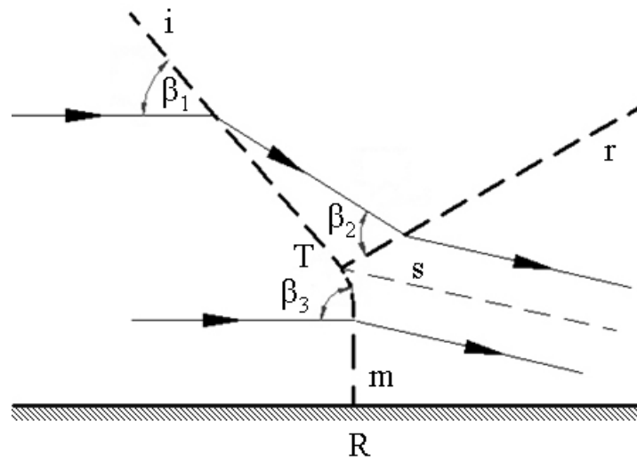
Figure 3.8: Mach reflection wave configuration
