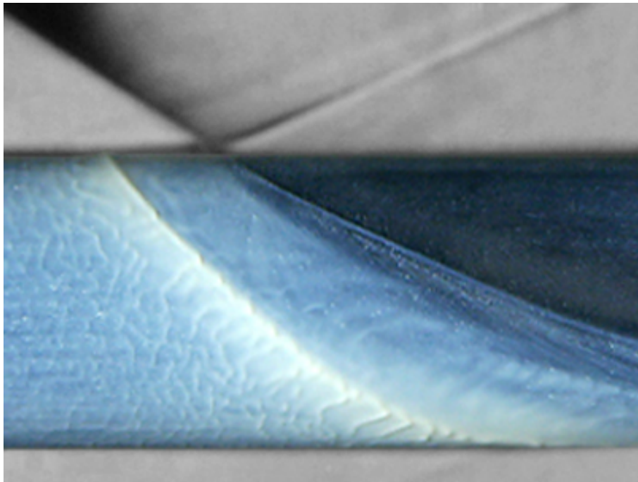
Figure 6.32: Superposition of schlieren and oil surface flow images, Hemisphere
