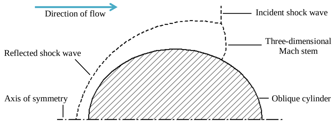
Figure 3.10: Three-dimensional shock wave reflection and diffraction around an oblique cylinder
