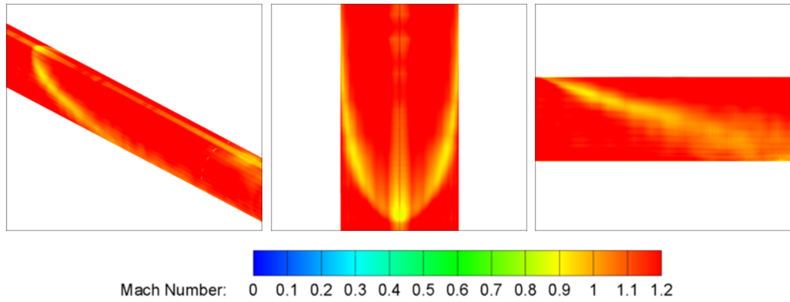
Figure 6.18: CFD Surface flow visualisation, Ogive
