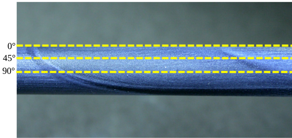
Figure 6.40: Separated region with meridian angles superimposed, Cone
