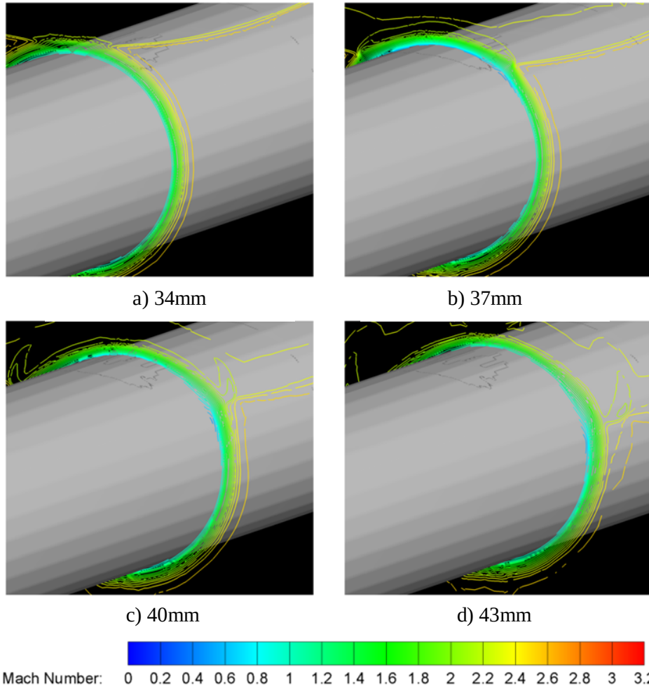
Figure 6.10: Mach number contour line plots transverse to the axis of the cylinder, Cone
