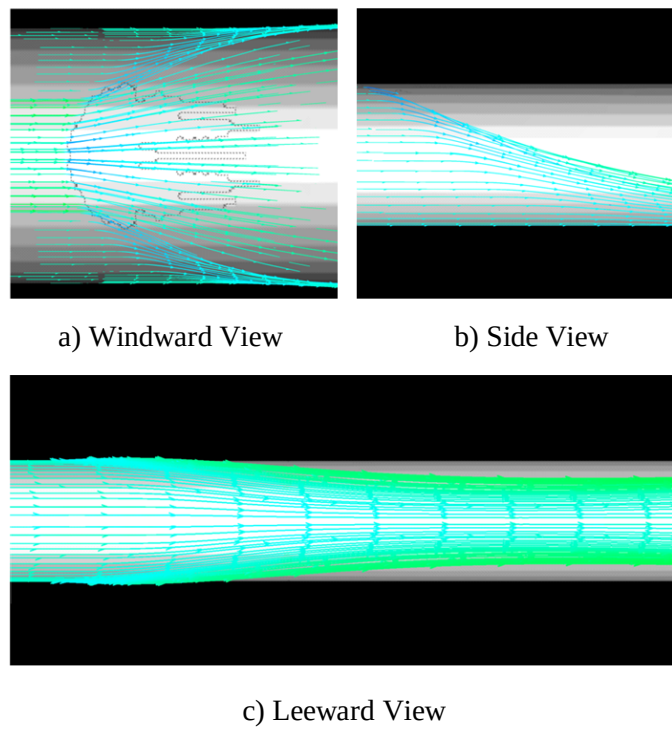
Figure 6.22: CFD Surface flow streamlines, Cone
