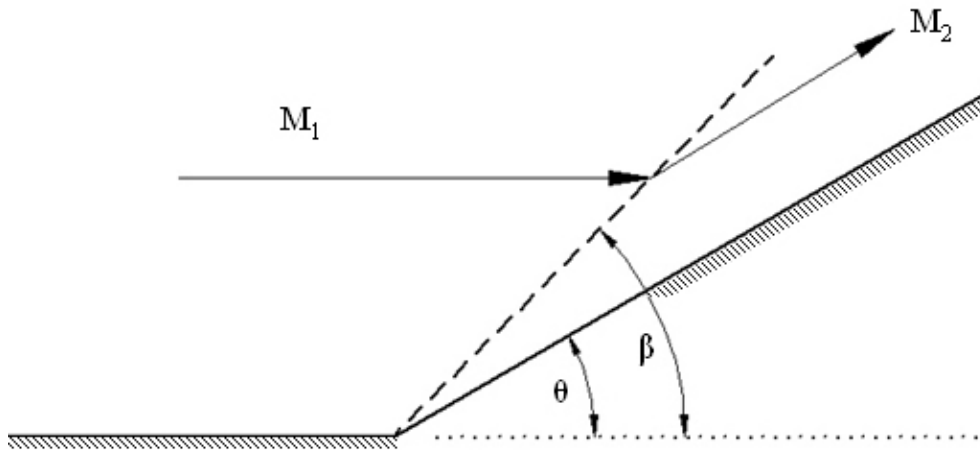
Figure 3.1: Supersonic compressible flow over a concave corner
