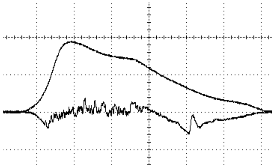
Figure A 5: Pressure trace from an unsuccessful test
