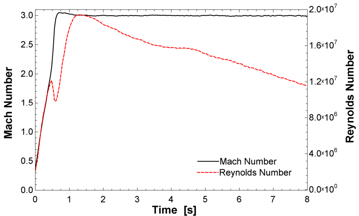
Figure 6.2: Mach and Reynolds number curves during a blow down ( M = 3.0 )
