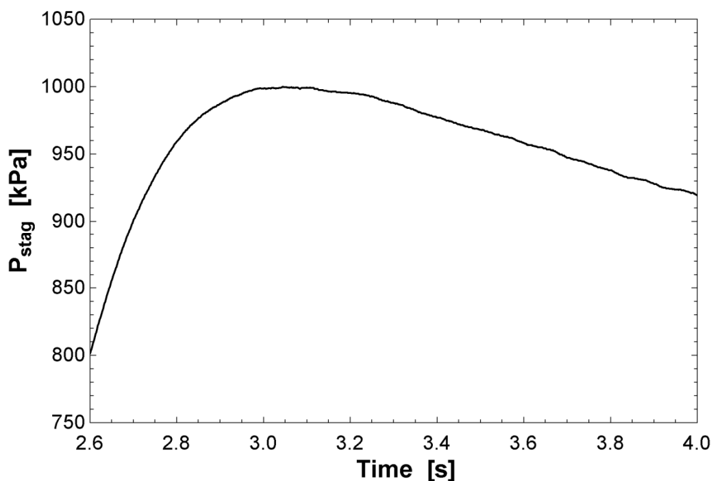
Figure A 7: Pressure trace showing vibration (December 2009)
