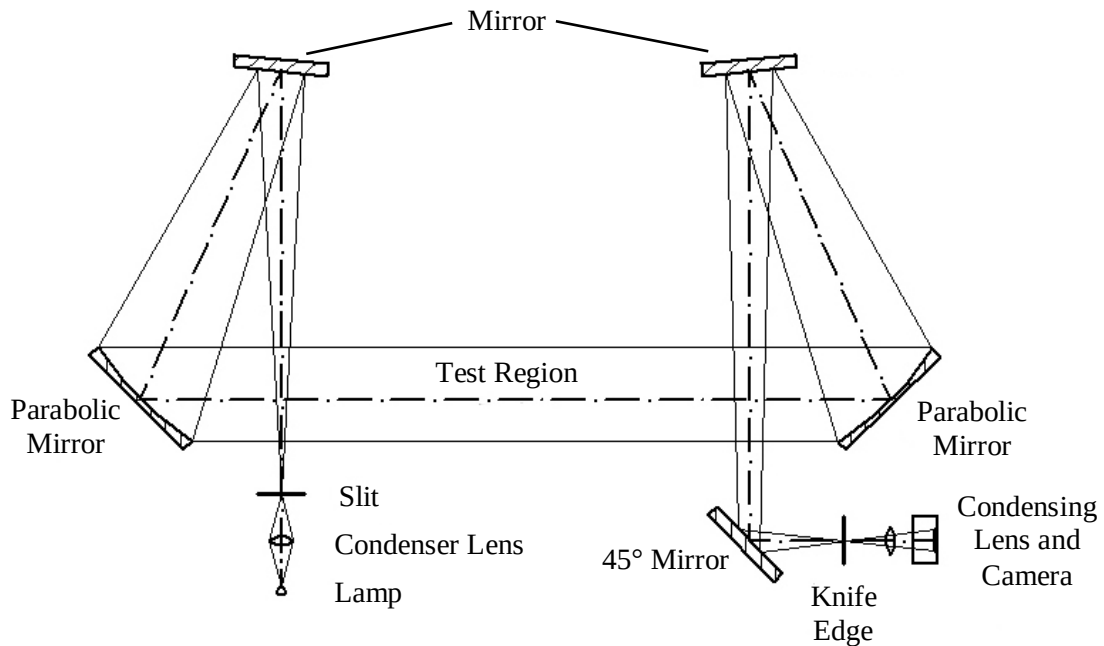
Figure 4.10: Schlieren photography layout
