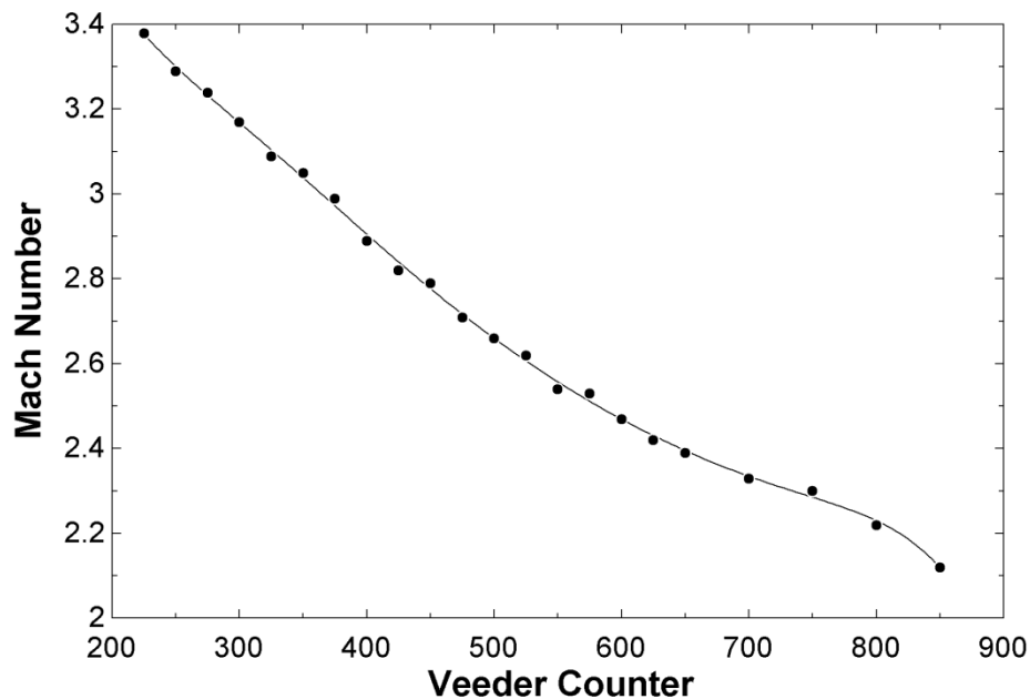
Figure 4.7: Mach number calibration curve
