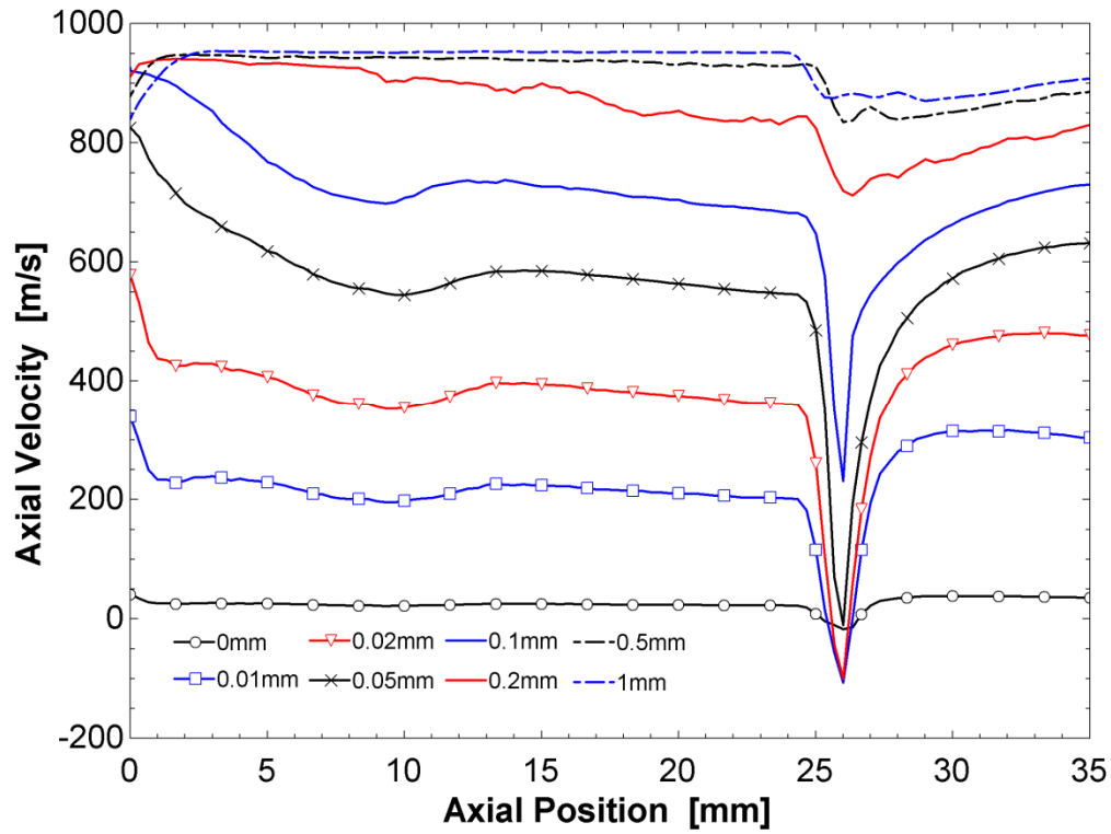
Figure 6.63: Axial velocity variation within the boundary layer, 0^\circ meridian, Hemisphere
