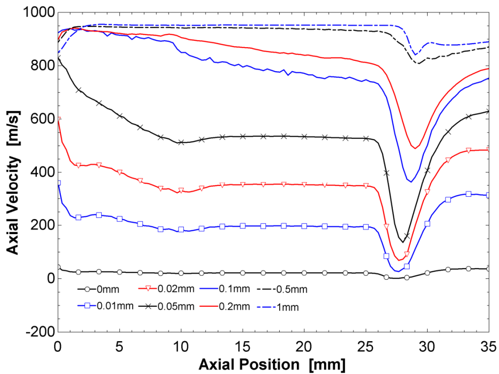
Figure 6.65: Axial velocity variation within the boundary layer, 45° meridian, Hemisphere
