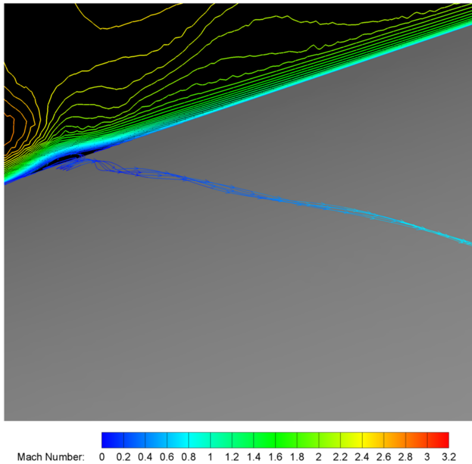
Figure 6.23: Streamlines within the separated region, Cone
