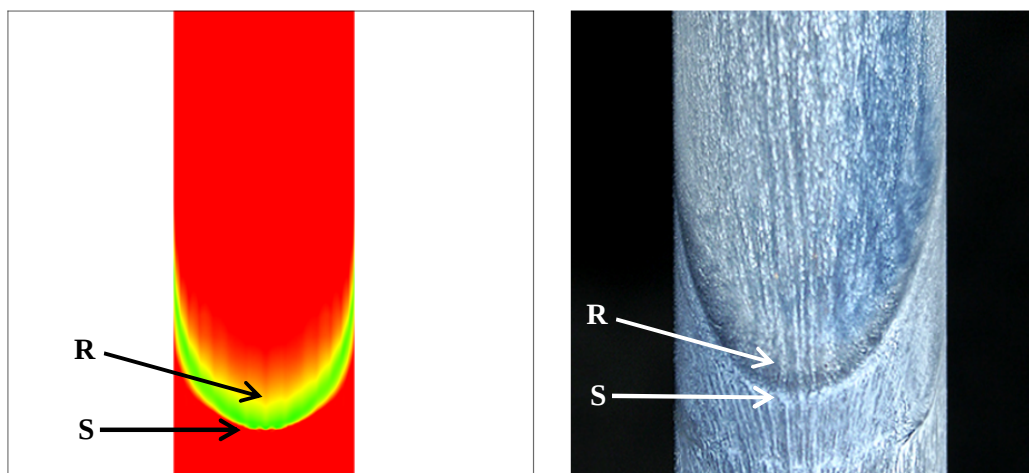
Figure 6.29: Separated region on the windward surface of the hemispherical SWBLI generator
