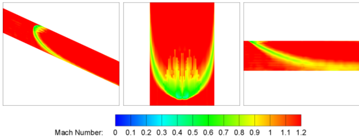
Figure 6.21: CFD surface flow visualisation, Cone
