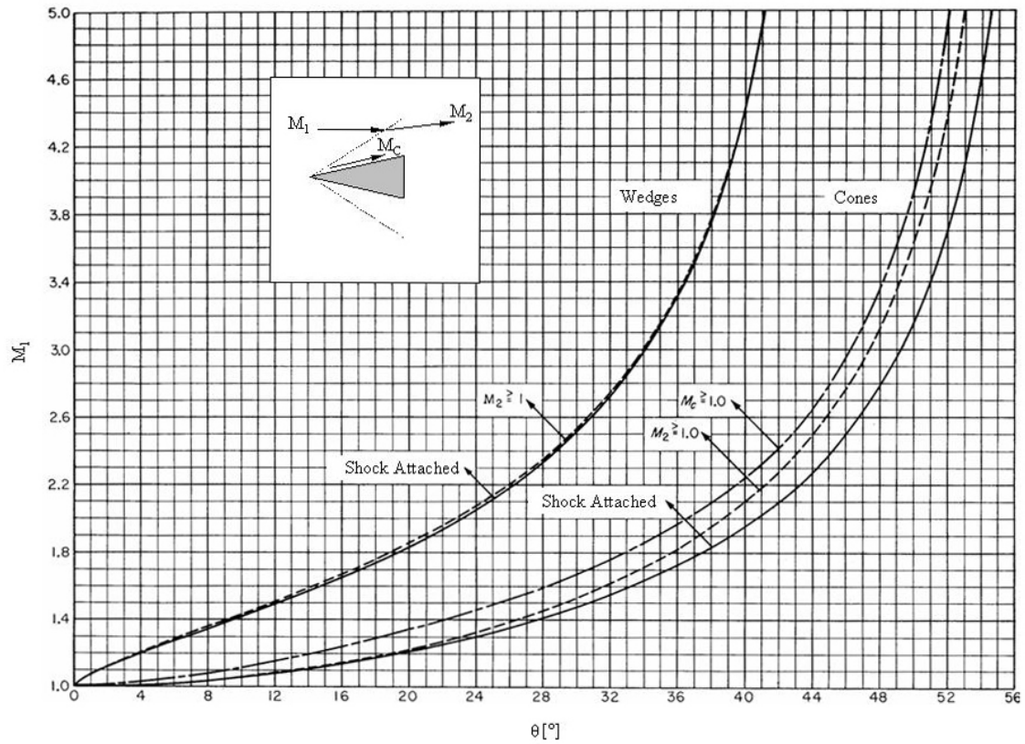
Figure 3.4: Shock attachment criteria, (NACA, 1953)
