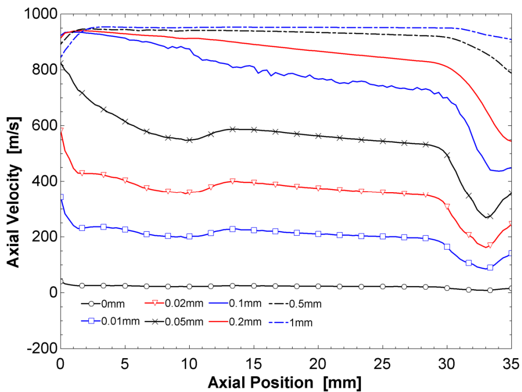
Figure 6.66: Axial velocity variation within the boundary layer, 90° meridian, Hemisphere
