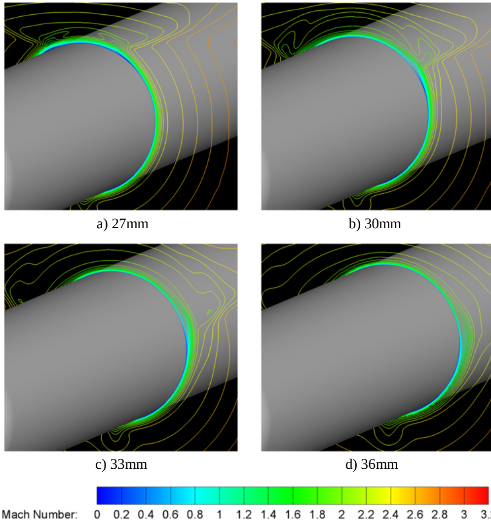
Figure 6.58: High resolution CFD Mach number contour line plots transverse to the axis of the cylinder, Hemisphere
