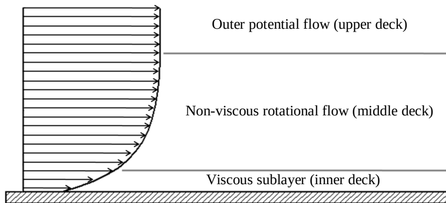
Figure 3.9: The multi-layer structure within a boundary layer (Delery and Dussauge, 2009)
