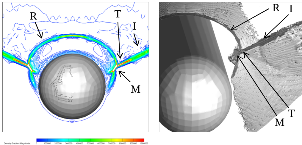
Figure 6.51: Viscous Simulation - Annotated shock reflection structure, 32mm
