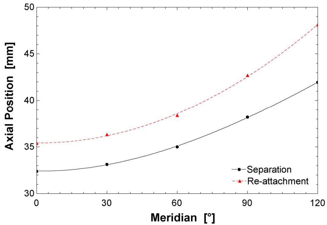
Figure 6.35: Separation and attachment co-ordinates for SWBLI, Cone
