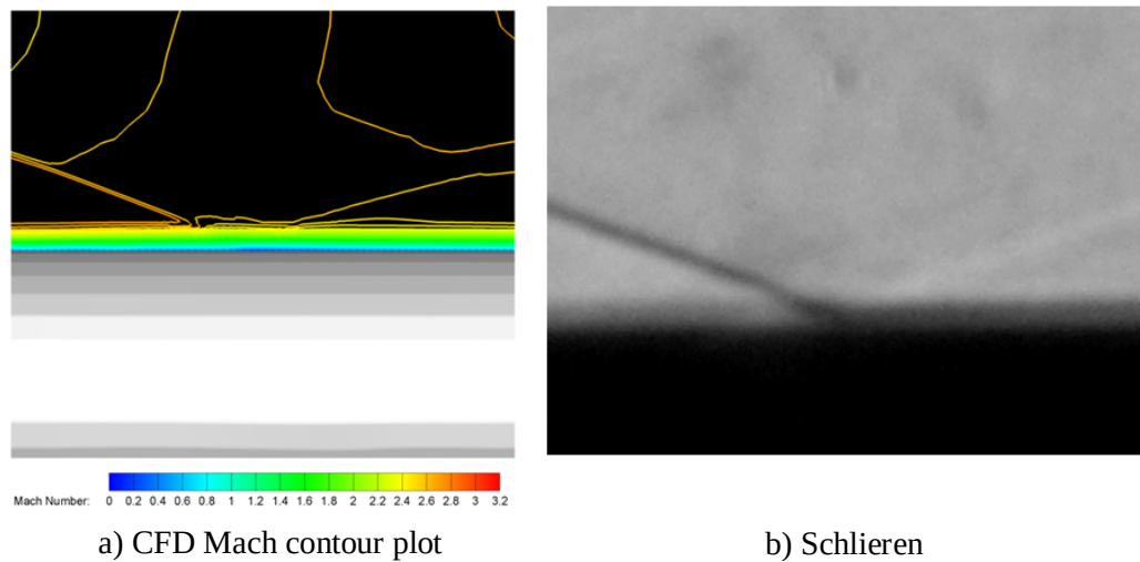
Figure 6.5: Magnified SWBLI on the 0° meridian, Ogive
