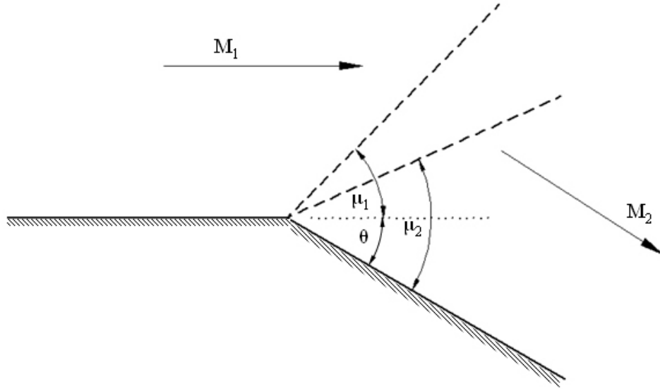
Figure 3.2: Supersonic compressible flow over a convex corner
