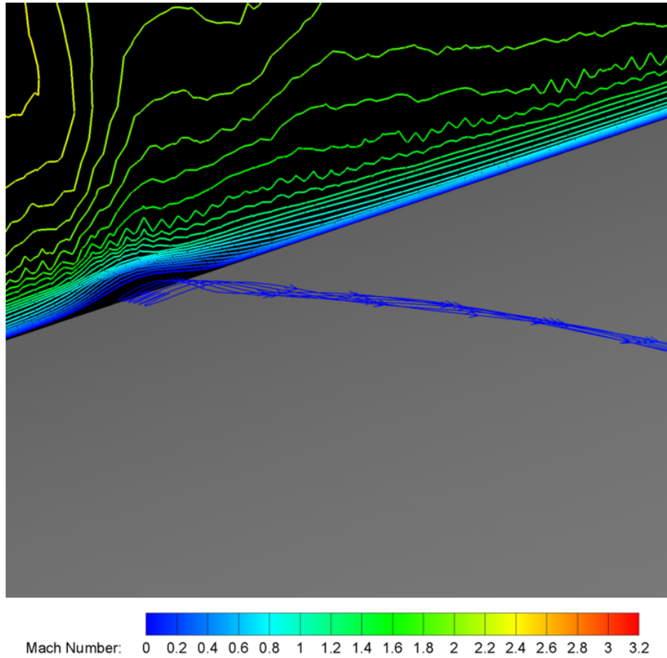
Figure 6.28: Streamlines within the separated region, Hemisphere
