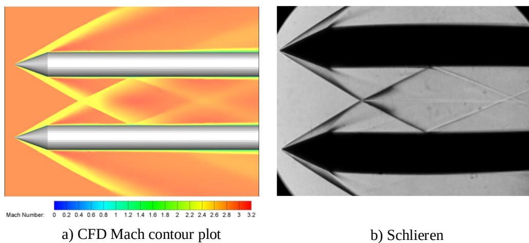
Figure 6.7: SWBLI on the 0° meridian, Cone
