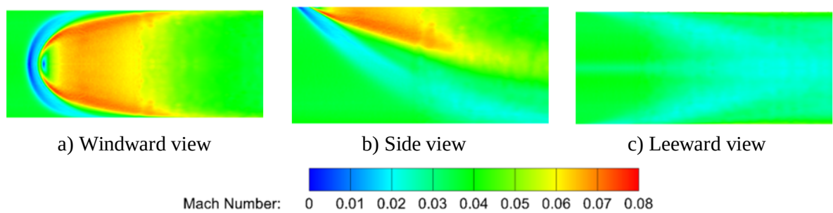
Figure 6.59: High resolution CFD surface flow patterns, Mach number contours, Hemisphere
