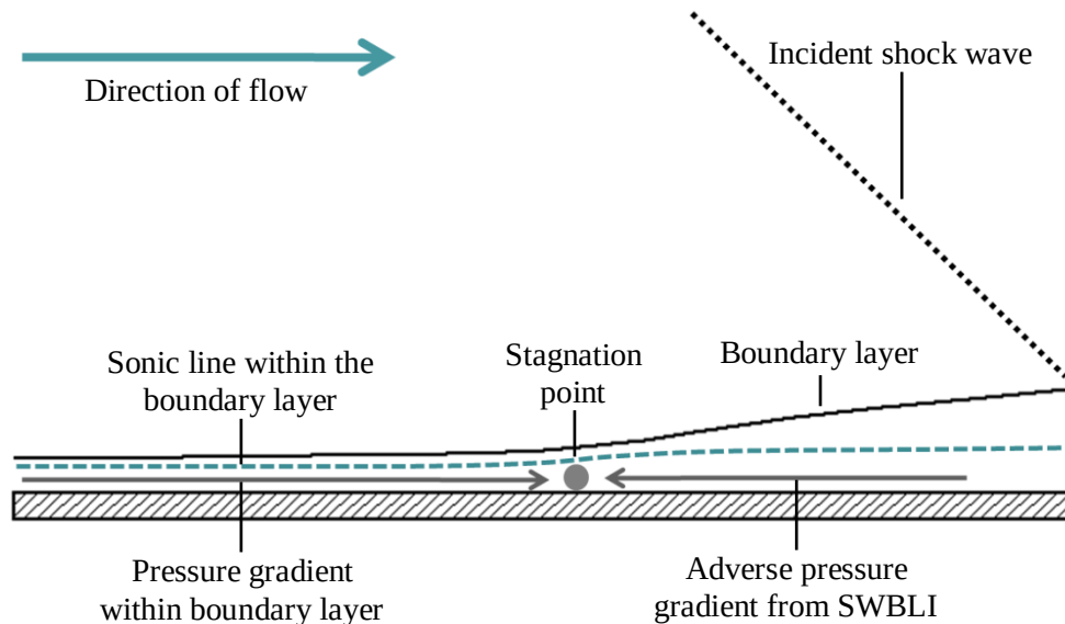
Figure 6.67: Stagnation point caused by upstream influence
