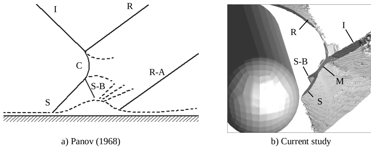
Figure 6.53: Comparison of SWBLI shock structure
