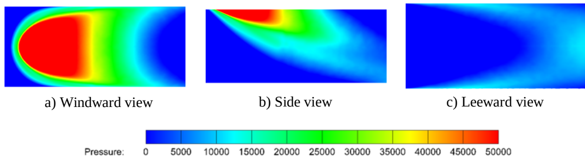
Figure 6.61: High resolution CFD surface flow patterns, Pressure (Pa) contours, Hemisphere
