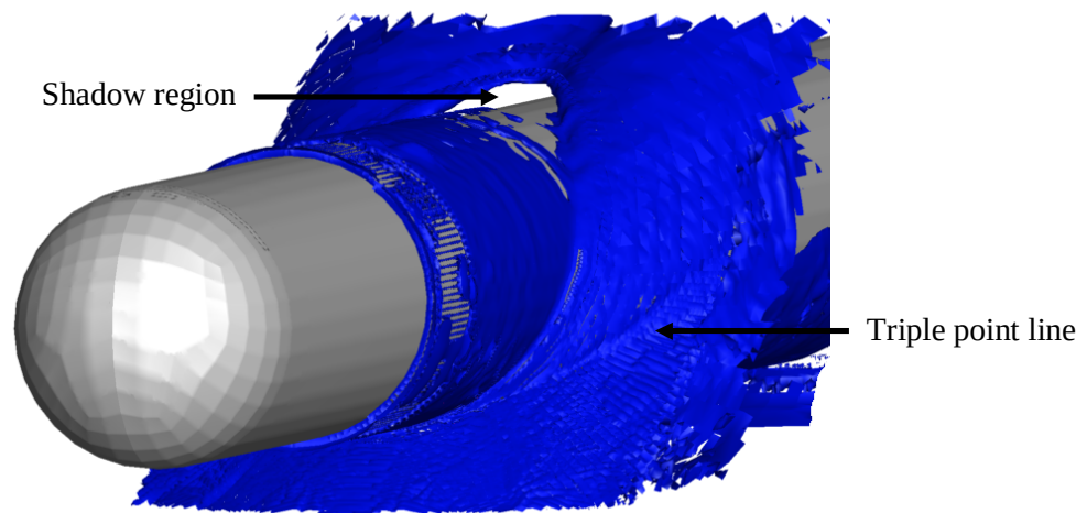
Figure 6.43: Viscous Simulation - Lee-side shock wave, Density gradient iso-surface, DG = 15000
