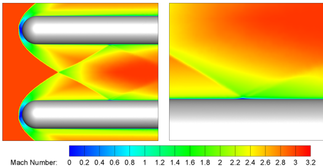
Figure 6.57: High resolution CFD SWBLI overview, Hemisphere
