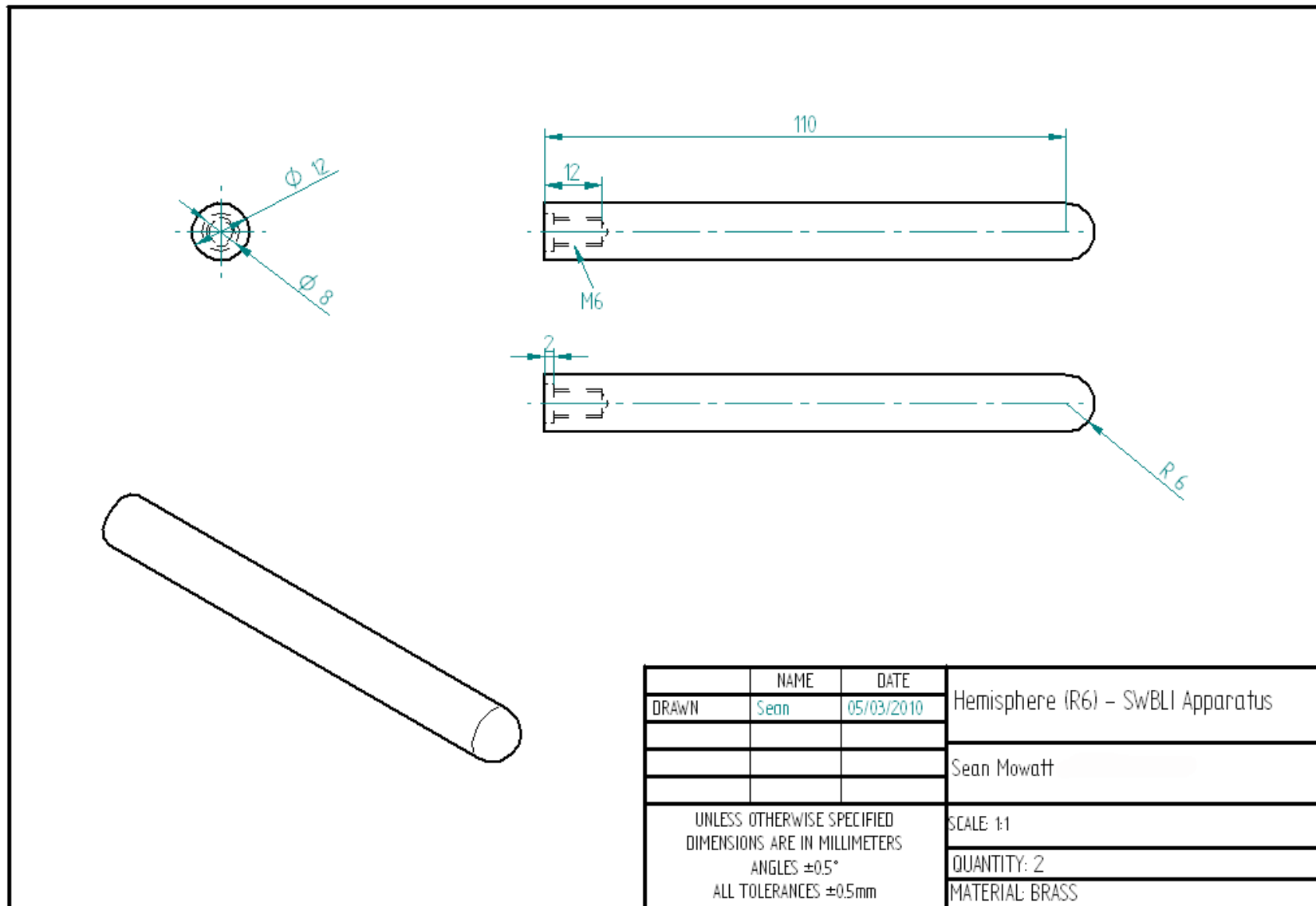
Figure C 3: Manufacturing drawings for the hemispherical SWBLI generator
