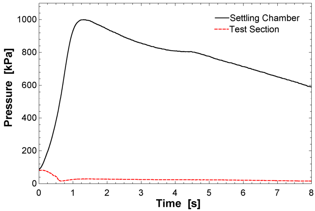
Figure A 8: Processed pressure trace from successful wind tunnel test, Mach 3.0
