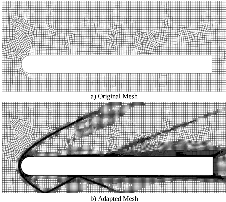
Figure 4.14: Mesh adaption scheme illustration
