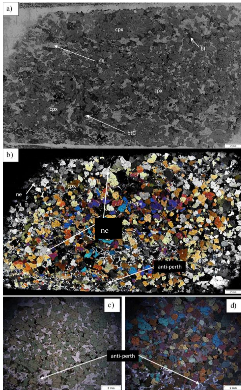
Figure 6.5: Photomicrographs of Melteigite sample 542215 a) full thin section scan in ppl, b) thin sections scan in xpl, c) anti-perthite present in the ijolite samples in ppl, d) anti-perthite present in the ijolite samples in xpl
