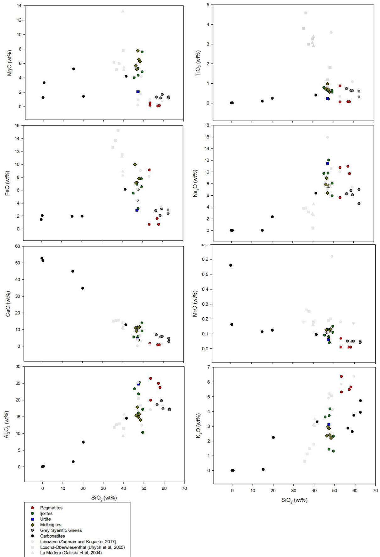
Figure 6.26 : Major element concentrations in wt% of the nepheline-bearing rocks, pegmatites, carbonatites and syenitic gneisses from the Singertât Complex.
