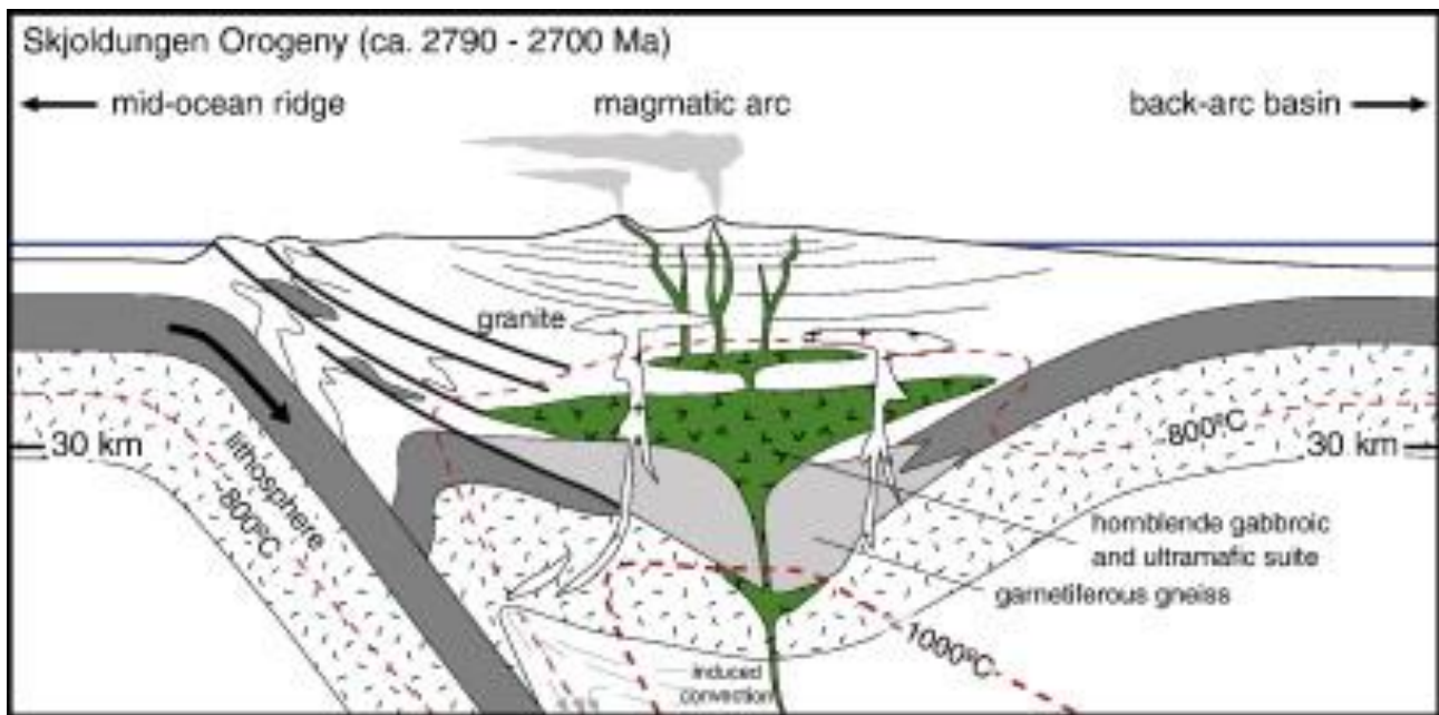
Figure 1.4: Schematic of the Skjoldungen Arc during the Skjoldungen Orogen taken from Bagas et al. (2013).
