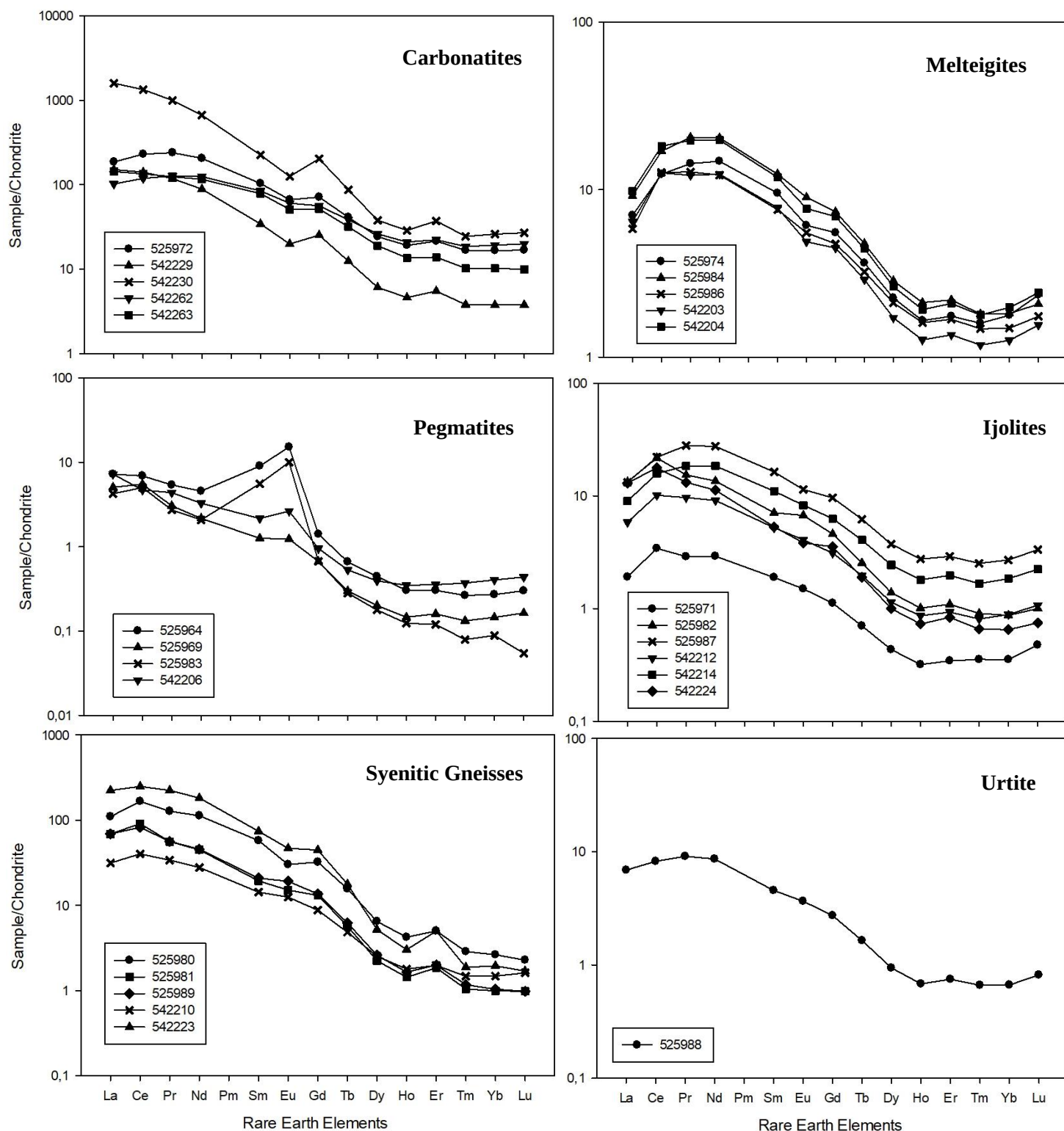
Figure 6.28: REE plots for different rock types that make up the Singertât Complex. The samples were normalized to chondrite (Anderson and Grevasse, 1988)
