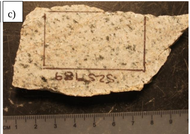
Figure 6.14: Hand samples of a) 542217, b) 525981 and c) 525989 which depicts syenitic gneisses showing the typical gneissic texture (alignment of aegirine-augite and biotite grains).
