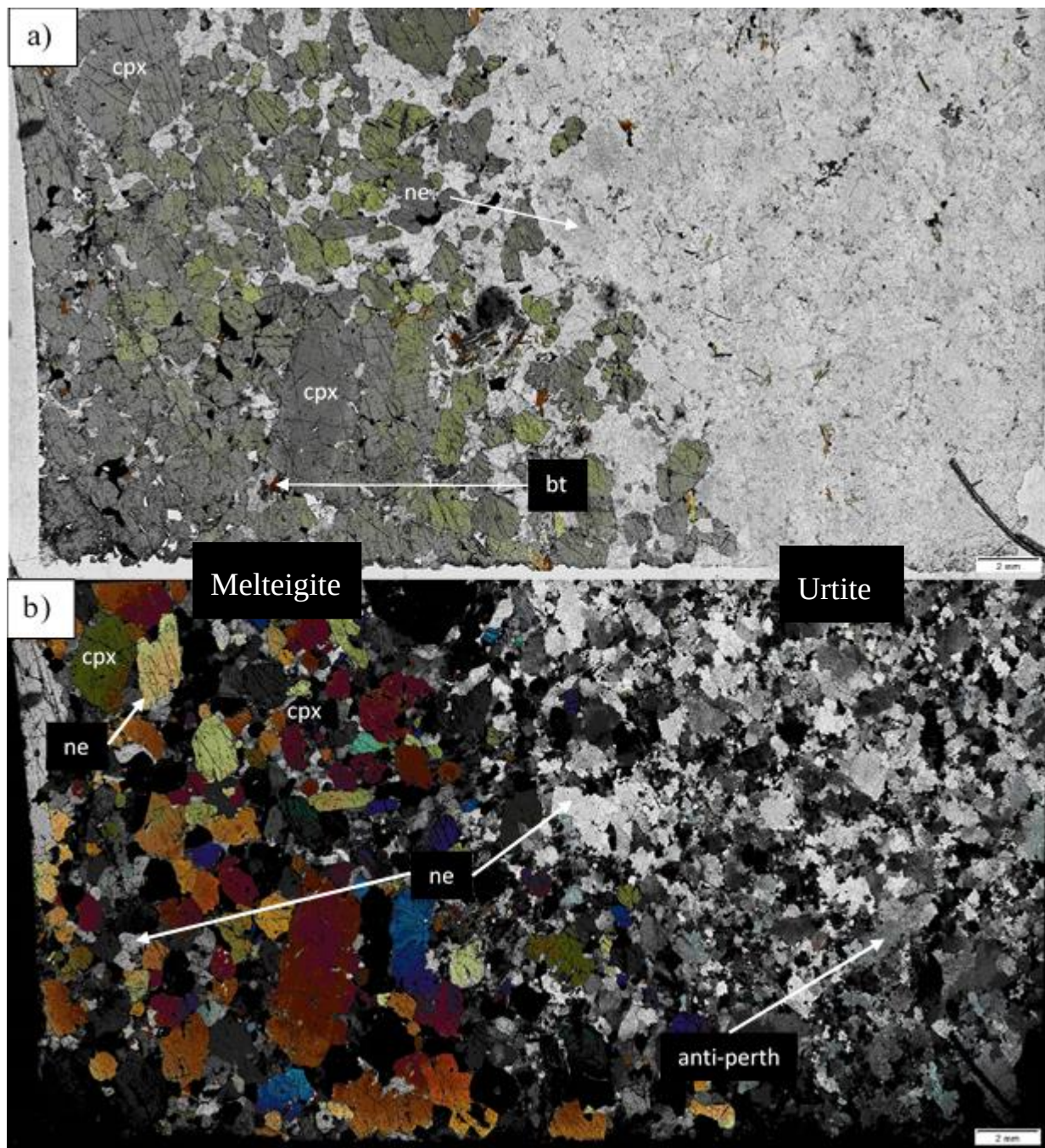
Figure 6.7: Photomicrographs of a layered nepheline-bearing rock sample 542216BII, which shows a gradational contact (indicated by the dashed white line) between an urtite and a melteigite layer. a) full thin section scans in ppl, b) thin sections scan in xpl.
