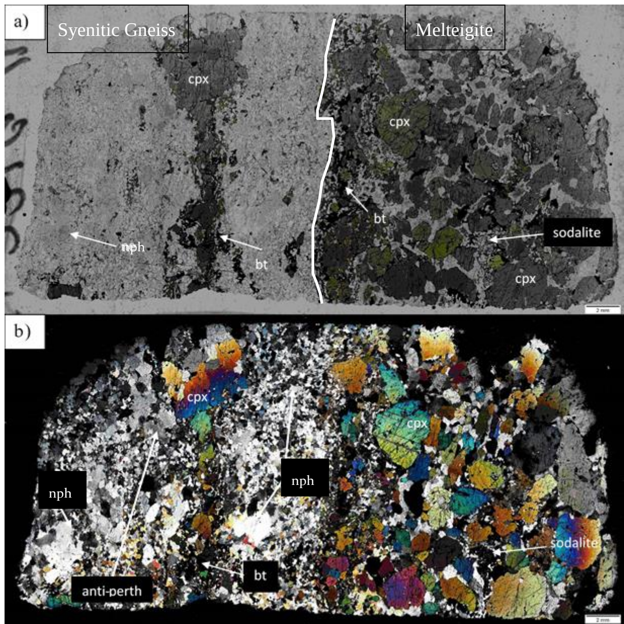
Figure 6.8: Photomicrographs of a layered nepheline-bearing rock sample 542219AII, which shows a sharp contact between a syenitic gneiss and a melteigite layer (indicated by the white line), with a melteigite vein cross cutting the syenitic gneiss. a) full thin section scans in ppl, b) thin sections scan in xpl.
