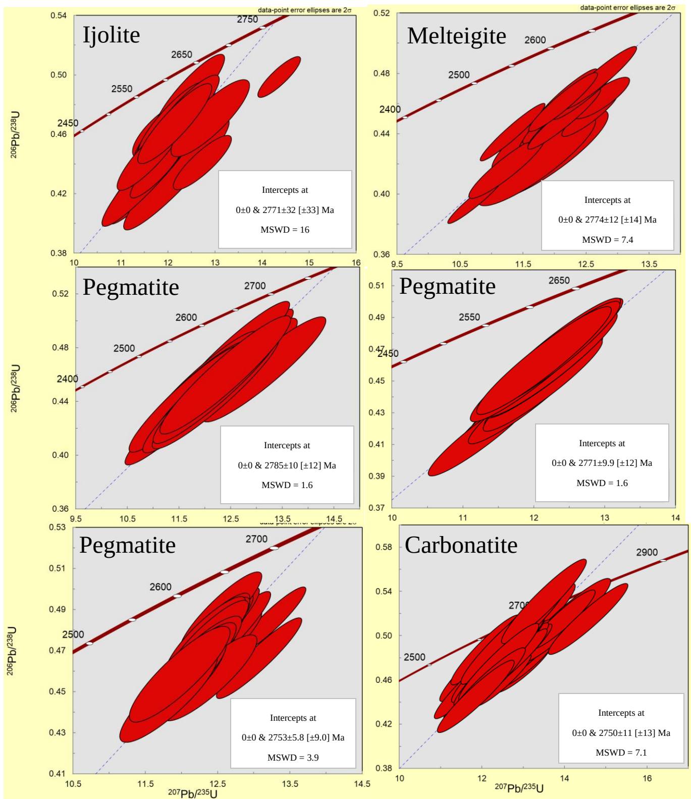
Figure 6.35: Concordia plots for the nepheline-bearing rocks, pegmatites and a carbonatite used to determine ^{207}\text{Pb}/^{206}\text{Pb} ages.
