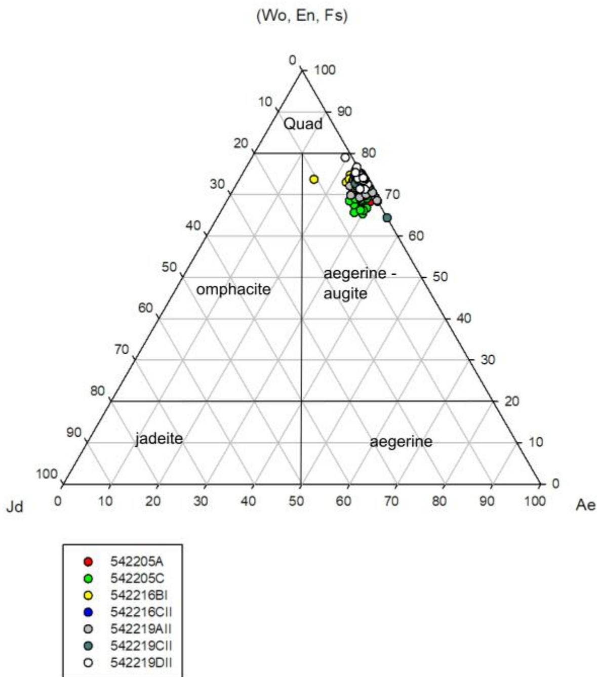
Figure 6.22: A ternary diagram representing the EPMA results for the clinopyroxene crystals found in the nepheline-bearing alkaline rocks of the Singertât Complex.
