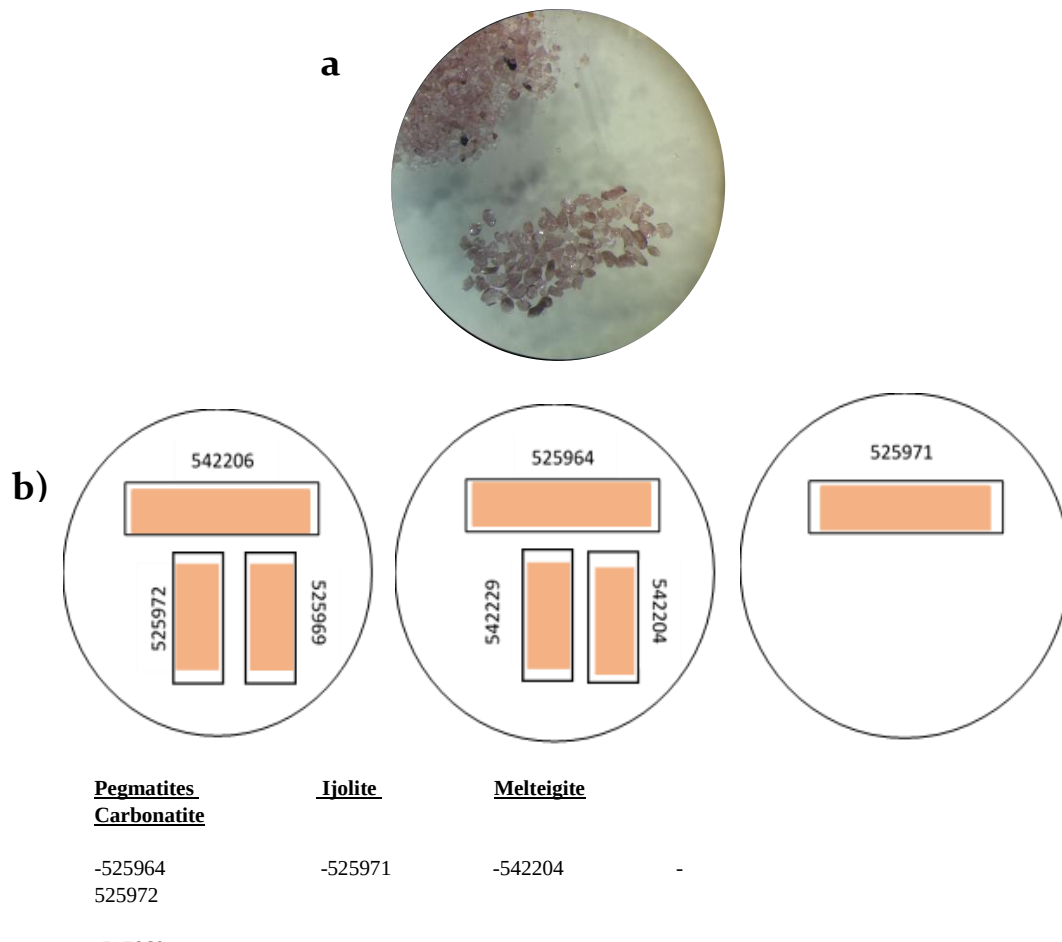
Figure 5.2: a) Photomicrograph of the zircon grains in sample 542206 as they were being picked, grains are 0.5 mm or less. Schematic maps showing the position of each sample on its respective grain mount, as well as the rock type of each sample.
