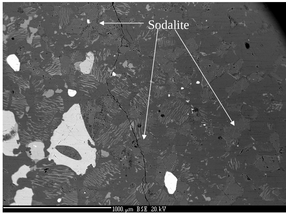
Figure 6.23: BSE taken of the EPMA image, which shows the sodalite that was analyzed in sample 542217B.
