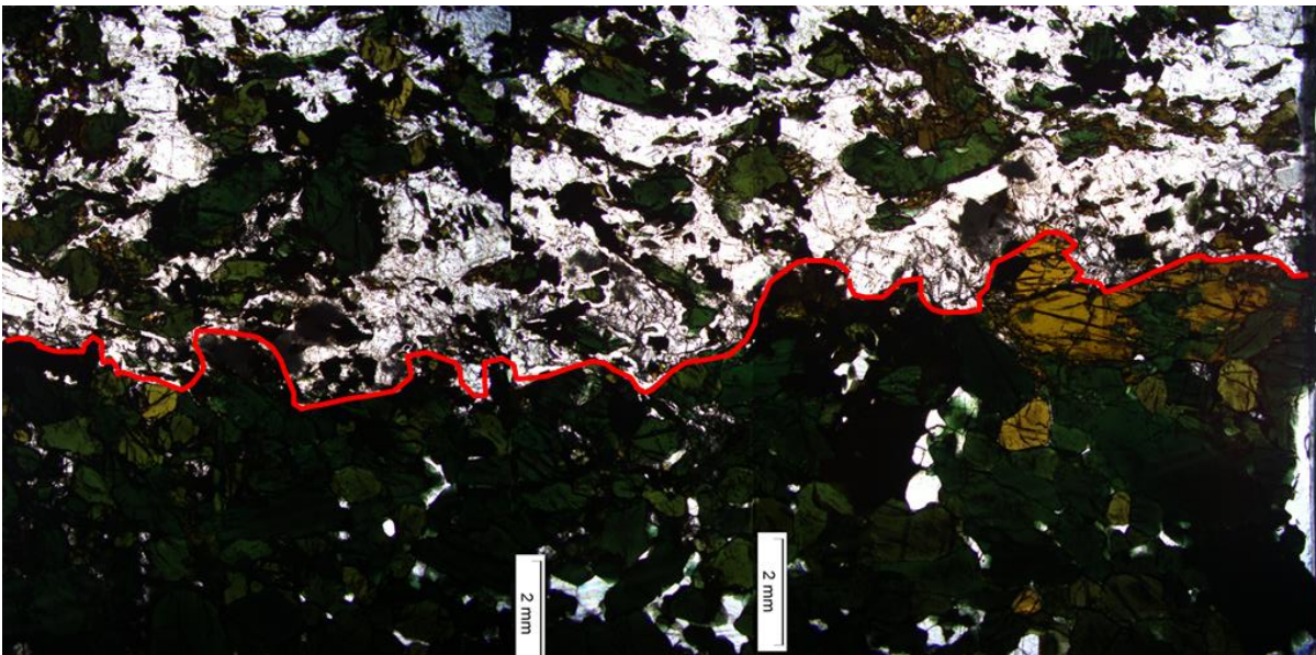
Figure 7.4: Photomicrograph showing a truncated boundary as a result of thermal erosion with in-situ crystallization of nepheline and anti-perthite along the boundary
