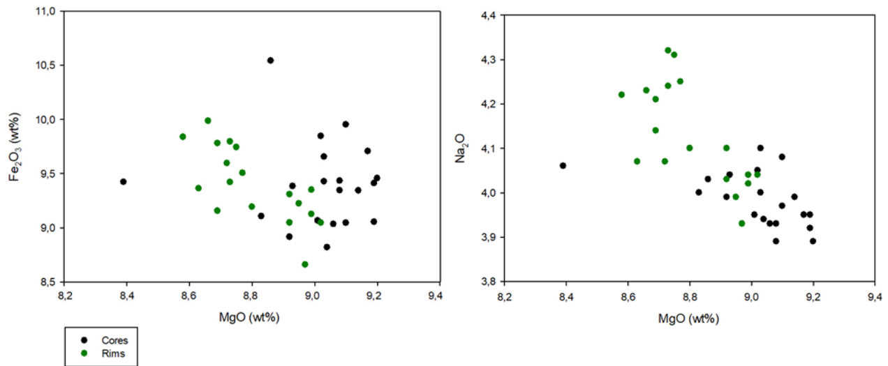
Figure 7.7: Variation diagrams for the layered sample 542205 which depicts variation from the core- rim data for aegerine-augite
