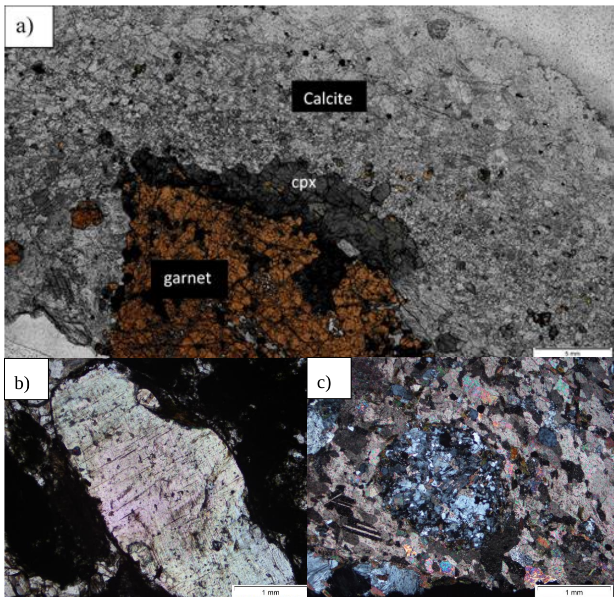
Figure 6.13: Photomicrographs of carbonatite sample 542249, which shows a garnet and clinopyroxene surrounded by a large amount of calcite. a) full thin section scans in ppl, b) nepheline xenocryst in carbonatite breccia in ppl and c) rounded fragments of ijolite in a carbonatite breccia in xpl.
