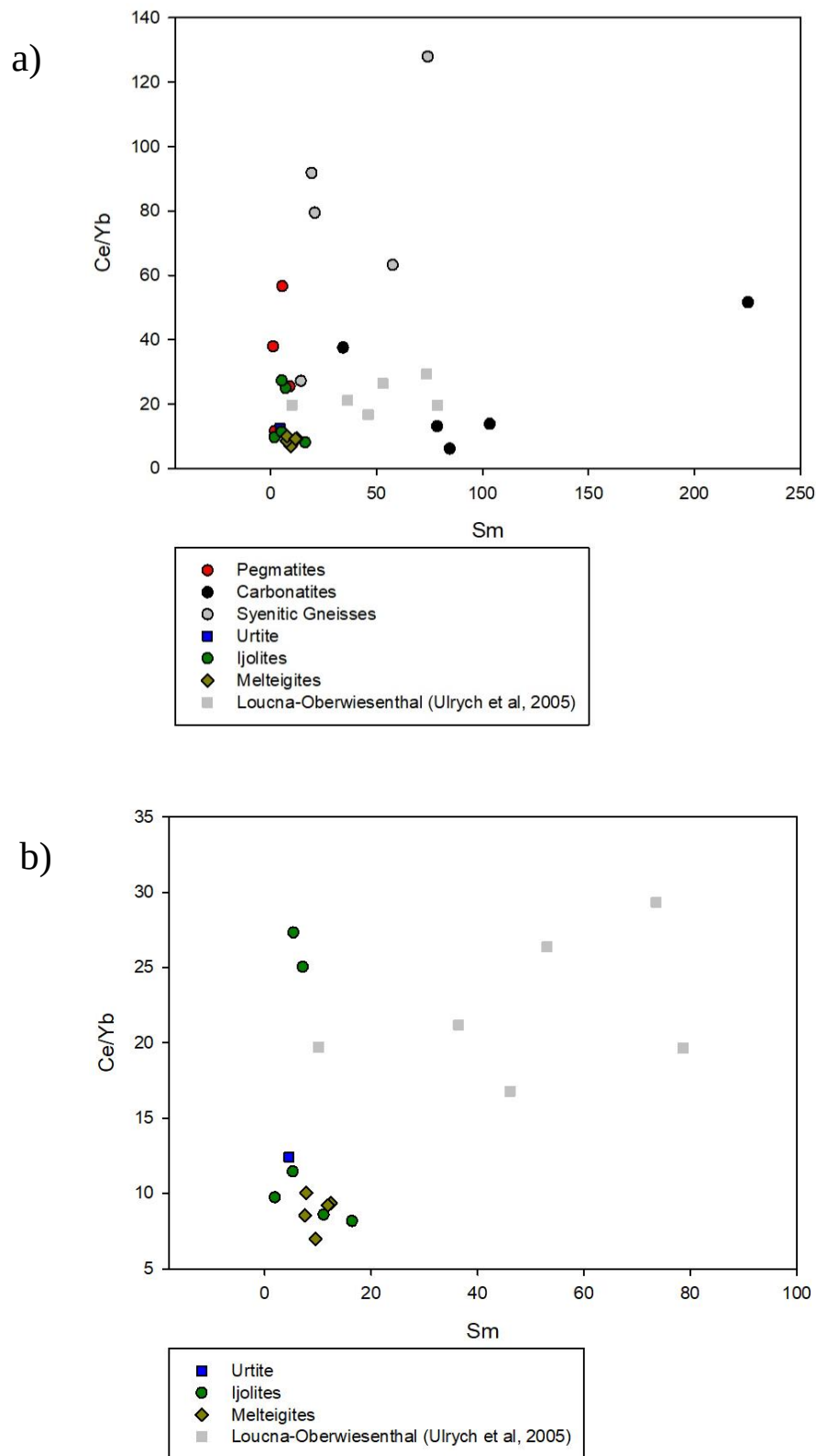
Figure 6.29: Trace element bivariate plot of Ce/Yb vs Sm which have been normalized to chondritic reference value using Anderson and Grevasse (1989), comparing the Singertât rocks as well as the alkaline rocks of Loucna-Oberwiesenthal. a) All Singertât rock types, b) Singertât nepheline-bearing alkaline rocks.
