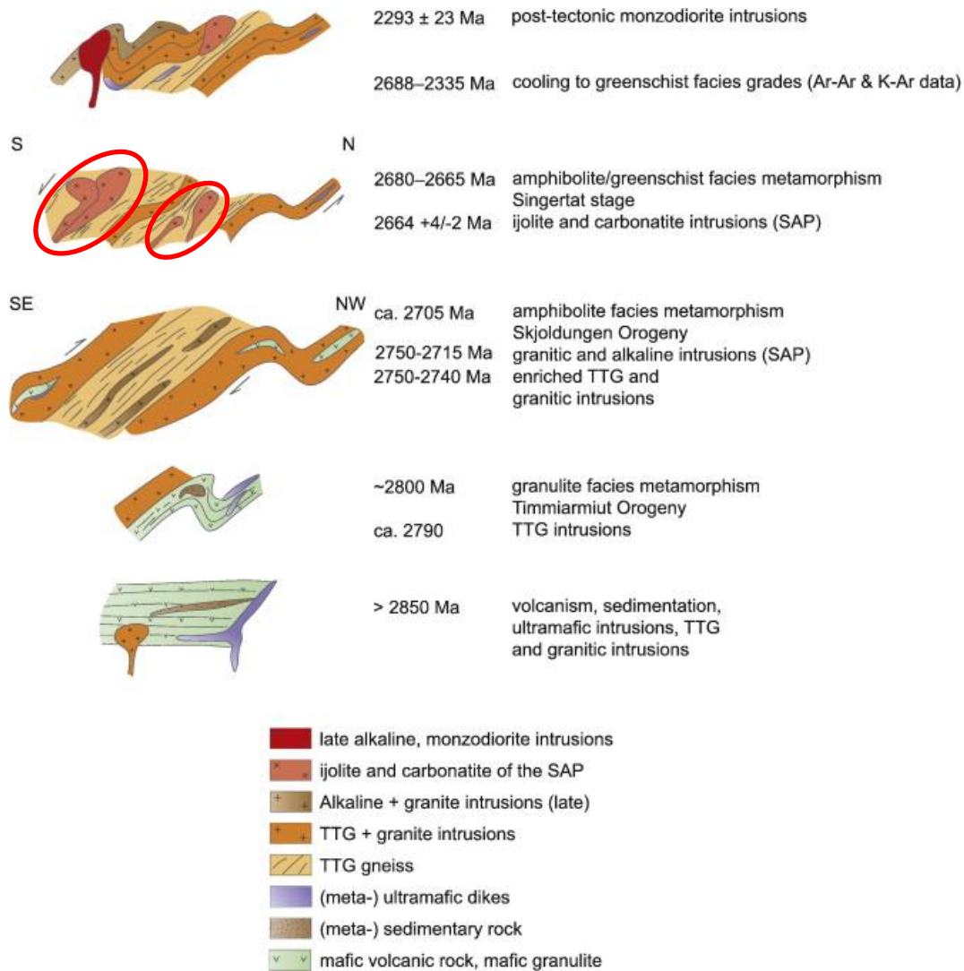
Figure 1.5: Synoptic sketch by Bagas et al. (2013), which depicts a proposed Late Archean to Early Proterozoic evolution of the NAC in southeast Greenland. The Singertât Complex intruded at approximately 2664 +4/-2 Ma (Nielson and Rosing, 1990 and Kolb et al., 2012a) and is indicated by the red circles.
