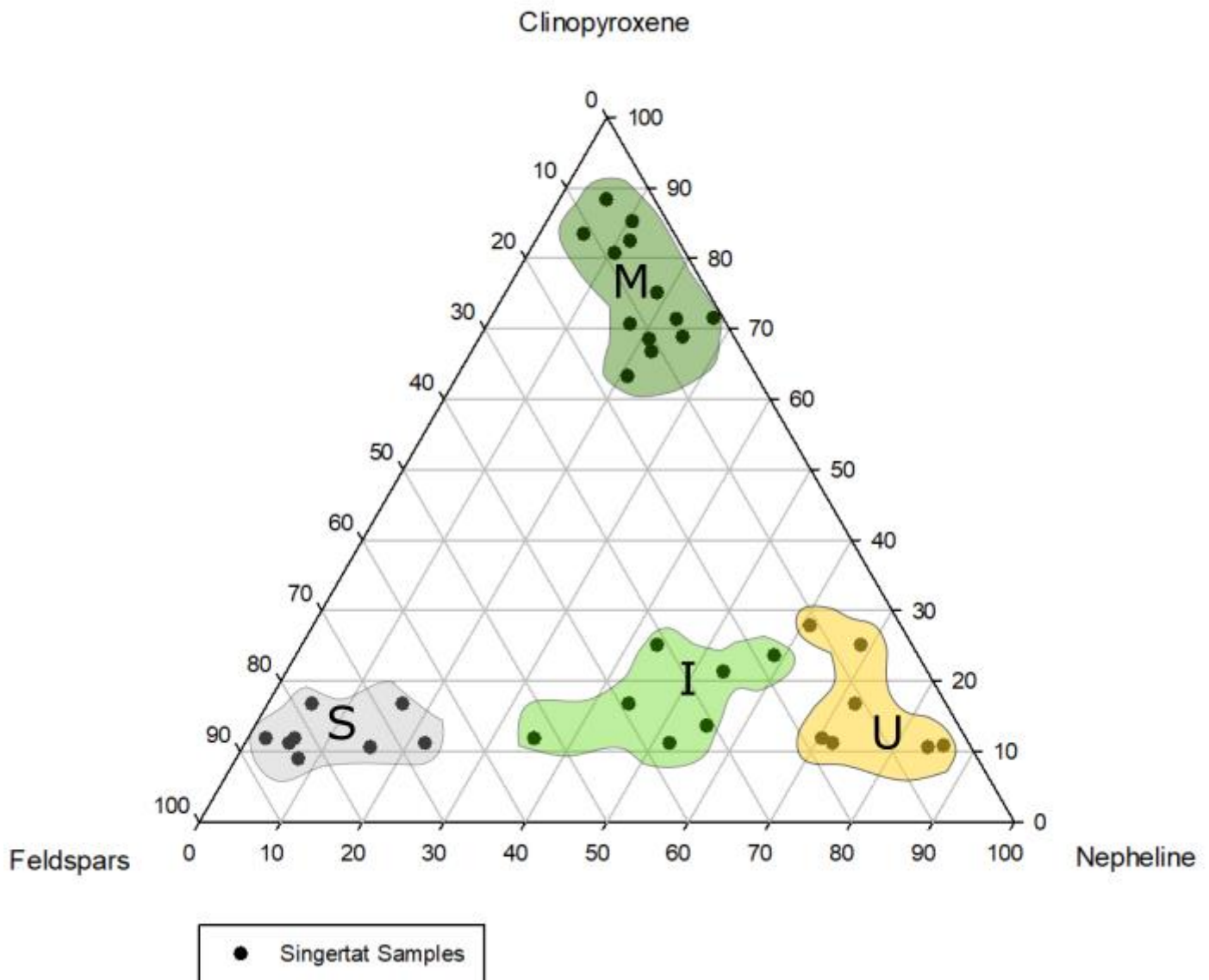
Figure 6.1: Ternary diagram used to classify the Singertât rock samples based on the modal abundances obtained during petrographic analyses. M = melteigites, I = ijolites, U = urtites and S = syenitic gneisses.
