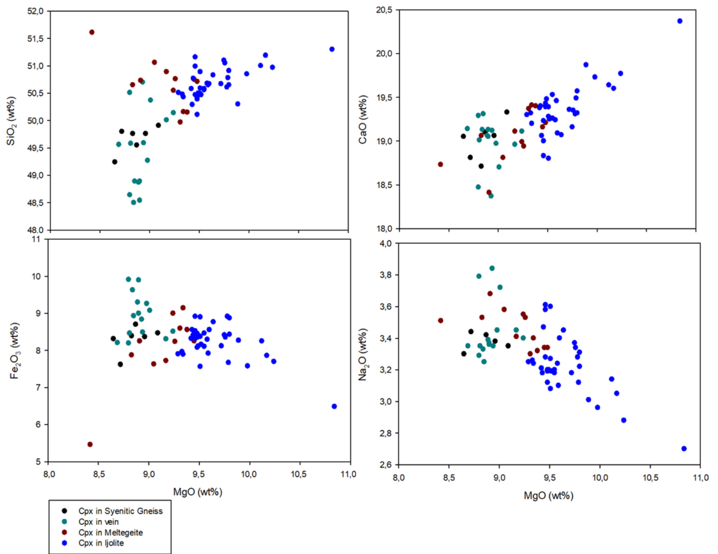
Figure 6.21: Variation diagrams depicting variations in mineral compositions for the layered sample 542219 which depicts the aegerine augite crystals in the syenitic gneiss, a vein of aegerine-augite within the syenitic gneiss, melteigite and ijolite.
