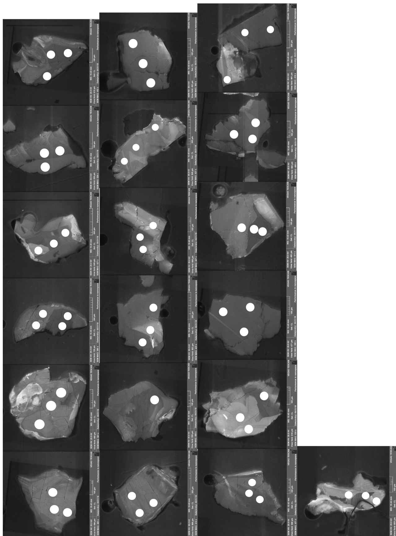
Figure 6.32: CL images depicting the laser spots of the magmatic zircons in the carbonatite breccia sample 525972
