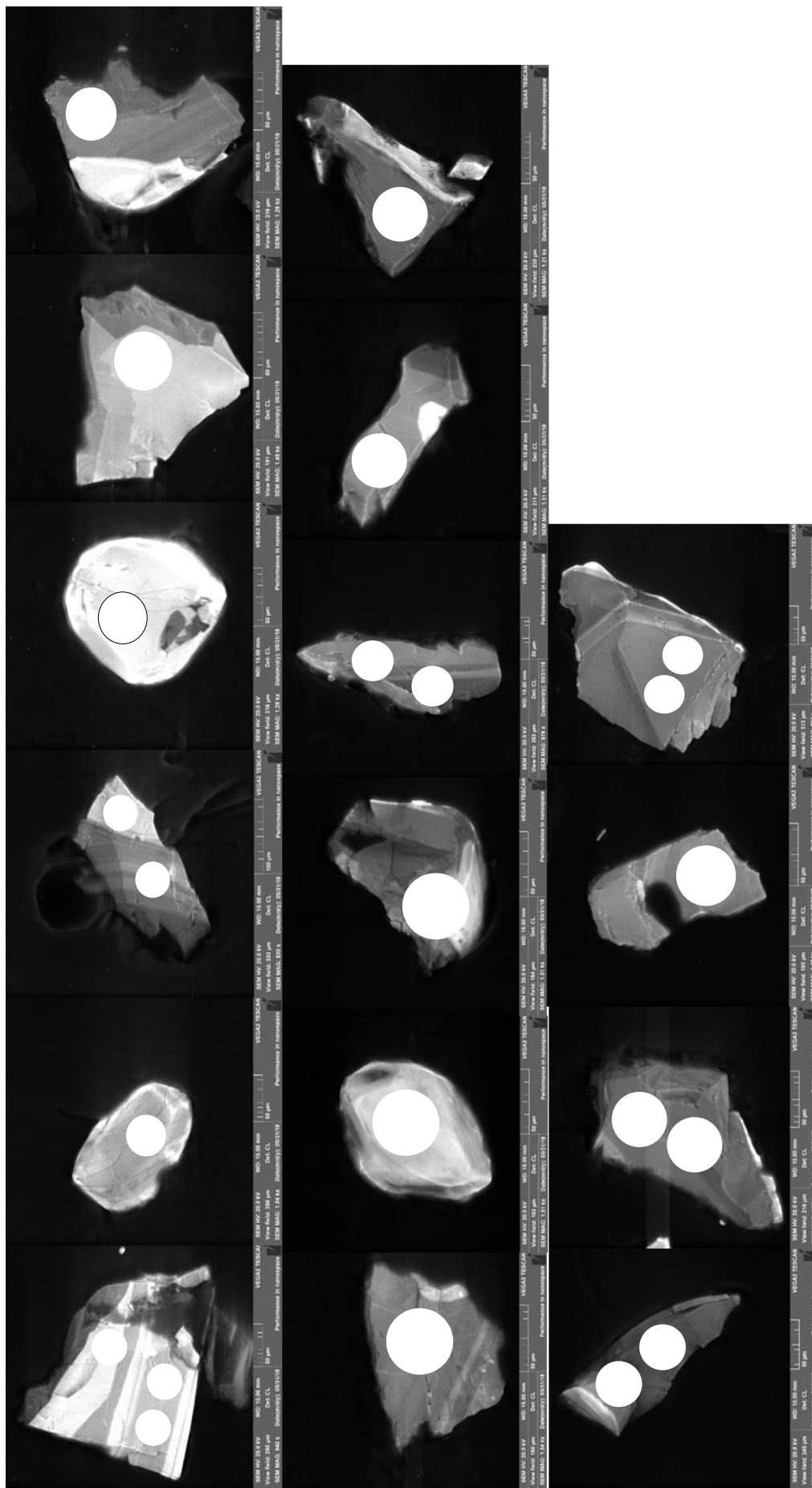
Figure 6.31: CL images depicting laser spot analyses of the magmatic zircons in the ijolite sample 525971
