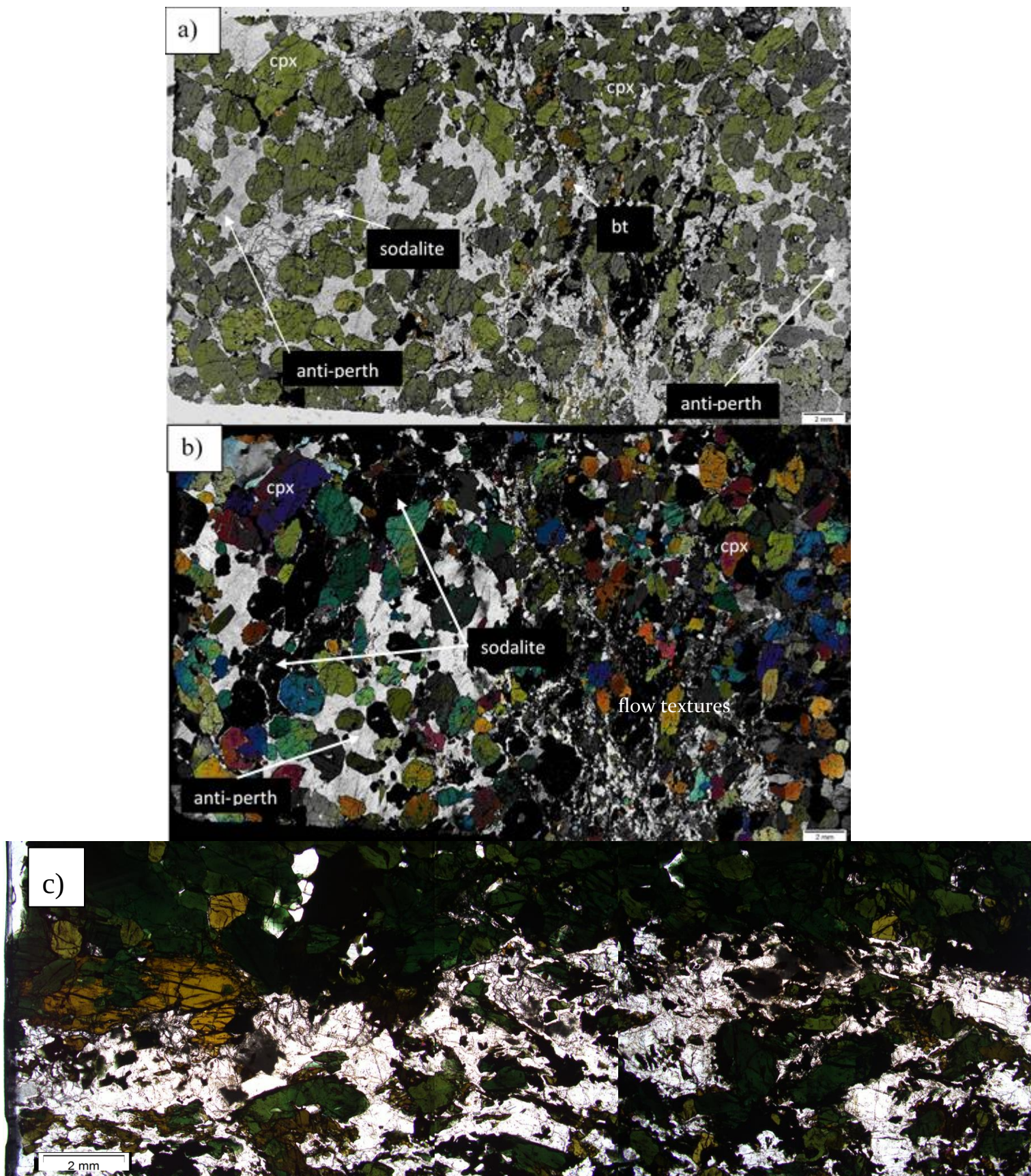
Figure 6.9: Photomicrographs of a layered nepheline-bearing rock sample 542219BII, which shows a gradational contact between an ijolite and a melteigite layer. In this sample there is little nepheline, however sodalite appears to be the dominant feldspathoid present and flow textures are observed in this sample, a) full thin section scan in ppl, b) thin sections scan in xpl c) depicts a truncated boundary seen in sample 542219CII.
