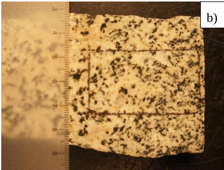
Figure 6.14: Hand samples of a) 542217, b) 525981 and c) 525989 which depicts syenitic gneisses showing the typical gneissic texture (alignment of aegirine-augite and biotite grains).
