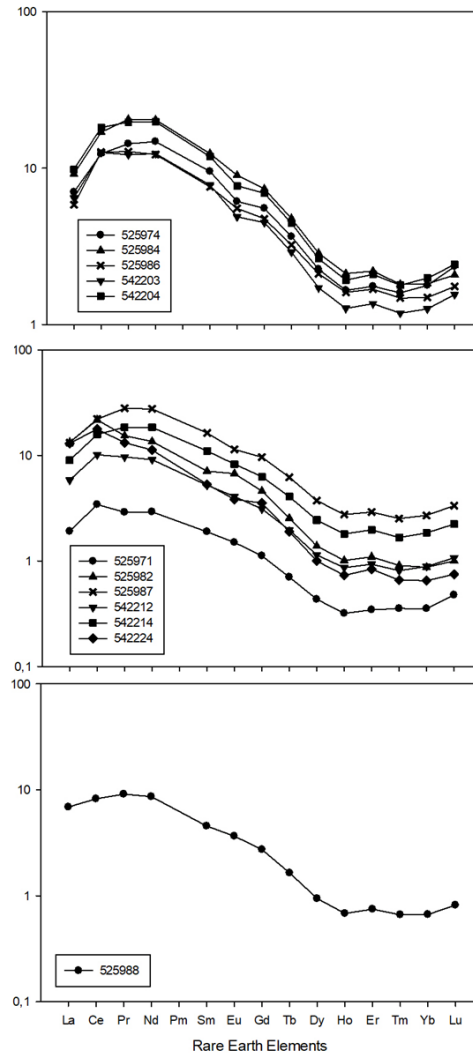
Figure 7.10: REE plots for the nepheline-bearing alkaline rocks of the Singertât Complex. The samples were normalized to chondrite (Anderson and Grevasse, 1988)
