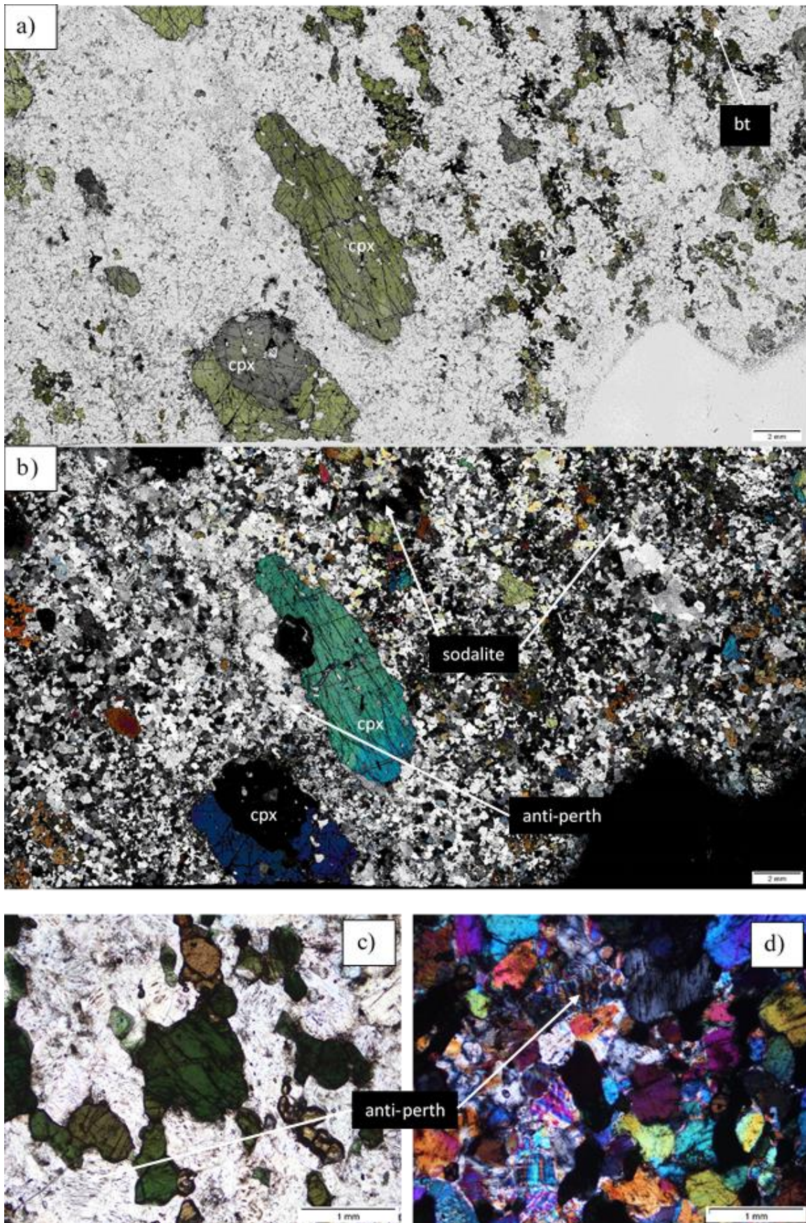
Figure 6.15: Photomicrographs of syenitic gneiss sample 542217B a) full thin section scan in ppl, b) thin sections scan in xpl, c) anti-perthite present in the ijolite samples in ppl, d) anti-perthite present in the ijolite samples in xpl.
