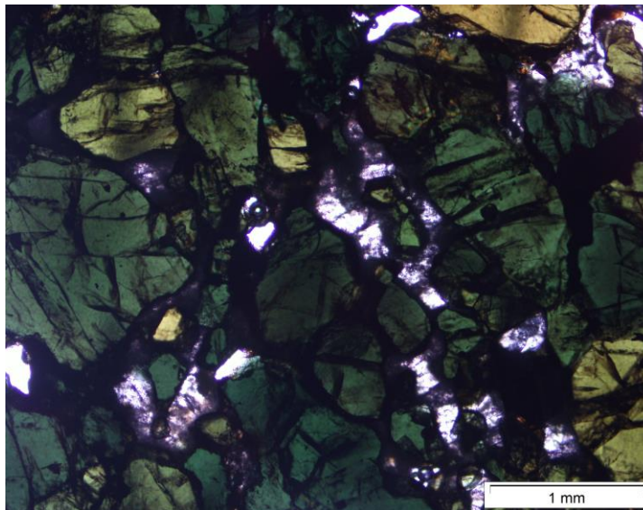
Figure 7.9: Melteigite depicting orthocumulate texture seen in the nepheline-bearing rocks of the Singertât Complex. We observe cumulate aegerine-augite with intercumulus nepheline.
