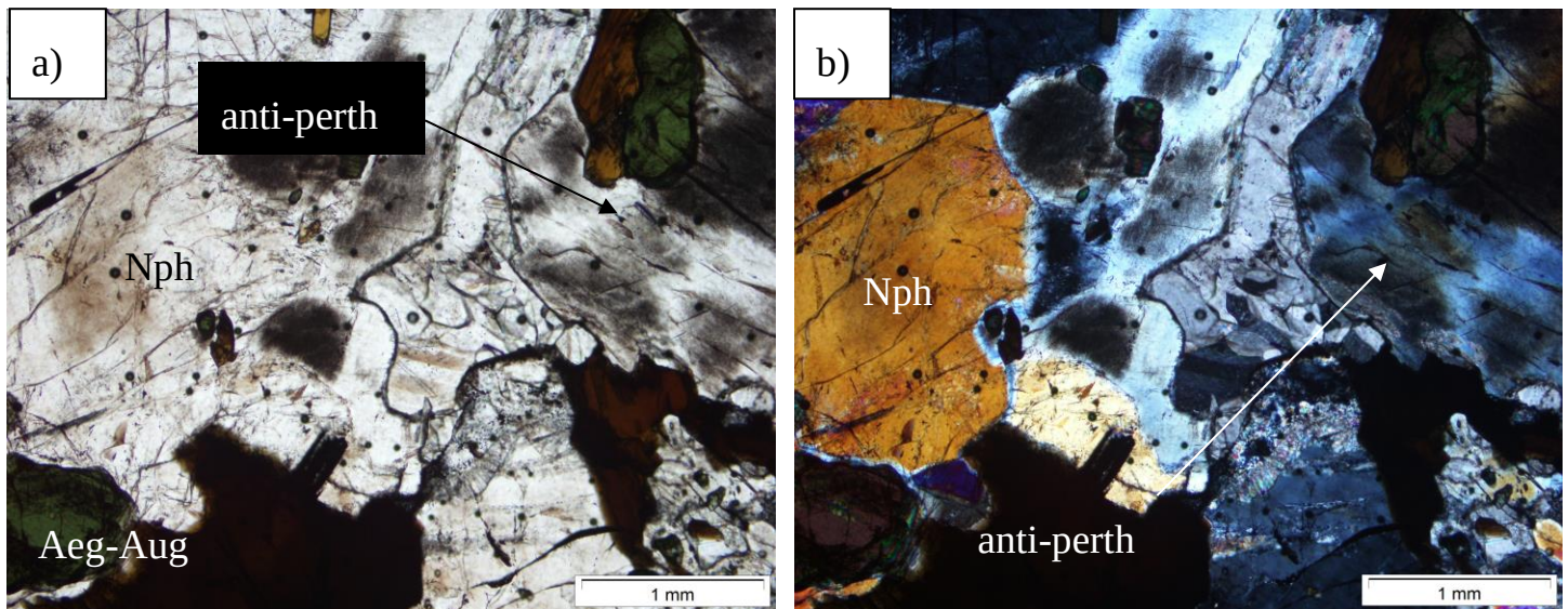
Figure 6.3: Photomicrographs of urtite sample 525988 showing the nepheline, anti-perthite and small percentage of clinopyroxene present in the sample. a) ppl, b) xpl.
