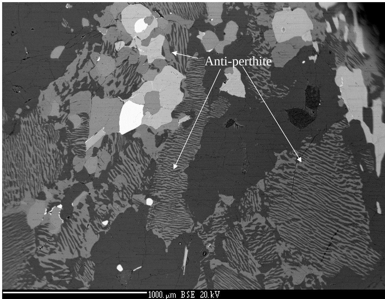
Figure 6.24: BSE image showing the anti-perthite that was analyzed in sample 542219. The dark grey lamellae are the orthoclase, while the lighter grey is the albite host.
