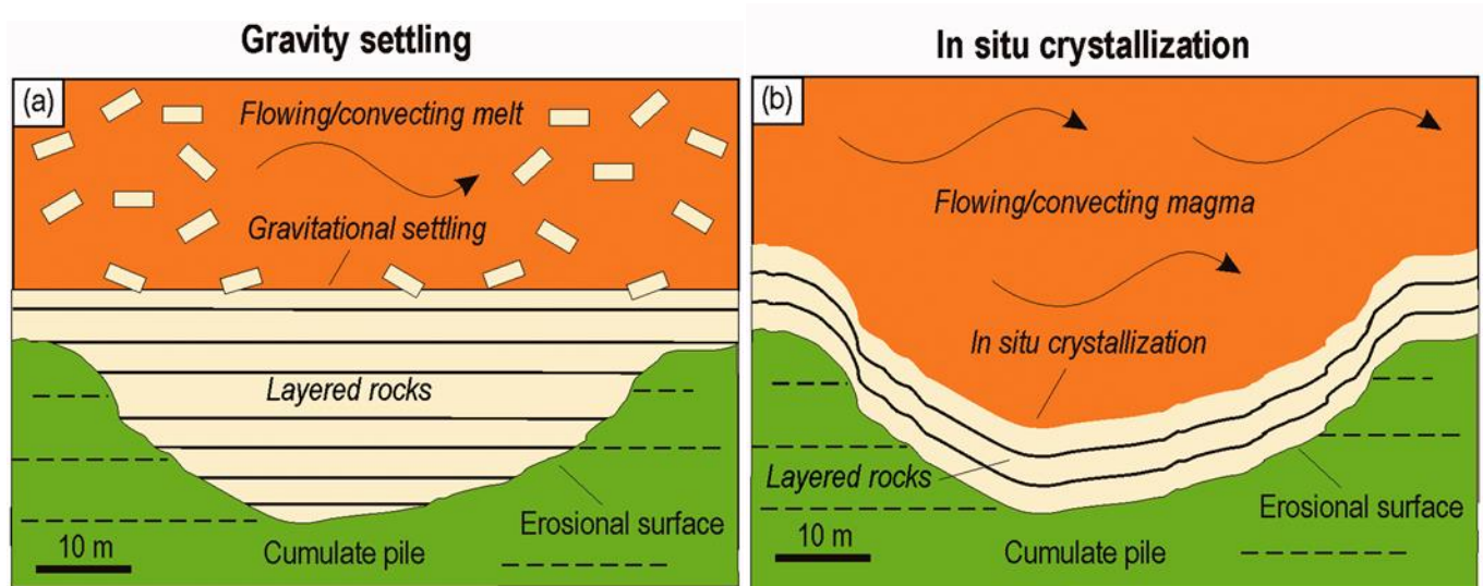
Figure 2.4: Predictions of the geometry of igneous layering within potholes owing to crystal settling (a) and in situ crystallization (b). Settling of crystals from flowing/convecting melt will form layered rocks that are discordant with respect to pothole margins. In contrast, in situ crystallization should result in layering that follows the outlines of pothole margins, (Latypov et al., 2015).
