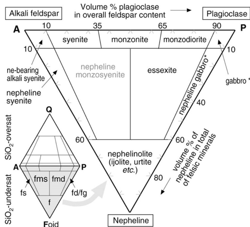
Figure 2.2: Generalized IUGS nomenclature for coarse-grained alkali rocks, based on the silica undersaturated portion of the QAPF diagram (bottom left). The main diagram shows the modal nomenclature applied to rocks, in which nepheline is the dominant Foid. The rock types seen at the top of the diagram with < 10% nepheline are said to be “nepheline-bearing” or “foiid bearing” rocks. f = foidolite, fmd = foid monzanite, fg = foid gabbro, P = feldspar >5% An, A = feldspar < 5% An. Taken from Gill (2010)
