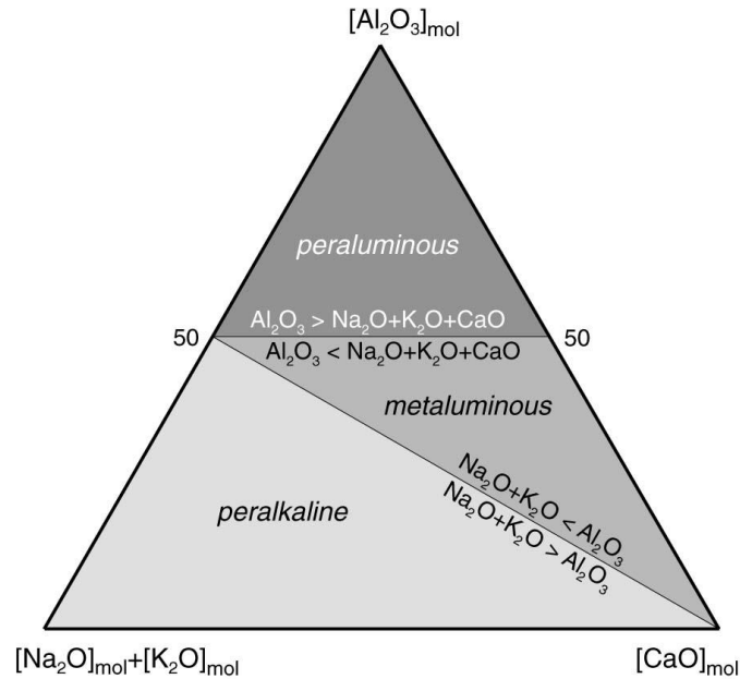
Figure 2.3: Ternary plot of peraluminous, metaluminous and peralkaline rocks, determined from whole rock \text{Na}_2\text{O} + \text{K}_2\text{O} , \text{Al}_2\text{O}_3 and \text{CaO} content (in molar proportions; Gill, 2010).
