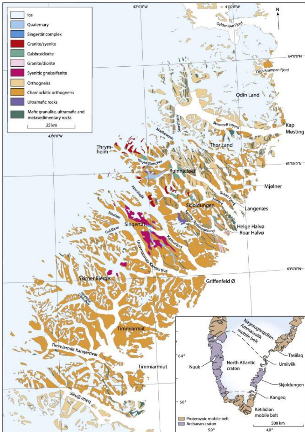
Figure 1.1: Schematic geological map showing the lithologies that make up the North Atlantic Craton (NAC). The inset shown on the bottom right of the geological map, shows the location of the SAIP and NAC in southern Greenland (Kolb et al., 2013).
