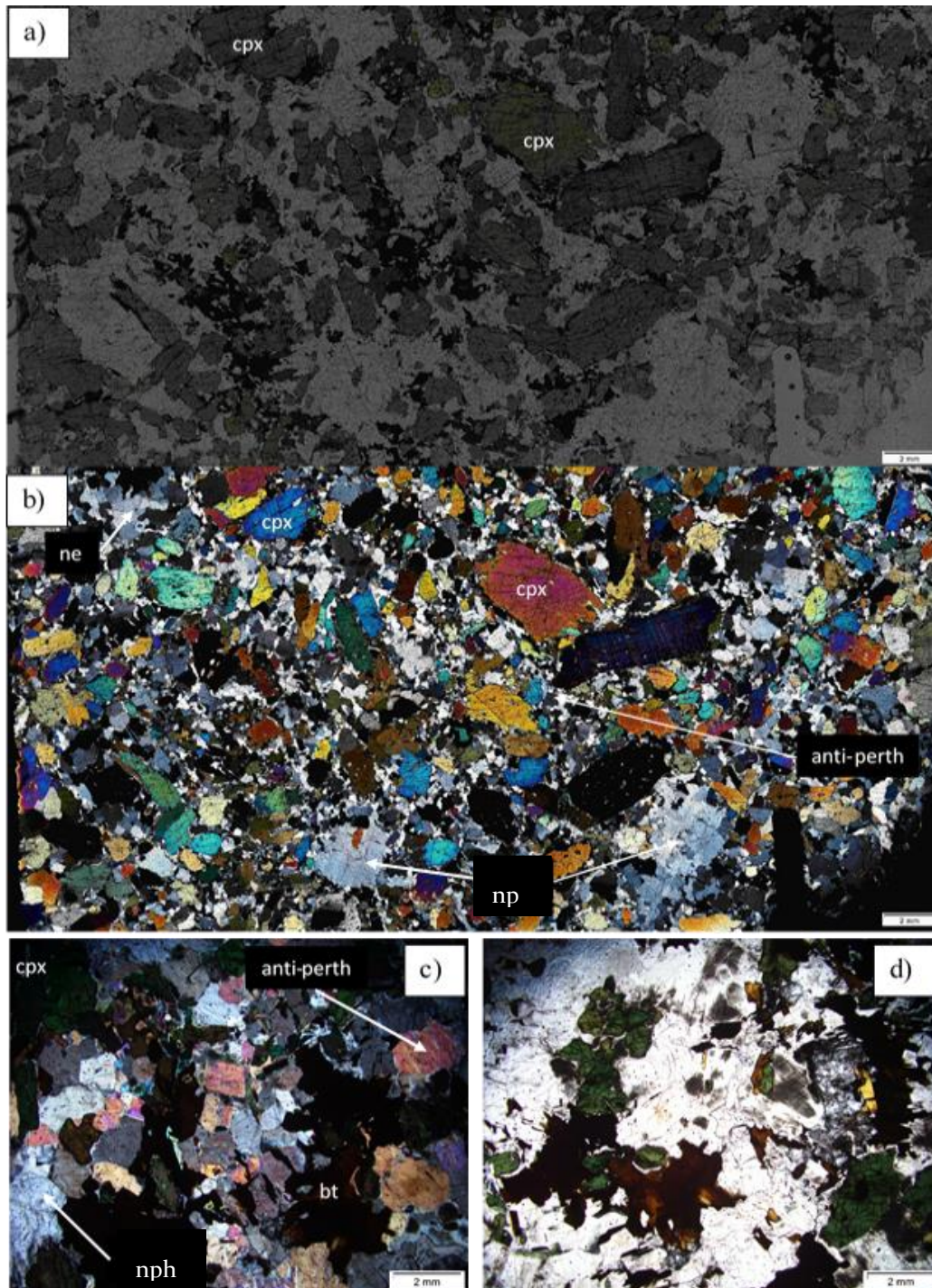
Figure 6.4: Photomicrographs of Ijolite samples 542214 a) full thin section scan in ppl, b) thin sections scan in xpl, c) anti-perthite present in the ijolite samples in ppl, d) anti-perthite present in the ijolite samples in xpl.
