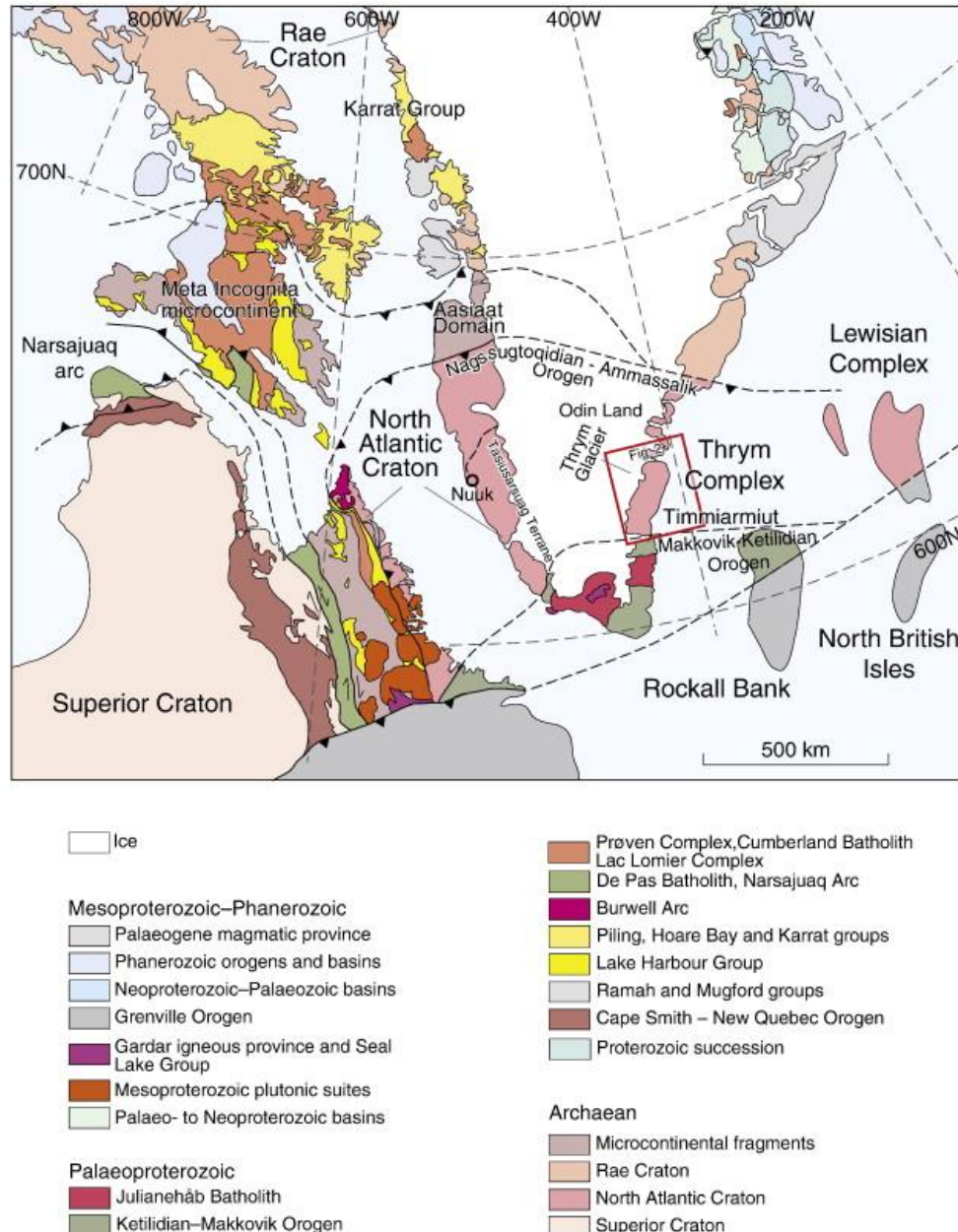
Figure 1.3: Schematic geological map showing the extent of the North Atlantic Craton (NAC). The red box shows the location of the SAIP on the NAC. (Bagas et al., 2013).
