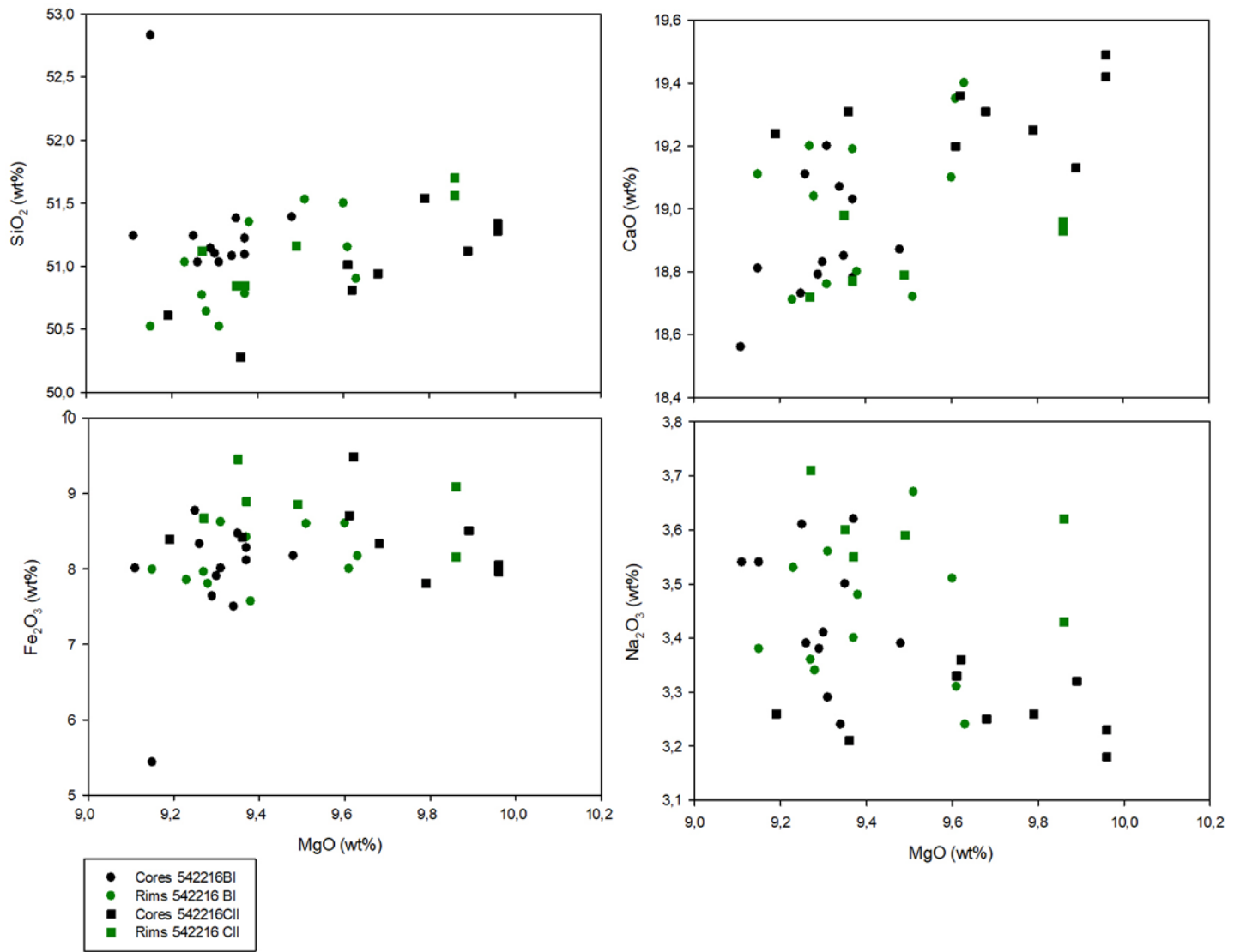
Figure 6.20: Variation diagrams depicting variations in mineral compositions for the layered samples 542216BI and 542216CII, which depicts the core- rim data for aegerine-augite.
