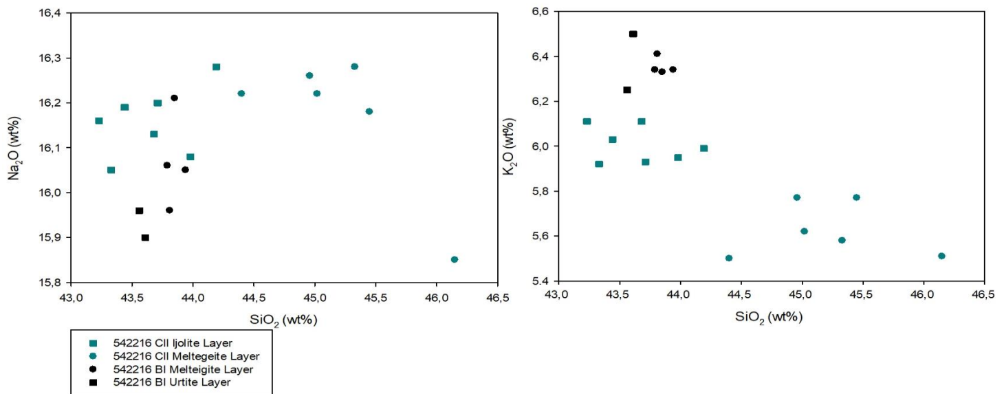
Figure 7.6: Depicting the compositionally different populations of nepheline across sharp boundaries in between and ijolite and a melteigite and a melteigite and urtite.
