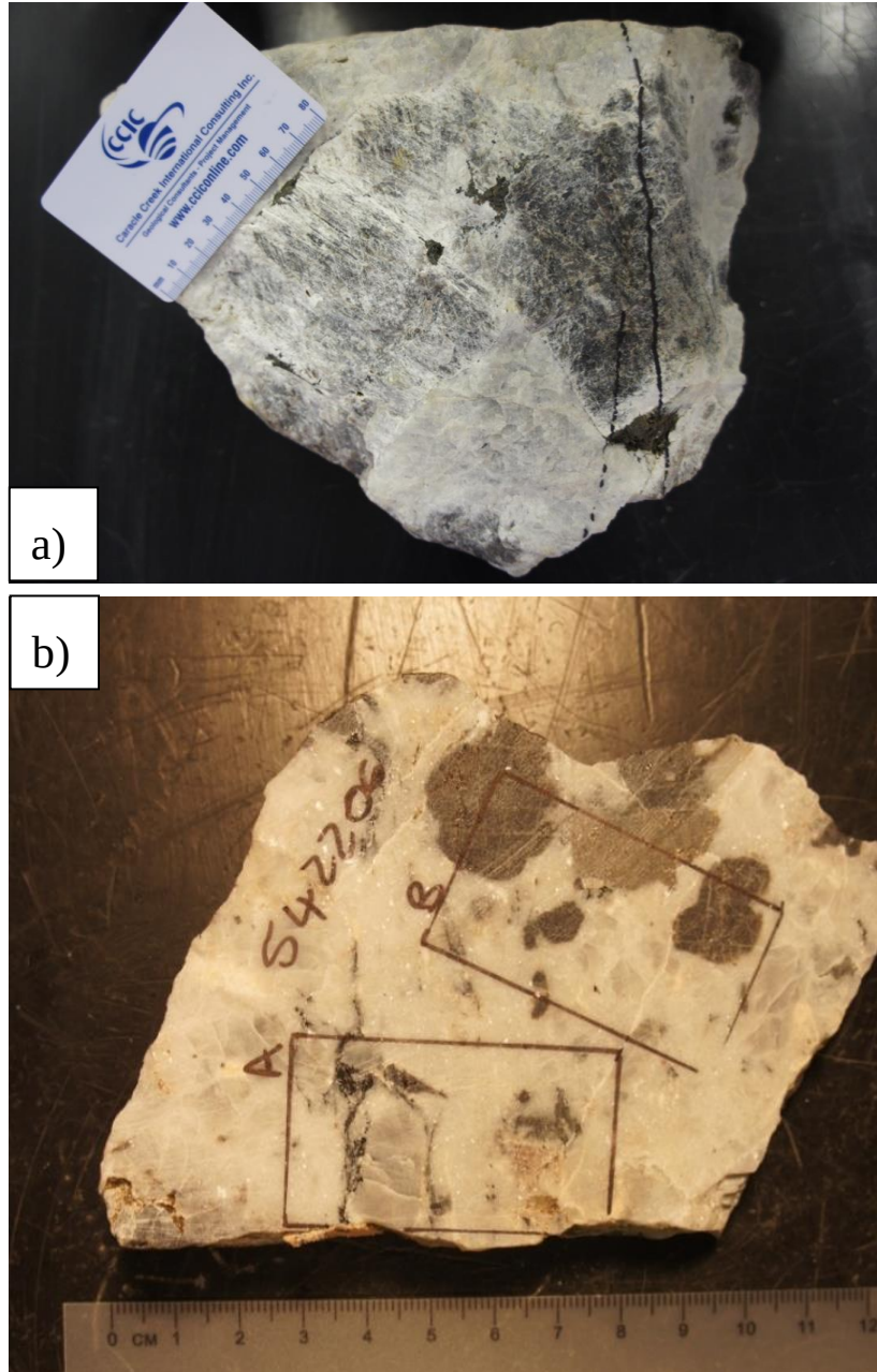
Figure 6.10: Hand samples of a) 525969 and b) 542206 which depicts pegmatitic nepheline (pale brown-grey), feldspars (white) and biotite (dark brown – black).
