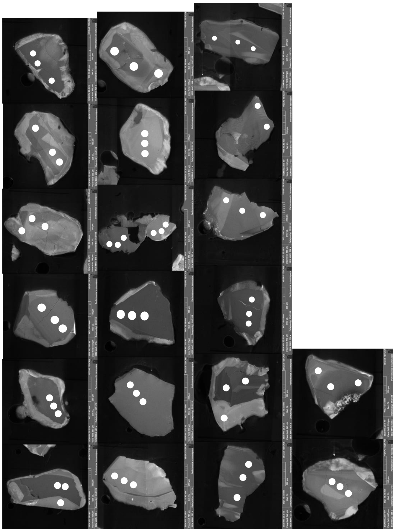
Figure 6.34: CL images depicting the laser spots of the magmatic zircons in the pegmatite sample 542206.
