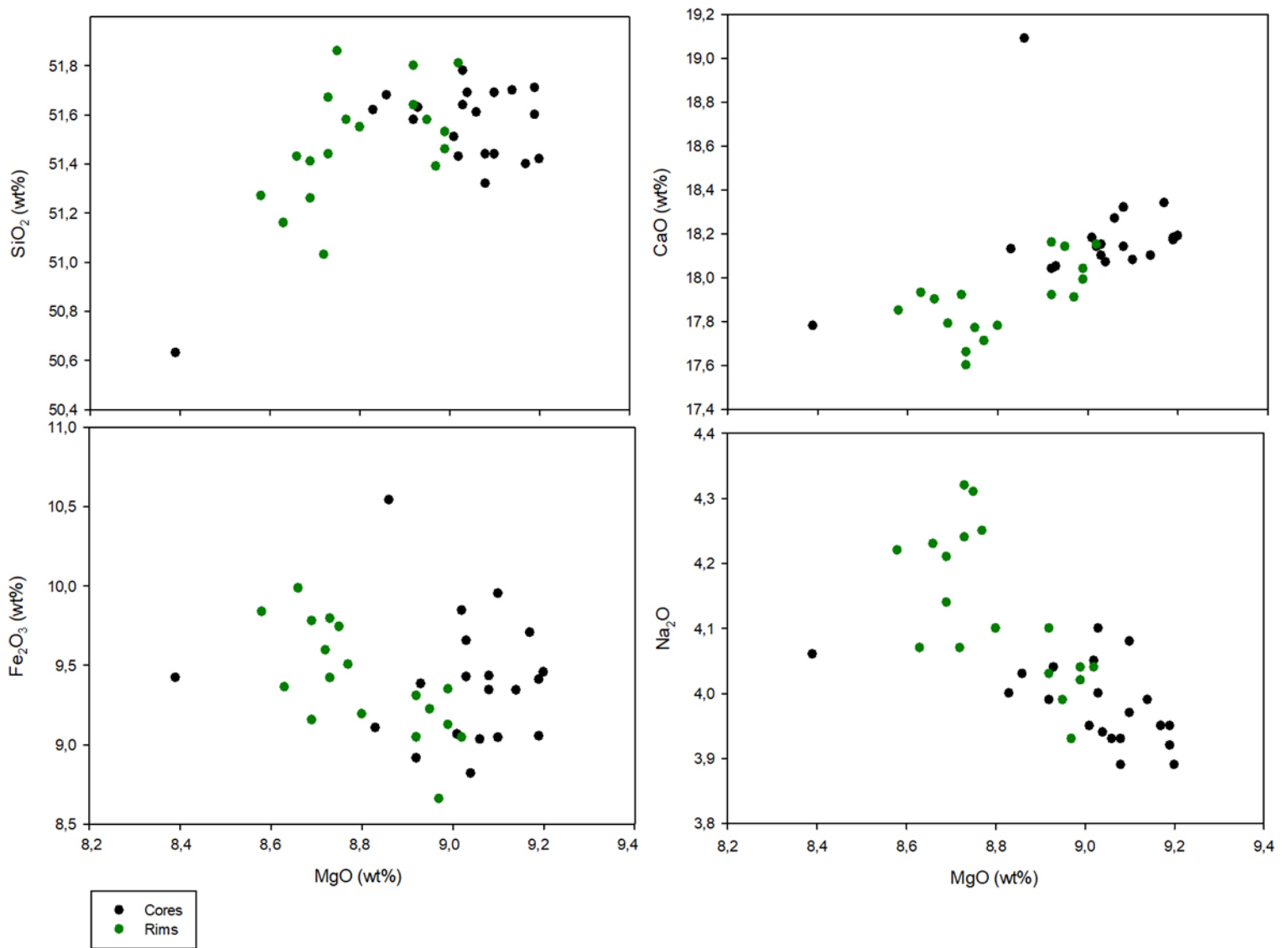
Figure 6.19: Variation diagrams depicting variations in mineral compositions for the layered sample 542205 which depicts the core- rim data for aegirine-augite.
