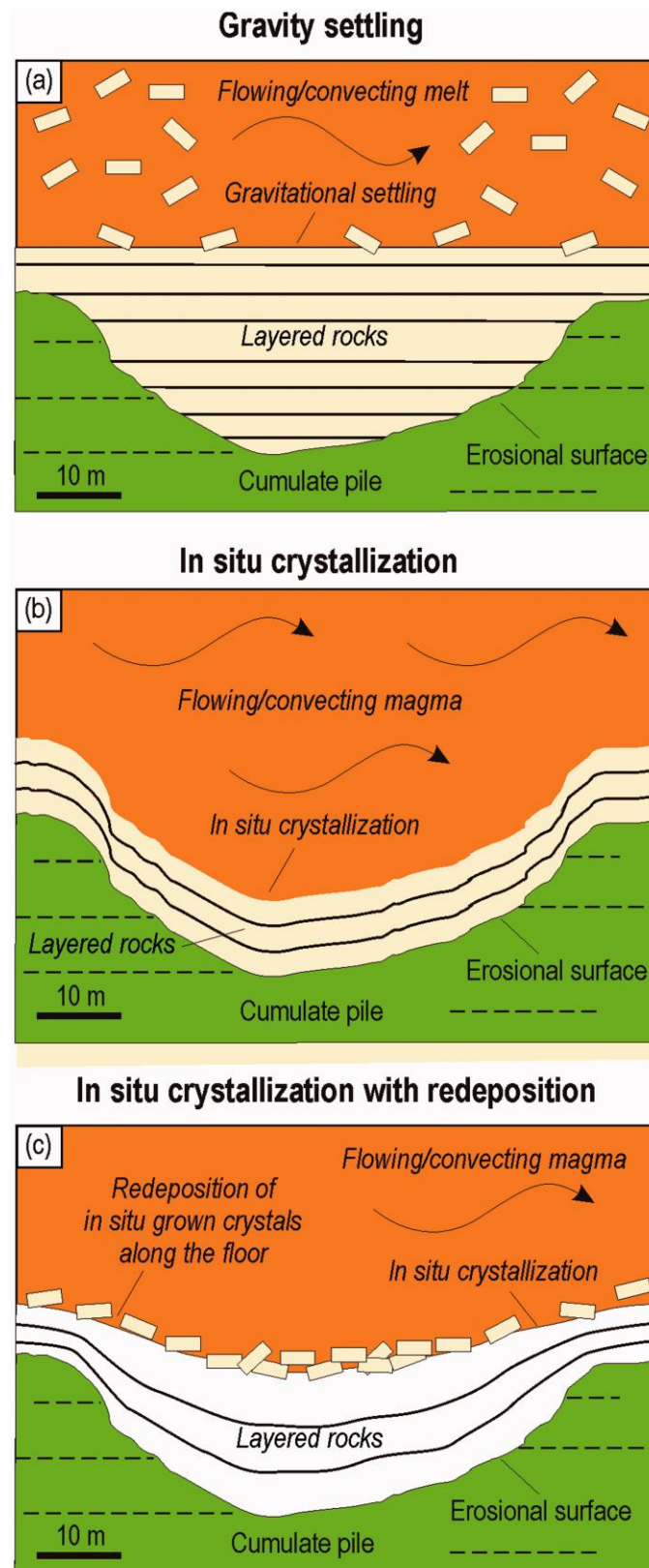
Figure 7.5: Predictions of the geometry of igneous layering within potholes owing to crystal settling (a) and in situ crystallization (b). Settling of crystals from flowing/convecting melt will form layered rocks that are discordant with respect to pothole margins. In contrast, in situ crystallization should result in layering that follows the outlines of pothole margins, (Latypov et al., 2015).
