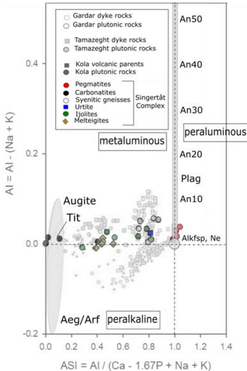
Figure 7.3: Whole-rock data in molecular proportions of the Singertât Complex in Comparison to the rocks from the Gardar Province, the Kola Peninsula and the Tamazeght complex plotted on an AI vs ASI diagram using the definitions by Frost & Frost (2008). The gray fields indicate the composition of important fractionating mineral phases (Marks et al., 2011).
