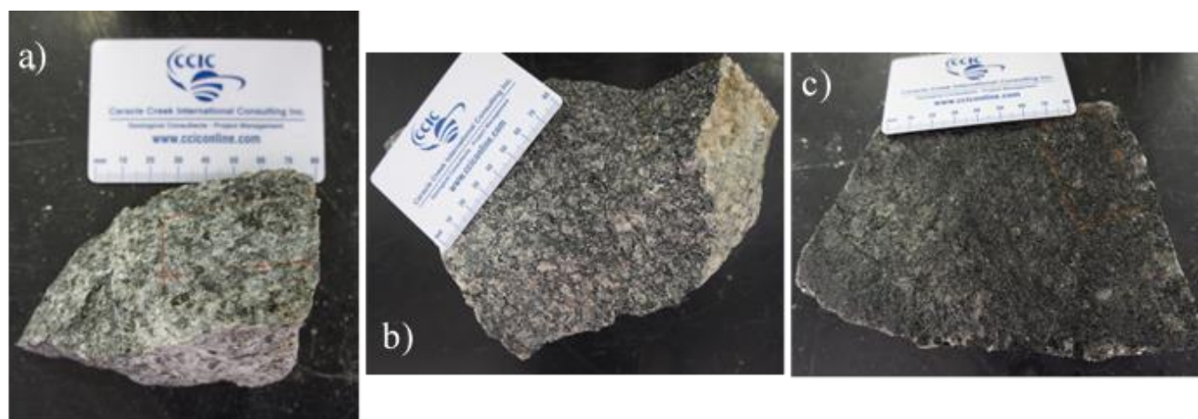
Figure 6.2: a) Urtite from the Singertât Complex, SE Greenland. The green mineral is clinopyroxene while the grey mineral is nepheline and the white mineral is alkali feldspar (Sample 525988). b) Ijolite from the Singertât Complex, SE Greenland. The black-green mineral is clinopyroxene, while the grey-brown mineral is nepheline and the white mineral is alkali feldspar (Sample 542214). c) Melteigite from the Singertât Complex, SE Greenland. The black-green mineral is clinopyroxene, while the grey-brown mineral is nepheline and the white mineral is alkali feldspar (Sample 542203).
