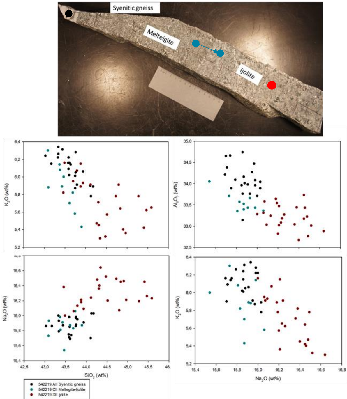
Figure 6.18: Variation diagrams depicting variations in mineral compositions for the layered sample 542219 using thin sections 542219 AII, CII and DII which transitions from syenitic gneiss to melteigite and then to ijolite. The black dots represent analyses from the syenitic gneiss layer, the blue dots represent analyses taken across the melteigite-ijolite transition and the red dots represent analyses from the ijolite layer.
