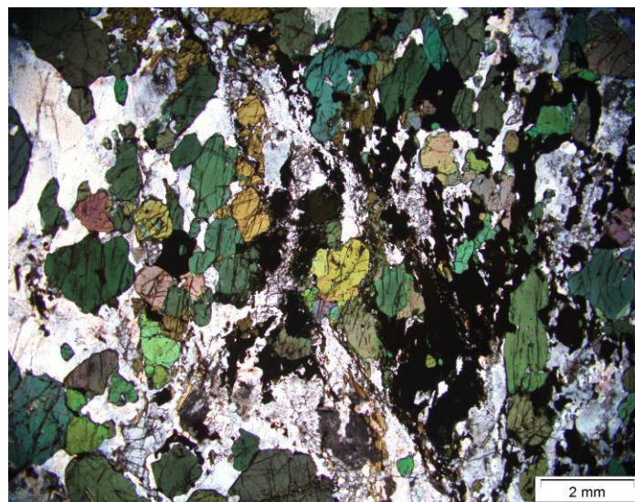
Figure 7.8: Sample 542219 depicting flow textures in a nepheline-bearing rock, which may have formed due to new magma being emplaced in a magma chamber resulting in convection currents which formed the flow textures.
