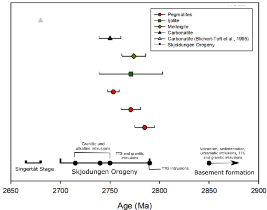
Figure 7.1: Geological timeline depicting the ages of the zircons analyzed in this study placing the timing of the Singertat Complex emplacement in the early stages of the Skjoldungen Orogen (Kolb et al. , 2013). Note that no error bar was provided for the Blichert-Toft et al. , 1995 age, seen as the gray triangle.
