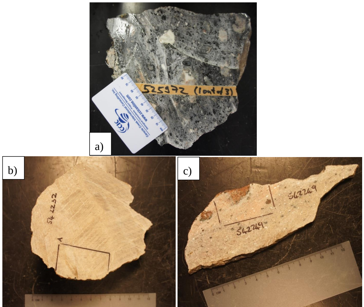
Figure 6.12: Hand samples of a)525972, b)542232 and c) 542249 which depicts a carbonatite breccia (contains fragments of nepheline-bearing rocks and pegmatite), a carbonatite containing almost 100% calcite and a carbonatite containing high Ti-garnet respectively.
