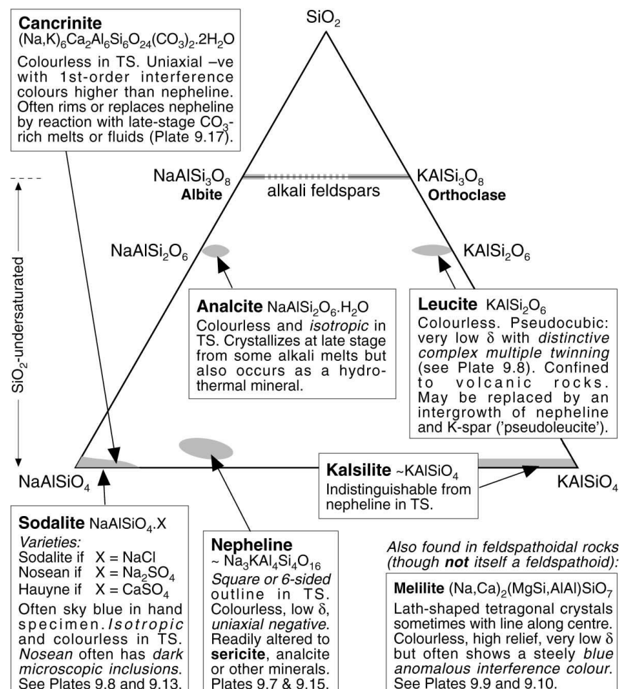
Figure 2.1: Ternary diagram showing how different feldspathoids relate compositionally and the different alkali feldspars (in molar proportions). Optical features of each feldspathoid is present. TS=thin section. Taken from Gill (2010).
