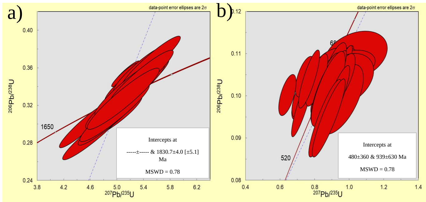
Figure 5.3: Concordia plots for the secondary standards that were measured while analyzing the Singertât Complex zircon samples a) CDQGNG b) Mud Tank.
