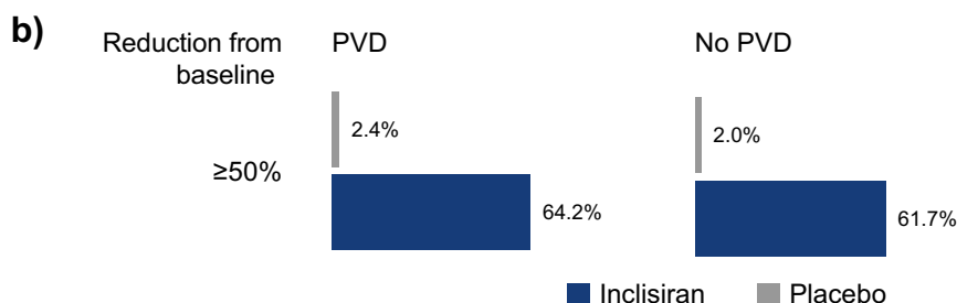
Fig. 3 The proportion of patients achieving pre-specified LDL-C thresholds and a percentage reduction in LDL-C ≥ 50% at day 510. a The proportion of patients achieving pre-specified LDL-C thresholds
