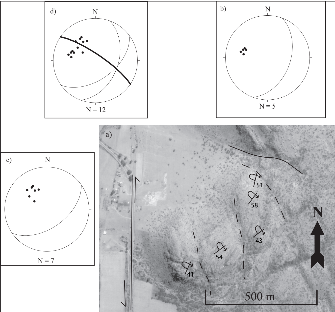
Fig. 2.19: (a) Enlargement of a 1:25 000 aerial photograph of a fold (labelled 2 in Fig. 2.10) in the outer northern parts of the collar of the Vredefort Dome (Central Rand Group) (locations 358-363, see Appendix No. 6) immediately east of the main road from Parys to Potchefstroom (R 53). (b) and (c) Poles to the bedding and the great circles are given as lower hemisphere equal area stereographic projections (Schmidt net) for the eastern limb (b) and western limb (c), and (d) for the constructed fold axial plane (bold circle).
