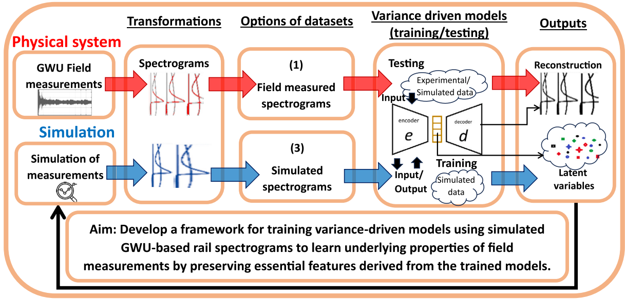
Fig. 2. Schematic representation of the methodology for this study.
