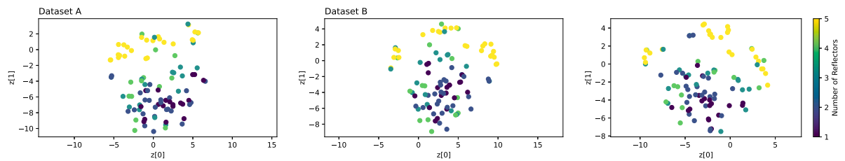
Fig. 18. t-SNE reduction of VAE 1600 latent variables recovered from simulated test samples to visualise the number of reflectors in spectrograms.
