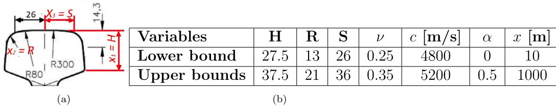
Fig. 9. (a) Standard UIC60 rail head profile highlighting parameters used to describe wear and (b) ranges for the variables used to generate simulated data.
