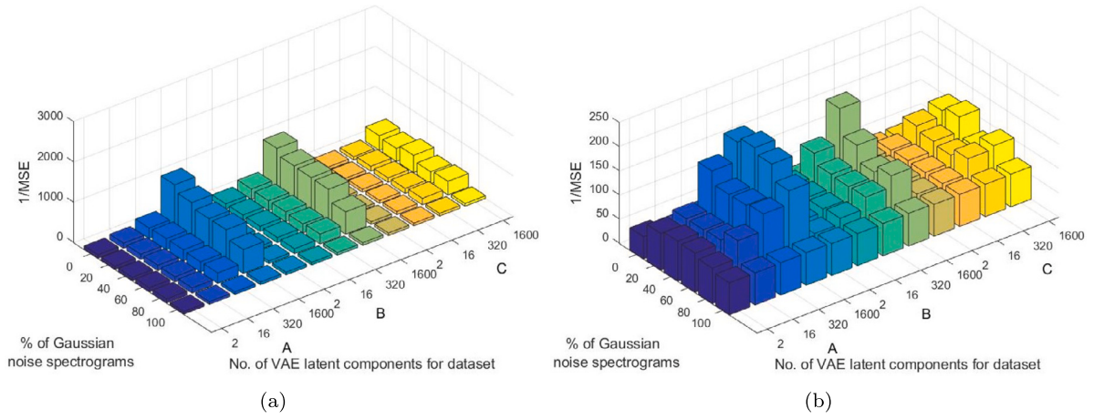
Fig. 13. Reciprocal of the mean squared error using the VAE models to reconstruct the error (sensitivity) of (a) spectrograms with coherent features only and (b) spectrograms with coherent features and added noise to each sample, versus the number of latent variables and the percentage of Gaussian noise spectrograms in a training batch.
