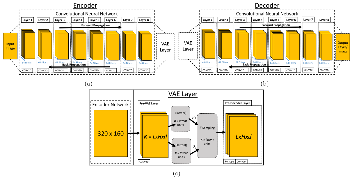
Fig. 3. The VAE network architecture including (a) encoder, (b) decoder and (c) VAE layer.
