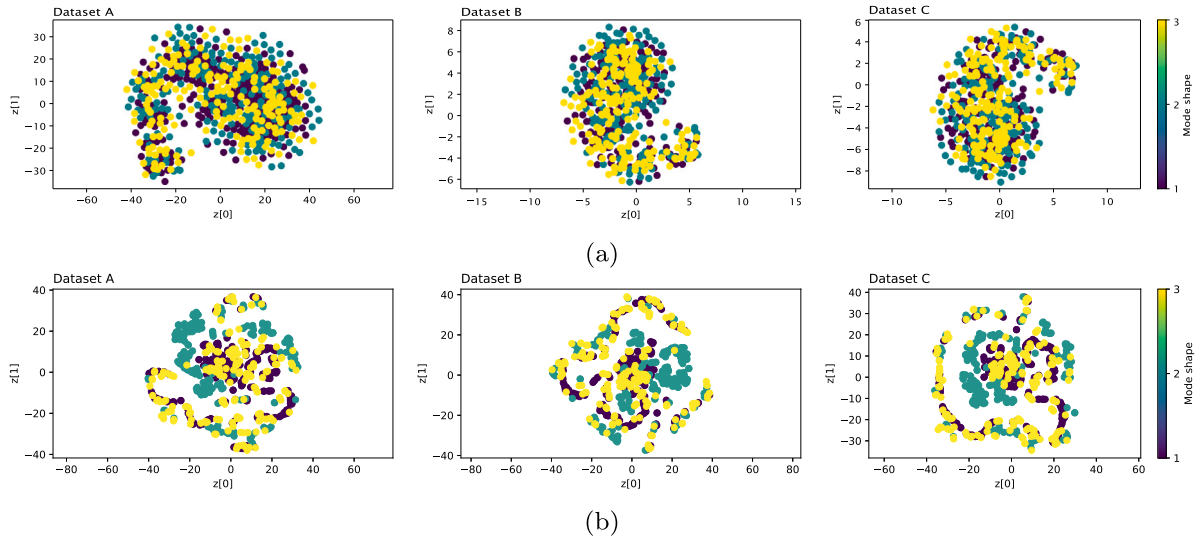
Fig. 20. t-SNE visualisation of the mode shape type using 1600 latent variables: (a) PCA (top row) and (b) VAE (bottom row).
