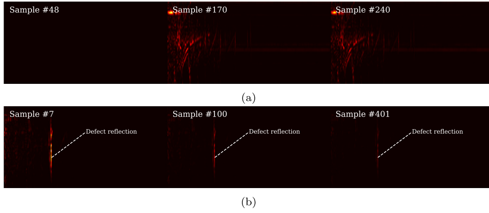
Fig. 23. The PCA inverse transform of sample spectrograms using only (a) PC1 and (b) PC3. The horizontal axes represent time in seconds, while the vertical axes denote the frequency of the reconstructed spectrograms.
