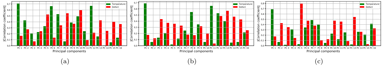
Fig. 26. Plots showing the correlation between the first 16 PCs and the measured temperature and artificial defect amplitude for models trained using simulated datasets (a) A, (b) B and (c) C.
