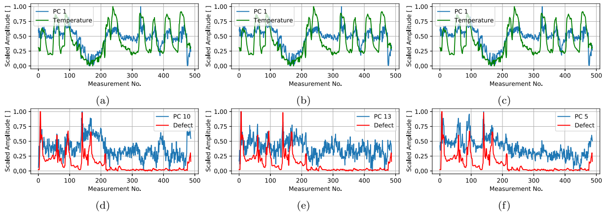
Fig. 27. Plots the measured temperature and the best-correlated PC for models trained using simulated datasets (a) A, (b) B and (c) C, and the measured defect amplitude and the best-correlated PC for models trained using simulated datasets (d) A, (e) B and (f) C.
