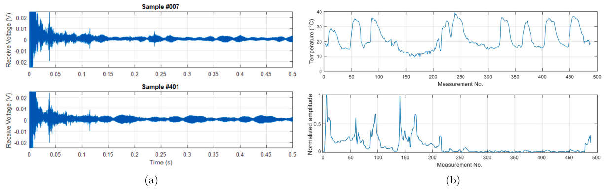
Fig. 5. (a) Pulse-echo measurements performed on a UIC60 rail with an artificial defect attached to the rail head. (b) Temperature measured in a cabinet placed near the rail and the normalised amplitude of a reflection from an artificial defect attached to the head of the rail.
