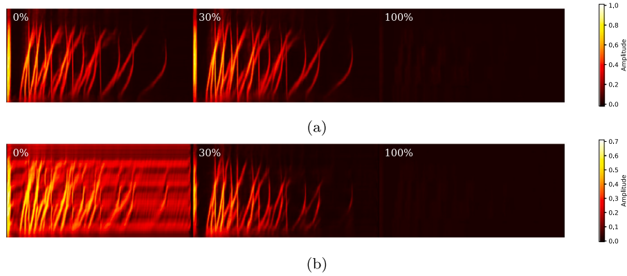
Fig. 14. Reconstructions of the samples in Figs. 10(a) and 10(b) using a VAE model trained with dataset A and 1600 latent components, under varying percentages of Gaussian noise spectrograms in the training batch: (a) shows the reconstruction of the sample spectrogram in Fig. 10(a), and (b) shows the reconstruction of the sample spectrogram in Fig. 10(b). The horizontal axes represent time in seconds, while the vertical axes denote the frequency of the reconstructed spectrograms.
