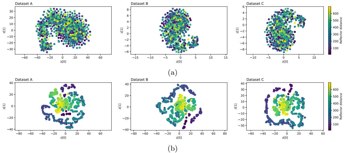
Fig. 21. t-SNE visualisation of the reflector distance using 1600 latent variables: (a) PCA (top row) and (b) VAE (bottom row).
