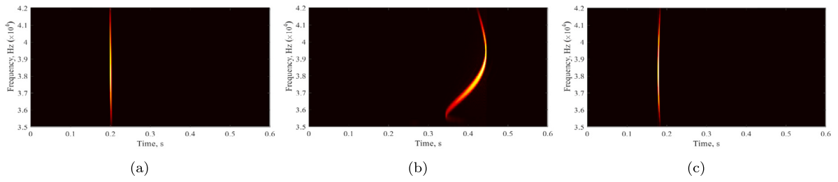
Fig. 19. Samples of the three main modes of propagation observed in experimental measurements: (a) Mode 1, (b) Mode 2 and (c) Mode 3.
