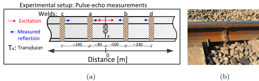
Fig. 4. (a) Illustration of the experimental setup with estimated weld distances from the transducer location. (b) Photograph of an aluminothermic weld.
