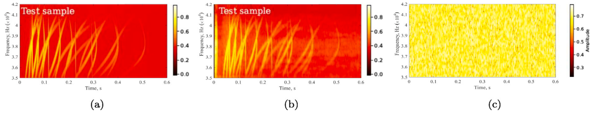
Fig. 10. Samples of the five-reflections spectrograms generated from SAFE models: (a) without Gaussian noise added and (b) with Gaussian noise added to each spectrogram, and (c) a sample of a Gaussian noise spectrogram included in the training batch.
