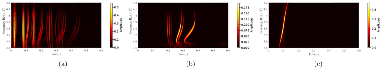
Fig. 8. Samples from datasets with (a) multiple weld reflections (dataset A), (b) single welds (dataset B) and (c) isolated propagating modes (dataset C).
