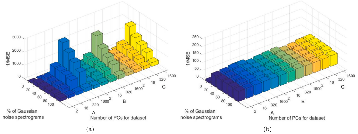
Fig. 11. Reciprocal of the mean squared error using the PCA models to reconstruct the error (sensitivity) of (a) spectrograms with coherent features only and (b) spectrograms with coherent features and added noise to each sample, versus the number of latent variables and the percentage of Gaussian noise spectrograms in a training batch.
