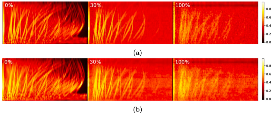
Fig. 12. Reconstructions of the samples in Figs. 10(a) and 10(b) using a PCA model trained with dataset A and 1600 latent components, under varying percentages of noise Gaussian spectrograms in the training batch: (a) shows the reconstruction of the sample spectrogram in Fig. 10(a), and (b) shows the reconstruction of the sample spectrogram in Fig. 10(b). The horizontal axes represent time in seconds, while the vertical axes denote the frequency of the reconstructed spectrograms.
