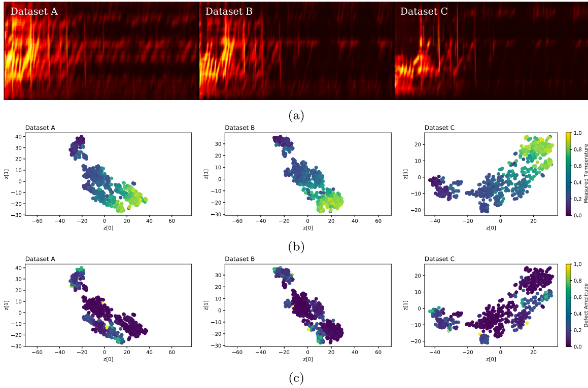
Fig. 25. (a) Sample spectrograms reconstructed (with the horizontal axes representing the time in seconds, while the vertical axes denote the frequency of the reconstructed spectrograms), (b) t-SNE visualisation for temperature and (c) a growing defect using a VAE model trained using 1600 latent variables and three simulated datasets.
