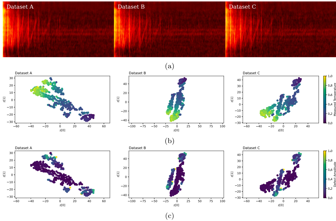
Fig. 24. (a) Sample spectrograms reconstructed (with the horizontal axes representing the time in seconds, while the vertical axes denote the frequency of the reconstructed spectrograms), (b) t-SNE visualisation for temperature and (c) a growing defect using a PCA model trained using 1600 latent variables and three simulated datasets.
