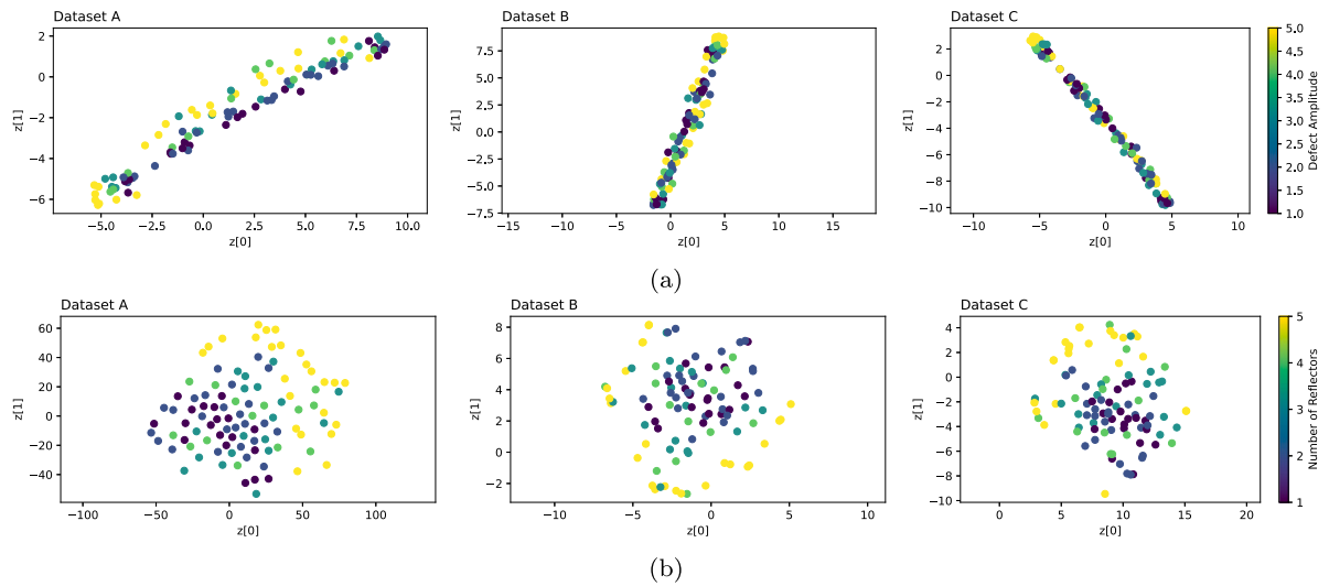
Fig. 16. t-SNE reduction of (a) 4 and (b) 1600 latent variables recovered from test simulated samples for models trained using PCA.
