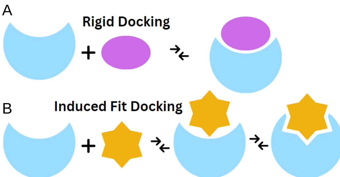
Figure 7: Comparing Rigid and Induced Fit Docking Models. A: In traditional virtual docking investigations, ligands are introduced into the binding site of a receptor under the assumption that the receptor remains rigid, referred to as the 'Lock-and-Key' model. However, relying on a fixed receptor may lead to inaccurate outcomes, as numerous proteins in reality exhibit dynamic side-chain or backbone movements, or both, when interacting with ligands. B: These dynamic alterations enable the receptor to modify its binding site to better match the shape and binding manner of the ligand, commonly known as 'Induced Fit Model'. Image was generated using Canva. (Koshland., 1995; Morrison et al. , 2006).
