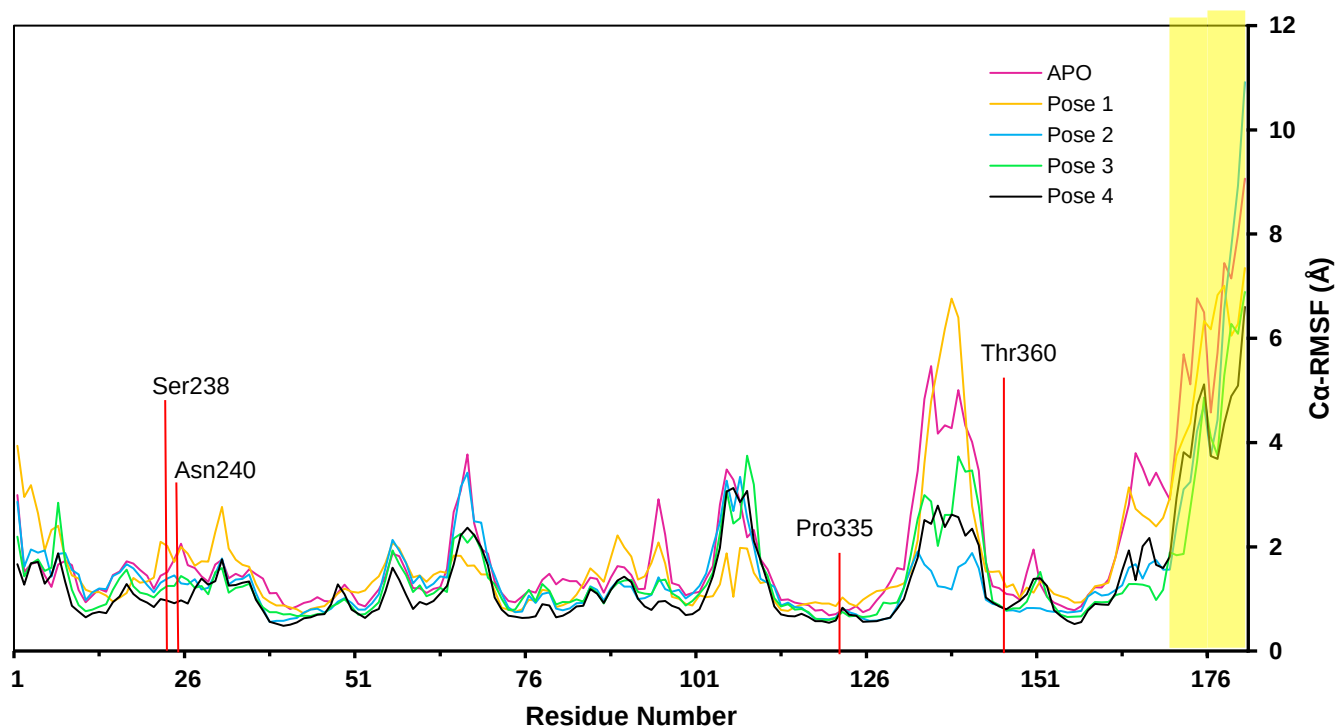
Figure 23: Ca-RMSF for each residue in the TBR1 T-box domain, emphasising residues involved in hydrogen bond formation with the ligand across the entire 250 ns simulation. The Ca RMSF value for each residue in the APO Protein (pink), Pose 1 (orange), Pose 2 (blue), Pose 3 (green) and Pose 4 (black) are shown. The CBD-interacting residues showing a common trend in the four poses are shown by red lines and are labelled. The yellow highlighted region represents the residues associated with direct DNA binding and thus functionality. The graph was generated using MS Excel based off calculations from Maestro Schrödinger.
