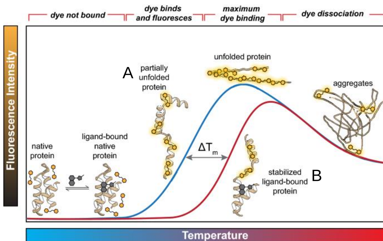
Figure 14: TSA Principle. A TSA measures the melting temperature ( T_m ) of the protein, which reflects the temperature at which half of the protein population transitions from a folded to an unfolded state upon increase in temperature. A: The exposure of hydrophobic residues, due to protein unfolding, results in increased fluorescence of SYPRO Orange dye – which binds to those hydrophobic patches. B: Compound binding to the target protein can enhance its stability, consequently elevating the T_m . Image was sourced from Samuel et al. , (2021).
