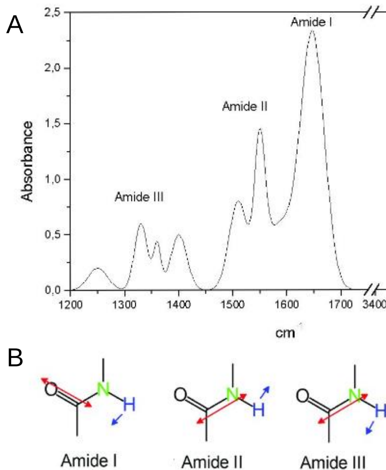
Figure 16: Amide I, Amide II and Amide III Vibrations in FTIR. A: Location of amide I ( 1600\text{--}1700\text{ cm}^{-1} ), amide II ( 1510\text{--}1580\text{ cm}^{-1} ), and amide III ( 1250\text{--}1350\text{ cm}^{-1} ) bands in an FTIR spectrum. B: Red arrows represent C=O and N-H stretching. Blue arrows represent N-H bending. The Amide I band predominantly arises from the stretching vibrations of the C=O bond, constituting 70% to 85% of the potential energy within the amide bond. Its determination is primarily governed by the backbone conformation, showing independence from the amino acid sequence, as well as charge or hydrophobic/phillic properties. The Amide II band primarily results from bending vibrations of the N—H bond (40 – 60% of the bonds potential energy), C-N stretching vibration (18 – 40% of potential energy) and C-C vibrations (roughly 10% of the potential energy). Amide II bands are responsive to variations in the conformation of a structure. Amide III bands are very complex bands and therefore, offer limited structural information. Image adapted from Ichikawa et al. , (2023). (Chirgadze and Nevskaya., 1976; Venyaminov and Kalnin., 1990; Ji et al. , 2020).
