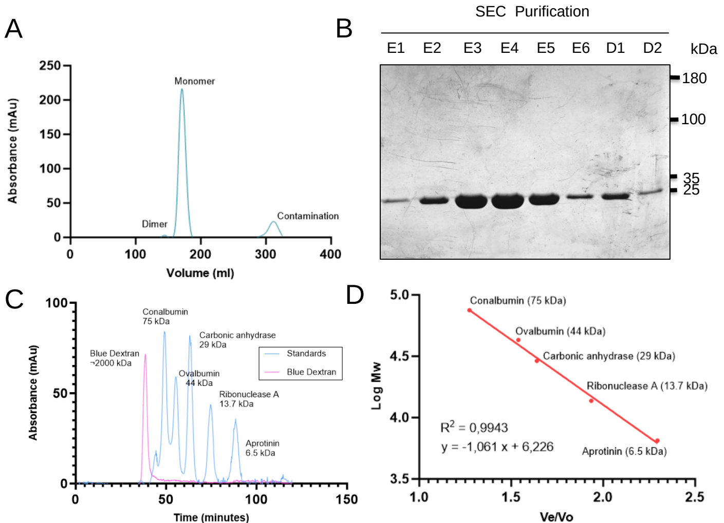
Figure 27: Purification and Purity of TBR1 T-box domain using SEC. A: The elution profile of the TBR1 T-box domain displays the sequential elution of the protein dimer, monomeric form of the protein, and lastly, some residual contamination. B: A 12.5% glycine SDS-PAGE gel, conducted under reducing conditions, exhibits the eluted fractions obtained from the purification process. E1-E6 corresponds to the elutions of TBR1 T-box domain collected in its monomeric form, while D1-D2 represents the eluted fractions collected in its dimeric form. Molecular weight markers are displayed on the right side of the gel (kDa). C: A standard curve for the TBR1 T-box domain is constructed based on the observed molecular weight marker bands on the SDS-PAGE Gel. The equation y = -1.275x + 2.225 is utilised, estimating the molecular weight of the TBR1 T-box domain monomer to be approximately 25.2 kDa. D: A set of GE Healthcare gel filtration standards is subjected to separation on the HiLoad™ 26/600 Superdex™ 75 prep-grade column. Blue dextran, with an exceptionally high molecular weight of approximately 2000 kDa, is run separately from the TBR1 standards. The TBR1 standards include Conalbumin (75 kDa), Ovalbumin (44 kDa), Carbonic anhydrase (29 kDa), Ribonuclease A (13.7 kDa), and Aprotinin (6.5 kDa). E: The standard curve generated from the SEC standards data results in a linear relationship with the equation y = -1.061x + 6.2263 . Utilising
