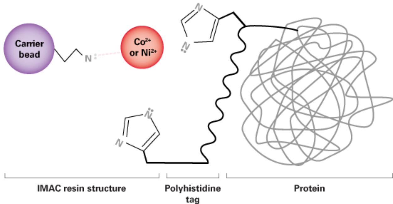
Figure 10: IMAC Resin Structure and Protein Purification Process. The diagram depicts the structure of an Immobilised Metal Affinity Chromatography (IMAC) resin containing cobalt ( \text{Co}^{2+} ) or nickel ( \text{Ni}^{2+} ) ions (red circle) and its interaction with a polyhistidine (His-tag) tag on a protein during the purification process. Each chelated ion has the ability to establish two hydrogen bonds with the nitrogen atoms in the imidazole side chain. Elution of the target protein is achieved by adjusting conditions such as imidazole concentration to disrupt the His-tag and metal ion interaction, releasing the purified protein from the column (Bornhorst and Falke., 2000).
