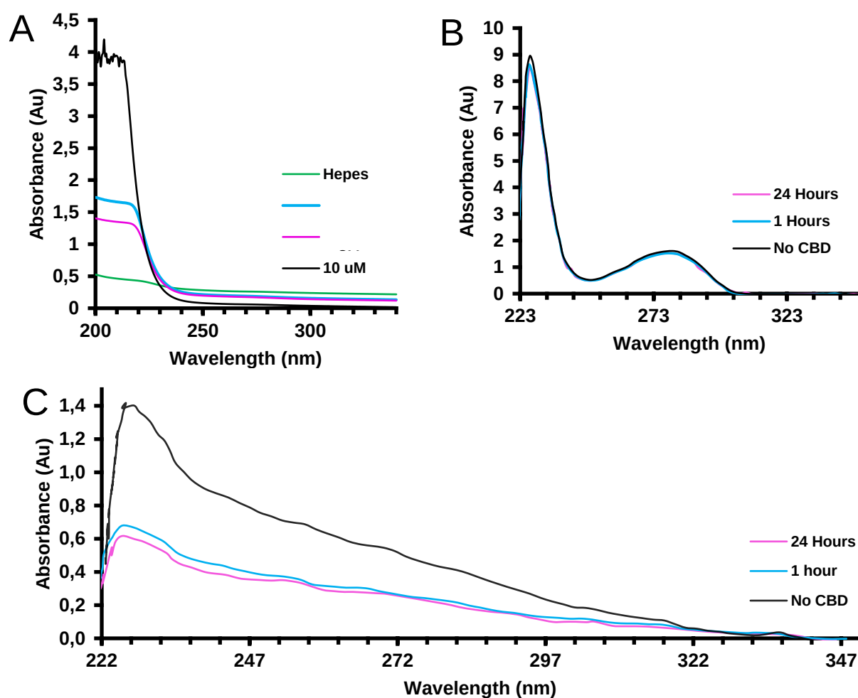
Figure 29: Absorbance Spectrum of CBD and Results of the PDA with TBR1 T-box Domain at 1 Hour and 24 Hours. A: Absorbance spectrum of 1 mg/mL CBD in methanol, diluted to 10 \mu\text{M} (black), 5 \mu\text{M} (blue) and 2.5 \mu\text{M} (pink) using HEPES buffer (0.2 M NaCl and 20 mM HEPES, pH 7.5). The spectrum was measured using a JASCO V-630 Spectrophotometer, showing absorbance (Au) plotted against wavelength
