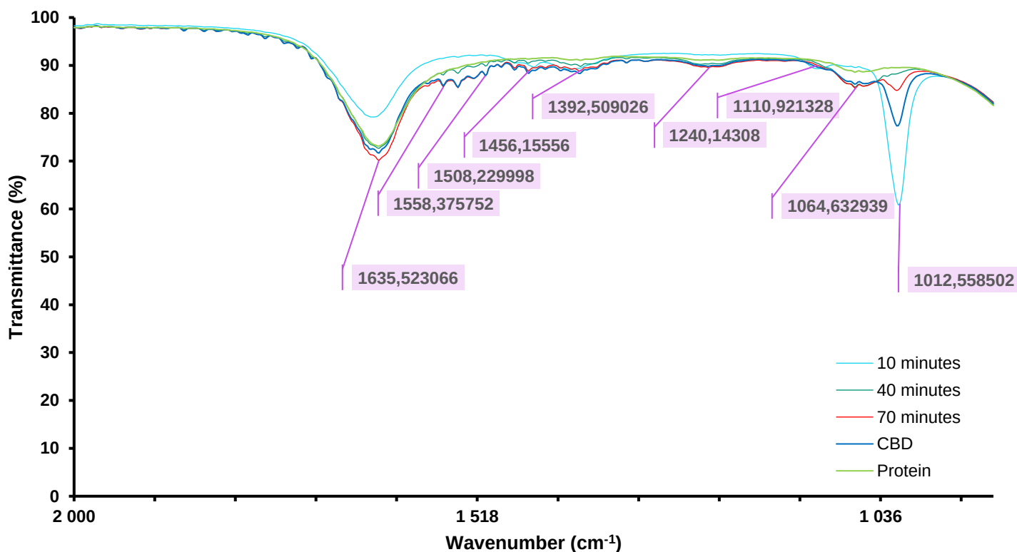
Figure 33: Time-resolved FTIR spectrum of the Interaction between CBD and TBR1 T-box Domain in the Amide region. This figure illustrates the dynamic changes observed in the Amide I, Amide II, and Amide III regions of the FTIR spectrum during the incubation of TBR1 T-box domain with CBD over varying time intervals. Notably, the Amide I band at 1635.52 \text{cm}^{-1} exhibits increasing absorbance with extended incubation. In the Amide II region, multiple bands at 1558.37, 1508.23, and 1456.16 \text{cm}^{-1} show escalating absorbance levels with incubation time, while the Amide III region displays a broad band at 1240.12 \text{cm}^{-1} . The interactions and changes in absorbance in these spectral regions offer valuable insights into the binding dynamics between CBD and the TBR1 T-box domain. These graphs were constructed using MS Excel.
