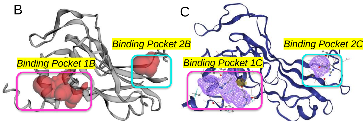
Figure 19: TBR1 T-box Domain Binding Pocket Prediction. A: Amino acid sequence of TBR1 T-box domain showing the secondary structure elements. Purple: 3_{10} helices. Pink: \pi -helix. Blue: turn. Green: bend. Grey: coil. Black: no structure and yellow: \beta -pleated sheets. The residues highlighted in light blue are key residues within the binding cavity. B: Predicted binding pockets by CASTP3.0 indicated in red, based on spatial geometric measurements such as area and volume. Pink square: largest binding pocket (labelled as Binding Pocket 1B) with an area of 212.038 \text{ \AA}^2 and volume of 91.819 \text{ \AA}^3 . Blue square: smaller binding pocket (labelled as Binding Pocket 2B) with an area of 71.645 \text{ \AA}^2 and a volume of 37.121 \text{ \AA}^3 . Any other predicted binding pockets occupied a volume of less than 8.950 \text{ \AA}^3 . C: Predicted binding pockets by ProteinsPlus indicated in purple, based on a combination of Protoss, DoGSiteScorer, and Geomine. This approach considers concavity, shape complementarity and hydrophobicity. Pink square: largest binding pocket (labelled as Binding Pocket 1C) with an area of 676.29 \text{ \AA}^2 , volume of 260.10 \text{ \AA}^3 and hydrophobicity of 0.74. Blue square: smaller binding pocket (labelled as Binding Pocket 2C) with an area of 287.08 \text{ \AA}^2 , a volume of 57.34 \text{ \AA}^3 and a hydrophobicity of 0.68. The larger binding pocket in both (pink) is located between \alpha 3 helix and the 3_{10}C -helix of the T-box domain, which is known to directly interact with DNA, whereas the smaller binding pocket (blue) is located near the e' beta pleated sheet, far from direct DNA binding regions (Tian et al. , 2018; Schöning-Stierand et al. , 2022).
