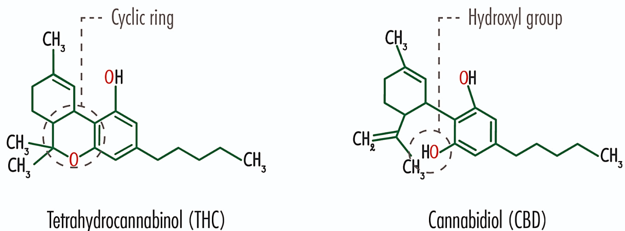
Figure 3: Chemical Structure of CBD and THC: (A): Structure of \Delta -9-THC. (B): Structure of CBD. CBD and THC share identical molecular formulas, denoted as C_{21}H_{30}O_2 . Despite having the same molecular formula, THC contains a cyclic ring which is key to its psychoactive effects. Additionally, their molecular weights are nearly indistinguishable, with THC possessing a mass of approximately 314.469 g/mol and CBD having a slightly lesser mass of around 314.464 g/mol. Image sourced from Hanuš et al. , (2005).
