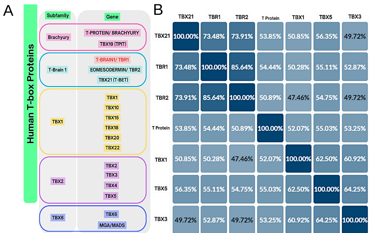
Figure 5: T-box Family Tree and Identity Matrix. A: The T-box protein superfamily in humans. The specific focus of this work, TBR1 (or T-Brain1), is highlighted in red and forms part of the T-Brain 1 subfamily. Other members of the Human T-box protein superfamily include Brachyury (in pink), TBX1 (in yellow), TBX2 (in light purple) and TBX6 (in dark purple). B: As TBR1 is a part of the T-Brain 1 subfamily, a percentage matrix of a multiple sequence alignment (UniProt Align) of the T-box domain is presented, showcasing its comparison with other members within this subfamily, such as TBR2 and TBX21. TBR1 is also contrasted with all other T-box proteins possessing crystallographically resolved structures, including TBXT (Brachyury), TBX1, TBX5, and TBX3, with all sequences sourced from Homo sapiens. TBR1 exhibits the highest similarity to TBR2 (EOMES) at 85.64%, followed by TBX21 at 73.48%, TBXT at 54.44%, TBX1 at 50.28%, TBX5 at 55.11%, and TBX3 at 52.87% (UniProt, 2023).
