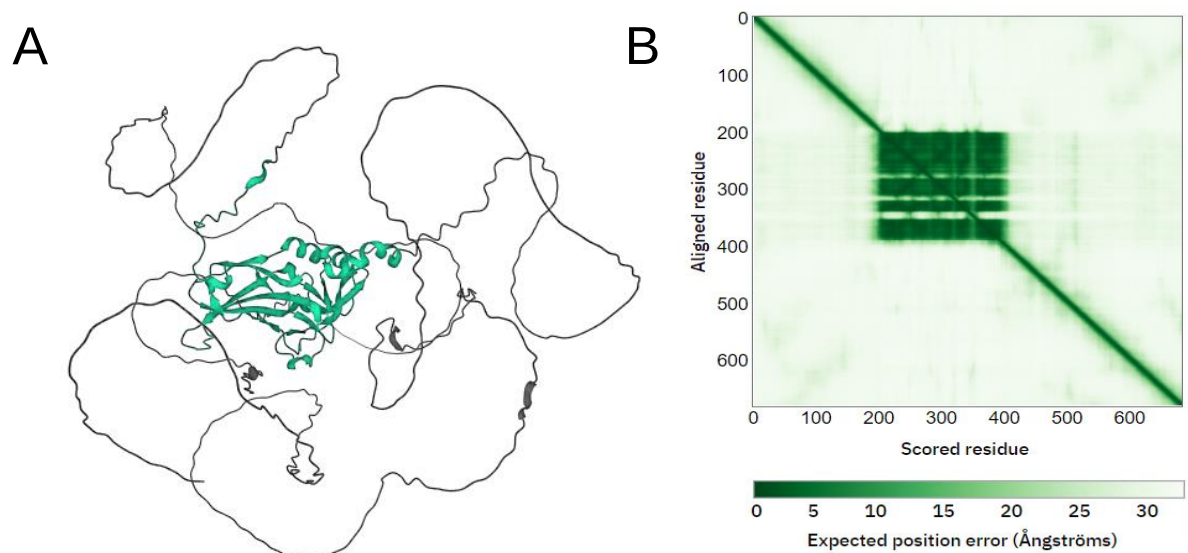
Figure 17: AlphaFold Predicted Structure of TBR1 T-box Domain. A: AlphaFold predicted structure of TBR1, with the T-box domain isolated in green. The Tbox domain is represented as having a very high confidence level (pLDDT > 90%) as shown by (B). B: Predicted aligned error (PAE) which assesses the reliability of the relative positioning and orientations of various domains within the predicted structure, offering insights into the confidence level in these aspects (Jumper et al. , 2021).
