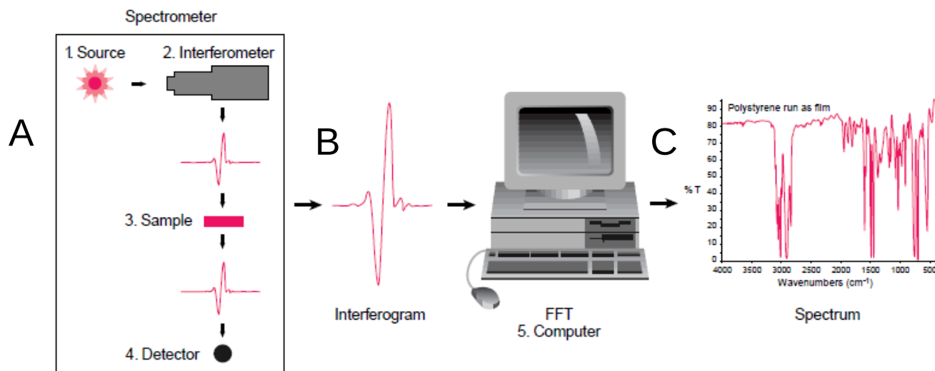
Figure 15: The fundamental principle underpinning Fourier Transform Infrared (FT-IR) spectroscopy. A: FT-IR leverages an interferometer—an optical device that bifurcates the incoming infrared beam into two optical beams. One of these beams reflects off a fixed mirror, while the other bounces off a movable mirror, capable of minute displacements from the beam splitter. B: As these two beams reconverge, they undergo interference, generating an interferogram. This unique signal encapsulates all the infrared frequencies originating from the source. Direct interpretation of this interferogram for sample analysis is not feasible. C: A computer executes a Fourier transformation, unmasking a comprehensive spectrum of intensity values at each frequency. Image sourced from Thermo Nicolet (Hasegawa., 2017).
