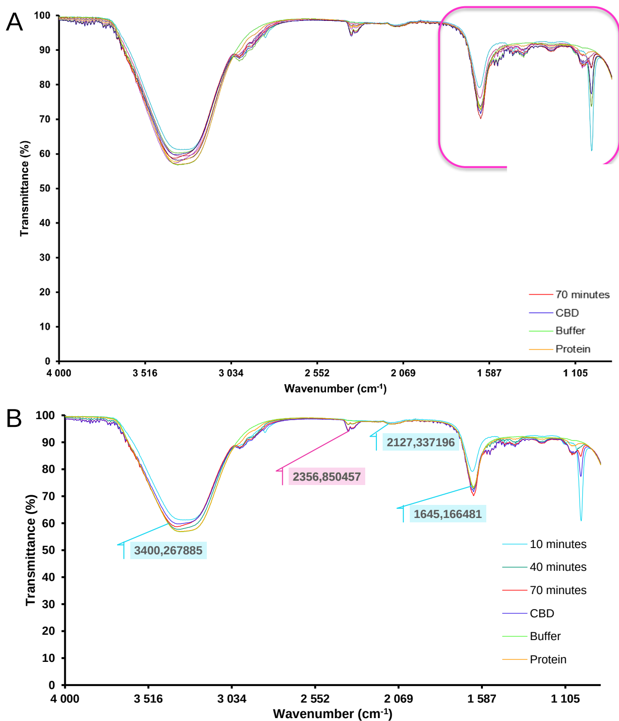
Figure 32: Time-resolved FTIR Spectrum of TBR1 T-box domain and CBD over 70 minutes. A: A solution containing 120 \mu\text{M} of the TBR1 T-box Domain was subjected to incubation with a 1 in 4 dilution of 1 mg/mL CBD in methanol, spanning a duration of 70 minutes. Measurements were acquired at 10-minute
