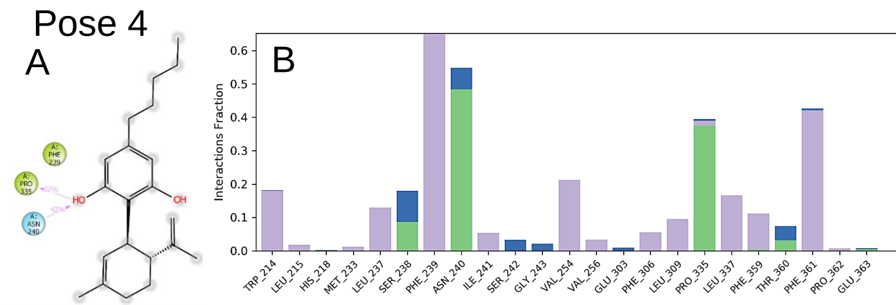
Figure 22: 2D Ligand Interaction Diagrams and Protein-Residue Bonds Distribution Across all Four Poses in 250 ns Simulation. A: The CBD ligand along with its interactions with the protein residues is observed, for the CBD-docked poses 1-4. The protein residues are represented by coloured circles, showing hydrophobic (green), negatively charged (red), and hydrophilic residues (blue). To highlight the significance of these interactions, the percentage of time they persist during the 250 ns simulation is displayed, with interactions exceeding 30% of the simulation time indicated in purple – representing hydrogen bonding. B: All the ligand-interacting protein residues with their respective bond distributions, including hydrogen bonds (green), hydrophobic interactions (purple), ionic bonds (pink) and water bridges (blue). Images and graphs generated using Maestro Schrödinger.
