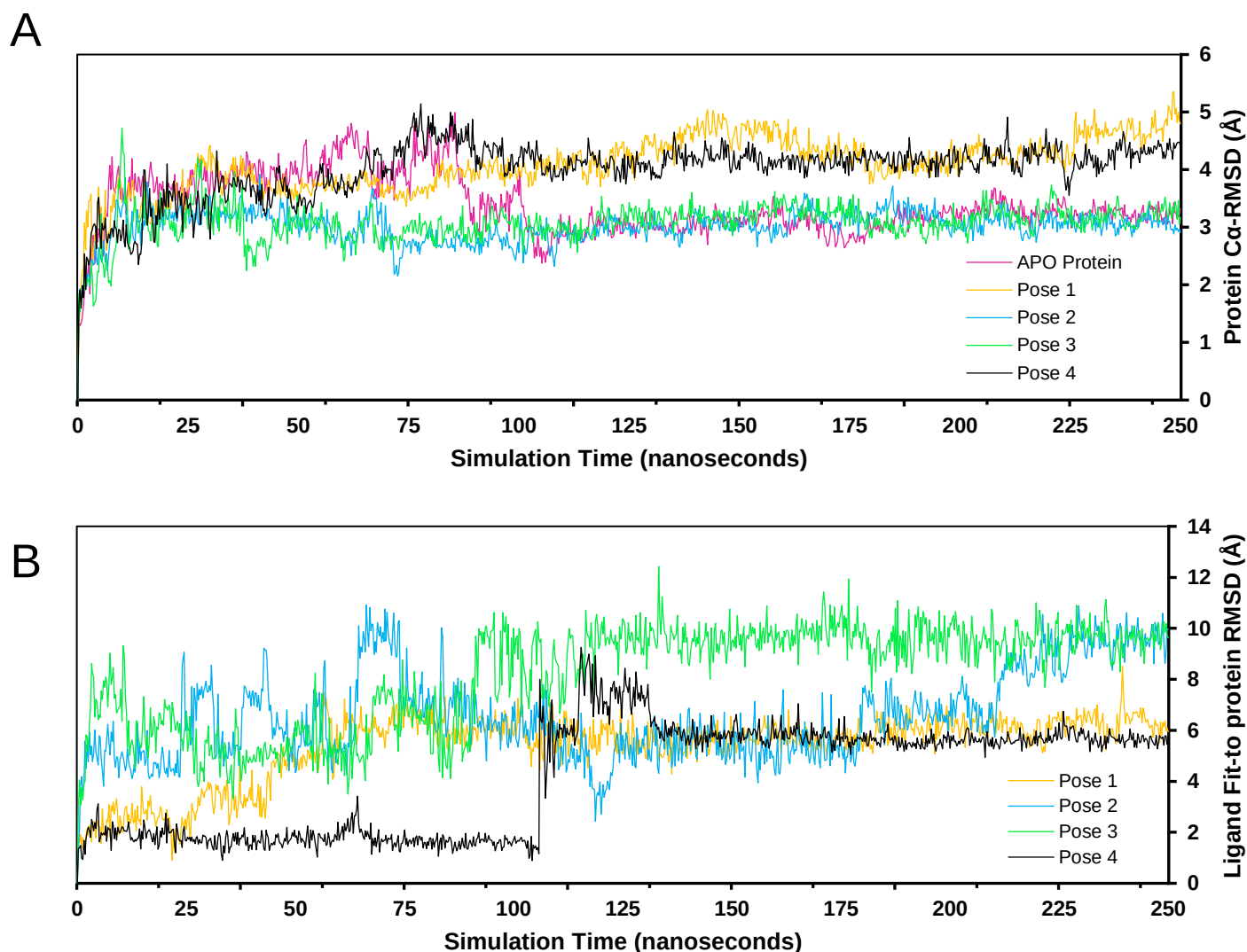
Figure 21: Protein C \alpha and LP-RMSD Plots for TBR1 T-box domain and CBD for the APO and CBD-docked TBR1 T-box domain systems. A: Protein backbone C \alpha -RMSD calculated for the APO protein (pink), CBD-docked Pose 1 (orange), Pose 2 (blue), Pose 3 (green) and Pose 4 (black) showing the average atomic deviation of C \alpha . The AlphaFold predicted structure of TBR1 T-box domain is used as reference. B: LP-RMSD calculated for Pose 1 (orange), Pose 2 (blue), Pose 3 (green) and Pose 4 (black). The CBD reference structure was obtained from PubChem (CID: 644019). Greater RMSD values correspond to greater deviations from the reference structure and conformational changes – reflecting stability of the complex. Graphs were generated using MS Excel and RMSD was calculated using Maestro Schrödinger.
