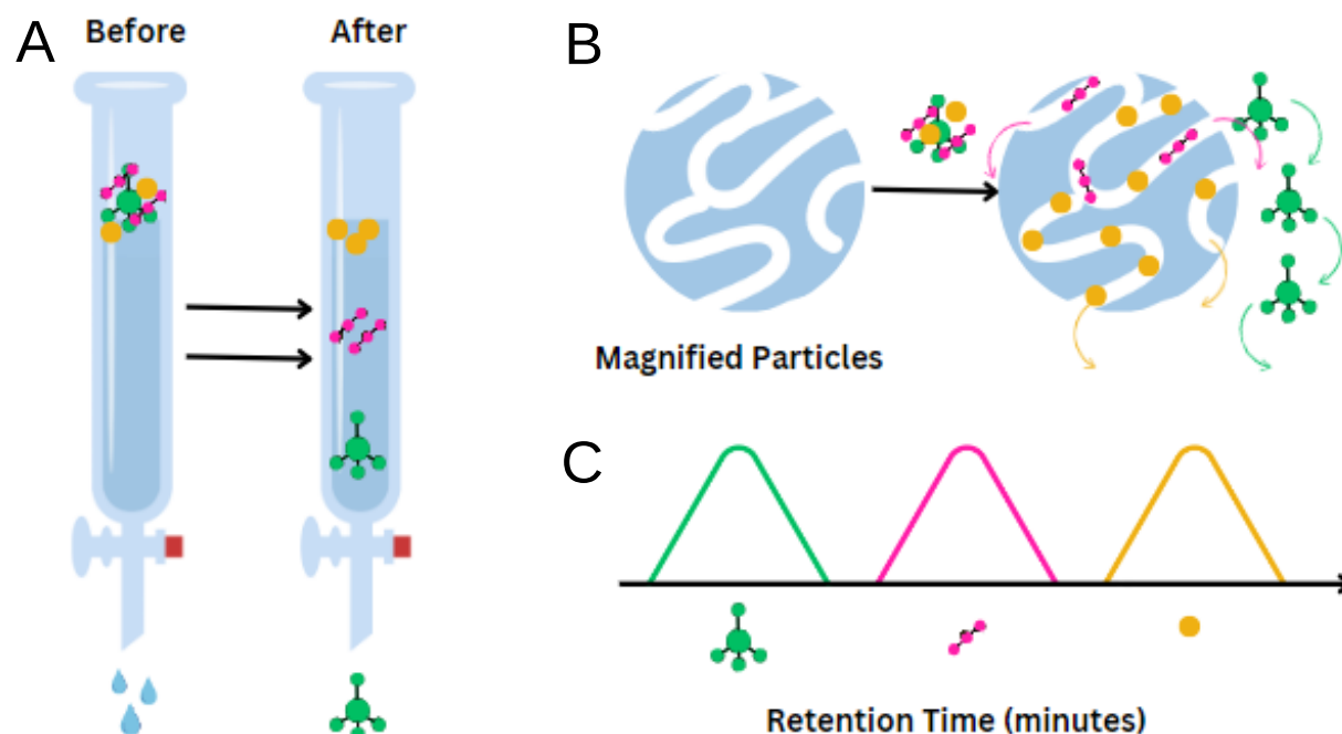
Figure 11: Principle for Size Exclusion Chromatography (SEC). A: As the solution traverses the column's stationary phase, predominantly comprised of beads, molecules undergo separation based on their Stokes radius. B: Larger molecules (green) are eluted first as they struggle to penetrate the porous matrix. In contrast, smaller molecules (orange) enter the pores, experiencing delayed elution due to their slower movement. C: Molecules of varying sizes exhibit distinct retention times, eluting according to their size (from large to small: Green, pink and orange). Those not interacting with the matrix are classified within the void volume, sharing an elution rate with the buffer. The image was created using Canva. (Carmack and Kelley., 1968; Sherman., 1999)
