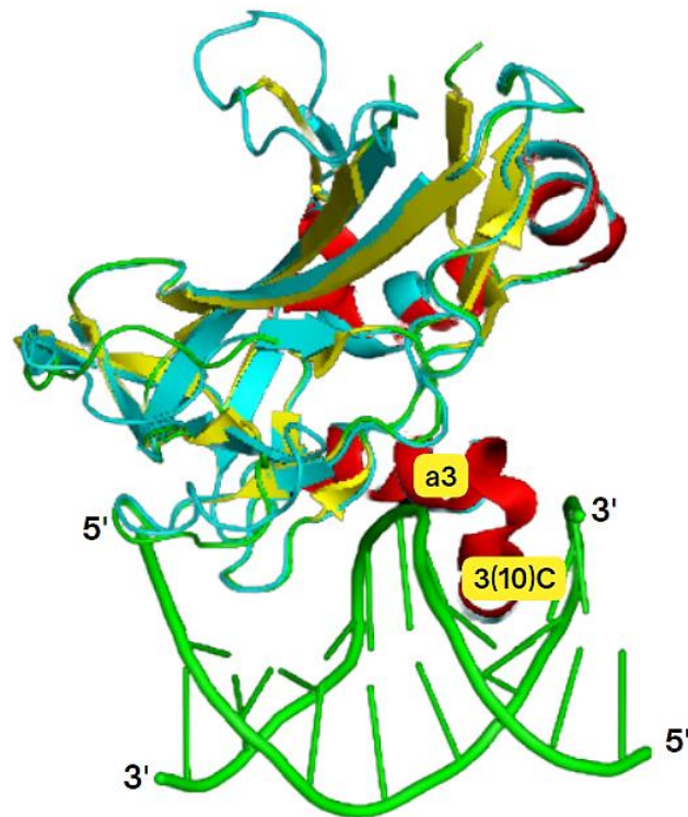
Figure 6: TBR1 T-box Domain Structure Comparison with TBX5. Structure alignment between the DNA binding domain of TBR1 in blue (UniProt ID: Q16650) and TBX5 in green (UniProt ID: Q99593) interacting with DNA (from the crystallised structure of TBX5 interacting with DNA). \beta -pleated sheets and \beta -barrels are shown as arrows. \alpha -helix structures are shown in red. \alpha 3 and 3_{10}C helices (yellow) are both directly interacting with the DNA (green) and present in both TBR1 and TBX5. Image generated using PyMOL MatchAlign (PyMOL Molecular Graphics System, Version 1.7 Schrödinger, LLC).
