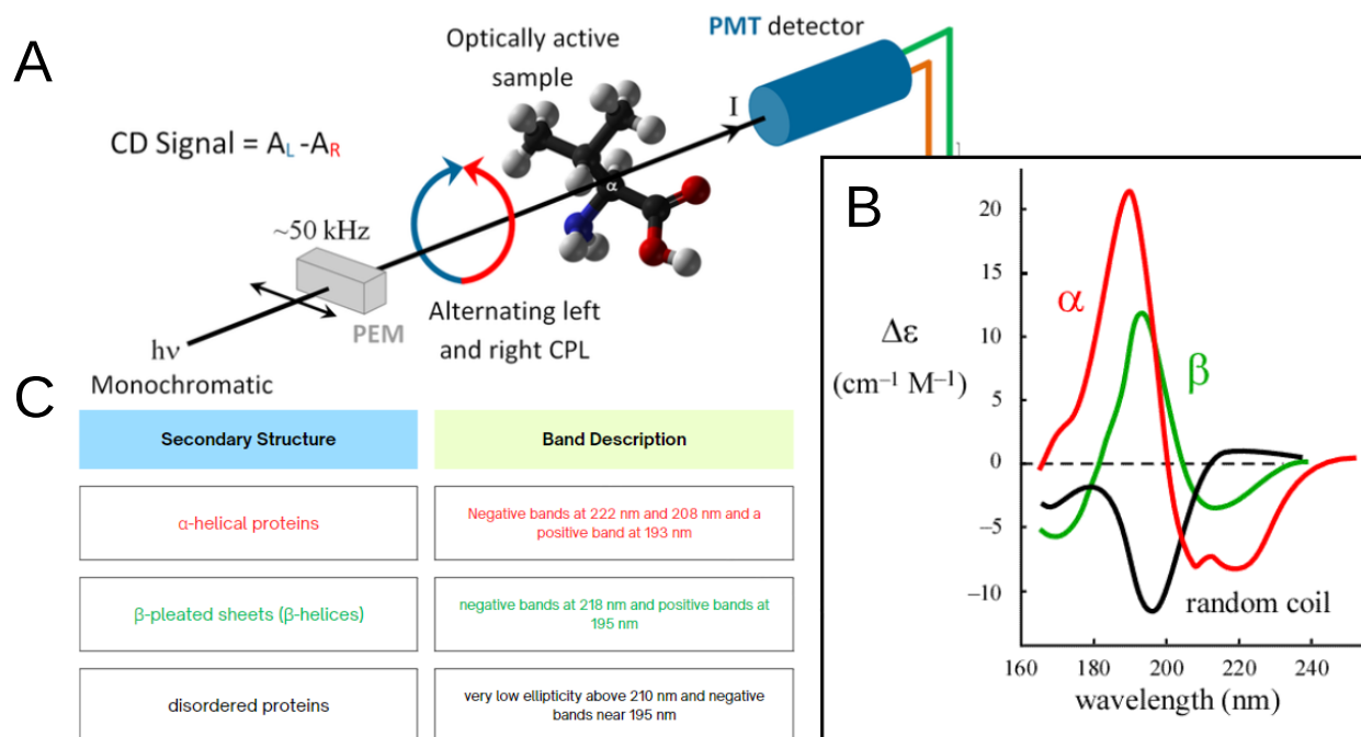
Figure 12: Principle of Far-UV CD. A: Linearly polarised light traverses a Photo Elastic Modulator (PEM), where it undergoes a transformation into alternating left and right circularly polarised light (CPL). This CPL comprises oscillating electric and magnetic fields, both rotating around the direction of propagation, thus forming sinusoidal wave patterns. The light is differently absorbed and detected by a Photo Multiplier Tube (PMT). Chiral molecules, including proteins, exhibit the capability to absorb this rotating light, a property that forms the basis for CD spectroscopy. B: CD spectra provide distinct signatures for various secondary structural elements of proteins, C: such as alpha helices (bands at 222 nm, 208 nm and 193 nm), beta sheets (bands at 218 nm and 195 nm), and random coils/ disordered proteins (bands at 210 nm and 195 nm). These spectral patterns offer a means to identify the presence and relative abundance of secondary structural motifs within the protein. Image created using Canva (Kelly et al. , 2005).
