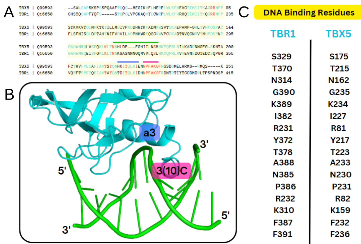
Figure 18:: Sequence and Structure Alignment between the T-box domains of TBR1 and TBX5. A: Sequence Alignment between the complete TBR1 (UniProt ID: Q16650) and TBX5 (UniProt ID: Q99593), where (A) shows only the region of interest – the T-box DNA binding domain. This domain is highlighted in yellow. Similar residues are shown in light blue, whereas the DNA interacting residues of TBX5 and the corresponding residues of TBR1 is shown in red. The structural alignment was performed using Clustal Omega. B: Structure alignment between the DNA binding domain of TBR1 (blue) interacting with DNA (from the crystallised structure of TBX5 interacting with DNA PDB: 2X6V) where only the \alpha 3 (purple) and 3_{10}C helices are present and predicted to interact with DNA. The structure alignment was performed using MatchAlign in PyMOL Molecular Graphics System, Version 2.5 Schrödinger, LCC. C: DNA binding residues of TBX5 and the corresponding TBR1 residues, as predicted from the sequence alignment (UniProt., 2023)
