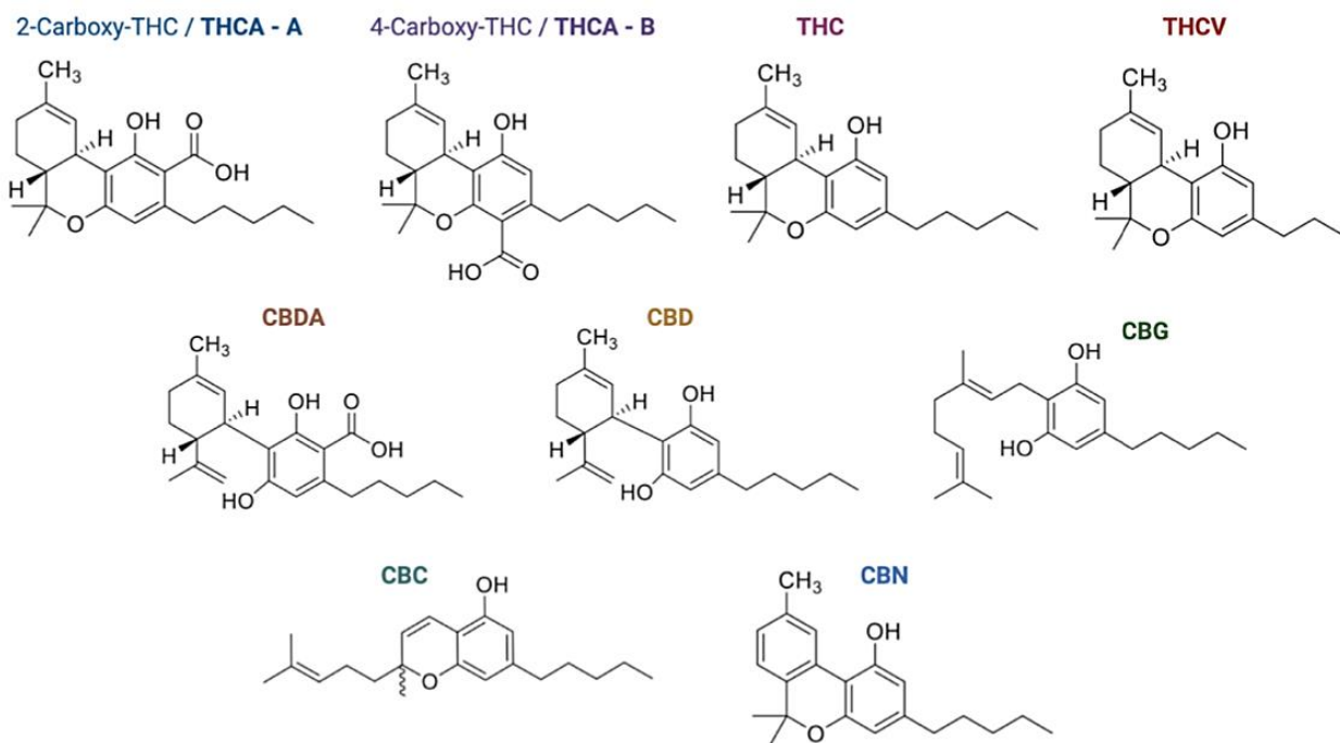
Figure 2: The Chemical Structure of the Main Phytocannabinoids found in Cannabis sativa . L. \Delta^9 -tetrahydrocannabinol ( \Delta^9 -THC), more commonly known as THC, has two acidic counterparts – THCA-A and THCA-B is shown, alongside Tetrahydrocannabivarin (THCV). Cannabidiol (CBD) can be seen alongside its acidic counterpart CBD acid (CBDA), together with cannabigerol (CBG), cannabichromene (CBC) and cannabinol (CBN). Adapted from (Tahir et al. , 2021).
