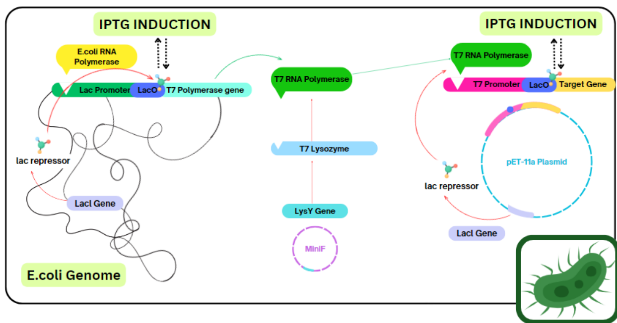
Figure 9: pET11-a Plasmid Expression System in T7 E.coli Cells. This figure illustrates the key regulatory elements within the T7 E.coli genome. Central to this regulation is the LacI gene, encoding the Lac Repressor, which binds to the lac promoter, preventing transcription of the T7 RNA polymerase gene by E. coli RNA polymerase. Introduction of IPTG disrupts this interaction, releasing the inhibition and enabling transcription of T7 RNA polymerase. Graphic created using Canva. (New England BioLab C3010I Datasheet).
