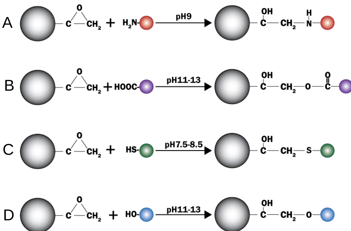
Figure 13: Epoxy Activated Agarose Pull-Down Assay: Epoxide-activated agarose is characterised by a dense distribution of epoxide groups, which engage in a ring-opening mechanism when encountering nucleophiles. These epoxide moieties readily undergo reactions with (A) primary amines, (B) carboxylic acids, (C) thiols and (D) hydroxyl groups, resulting in the formation of stable (A and B) secondary amide, (C) thioester and (D) ether linkages, respectively. Notably, thiol groups particularly favour these reactions, requiring a buffered system near physiological pH (pH 7.5-8.5). In contrast, epoxide groups necessitate elevated pH conditions to react with hydroxyl groups (pH 11-13) and moderately alkaline conditions for engaging amine groups (pH 9).
