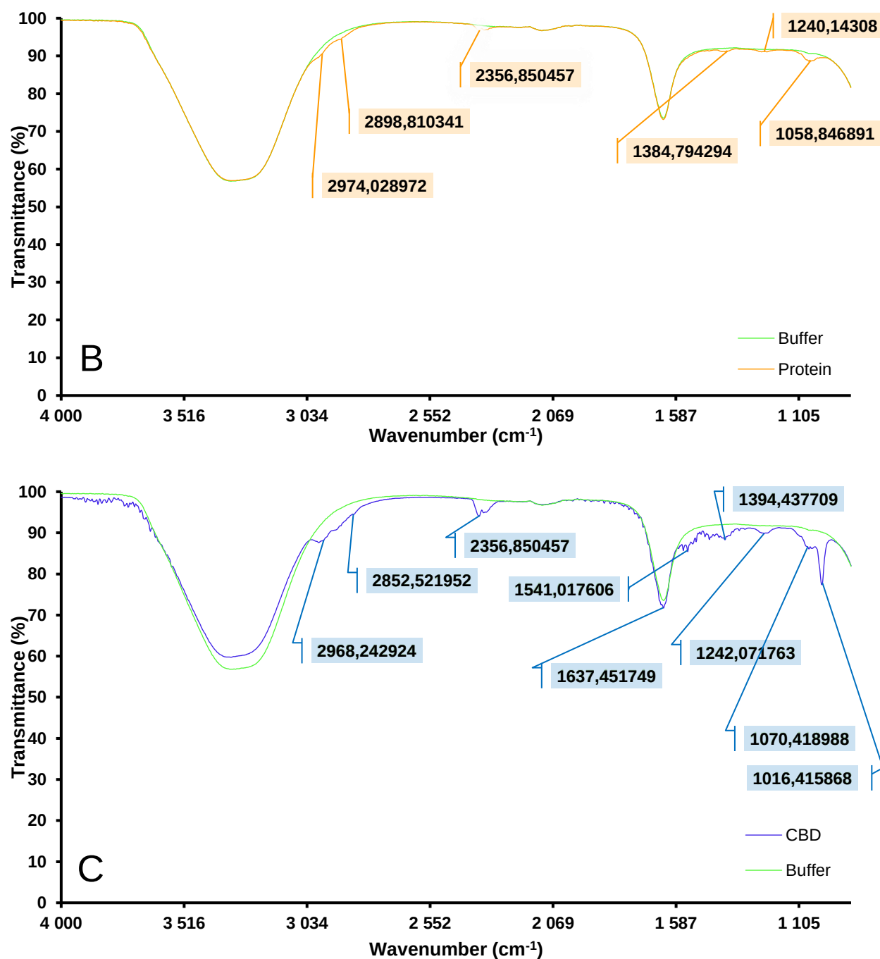
Figure 31: FTIR Spectra of Equilibration Buffer, CBD and TBR1 T-box Domain Controls. A: The green FTIR spectrum of equilibration buffer (30 mM imidazole, 500 mM NaCl and 20 mM Tris). Strong and broad bands observed between 3373.27 and 3242.12 cm -1 , a medium peak at 1637.45 cm -1 and a small band at 2111.91 cm -1 . B: Comparison FTIR spectra of equilibration buffer (green) and TBR1 T-box domain in equilibration buffer (orange). Peaks are observed at 2974.03 cm -1 , 2898.81 cm -1 , 2356.85 cm -1 , 1384.79 cm -1 , 1240.14 cm -1 and 1058.84 cm -1 . C: Comparison FTIR spectrum of a 1 in 4 dilution of CBD (1 mg/mL in methanol) in equilibration buffer (dark blue) and equilibration buffer (green). Bands are observed from
