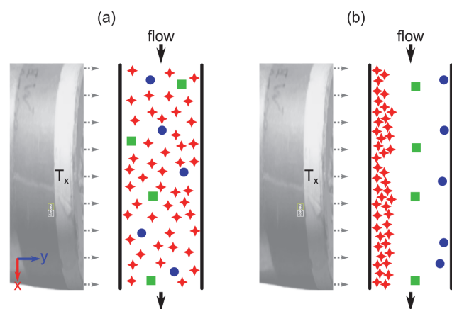
Fig. 1: Schematic top-view representation of ultrasonic cell separation in a capillary before (a) and after (b) sonication with a single-element transducer T_x .
