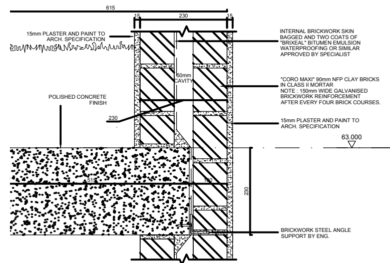
DETAIL A 1:10
