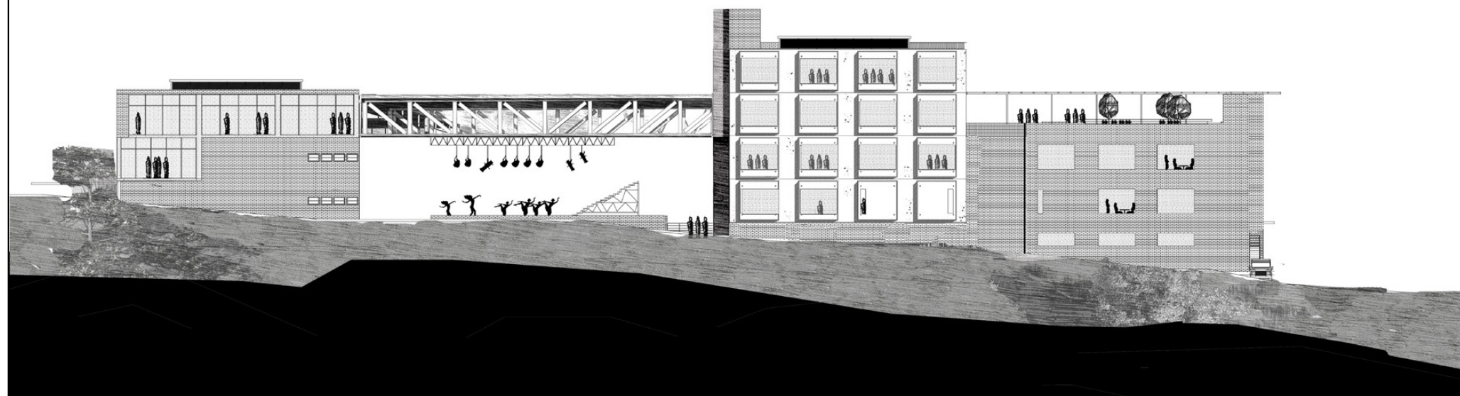
SOUTH ELEVATION NTS
