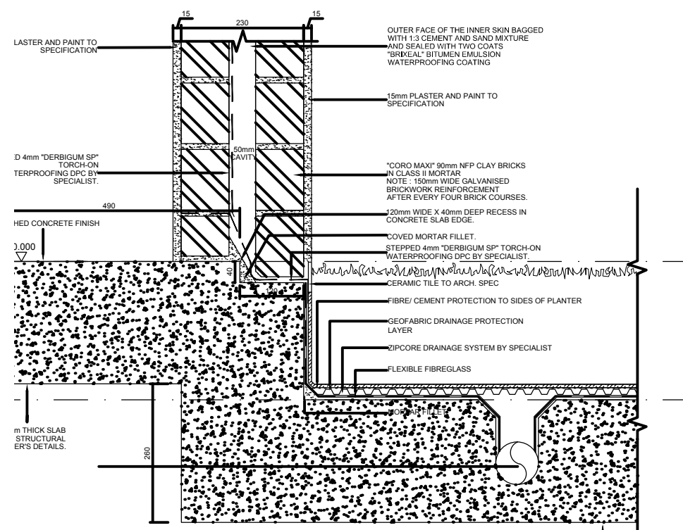
DETAIL C 1:10
