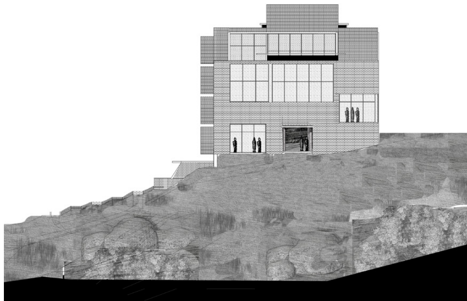
WEST ELEVATION NTS
