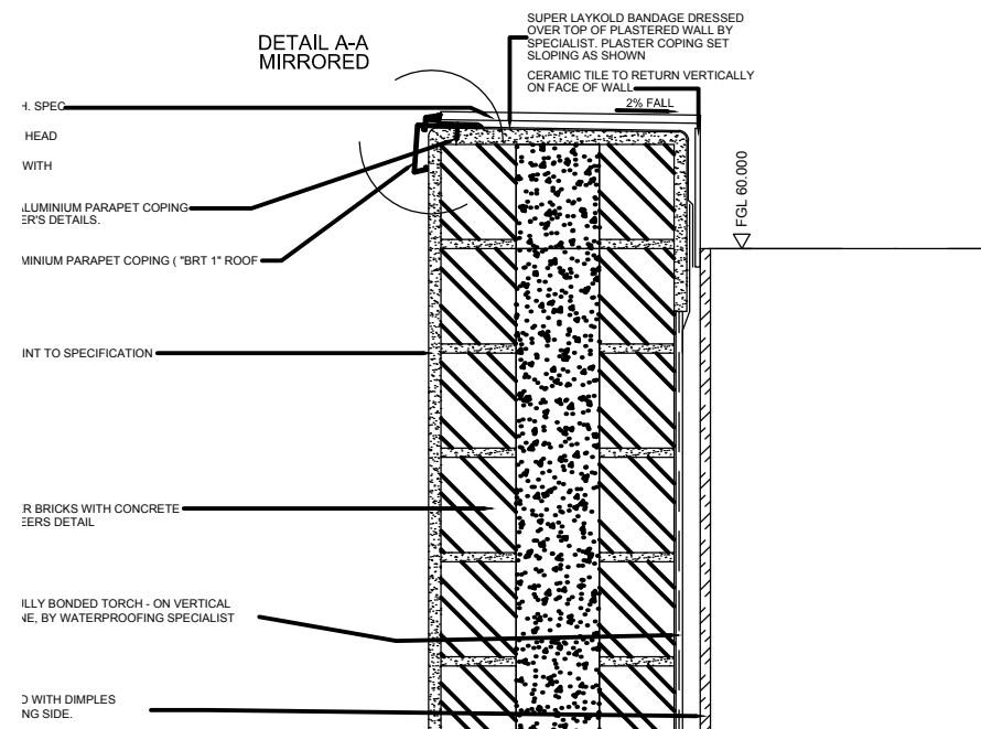
DETAIL B 1:10
