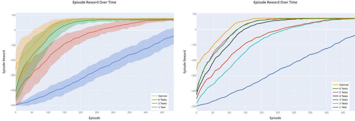
(a) Learning curves after 1, 3 and 6 training tasks, (b) Learning curves for all number of tasks without compared with the optimal option performance confidence intervals for the sake of clarity
