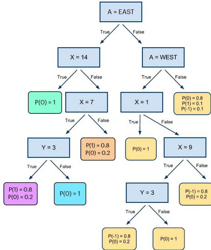
(b) Decision tree model for predicting the change in the X state variable for the domain shown in Figure 2.1a
