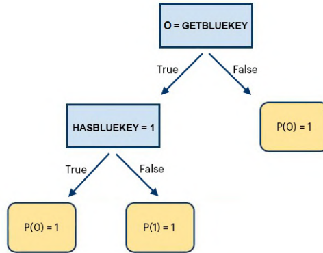
Figure 3.5: Decision tree for the hasBlueKey state variable. The tree is split on options and state variables, shown by the blue rectangles. The leaves provide probabilistic predictions on how the hasBlueKey variable will change.
