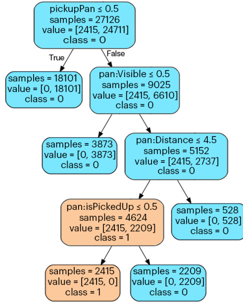
Figure 4.14: Converged decision tree for the pan:isPickedUp state variable.
