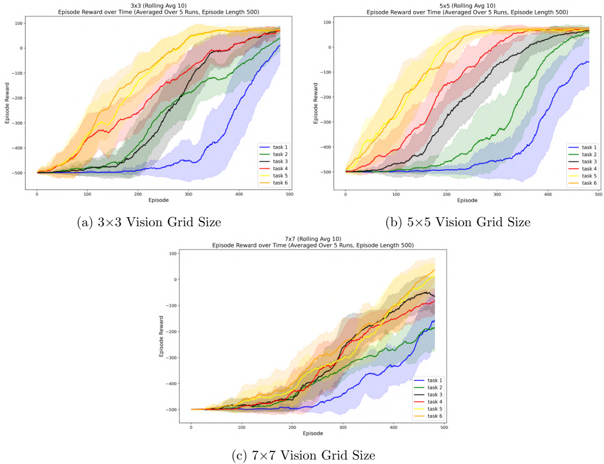
Figure B.1: Comparison of factored option performance for various vision grid sizes.
