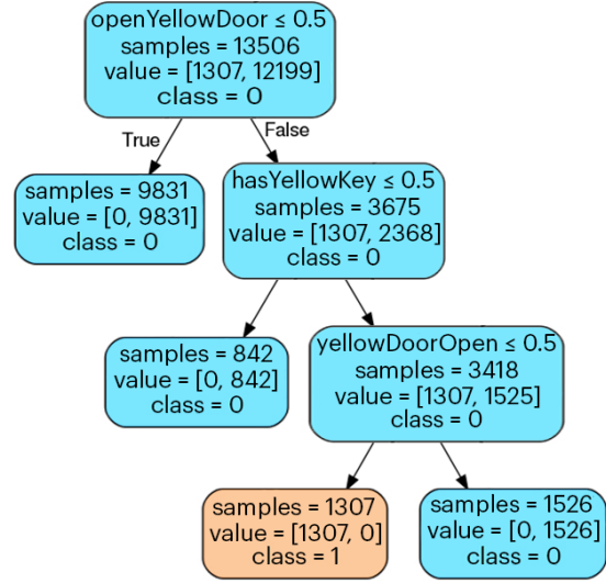
(b) yellowDoorOpen Tree
