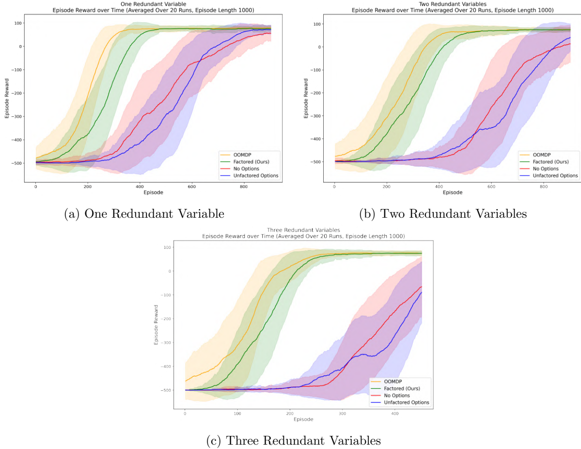
Figure C.1: Comparison average reward per episode for domains with various numbers of redundant variables. Our framework is compared to DOORMAX, no option Q-Learning and unfactored option SMDP Q-Learning. Graphs are plotted using a rolling average with a window size of 20 episodes.
