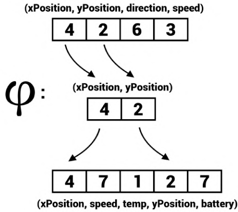
Figure 3.2: Example of how the factored state set is used to generate factored representations, which can then be mapped to new domains. In this example, \phi refers to the set of variables xPosition and yPosition , on which the option depended. Assuming that the top state is an initiation set for the option, the factored option would be able to be initiated in the bottom state as the dependent variables match.
