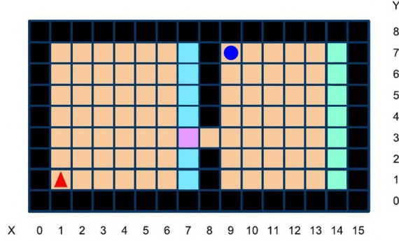
(a) Gridworld domain consisting of two rooms connected by a hallway. Cells are coloured to match the corresponding leaves in the tree below. The red triangle indicates the agent's location and the blue circle indicates the location of a ball object.
