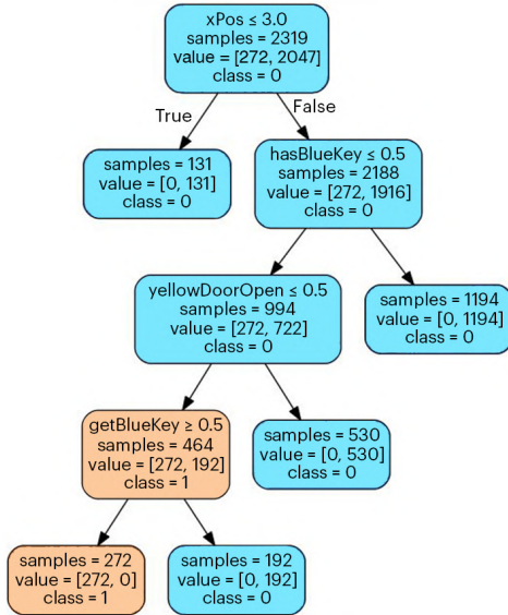
(a) hasBlueKey decision tree model after one training domain (Figure 4.3)
