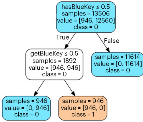
(a) hasBlueKey Tree
