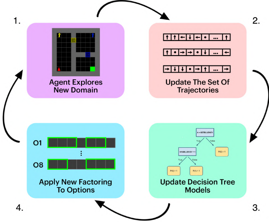
Figure 3.1: Diagram illustrating the framework’s factor learning process. First, the agent explores the domain, attempting to solve the initial task. This generates a set of trajectories which are used as input for the decision tree models of the state variables. From these models factored representations are learned for each option available to the agent. These factored options are then made available to the agent, and it is given a new task to solve. This process continues and the factored representations are refined after each cycle.
