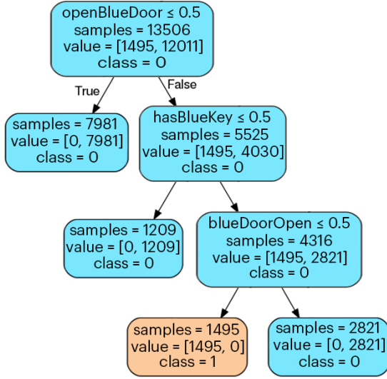
(a) blueDoorOpen Tree
