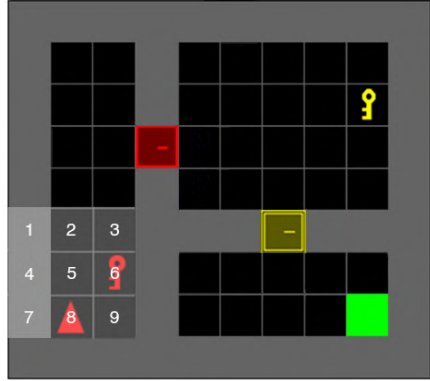
(a) Training domain with a 3 \times 3 local agent view, labelled 1 through 9.
