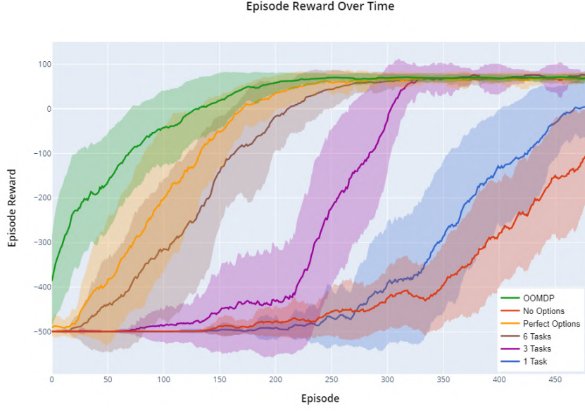
(a) Average reward per episode after 1, 3 and 6 training tasks given to our framework, compared with the optimal option performance. Shaded areas indicate a single standard deviation.
