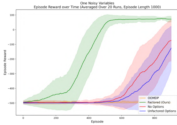
(a) One Noisy Variable
