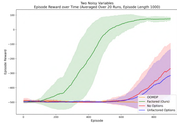
(b) Two Noisy Variables
