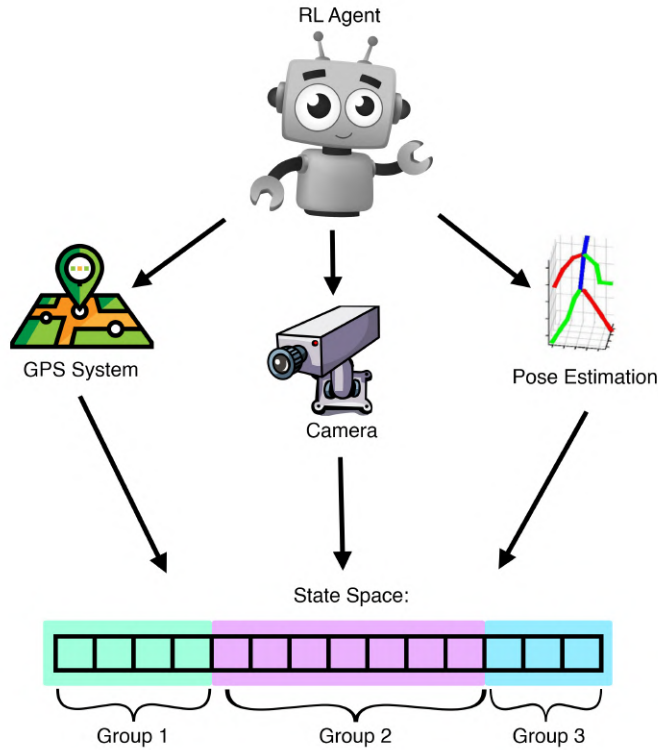
Figure 3.6: Diagram illustrating the application of variable groupings. The agent has information from three different systems: a GPS system providing the agent’s location, a camera showing the agent’s visual observation and a pose estimation system describing the joint angles of the agent. Observations from these three systems are concatenated together to form the entire state space. We aggregate all the individual readings or variables into three separate groups, one for each system.
