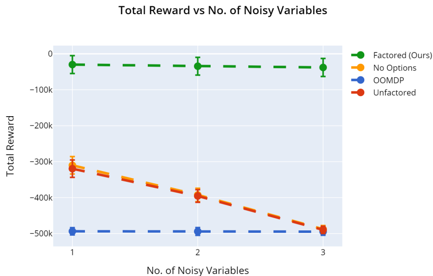
Figure 4.10: Comparison of total reward accumulated for domains containing various numbers of noisy variables. The bars on each point indicate one standard deviation, as each experiment is averaged over 10 random seeds
