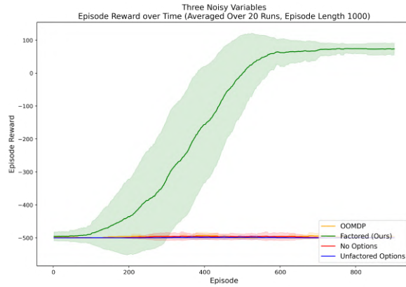
(c) Three Noisy Variables
