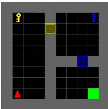
Figure 3.3: Example Minigrid domain, consisting of 3 rooms. Each room is connected by a locked door, which can only be unlocked by using the key corresponding to the door colour. The agent location is indicated by the red triangle and the goal state by the green square.
