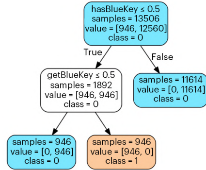
(b) hasBlueKey decision tree model after six training domains
