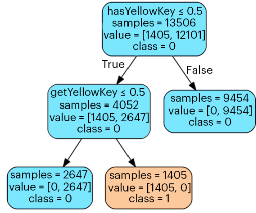
(b) hasYellowKey Tree
