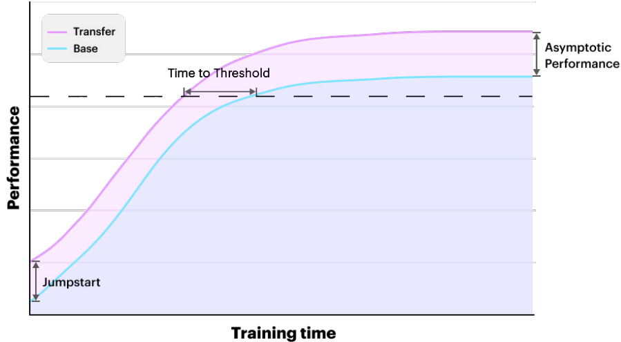
Figure 2.2: Graph depicting the different metrics for evaluating transfer. Jumpstart, asymptotic performance and time to threshold are indicated on the graph, while total reward can be calculated as the area under the learning curves [Taylor and Stone 2009].
