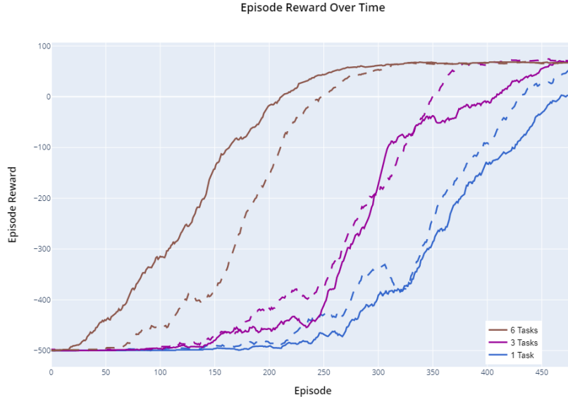
Figure 4.8: Comparison between 1, 3 and 6 training tasks for both grouping methods. The dotted lines show performance of the grouping threshold of 1 item, while the solid lines indicate the grouping threshold of at least half of the items.
