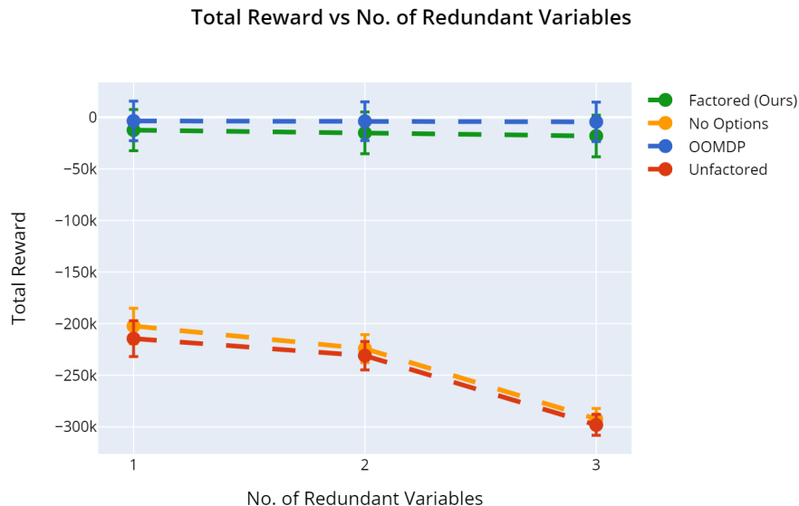
Figure 4.9: Comparison of total reward accumulated by different algorithms for domains containing various numbers of redundant variables. The bars on each point indicate one standard deviation, as each experiment is averaged over 10 random seeds.
