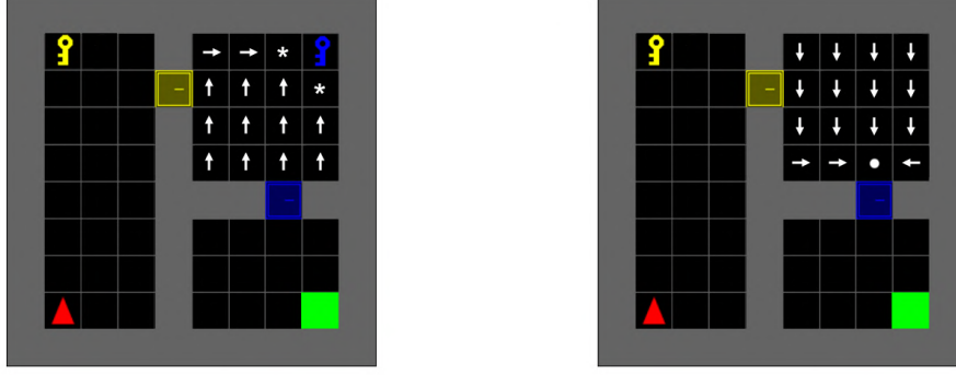
(a) Option policy to collect blue key
