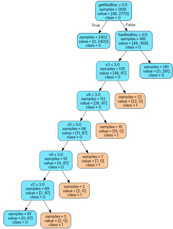
(b) hasRedKey decision tree model learned from training domain shown in Figure 4.5a
