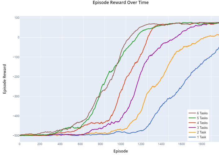
(b) Learning curves for all number of tasks without confidence intervals for the sake of clarity
