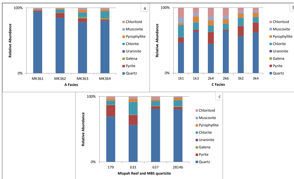
Figure 4.1: Relative mineral abundance in samples representing the Vaal Reef samples. (a) The A Facies at Moab Khotsoeng 370 geozone is dominated by quartz. (b) The C Facies at Kopanang 440 (1k1 and 1k3) and 460 (2k4, 2k6, 3k2 and 3k4) geozones are pyrite-rich and exhibit high sheet silicate abundances. (c) The Mizpah Reef samples are pyrite-rich and the MB5 footwall samples are quartz-rich.
