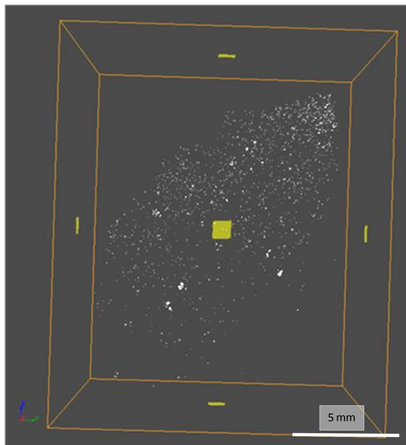
Figure 6.14: 3D visualisation of the distribution of uranium-bearing minerals and gold (both minerals are seen as one component) from sample 3k2. Other mineral components are transparent allowing visualisation of these minerals only.
