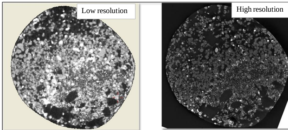
Figure 6.5: Illustration of tomograms of the same sample at different resolutions (low and high resolution). At low resolution, minerals touch one another and contrast is not well defined; at high resolution individual minerals are now distinguished and contrast is well-defined.
