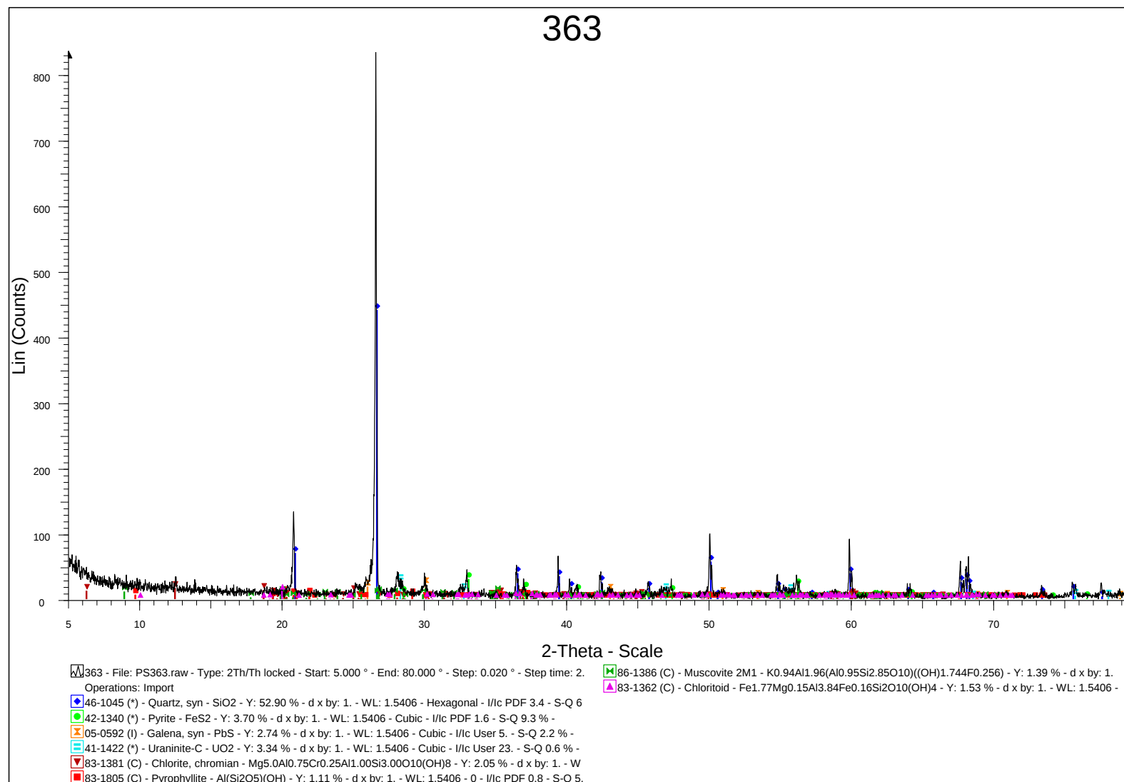
Appendix 18: Diffractogram of sample MK363 from Moab Khotsonq Mine representing the 370 geozone.
