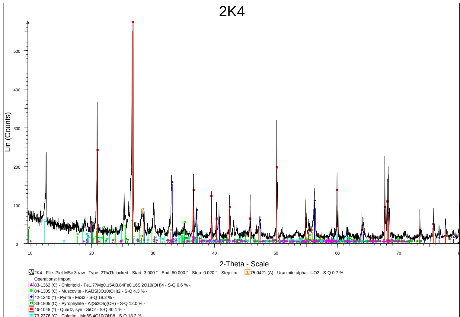
Appendix 22: Diffractogram of sample 2k4 from Kopanang Mine representing the 460 geozone.
