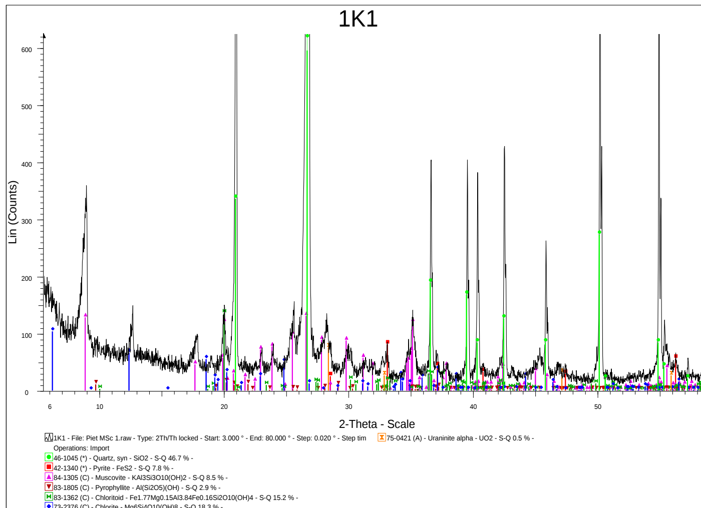
Appendix 20: Diffractogram of sample 1K1 from Kopanang Mine representing the 440 geozone.
