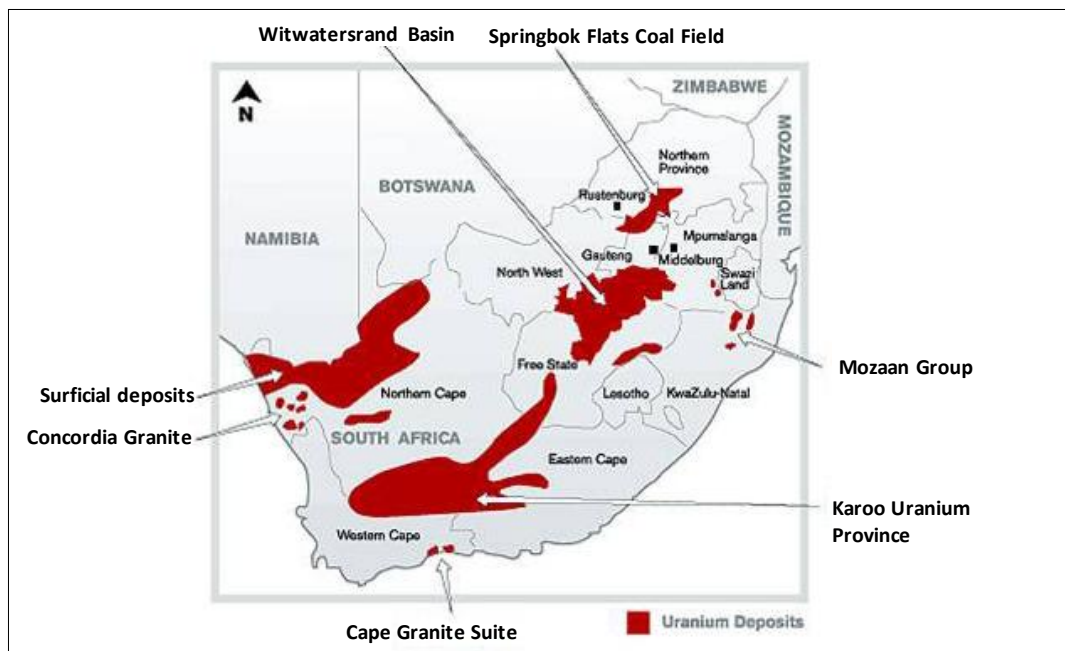
Figure 1.1: Distribution of uranium provinces and deposits in South Africa (after Cole, 1998). The Witwatersrand Basin is the largest uranium deposit followed by the Karoo, marine phosphates, and other surficial deposits.
