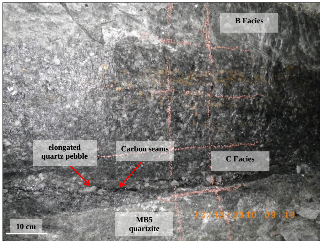
Figure 3.10: The Vaal Reef C Facies at the 440 geozone; the carbon seam is developed at the base of the reef and the quartz clasts are sub-angular and elongated. The reef rests directly on the MB5 quartzite footwall and no Witkop conglomerate was observed.
