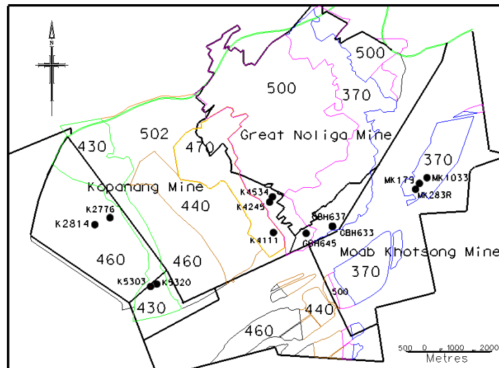
Figure 3.13: Layout of the localities of thirteen drilled boreholes are shown on the map, seven from Kopanang Mine, three from Great Noligwa Mine and three from Moab Khotsoang Mine. The boreholes represent different geozones across the three mines (AngloGold Ashanti internal report, 2001).
