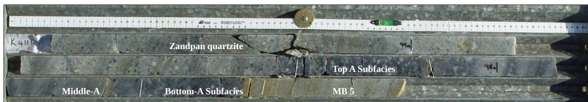
Figure 3.19: Photograph of borehole K4111 intersecting the MB5 quartzite, Bottom A Subfacies, Middle A Subfacies, Top A Subfacies and the Zandpan quartzite.
