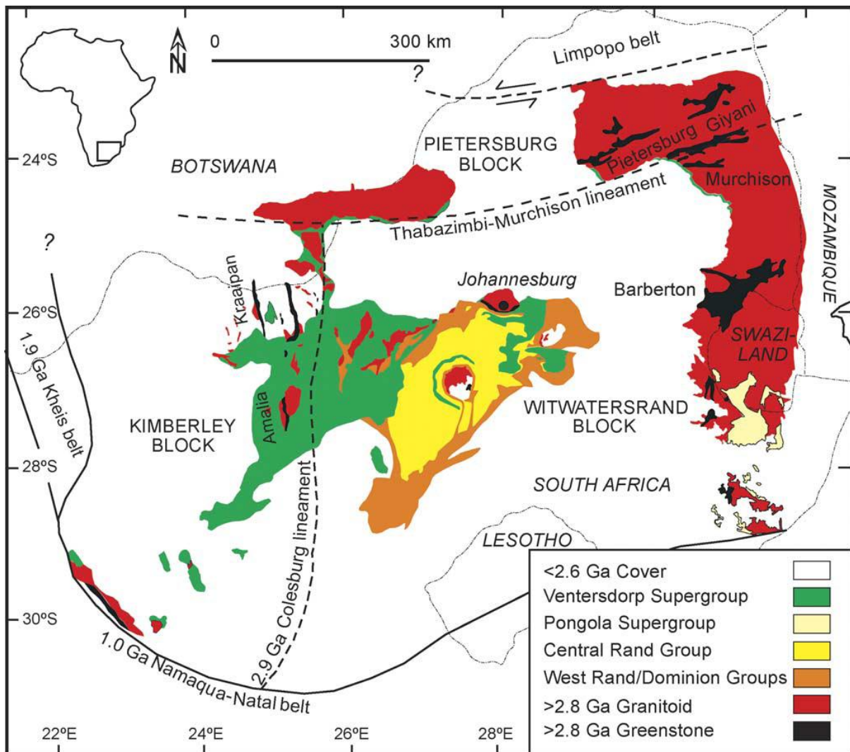
Figure 2.1: The Witwatersrand Supergroup with the West Rand and Central Rand Groups occupying the centre of the three crustal blocks of the Kaapvaal Craton constituted by older granitoids and greenstone formations (after Frimmel, 2005).
