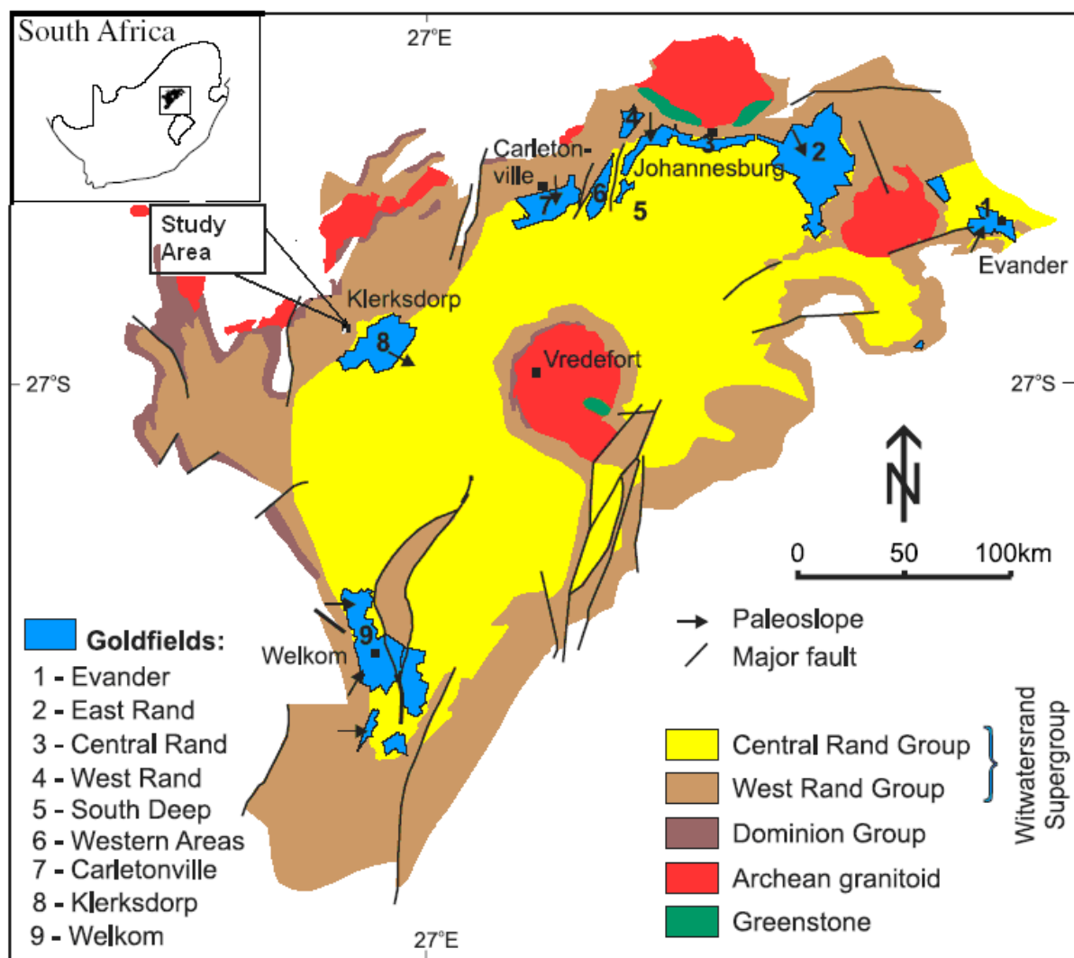
Figure 1.2: Simplified geological map of the Witwatersrand Basin showing the Archaean granitoid domes, the nine major Goldfields, major faults and palaeocurrent directions of reefs in the Central Rand Group (after Frimmel and Minter, 2002).
