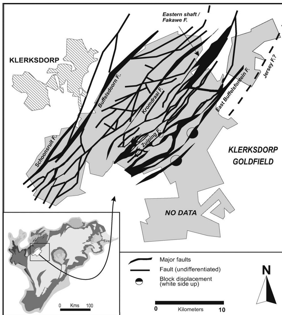
Figure 3.3: Geological map of major structures in the Witwatersrand Supergroup in the Klerksdorp goldfield with the younger cover removed (after Dankert and Hein, 2010).
