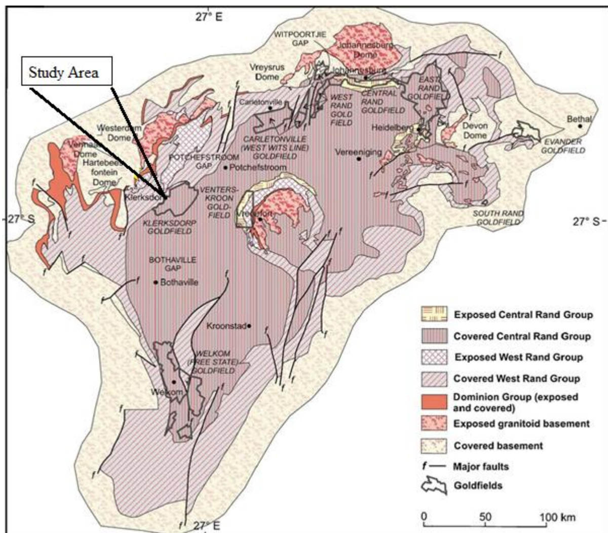
Figure 3.1: Locality map of the Witwatersrand Basin Goldfields, with the Klerksdorp Goldfield in the proximity of Klerksdorp town. The Vaal Reef occurs southwards where the AngloGold Ashanti properties are found (Rantzsch et al. , 2011).
