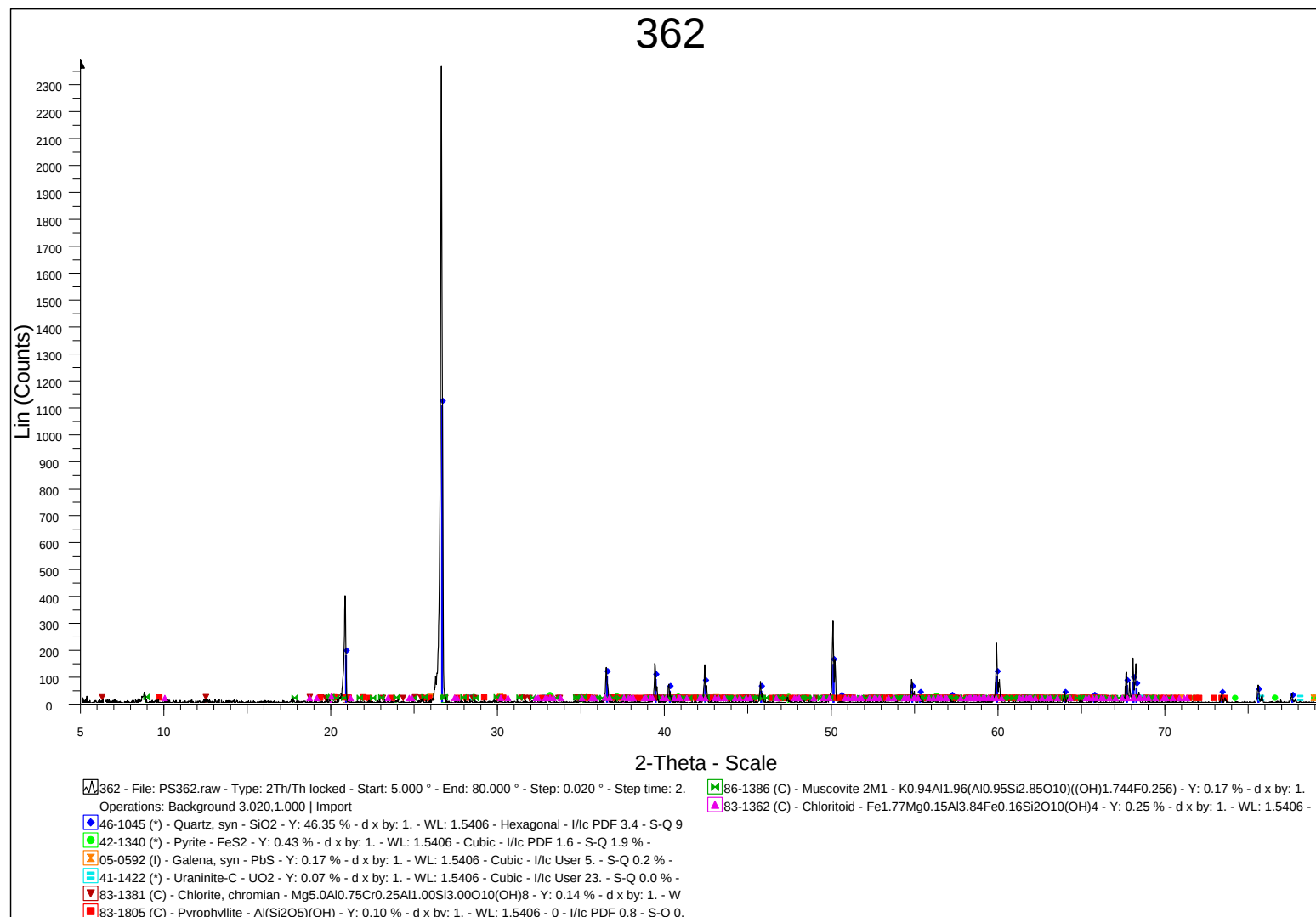
Appendix 17: Diffractogram of sample MK362 from Moab Khotsonq Mine representing the 370 geozone.
