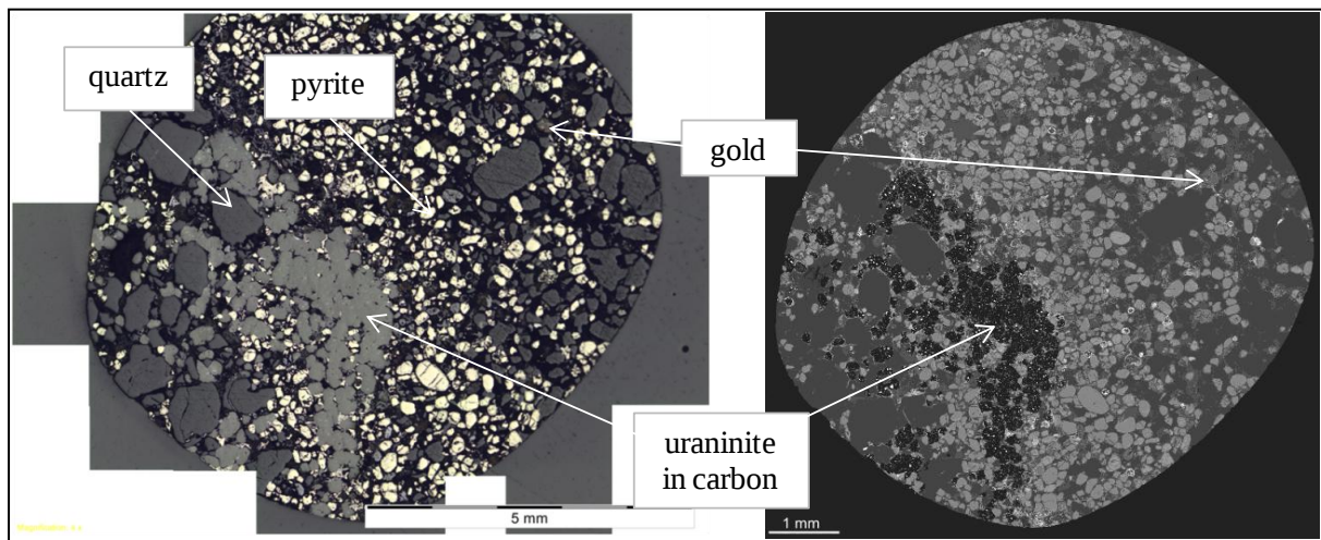
Figure 6.8: Photomicrograph (left) and backscattered electron (BSE) image (right) of sample 1k4 showing the distribution of uraninite in the carbonaceous matter and a gold grain (top right).
