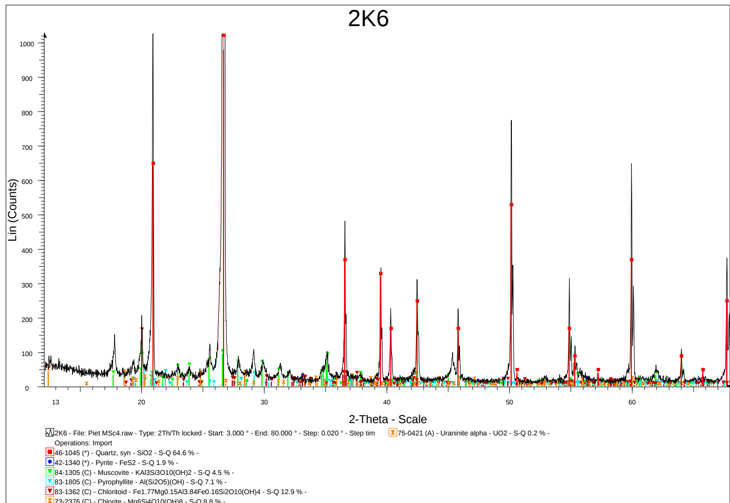
Appendix 23: Diffractogram of sample 2k6 from Kopanang Mine representing the 460 geozone.
