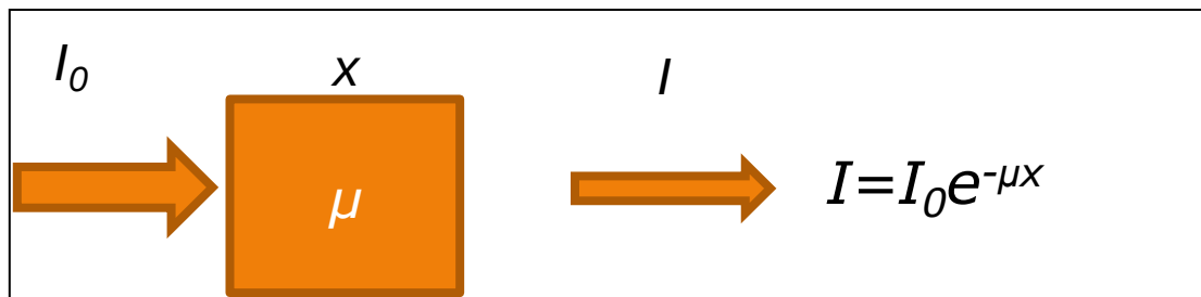
Figure 6.1: Illustration of Beer-Lambert Law of linear attenuation (de Beer et al. , 2004).
