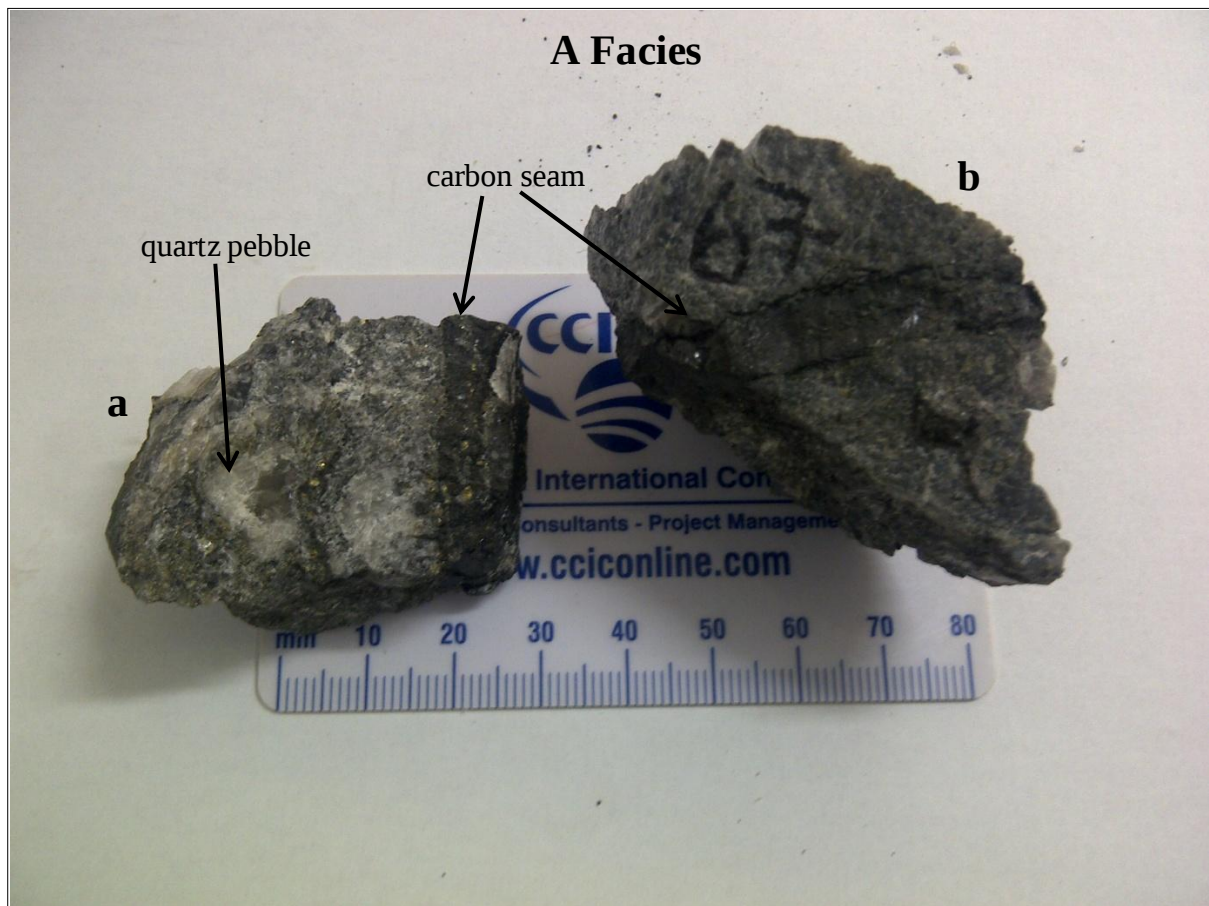
Figure 4.7: Hand specimens of the top of the Vaal Reef A Facies from Moab Khotsoong Mine 370 geozone. (a) Sample with oligomictic quartz pebbles and the carbonaceous seams enclosing pyrite grains. (b) Sample showing the carbonaceous seam cutting across the matrix; the sample is composed of a grey matrix with a few occurrences of sulphide minerals.
