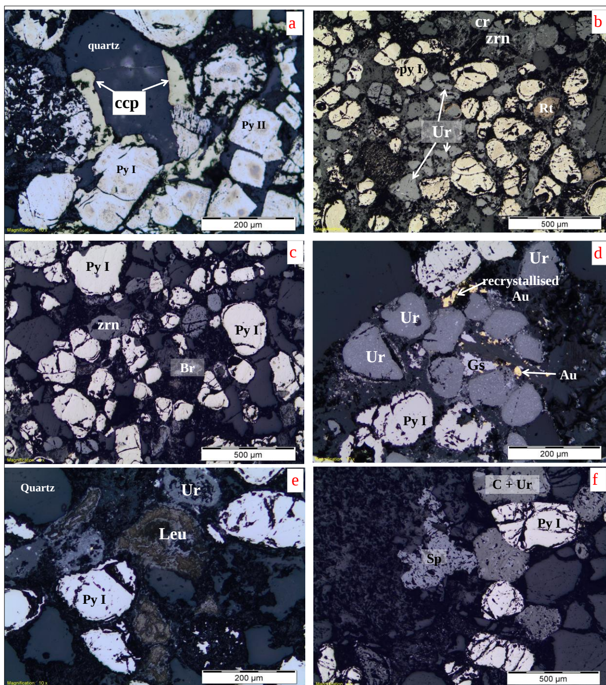
Figure 4.4: Reflected light photomicrographs of conglomerates from the Vaal Reef C Facies at Kopanang Mine. a) Allogenic (Py I) and authigenic (Py II) pyrite with chalcopyrite (Ccp) interstitial to quartz. b) Typical Vaal Reef occurrence of uraninite (Ur) with zircon (Zrn), chromite (Chr), rutile (Rt) and pyrite. c) Brannerite (Br) in the matrix with uraninite. d) Uraninite in association with pyrite, gersdorffite (Gs) and gold (Au). e) Uraniferous leucoxene (Leu) in matrix. f) Uraninite in association with brannerite.
