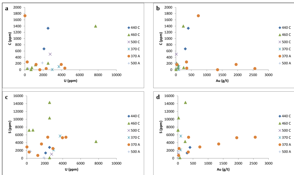
Figure 5.1: Plots of: (a) Whole-rock uranium vs. carbon from the A and C Facies samples. The C Facies and A Facies from the 370 geozone is generally uranium-rich. The 440 geozone representing the C Facies is carbon-rich. (b) Gold vs. Carbon; the A Facies 370 Geozone is more gold-rich than the C Facies samples. (c) Uranium vs sulphur; the C Facies is more sulphur-rich than the A Facies. (d) A plot of gold vs. sulphur.
