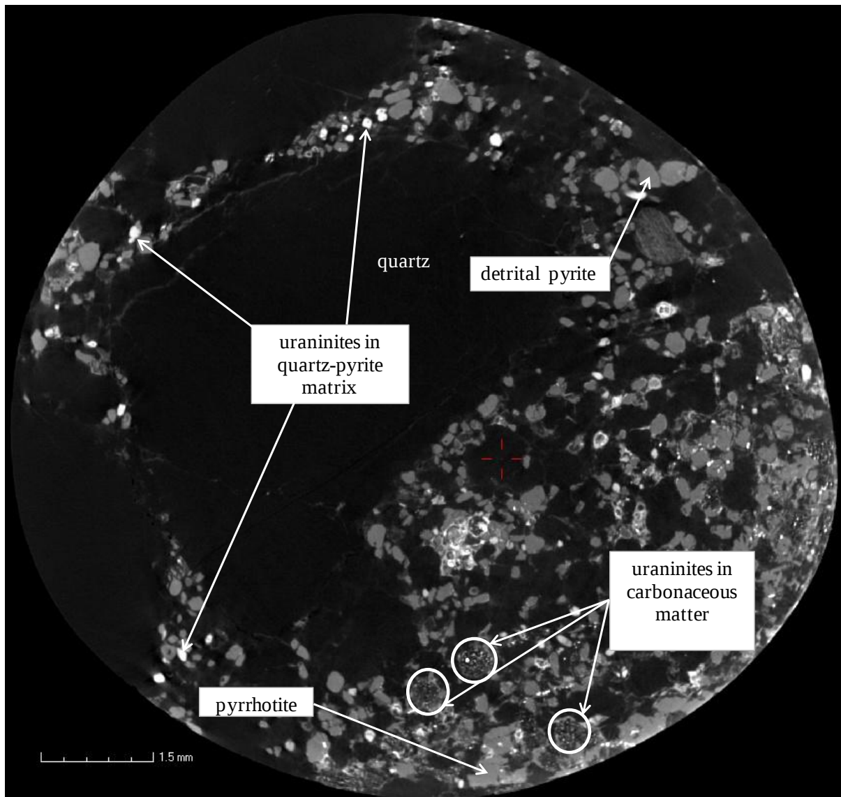
Figure 6.11: A tomogram slice of sample 3k2 showing the distribution of uraninite grains in the quartz-pyrite matrix and the carbonaceous matter (fly-speck carbon).
