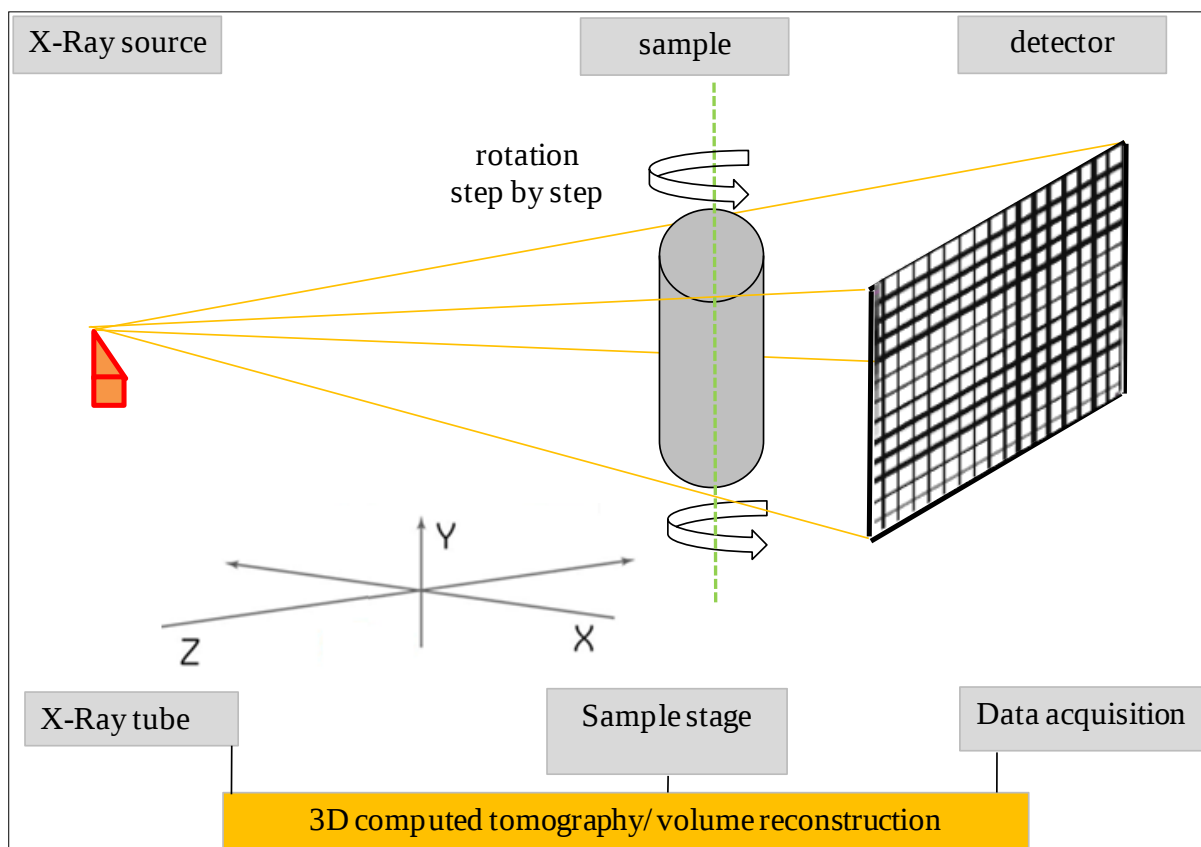
Figure 6.2: Illustration of basic operation principles and components of 3D X-ray computed tomography. X-rays are produced from a tube at a point source in a form of a cone beam and pass through a rotating sample. The attenuated X-ray signal results are recorded by the detector. The data acquired are reconstructed into a 3D volume by volume reconstruction software (Nshimirimana et al. , 2011).
