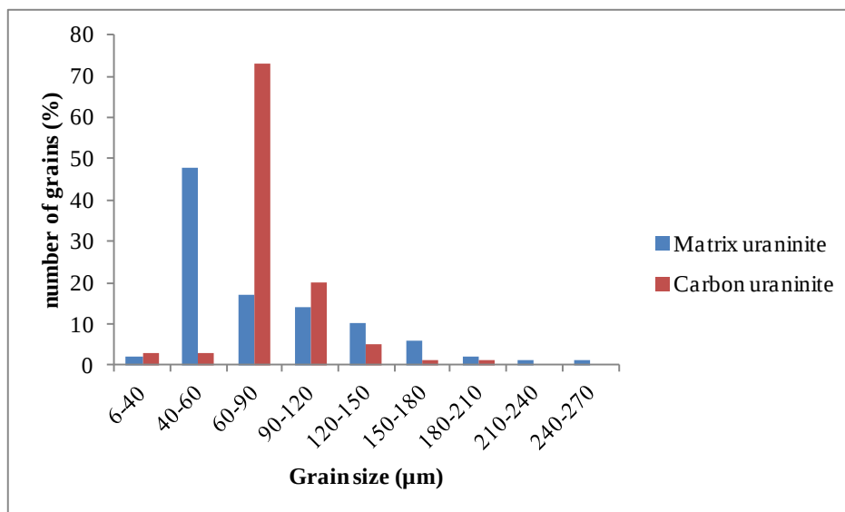
Figure 6.17: A plot of size vs number of grains in percentage in the matrix and the carbonaceous matter.
