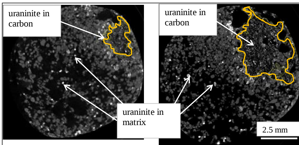
Figure 6.15: Tomogram slices from sample 1k4 showing the distribution of uraninite grains in the matrix and carbonaceous matter (outlined in yellow) acquired from Image J software.
