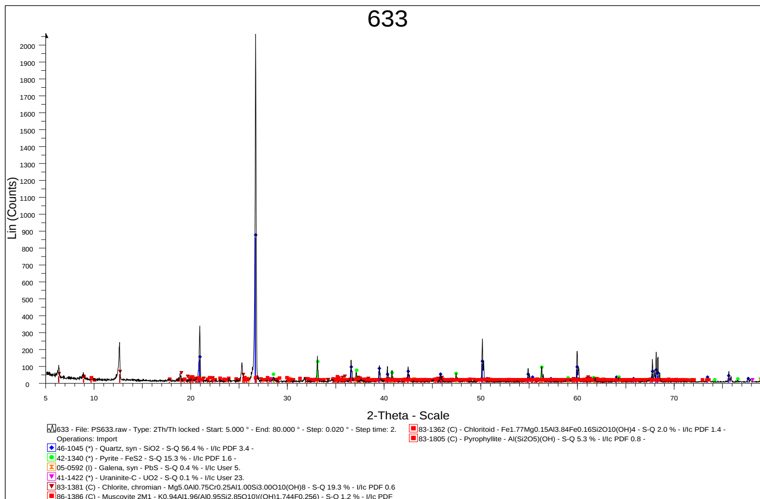
Appendix 26: Diffractogram of sample GBH 633 from Great Noligwa Mine representing the 370 geozone.
