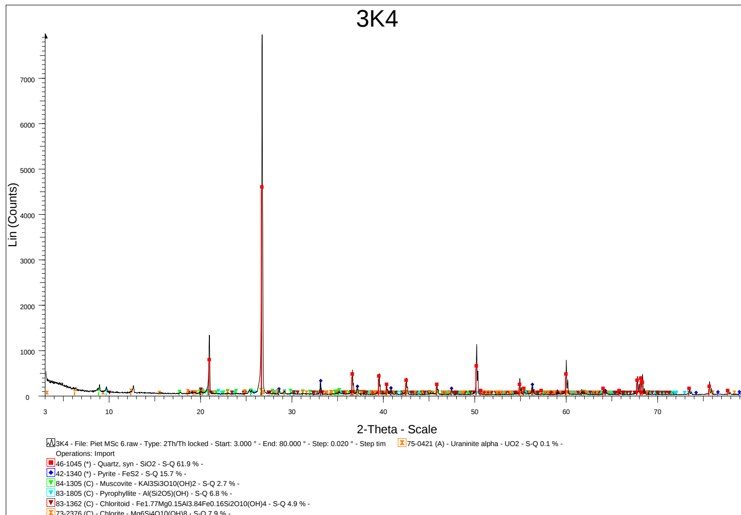
Appendix 25: Diffractogram of sample 3k4 from Kopanang Mine representing the 460 geozone.
