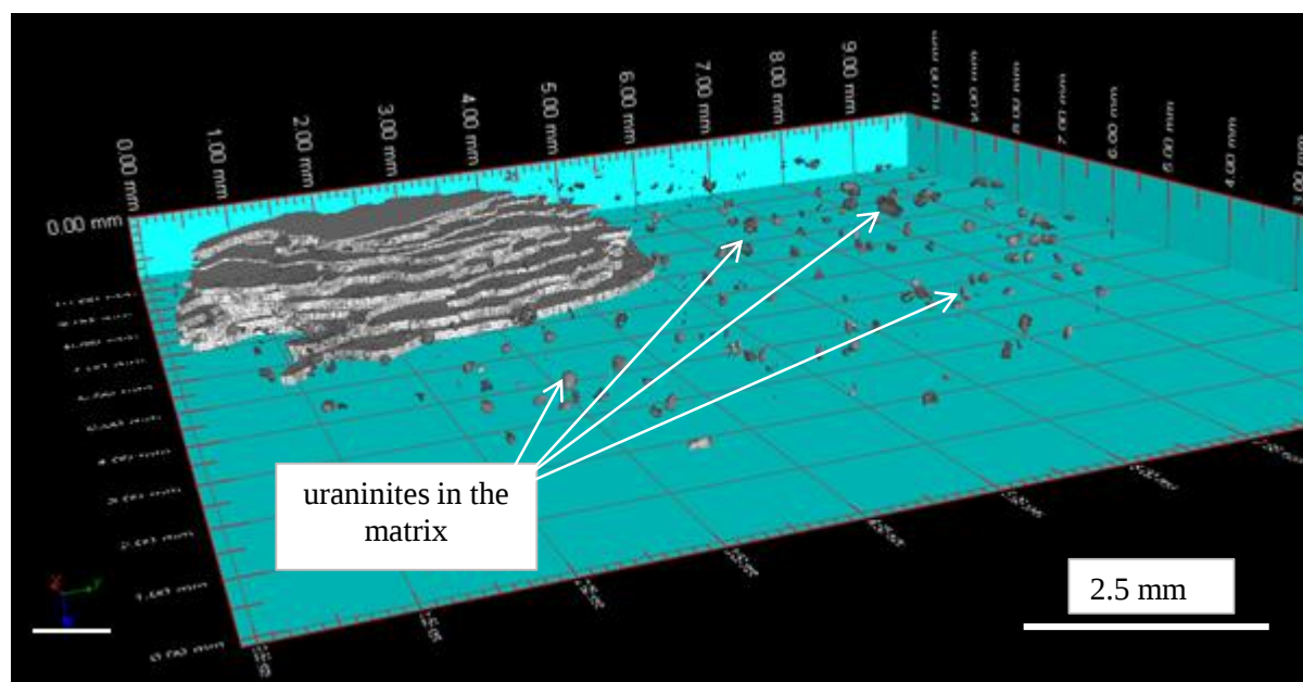
Figure 6.16: Illustration of 3D volume from slice 1515 to slice 1616 obtained from sample 1k4 using VGStudioMax showing only uranium group of minerals occurring in the matrix.
