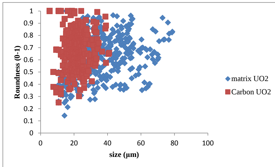
Figure 6.19: A plot of roundness vs. size of uranium group of minerals grains in the matrix and the carbonaceous matter obtained from Image-J.
