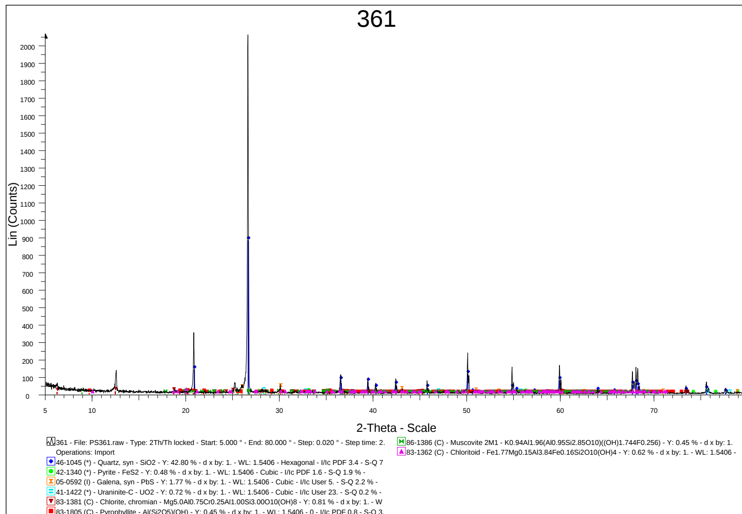
Appendix 16: Diffractogram of sample MK361 from Moab Khotsong Mine representing the 370 geozone.
