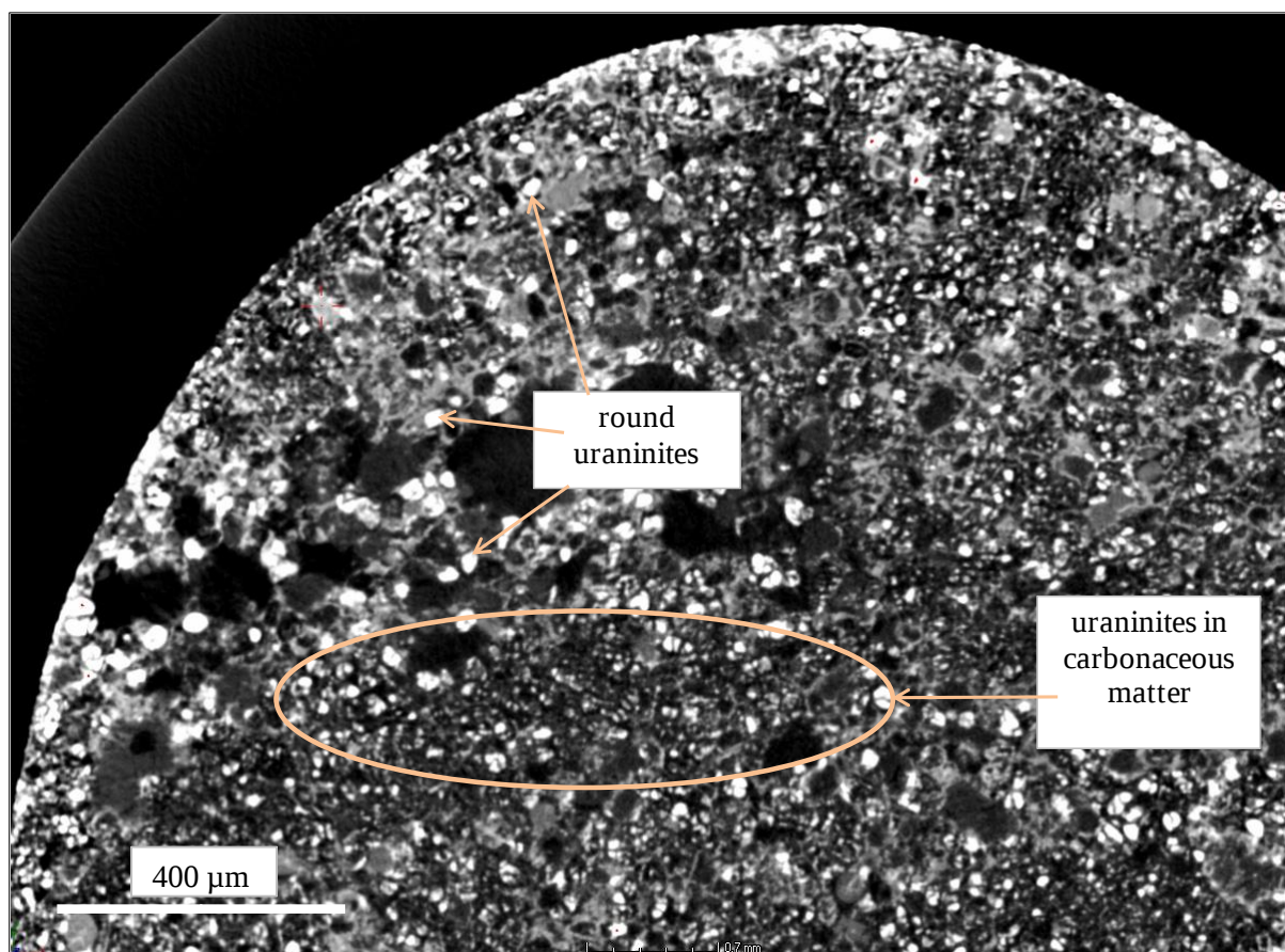
Figure 6.12: A tomogram slice of sample Mk367 showing the distribution of uraninite grains in the quartz-pyrite matrix and the carbonaceous matter.
