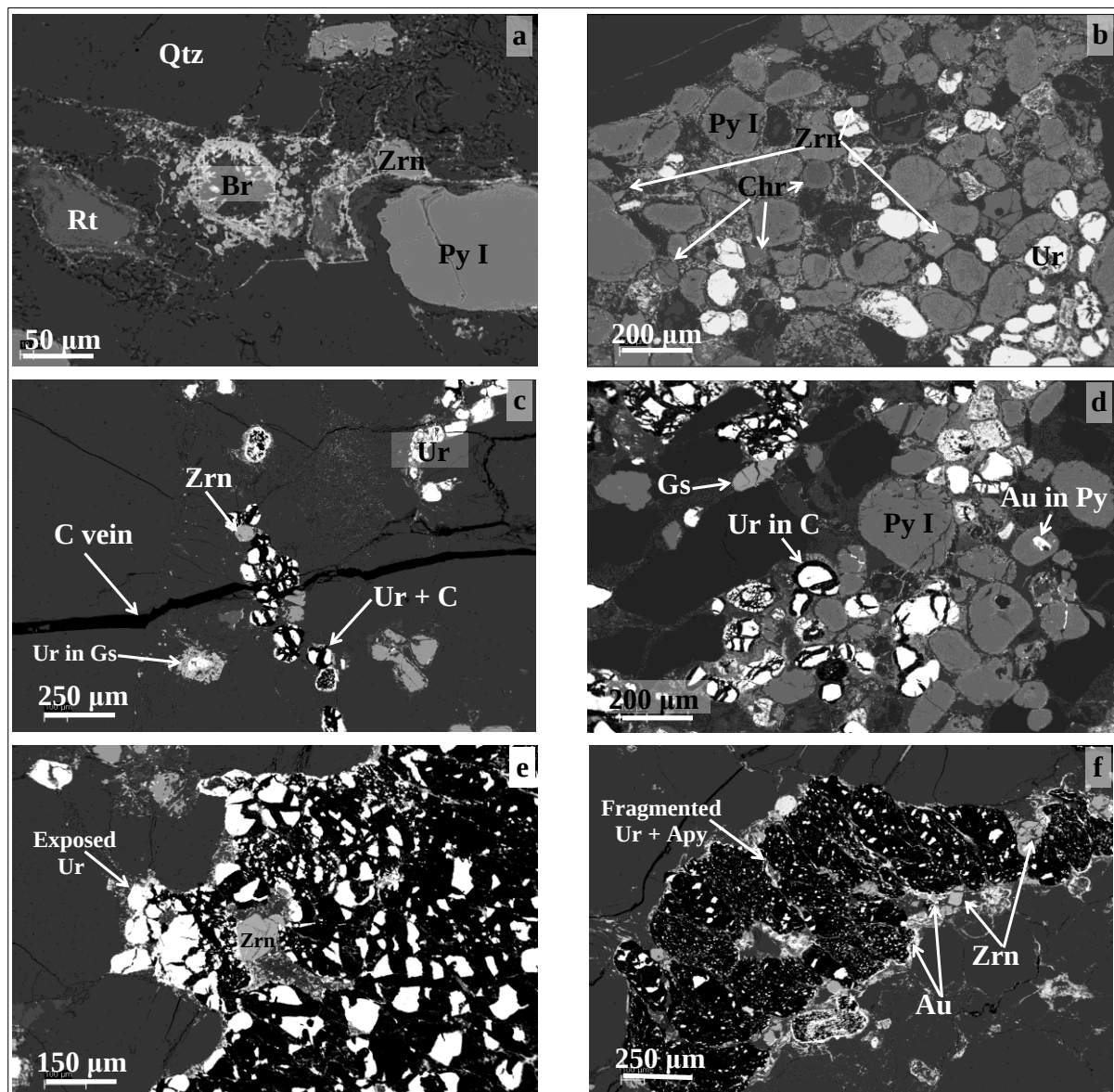
Figure 4.6: Backscattered electron (BSE) images from Kopanang Mine C Facies samples. a) Needle-shaped brannerite (Br) in the matrix with rutile (Rt), zircon (Zrn) and pyrite (PyI). b) Allogenic or detrital nature of pyrite, zircon, chromite (Chr) and uraninite (Ur). c) Uraninite grains fragmented by carbon (C) fly speck with a second generation of carbon vein devoid of uranium mineralisation; uraninite enclosed in gersdorffite (Gs). d) Occurrence of detrital uraninite with cracks infilled by carbon; rounded pyrite and gersdorffite occur with uraninite. e) Uraninite grains that were not covered by carbonaceous matter. f) Carbonaceous seam fragmenting uraninite and arsenopyrite (Apy), with zircon and gold on the edges of the seam.
