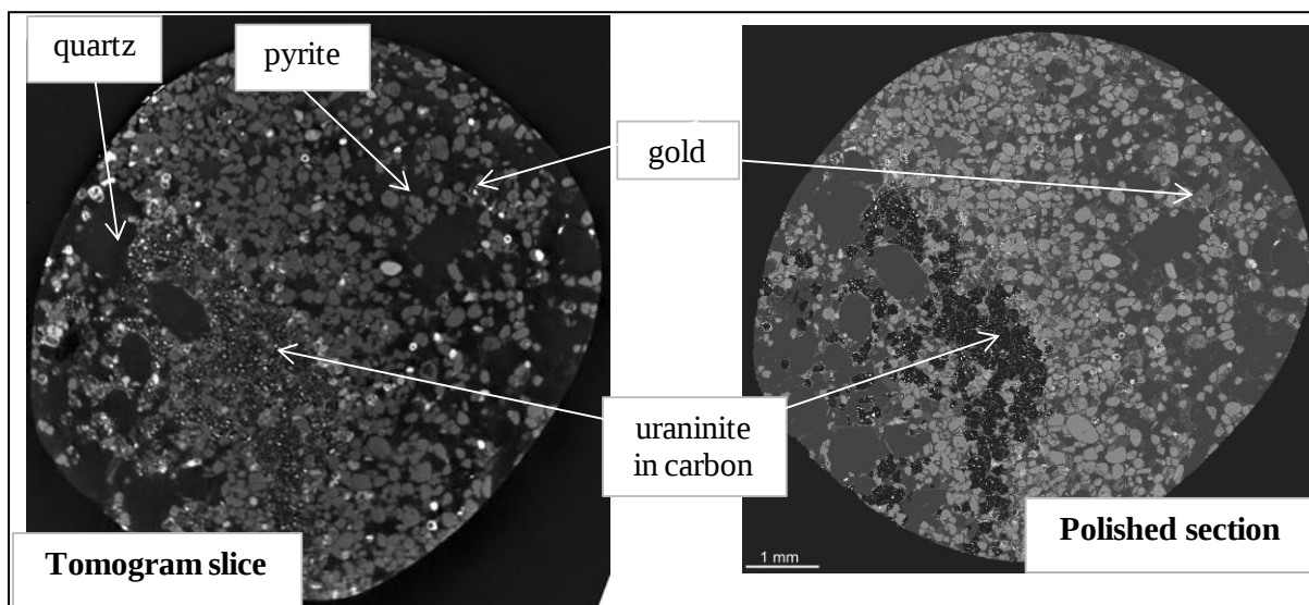
Figure 6.9: Comparison of 3D tomogram slice (left) and BSE image (right) of sample 1k4.
