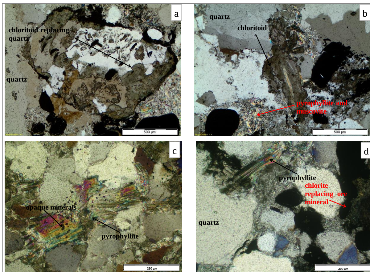
Figure 4.8: Photomicrographs of silicate and phyllosilicate minerals of the Vaal Reef C Facies, all images were taken under cross polarised light (Xpl). (a) Chloritoid replacing a quartz grain. (b) Large grain of chloritoid replacing quartz and fine-grained pyrophyllite-muscovite in the matrix. (c) Pyrophyllite laths enclosing opaque minerals in the quartz matrix. (d) Pyrophyllite laths in the quartz matrix, and chlorite replacing opaque minerals.
