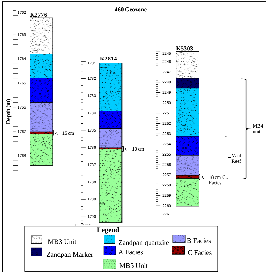
Figure 3.17: Boreholes K2776, K2814 and K5303 intersecting the Vaal Reef. The C Facies is the primary economic facies hosting high grades of gold and uranium; the thickness of the C Facies is 15 cm in borehole K2776, 10 cm in borehole K2814 and 18 cm in borehole K5303.
