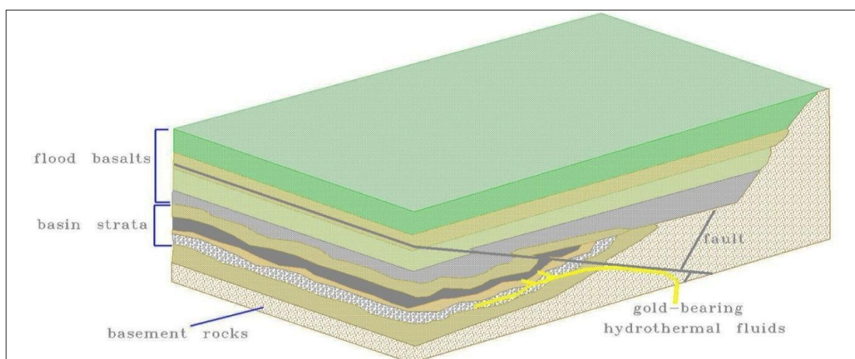
Figure 2.4: Illustration of the hydrothermal fluids (2.7-2.0 Ga) from later processes within the Witwatersrand Basin. Gold has been derived from hydrothermal sources from deep within the earth's crust and carried along faults into the basin after deposition of the conglomerates (after Kirk et al. , 2003).
