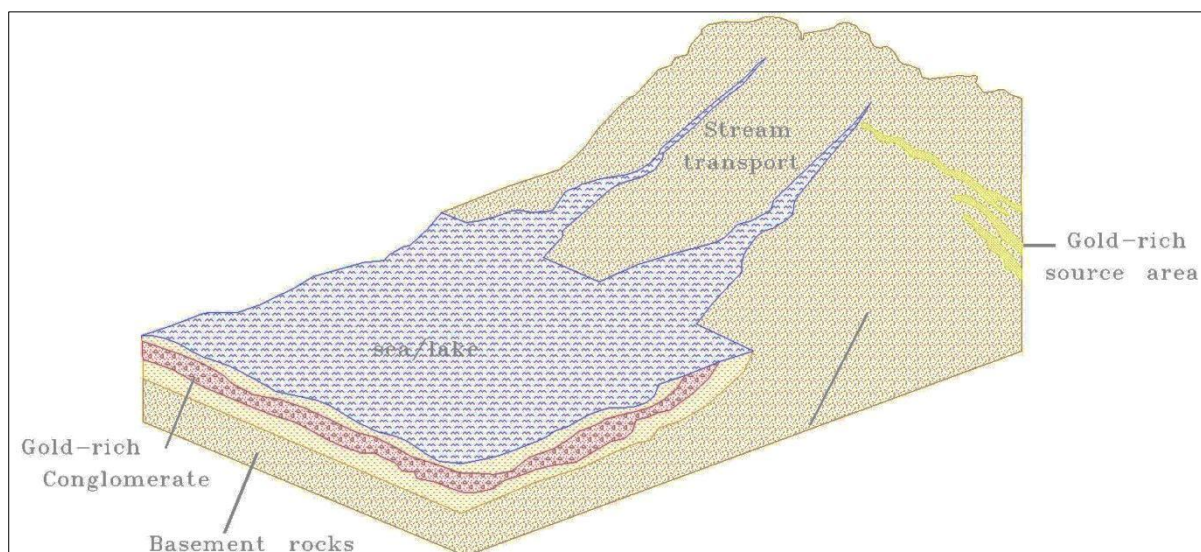
Figure 2.3: Illustration of the placer model with greenstone gold-rich sources areas suggested to be komatiites or metamorphosed basalts older (3.5-2.9 Ga) than the deposition of the Witwatersrand Basin. Detrital gold has been mechanically eroded from the old source areas into the basin (sea or lake) by deltaic fluvial processes. The age of the gold in the basin is similar to the older gold sources (after Kirk et al. , 2003).
