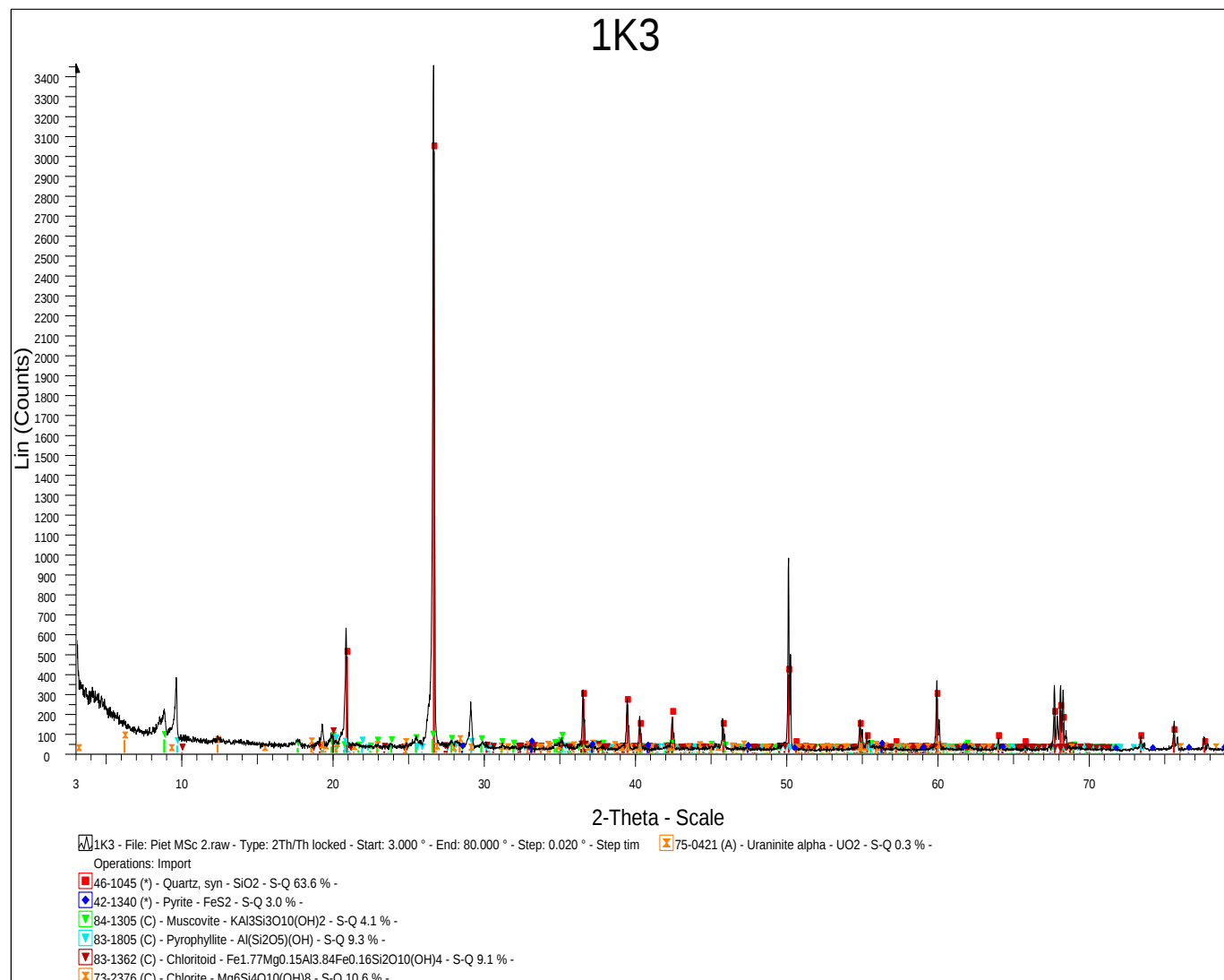
Appendix 21: Diffractogram of sample 1K3 from Kopanang Mine representing the 440 geozone.
