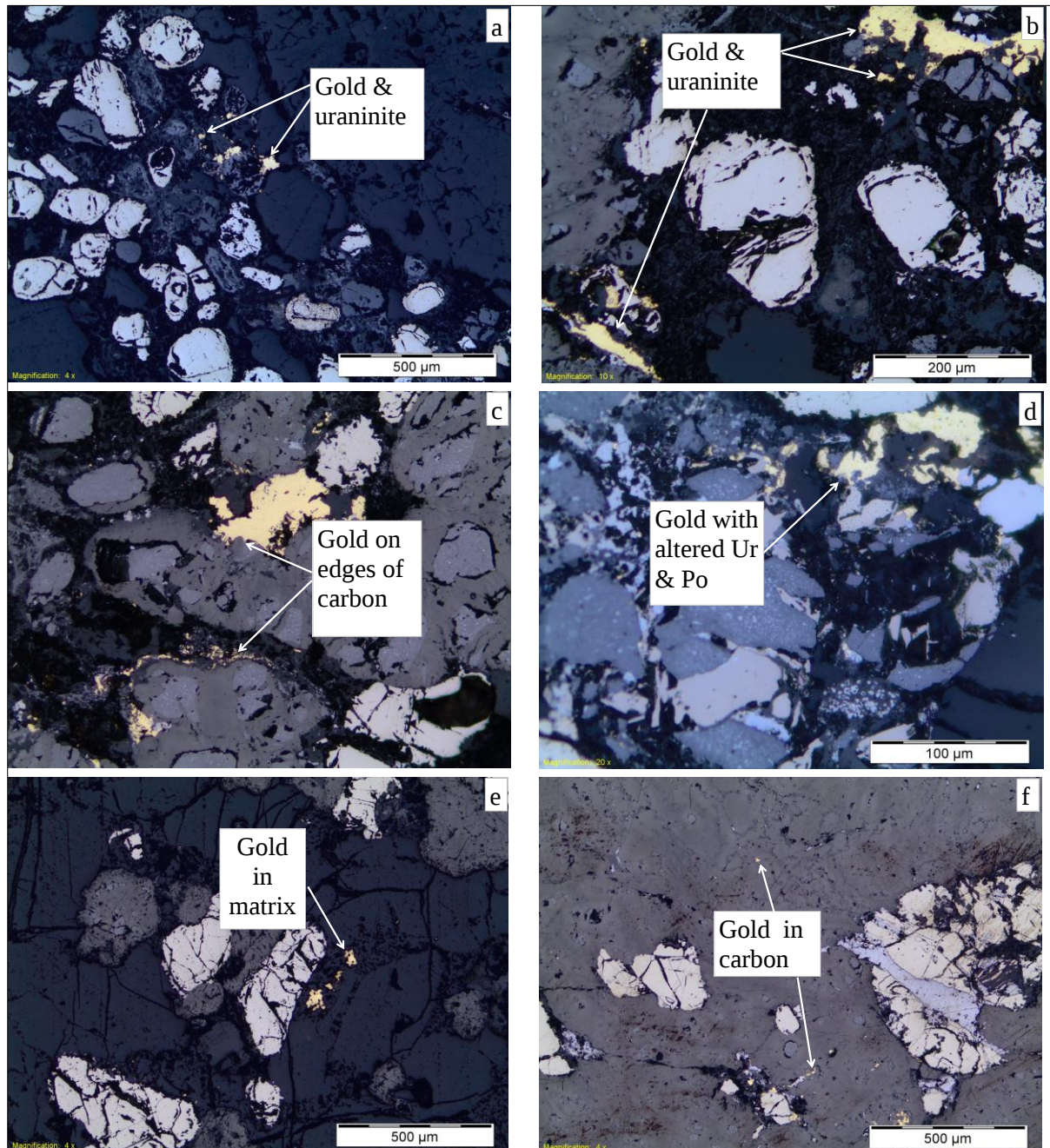
Figure 4.12: Photomicrographs of gold grains in the Vaal Reef matrix and carbonaceous occurrences. a) Gold associated with detrital matrix minerals such as uraninite and Pyrite. b) Irregular and elongated-shaped gold with the matrix and carbonaceous matter. c) Gold occurring interstitial to the carbonaceous matter. d) Gold associated with uraninite and pyrrhotite (Po). e) Gold trapped in a quartz pebble. f) Thin gold grains interstitial to the carbonaceous groundmass.
