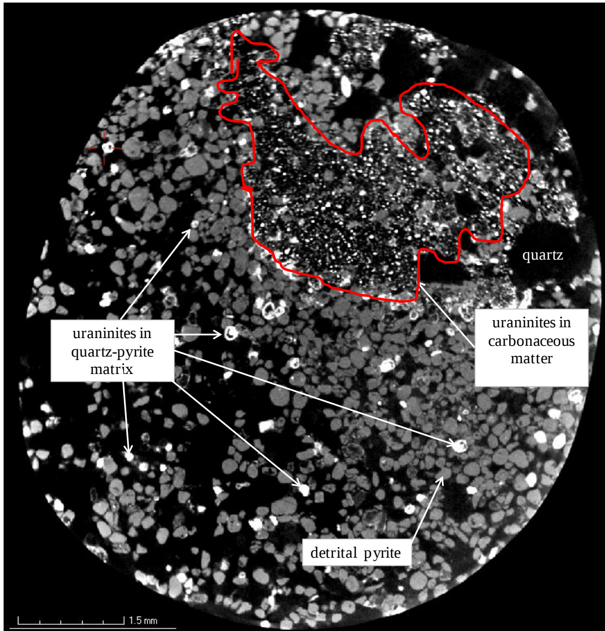
Figure 6.10: A tomogram slice of sample 1k4 showing the distribution of uraninite grains in the quartz-pyrite matrix and the carbonaceous matter (outlined in red).
