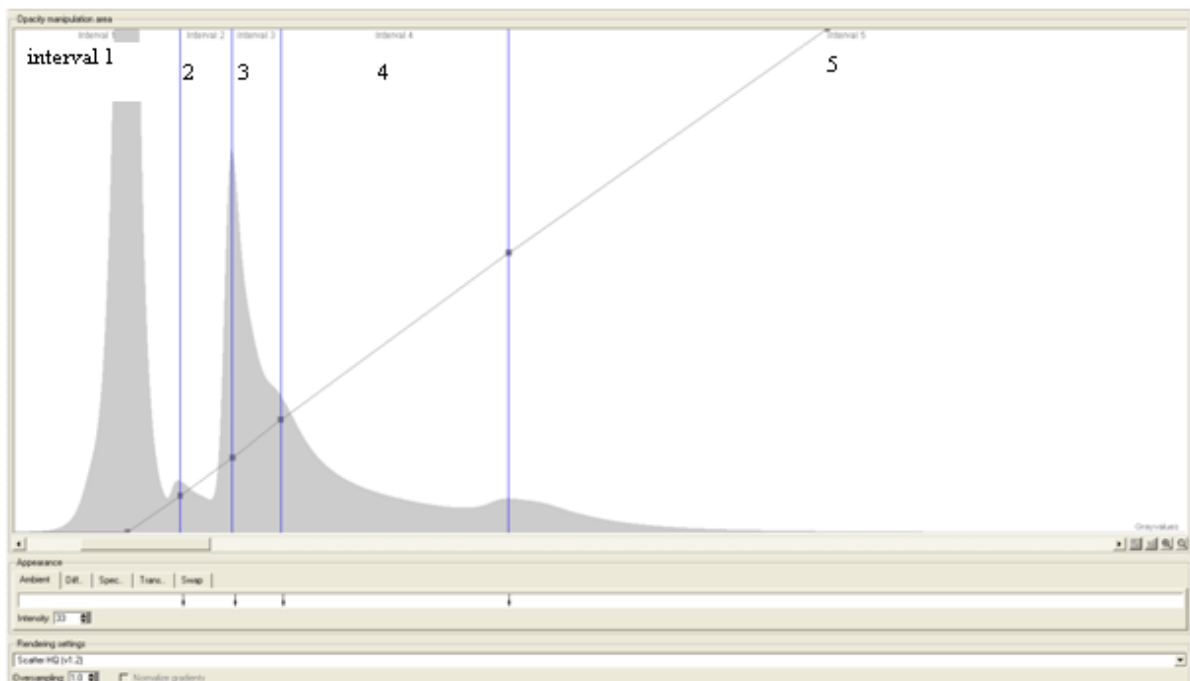
Figure 6.7: Example of a grey value histogram obtained from VGStudioMax 2.1 imaging software showing peaks that represent intervals of (1) air, carbonaceous matter (2) quartz and silicate minerals (3), sulphide minerals (4), uranium-bearing minerals and gold (5) derived from thresholding.
