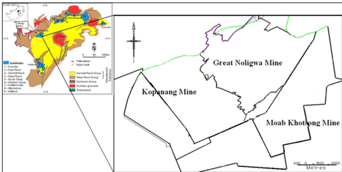
Figure 3.4: Locality map of Kopanang, Great Noligwa and Moab Khotsoong Mines in the Klerksdorp Goldfield (after Frimmel, 2005 and AngloGold Ashanti internal report, 2001).
