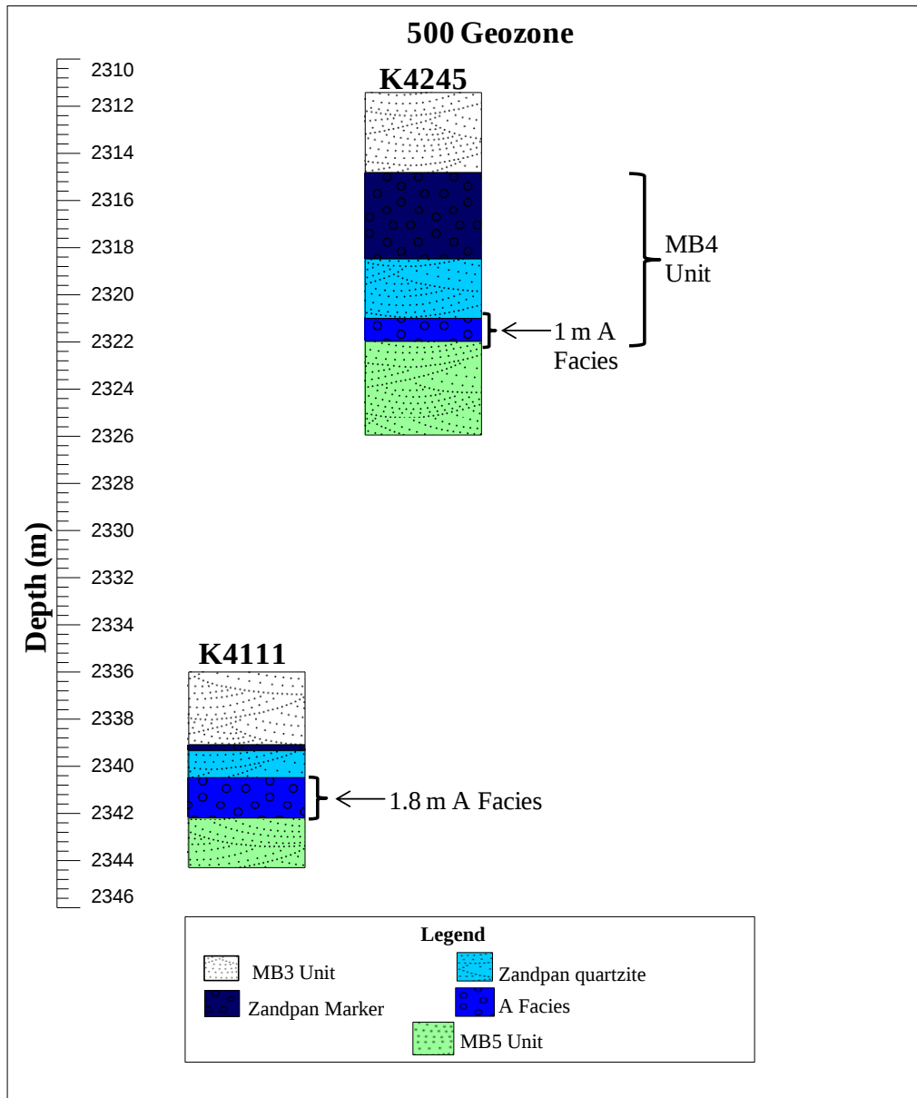
Figure 3.18: Stratigraphic section of the Vaal Reef in boreholes K4111 and K4245 from Kopanang Mine representing the 500 geozone.
