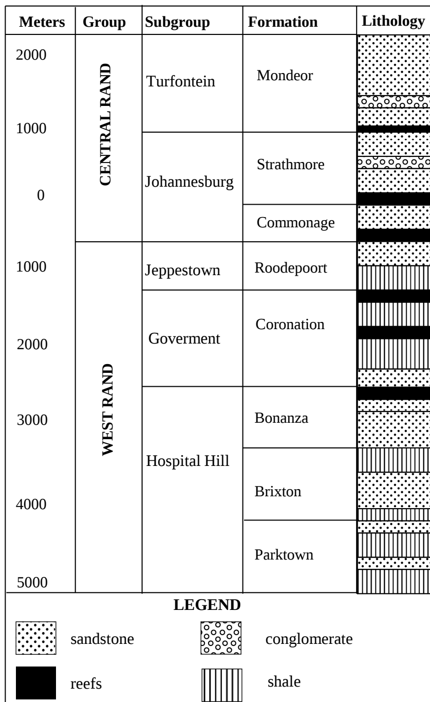
Figure 2.2: Simplified stratigraphic column of the Witwatersrand Supergroup, Subgroups, common Formations and lithologies (after Frimmel, 2005).
