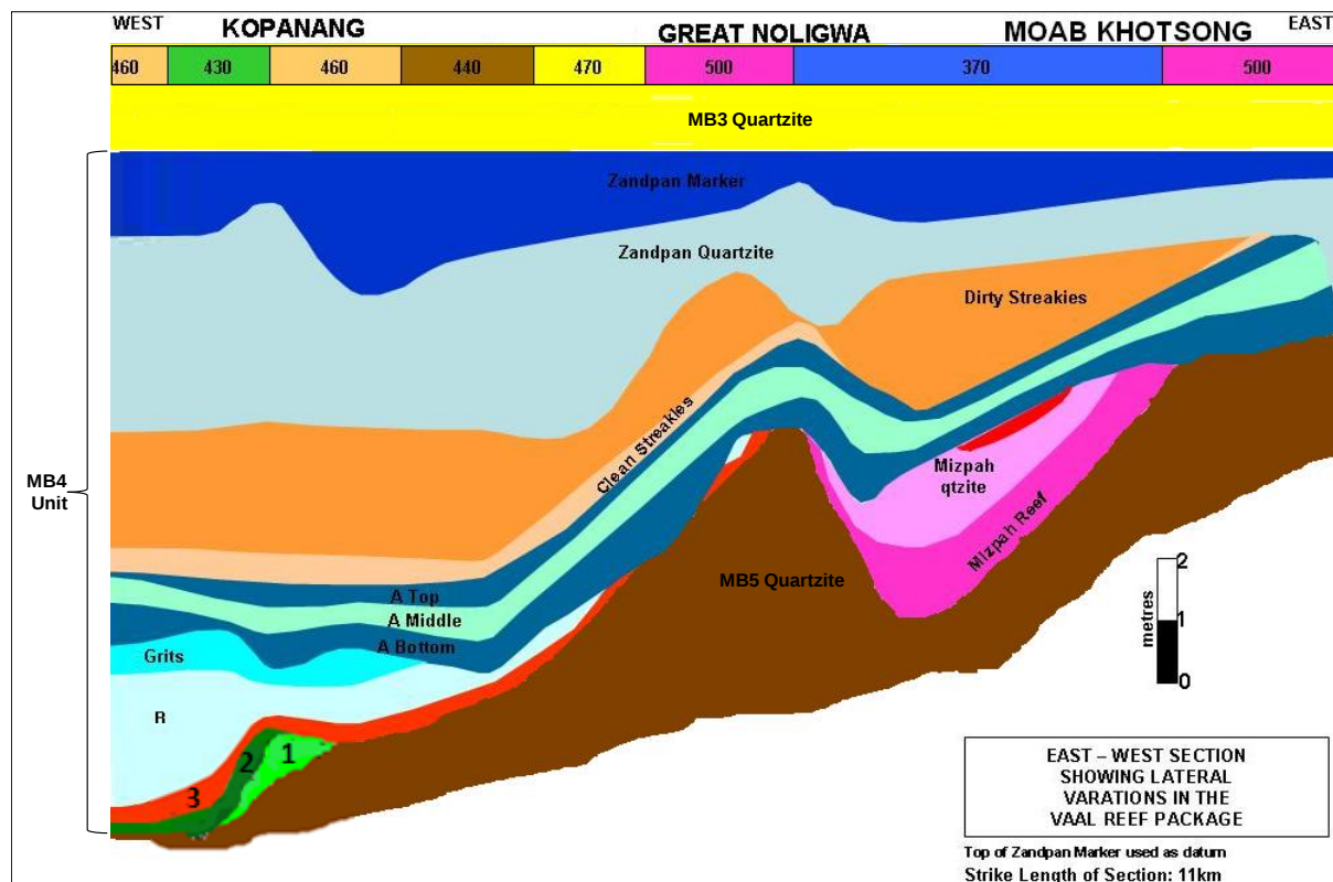
Figure 3.5: East-west cross-section of Kopanang and Great Noligwa Mines showing lateral variations of the Vaal Reef package (C [3], B and A Facies) resting on the Witkop (1) and Grootdraai Facies (2) within the MB4 unit. The latter is overlain by the MB3 quartzite and underlain by the MB5 quartzite. The Vaal Reef package from east to west is represented by six geozones (AngloGold Ashanti internal report, 2001).
