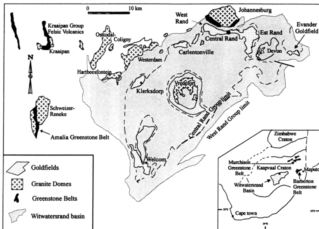
Figure 2.5: Illustration of the locality of the Witwatersrand Basin with its major goldfields surrounded by older Archaean greenstone and basement granites throughout the entire basin. The location of the Witwatersrand Basin within the Kaapvaal Craton is shown in the insert map (after Poujol et al. , 1999).
