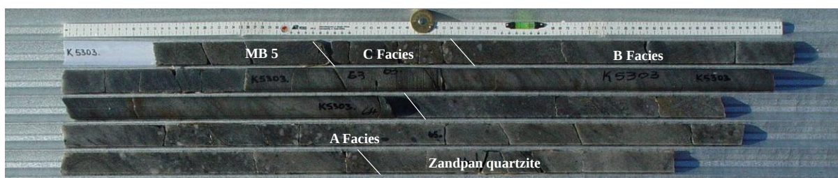
Figure 3.16: Photograph of Borehole K5303 intersecting the MB5, C Facies, B Facies, A Facies and the Zandpan quartzite.
