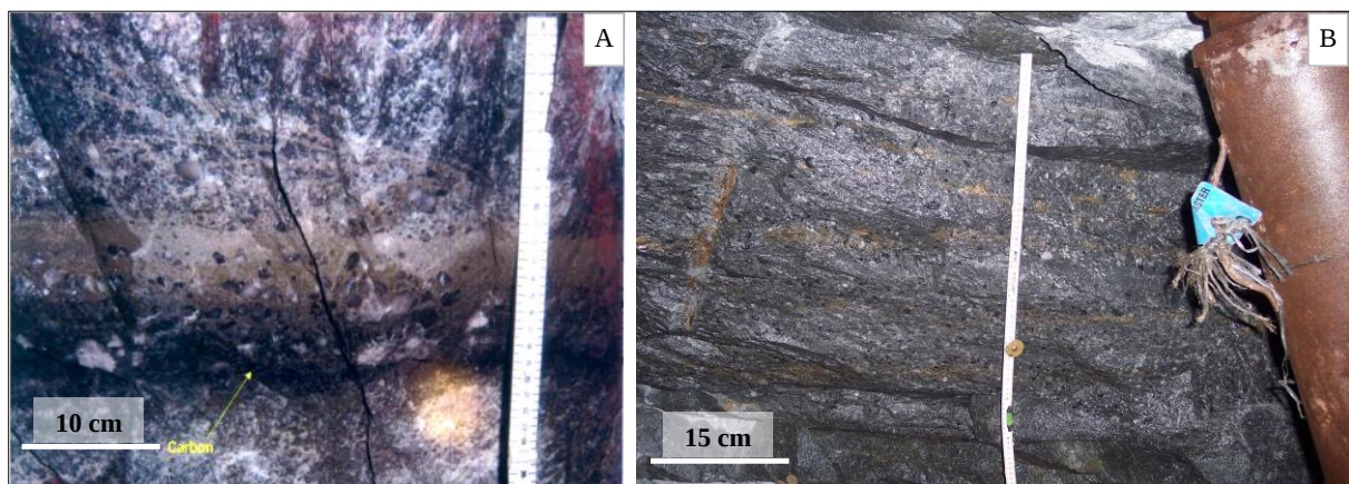
Figure 3.6: Layout of the Vaal Reef. a) The Vaal Reef C Facies at Kopanang Mine overlies the MB5 quartzite with a carbon seam at the base of the reef and a pyrite-rich matrix. b) The Vaal Reef A Facies at Moab Khotsong Mine showing the MB5 quartzite footwall overlain by the reef polymictic conglomerate.
