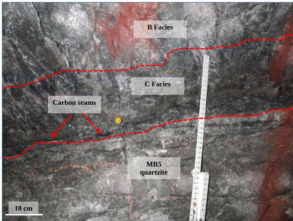
Figure 3.8: The Vaal Reef C Facies in the 460 geozone with thin carbonaceous matter at the bottom of the reef; the reef is overlain by the B Facies and rests on the MB5 quartzite footwall. The Grootdraai conglomerate was not observed.
