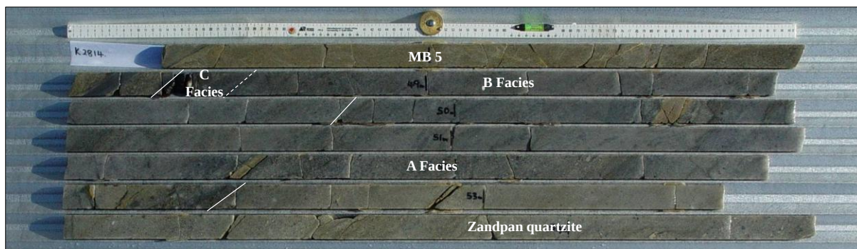
Figure 3.15: Photograph of borehole K2814 intersecting the MB5 quartzite, C Facies, B Facies, A Facies and the Zandpan quartzite.
