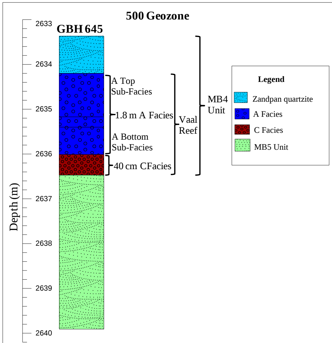
Figure 3.21: Stratigraphic section of the Vaal Reef in borehole GBH 645 from Great Noligwa Mine showing the development of C and A Facies overlying each other. The borehole represents the 500 geozone.
