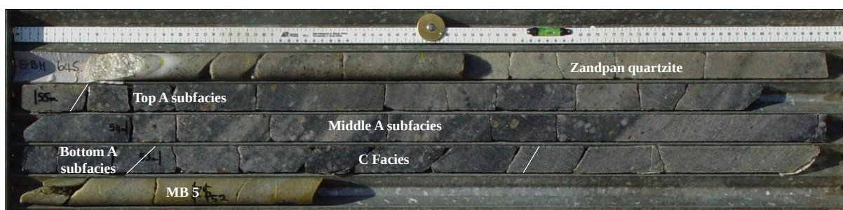
Figure 3.20: Photograph of borehole GBH 645 intersecting the MB5 quartzite, C Facies, Bottom A Subfacies, Middle A Subfacies, Top A Subfacies and the Zandpan quartzite.
