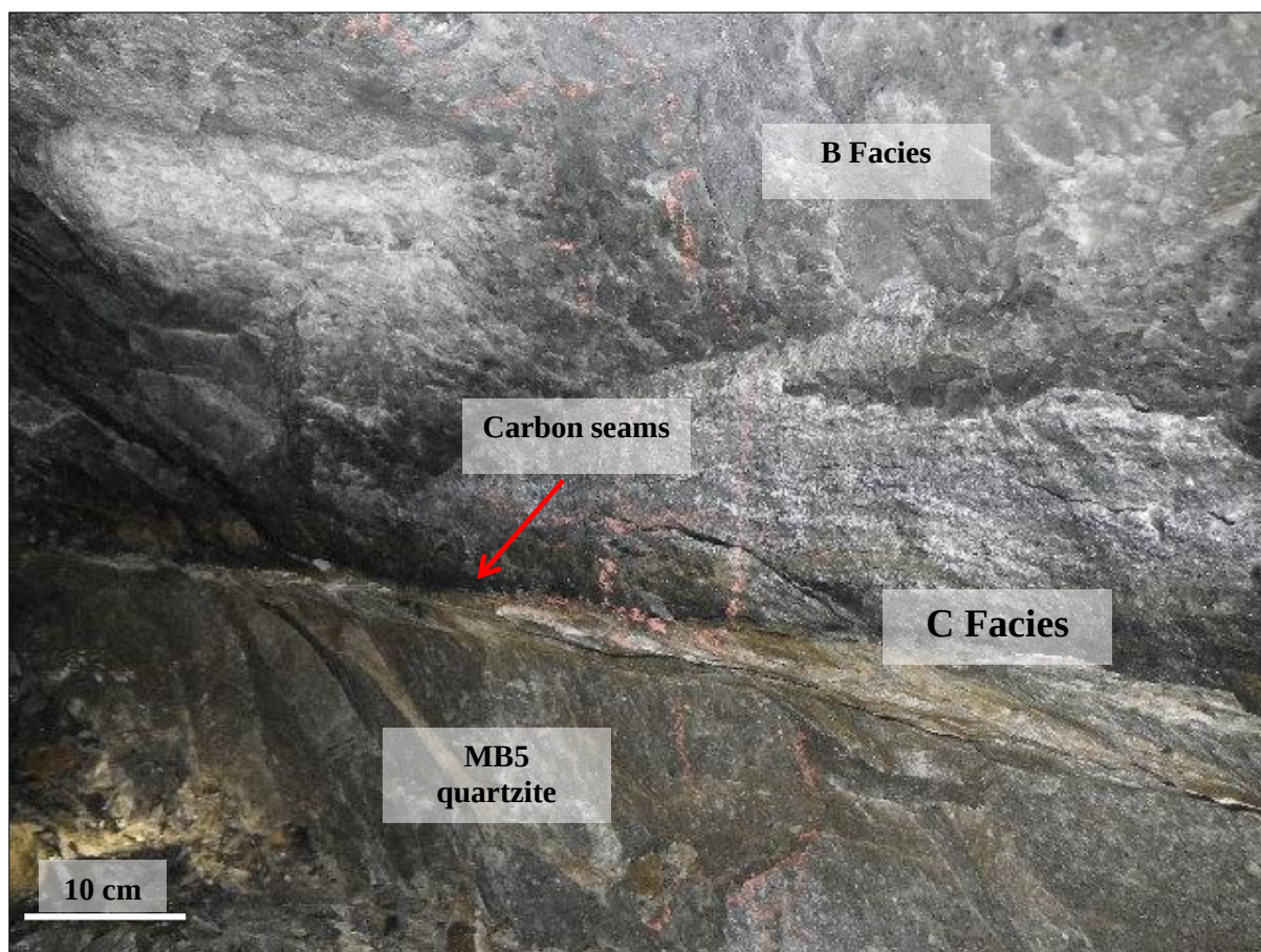
Figure 3.9: The Vaal Reef C Facies in the 430 geozone overlain by the B Facies with a carbon seam at the bottom of the reef; the Vaal reef rests on the MB5 quartzite footwall. No Grootdraai conglomerate was observed.
