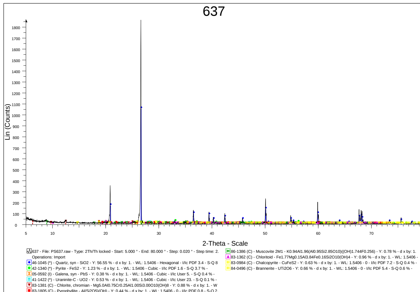
Appendix 27: Diffractogram of sample GBH 637 from Great Nologwa Mine representing the 370 geozone.
