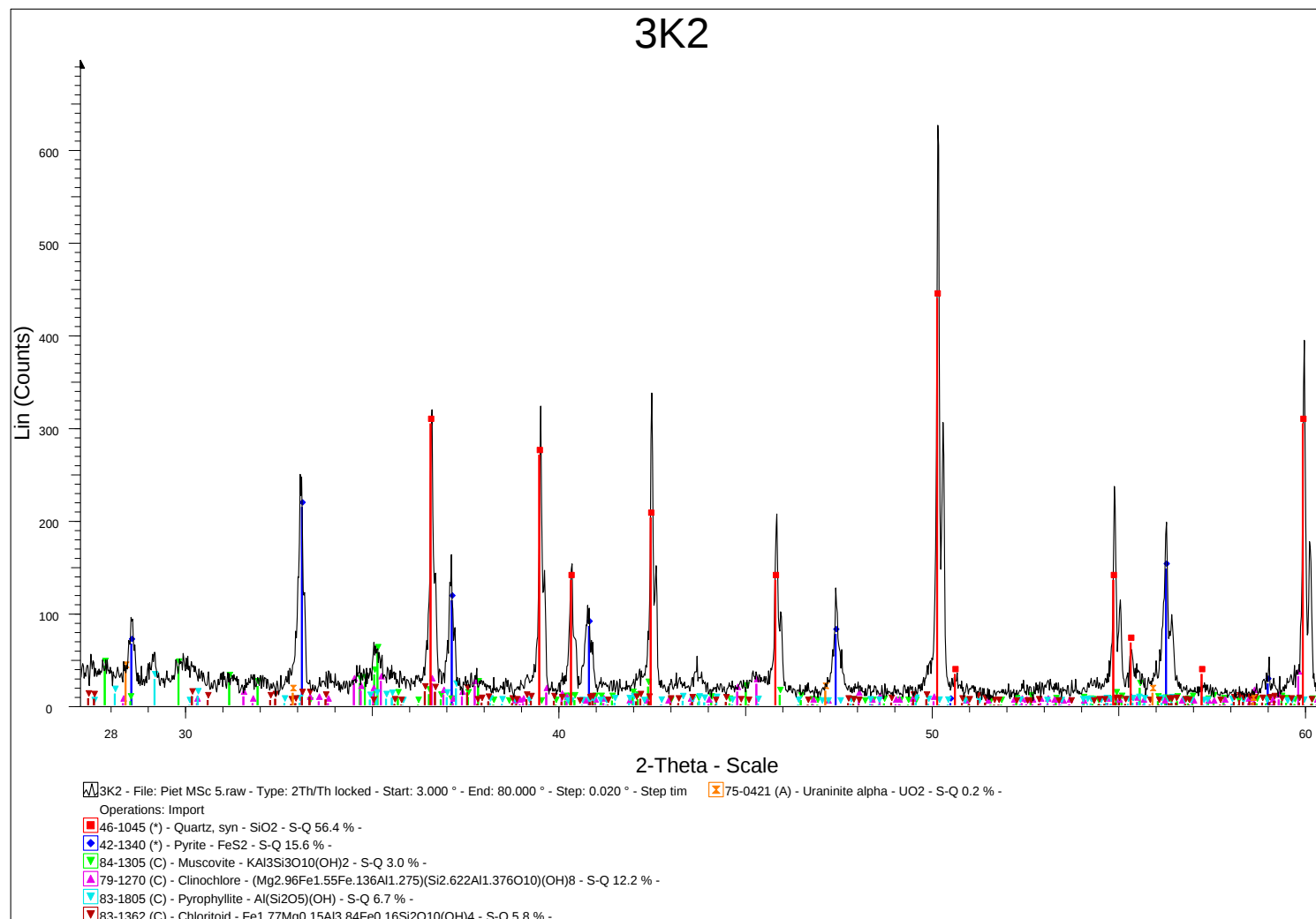
Appendix 24: Diffractogram of sample 3k2 from Kopanang Mine representing the 460 geozone.
