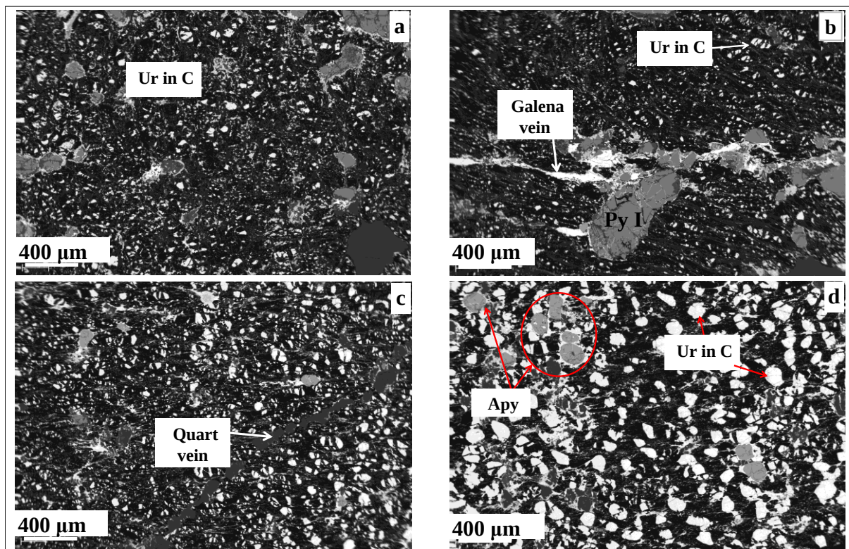
Figure 4.10: Backscattered electron images of Moab Khotsong samples. a) Fragmented uraninite grains and pyrite in a carbonaceous groundmass. b) Elongated carbonaceous seam with fragmented uraninite grains, galena vein cross-cuts the carbonaceous seam. c) Quartz vein cross-cuts a carbonaceous seam. d) Carbonaceous seam dominated by uraninite with minor arsenopyrite grains circled in the red ring.
