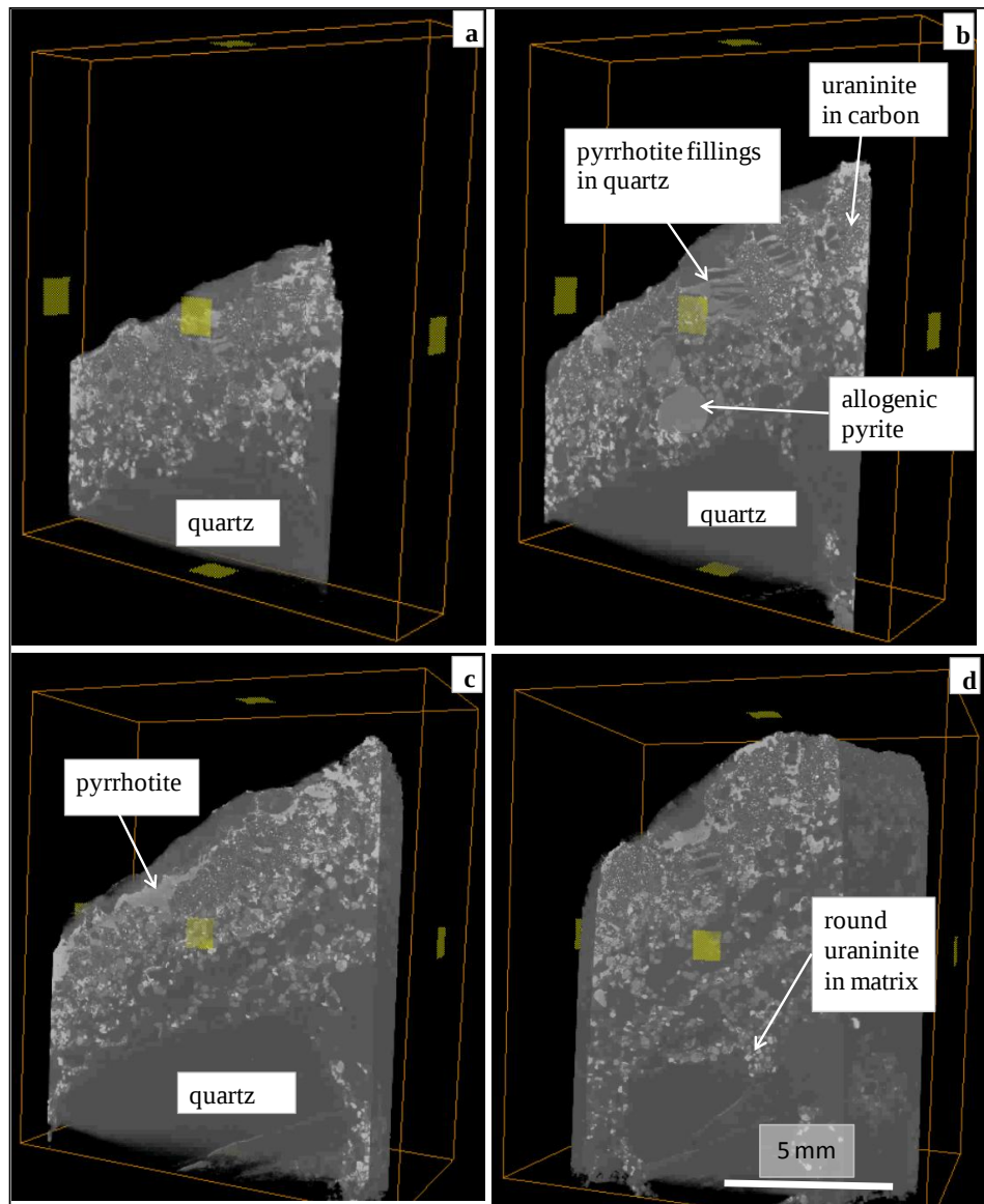
Figure 6.13: A series of longitudinal tomograms from sample 3k2 illustrating the 3D nature and distribution of uranium minerals (white), sulphide minerals (light grey) and quartz (dark grey).
