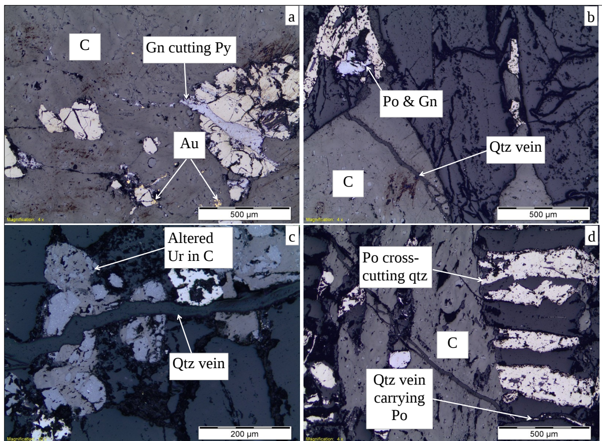
Figure 4.11: Photomicrographs of sample sections displaying infillings and veinlets. a) Cracked detrital pyrite (Py) filled by galena (Gn) veinlets that extend into the carbonaceous matter (C) groundmass, recrystallised gold grains are observed in the carbonaceous matter. b) Pyrrhotite (Po) and galena as infillings in the fractured quartz; a quartz vein is observed crosscutting the carbonaceous matter. c) A quartz vein cuts across a series of fly specks that hosts fragmented detrital uraninite. d) A set of parallel pyrrhotite layers cross-cutting a quartz pebble; a quartz vein carrying pyrrhotite cuts through the carbonaceous matter.
