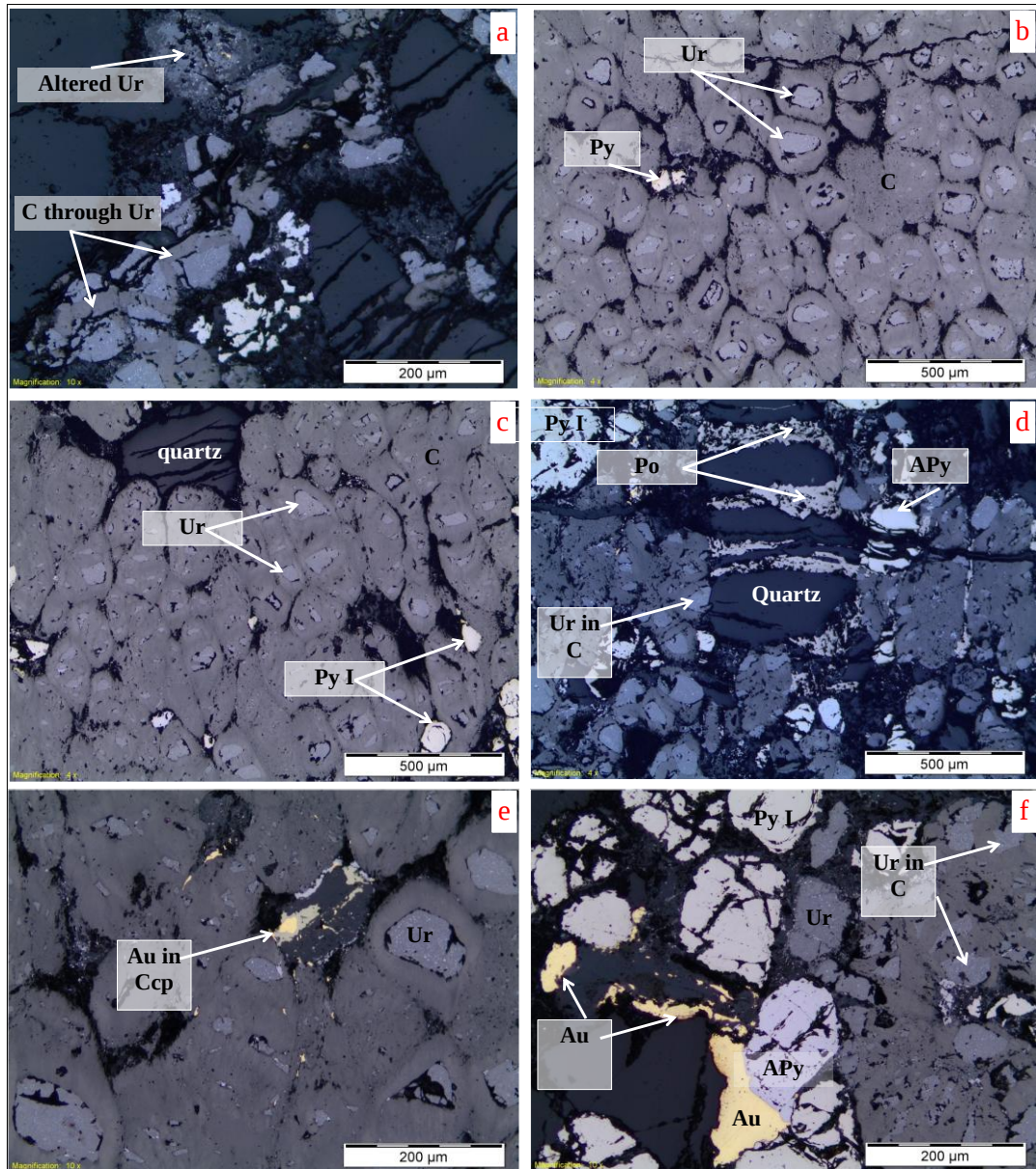
Figure 4.5: Reflected light photomicrographs of carbonaceous matter in the Vaal Reef C Facies at Kopanang Mine. a) Fragmented uraninite (Ur) grains cross-cut by carbonaceous matter. b) Uraninite enclosed in carbonaceous (C) seam. c) Uraninite in carbonaceous matter with grains fragmented. d) Authigenic pyrrhotite (Po) infilling quartz cracks; carbonaceous matter in close association with uraninite and arsenopyrite (APy). e) Authigenic gold (Au) in chalcopyrite (Ccp) in a fractured quartz grain, surrounded by carbonaceous matter enclosing uraninite grains. f) Gold in matrix associated with arsenopyrite (APy), there are two populations of uraninites, in the matrix and also surrounded by the carbonaceous matter.
