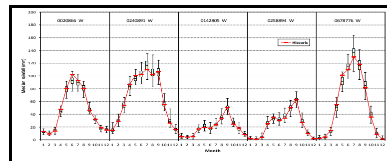
Figure 4.28b Box plots of monthly median rainfalls for stations 0020866 W, 0240891 W, 0142805 W, 0258894 W and 0678776 W from VLB generator
