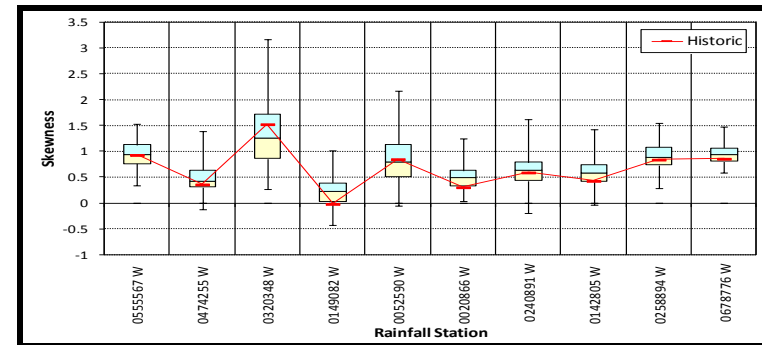
Figure 4.23b Box plots of skewness of annual rainfalls from VLB generator
