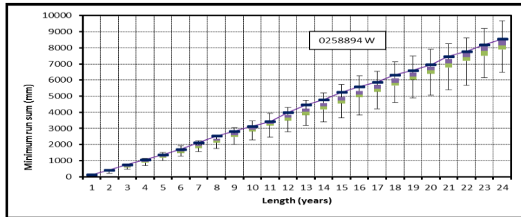
Figure 4.14a Box plots of minimum run sums for station 0258894 W from EMD-VLB generator
