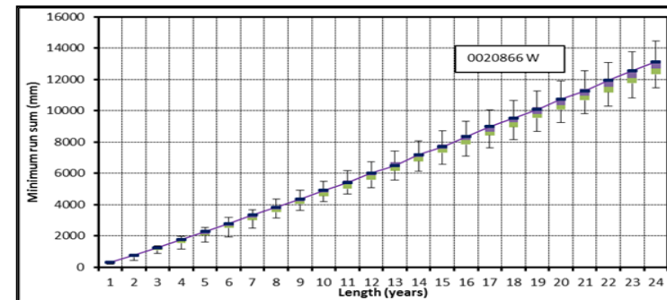
Figure 4.11a Box plots of minimum run sums for station 0020866 W from EMD-VLB generator
