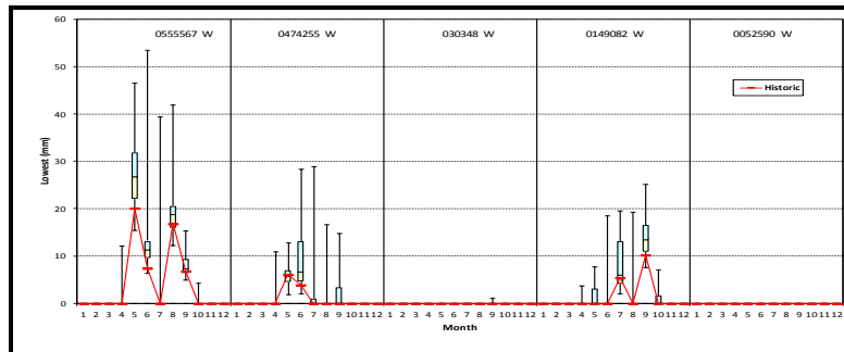
Figure 4.33b Box plots of monthly lowest rainfalls for stations 0555567 W, 0474255 W, 030348 W, 0149082 W and 0052590 W from VLB generator
