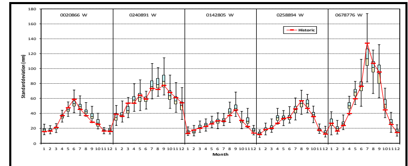
Figure 4.38b Box plots of monthly standard deviations for stations 0020866 W, 0240891 W, 0142805 W, 0258894 W and 0678776 W from VLB generator
