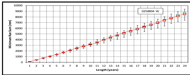
Figure 4.14b Box plots of minimum run sums for station 0258894 W from VLB generator
