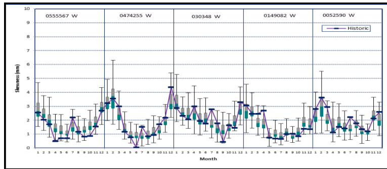
Figure 4.39a Box plots of monthly skewness of rainfalls for stations 0555567 W, 0474255 W, 030348 W, 0149082 W and 0052590 W from EMD-VLB generator
