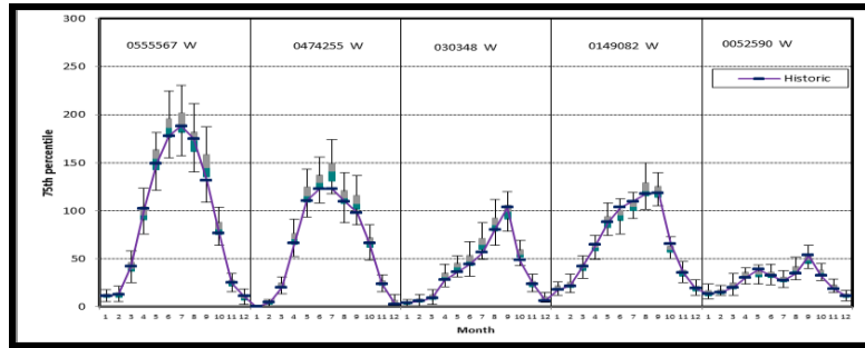
Figure 4.31a Box plots of monthly 75 th percentile rainfalls for stations 0555567 W, 0474255 W, 030348 W, 0149082 W and 0052590 W from EMD-VLB generator
