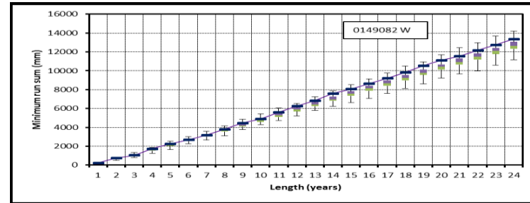
Figure 4.9a Box plots of minimum run sums for station 0149082 W from EMD-VLB generator
