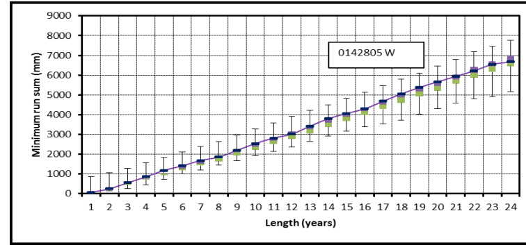
Figure 4.13a Box plots of minimum run sums for station 0142805 W from EMD-VLB generator
