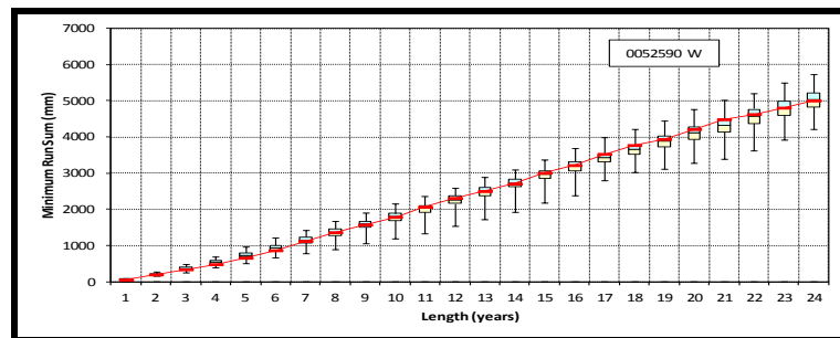
Figure 4.10b Box plots of minimum run sums for station 0052590 W from VLB generator
