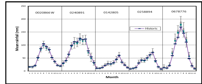
Figure 4.26a Box plots of monthly mean rainfalls for stations 0020866 W, 0240891 W, 0142805 W, 0258894 W and 0678776 W from EMD-VLB generator
