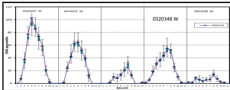
Figure 4.29a Box plots of monthly 25 th percentile rainfalls for stations 0555567 W, 0474255 W, 0320348 W, 0149082 W and 0052590 W from EMD-VLB generator
