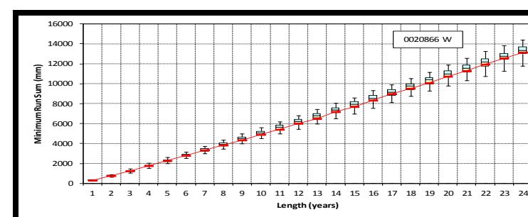
Figure 4.11b Box plots of minimum run sums for station 0020866 W from VLB generator
