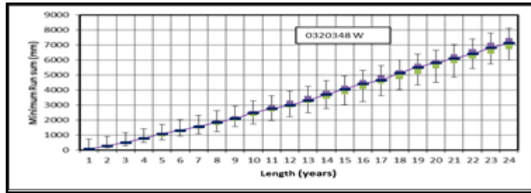
Figure 4.8a Box plots of minimum run sums for station 0320348 W from EMD-VLB generator
