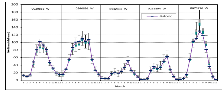
Figure 4.28a Box plots of monthly median rainfalls for stations 0020866 W, 0240891 W, 0142805 W, 0258894 W and 0678776 W from EMD-VLB generator
