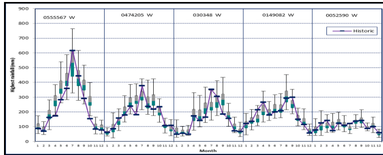
Figure 4.35a Box plots of monthly highest rainfalls for stations 0555567 W, 0474205 W, 030348 W, 0149082 W and 0052590 W from EMD-VLB generator
