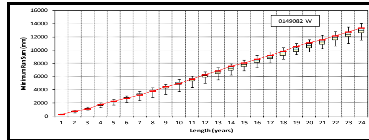
Figure 4.9b Box plots of minimum run sums for station 0149082 W from VLB generator
