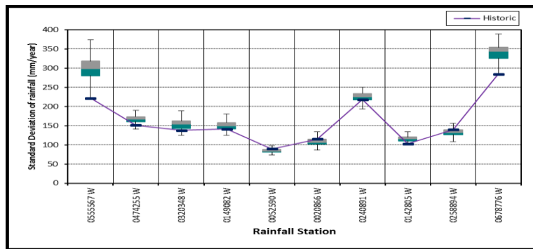
Figure 4.22a Box plots of standard deviation of annual rainfall from EMD-VLB generator
