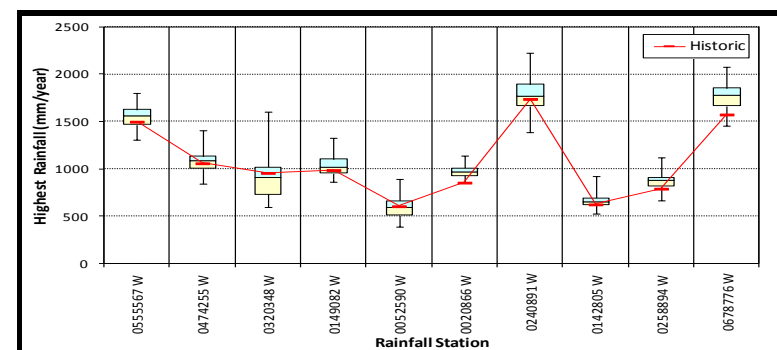
Figure 4.21b Box plots of highest annual rainfalls from VLB generator
