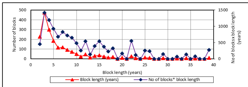
Figure 4.1 Number of blocks generated and the total length of blocks of specified length from the EMD-VLB generator.
