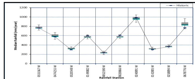
Figure 4.17a Box plots of annual median rainfall from EMD-VLB generator
