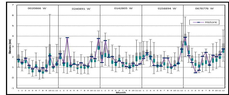
Figure 4.40a Box plots of monthly skewness for stations 0020866 W, 0240891 W, 0142805 W, 0258894 W and 0678776 W from EMD-VLB generator
