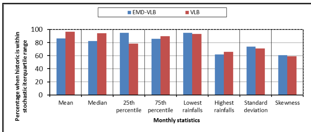
Figure 4.41 Percentages when the historic monthly values are within the interquartile ranges of the stochastic monthly statistics from the EMD-VLB and the VLB generators
