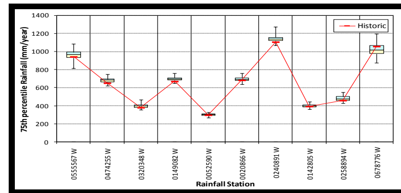
Figure 4.19b Box plots of annual 75 th percentile rainfalls from VLB generator
