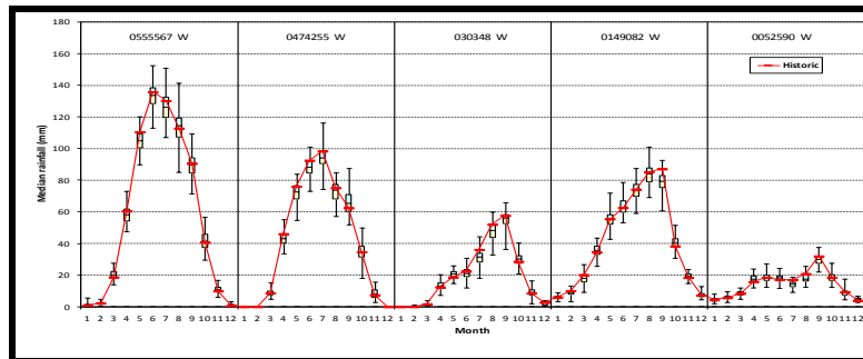
Figure 4.27b Box plots of monthly median rainfalls for stations 0555567 W, 0474255 W, 030348 W, 0149082 W and 0052590 W from VLB generator
