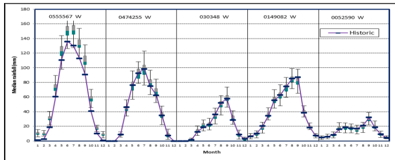
Figure 4.27a Box plots of monthly median rainfalls for stations 0555567 W, 0474255 W, 030348 W, 0149082 W and 0052590 W from EMD-VLB generator
