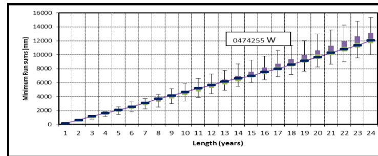
Figure 4.7a Box plots of minimum run sums for station 0474255 W from EMD-VLB generator
