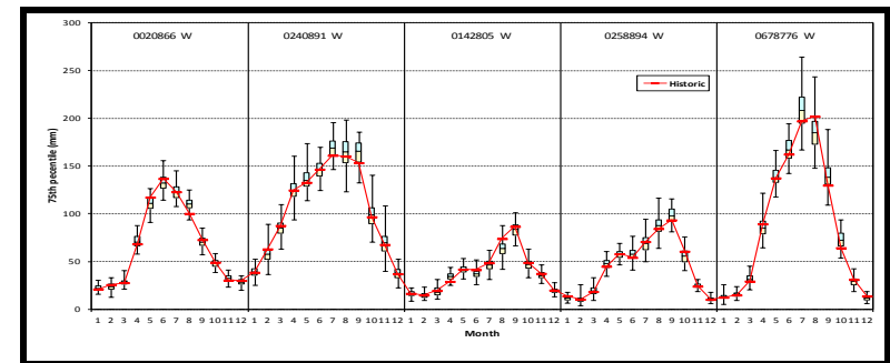
Figure 4.32b Box plots of monthly 75 th percentile rainfalls for stations 0020866 W, 0240891 W, 0142805 W, 0258894 W and 0678776 W from VLB generator
