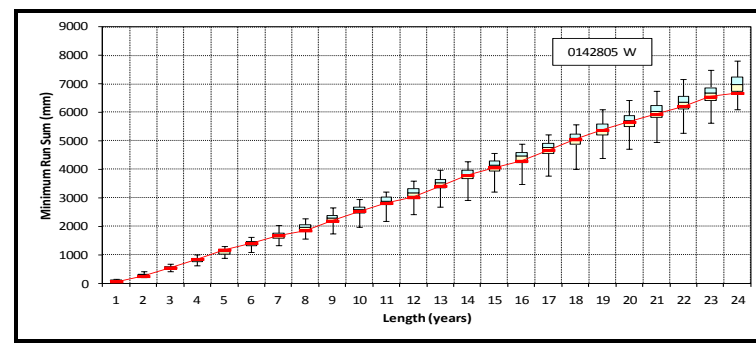
Figure 4.13b Box plots of minimum run sums for station 0142805 W from VLB generator
