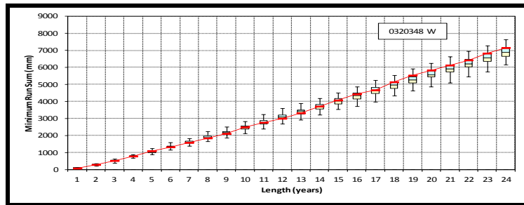
Figure 4.8b Box plots of minimum run sums for station 0320348 W from VLB generator
