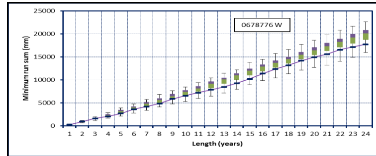
Figure 4.15a Box plots of minimum run sums for station 0678776 W from EMD-VLB generator
