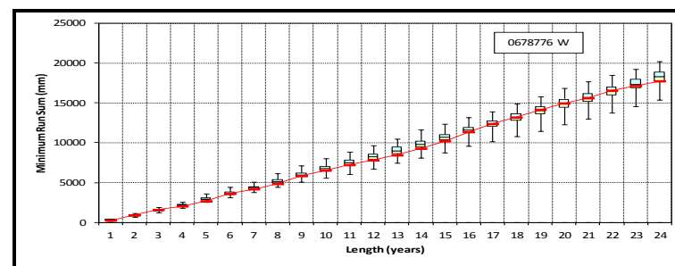
Figure 4.15b Box plots of minimum run sums for station 0678776 W from VLB generator
