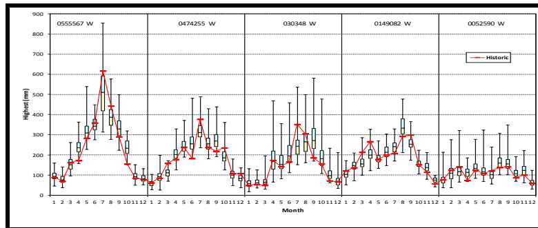
Figure 4.35b Box plots of monthly highest rainfalls for stations 0555567 W, 0474255 W, 030348 W, 0149082 W and 0052590 W from VLB generator
