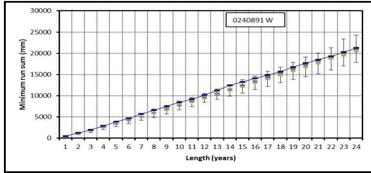
Figure 4.12a Box plots of minimum run sums for station 0240891 W from EMD-VLB generator
