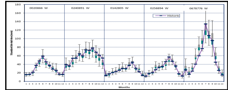
Figure 4.38a Box plots of monthly standard deviations for stations 0020866 W, 0240891 W, 0142805 W, 0258894 W and 0678776 W from EMD-VLB generator
