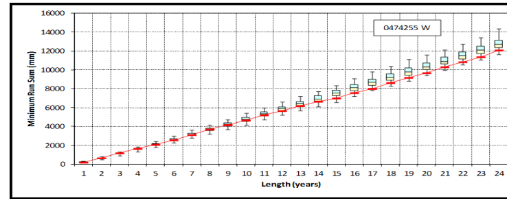
Figure 4.7b Box plots of minimum run sums for station 0474255 W from VLB generator
