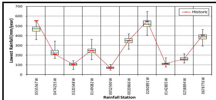
Figure 4.20b Box plots of lowest annual rainfalls from VLB generator
