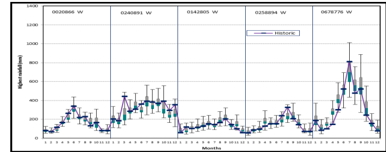
Figure 4.36a Box plots of monthly highest rainfalls for stations 0020866 W, 0240891 W, 0142805 W, 0258894 W and 0678776 W from EMD-VLB generator
