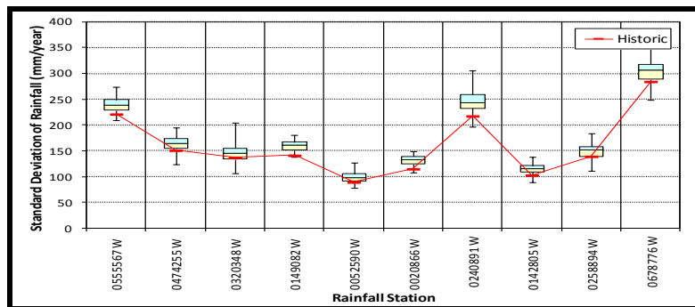
Figure 4.22b Box plots of standard deviation of annual rainfall from VLB generator
