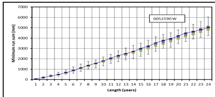
Figure 4.10a Box plots of minimum run sums for station 0052590 W from EMD-VLB generator
