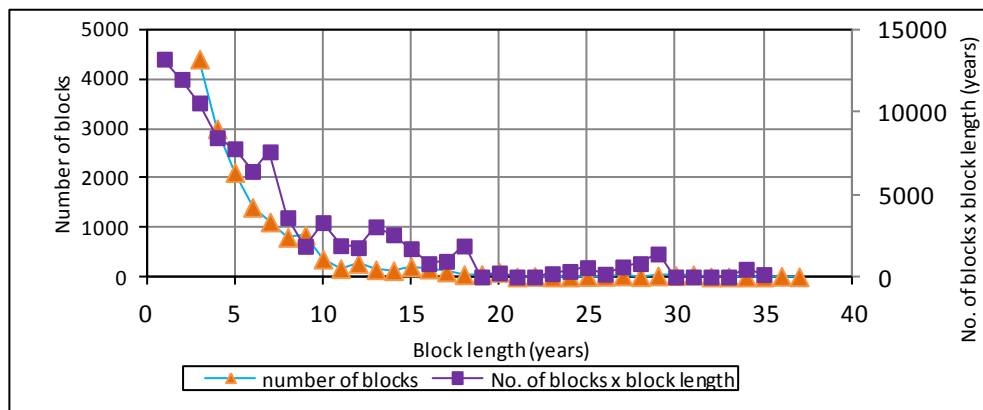
Figure 4.2 Number of blocks generated and the total length of blocks of specified length from the VLB generator.
