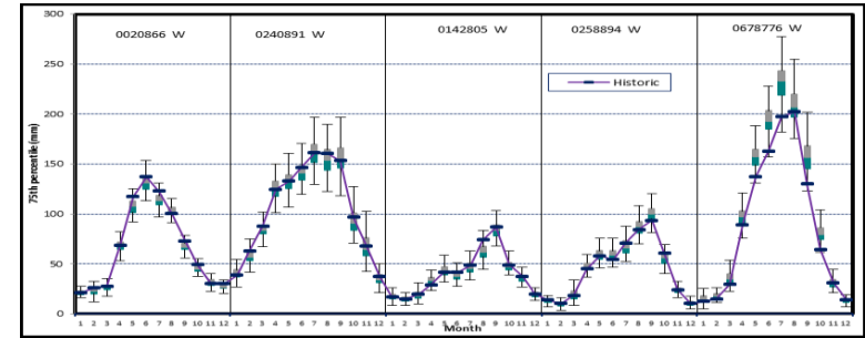
Figure 4.32a Box plots of monthly 75 th percentile rainfalls for stations 0020866 W, 0240891 W, 0142805 W, 0258894 W and 0678776 W from EMD-VLB generator
