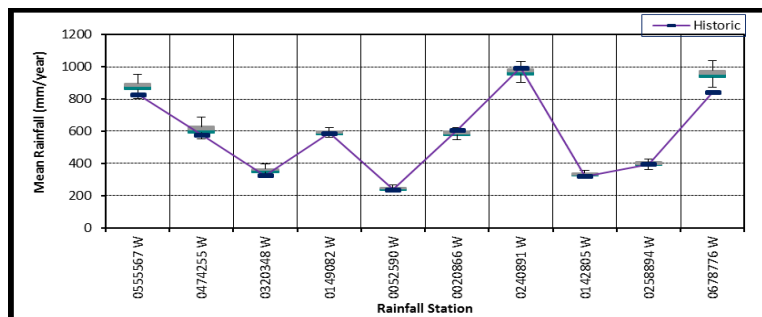
Figure 4.16a Box plots of annual mean rainfall from EMD-VLB generator
