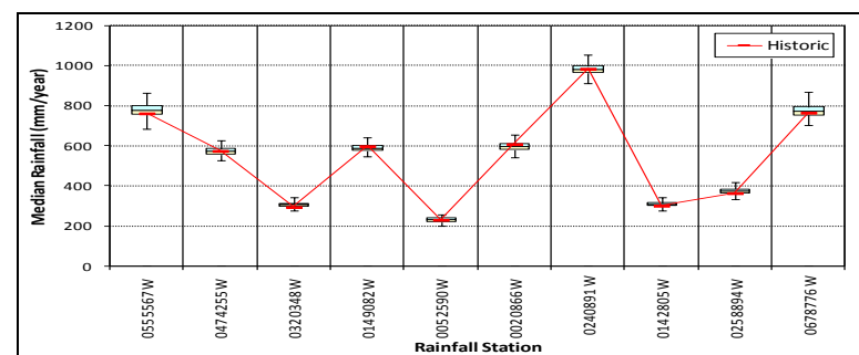
Figure 4.17b Box plots of annual median rainfall from VLB generator
