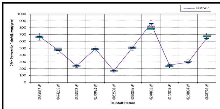
Figure 4.18a Box plots of annual 25 th percentile rainfalls from EMD-VLB generator
