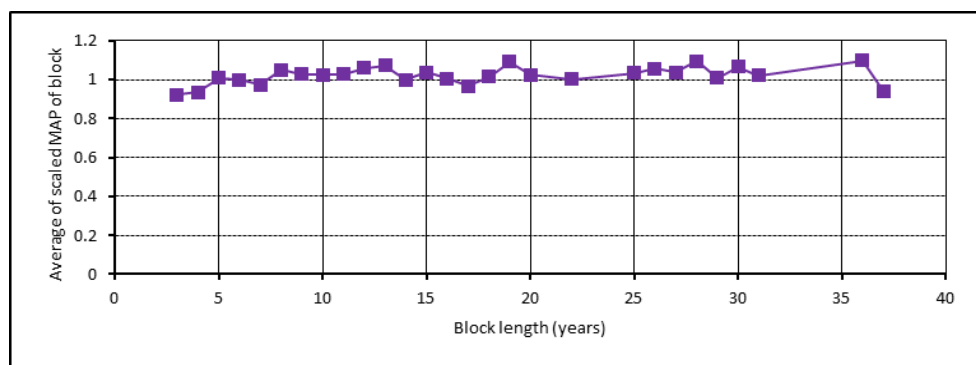
Figure 4.4 Scale average MAP of rainfall from the VLB generator.
