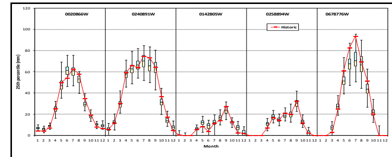
Figure 4.30b Box plots of monthly 25 th percentile rainfalls for stations 0020866 W, 0240891 W, 0142805 W, 0258894 W and 0678776 W from VLB generator
