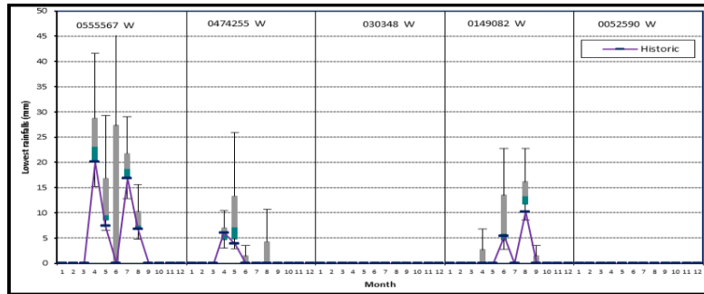
Figure 4.33a Box plots of monthly lowest rainfalls for stations 0555567 W, 0474255 W, 030348 W, 0149082 W and 0052590 W from EMD-VLB generator
