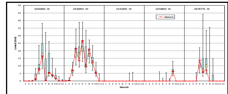
Figure 4.34b Box plots of monthly lowest rainfalls for stations 0020866 W, 0240891 W, 0142805 W, 0258894 W and 0678776 W from VLB generator
