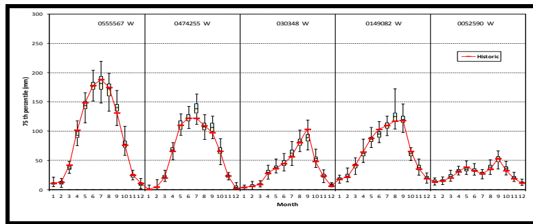
Figure 4.31b Box plots of monthly 75 th percentile rainfalls for stations 0555567 W, 0474255 W, 030348 W, 0149082 W and 0052590 W from VLB generator
