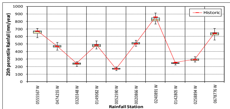
Figure 4.18b Box plots of annual 25 th percentile rainfalls from VLB generator
