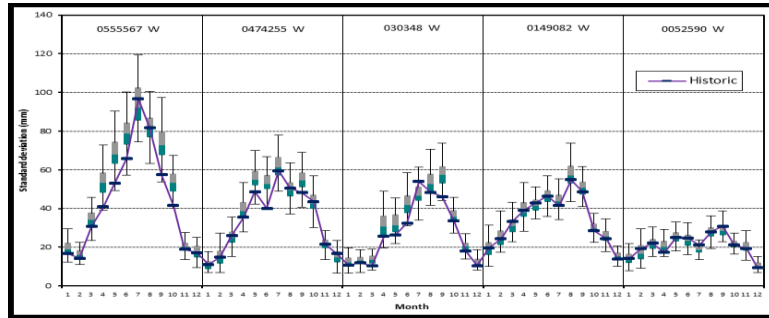
Figure 4.37a Box plots of monthly standard deviations for stations 0555567 W, 0474255 W, 030348 W, 0149082 W and 0052590 W from EMD-VLB generator
