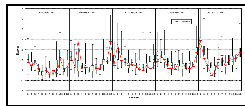
Figure 4.40b Box plots of monthly skewness for stations 0020866 W, 0240891 W, 0142805 W, 0258894 W and 0678776 W from VLB generator
