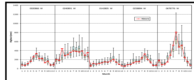
Figure 4.36b Box plots of monthly highest rainfalls for stations 0020866 W, 0240891 W, 0142805 W, 0258894 W and 0678776 W from VLB generator
