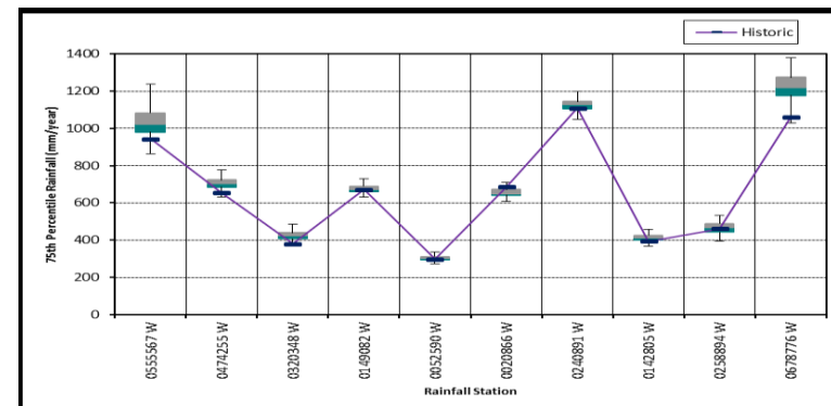
Figure 4.19a Box plots of annual 75 th percentile rainfalls from EMD-VLB generator
