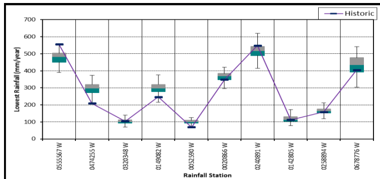
Figure 4.20a Box plots of lowest annual rainfalls from EMD-VLB generator
