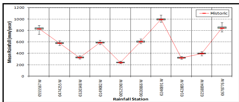
Figure 4.16b Box plots of annual mean rainfall from VLB generator
