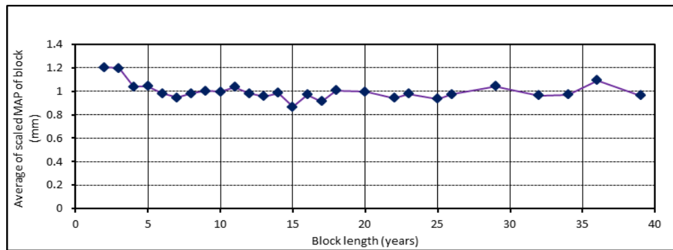
Figure 4.3 Scale average MAP of rainfall from the EMD-VLB generator.
