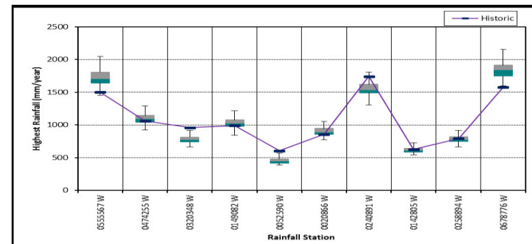
Figure 4.21a Box plots of highest annual rainfalls from EMD-VLB generator
