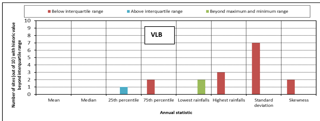
Figure 4.24 The number of times historic statistics fall beyond interquartile ranges of the box plots of stochastic sequences of the EMD-VLB and VLB generator.
