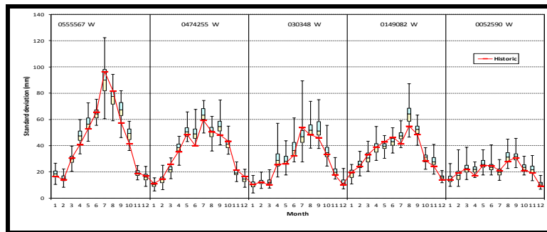
Figure 4.37b Box plots of monthly standard deviations for stations 0555567 W, 0474255 W, 030348 W, 0149082 W and 0052590 W from VLB generator
