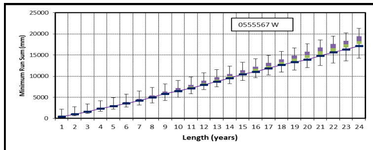
Figure 4.6a Box plots of minimum run sums for station 0555567 W from EMD-VLB generator
