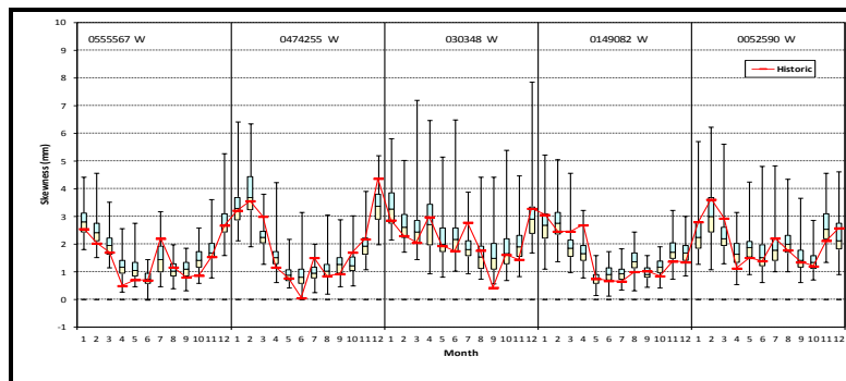
Figure 4.39b Box plots of monthly skewness of rainfalls for stations 0555567 W, 0474255 W, 030348 W, 0149082 W and 0052590 W from VLB generator
