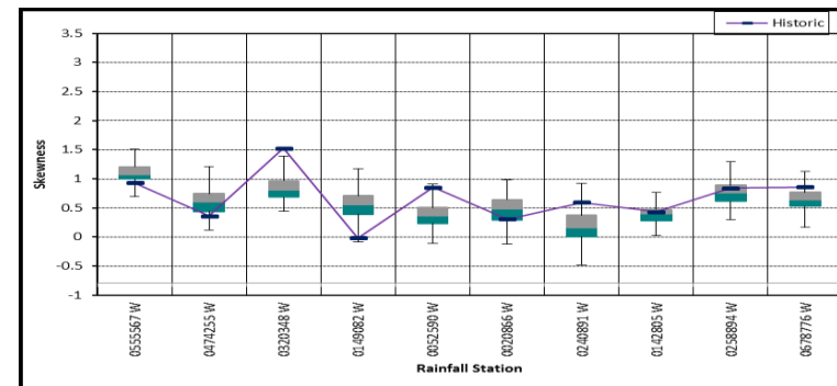
Figure 4.23a Box plots of skewness of annual rainfalls from EMD-VLB generator
