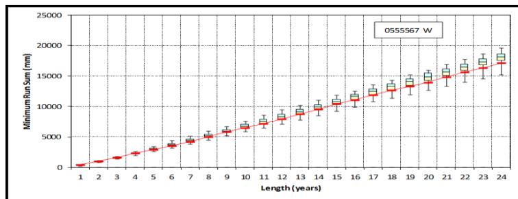
Figure 4.6b Box plots of minimum run sums for station 0555567 W from VLB generator
