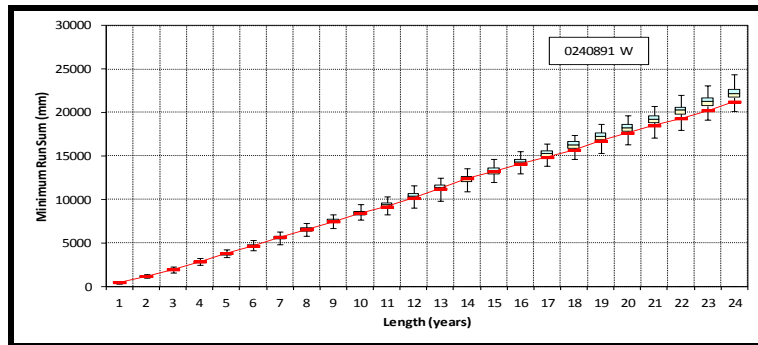
Figure 4.12 b Box plots of minimum run sums for station 0240891 W from VLB generator
