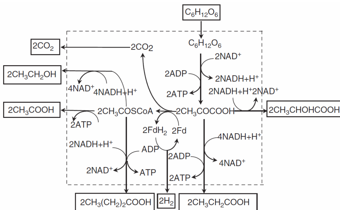
Figure 1.2. Summary of glucose fermentation pathways that can be engaged with hydrogen production optimised when the system is driven towards acetic acid generation (Ren et al. , 2006).
