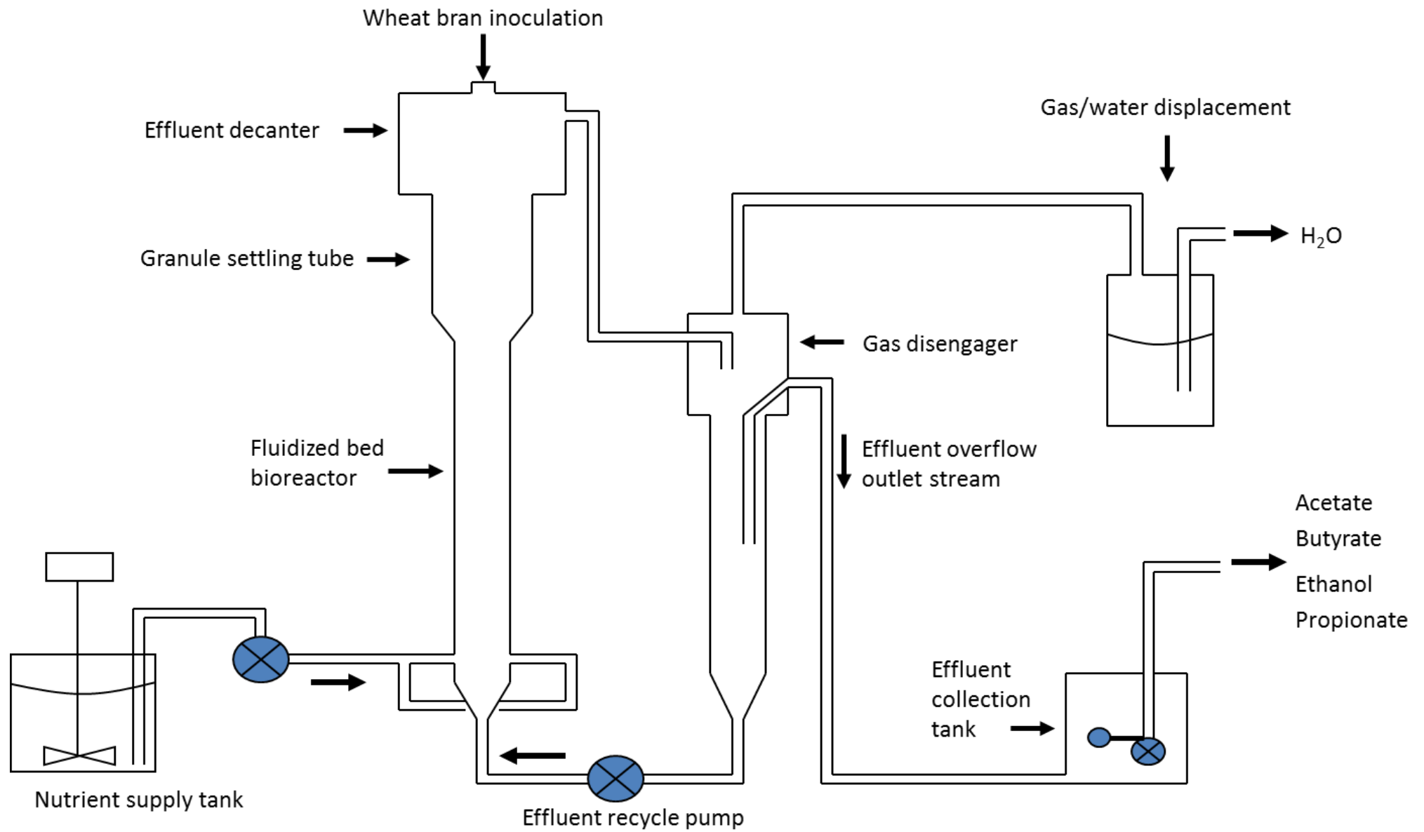
Figure 2.1. Diagrammatic representation of the bioreactor system showing inorganic nutrient supply, the primary bioreactor column, the gas/liquid disengager column, recycle pump and an effluent collection tank. Total gas production was measured via the gas/water displacement bottle. The principal metabolic by-products of the fermentation process are also shown.
