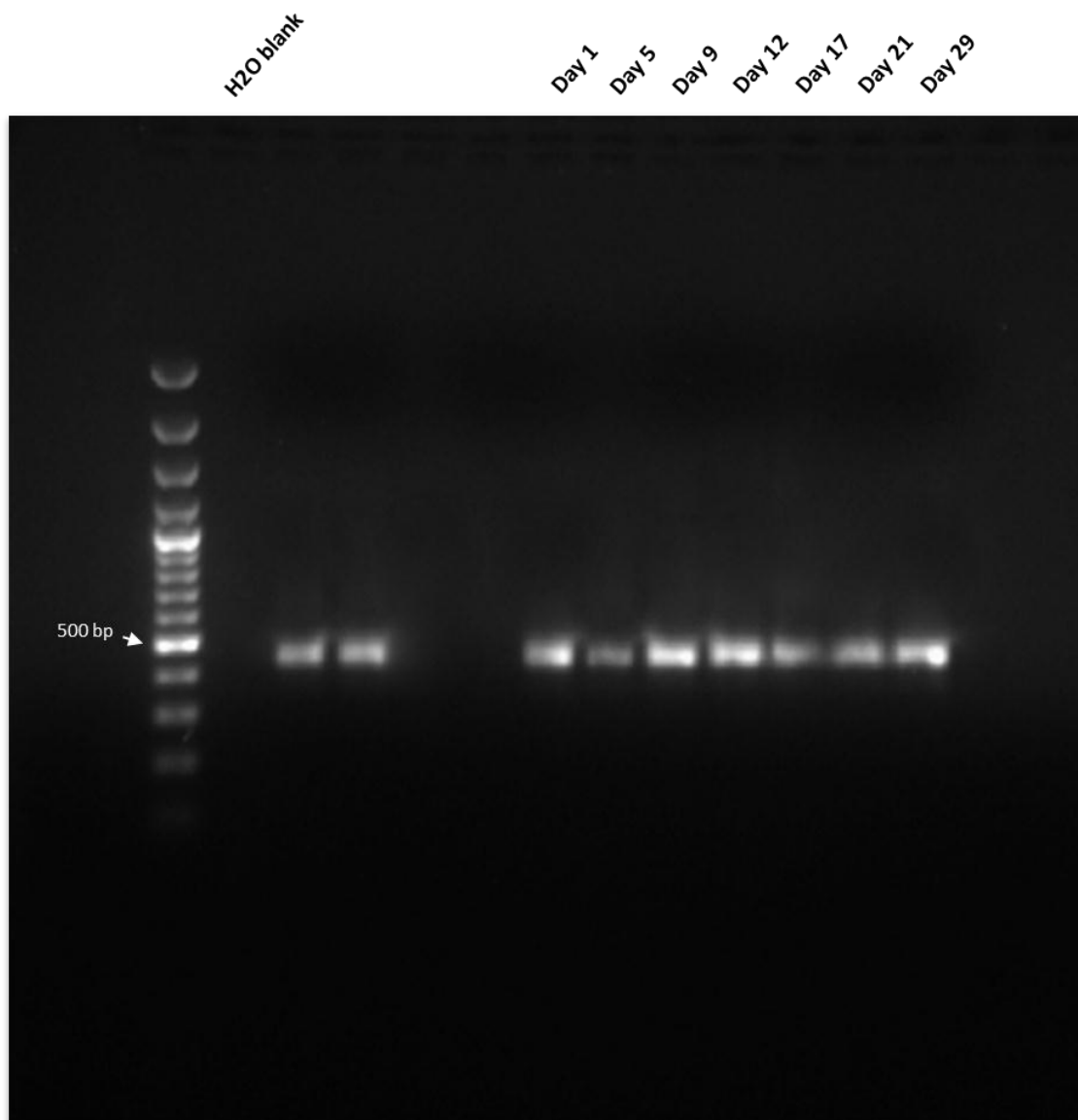
Figure 3.2. Agarose gel electrophoresis of successfully amplified 16S rDNA fragments (460 – 500 bp) obtained from DNA of samples on the respective days (labelled). Lane 1 showing a water blank indicating no contamination during the reaction. The unlabelled lanes containing amplified products were a confirmation of a previous amplification reaction.
