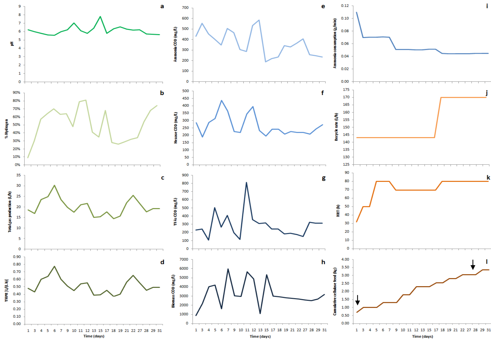
Figure 3.1. Time course profiles of parameter data obtained during bioreactor operation. (a) pH; (b) H 2 percentage of (c) total gas production; (d) VHPR; (e-h) COD concentrations for ammonia, hexoses, VFAs and biomass respectively; (i) ammonia consumption; (j) bioreactor recycle rate; (k) HRT; and (l) cumulative cellulose feed with arrows indicating sucrose addition.
