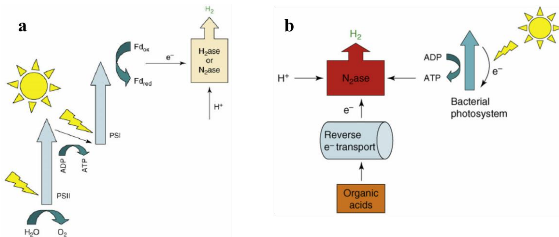
Figure 1.1. (a) Biophotolysis occurring in a photosynthetic system, depicted are photosystems I and II (PSI and PSII), the electron carrier, ferredoxin (Fd) and the hydrogen-evolving enzymes, hydrogenase and nitrogenase ( H_2ase and N_2ase ) (b) The photofermentation process whereby organic acids act as electron donors, which follows reverse electron transport and together with ATP generated by light energy, nitrogenase reduces the proton to hydrogen (Hallenbeck and Ghosh, 2009).
