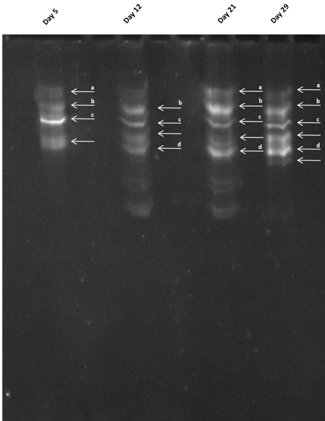
Figure 3.3. Polyacrylamide gel electrophoresis of a denaturing gradient electrophoresis performed on the PCR samples depicted. Arrows indicate distinct 16S rDNA fragments belonging to bacteria that were prevalent in the AFBR, while the letters (a-d) correspond to common bands on the respective sampling days. Day 5 shows a clearly dominant bacterial species. Faint bands are visible further down along the lanes of sample Day 12, Day 21 and Day 29, with a diminishing concentration in each, thus these were excluded from analysis.
