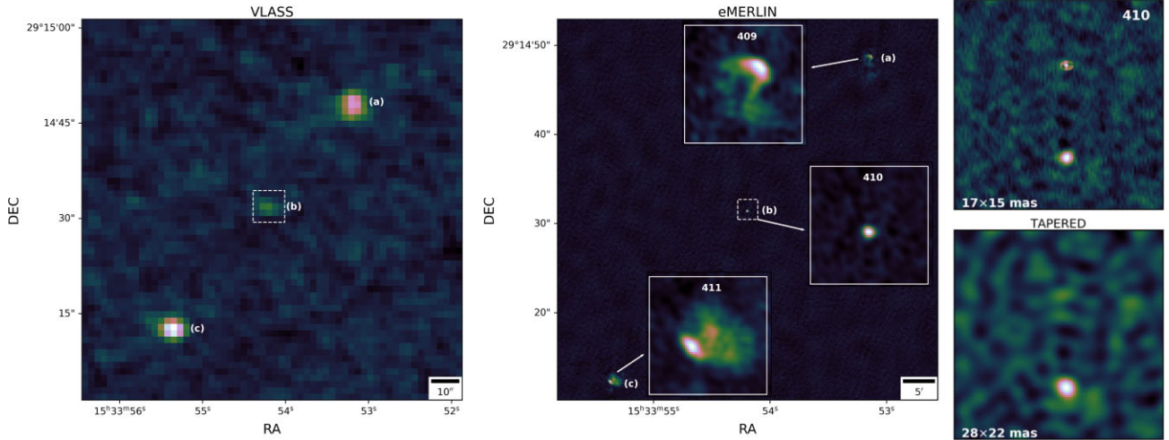
Figure 8. The source J153354+291431 shows two bright compact cores on the VLBI image (NOTAPER and TAPERED), which are located within a double-lobed structure indicating the presence of highly collimated radio jet structures at galactic scales in both the VLASS and the e -MERLIN images. The VLASS image shows three unresolved sources at (a), (b), and (c) which correspond to three e -MERLIN sources (PC 409, 410, and 411, respectively). Whereas the source at point (b) remains faint and compact in e -MERLIN, the sources at points (a) and (c) are resolved out revealing extended radio emissions with edge-brightened outer lobes showing some hot spots. The faint component (b) is coincident with the centre of the host galaxy in both VLASS and e -MERLIN. On the other hand, VLBI completely resolves out these outer lobes and hotspots, but only partially resolves the faint component (b) to reveal two bright compact cores in the notaper image. These two VLBI cores are separated by \sim 130 mas corresponding to \sim 1.1 kpc, which is well within the 2.5 kpc orbital separations between paired supermassive black holes proposed by Burke-Spolaor (2011). The fainter (northern core) is detected at \sim 5.5\sigma and the brightest (southern core) is detected at \sim 18.4\sigma . In the tapered image, the fainter northern core remains undetected, whereas the brighter southern core is detected at 14.7\sigma . The distance between the two lobes in e -MERLIN is \sim 46'' , translating to a linear size of \sim 0.4 Mpc, assuming z \sim 1.25 .
