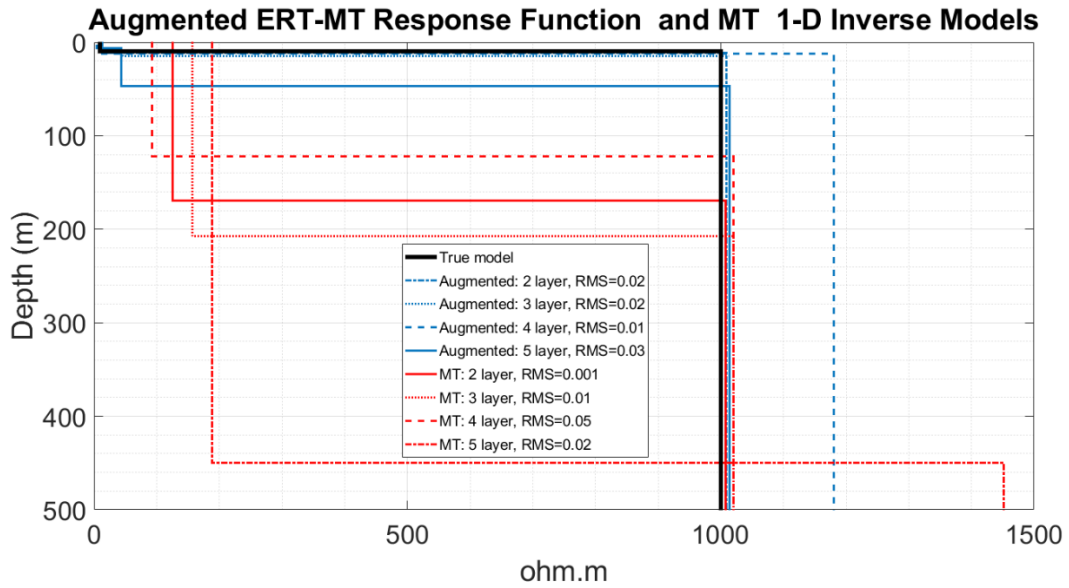
Figure 4.5. Augmented ERT-MT response function (blue to purple) and MT (red to yellow) 1-D resistivity inverse models. The true resistivity model is represented by a black line. The augmented ERT-MT response function resulted in a 1-D inverse models that depicts an improvement of up to ~91% in recovering the true resistivity model.
