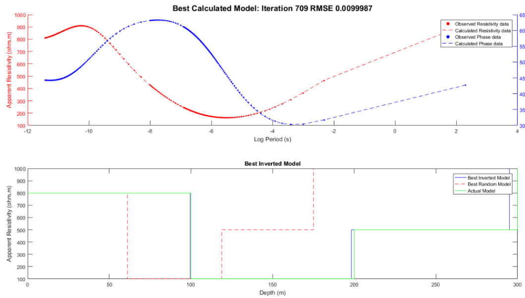
Figure 2.23. A 1-D MT inverse model calculated using the algorithm developed in this thesis (Appendix A.2.). The green line represents the actual resistivity model, the red dashed line is the starting model calculated from the Monte Carlo simulations and the blue line is the lowest root mean square resistivity inverse model.
