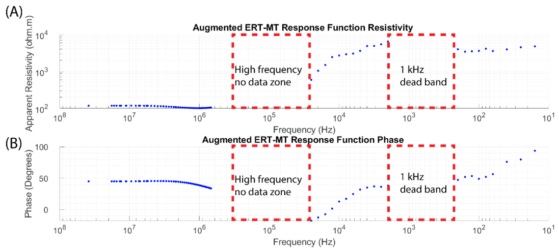
Figure 4.19. (A) Edited augmented ERT-MT response function resistivity data. (B) Edited augmented ERT-MT response function phase data.
