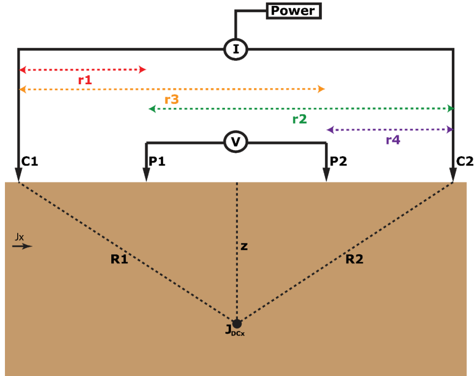
Figure 4.1. Sketch of a typical ERT array. C1 and C2 are current electrodes while P1 and P2 are potential electrodes. The distance between current electrodes and potential electrodes is represented as distances r_1 , r_2 , r_3 and r_4 respectively. J_x is the current density in the horizontal direction. J_{DCx} is the horizontal current density measured at that point, with a depth of z and distance R_1 and R_2 away from current electrodes C1 and C2 respectively.
