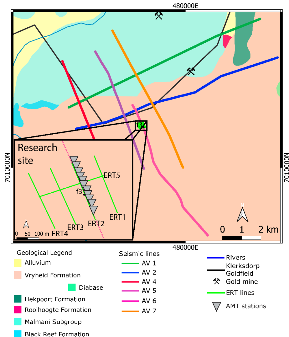
Figure 5.8. A geological map showing the planned survey site targeting low-velocity zones mapped in the P-wave seismic tomography inverse model. We collected data from 5 electrical resistivity tomography survey lines, 11 audio magnetotelluric stations, and 15 magnetic survey lines. Seismic line AV 6 runs through the center of our research site.
