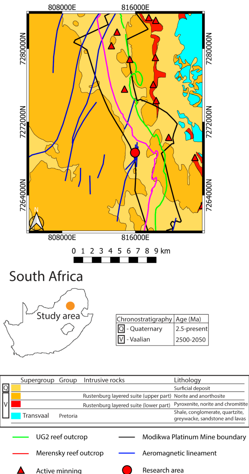
Figure 4.12. Regional geology map showing the ERT and MT survey site as a red circle and the dark blue lines represent aeromagnetic lineaments interpreted as a dyke swarm in the area (modified from Steyn, 1990).
