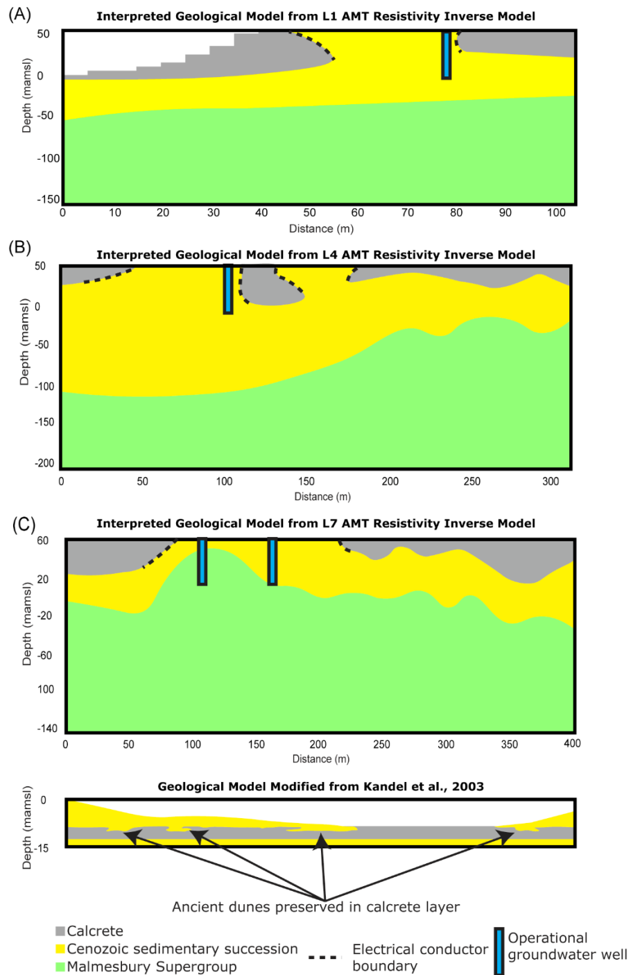
Figure 3.12. (A) Geological model interpreted from resistivity inverse model calculated from AMT line L1. (B) Geological model interpreted from resistivity inverse model calculated from AMT line L4. (C) Geological model interpreted from resistivity inverse model calculated from AMT line L7. (A) Geological model modified from Kandel et al. (2003), showing ancient dunes preserved in the calcrete layer near the Yzerfontein–Geelbek dune cordon. The breaks in the calcrete layer seen in all the resistivity inverse models resemble the same breaks in the Kandel et al. (2003) geological model. Therefore, the breaks in the calcrete in our study area are likely as a result of preserved ancient dune fields.
