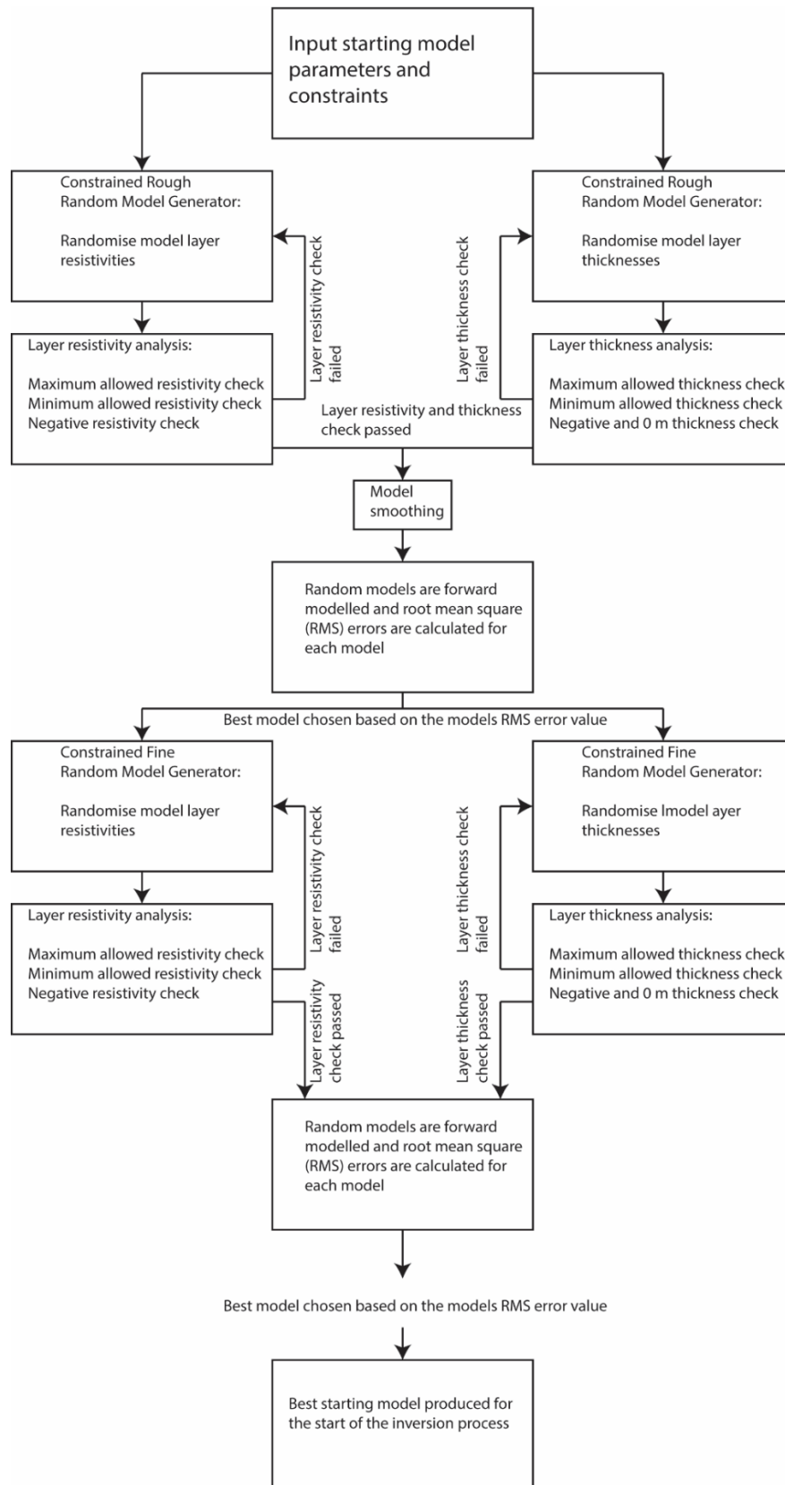
Figure 2.21. Algorithm workflow map for the Monte Carlo random model generators
