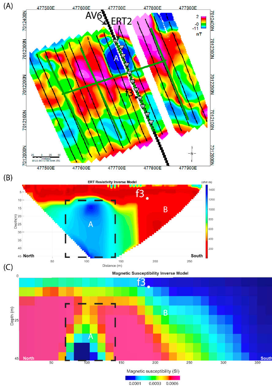
Figure 5.11. (A) Reduced and leveled magnetic map with black dots representing the magnetic readings collected along the survey lines. Green lines show the position of the ERT lines and 11 audio magnetotelluric stations are shown as grey triangles. Black squares show the receiver positions for a portion of seismic line AV 6. (B) Resistivity inverse model for ERT2, with a root mean square error of 5. The resistive dolomites ( \sim 800 \Omega \cdot \text{m} ) are discontinued \sim 170 \text{ m} along the profile by a conductor ( \sim 100 \Omega \cdot \text{m} ) interpreted as a fault zone, labeled B. A vertical resistor ( 1200\text{--}1400 \Omega \cdot \text{m} ), labeled A, \sim 60\text{--}150 \text{ m} along the profile, is situated in the same location as the inferred cavity mapped on the reduced and leveled magnetic map. (C) 3-D Magnetic susceptibility inverse model slice along survey line ERT2. Both the position of the low susceptibility ( \sim 0.0001 ) fault zone and the inferred cavity match the position seen in the resistivity inverse model for the same line.
