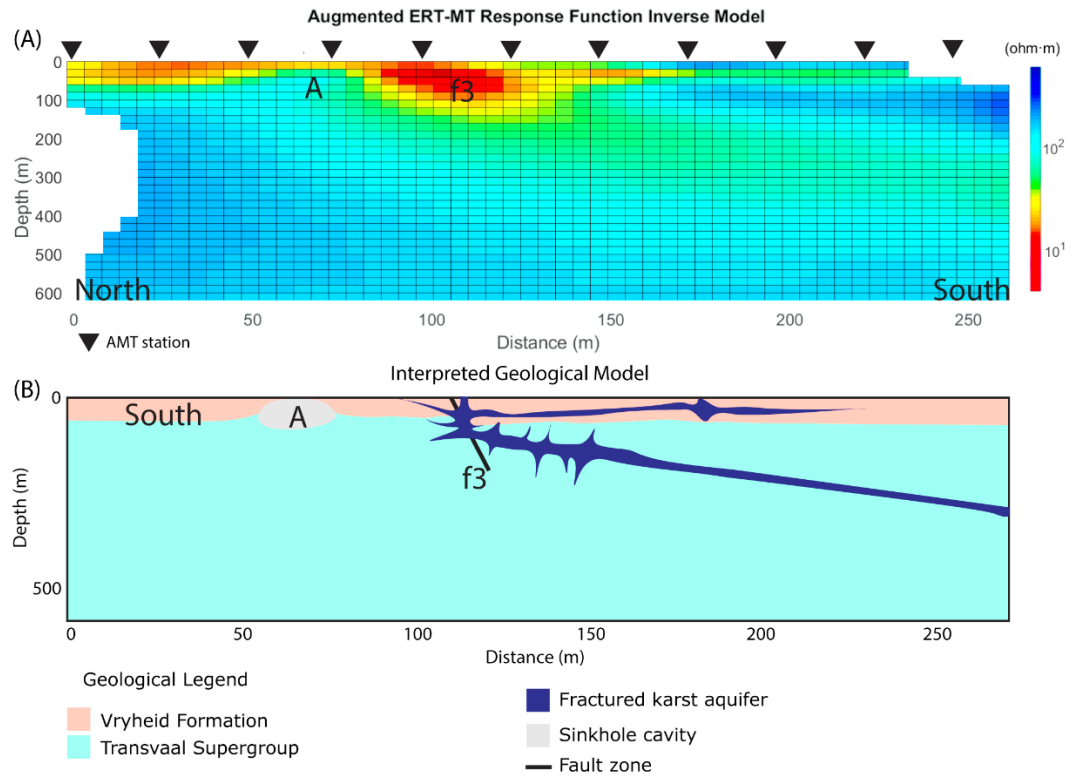
Figure 5.14. (A) Augmented ERT-MT response function resistivity inverse model along survey line ERT2. The white cells in this model represent cells with low confidence calculated from the model confidence assessment algorithm. (B) A geological model interpreted from the augmented ERT-MT response function resistivity inverse model along survey line ERT2. The fractured karst aquifer is confined between ~100-400 m deep. A inferred cavity is interpreted at position A.
