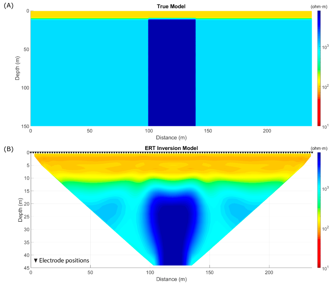
Figure 4.9. (A) True resistivity model with a conductive (100 \Omega\cdot\text{m} ) overburden to a depth of 10 m and an underlying resistive (8000 \Omega\cdot\text{m} ) dyke embedded in a 1000 \Omega\cdot\text{m} half-space. (B) ERT inverse model with an RMSE of 0.3. The resistive dyke and the conductive overburden is recovered in the inverse model.
