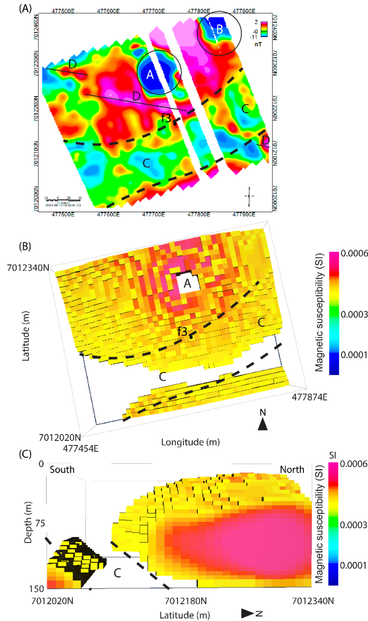
Figure 5.10. (A) Reduced and leveled magnetic map. Positions A and B show two negative magnetic intensity ( \sim -11 nT) zones. Zone C, marked by the black stippled line, offsets the positive magnetic intensity lineament marked as D. Position f3 shows the location of the low velocity zone seen along P-wave seismic tomography inverse model for seismic line AV 6. (B) A top down view of the magnetic susceptibility inverse model calculated from the reduced and leveled residual magnetic grid. An isovolume of susceptibilities between 0.0004 and 0.0006 SI shows a 'break' in the dolomites in the area labeled C. The residual negative magnetic intensity ( \sim -11 nT) zone at position A, correlates with a cavity in the dolomites at that same position in the magnetic susceptibility inverse model. (C) Easterly side view of the magnetic susceptibility inverse model. An isovolume of susceptibilities between 0.0004 and 0.0006 SI shows a drop in depth in the dolomites from \sim 15 m to \sim 110 m deep in the area labeled C.
