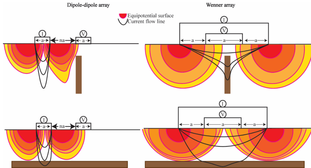
Figure 2.17: A dipole-dipole and Wenner array equipotential surface interaction comparison for both vertical and horizontal conductive geological structures represented by the brown rectangles, the black line represent current flow lines (modified from Dentith and Mudge, 2014).
