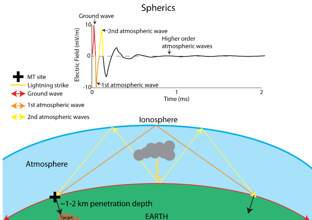
Figure 2.4. Lightning storms near the equatorial regions generate electromagnetic fields, known as spherics, that travel along a wave guide between the Earth's surface and the ionosphere. These electromagnetic fields are the main source field for magnetotelluric signal > 1Hz. The electromagnetic fields are vertically incident plane waves at the Earth's surface and propagate through the Earth to ~2 km deep.
