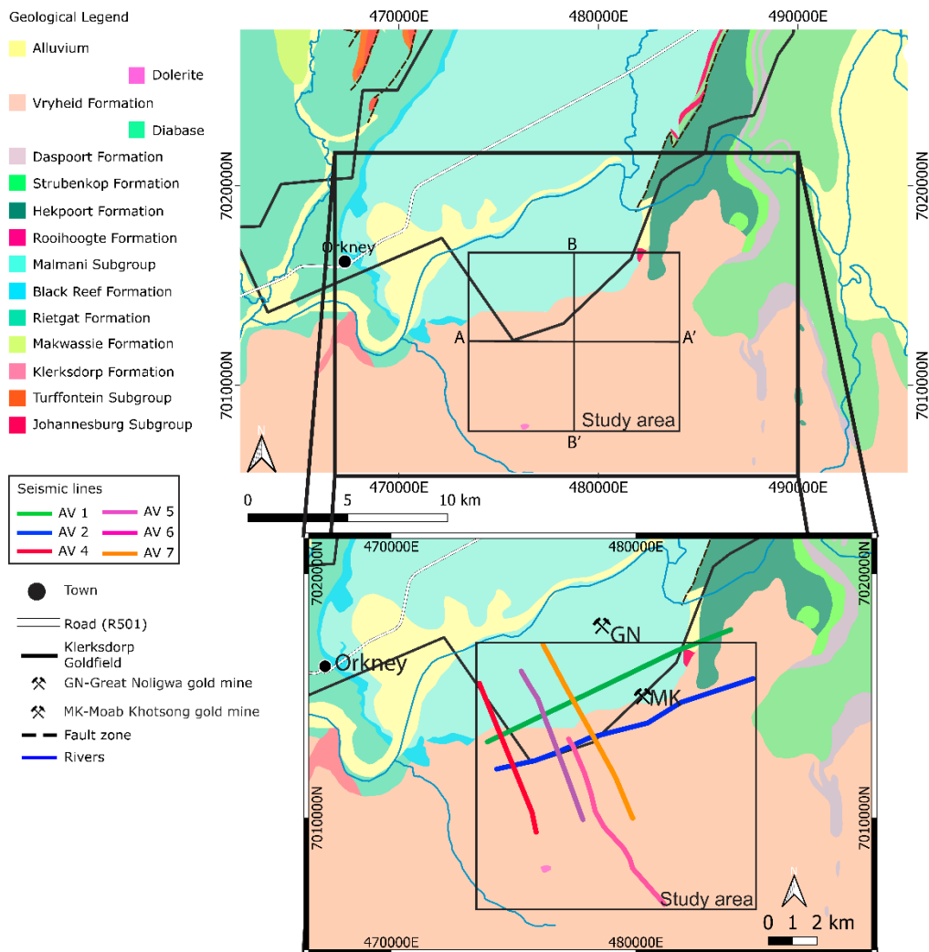
Figure 5.2. Geological map (modified from the following maps sheets, Wilkinson, K.J., and Coetsee, F., 1986; Retief, P.F., 2000) with seismic line positions collected by Gold Division of the Anglo-American Corporation in 1983.
