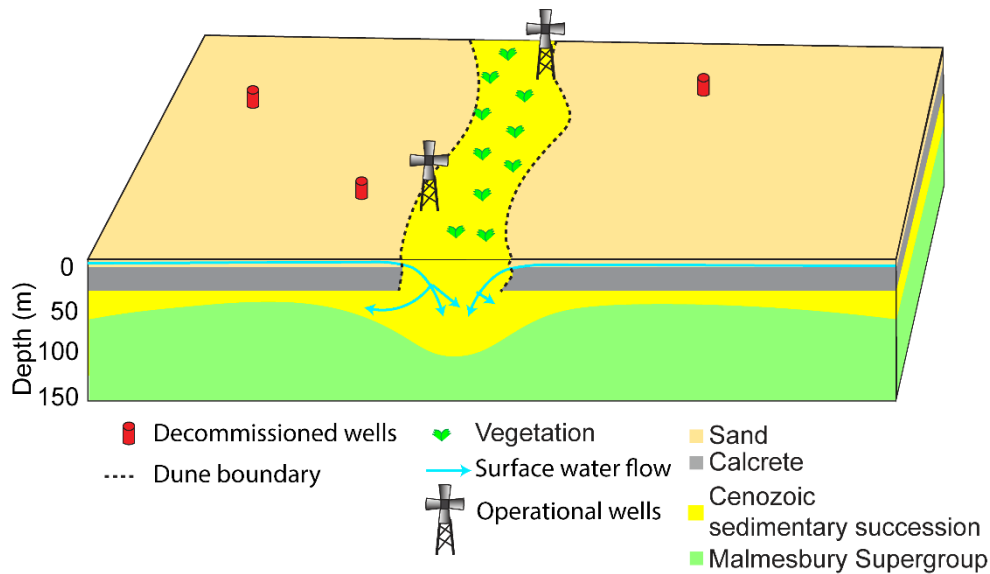
Figure 3.15. The proposed geological model interpreted from both the resistivity and magnetic susceptibility inverse models. Groundwater infiltrates the Cenozoic sedimentary succession through preserved ancient dune outcrops by disrupting the calcrete and clay aquitard above.
