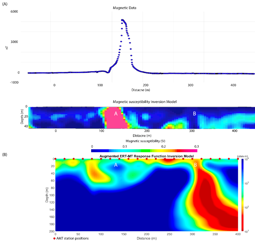
Figure 4.24. (A) A slice from the magnetic susceptibility inverse model along the AMT line shows the magnetic dyke, labeled “A”, and the north-south fault, labeled “B”. (B) The resistivity inverse model, calculated from the augmented ERT-MT response function, shows that both the dyke and the fault zone in both inverse models line up.
