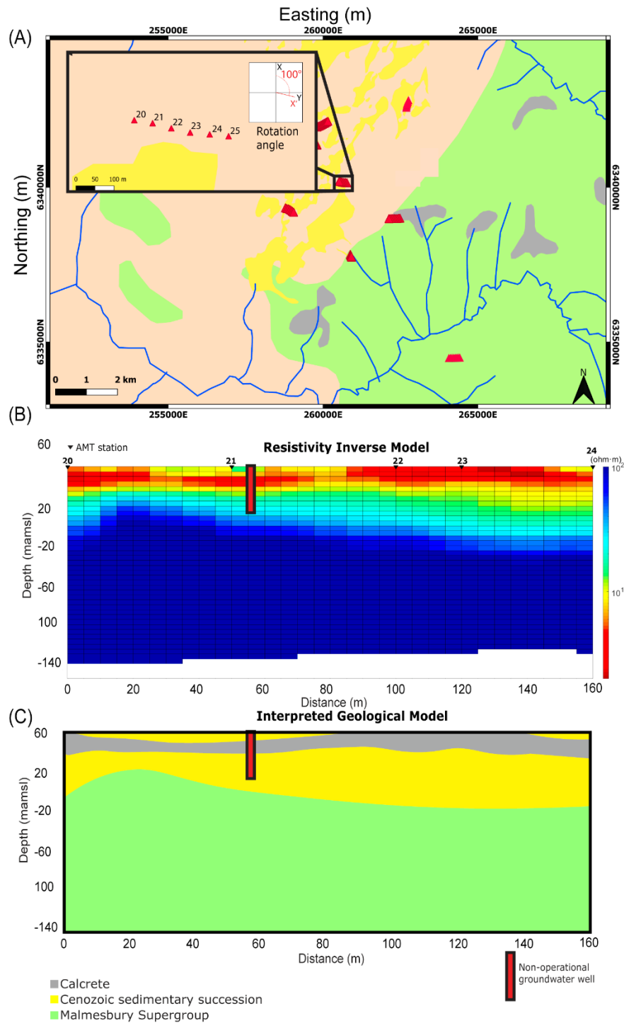
Figure 3.10. (A) The location of the 6 AMT stations, along L5, used in the resistivity inverse model is shown on this map. The rotation angle for these stations is 100^\circ . (B) The resistivity inverse model shows a continuous conductor at a depth of 55 mamsl. This conductor is interpreted as the clay and calcrete aquitard. White cells with low confidence are present below -140 mamsl. The root mean square error of the model is 1.6. (C) The geological model shows that the non-productive well intersects the aquifer below the aquitard but the groundwater conductivity in the aquifer is > \sim 2000 \mu\text{S/cm} .
