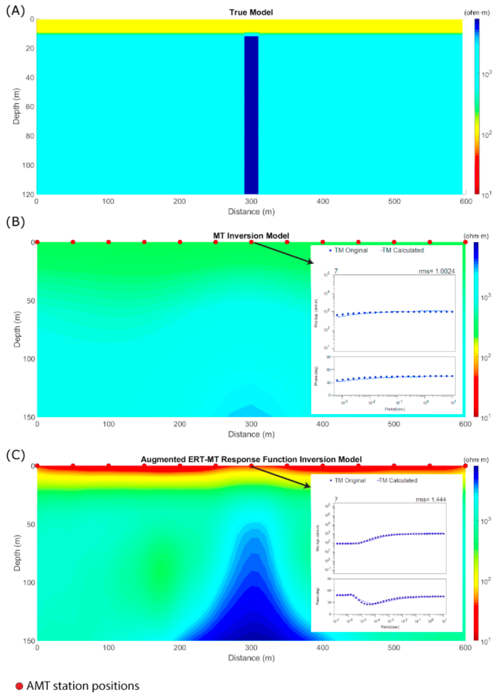
Figure 4.8. (A) True resistivity model that we are trying to recover has a conductive ( 100 \Omega\cdot\text{m} ) overburden, to a depth of 10 m, and an underlying resistive ( 8000 \Omega\cdot\text{m} ) dyke embedded in a 1000 \Omega\cdot\text{m} half-space. (B) Resistivity inverse model only using audio magnetotelluric data. A resistor is mapped at 300 m along the profile but is at a depth of ~150 m. The conductive overburden is absent from this model. The RMSE for this model is 0.6. (C) Resistivity inverse model using the augmented ERT-MT response function. A resistor is again mapped at 300 m along the profile but is constrained to ~100-200 m wide. Also, the conductive overburden is mapped in this inverse model to a depth of 10 m. The RMSE for this model is 0.5.
