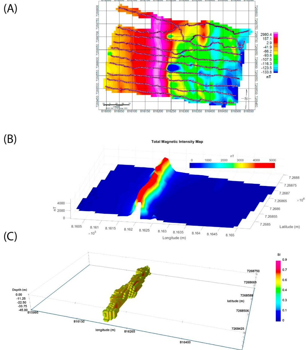
Figure 4.14. (A) Total magnetic intensity map of the magnetic data collected over the study area. White dots indicate actual magnetic readings from the magnetometer. (B) Total magnetic intensity observation data grid used for the 3-D magnetic susceptibility inverse model calculation. (C) The 3-D magnetic susceptibility inverse model shows a ~30 m wide dyke isovolume with a magnetic susceptibility of ~0.6 SI with a north-south strike in our study area.
