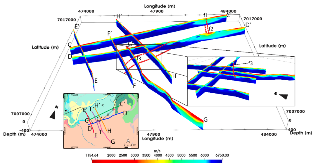
Figure 5.7. A three-dimensional spatial representation of all 6 seismic lines in our study area. Low velocity zones at Position f1 and f2 correspond with the fault continuation. The red line labeled f3 shows a low velocity zone propagating through P-wave seismic tomography inverse models associated with seismic lines AV 2, AV 5, AV 6 and AV 7.
