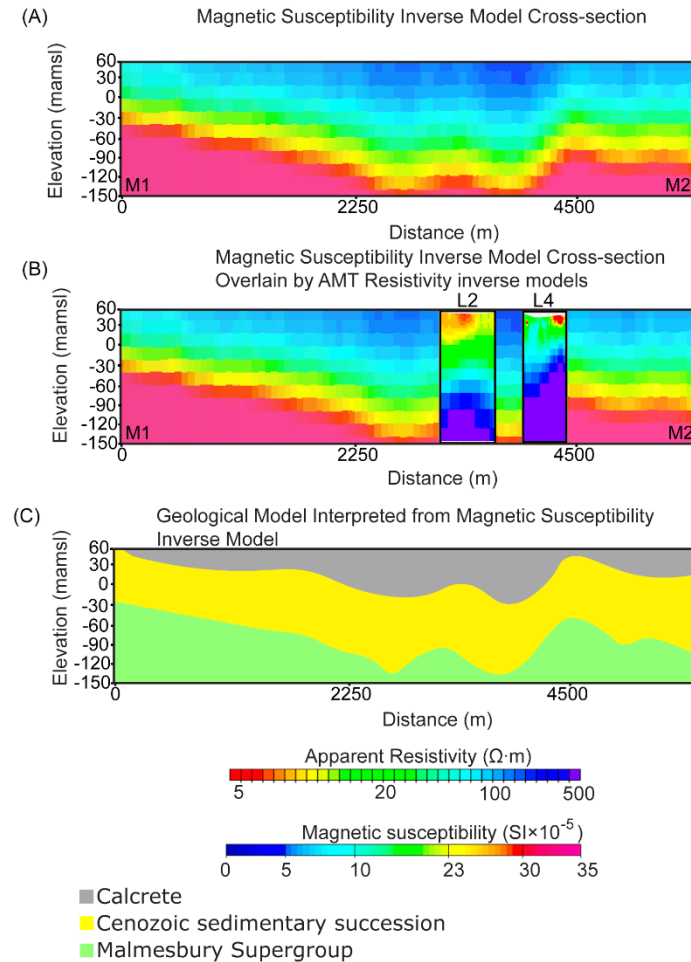
Figure 3.11. (A) A cross-section, along a traverse between M1 and M2, from the 3-D magnetic susceptibility inverse model. (B) Resistivity inverse models along lines L2 and L4 overlain on the magnetic susceptibility inverse model cross-section. The resistivity inverse models map the edges of inferred channels formed much later in Cenozoic times by exploiting possible minor synclinal folds in the basement Malmesbury Supergroup and correlate with the edges of channels seen in the basement Malmesbury Supergroup in the magnetic susceptibility inverse model. (C) The geological model interpreted from the magnetic susceptibility inverse model.
