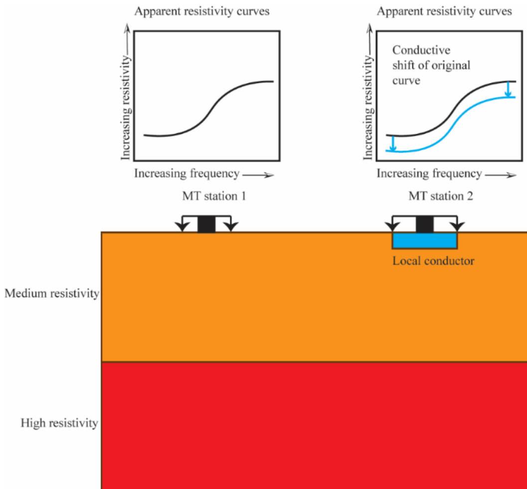
Figure 2.11: Example of the static shift effect over a local conductive body. Local near surface conductor shown in blue. The geological model consists of an upper medium resistive lithological layer, in orange, underlain by a highly resistive half-space, shown in red. The static shift effect is shown within the apparent resistivity curve plot.
