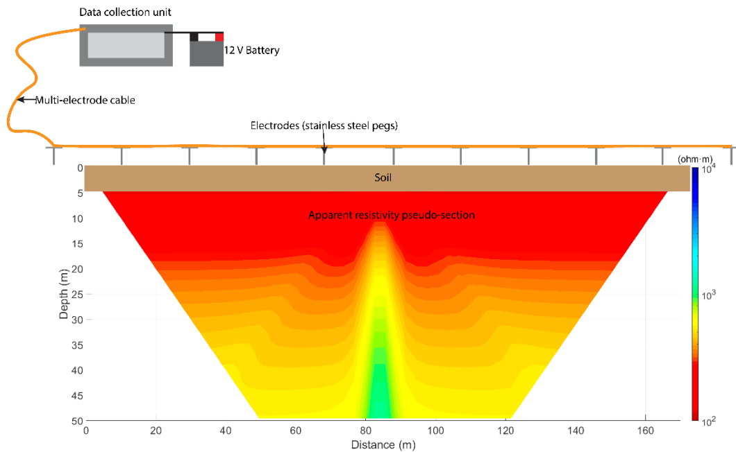
Figure 2.15: Sketch of a typical two-dimensional resistivity array setup. The potential difference between electrodes is used to calculate an apparent resistivity value as shown in the apparent resistivity pseudo-section.
