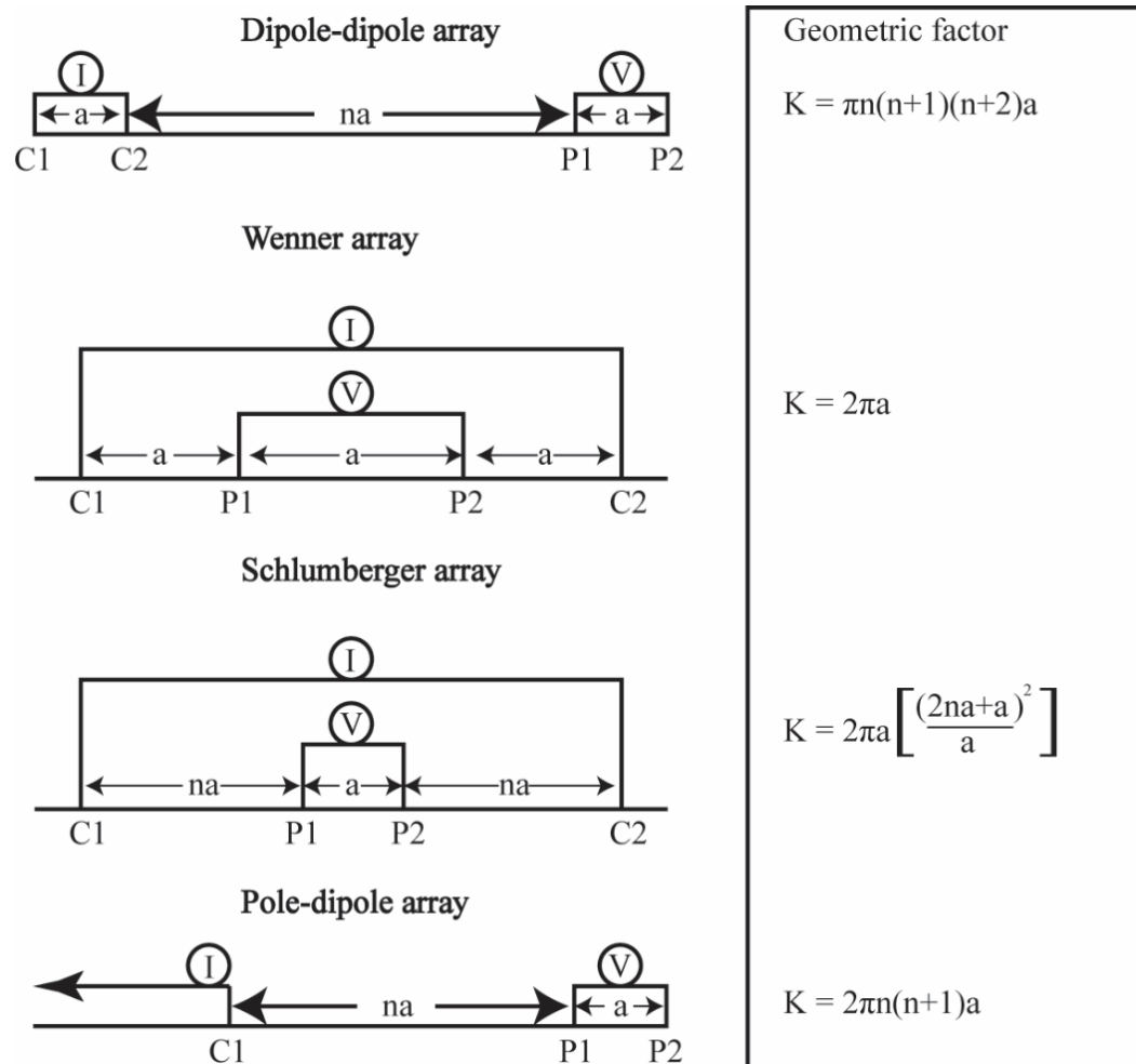
Figure 2.16: Common ERT configurations and corresponding geometric factors (modified from Dentith and Mudge, 2014). C represents current electrodes, P represents potential electrodes, a is the spacing between electrodes and n is a spacing modifier as the array is extended. I is the amp meter for the applied current and V is the voltmeter required for measuring the change in potential.
