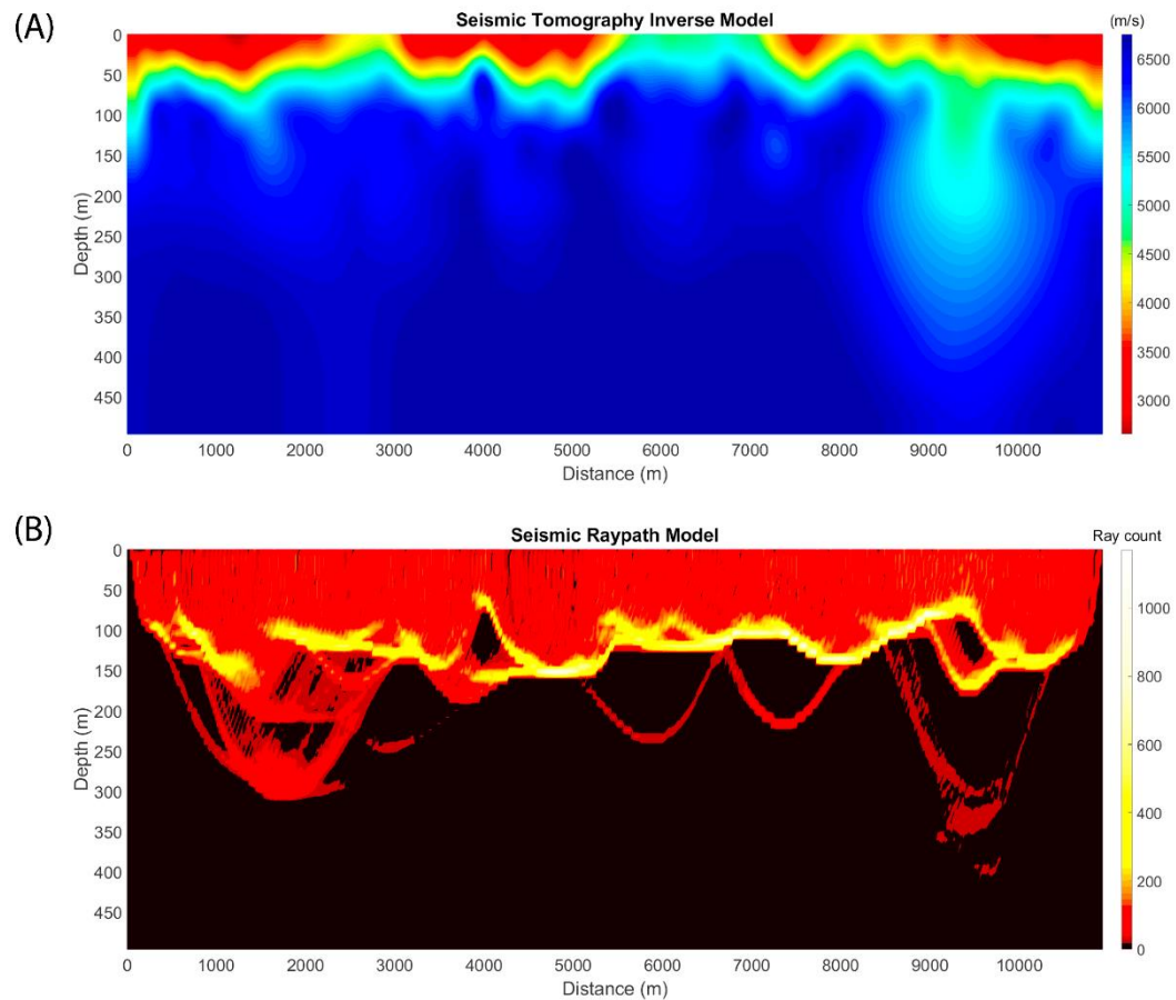
Figure 5.4. (A) P-wave seismic tomography inverse model of seismic line AV 1. The inverse model has a root mean square error of 6 ms. (B) The seismic ray paths raytraced through the velocity model. Black areas indicate zones with no ray traces.
