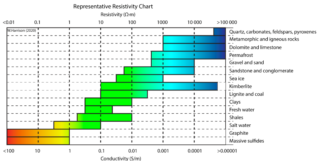
Figure 2.2. Resistivity chart for different materials (modified and consolidated after Palacky, 1987 and Dentith and Mudge, 2014).
