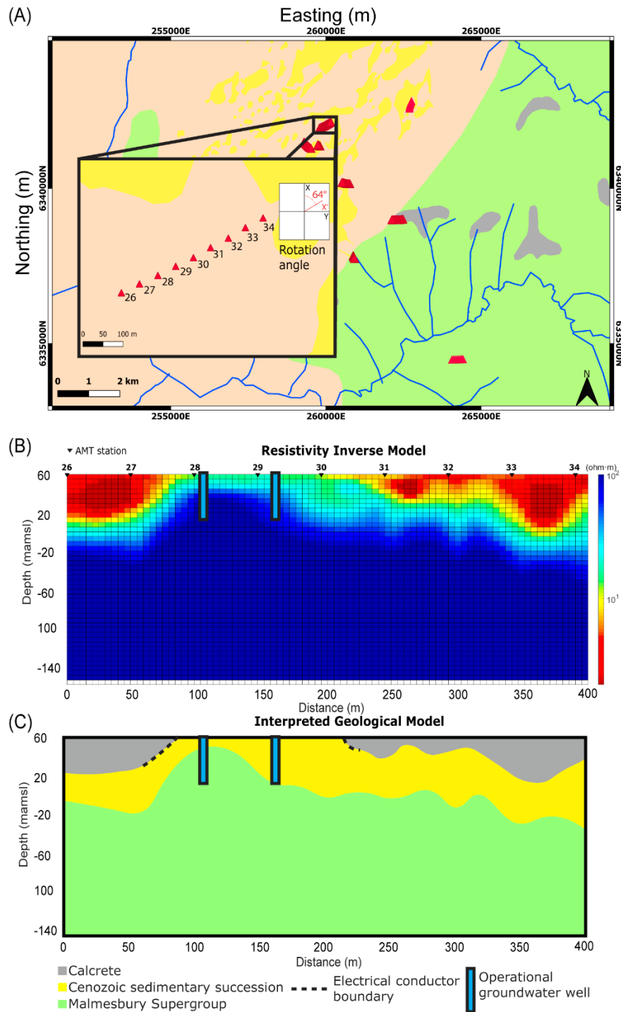
Figure 3.9. (A) The locality map shows the position of 9 AMT stations along survey line L7. This is one of the longest lines of AMT data collected on the farm. The impedance tensor for the stations is rotated by 64° following the strike of the wells. (B) The resistivity inverse model shows the resistor, in this case, is buried by a layer of fine sands (green). Even though the resistor is buried two wells still recharge from the buried resistive area. The root mean square error of the model is 1.6. (C) A geological model interpreted from the resistivity inverse model shows that both wells intersect the break in the conductive aquitard.
