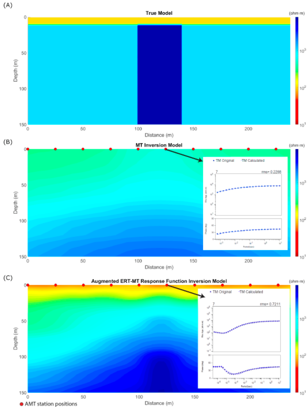
Figure 4.11. (A) The true resistivity model has a conductive ( 100 \Omega \cdot m ) overburden, to a depth of 10 m, and an underlying resistive ( 8000 \Omega \cdot m ) dyke embedded in a 1000 \Omega \cdot m half-space. The model is 238 m in length almost half the size of the previous model tested. (B) Resistivity inverse model only using audio magnetotelluric data. No clear resistor is mapped at 300 m along the profile. Again, the conductive overburden is absent in this inverse model. The inverse model had an RMSE of 0.3. (C) Resistivity inverse model using the augmented ERT-MT response function. A resistor is mapped at 300 m along the profile but is constrained to ~100 m. Also, the conductive overburden is again mapped in this inverse model. The inverse model had an RMSE of 0.3.
