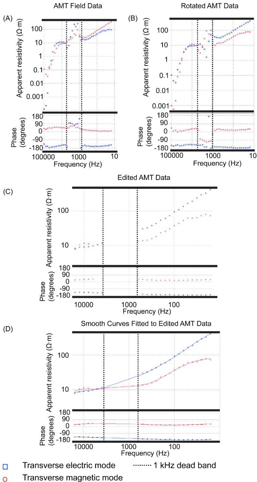
Figure 3.3. (A) Representative quality AMT field data. (B) Rotated AMT data so the X and Y direction is perpendicular and parallel to geological strike respectively. (C) Masked data in the 1 kHz dead band and >31 kHz where signal strength was low. (D) Removed noise spikes and fitted smooth (D+) curves to the remaining data points.
