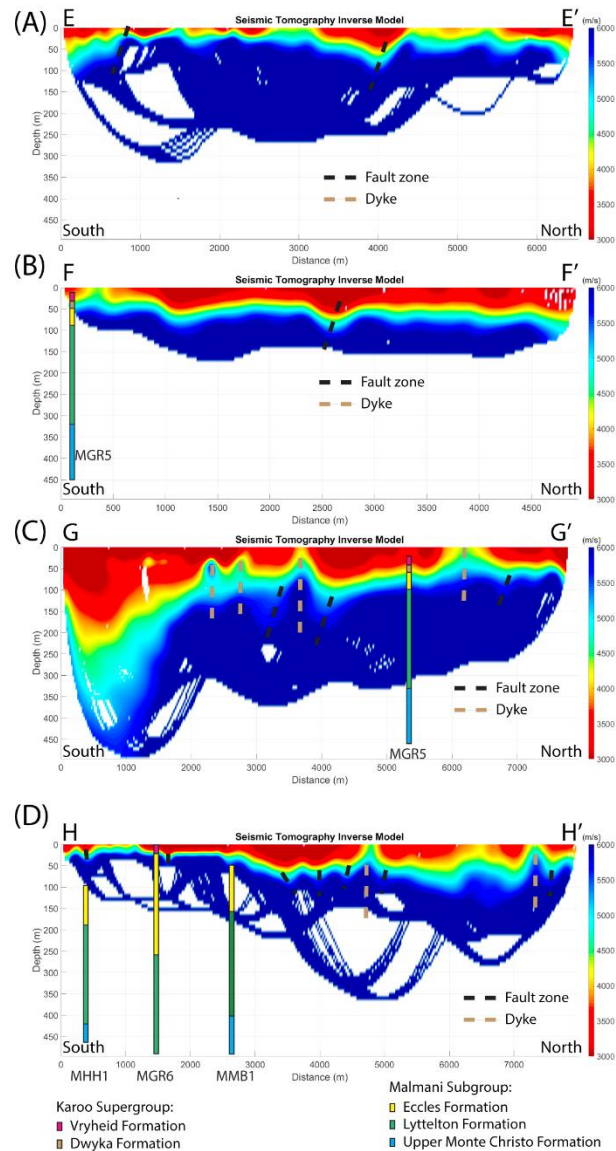
Figure 5.6. (A) P-wave seismic tomography inverse model of seismic line AV 4 with a root mean square error of 5 ms. Two fault zones are mapped in the dolomites. (B) P-wave seismic tomography inverse model of seismic line AV 5 with a root mean square error of 4 ms. Velocities between \sim 3000 - 4500 m/s map the Karoo supergroup and matches the borehole log MGR5. Velocities between \sim 5000 - 6000 m/s (blue) representing the Malmani subgroup also match the borehole log. A fault zone is mapped at \sim 2500 m along the profile. (C) P-wave seismic tomography inverse model of seismic line AV 6 with a root mean square error of 9 ms. Faults and dykes can be seen clearly compartmentalizing the dolomites in the inverse model. (D) P-wave seismic tomography inverse model of seismic line AV 7 with a root mean square error of 7 ms. Velocities between \sim 5000 - 6000 m/s (blue) in the Malmani subgroup correlate with all three boreholes along the survey line. Again, faults and dykes can be seen compartmentalizing the dolomites. Dykes and faults are mapped from underground mapping and subsurface boreholes.
