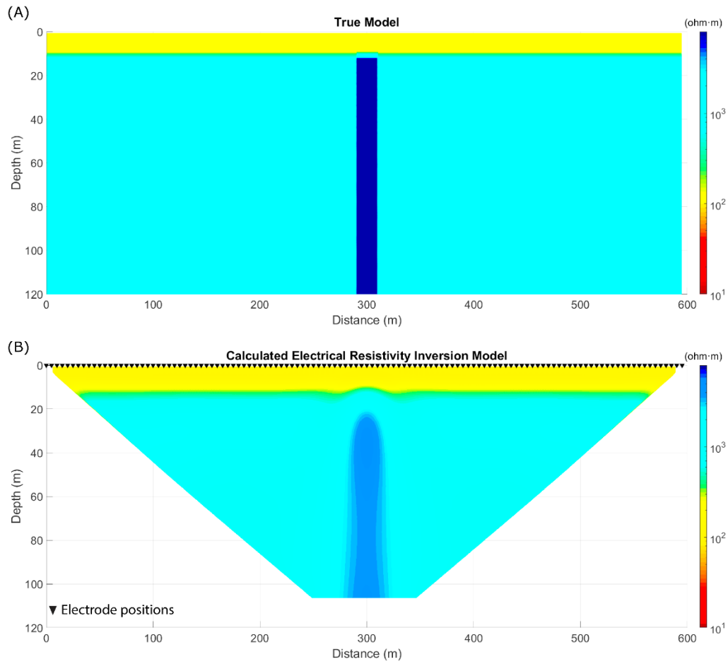
Figure 4.6. (A) True resistivity model with a conductive ( 100 \Omega \cdot m ) overburden, to a depth of 10 m, and an underlying resistive ( 8000 \Omega \cdot m ) dyke embedded in a 1000 \Omega \cdot m half-space. (B) ERT inverse model with an RMSE of 0.36. The ERT inverse model recovers both the conductive overburden and the dyke.
