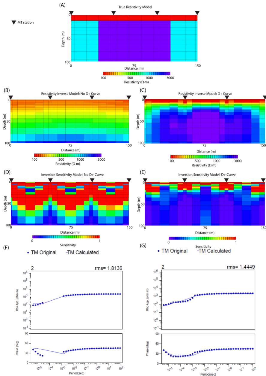
Figure 4.3. (A) True resistivity model. (B) Resistivity inverse model of the augmented ERT-MT response function without the use of smooth D+ curves. (C) Resistivity inverse model of the augmented ERT-MT response function with the use of smooth D+ curves. (D) Inverse model sensitivity map of the augmented ERT-MT response function without the use of smooth D+ curves. Sensitivities are spread throughout the inverse model. (E) Inverse model sensitivity map of the augmented ERT-MT response function with the use of smooth D+ curves. Sensitivities are isolated in the top 10 m where the conductive layer is situated. (F) Augmented ERT-MT response function, without D+ curve data filling the gap, apparent resistivity and phase plots with calculated inverse model apparent resistivity and phase. (G) Augmented ERT-MT response function, with D+ curve data filling the gap, apparent resistivity and phase plots with calculated inverse model apparent resistivity and phase.
