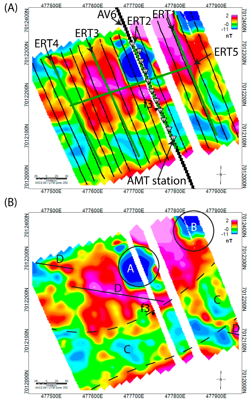
Figure 5.9. (A) Reduced and leveled magnetic map with black dots representing the magnetic readings collected along the survey lines. Black squares show the receiver positions for a portion of the seismic line AV 6. (B) Reduced and leveled magnetic data collected at our research site. Positions A and B show two negative residual magnetic intensity ( \sim -11 nT) zones. Zone C, marked by the black stippled line, offsets the positive residual magnetic intensity lineament marked as D. Position f3 shows the location of the low velocity zone seen along P-wave seismic tomography inverse model for seismic line AV 6.
