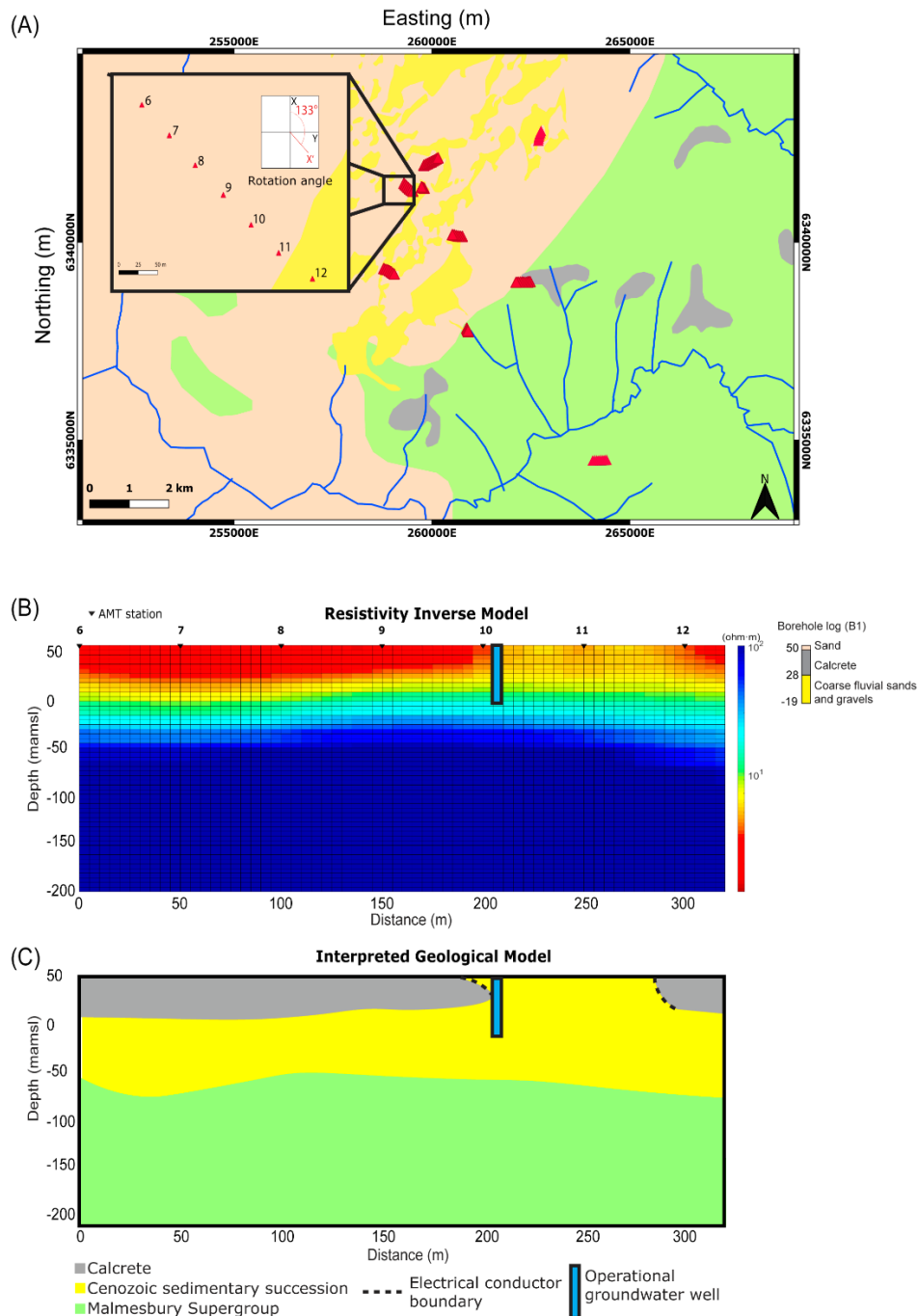
Figure 3.7. (A) This locality map shows the positions of the 7 AMT stations, from L2, used for the resistivity inverse model. The impedance tensor is rotated 133°, which rotates the TM mode perpendicular to the strike of wells and vegetation at this site. (B) The resistivity inverse model again maps the conductive clay and calcrete aquitard at the surface of the model. A resistor breaks the continuity of the aquitard. A well sunk near the edge of the clay and calcrete aquitard intersect slightly more saline groundwater than the well at line L1. The calcrete and clay aquitard mapped by the borehole matches the conductivity layer. The coarse fluvial sands match with the green layer of the resistivity inverse model, which is the target aquifer in the area. The root mean square error of the model is 2.5. (C) A geological model interpreted from the resistivity inverse model.
