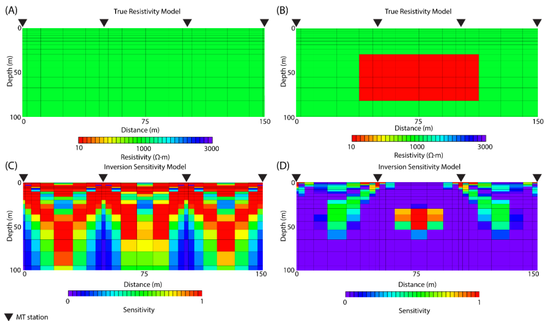
Figure 4.2. (A) True resistivity model of a 1000 \Omega \cdot \text{m} half space. (B) True resistivity model of a 1000 \Omega \cdot \text{m} half space with an embedded 10 \Omega \cdot \text{m} conductor. (C) Sensitivity model for the inverse model calculation from forward modeled MT data of the 1000 \Omega \cdot \text{m} half space, with a frequency range of 10 - 10000000 Hz. Most of the model sensitivity is in a distinctive cone shape distribution throughout the half space. (D) Sensitivity model for the inverse model calculation from forward modeled MT data of the 1000 \Omega \cdot \text{m} half space with the embedded 10 \Omega \cdot \text{m} conductor, with a frequency range of 10 - 10000000 Hz. Most of the model sensitivity is located near the center of the conductor.
