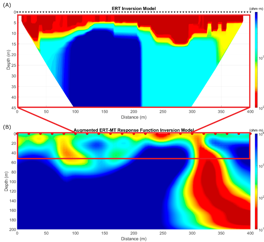
Figure 4.23. (A) East-west ERT inverse model over the audiomagnetotelluric line. (B) Resistivity inverse model using the augmented ERT-MT response function. The resistor at 150 m is mapped in both the ERT and augmented ERT-MT response function inverse model.
