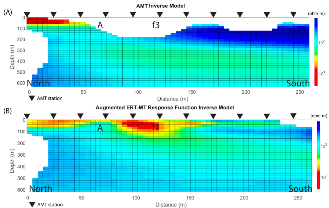
Figure 5.13. (A) Standard AMT resistivity inverse model with a minimum root mean square error of 5. (B) Augmented ERT-MT response function resistivity inverse model with a root mean square error of 2.3. Greater detail is seen in the near surface (< 100 m deep) of the augmented response function resistivity inverse model while retaining the deeper features from the standard AMT resistivity inverse model. f3 marks the location of the low velocity zone in the P-wave seismic tomography inverse model for a portion seismic line AV 6. Position A marks the location of the cavity seen in both the ERT and magnetic susceptibility inverse models. The white cells in these models represent cells with low confidence calculated from the model confidence assessment algorithm.
