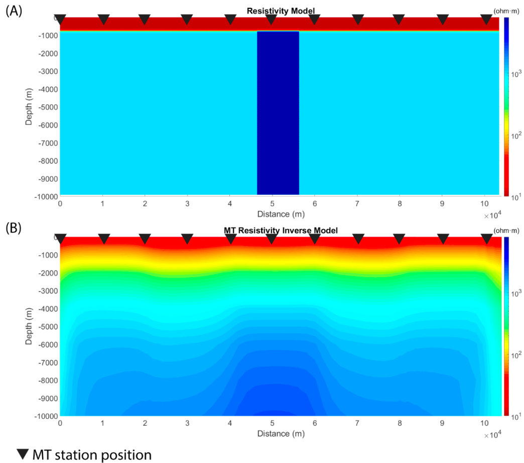
Figure 2.10. (A) True resistivity model with an 800 m thick 10 \Omega \cdot \text{m} conductive overburden above a 1000 \Omega \cdot \text{m} half-space. An 8000 \Omega \cdot \text{m} resistive vertical dyke is embedded within the half space. (B) MT resistivity inverse model shows how the conductive overburden obscures the resistive dyke beneath. The frequency range used is 0.00001 Hz – 100 000 Hz.
