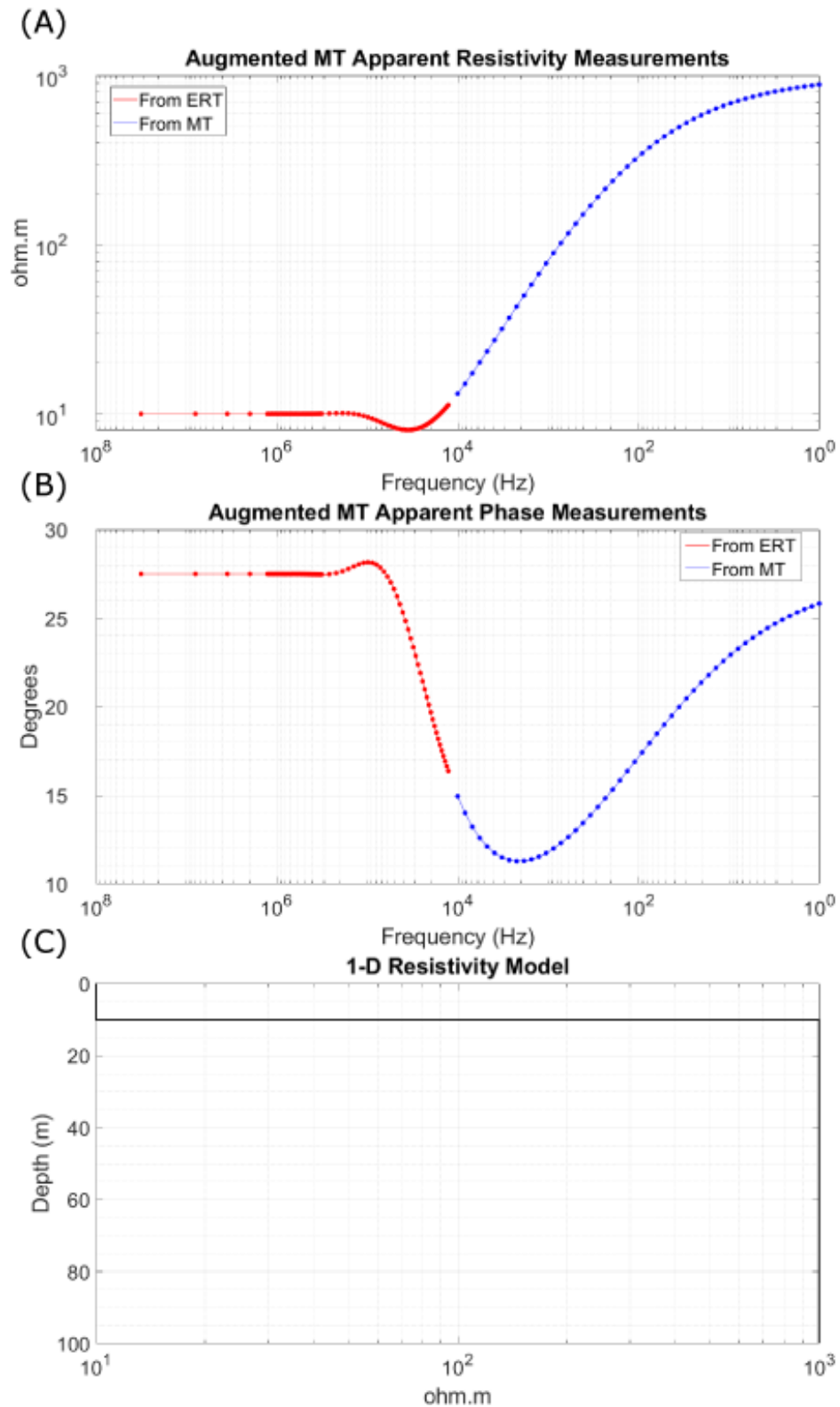
Figure 4.4. (A) Calculated apparent MT resistivity response from ERT (red) and MT (blue) data. (B) Calculated apparent MT phase response from ERT (red) and MT (blue) data. (C) True 1-D resistivity model with a 10 \Omega\cdot\text{m} overburden to a depth of 10 m overlaying a 1000 \Omega\cdot\text{m} half-space.
