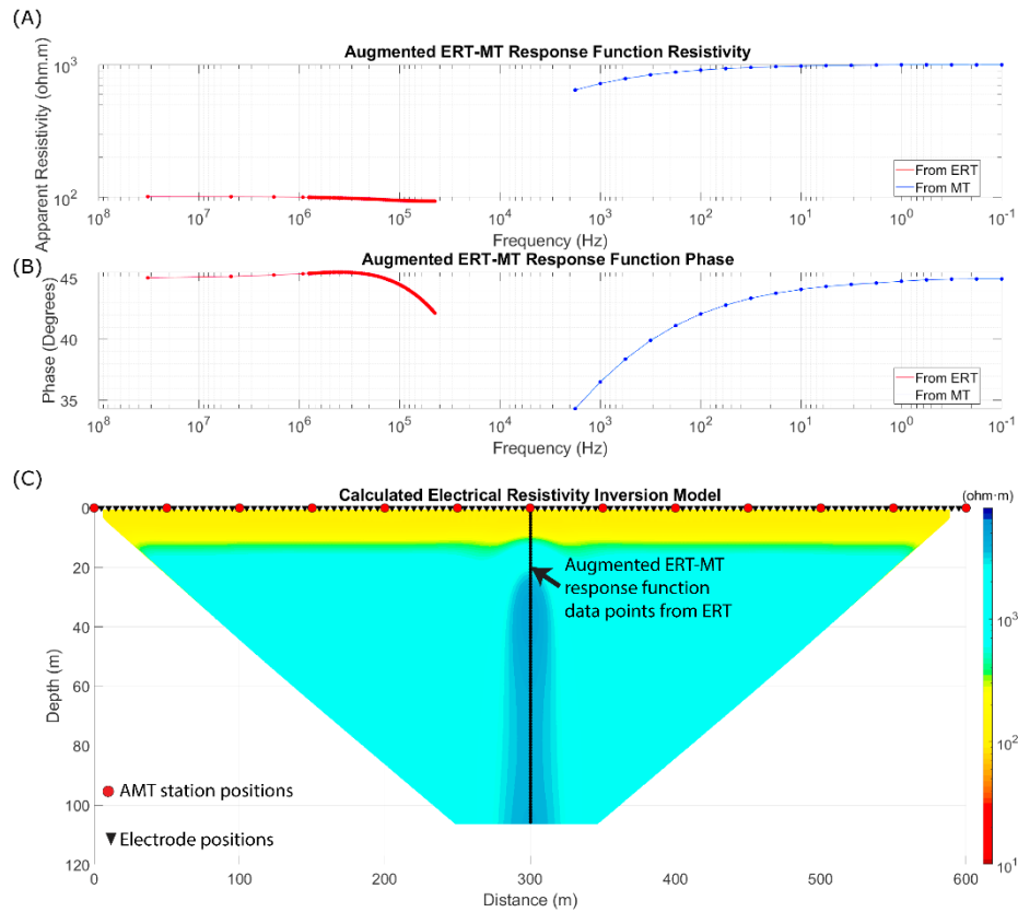
Figure 4.7. (A) Calculated apparent magnetotelluric resistivity response from augmented ERT-MT response function (red) and audio magnetotelluric (blue) data. (B) Calculated apparent magnetotelluric phase response from augmented ERT-MT response function (red) and audio magnetotelluric (blue) data. (C) ERT inverse model used to calculate the augmented ERT-MT response function. The black dots show the location of data points derived from the augmented ERT-MT response function. The gap between \sim 1000 Hz- 100000 Hz is due to the shorter ERT array so the depth penetration is insufficient for frequency overlap.
