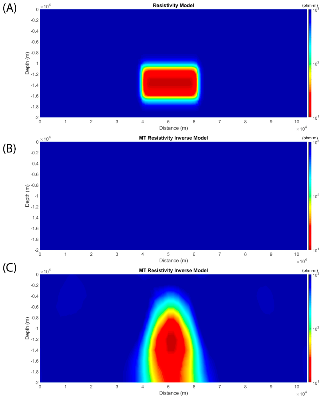
Figure 2.9. (A) True resistivity model, with a 10 \Omega\cdot\text{m} conductor 15 km deep. (B) Resistivity inverse model using AMT data measured between 1-100,000 Hz. The conductor is absent in the resistivity inverse model since the MT data used is too high frequency to measure at the depth of the conductor. (C) A Resistivity inverse model using MT data measured between 0.00001-1 Hz shows the conductor at 15 km deep.
