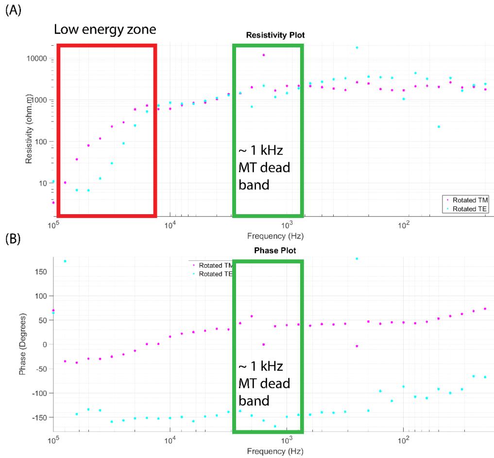
Figure 2.12. (A) Rotated resistivity plot of MT data. (B) Rotated phase plot of MT data. The green block shows the \sim 1 kHz dead band that affects MT data quality and the red block shows low energy levels in the high frequencies.
