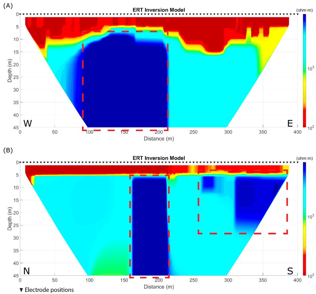
Figure 4.16. (A) East-west ERT 2-D inversion model highlighting the dolerite dyke location with a dashed red box. The resistivity inverse model has a root mean square error of 1.8. (B) North-south ERT 2-D inversion model. The dyke was intersected twice along the ERT line indicated by the two red dashed boxes. The resistivity inverse model has a root mean square error of 1.7.
