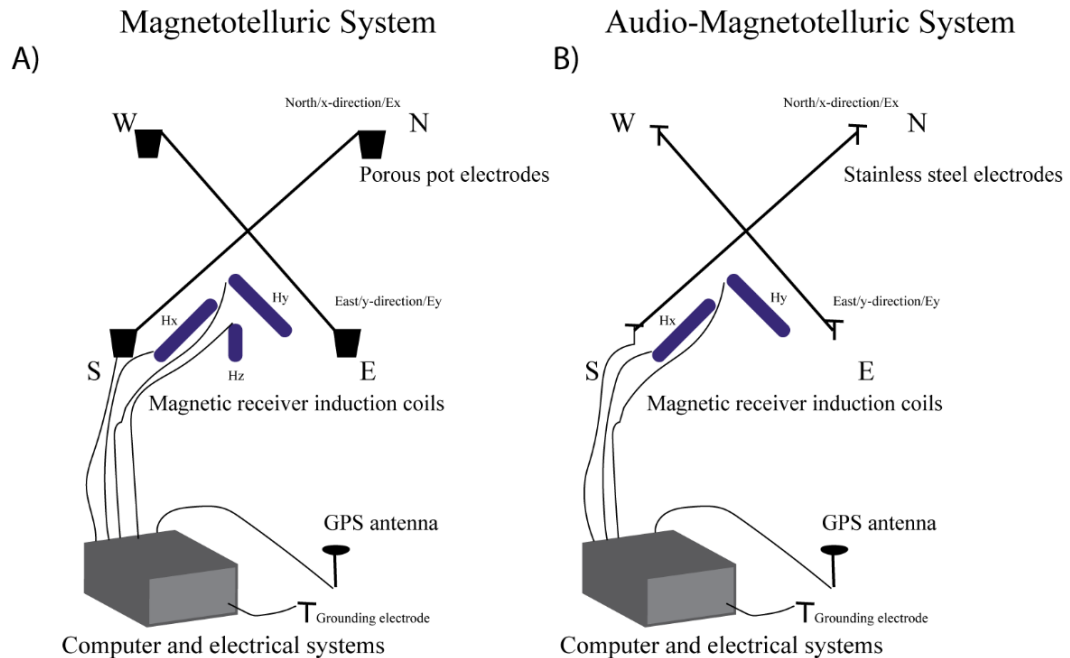
Figure 2.7. (A) A typical MT station setup with two dipoles in the X and Y direction and three induction coils in the X, Y and Z directions. This system will be used for deeper (up to \sim 40 km deep) exploration where the measured electromagnetic signals are < \sim 1 Hz. (B) A typical AMT system also has two dipoles in the X and Y direction but only two magnetic induction coils in the X and Y direction. This system will be used for shallower (up to \sim 2 km deep) exploration where the measured electromagnetic signals are > \sim 1 Hz. The Z direction magnetic induction coil is usually left out in AMT soundings since it is sensitive to high frequency noise in the magnetic field.
