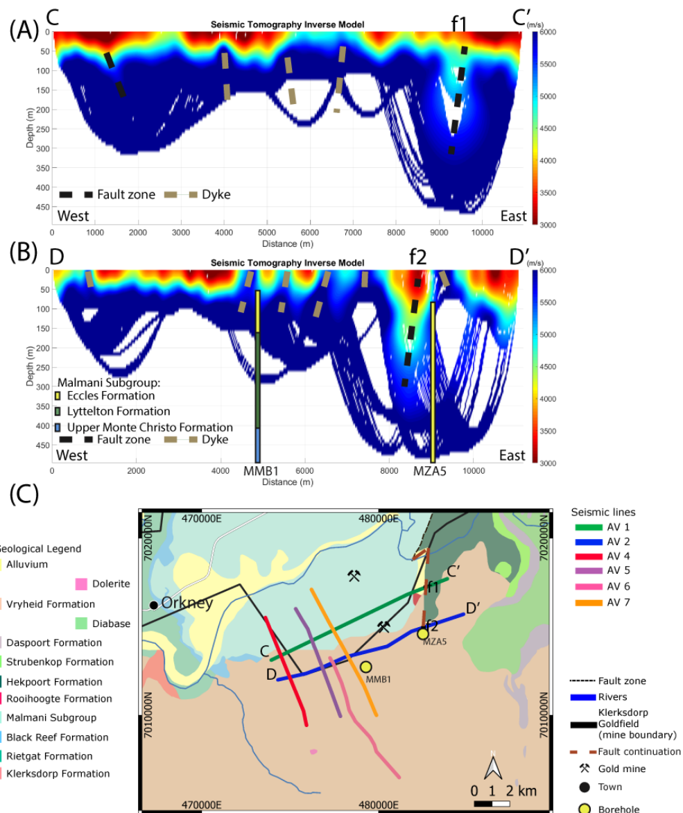
Figure 5.5. (A) P-wave seismic tomography inverse model of seismic line AV 1 with a root mean square error of 6 ms. A fault zone, with low velocities dipping down to a ~350 m depth, shown at position f1 maps the continuation of the fault depicted on the existing geological map of the area. Velocities between ~5000-6000 m/s (blue) represent the Malmani subgroup, and velocities between ~3000-4500 m/s indicate the Vryheid Formation, part of the Karoo supergroup, overlaying the Malmani subgroup, part of the Transvaal Supergroup. Dykes and faults are mapped from underground mapping and subsurface boreholes. (B) P-wave seismic tomography inverse model of seismic line AV 2 with a root mean square error of 7 ms. Position f2 shows the fault zone continuing from AV 1 with a low-velocity zone being traced down to a ~300 m deep. Dykes and faults are mapped from underground mapping and subsurface boreholes. (C) Geological map showing the position of the seismic lines and boreholes being indicated by yellow circles. The continuation of the existing fault zone between position f1 and f2 is indicated with a red line between AV 1 and AV 2.
