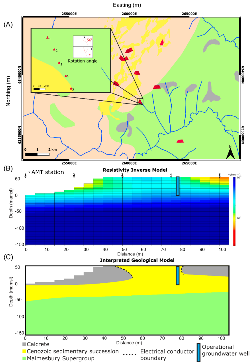
Figure 3.6. (A) A locality map that shows the position of the 5 AMT sites, from L1 represented as red triangles, used for the inverse model. The AMT impedance tensor for these sites is rotated by 156^\circ to lineup the TM and TE modes perpendicular and parallel to the lithological strike respectively. (B) The resistivity inverse model maps a conductive layer between \sim 50 - 20 mamsl deep. This layer is interpreted as the calcrete and clay aquitard present on the farm. A break in the conductor, between 40 m and 80 m along the profile, where a lite blue resistor is preventing the formation of the aquitard in this area. One of the farms' flagship freshwater wells is sunk in the area of the break in the conductor. Between 50-0 mamsl and 0-40 m along the profile, white cells show a region of low confidence calculated by the model confidence assessment algorithm. The root mean square error of the model is 2.9. (C) A geological model interpreted from the resistivity inverse model.
