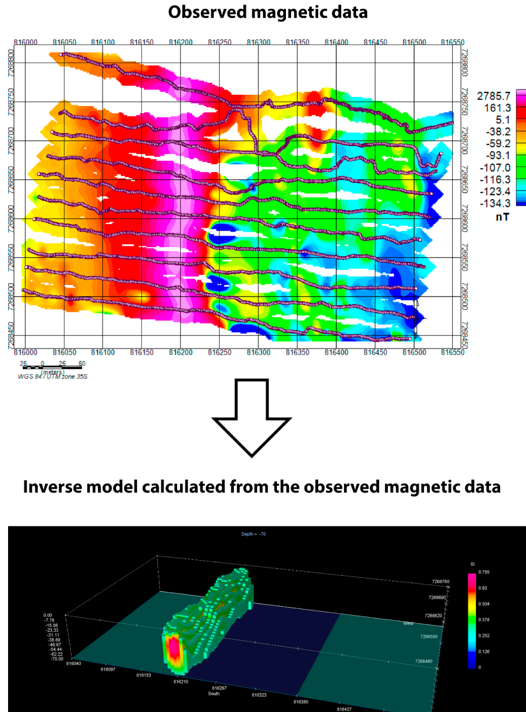
Figure 2.19. Magnetic data collected in the field is used to calculate a magnetic susceptibility 3-D inverse model. White dots represent magnetic data points. The magnetic susceptibility 3-D inverse model shows the isovolume of the dyke that we are interested in.
