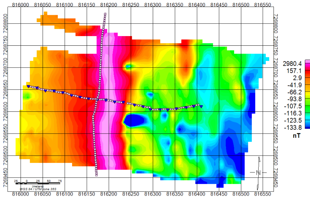
Figure 4.15. Total magnetic intensity map of the study area. White squares represent ERT electrode positions. Blue triangles show AMT station positions. The east-west survey lines run perpendicular to the strike of the target dyke in our study area.
