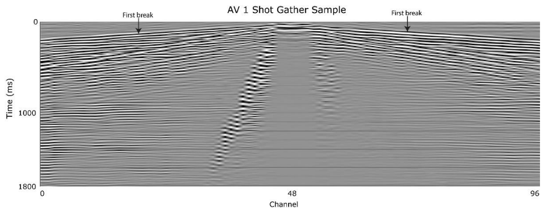
Figure 5.3 Shot gather taken from seismic line AV 1 showing the location of picked first breaks.
