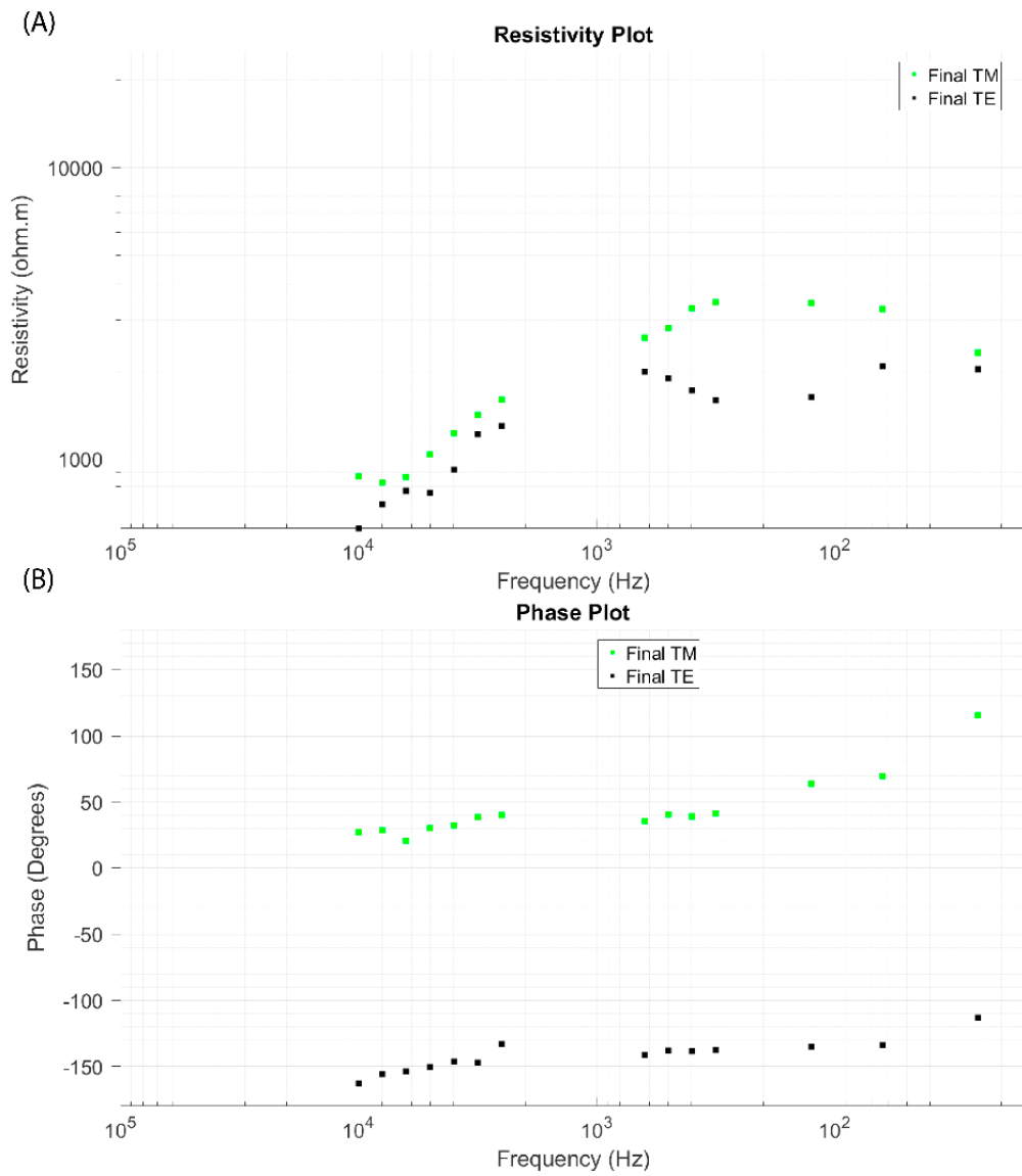
Figure 2.13. (A) Rotated and edited resistivity plot of MT data. (B) Rotated and edited phase plot of MT data.
