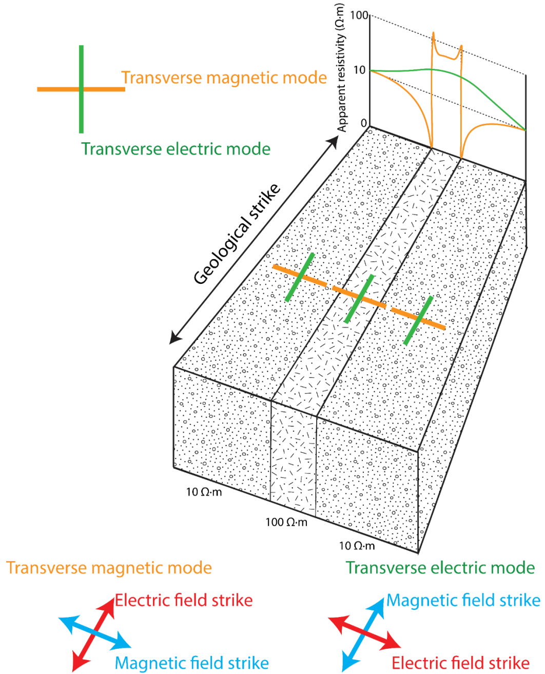
Figure 2.3. Sketch showing the strike of the electric and magnetic field for both the transverse magnetic and electric modes in a heterogeneous half space. The transverse magnetic mode is perpendicular to geological strike while the transverse electric mode is parallel to geological strike.
