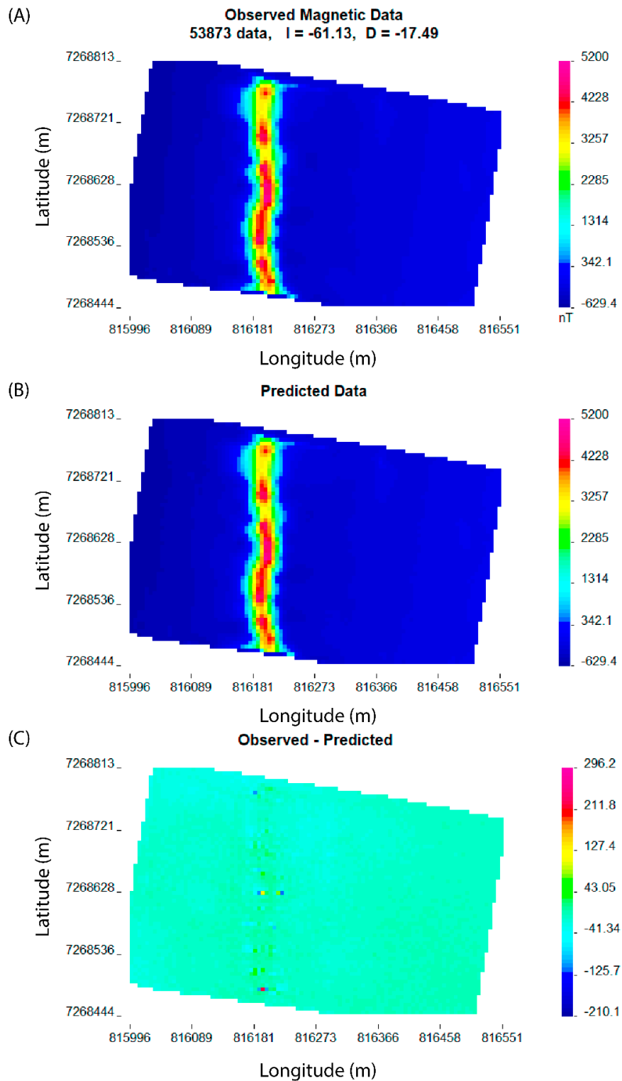
Figure 4.13. (A) The observed magnetic data collected over our research site. (B) Predicted magnetic data calculated from the inversion algorithm. (C) The misfit map is created by subtracting the predicted data from the observed data and the resulting difference is mapped as a misfit value on the map.
