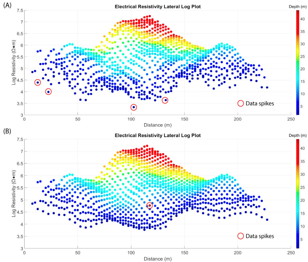
Figure 2.18. (A) Electrical resistivity tomography raw data plot. (B) Electrical resistivity tomography smoothed and spiked removed data.
