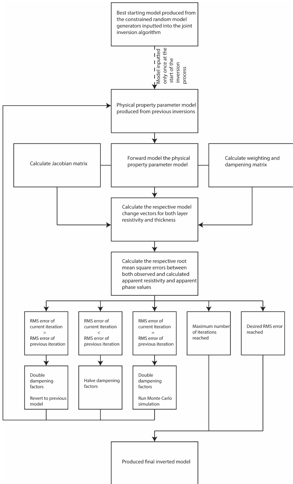
Figure 2.22. Algorithm workflow map for the least squares inversion.
