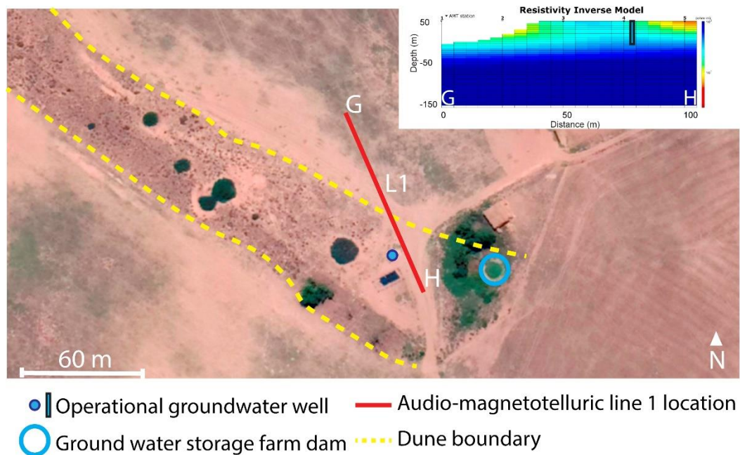
Figure 3.14. Outcropping paleochannel outlined on the satellite image. There is a clear contrast between the coarse orange color ancient dune sediments and the fine grain grey color sediments overlying the calcrete and clay aquitard. The operational well is recharged by the ancient dune outcrop and is used to replenish a farm dam just east of the well.
