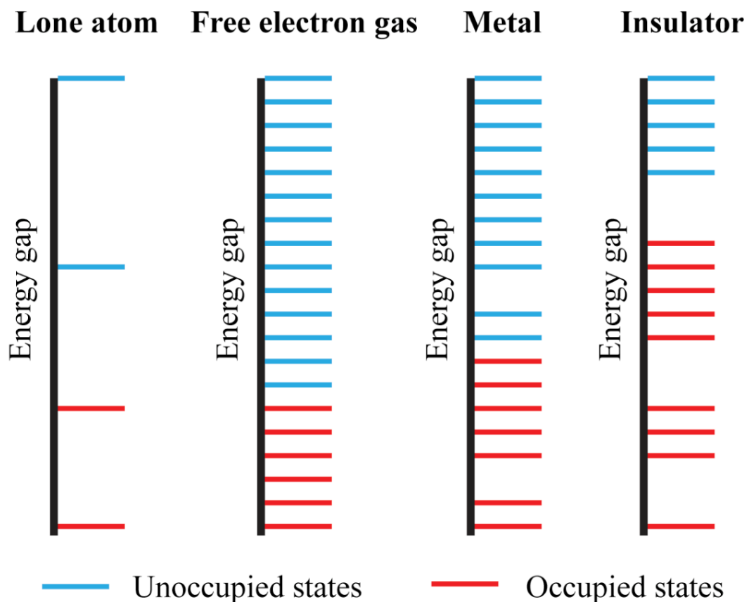
Figure 2.1 Electron energy spectra at absolute zero for different systems.
