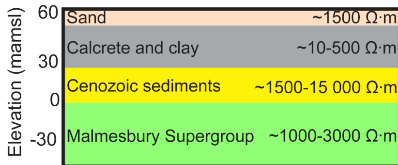
Figure 3.2. Geological map of Waterboerskraal. Audio magnetotelluric stations are indicated as red triangles. Ten audio magnetotelluric traverses were collected in total around the farm. A simplified geological cross-section based on borehole (green dots) data, of the study area, is shown with expected electrical resistivity values, taken from the South African Council for Geoscience publicly available physical property database (Mare, 1999). The yellow Sandveld group was mapped using satellite images, where the color and texture of sediments seen at dune plumes in the surrounding area matched the color and texture in our research site.
