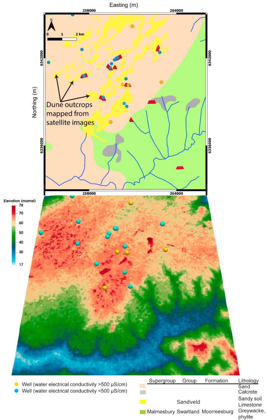
Figure 3.13. A shuttle radar topography mission elevation map of the geological map shows that operational (groundwater conductivity <500 \mu\text{S}/\text{cm} ) have an average elevation range of ~50-58 mamsl, while non-operational wells (groundwater conductivity >500 \mu\text{S}/\text{cm} ) have an average elevation range of ~65-78 mamsl. This is likely due to the faster rate of weathering in the preserved dunes when compared to the calcrete aquitard. Most of the operational groundwater wells are situated on or near the yellow ancient dune outcrops mapped by satellite images on the geological map.
