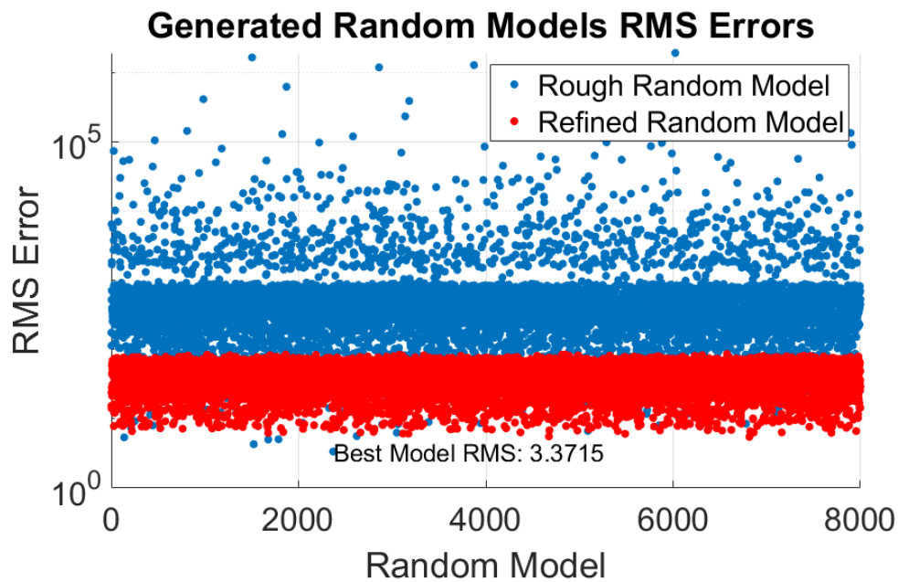
Figure 2.20. A plot shows the root mean square (RMS) error for models calculated using the Monte Carlo simulation.
