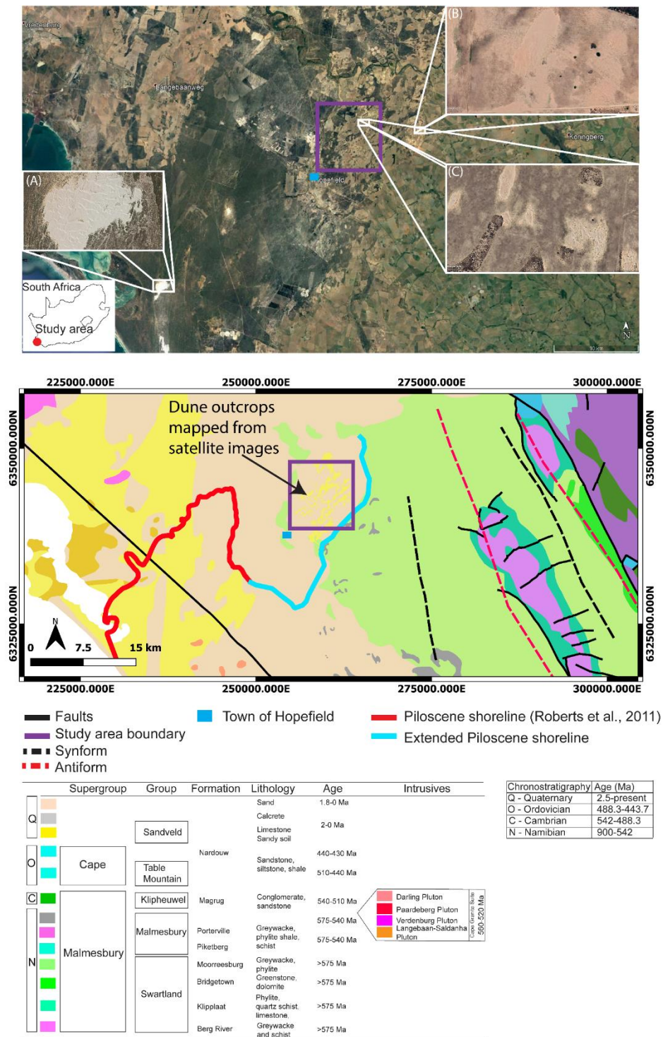
Figure 3.16. The red line marks the previously mapped Pliocene shoreline from Roberts et al. (2011). We make use of the satellite imagery and geophysical mapping to extend (blue line) the Pliocene shoreline further north-east. (A) Shows the location of the Yzerfontein–Geelbek dune cordon. (B) Orange colored matured dunes stabilized by vegetation in our study area. (C) Shows matured dunes furthest east from the present-day shoreline, marking the boundary of the Pliocene shoreline.
