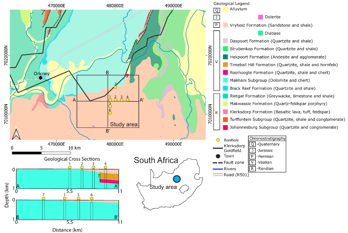
Figure 5.1. Geological map (modified from the following maps sheets, Wilkinson, K.J., and Coetsee, F., 1986; Retief, P.F., 2000) of surrounding the study area at the edge of the Klerksdorp Goldfield situated on the Witwatersrand Basin.
