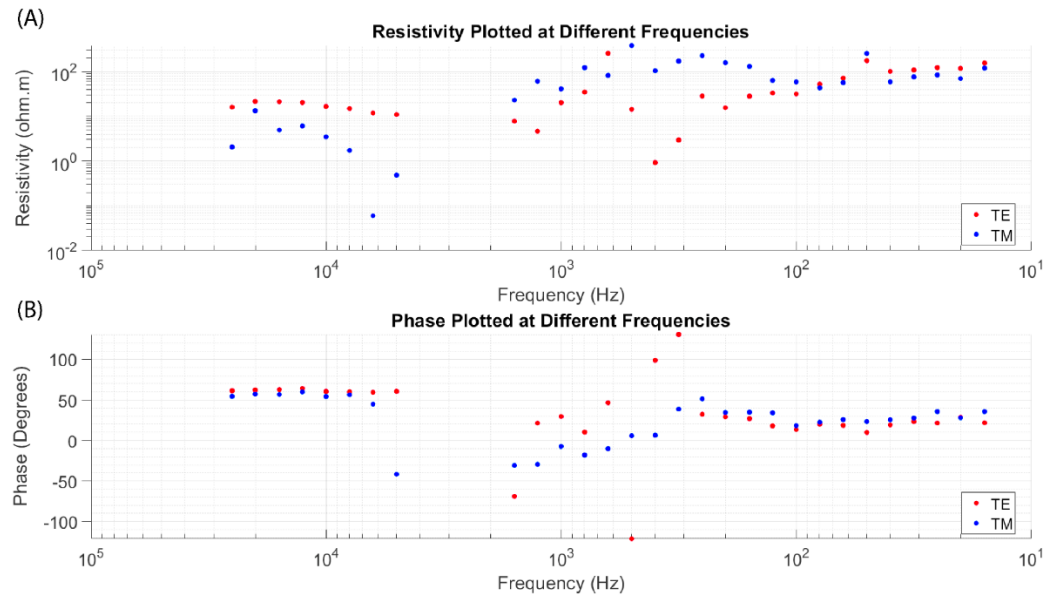
Figure 5.12. (A) TE and TM resistivity values collected from AMT station AMT1. (B) TE and TM phase values collected from AMT station AMT1. The TE mode is more susceptible to noise saturation since the TE mode strikes parallel with the surrounding powerlines in the study area.
