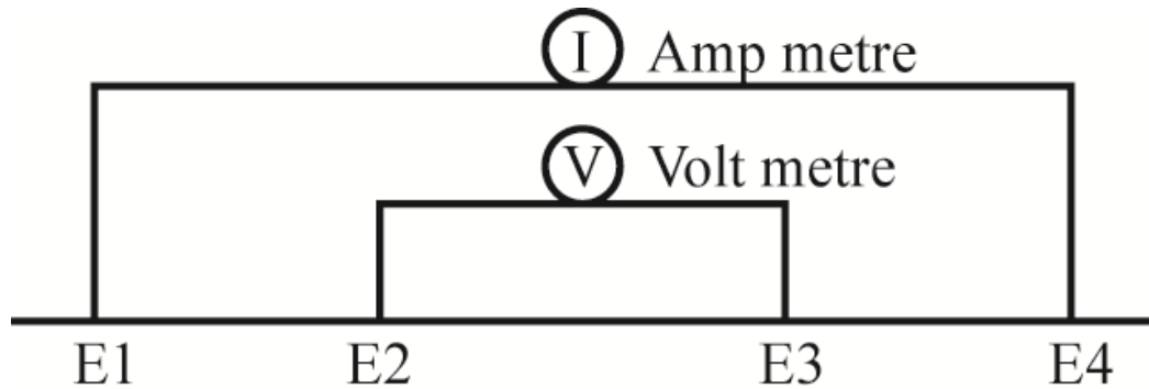
Figure 2.14: Four-point electrode configuration sketch, where E represents electrodes.
