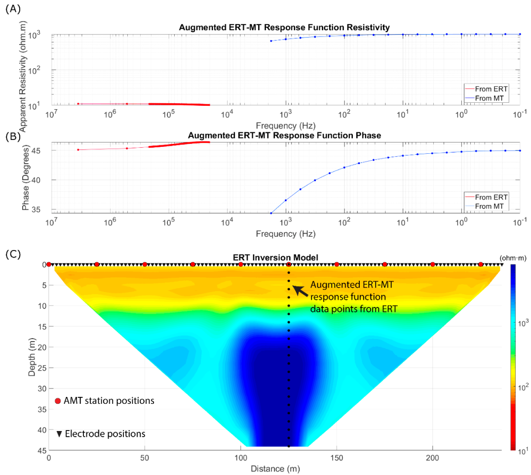
Figure 4.10. (A) Calculated apparent magnetotelluric resistivity response from ERT (red) and audio magnetotelluric (blue) data. Calculated phase response from ERT (red) and MT (blue) data. (C) ERT inverse model used to calculate the augmented ERT-MT response function. The black dots show the location of data points derived from the augmented ERT-MT response function. The gap between \sim 1000 Hz- 100000 Hz is due to the shorter ERT array so the depth penetration is insufficient for frequency overlap
