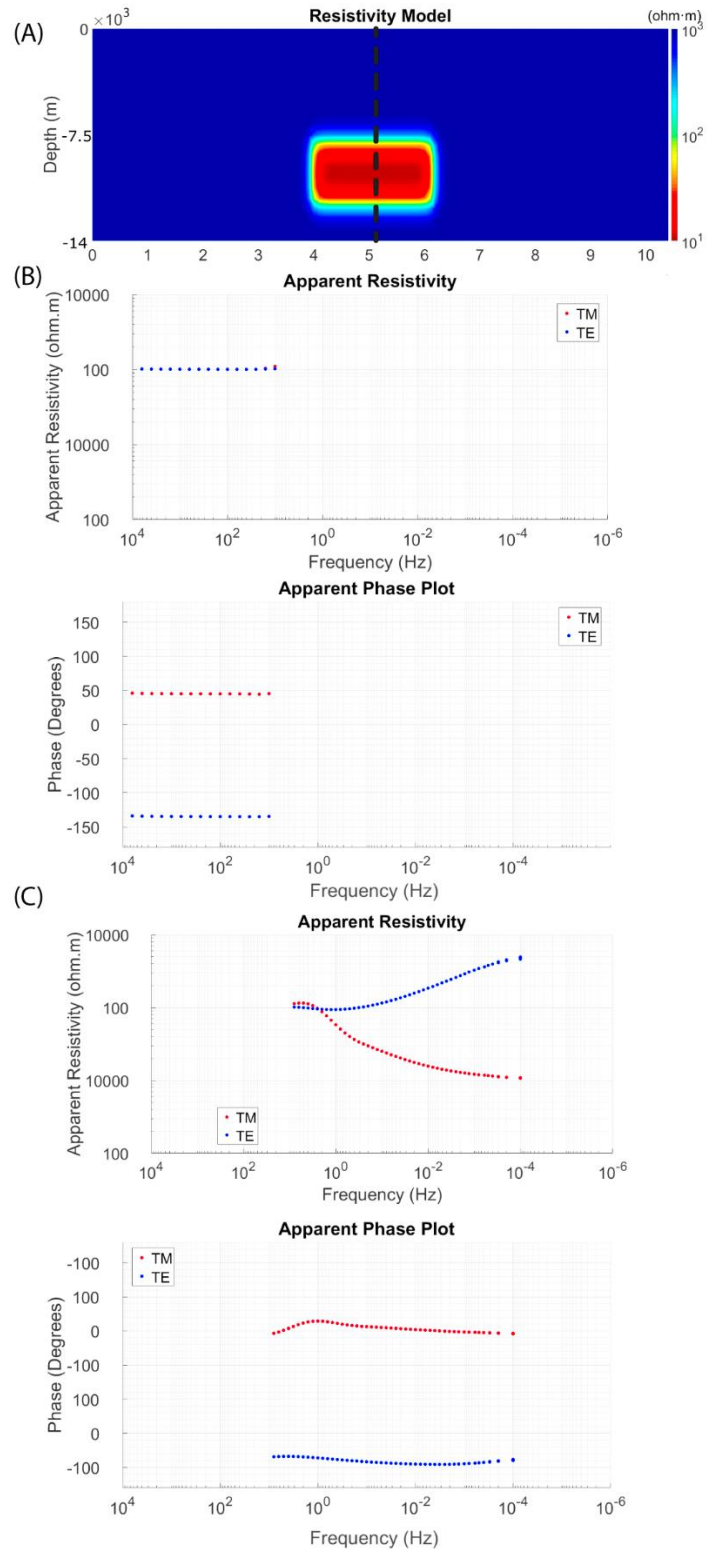
Figure 2.8. (A) Resistivity model with a 10 \Omega\cdot\text{m} conductor 7.5 km deep. (B) Resistivity and phase measurements between 10-10000 Hz. Data is 1-D in nature
