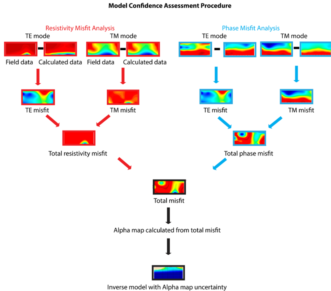
Figure 3.4. This schematic map illustrates the procedure followed by the model confidence assessment algorithm. The misfit for both the resistivity and phase data, for both the TE and TM mode, are calculated. The misfit for the resistivity and phase data is summed and normalized to create a total misfit map for the inverse model. The total misfit model is transformed into an alpha map that controls the translucency of cells within the inverse model. Transparent cells indicate regions of low confidence.
